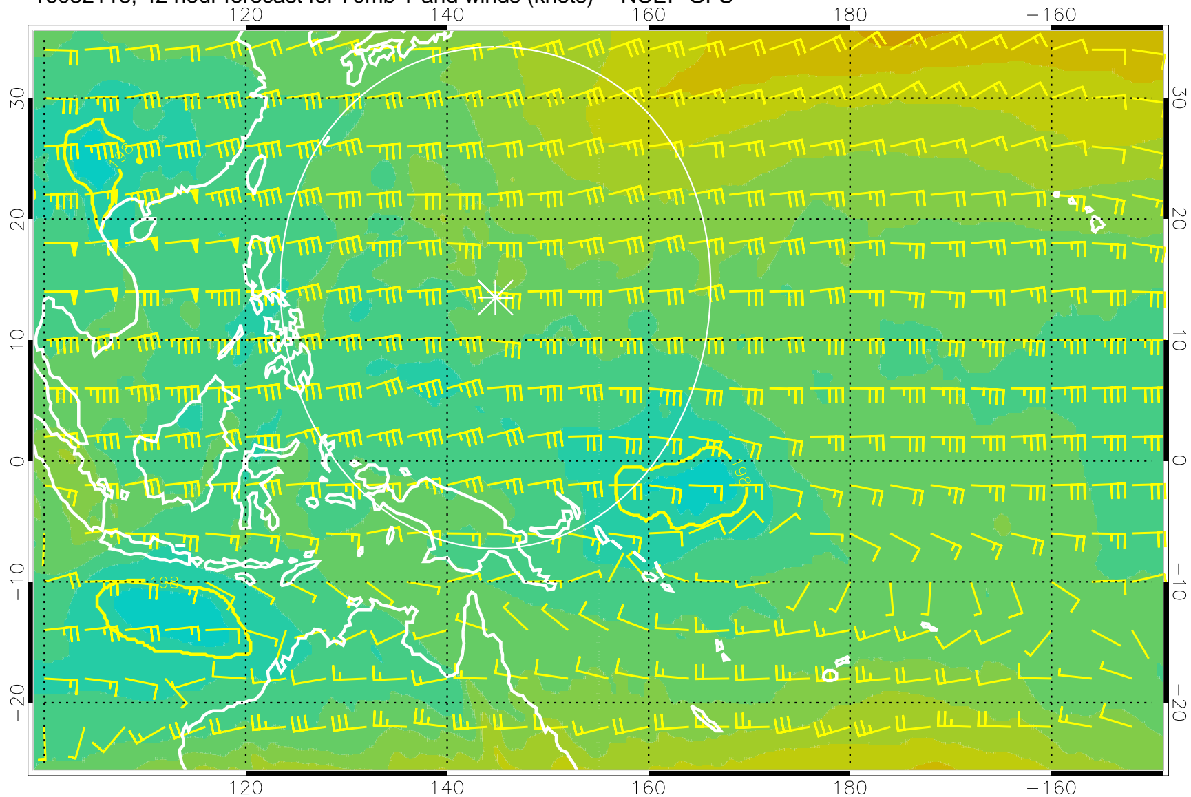
16082118, 42 hour forecast for 70mb T and winds (knots) -- NCEP GFS
