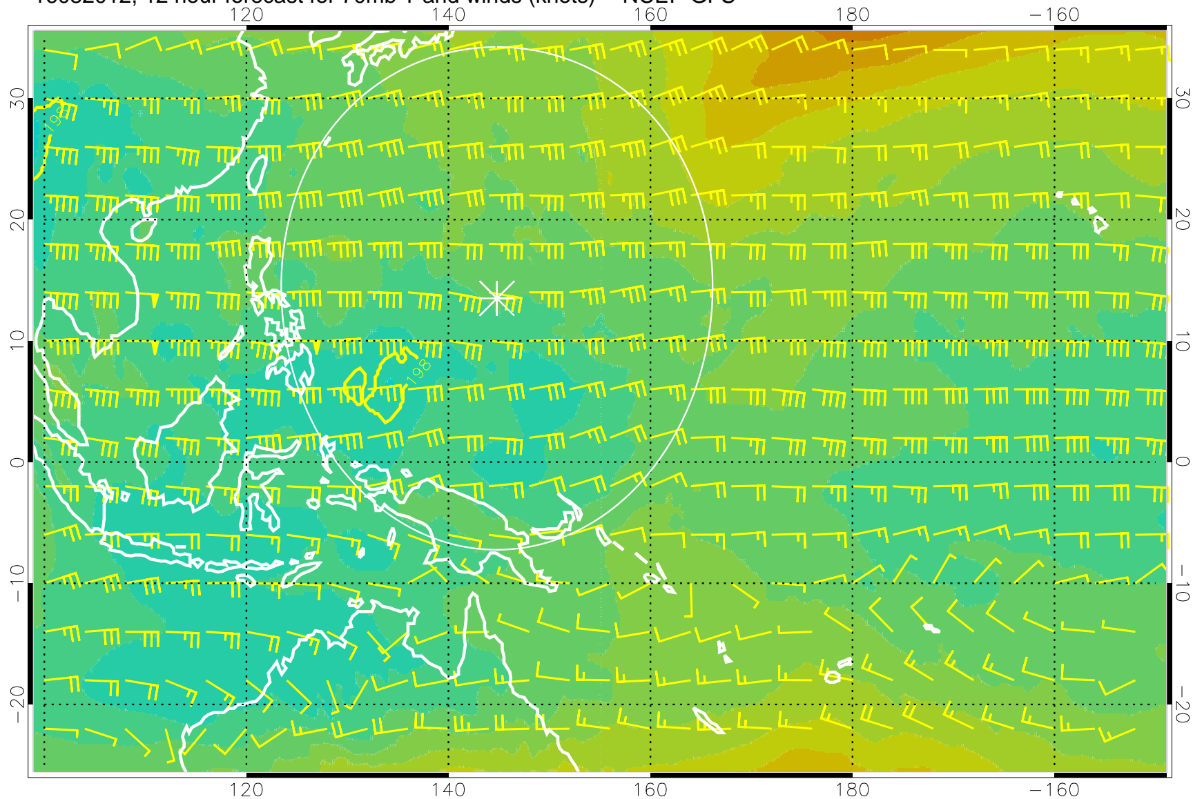
16082012, 12 hour forecast for 70mb T and winds (knots) -- NCEP GFS
