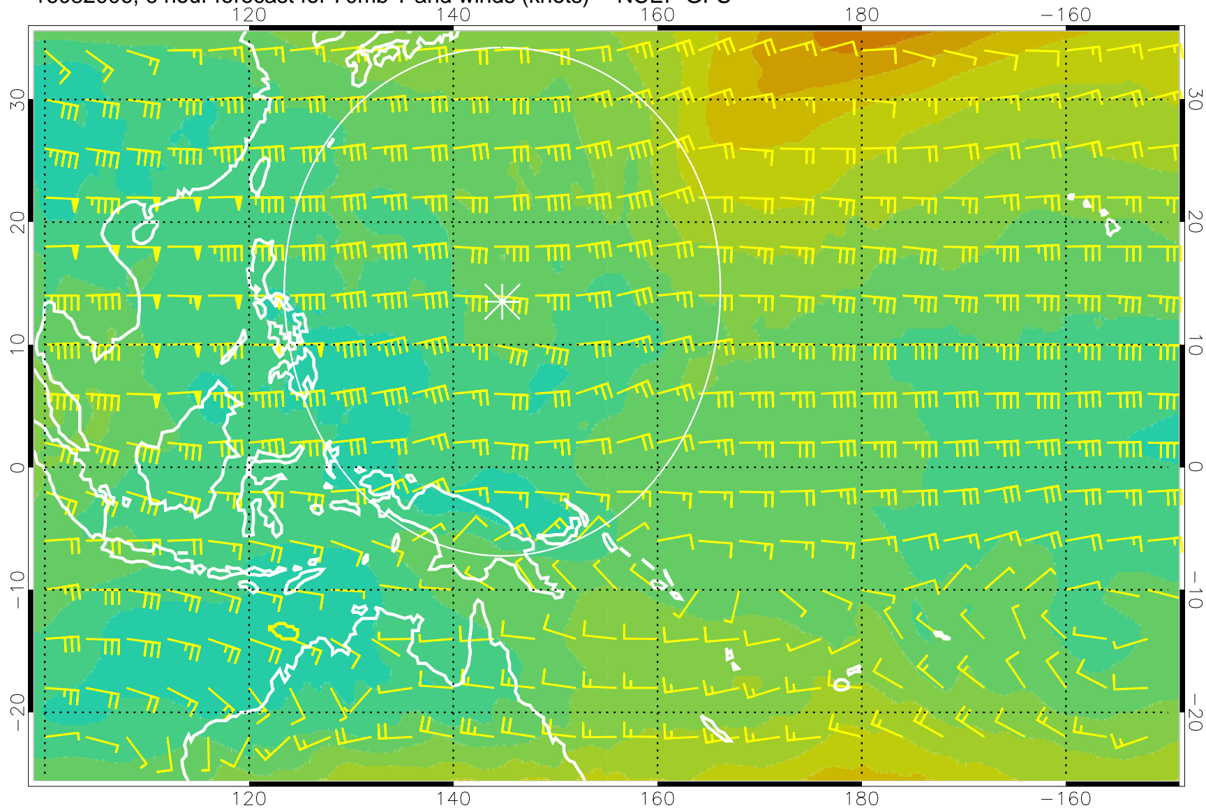
16082006, 6 hour forecast for 70mb T and winds (knots) -- NCEP GFS
