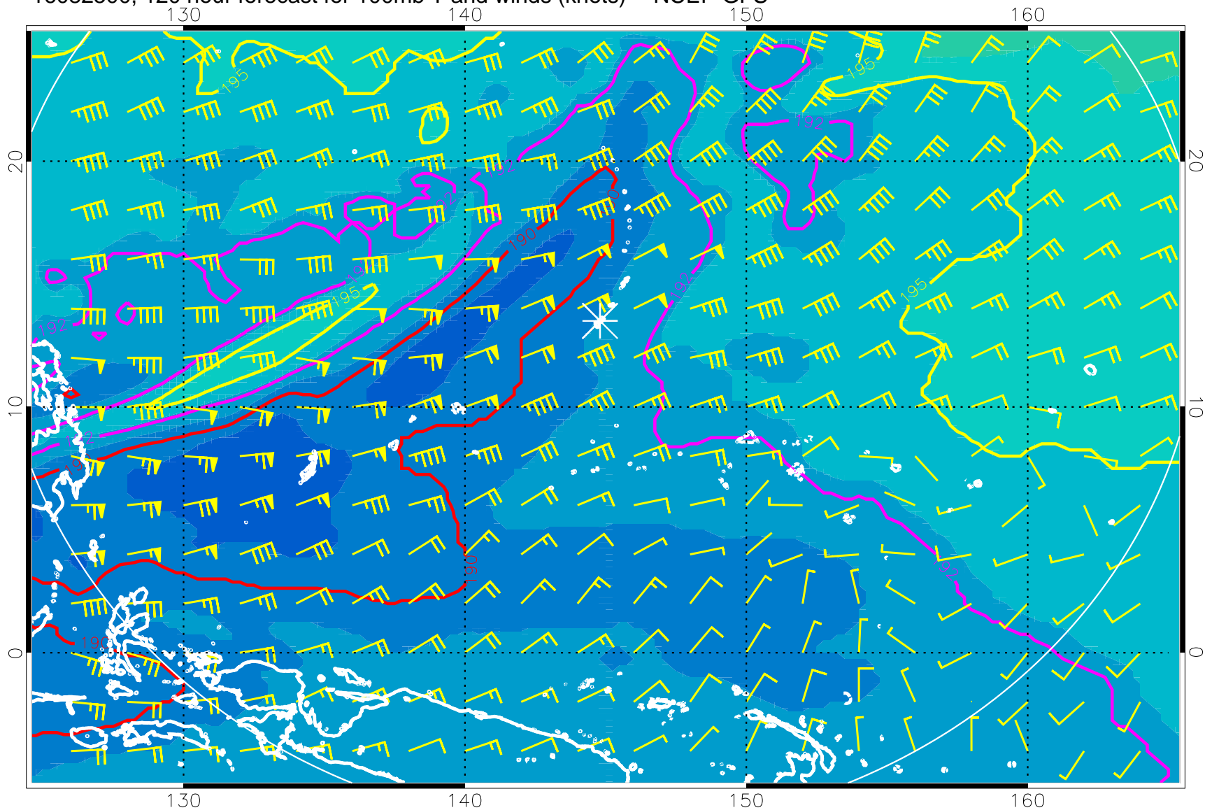
16082500, 120 hour forecast for 100mb T and winds (knots) -- NCEP GFS
