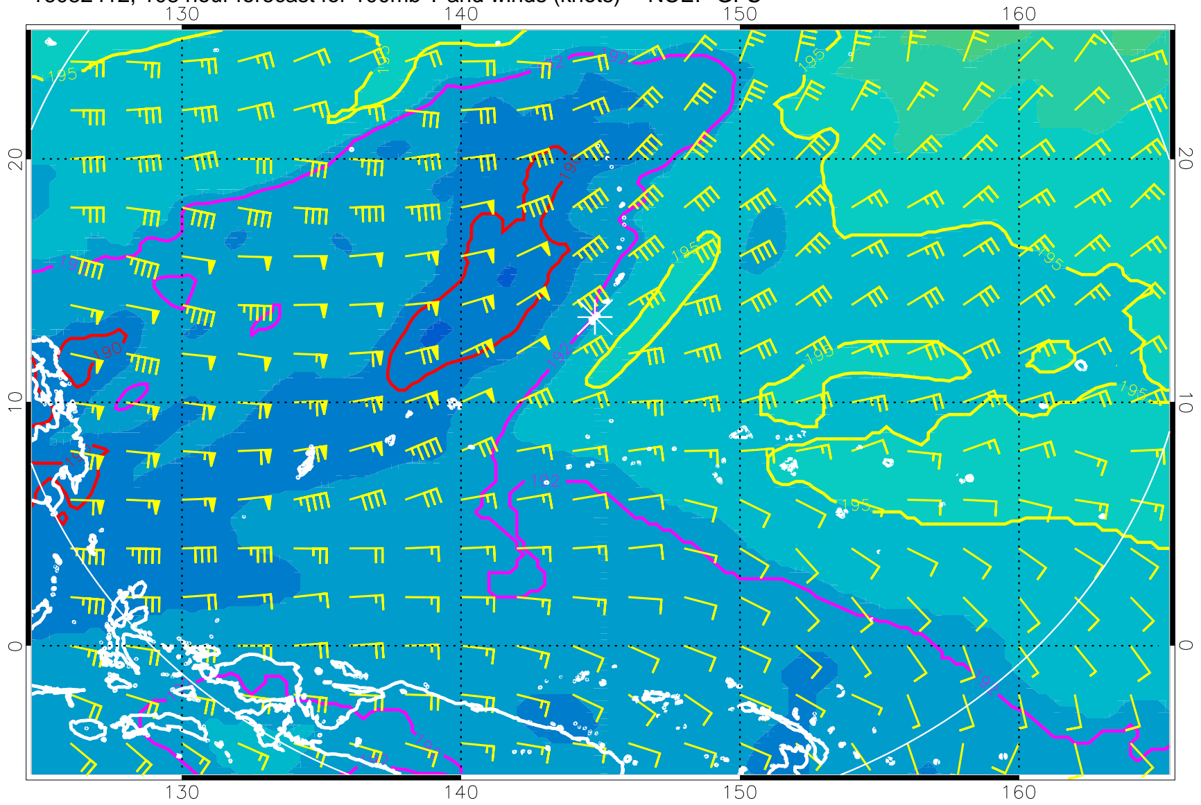
16082412, 108 hour forecast for 100mb T and winds (knots) -- NCEP GFS
