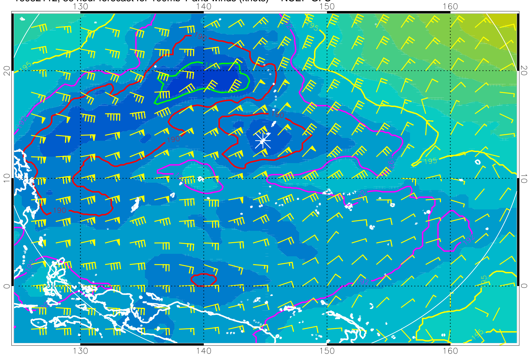
16082112, 36 hour forecast for 100mb T and winds (knots) -- NCEP GFS
