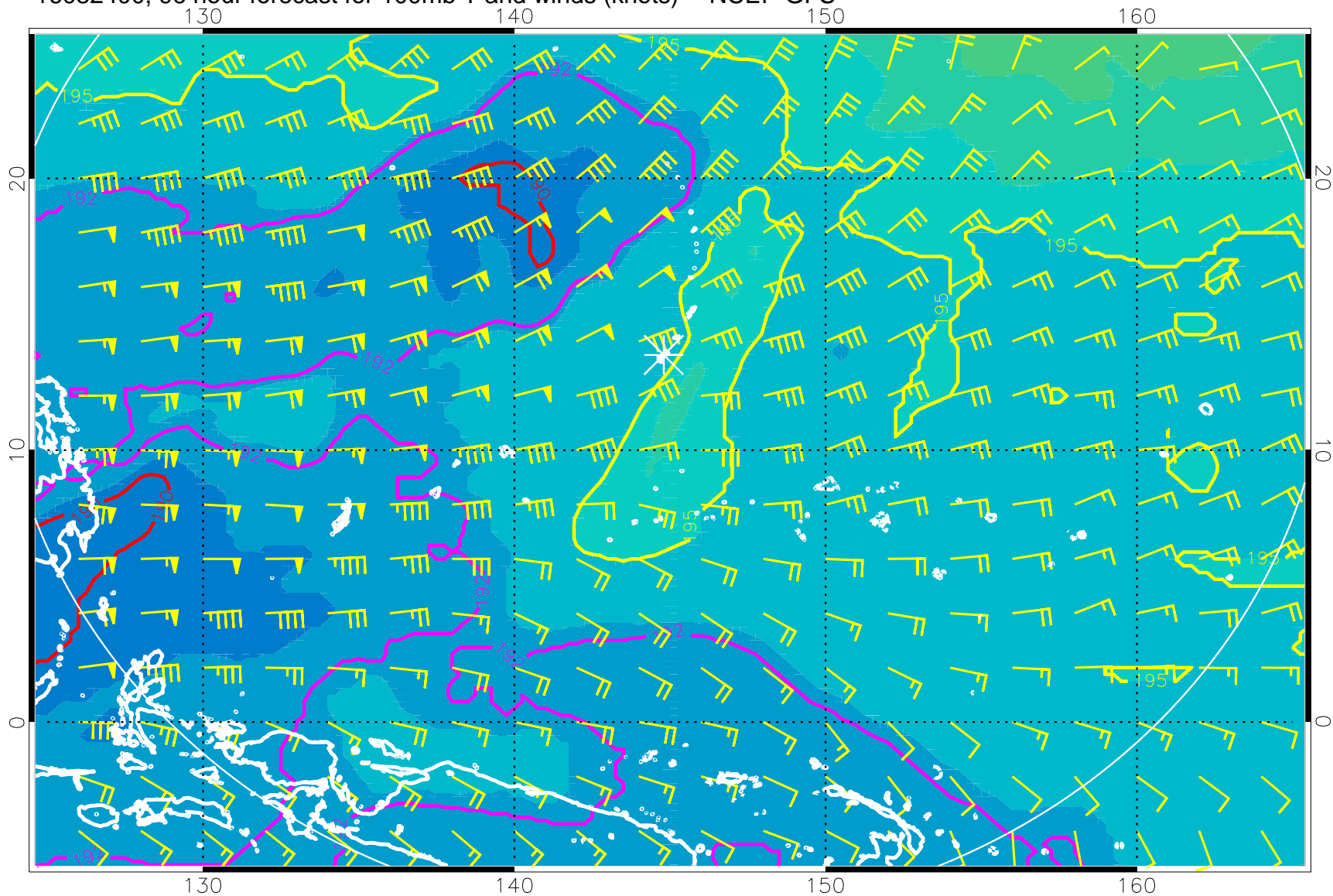
16082400, 96 hour forecast for 100mb T and winds (knots) -- NCEP GFS
