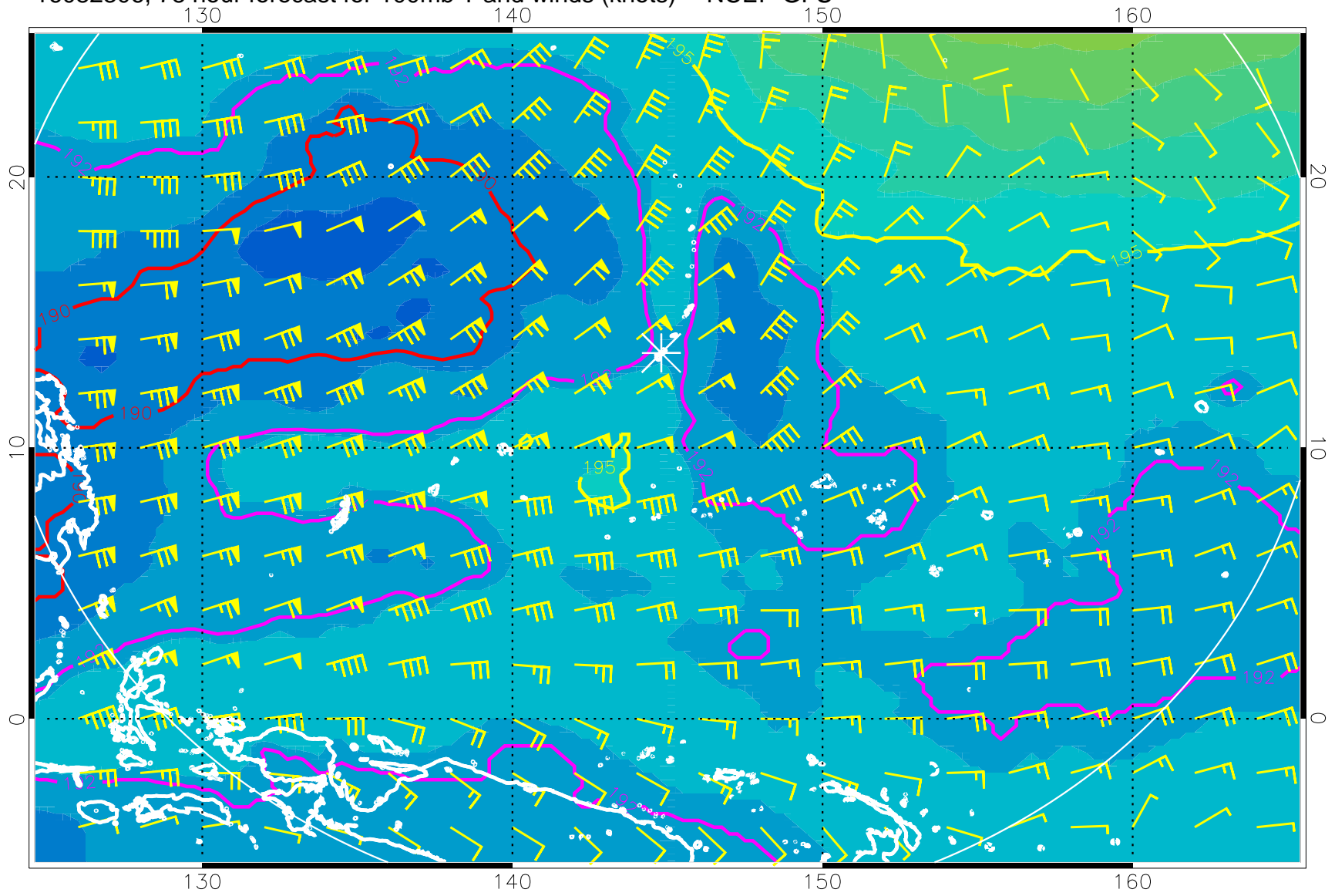
16082306, 78 hour forecast for 100mb T and winds (knots) -- NCEP GFS
