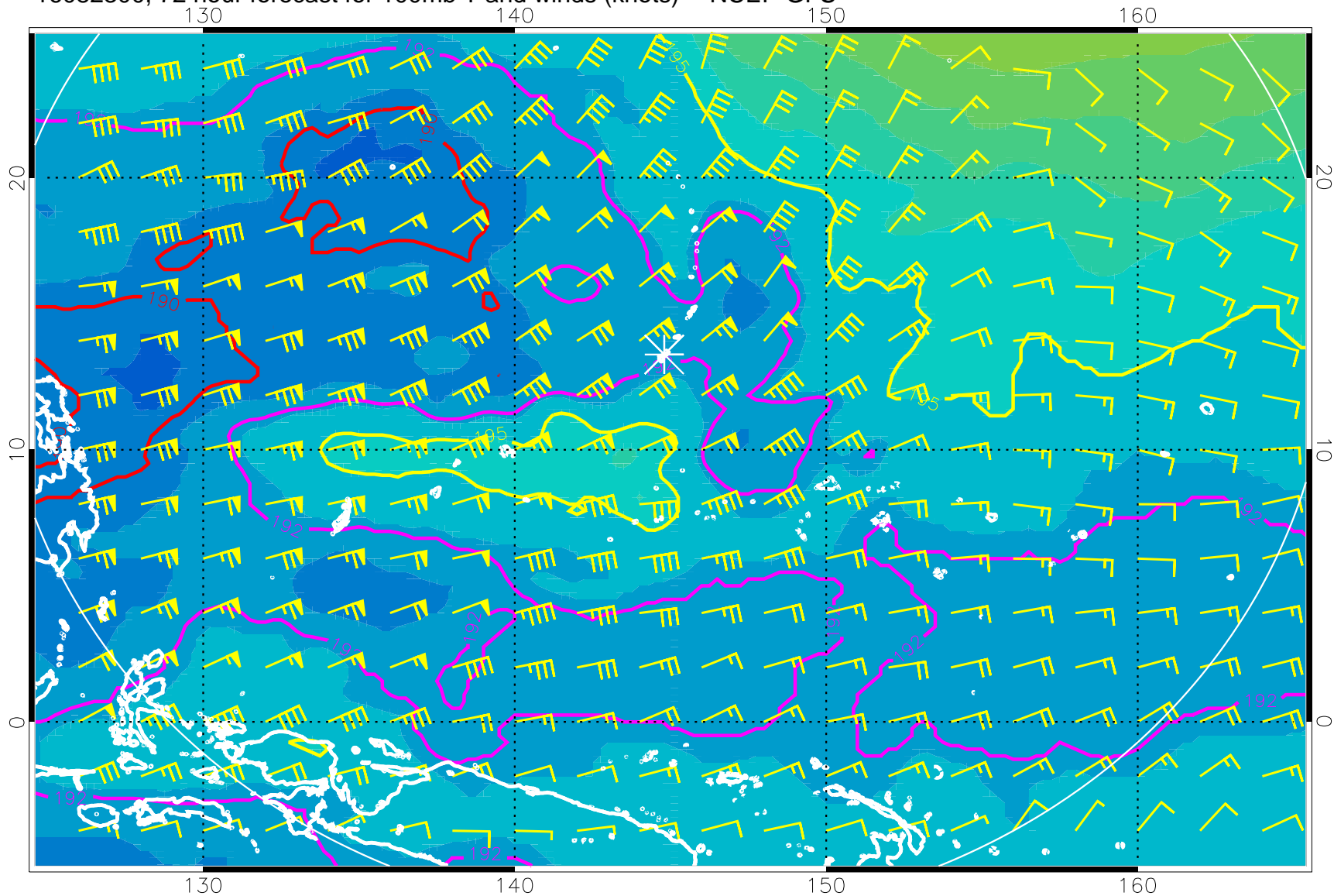
16082300, 72 hour forecast for 100mb T and winds (knots) -- NCEP GFS
