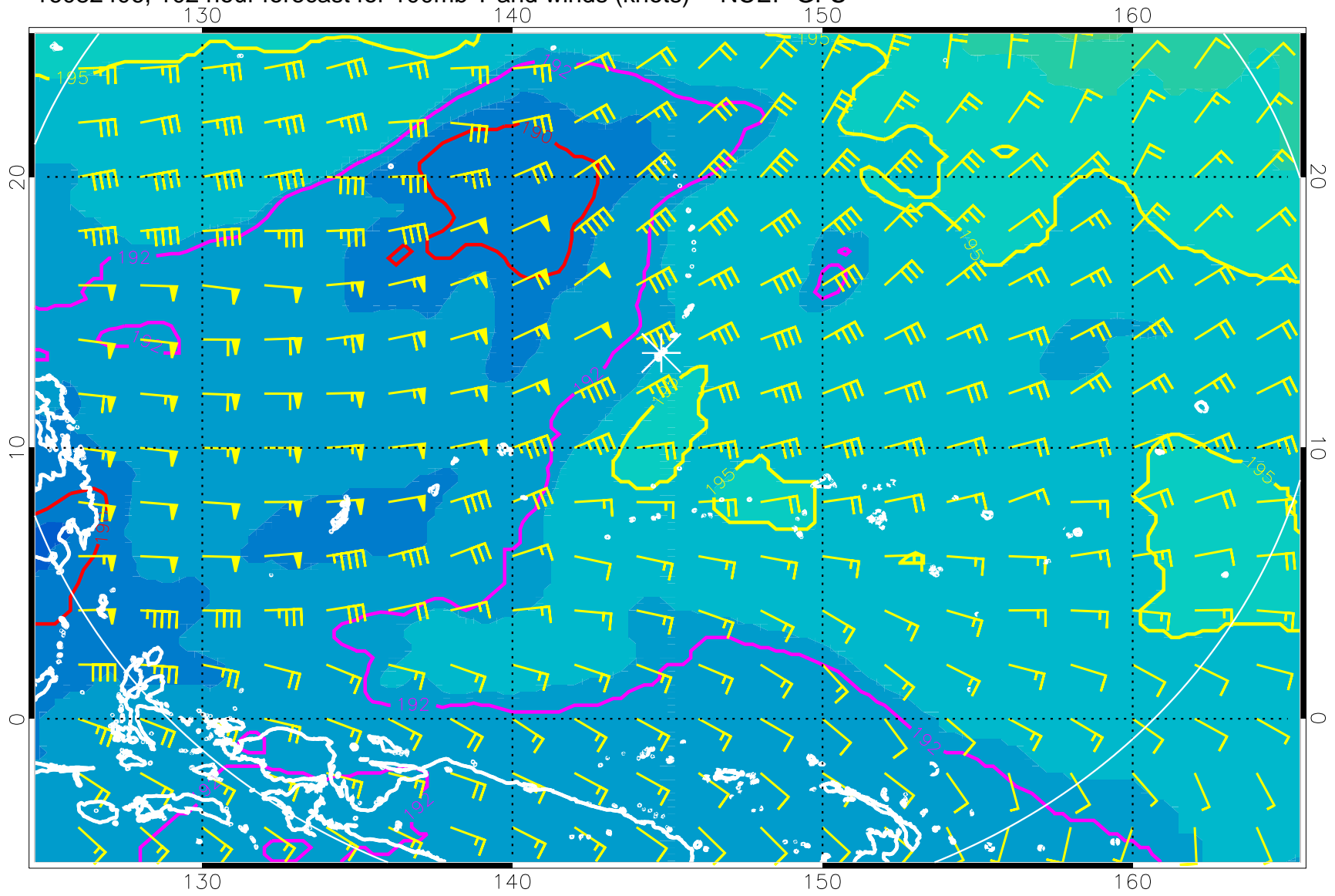
16082406, 102 hour forecast for 100mb T and winds (knots) -- NCEP GFS
