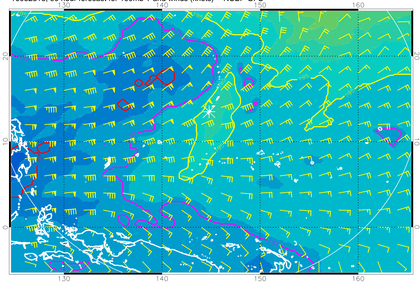
16082318, 90 hour forecast for 100mb T and winds (knots) -- NCEP GFS
