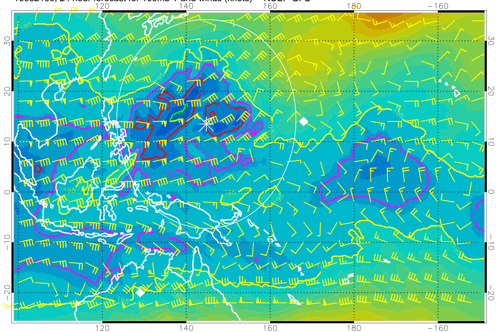
16082100, 24 hour forecast for 100mb T and winds (knots) -- NCEP GFS
