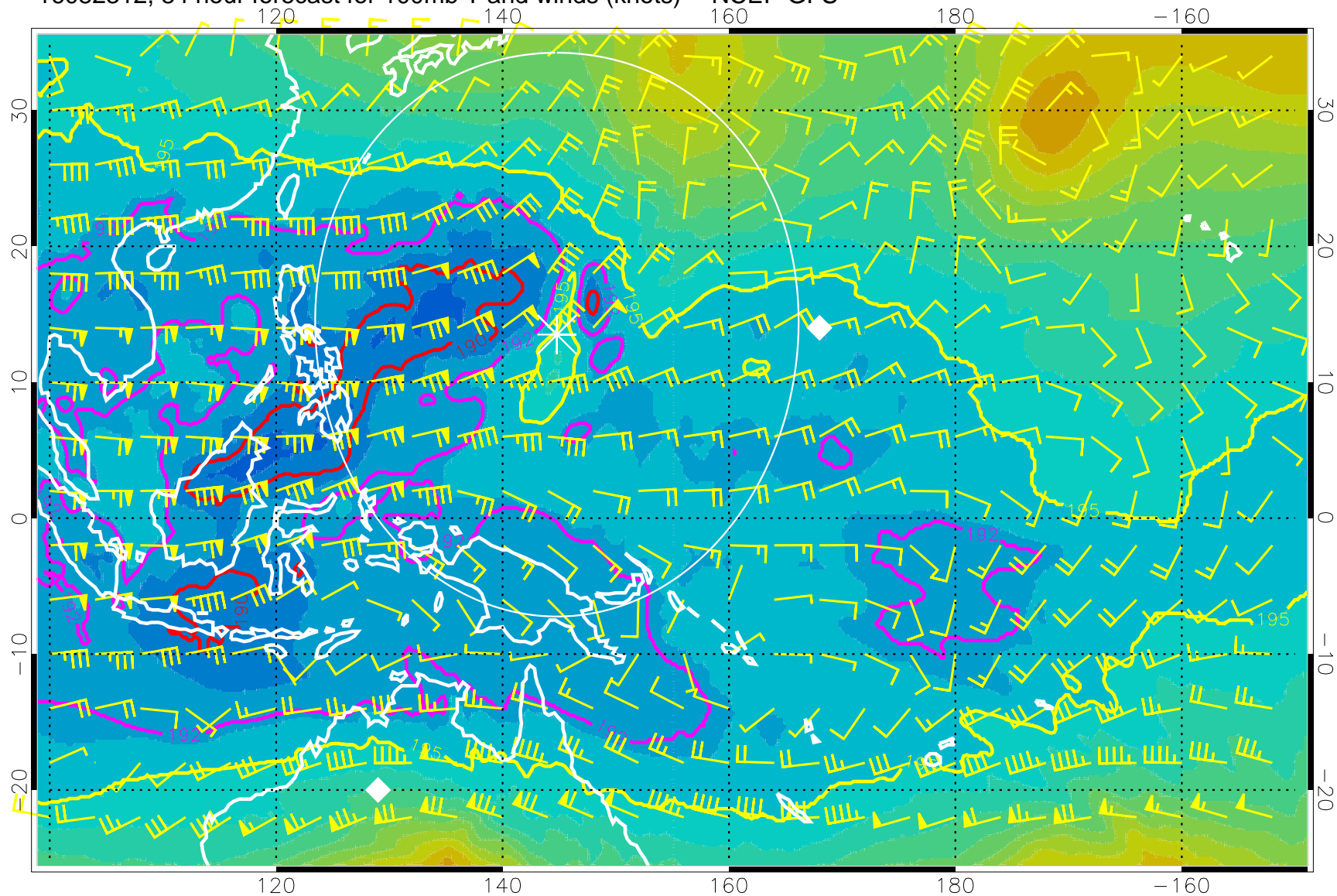
16082312, 84 hour forecast for 100mb T and winds (knots) -- NCEP GFS
