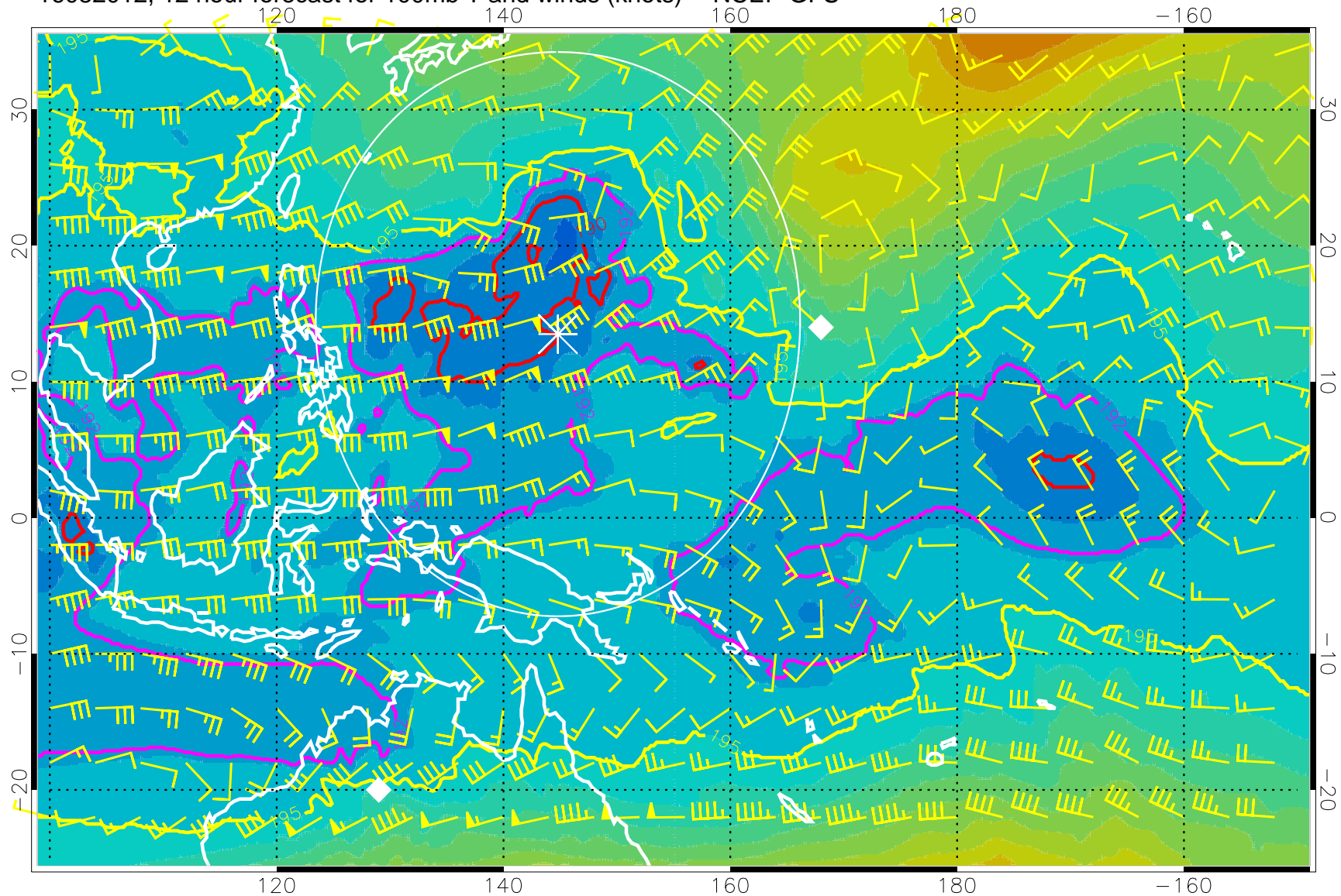
16082012, 12 hour forecast for 100mb T and winds (knots) -- NCEP GFS
