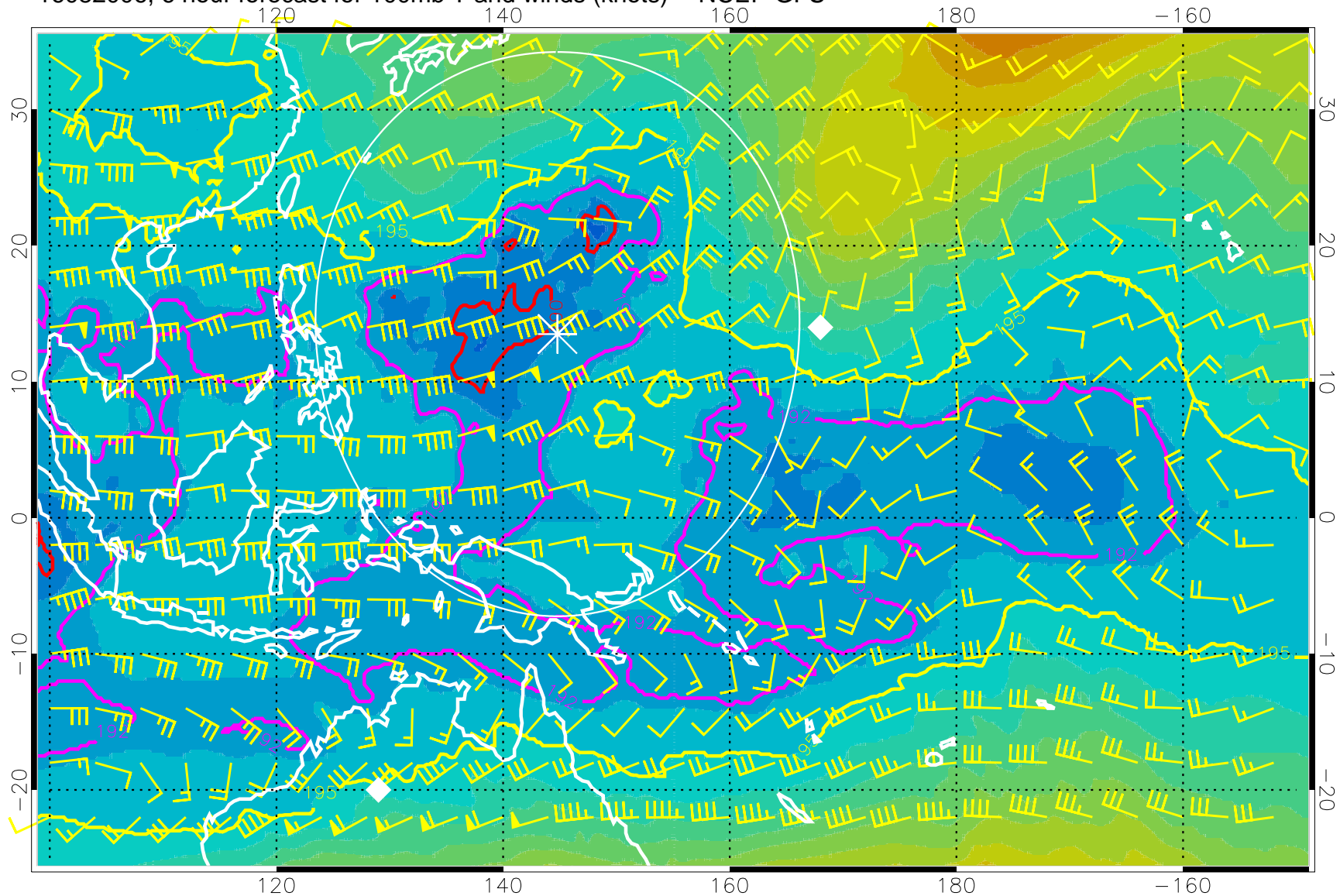
16082006, 6 hour forecast for 100mb T and winds (knots) -- NCEP GFS
