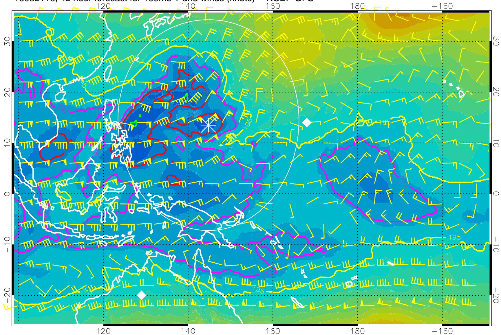
16082118, 42 hour forecast for 100mb T and winds (knots) -- NCEP GFS
