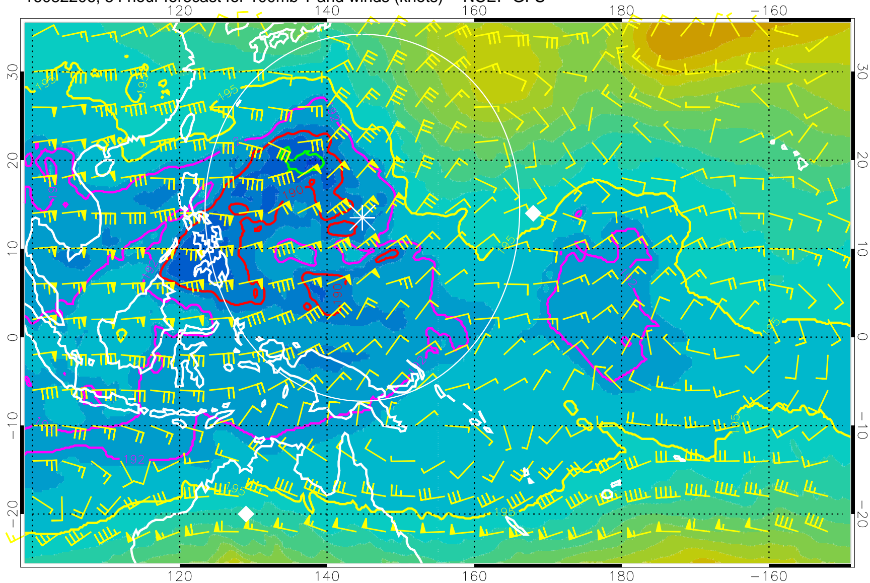
16082206, 54 hour forecast for 100mb T and winds (knots) -- NCEP GFS
