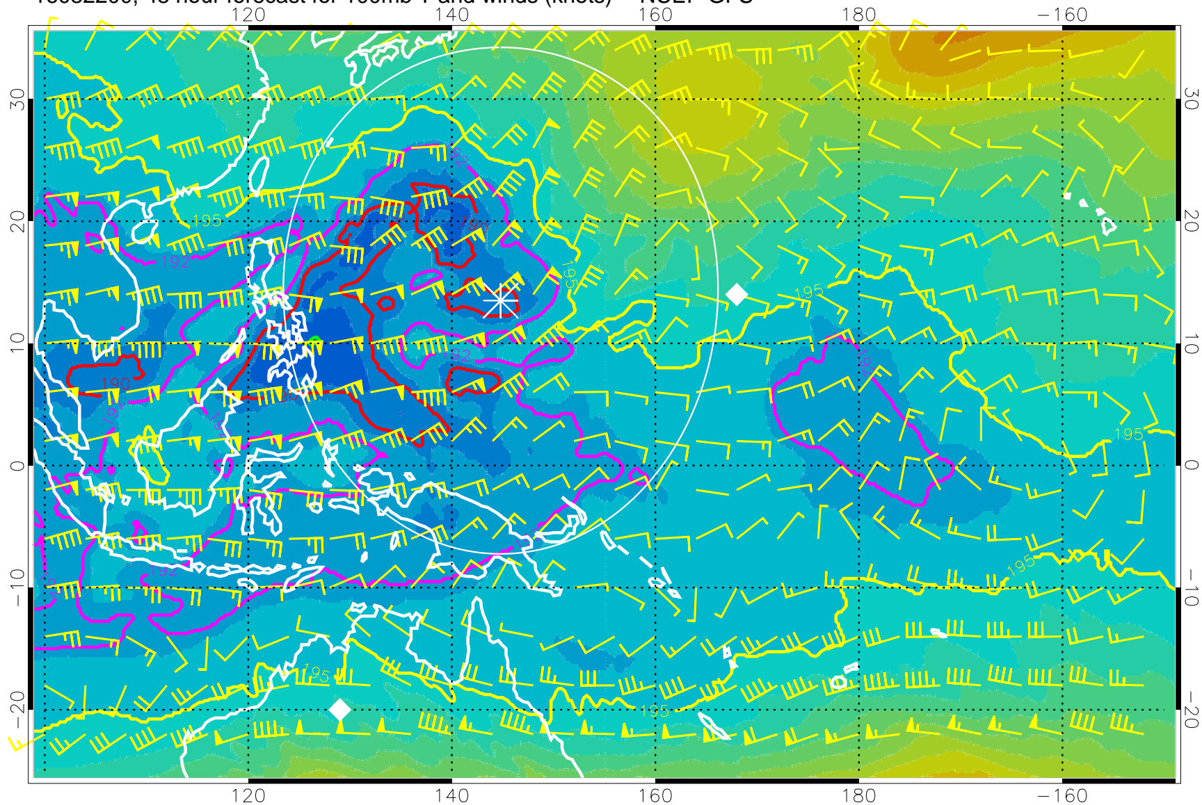
16082200, 48 hour forecast for 100mb T and winds (knots) -- NCEP GFS
