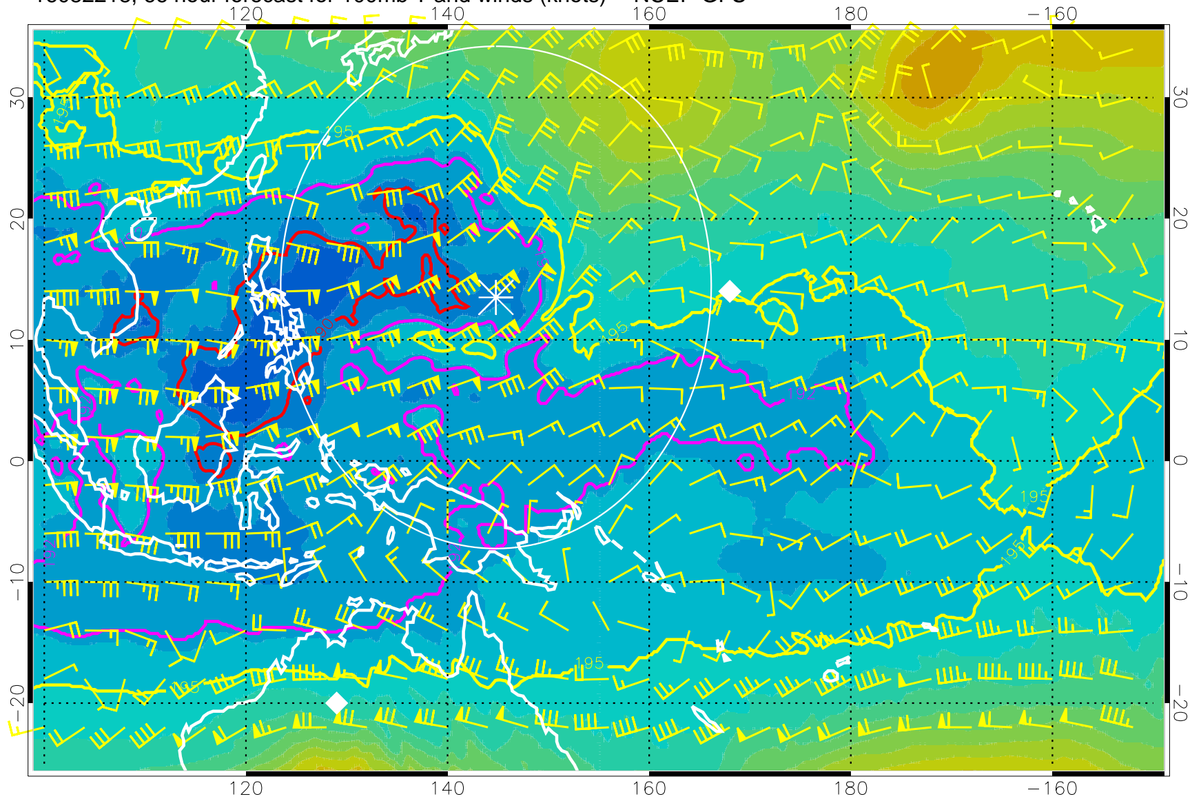
16082218, 66 hour forecast for 100mb T and winds (knots) -- NCEP GFS
