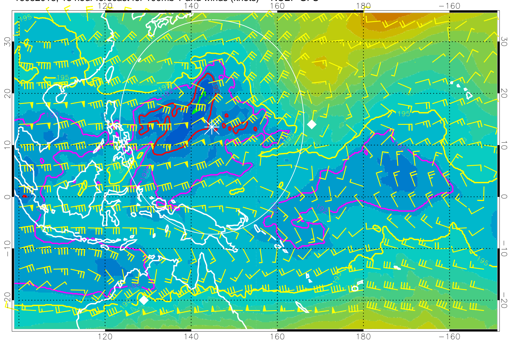
16082018, 18 hour forecast for 100mb T and winds (knots) -- NCEP GFS
