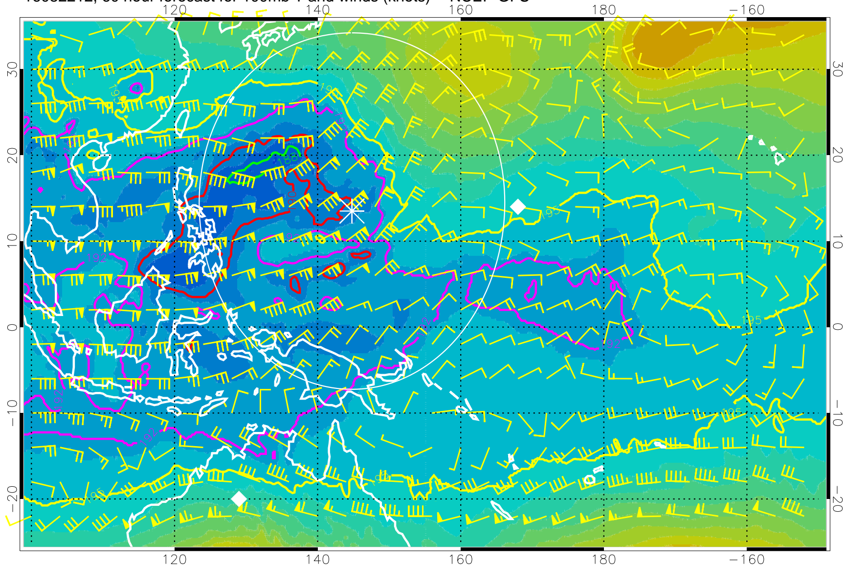
16082212, 60 hour forecast for 100mb T and winds (knots) -- NCEP GFS
