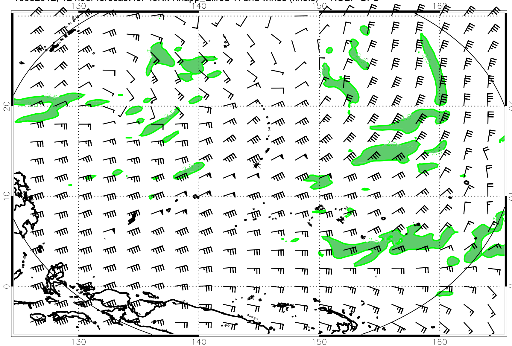
16082012, 12 hour forecast for 49Kft Knapp_Ellrod TI and winds (knots) -- NCEP GFS
