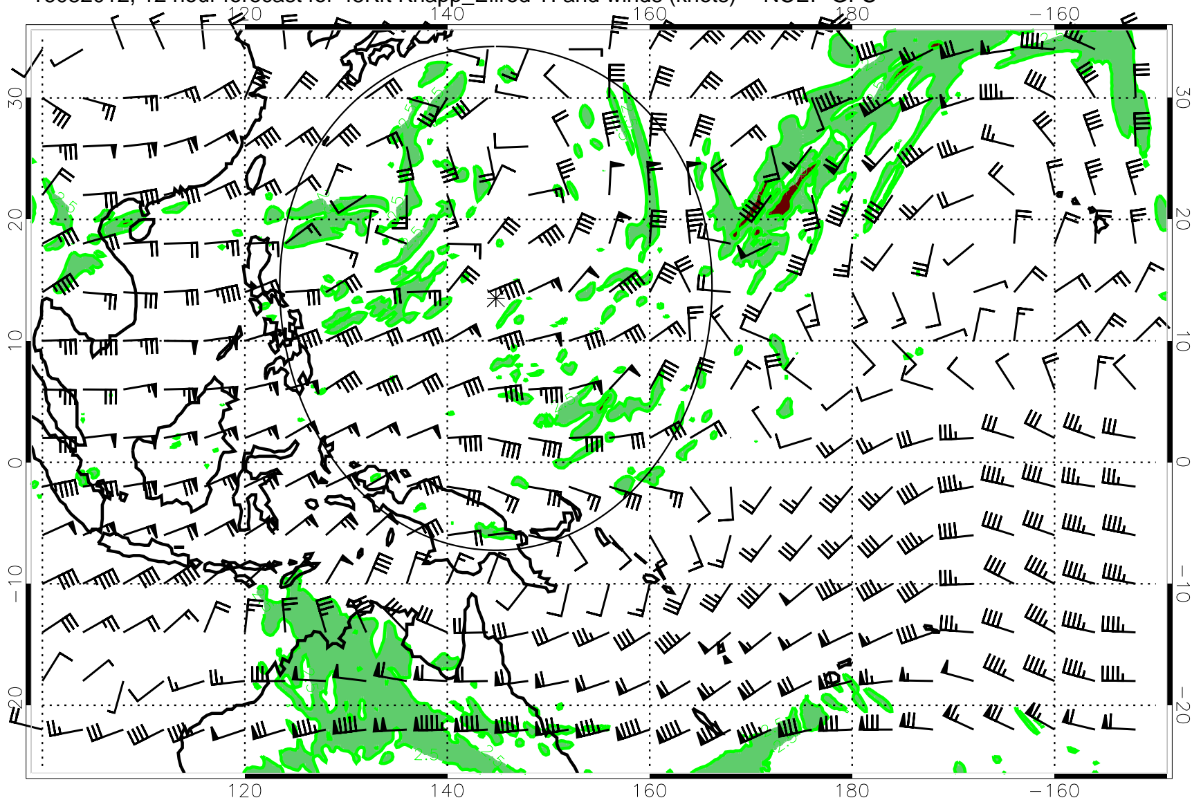
16082012, 12 hour forecast for 45Kft Knapp_Ellrod TI and winds (knots) -- NCEP GFS
