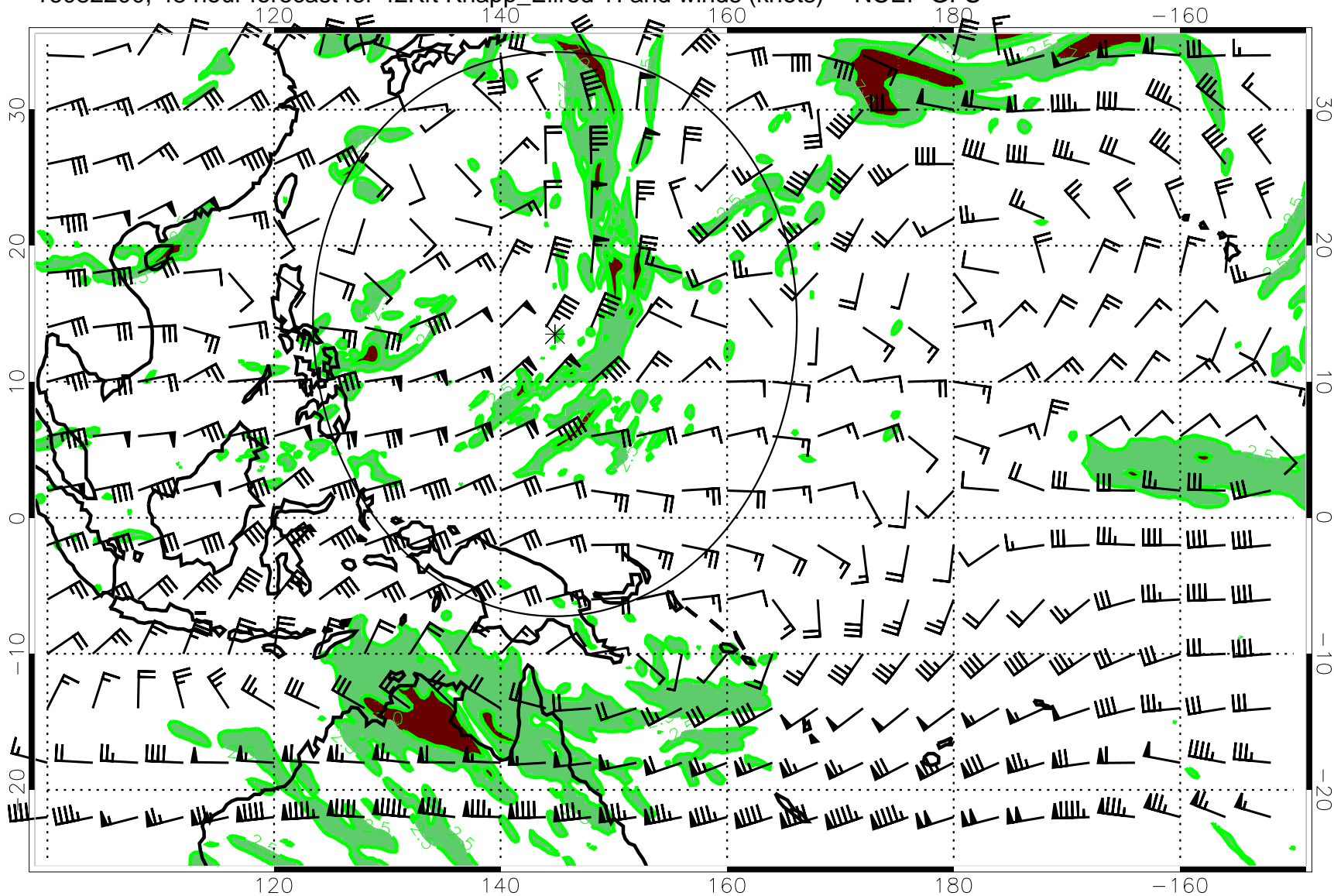
16082200, 48 hour forecast for 42Kft Knapp_Ellrod TI and winds (knots) -- NCEP GFS
