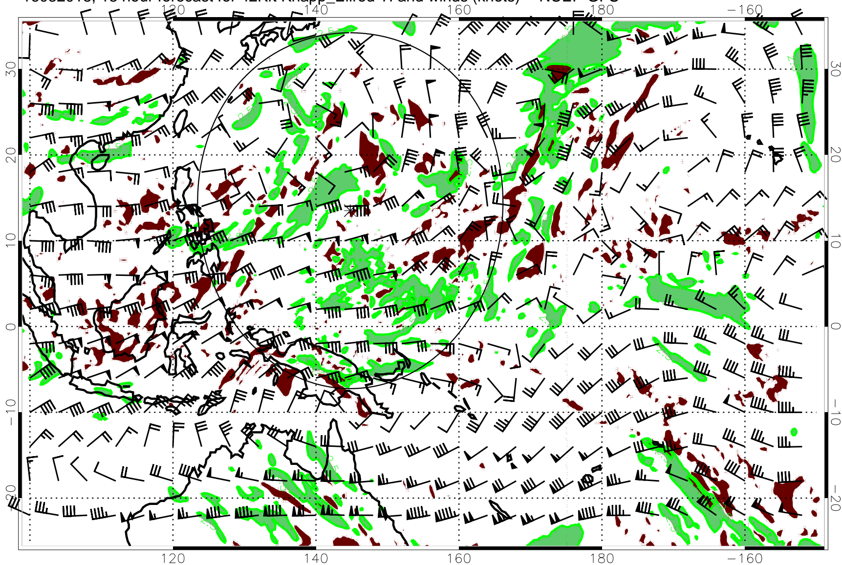
16082018, 18 hour forecast for 42Kft Knapp_Ellrod TI and winds (knots) -- NCEP GFS
