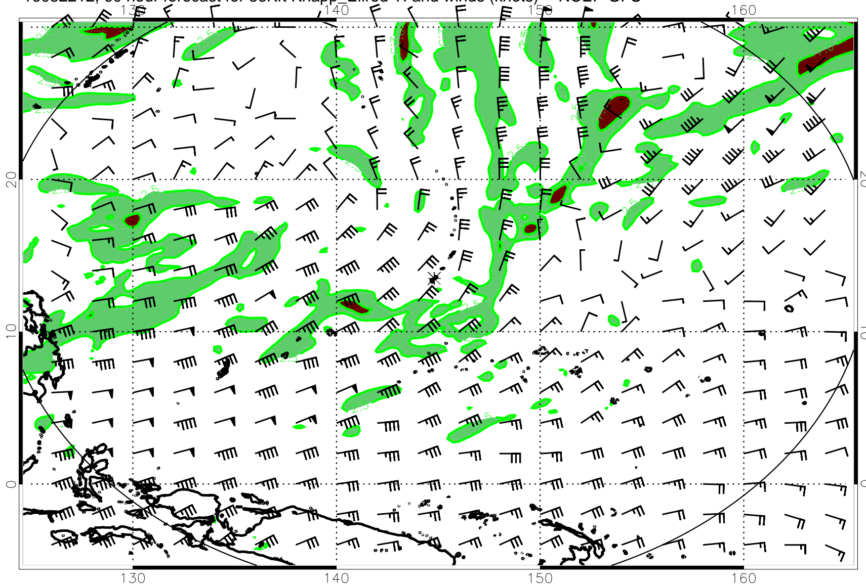
16082212, 60 hour forecast for 36Kft Knapp_Ellrod TI and winds (knots) -- NCEP GFS
