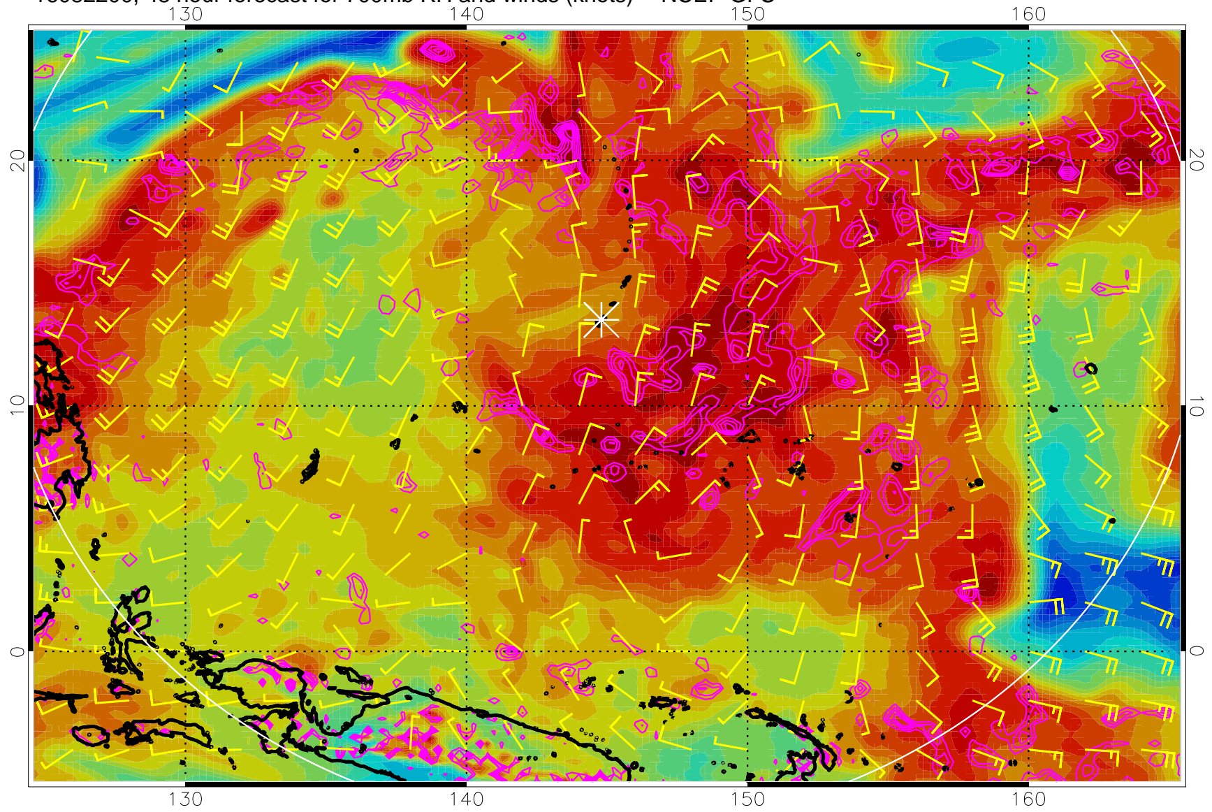
16082200, 48 hour forecast for 700mb RH and winds (knots) -- NCEP GFS
