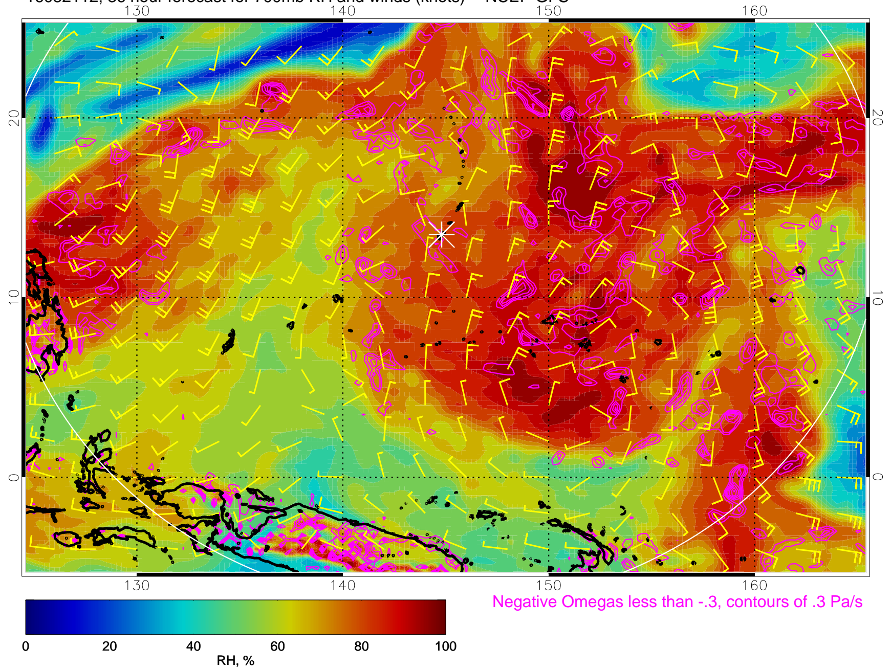
16082112, 36 hour forecast for 700mb RH and winds (knots) -- NCEP GFS
