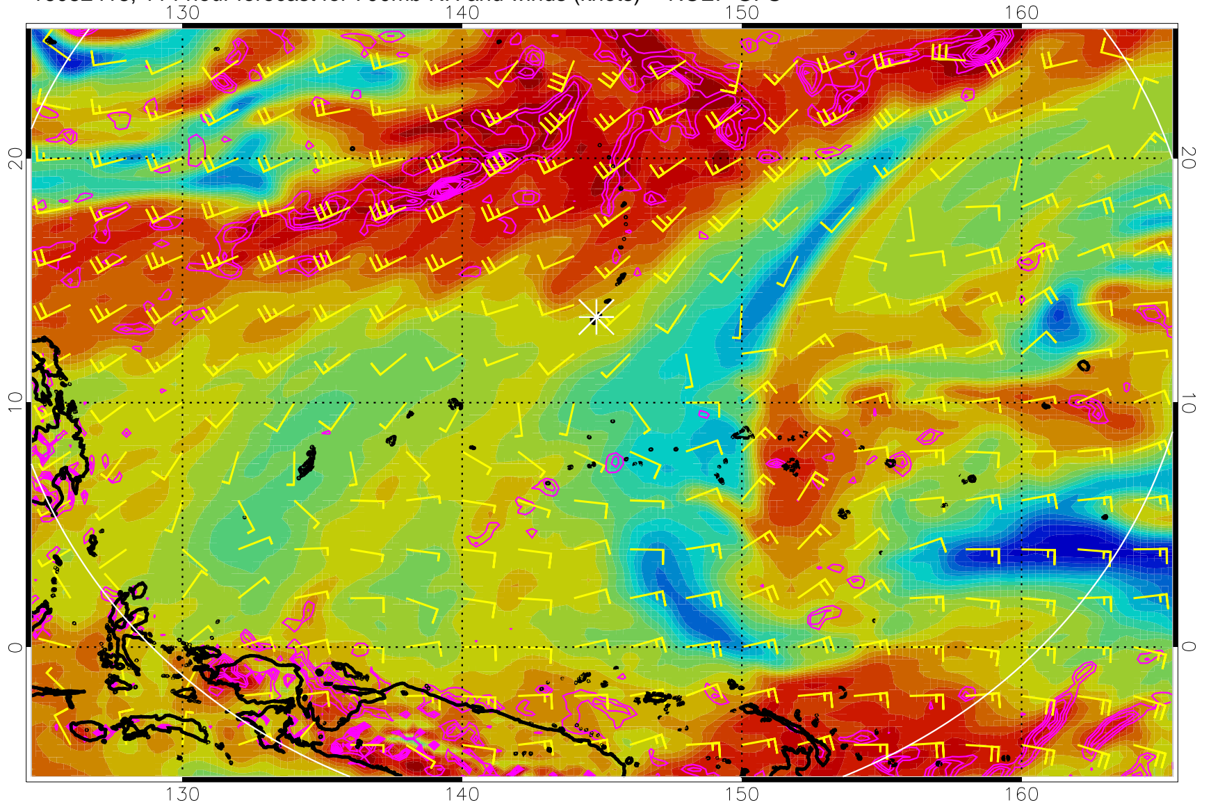
16082418, 114 hour forecast for 700mb RH and winds (knots) -- NCEP GFS
