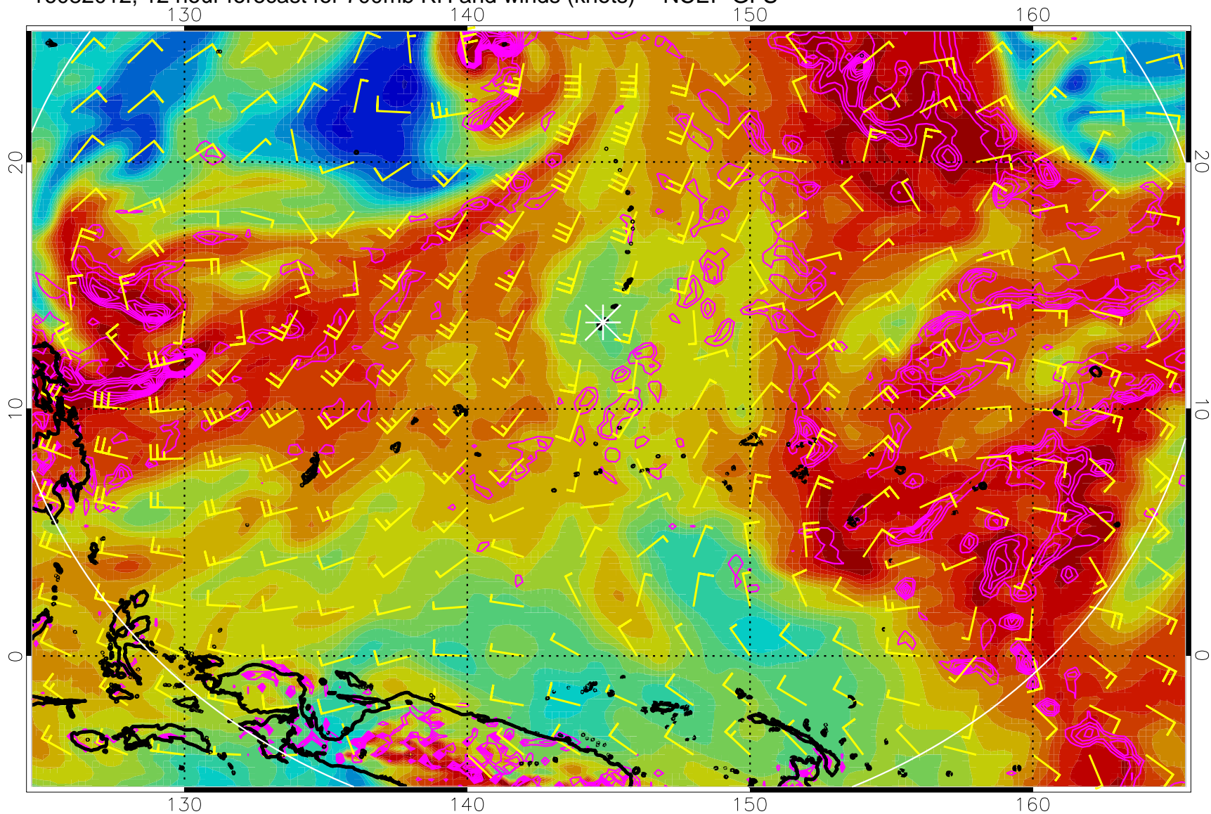
16082012, 12 hour forecast for 700mb RH and winds (knots) -- NCEP GFS
