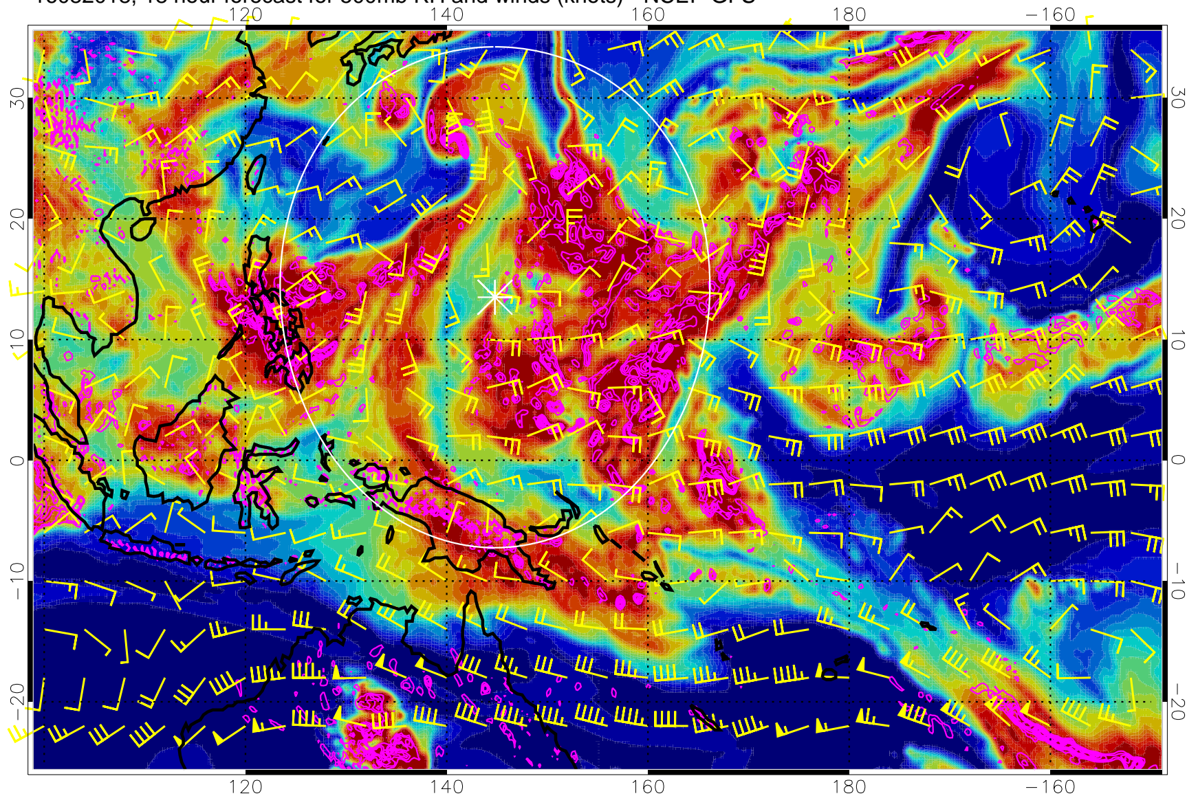
16082018, 18 hour forecast for 500mb RH and winds (knots) - NCEP GFS
