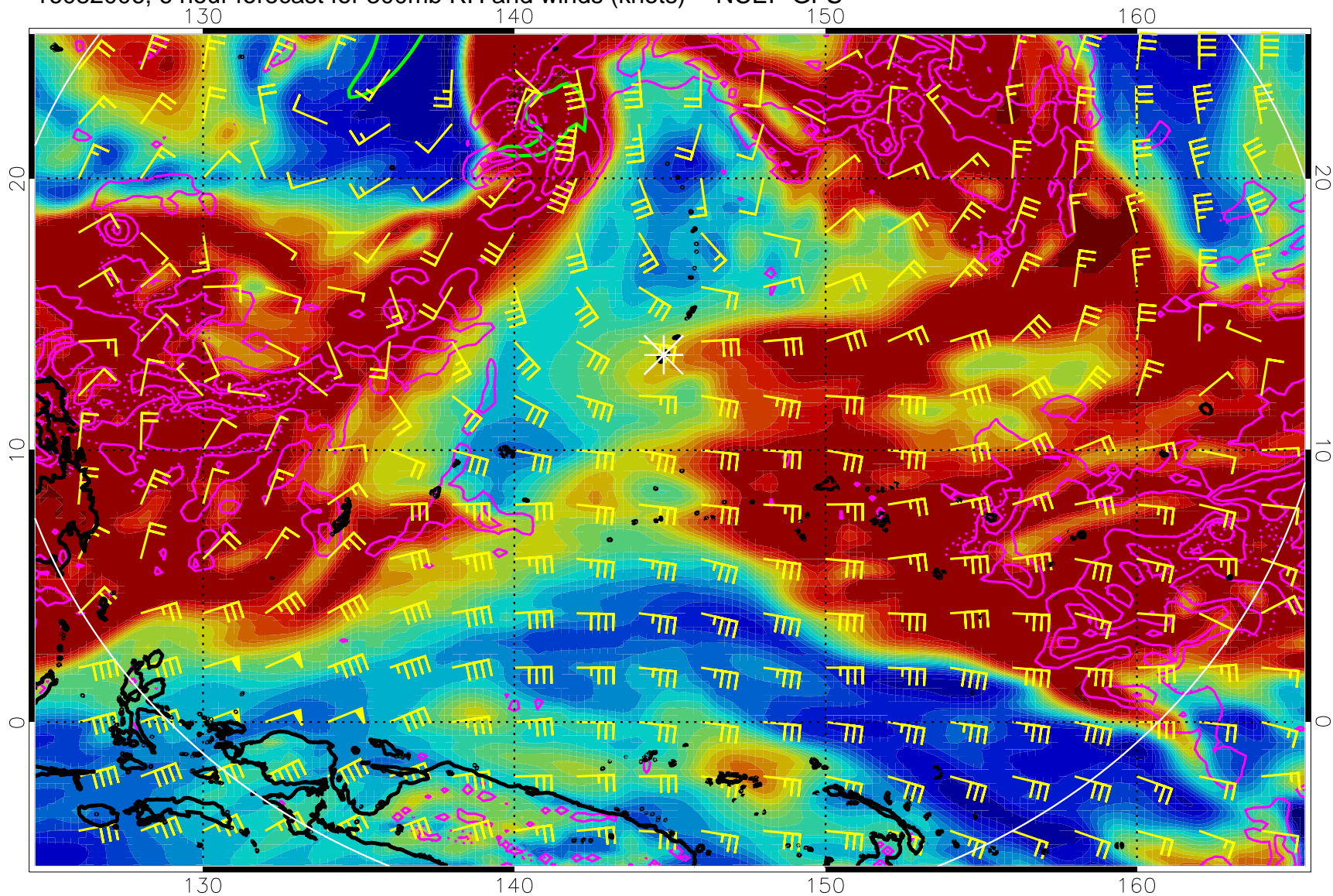
16082006, 6 hour forecast for 300mb RH and winds (knots) -- NCEP GFS
