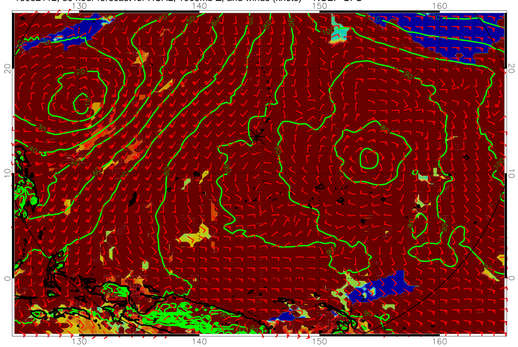
16082112, 36 hour forecast for HCAL, 1000mb Z, and winds (knots) -- NCEP GFS
