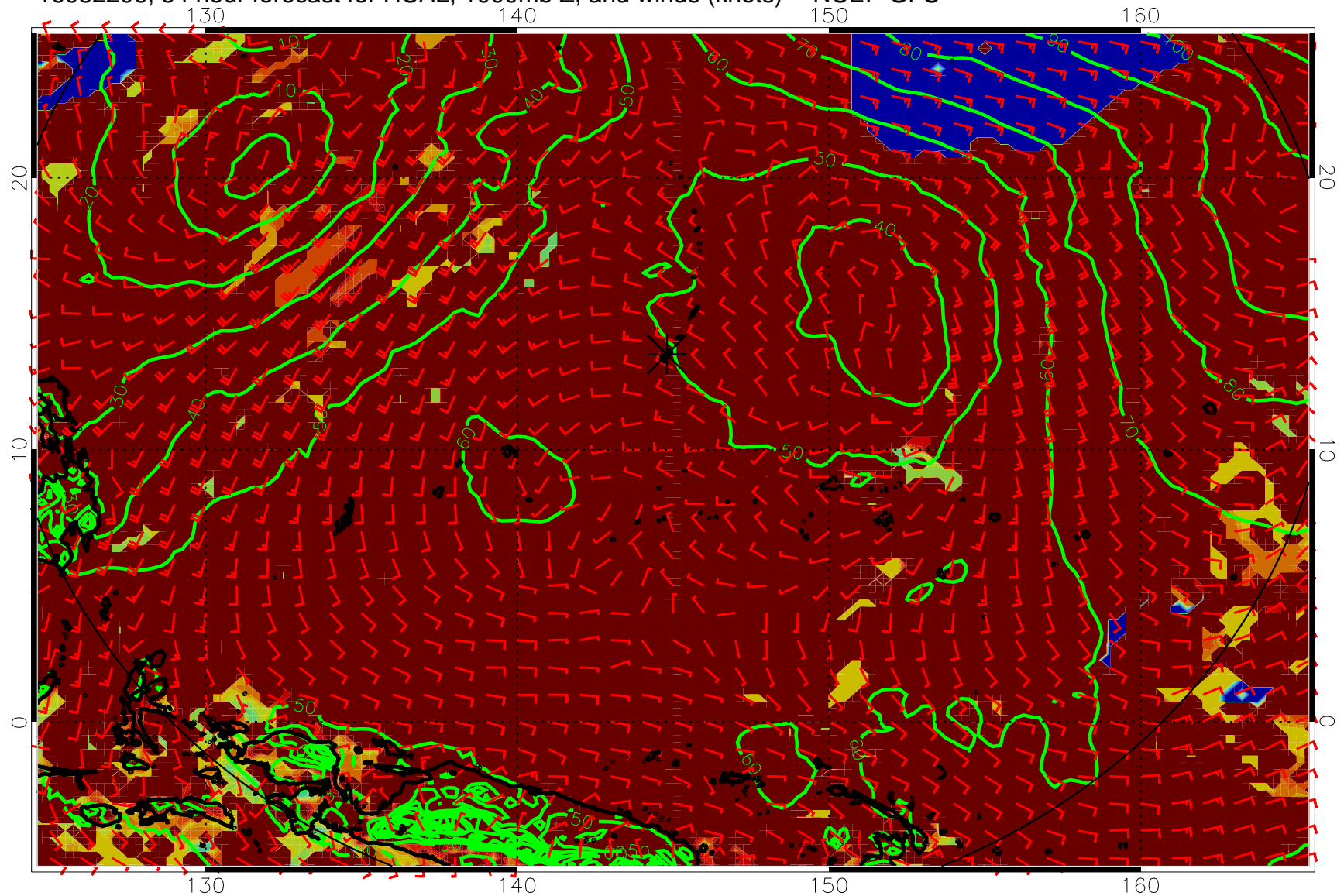
16082206, 54 hour forecast for HCAL, 1000mb Z, and winds (knots) -- NCEP GFS
