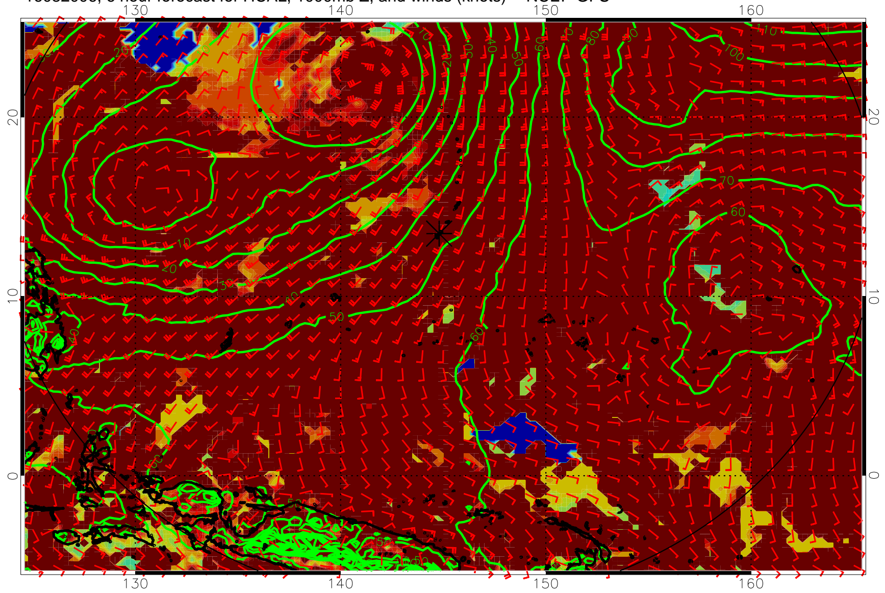
16082006, 6 hour forecast for HCAL, 1000mb Z, and winds (knots) -- NCEP GFS
