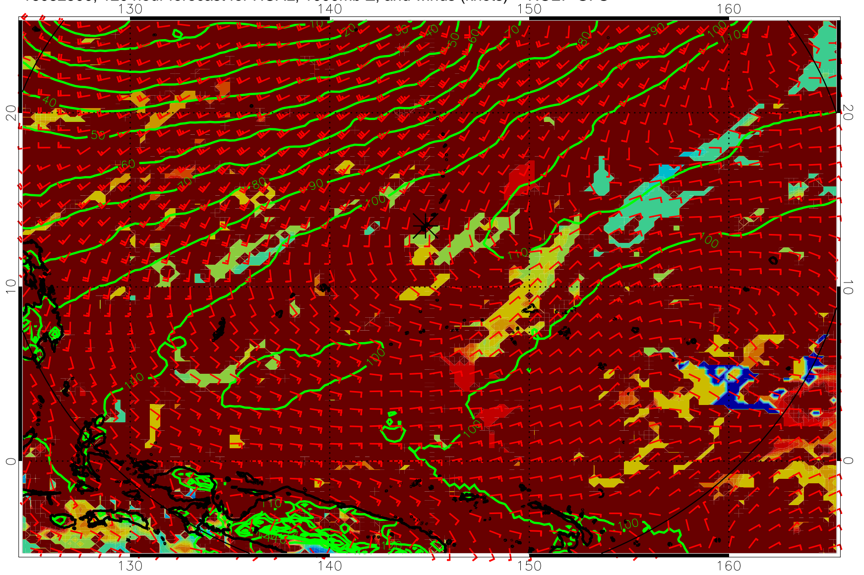
16082500, 120 hour forecast for HCAL, 1000mb Z, and winds (knots) -- NCEP GFS
