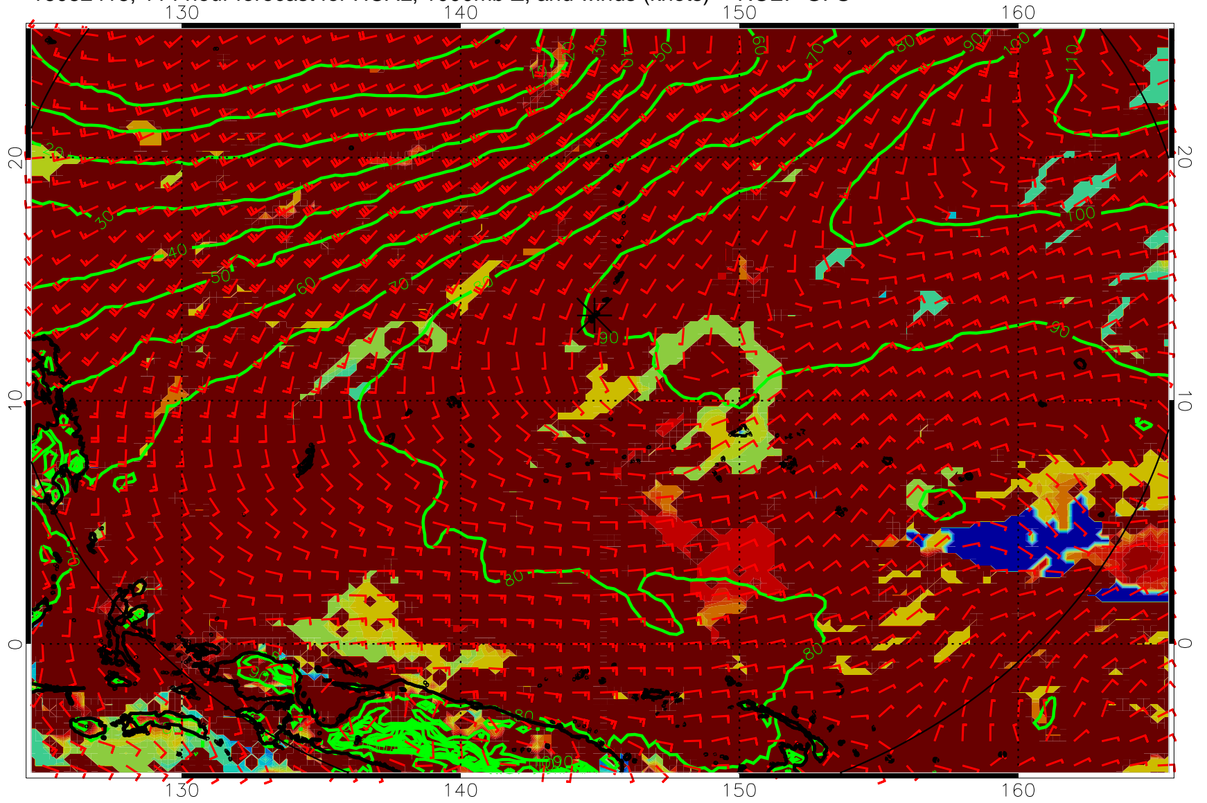
16082418, 114 hour forecast for HCAL, 1000mb Z, and winds (knots) -- NCEP GFS
