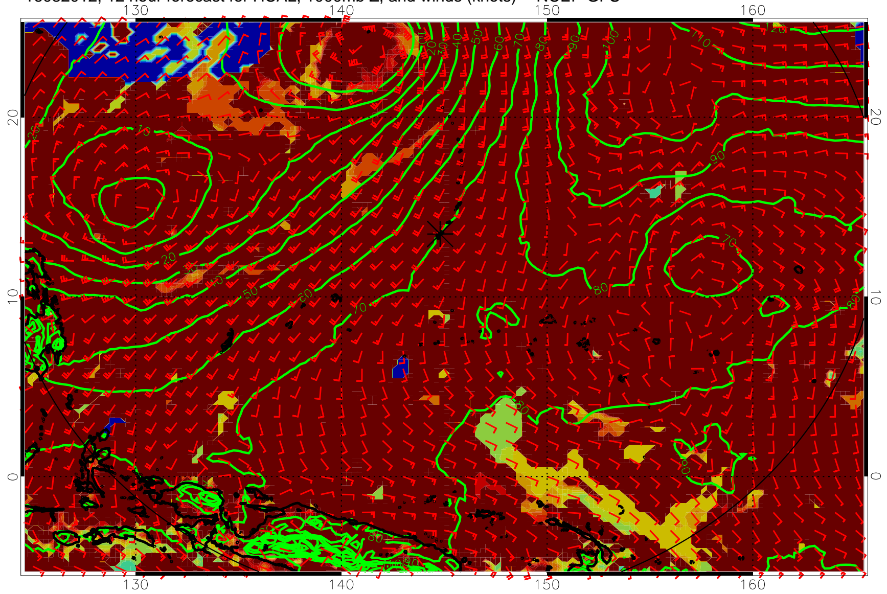
16082012, 12 hour forecast for HCAL, 1000mb Z, and winds (knots) -- NCEP GFS
