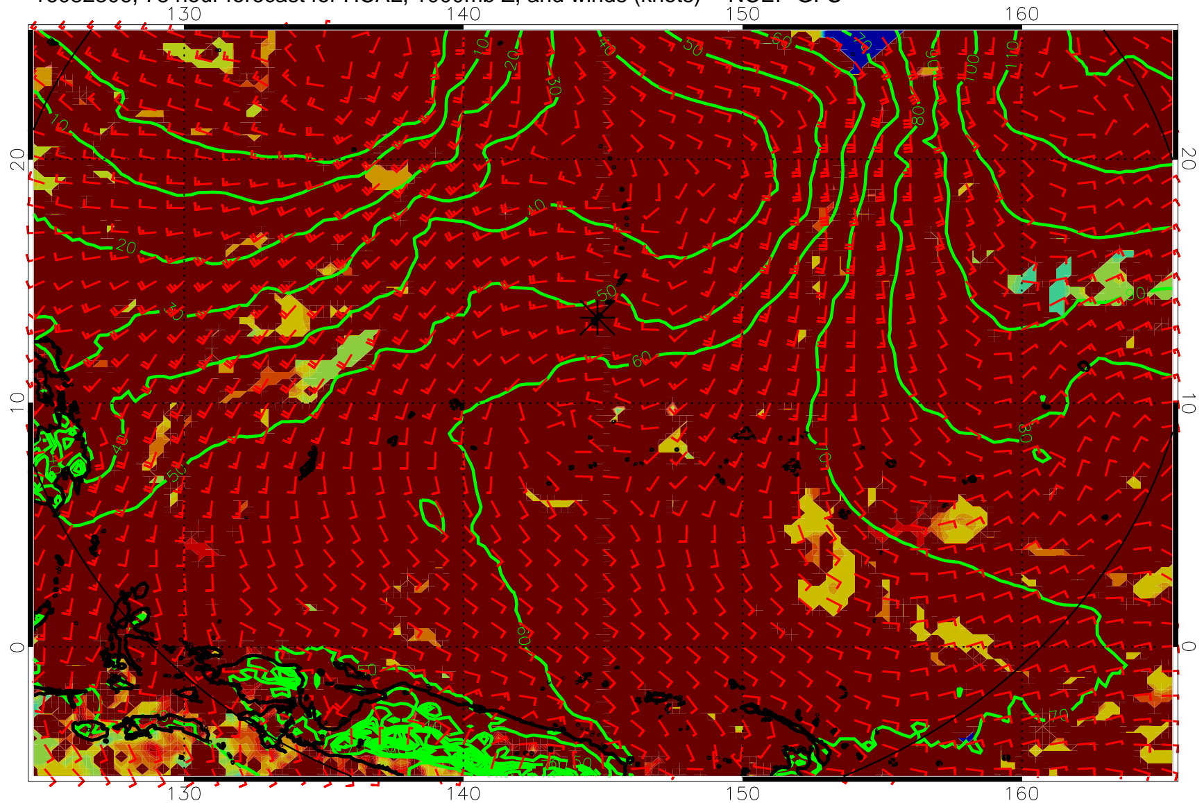
16082306, 78 hour forecast for HCAL, 1000mb Z, and winds (knots) -- NCEP GFS
