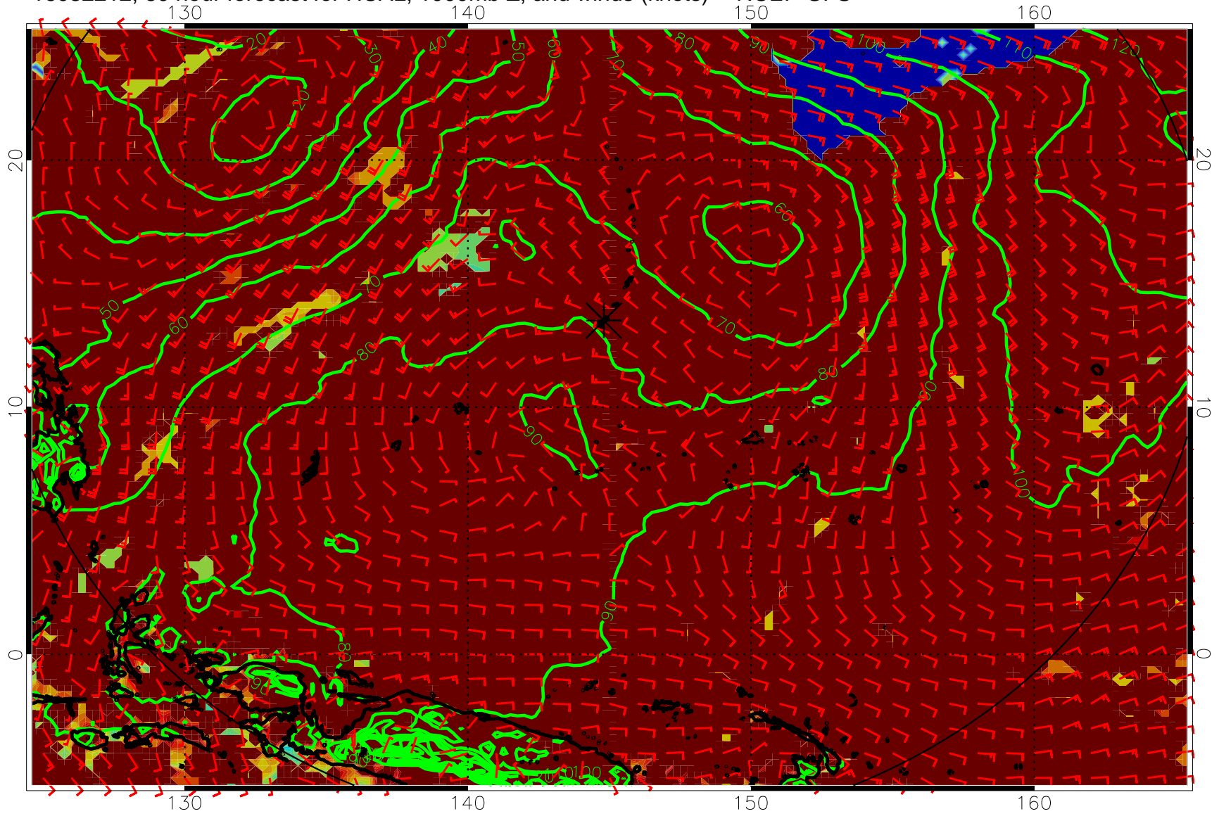
16082212, 60 hour forecast for HCAL, 1000mb Z, and winds (knots) -- NCEP GFS
