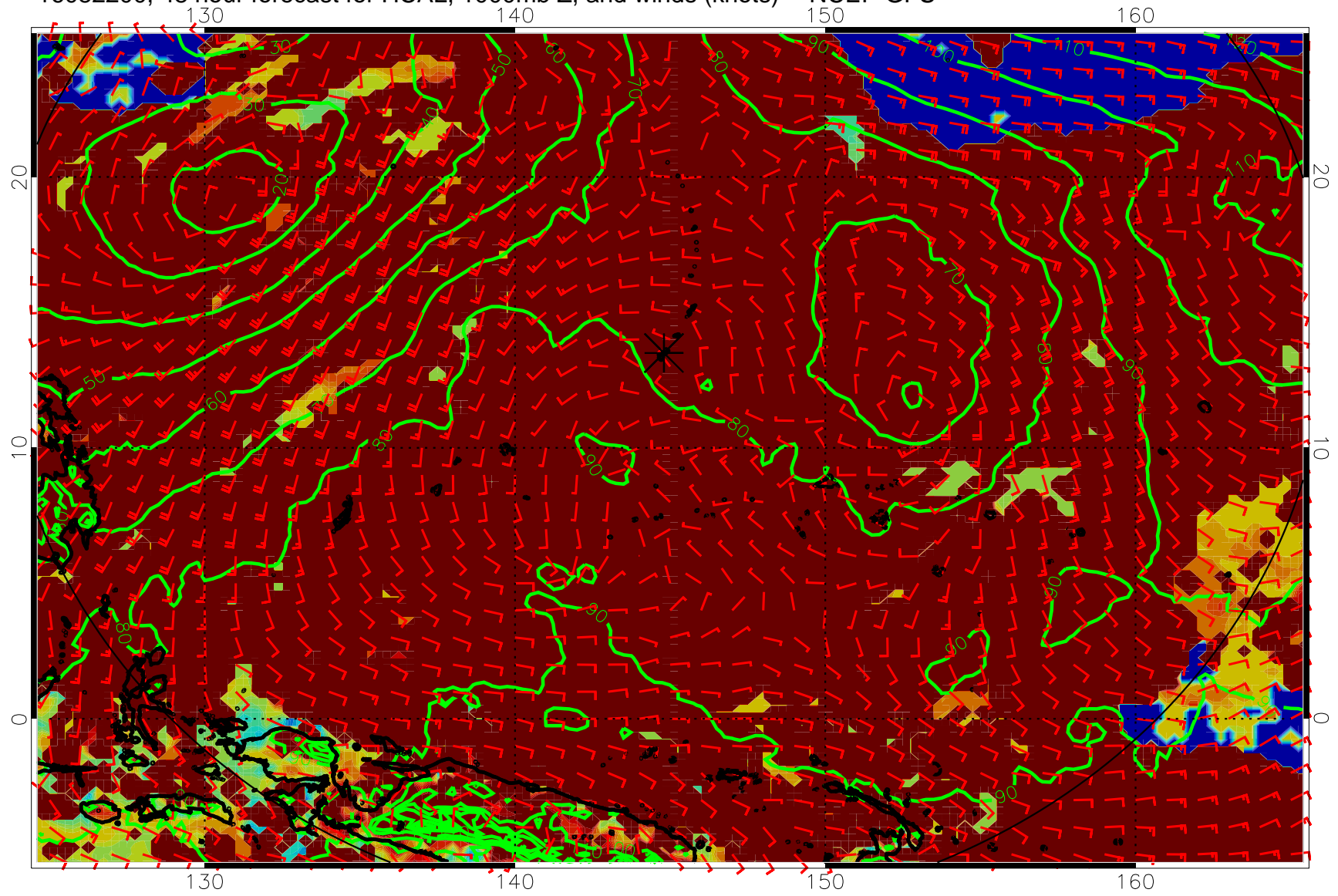
16082200, 48 hour forecast for HCAL, 1000mb Z, and winds (knots) -- NCEP GFS
