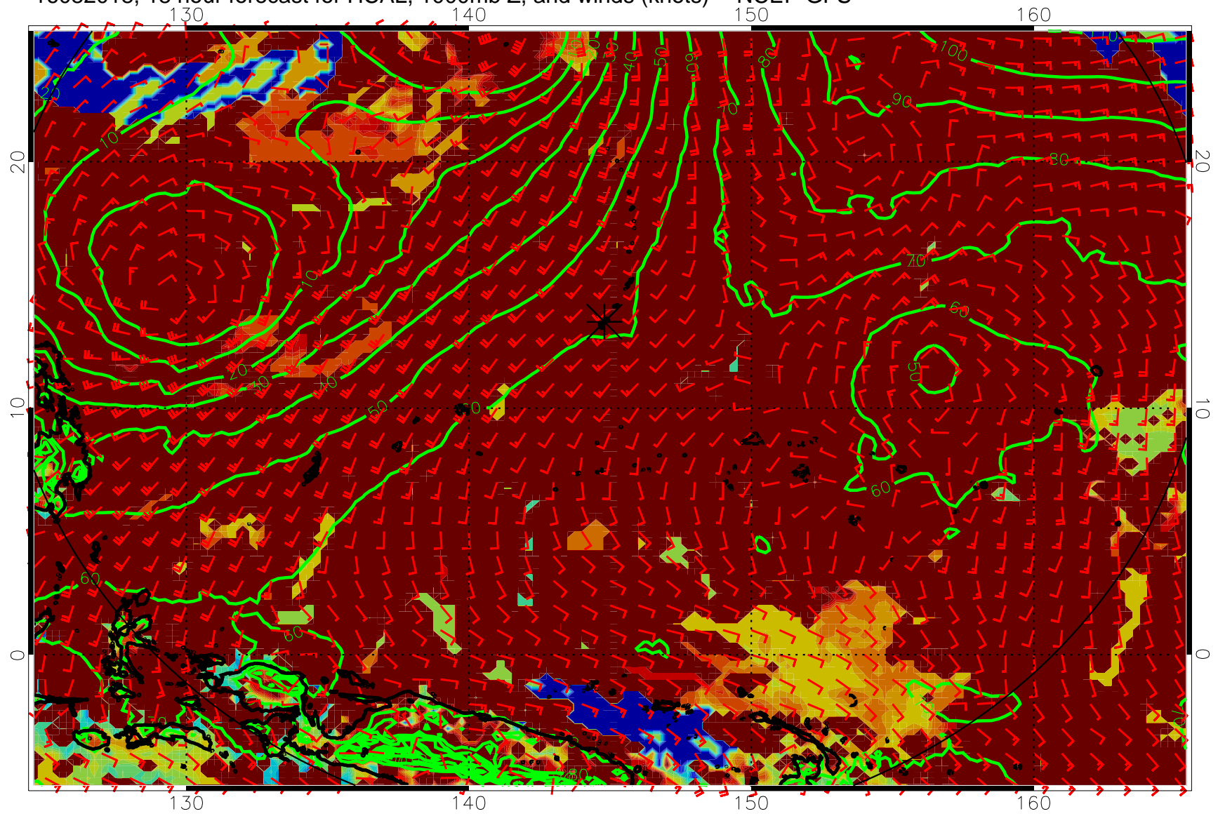
16082018, 18 hour forecast for HCAL, 1000mb Z, and winds (knots) -- NCEP GFS
