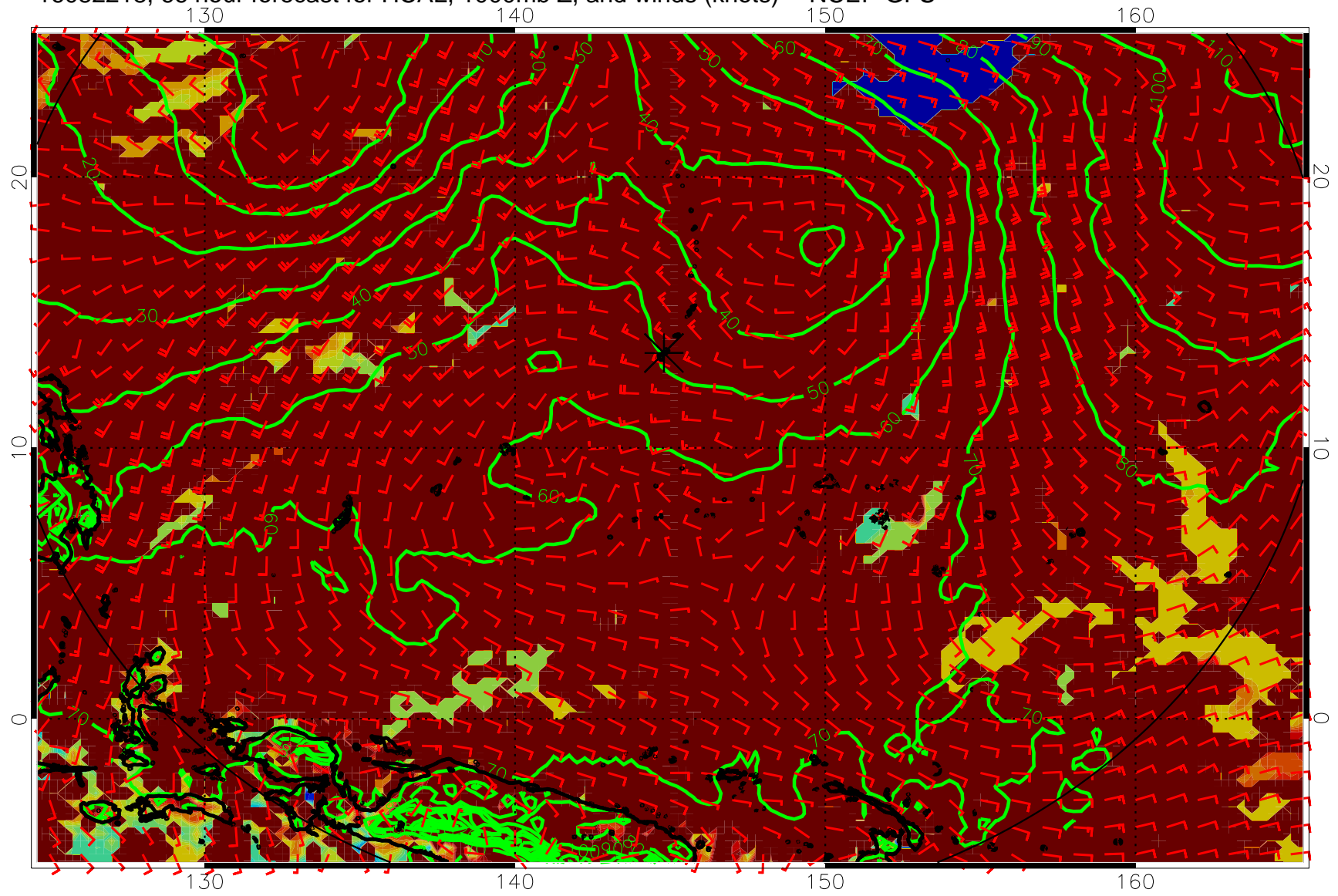
16082218, 66 hour forecast for HCAL, 1000mb Z, and winds (knots) -- NCEP GFS
