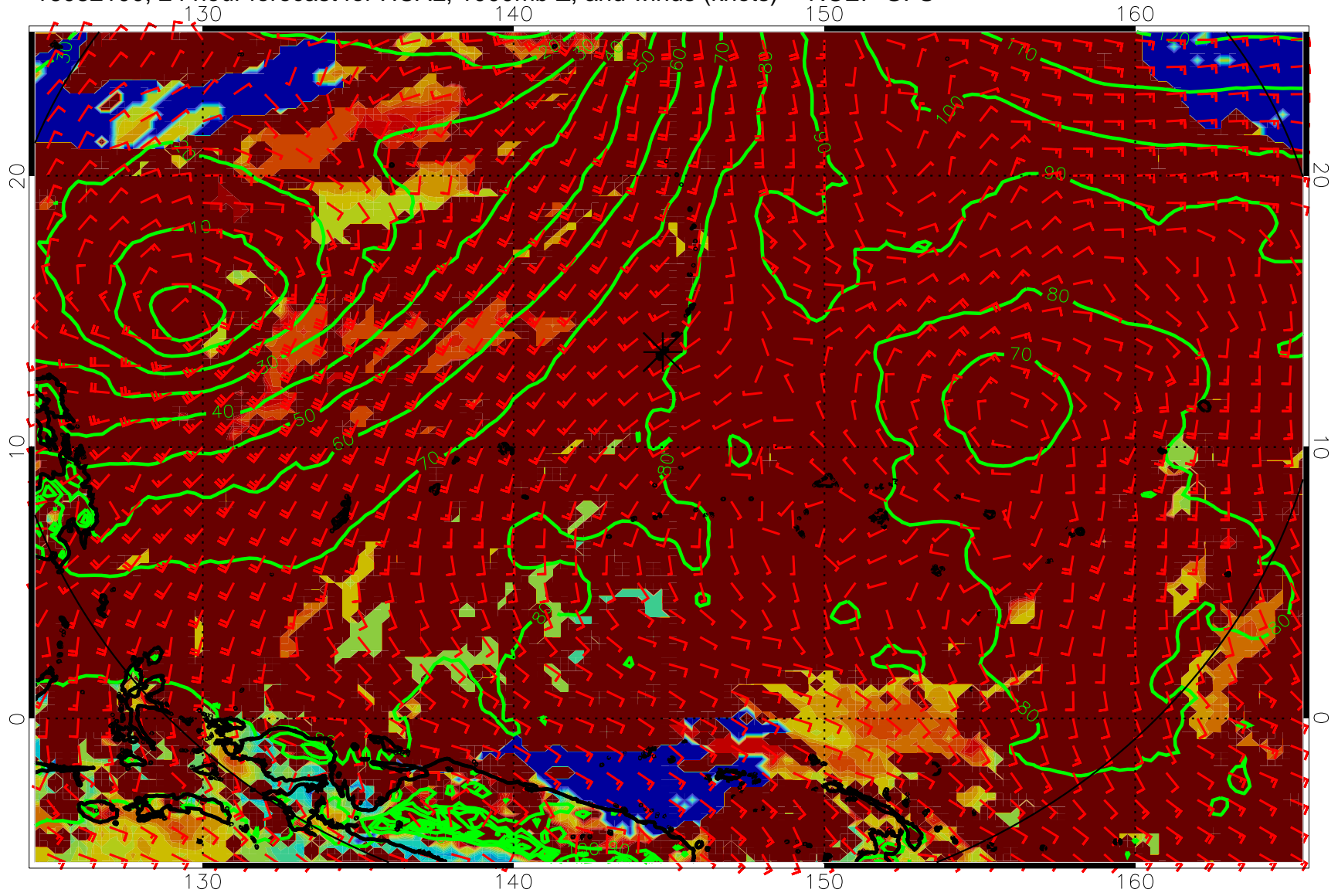
16082100, 24 hour forecast for HCAL, 1000mb Z, and winds (knots) -- NCEP GFS
