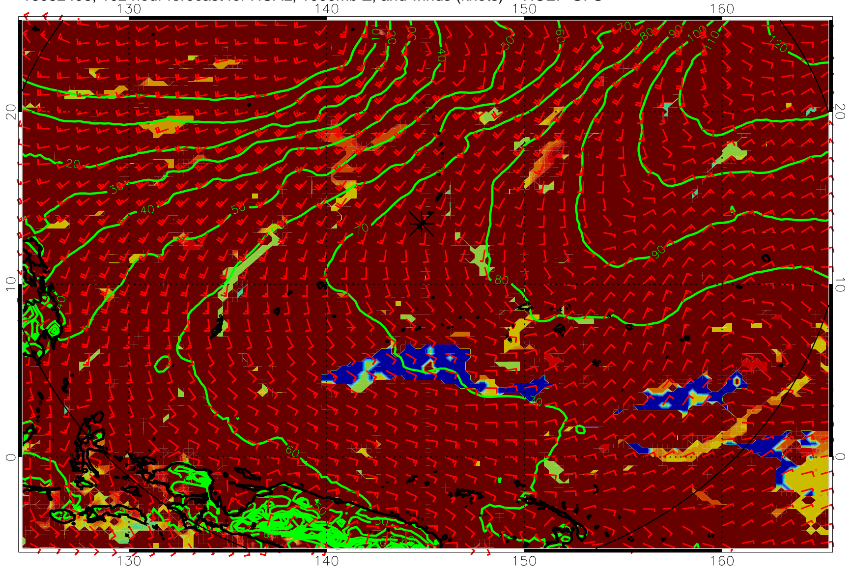
16082406, 102 hour forecast for HCAL, 1000mb Z, and winds (knots) -- NCEP GFS
