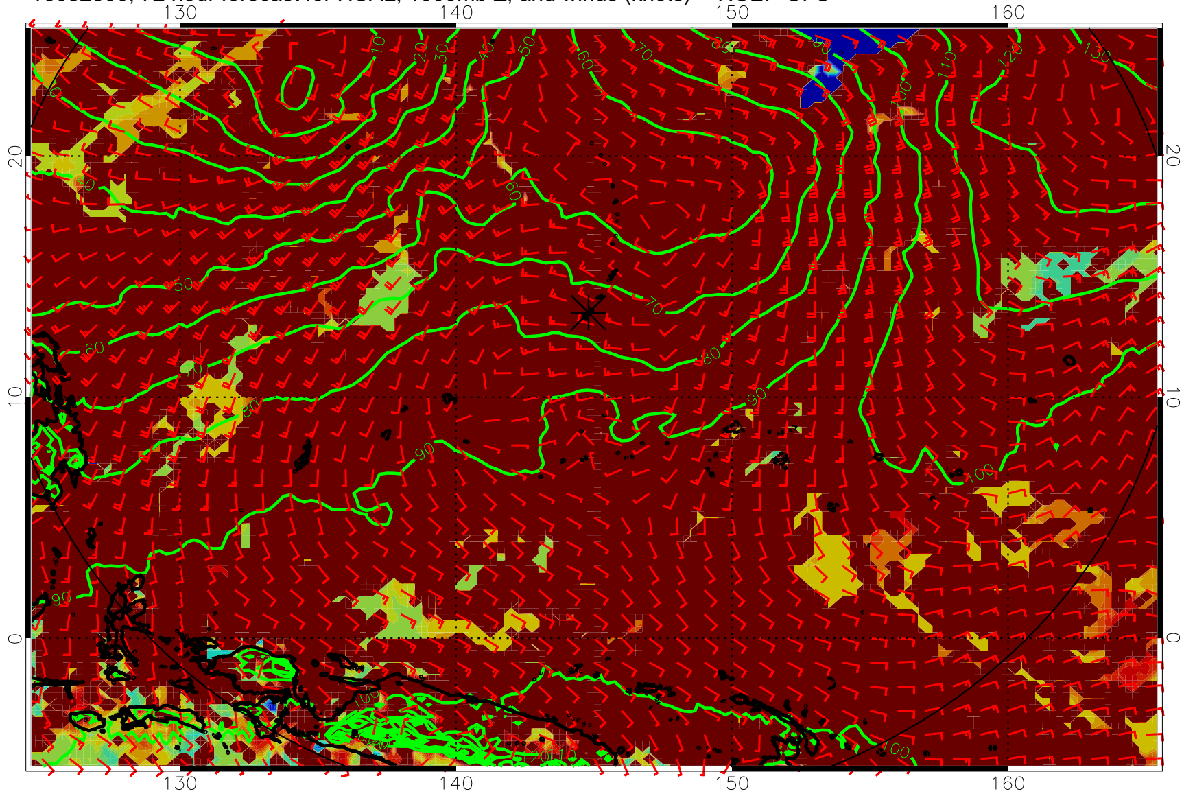
16082300, 72 hour forecast for HCAL, 1000mb Z, and winds (knots) -- NCEP GFS
