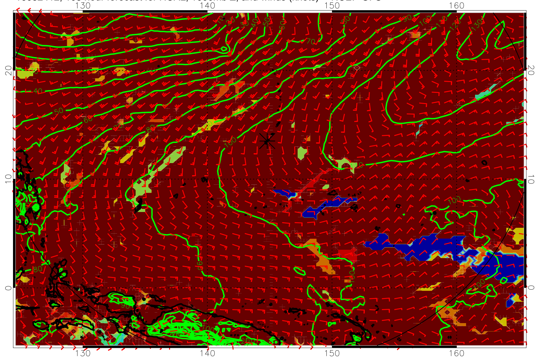
16082412, 108 hour forecast for HCAL, 1000mb Z, and winds (knots) -- NCEP GFS
