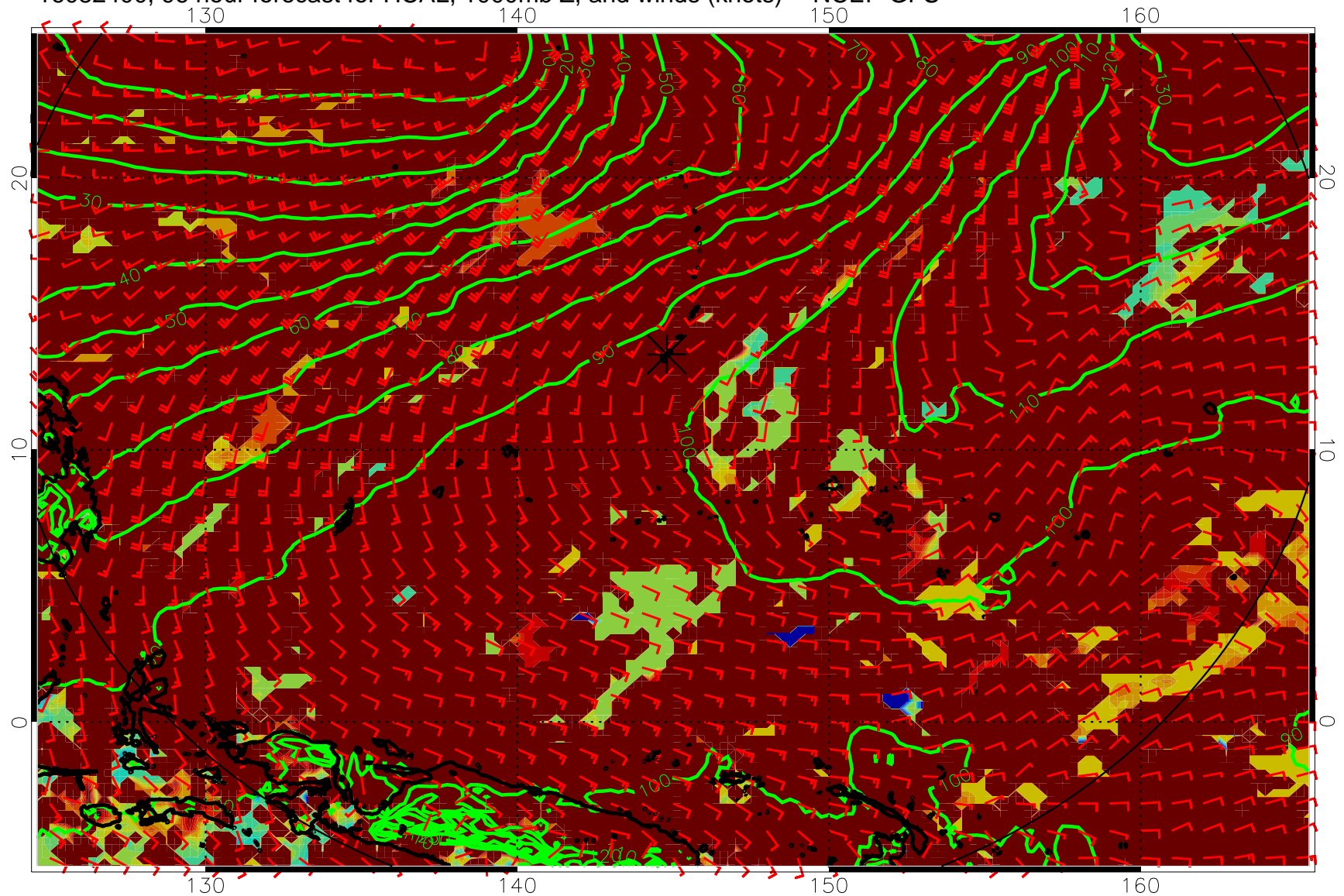
16082400, 96 hour forecast for HCAL, 1000mb Z, and winds (knots) -- NCEP GFS
