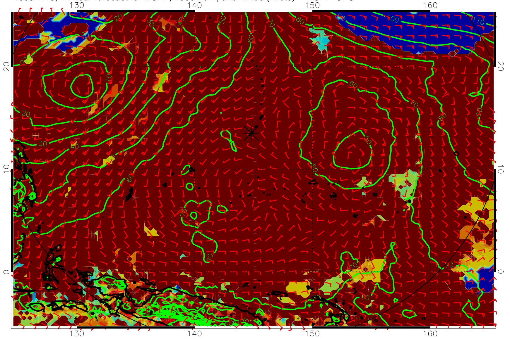
16082118, 42 hour forecast for HCAL, 1000mb Z, and winds (knots) -- NCEP GFS
