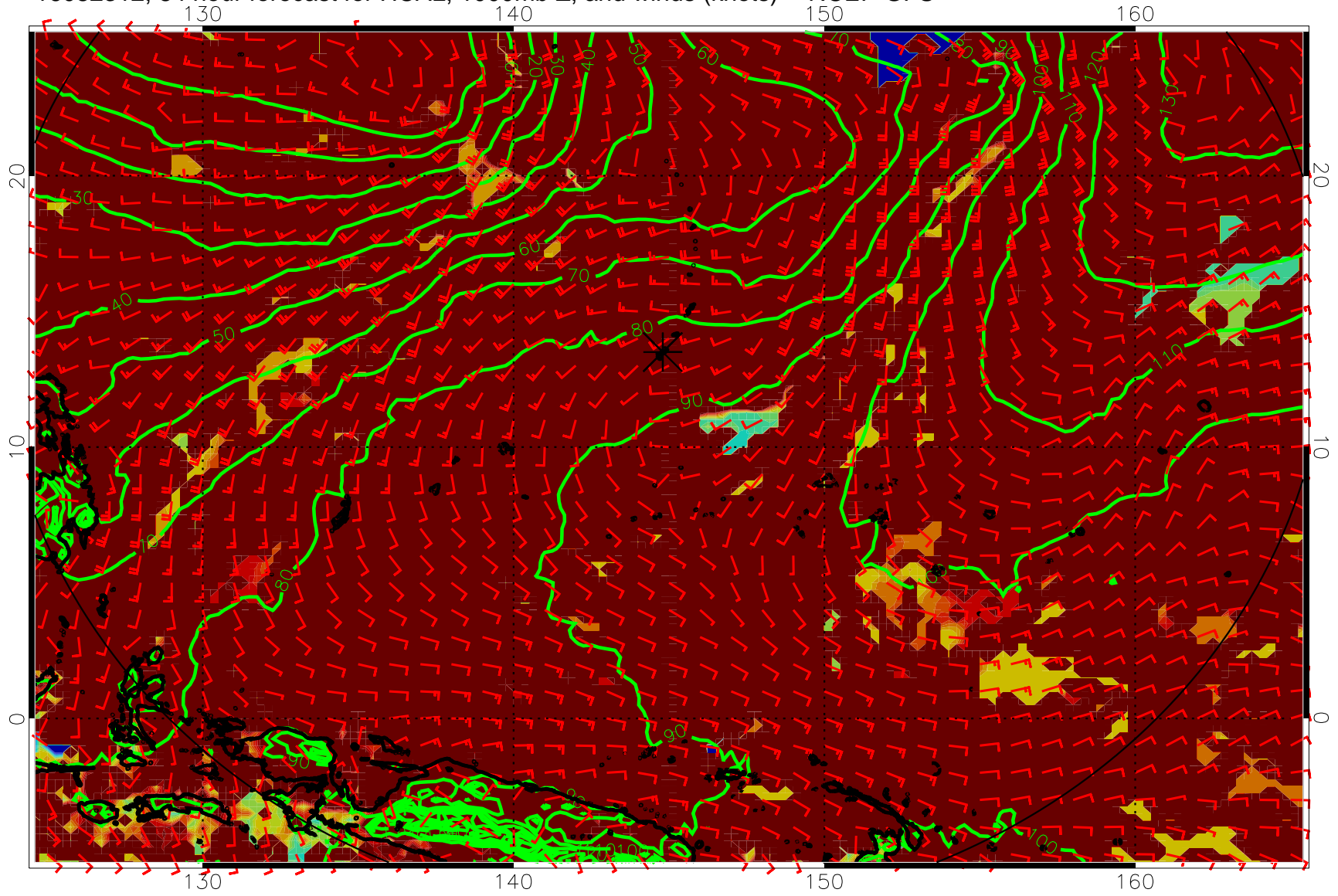
16082312, 84 hour forecast for HCAL, 1000mb Z, and winds (knots) -- NCEP GFS
