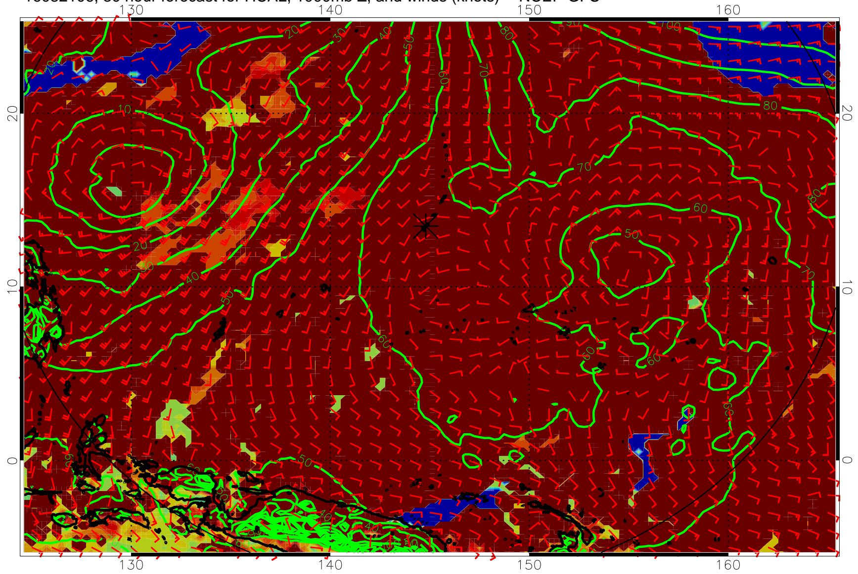
16082106, 30 hour forecast for HCAL, 1000mb Z, and winds (knots) -- NCEP GFS
