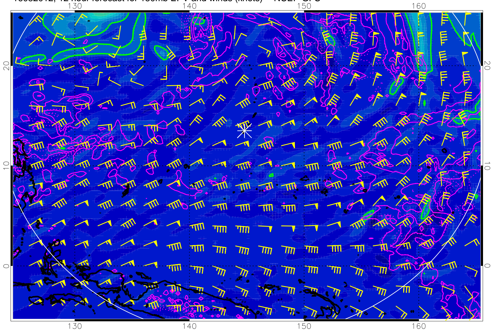
16082012, 12 hour forecast for 150mb EPV and winds (knots) -- NCEP GFS
