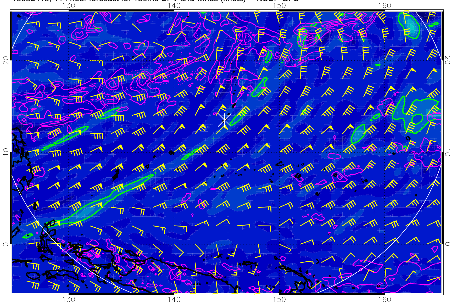
16082418, 114 hour forecast for 150mb EPV and winds (knots) -- NCEP GFS
