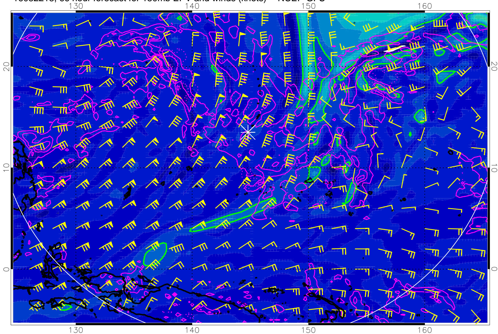
16082218, 66 hour forecast for 150mb EPV and winds (knots) -- NCEP GFS
