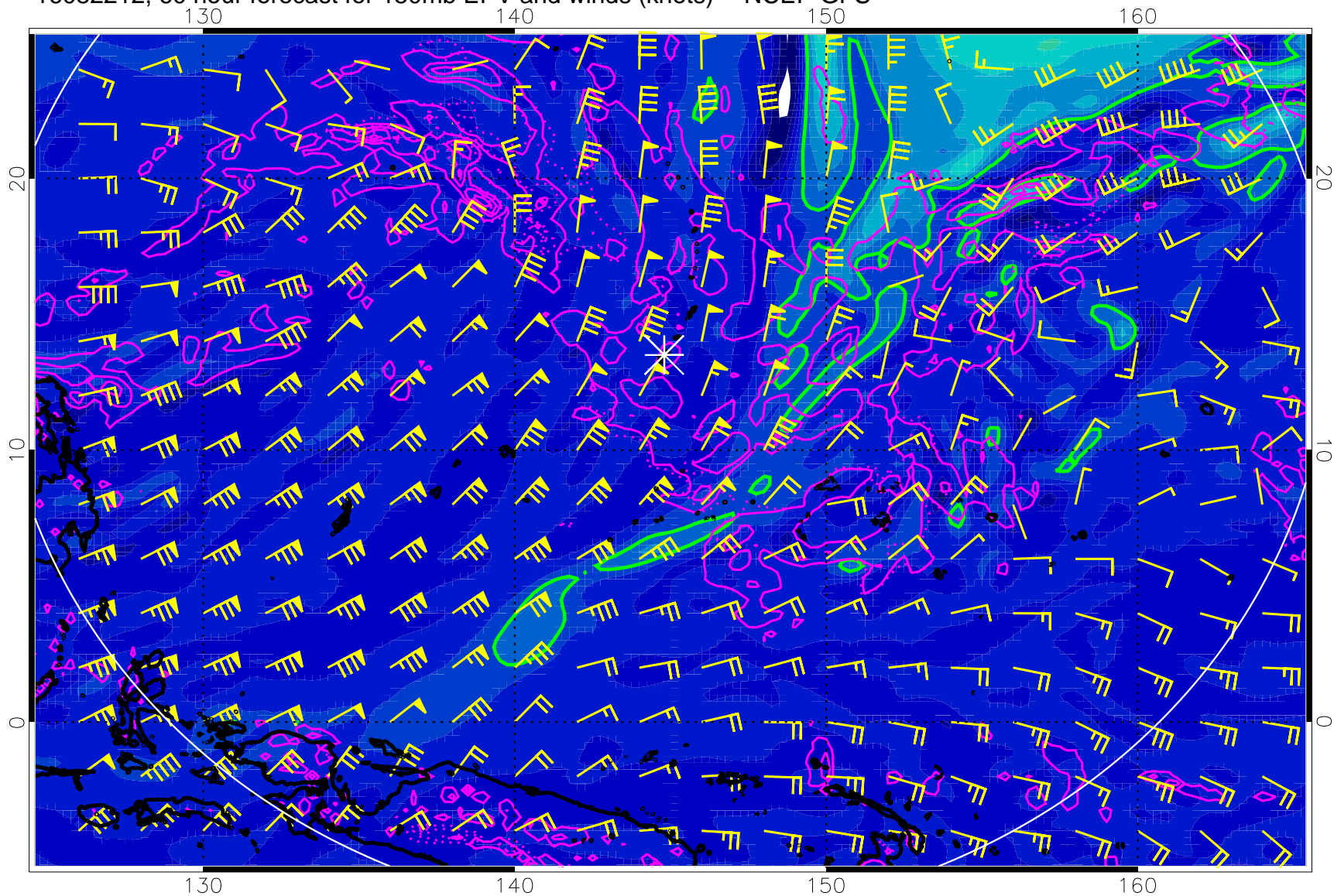
16082212, 60 hour forecast for 150mb EPV and winds (knots) -- NCEP GFS
