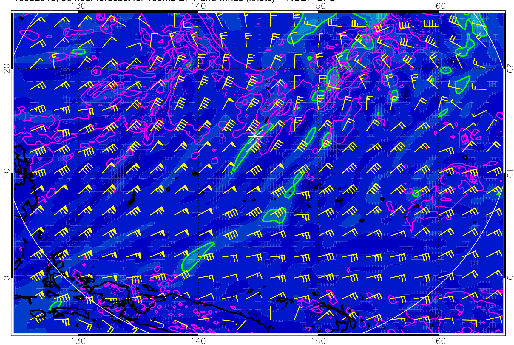
16082318, 90 hour forecast for 150mb EPV and winds (knots) -- NCEP GFS
