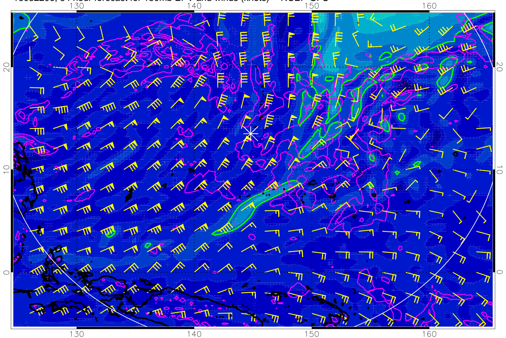
16082206, 54 hour forecast for 150mb EPV and winds (knots) -- NCEP GFS
