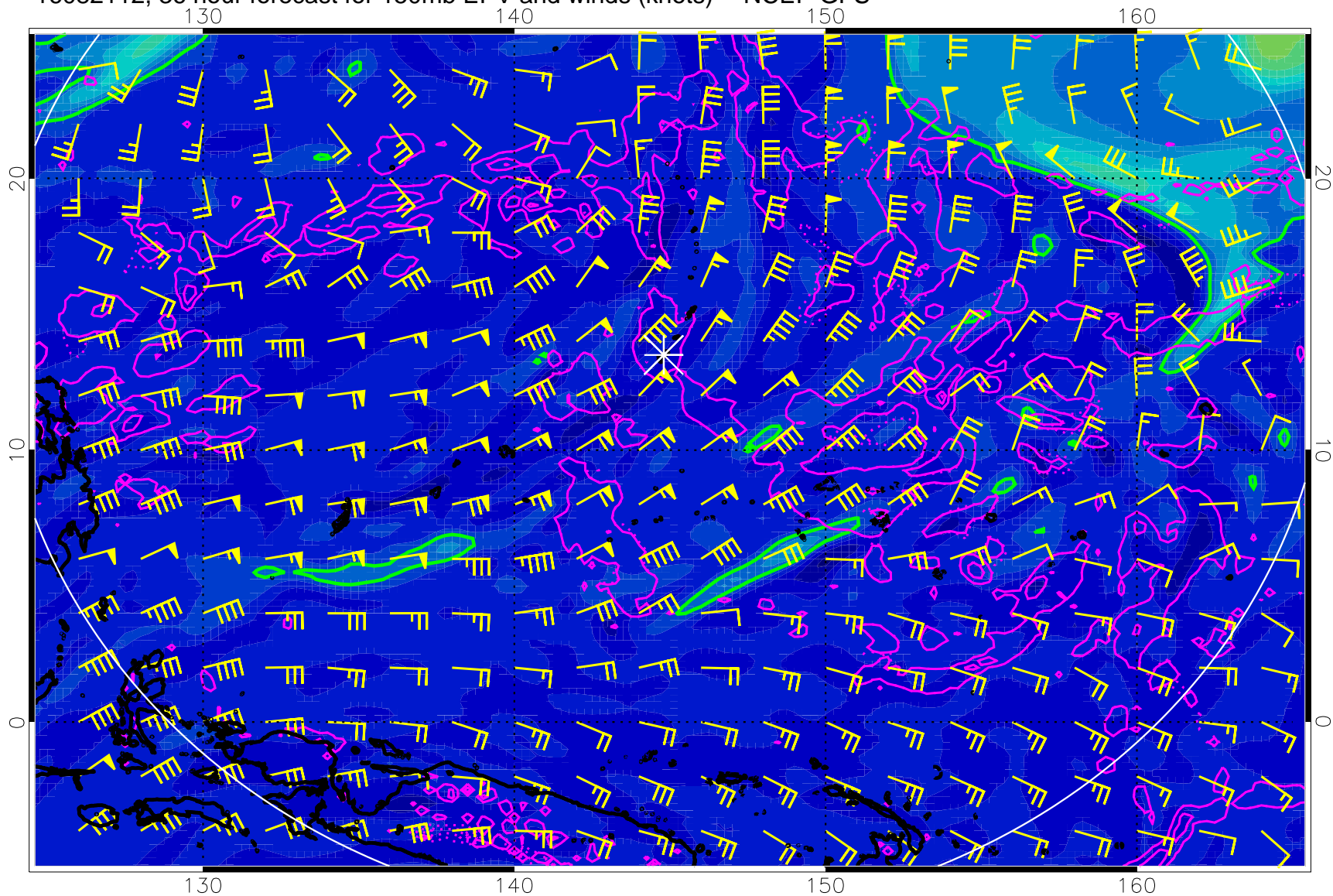
16082112, 36 hour forecast for 150mb EPV and winds (knots) -- NCEP GFS
