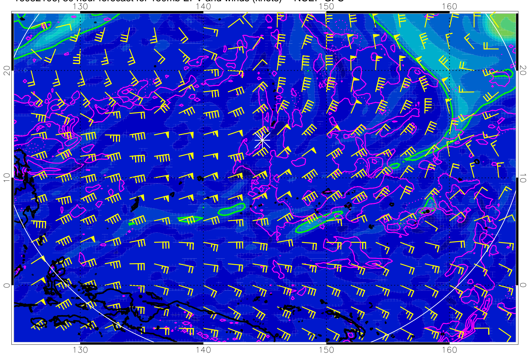
16082106, 30 hour forecast for 150mb EPV and winds (knots) -- NCEP GFS
