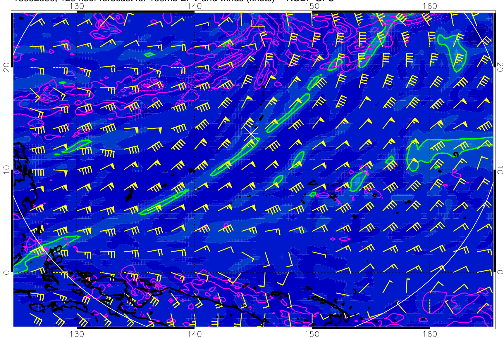
16082500, 120 hour forecast for 150mb EPV and winds (knots) -- NCEP GFS
