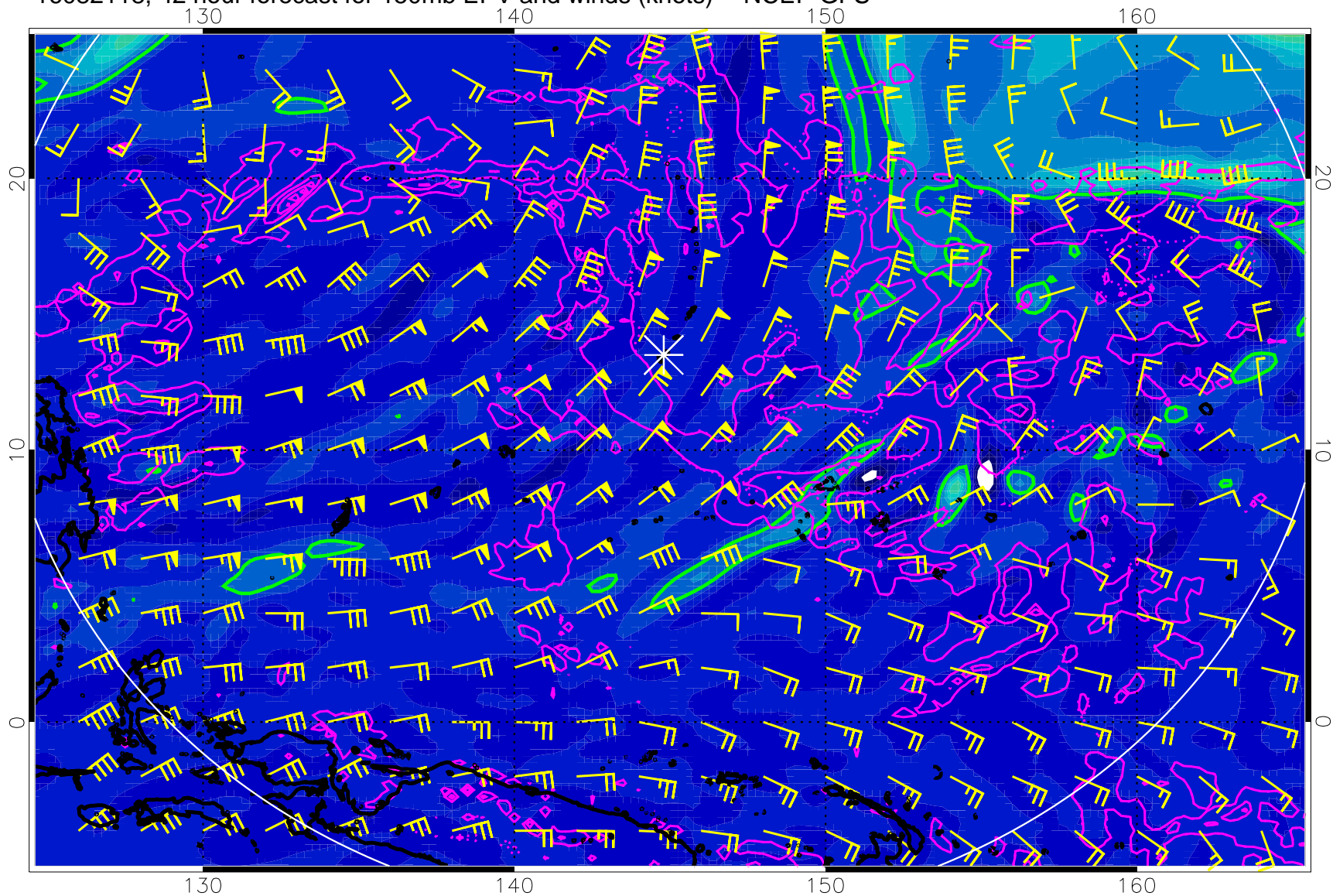
16082118, 42 hour forecast for 150mb EPV and winds (knots) -- NCEP GFS
