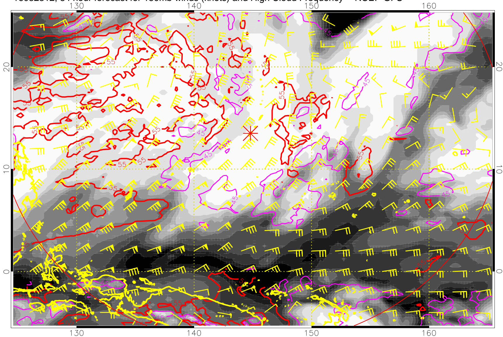
16082312, 84 hour forecast for 150mb winds (knots) and High Cloud Frequency -- NCEP GFS
