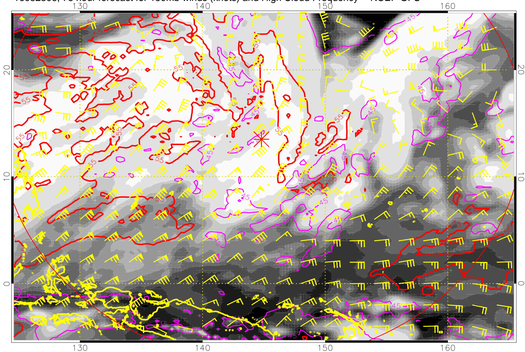
16082306, 78 hour forecast for 150mb winds (knots) and High Cloud Frequency -- NCEP GFS
