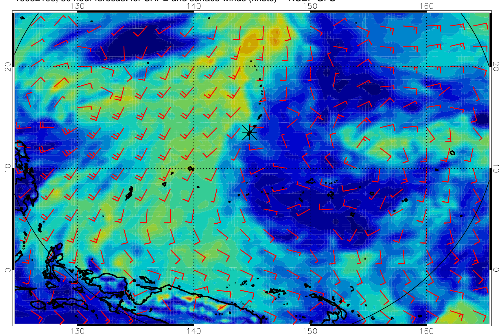
16082106, 30 hour forecast for CAPE and surface winds (knots) -- NCEP GFS
