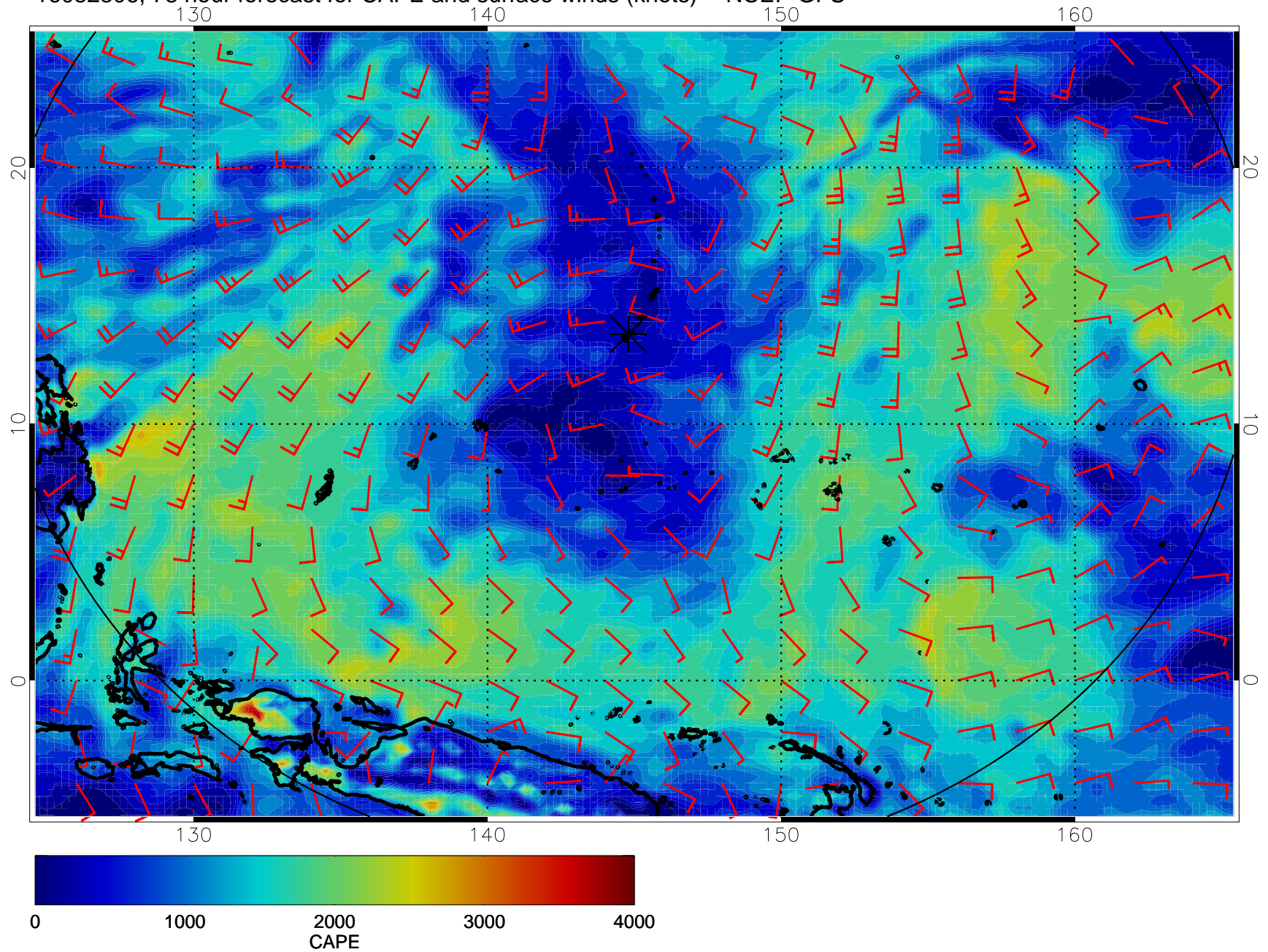
16082306, 78 hour forecast for CAPE and surface winds (knots) -- NCEP GFS
