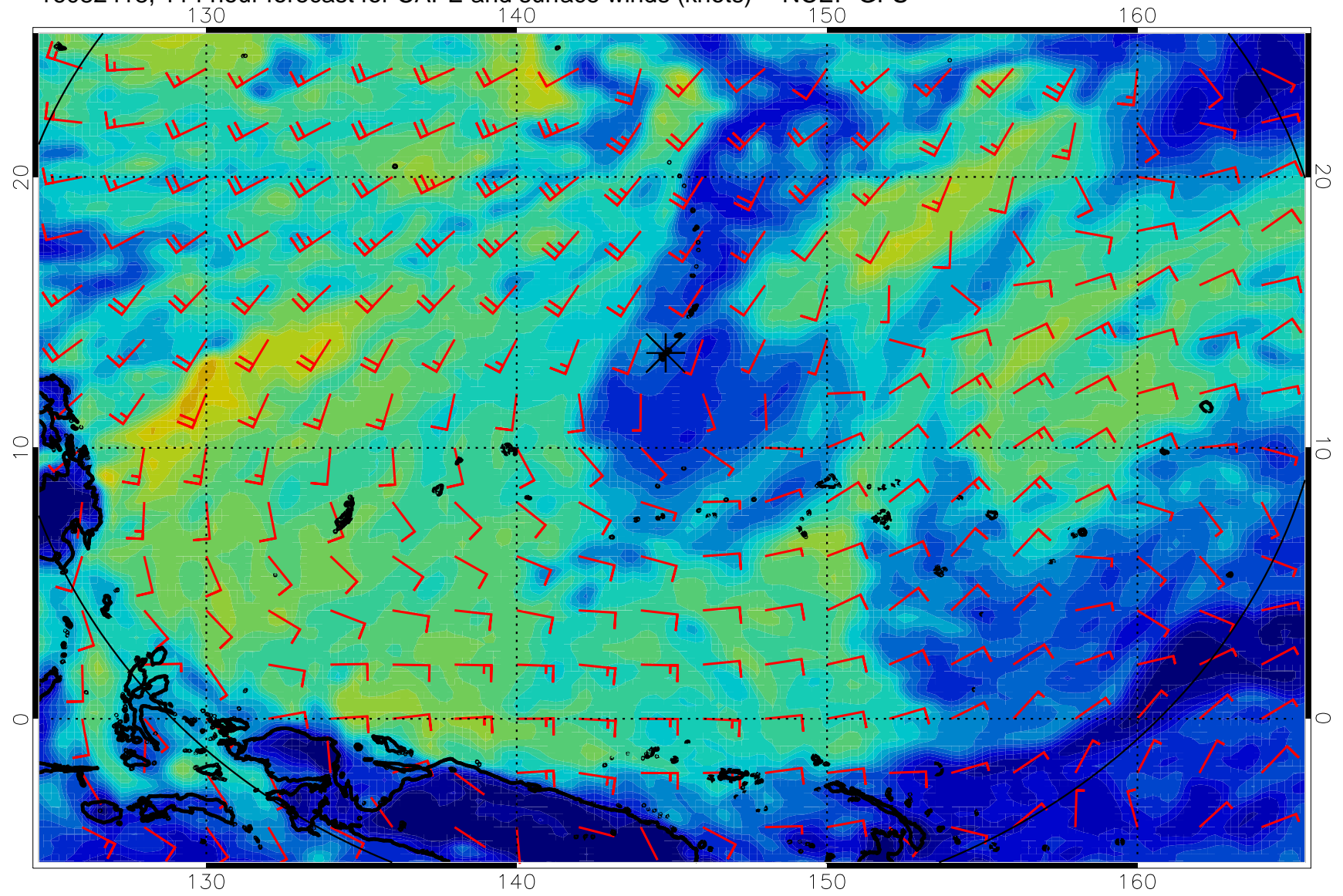
16082418, 114 hour forecast for CAPE and surface winds (knots) -- NCEP GFS
