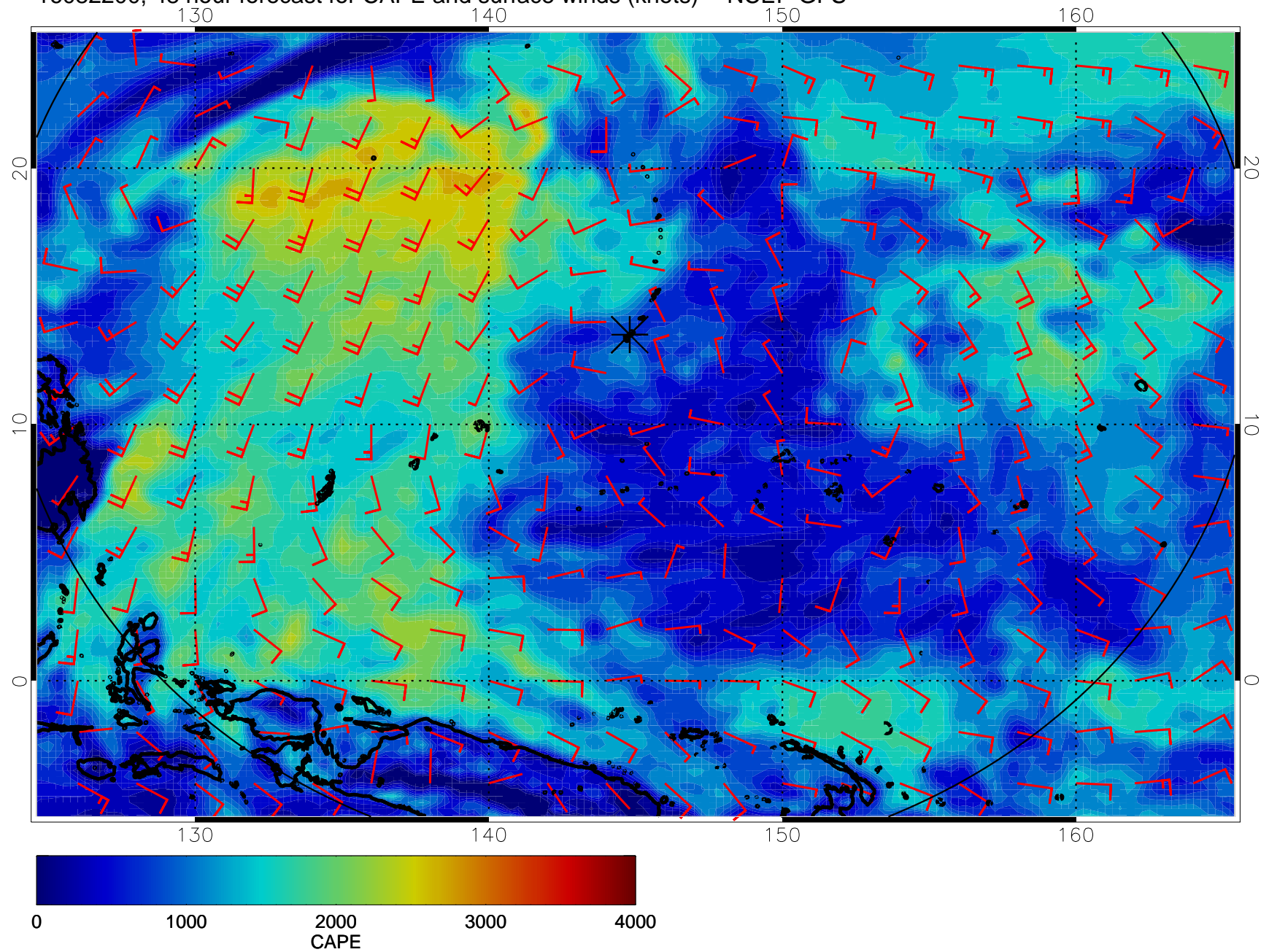
16082200, 48 hour forecast for CAPE and surface winds (knots) -- NCEP GFS
