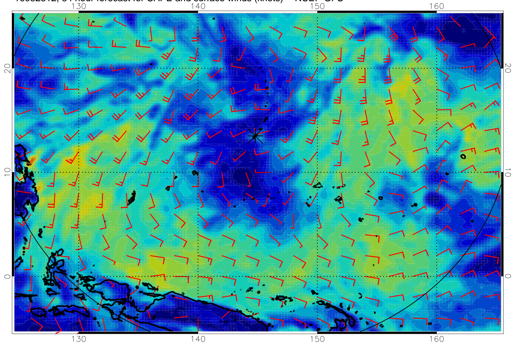
16082312, 84 hour forecast for CAPE and surface winds (knots) -- NCEP GFS
