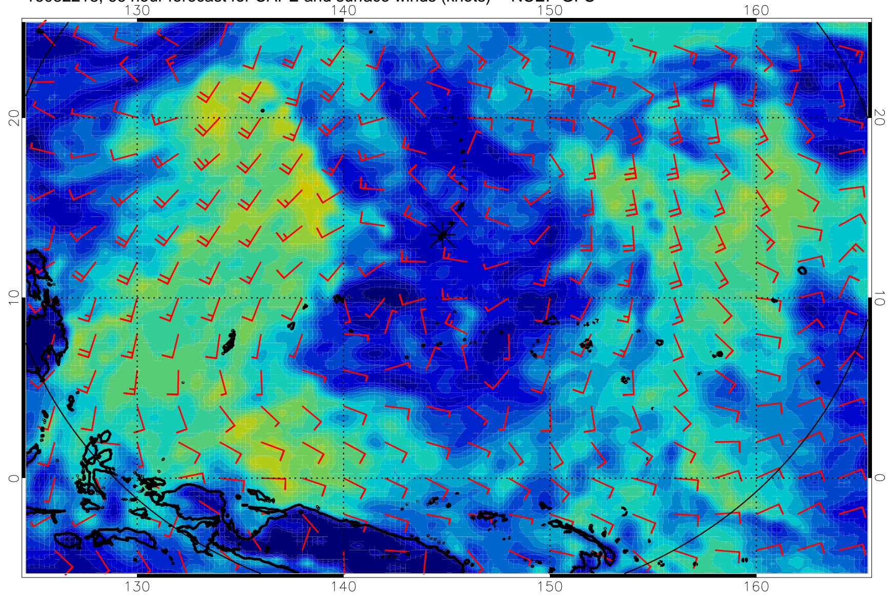
16082218, 66 hour forecast for CAPE and surface winds (knots) -- NCEP GFS
