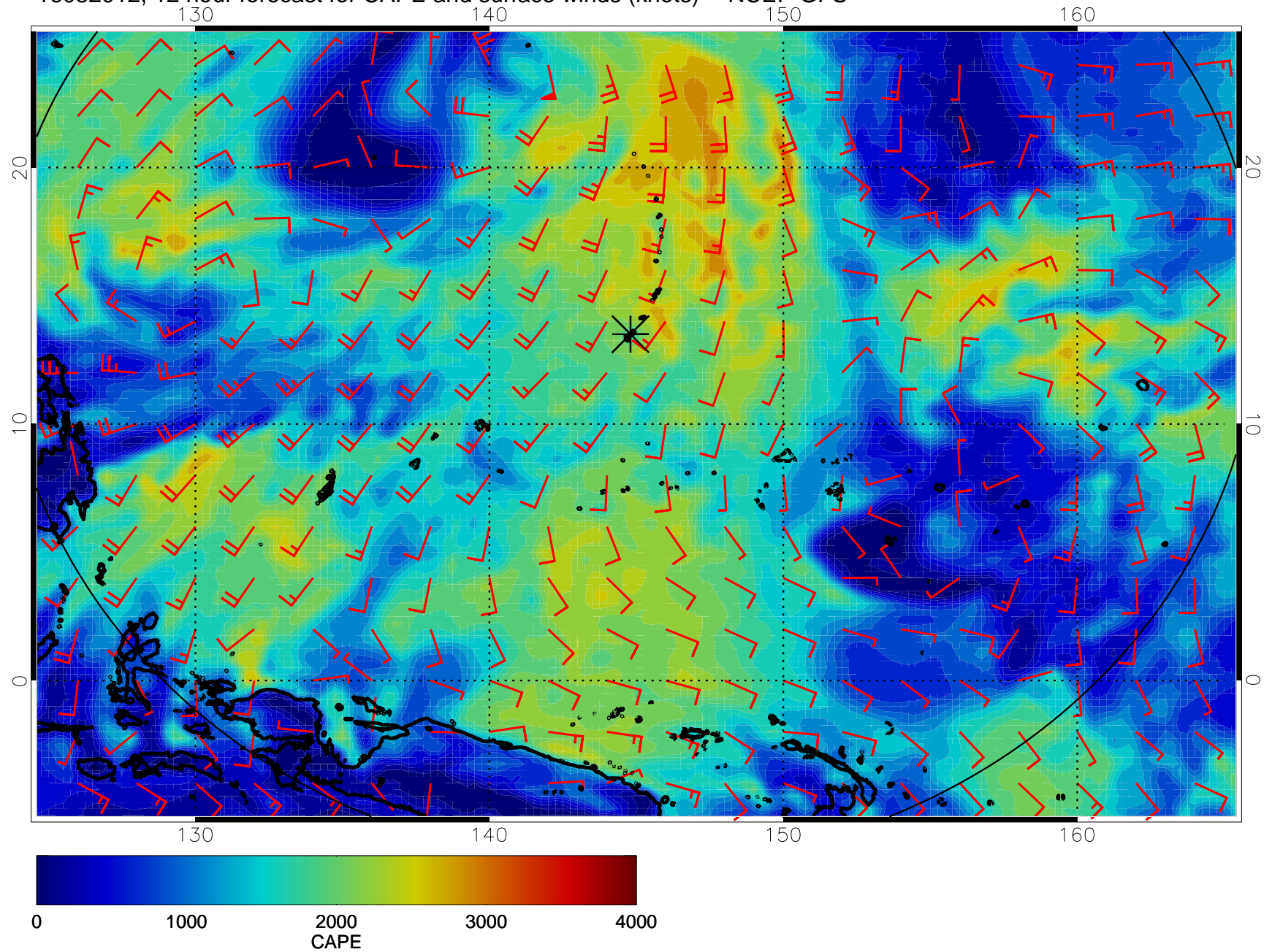
16082012, 12 hour forecast for CAPE and surface winds (knots) -- NCEP GFS
