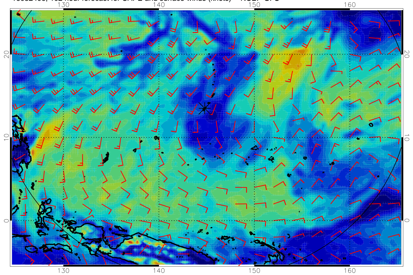
16082406, 102 hour forecast for CAPE and surface winds (knots) -- NCEP GFS
