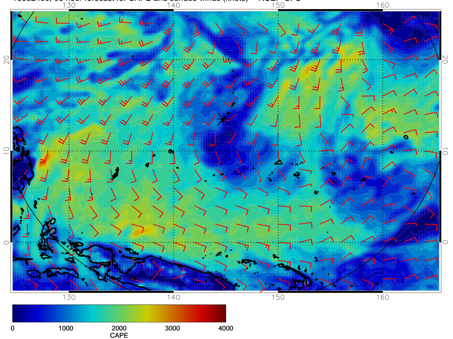
16082400, 96 hour forecast for CAPE and surface winds (knots) -- NCEP GFS
