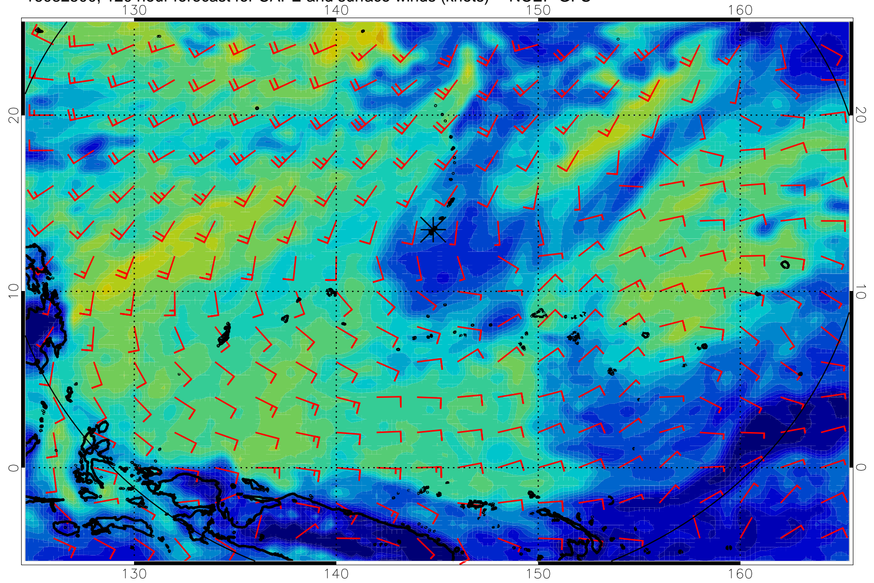
16082500, 120 hour forecast for CAPE and surface winds (knots) -- NCEP GFS
