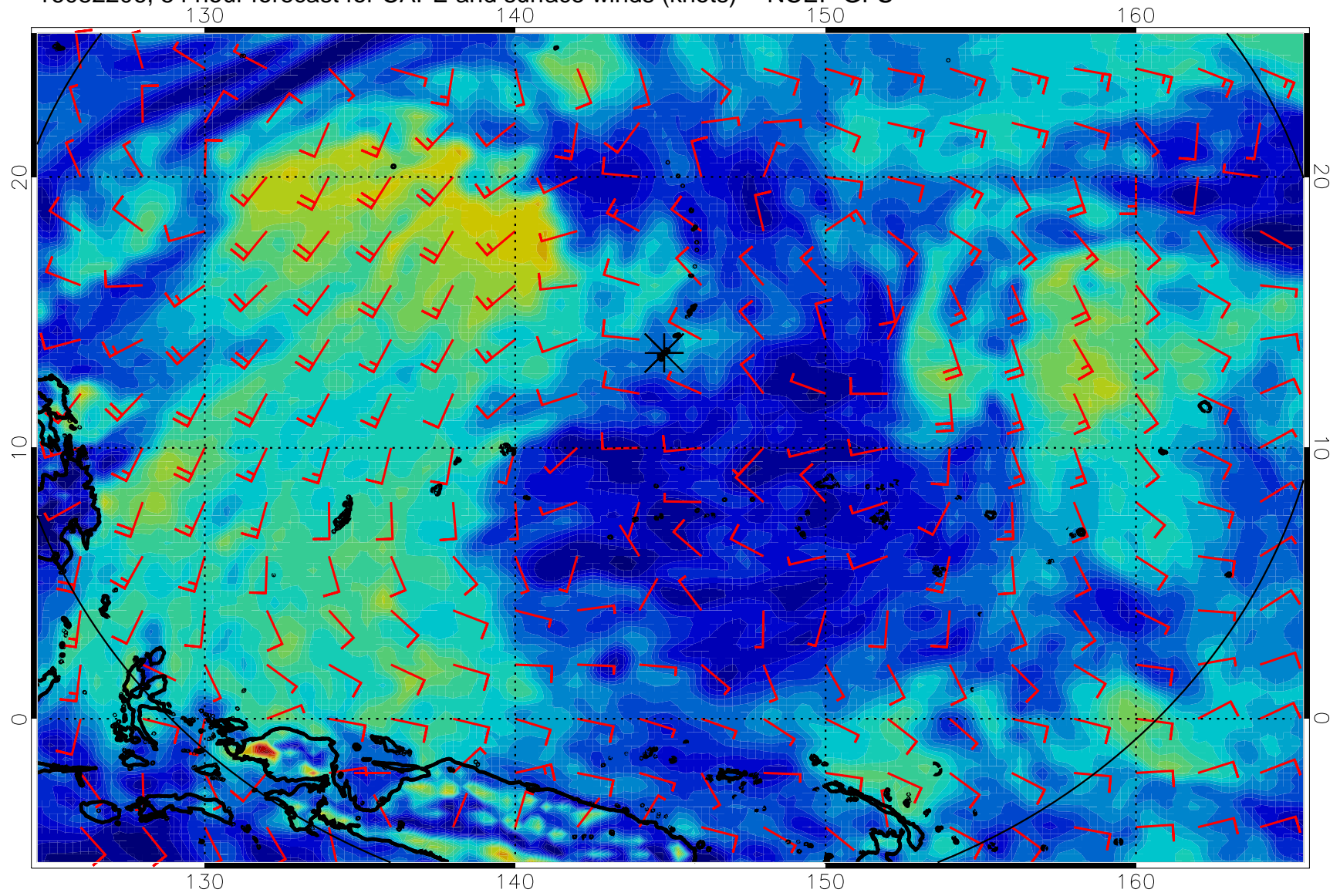
16082206, 54 hour forecast for CAPE and surface winds (knots) -- NCEP GFS
