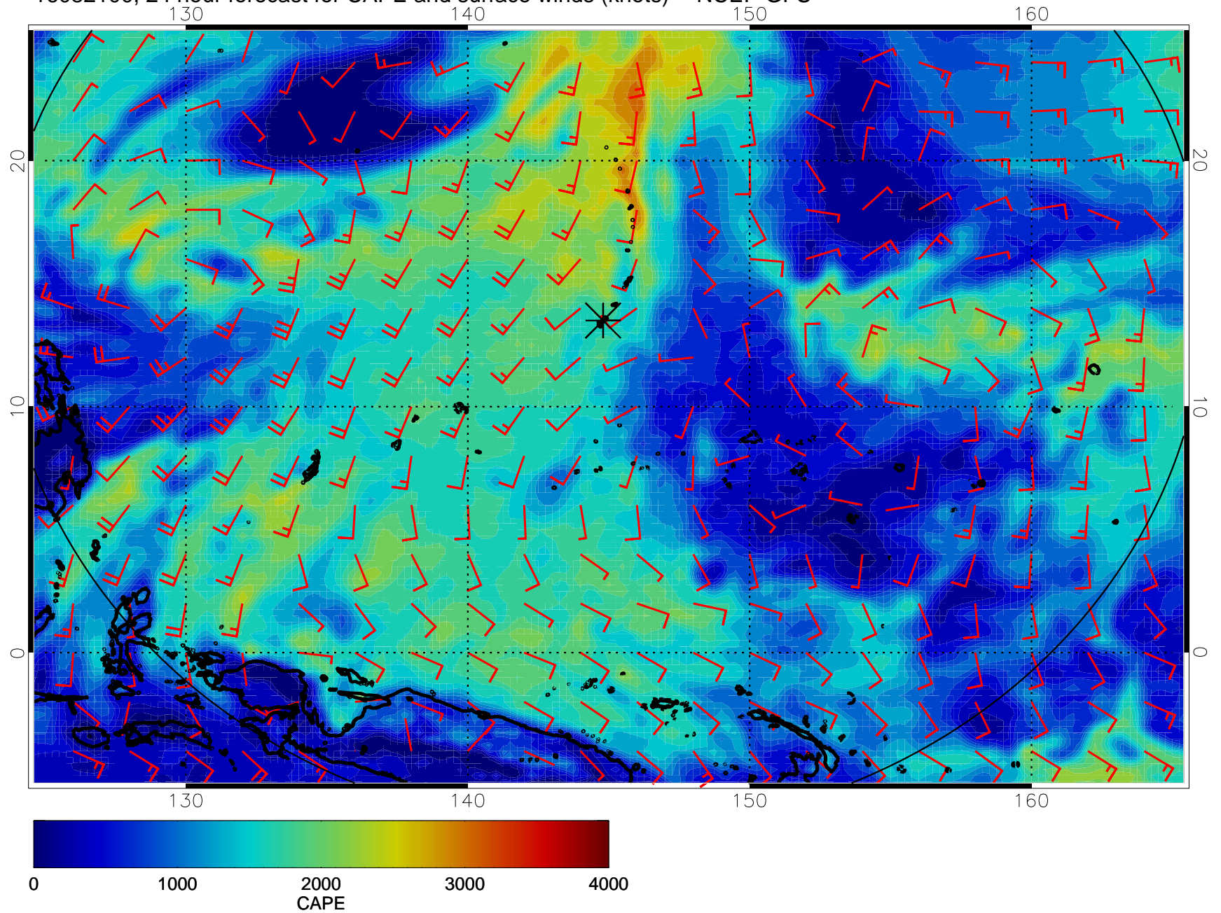
16082100, 24 hour forecast for CAPE and surface winds (knots) -- NCEP GFS
