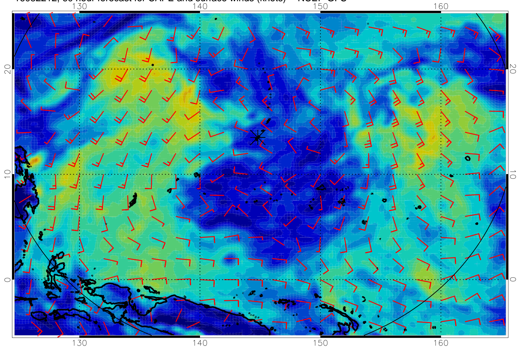
16082212, 60 hour forecast for CAPE and surface winds (knots) -- NCEP GFS
