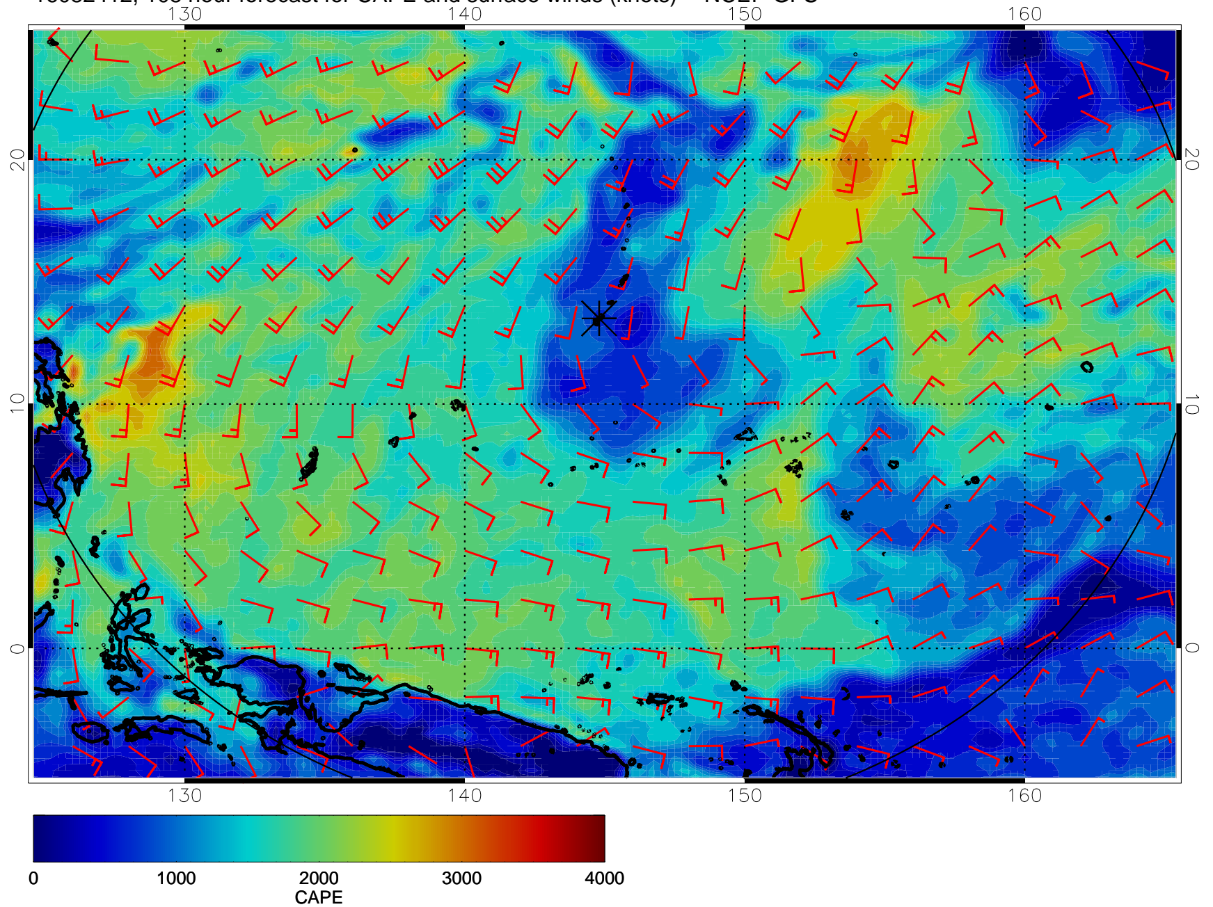
16082412, 108 hour forecast for CAPE and surface winds (knots) -- NCEP GFS
