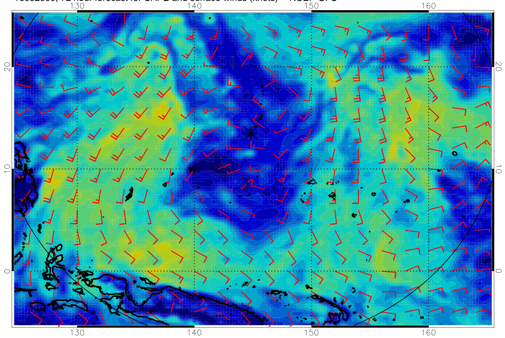
16082300, 72 hour forecast for CAPE and surface winds (knots) -- NCEP GFS
