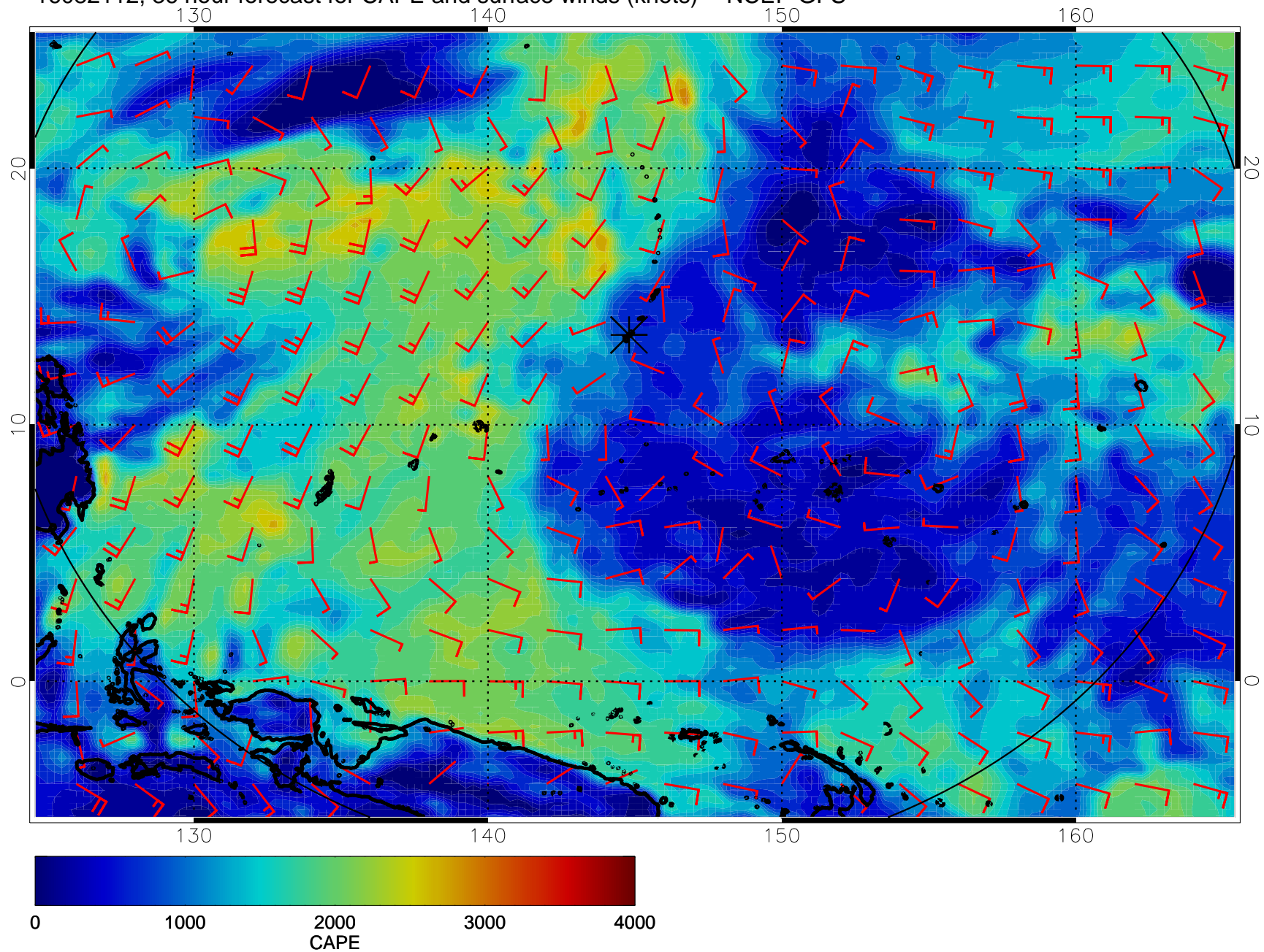
16082112, 36 hour forecast for CAPE and surface winds (knots) -- NCEP GFS
