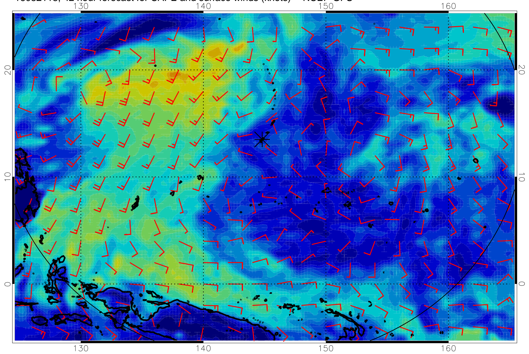
16082118, 42 hour forecast for CAPE and surface winds (knots) -- NCEP GFS
