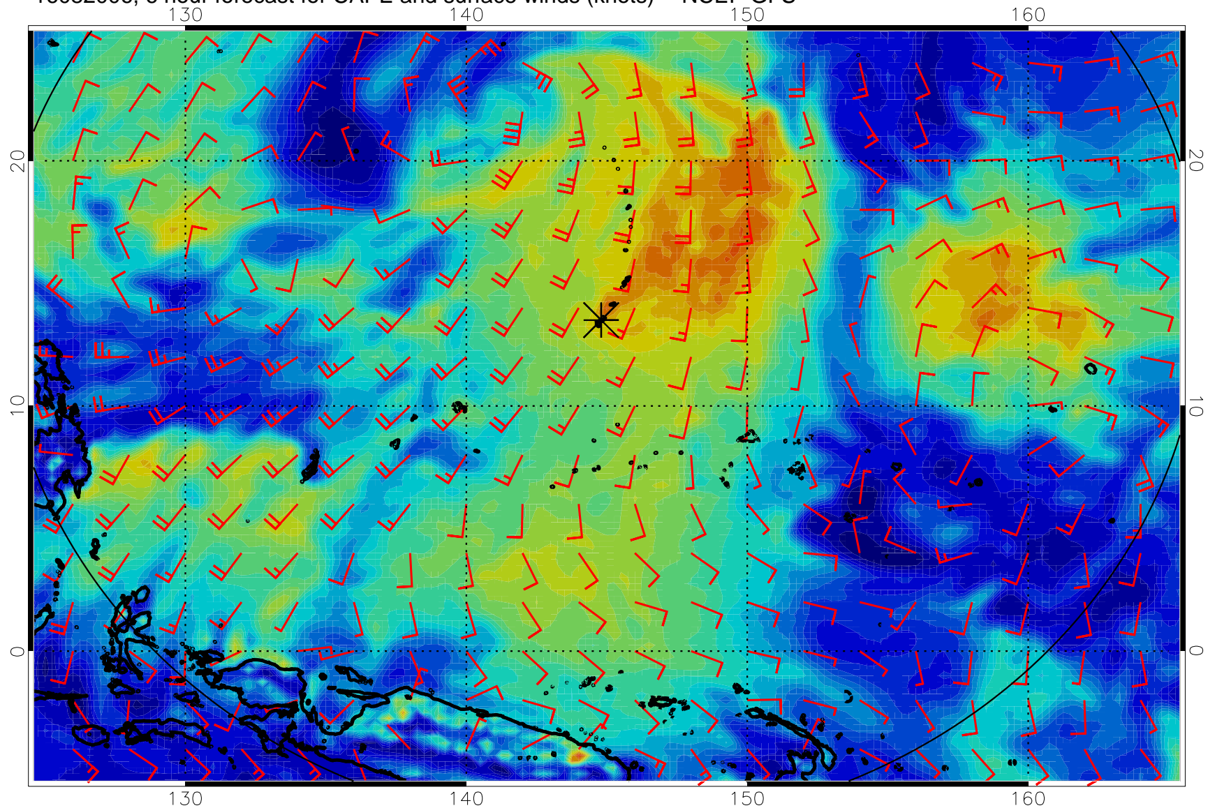
16082006, 6 hour forecast for CAPE and surface winds (knots) -- NCEP GFS
