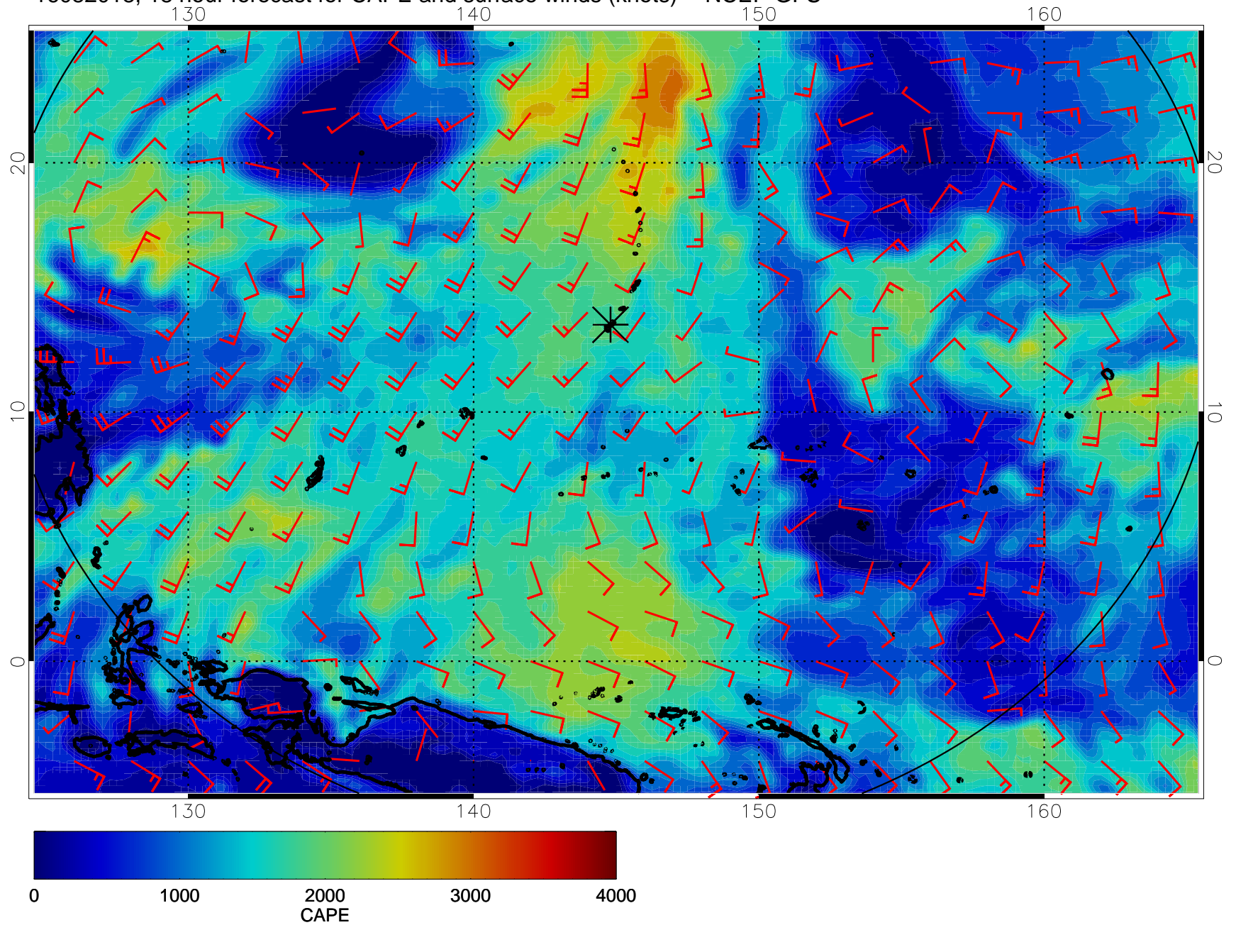
16082018, 18 hour forecast for CAPE and surface winds (knots) -- NCEP GFS
