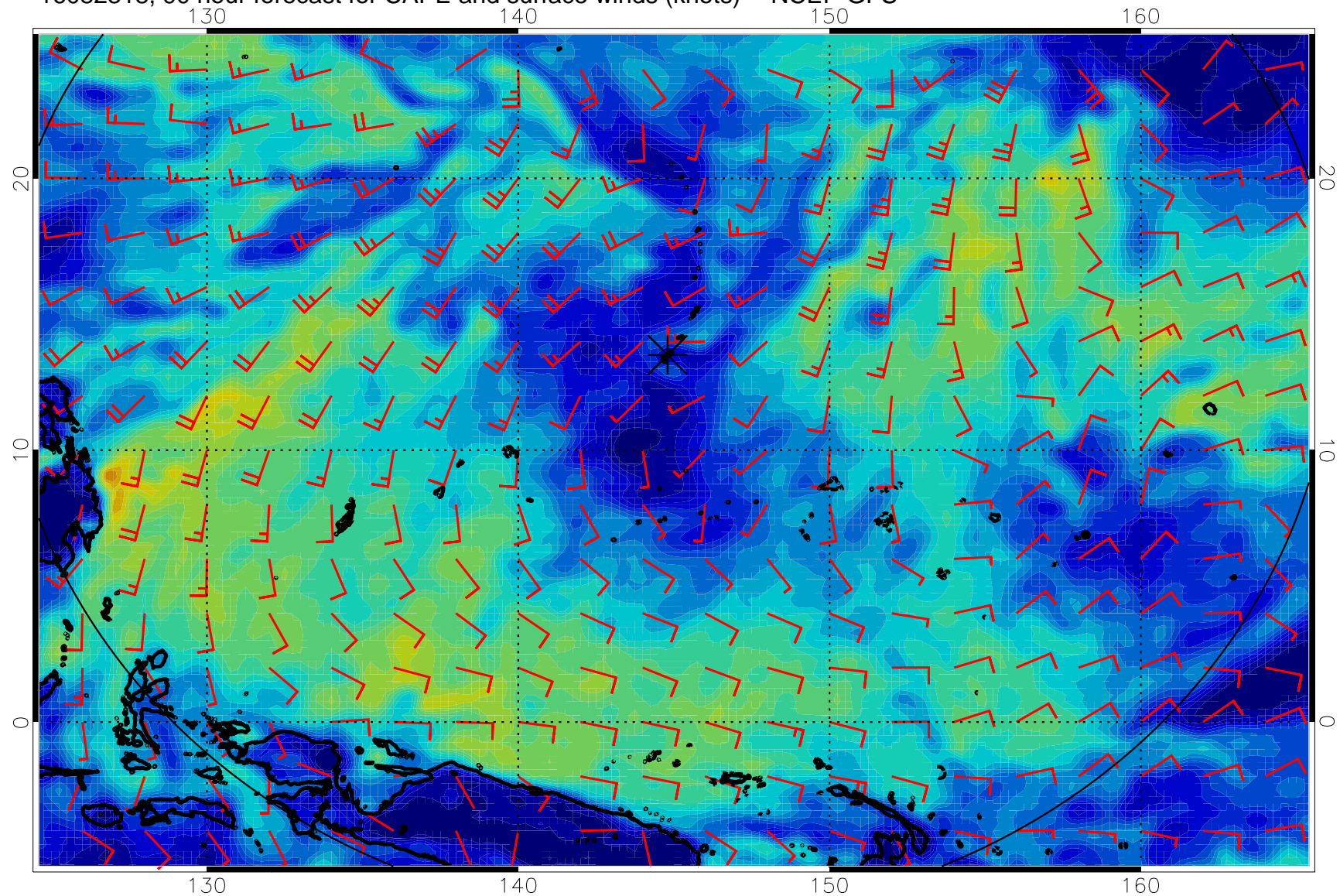
16082318, 90 hour forecast for CAPE and surface winds (knots) -- NCEP GFS
