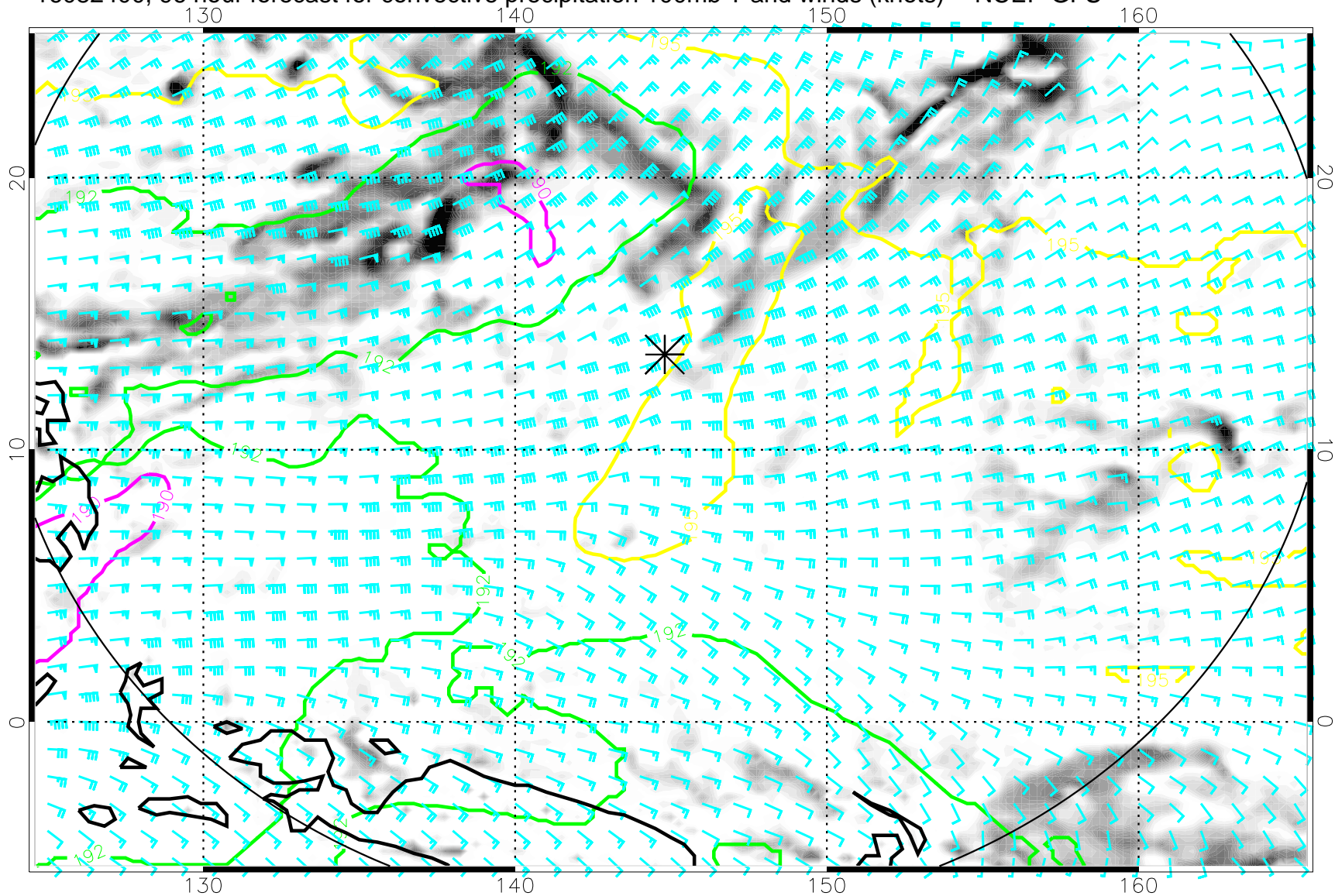
16082400, 96 hour forecast for convective precipitation 100mb T and winds (knots) -- NCEP GFS
