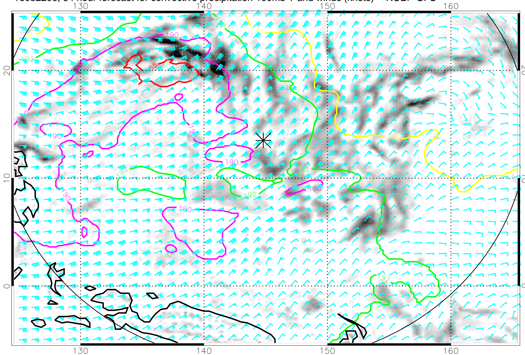
16082206, 54 hour forecast for convective precipitation 100mb T and winds (knots) -- NCEP GFS
