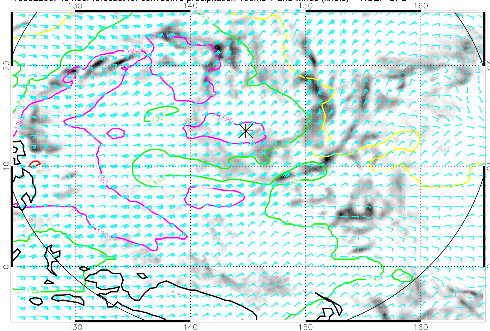
16082200, 48 hour forecast for convective precipitation 100mb T and winds (knots) -- NCEP GFS
