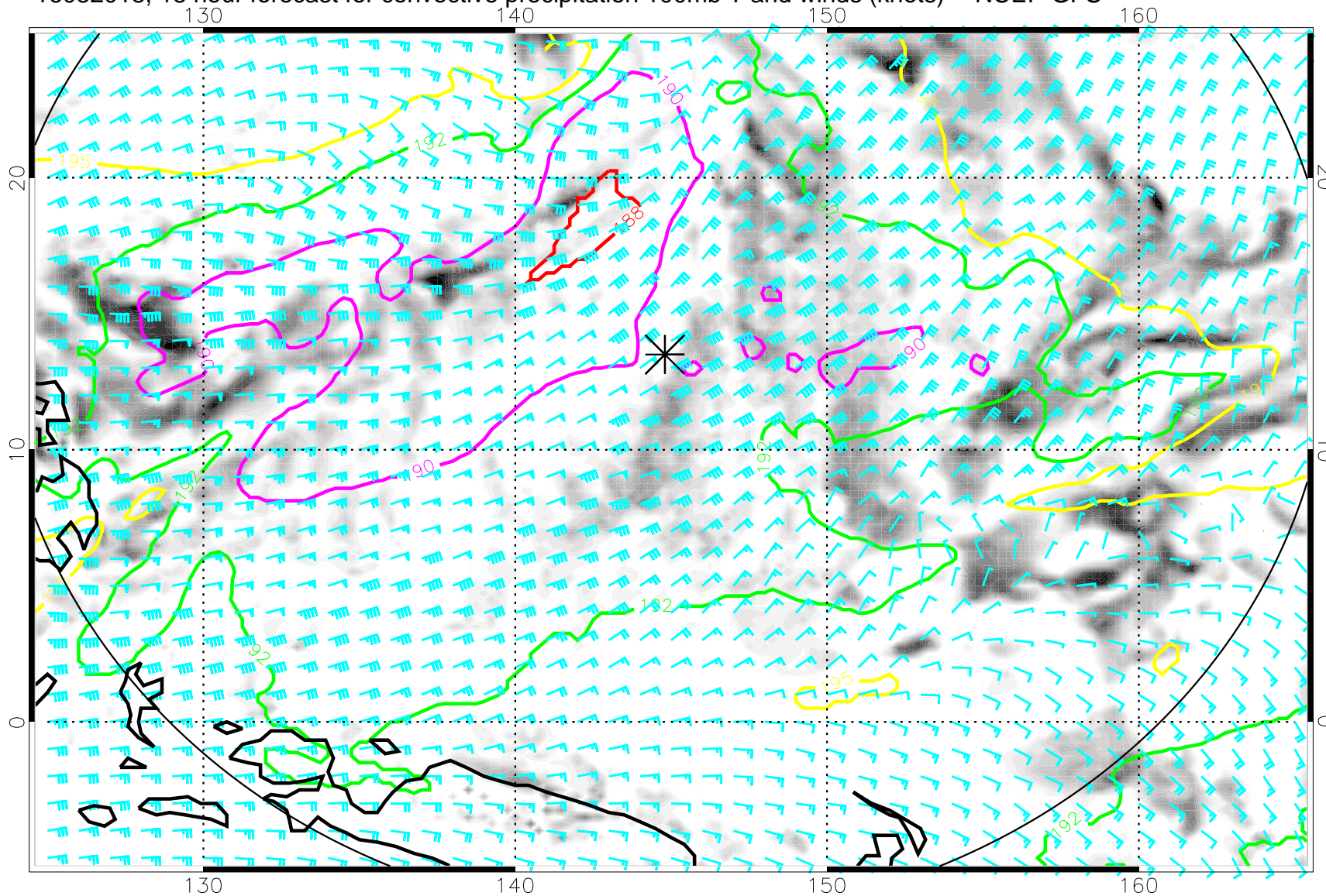
16082018, 18 hour forecast for convective precipitation 100mb T and winds (knots) -- NCEP GFS
