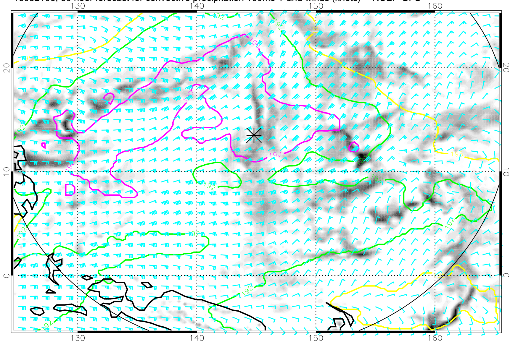
16082106, 30 hour forecast for convective precipitation 100mb T and winds (knots) -- NCEP GFS
