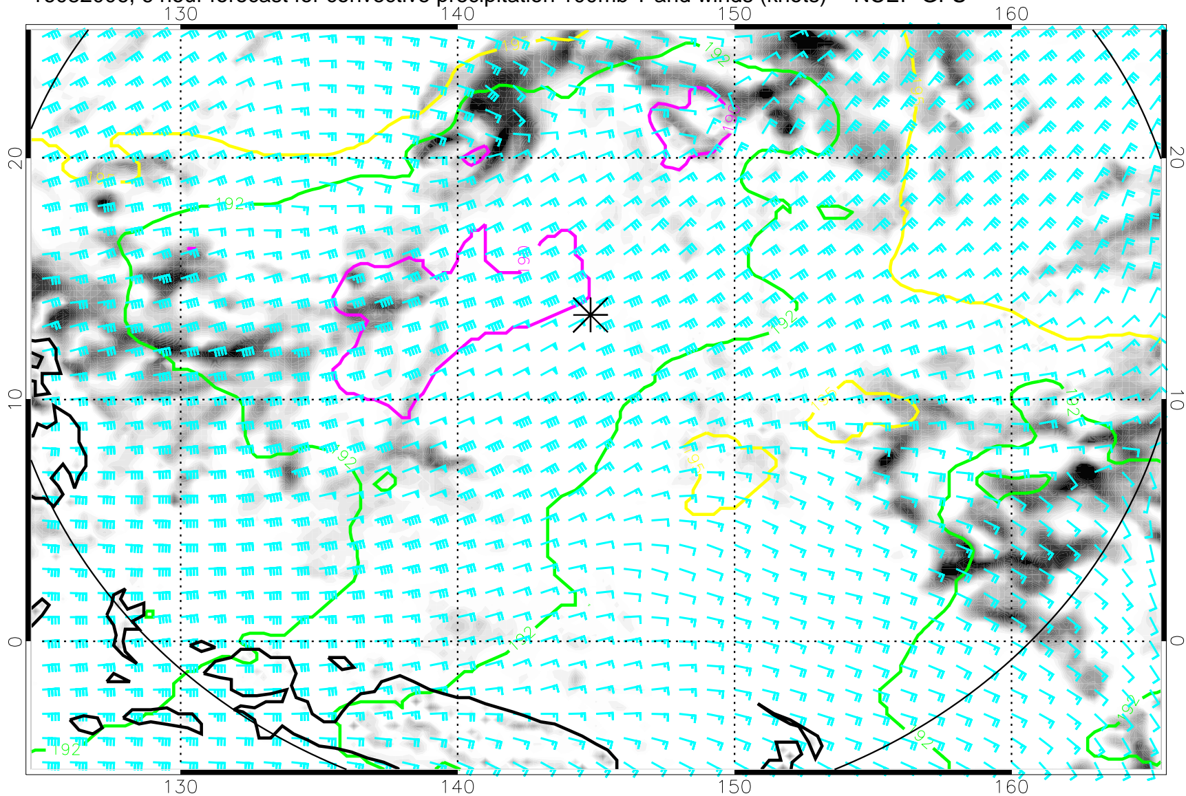
16082006, 6 hour forecast for convective precipitation 100mb T and winds (knots) -- NCEP GFS
