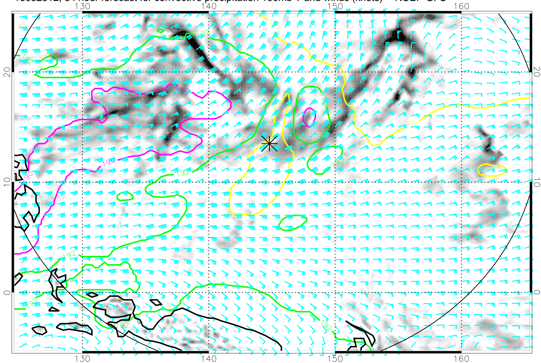
16082312, 84 hour forecast for convective precipitation 100mb T and winds (knots) -- NCEP GFS
