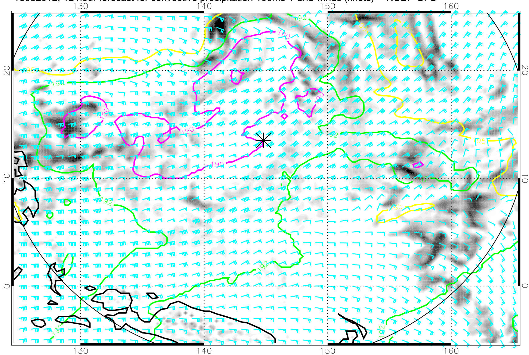
16082012, 12 hour forecast for convective precipitation 100mb T and winds (knots) -- NCEP GFS
