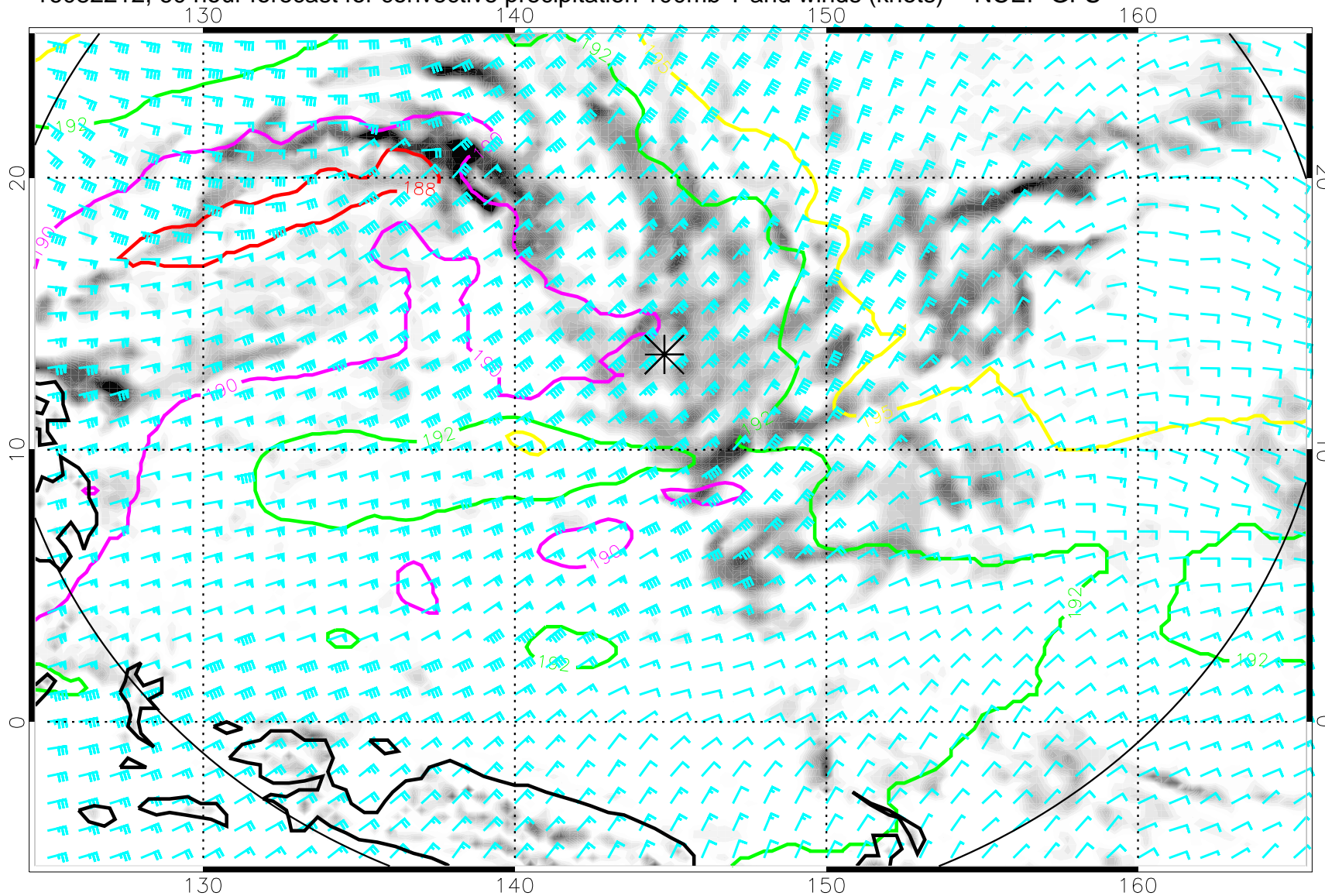
16082212, 60 hour forecast for convective precipitation 100mb T and winds (knots) -- NCEP GFS
