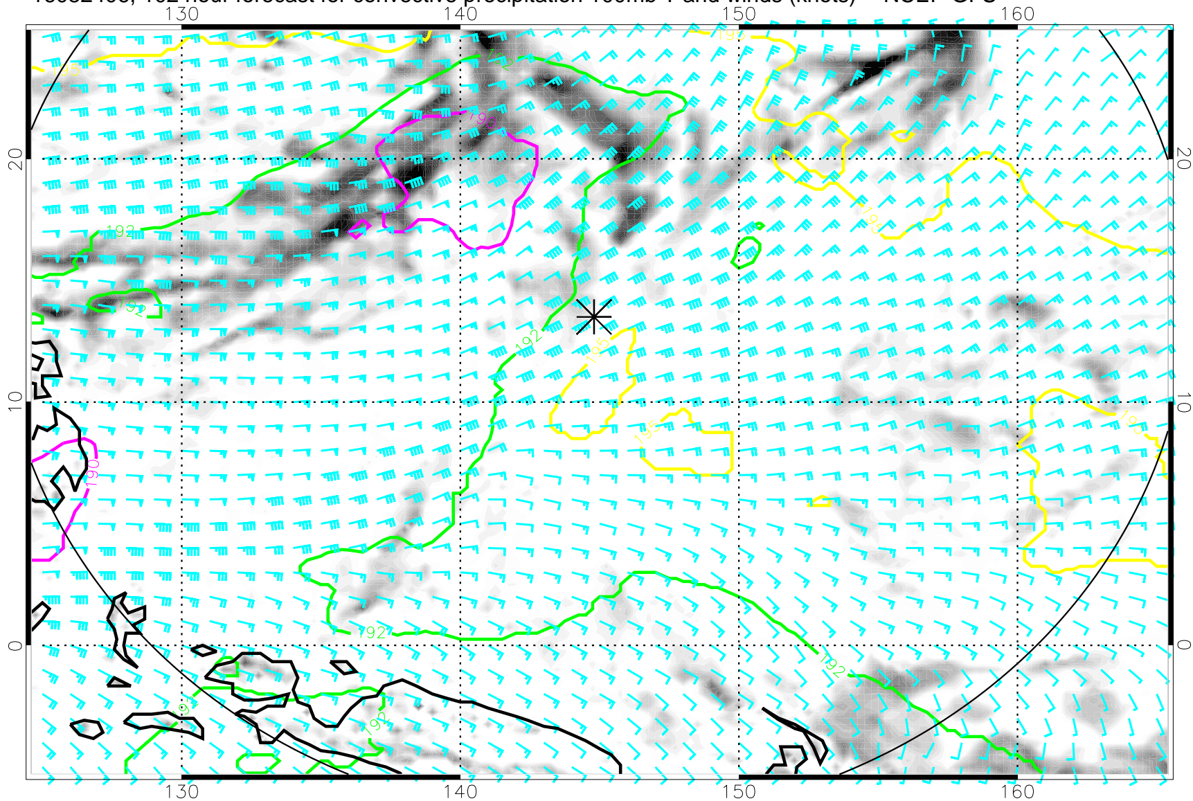
16082406, 102 hour forecast for convective precipitation 100mb T and winds (knots) -- NCEP GFS
