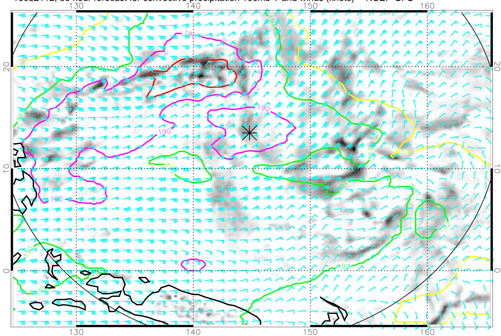
16082112, 36 hour forecast for convective precipitation 100mb T and winds (knots) -- NCEP GFS
