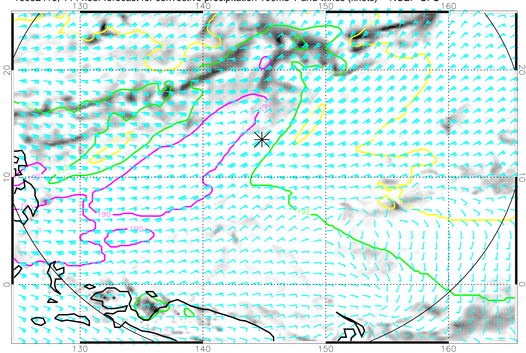
16082418, 114 hour forecast for convective precipitation 100mb T and winds (knots) -- NCEP GFS
