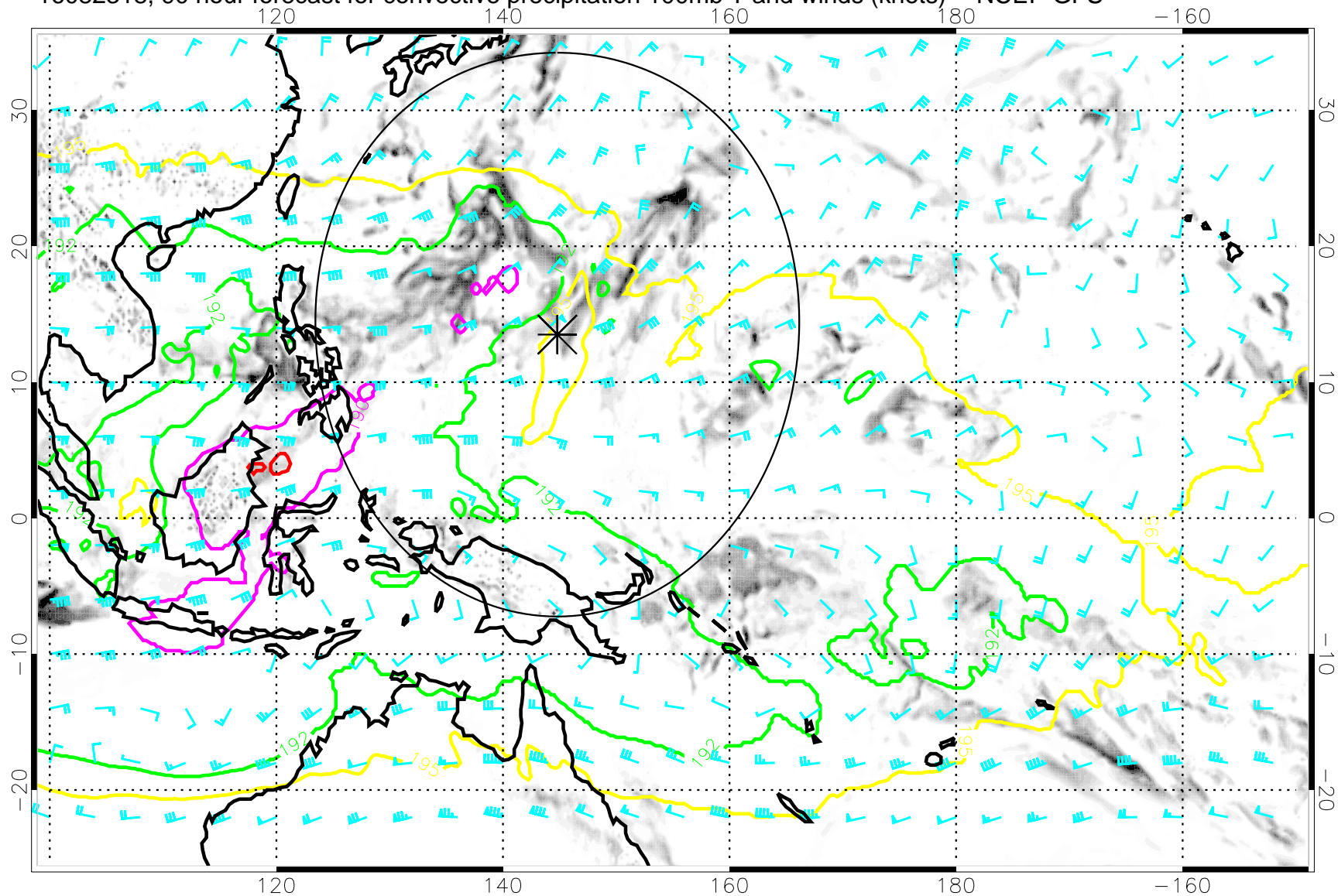
16082318, 90 hour forecast for convective precipitation 100mb T and winds (knots) -- NCEP GFS
