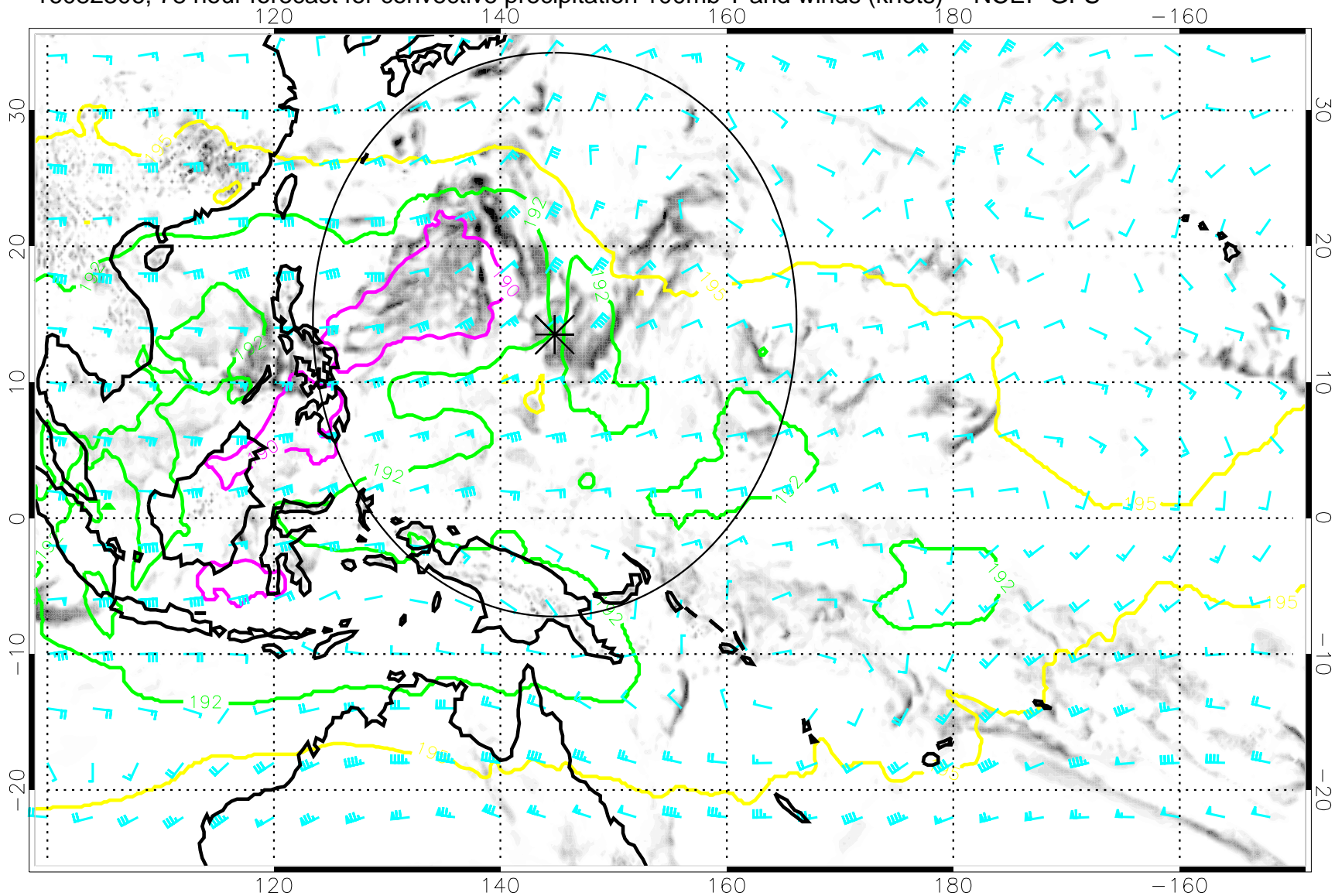
16082306, 78 hour forecast for convective precipitation 100mb T and winds (knots) -- NCEP GFS
