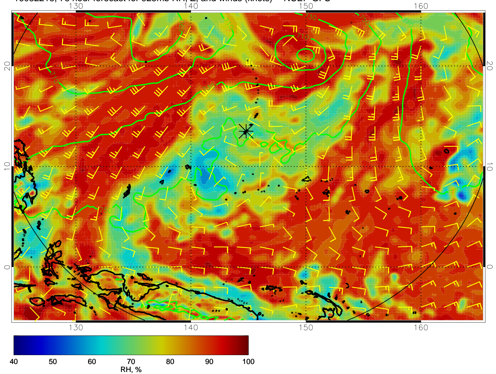
16082218, 78 hour forecast for 925mb RH, Z, and winds (knots) -- NCEP GFS
