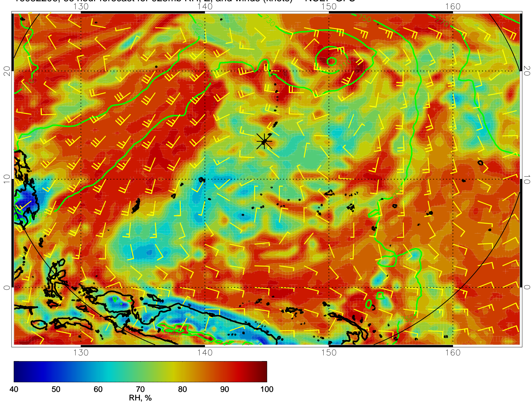
16082206, 66 hour forecast for 925mb RH, Z, and winds (knots) -- NCEP GFS
