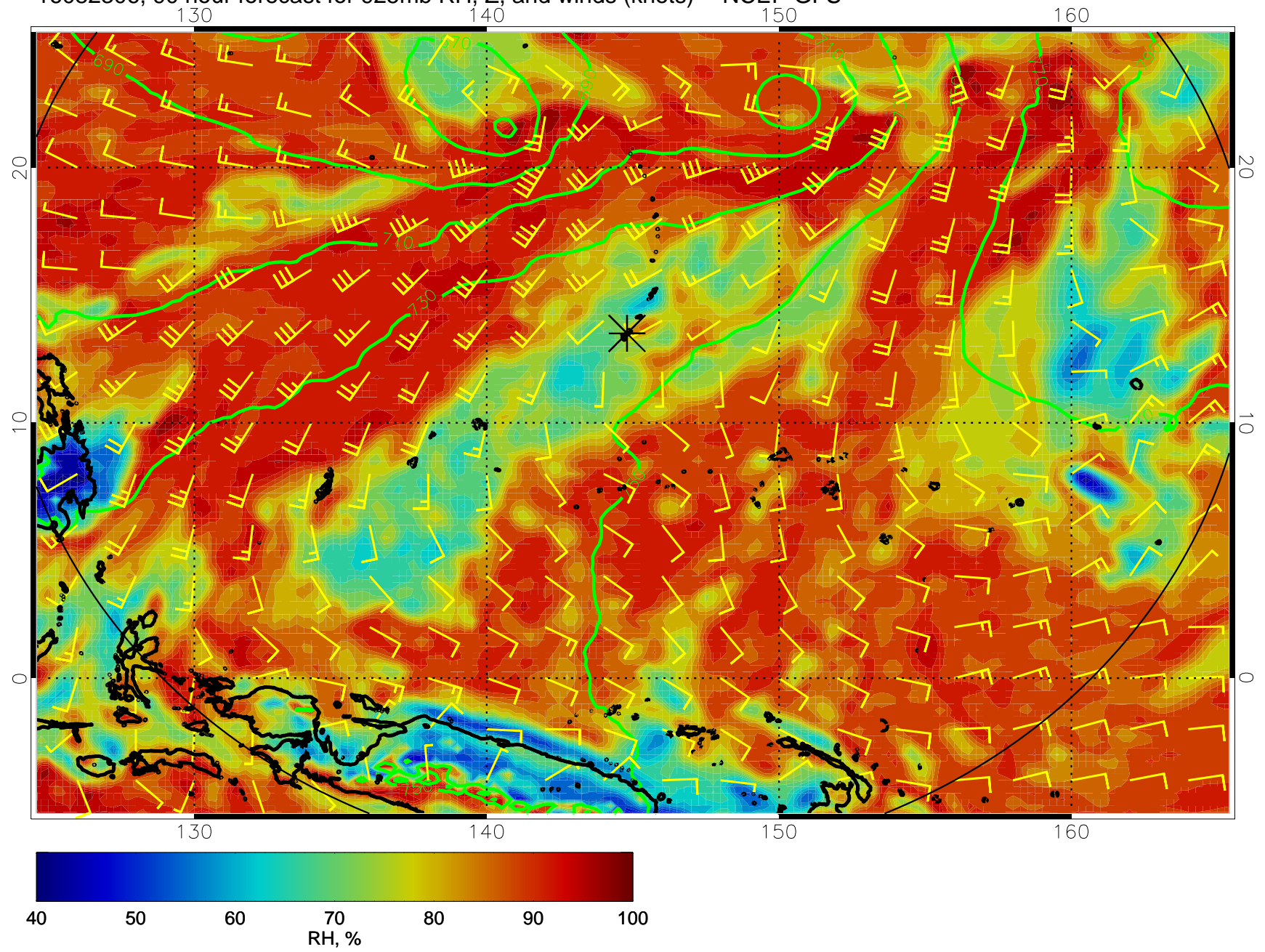
16082306, 90 hour forecast for 925mb RH, Z, and winds (knots) -- NCEP GFS
