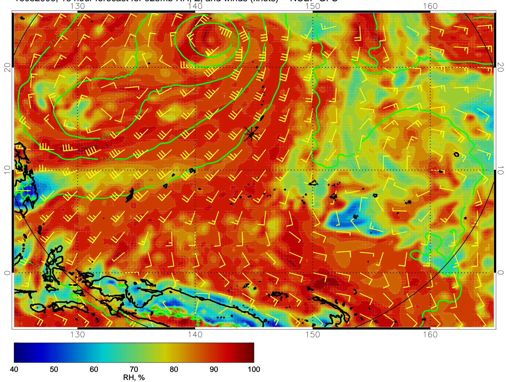
16082006, 18 hour forecast for 925mb RH, Z, and winds (knots) -- NCEP GFS
