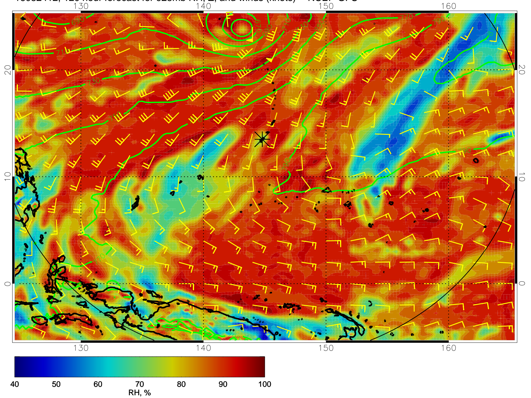
16082412, 120 hour forecast for 925mb RH, Z, and winds (knots) -- NCEP GFS
