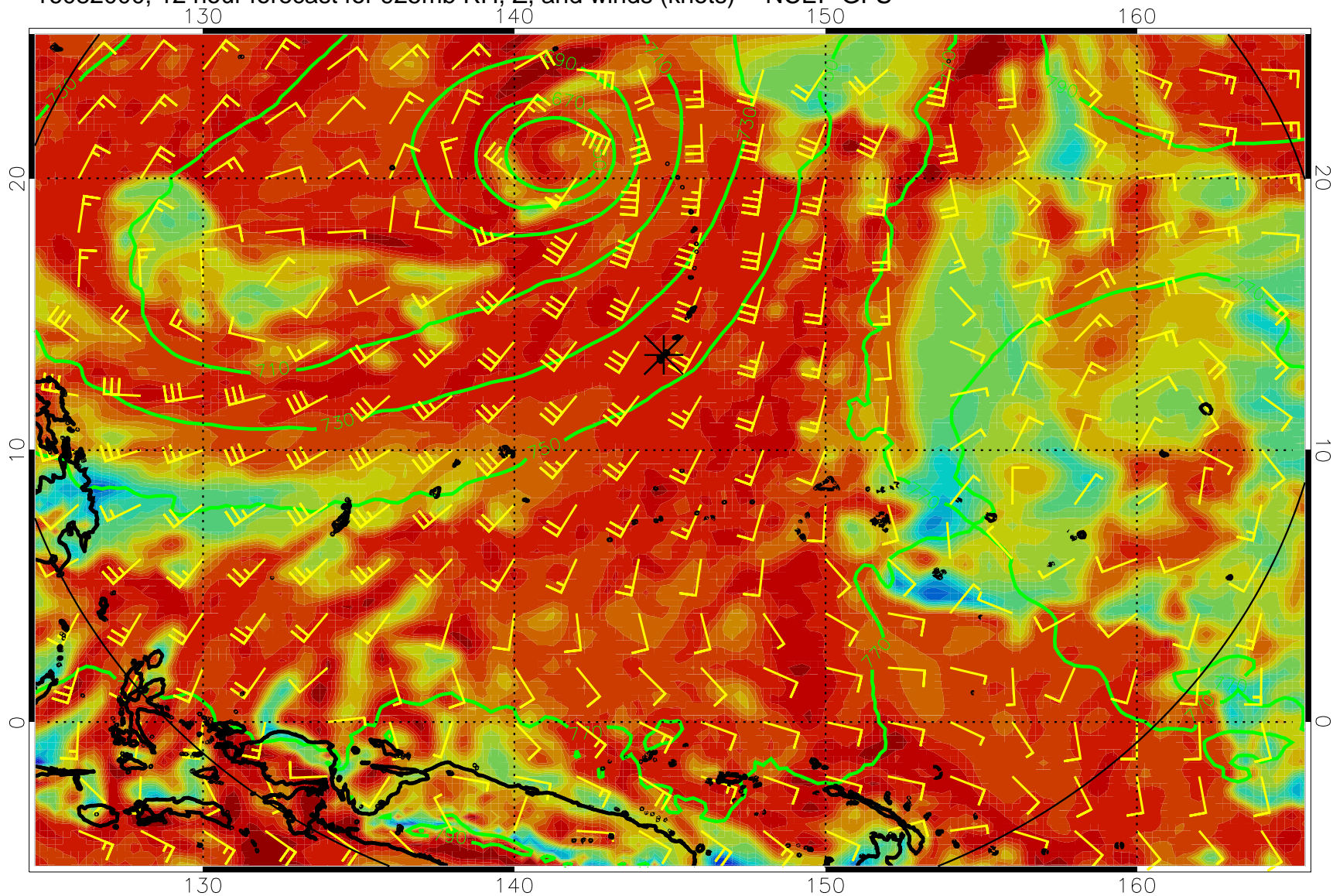
16082000, 12 hour forecast for 925mb RH, Z, and winds (knots) -- NCEP GFS
