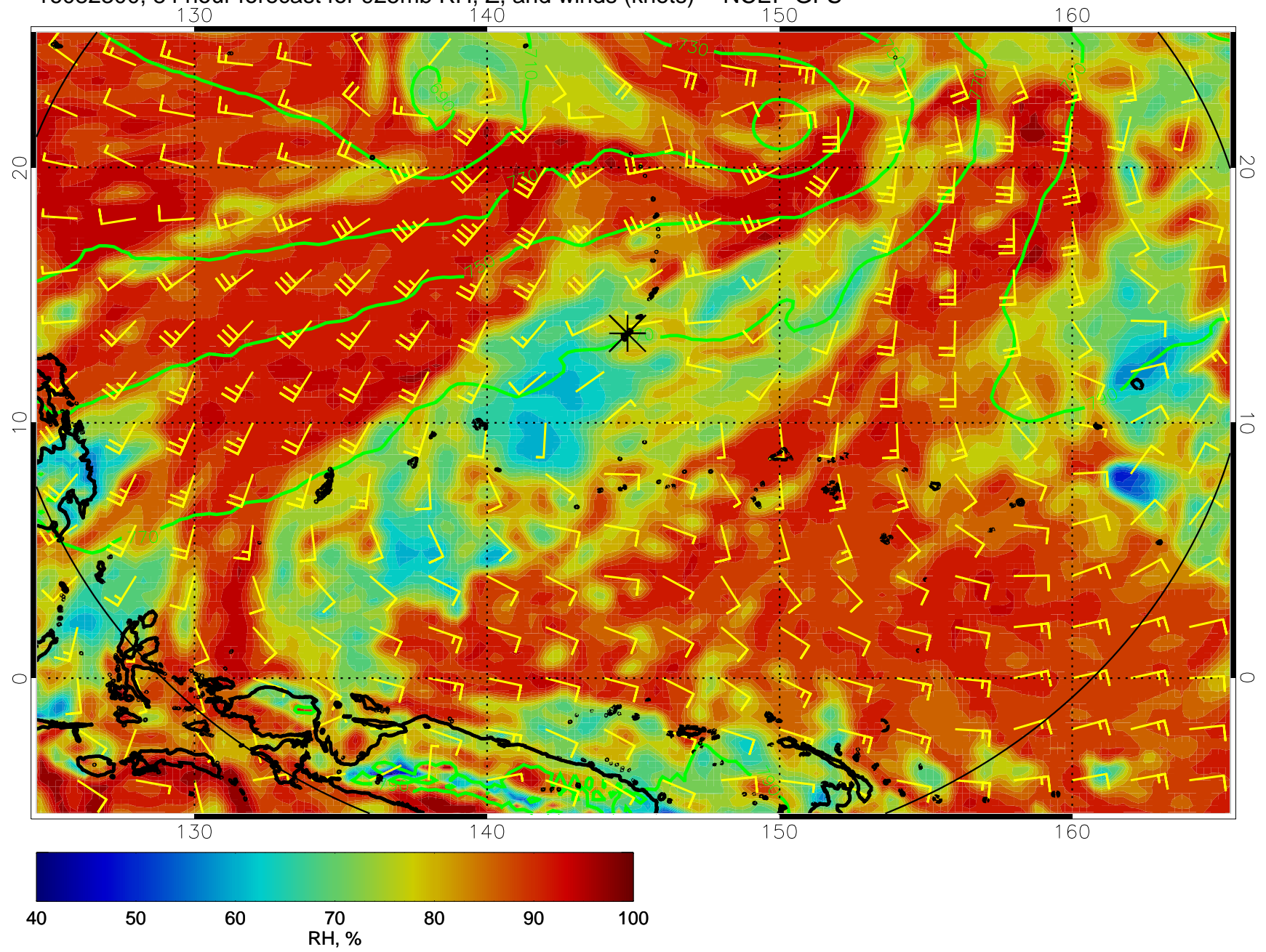
16082300, 84 hour forecast for 925mb RH, Z, and winds (knots) -- NCEP GFS
