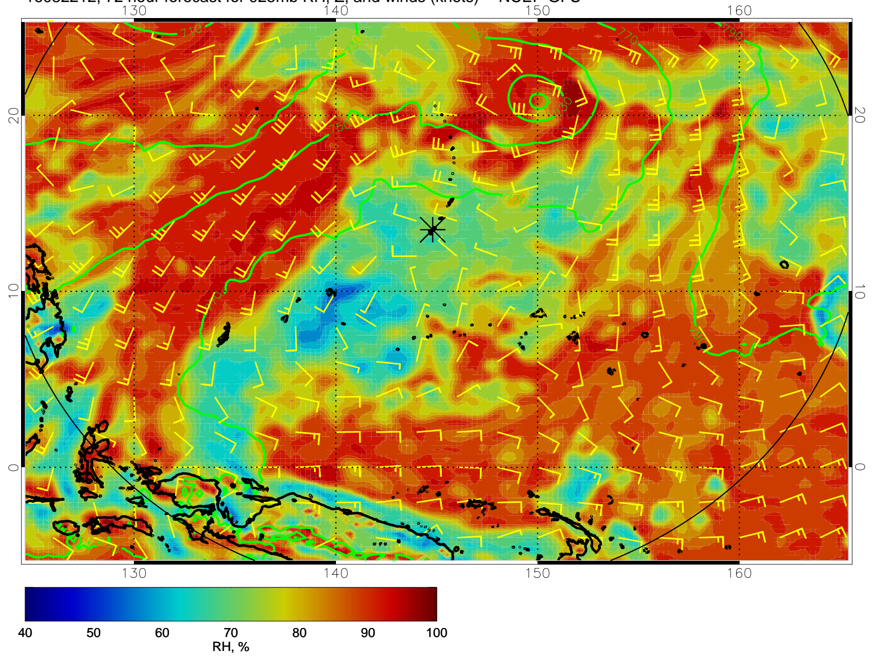
16082212, 72 hour forecast for 925mb RH, Z, and winds (knots) -- NCEP GFS
