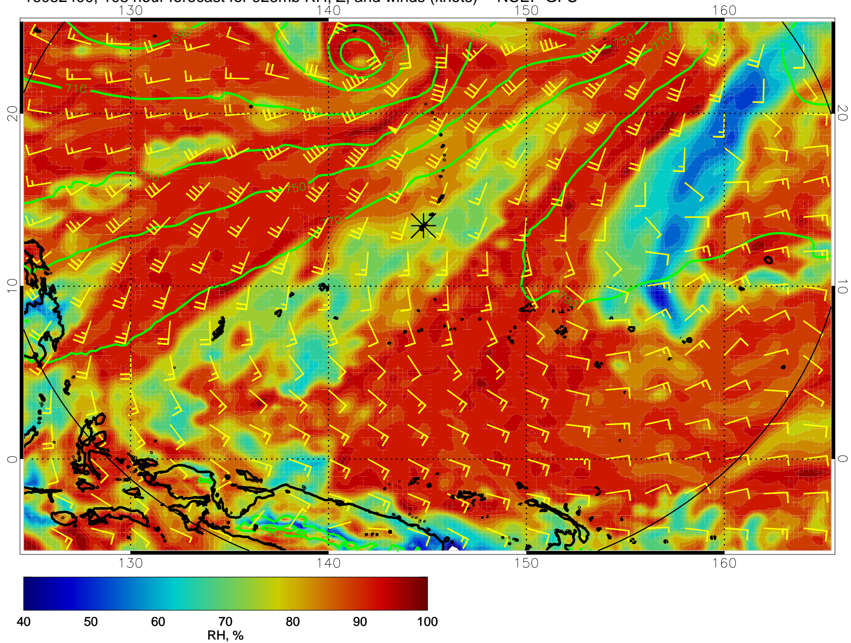
16082400, 108 hour forecast for 925mb RH, Z, and winds (knots) -- NCEP GFS
