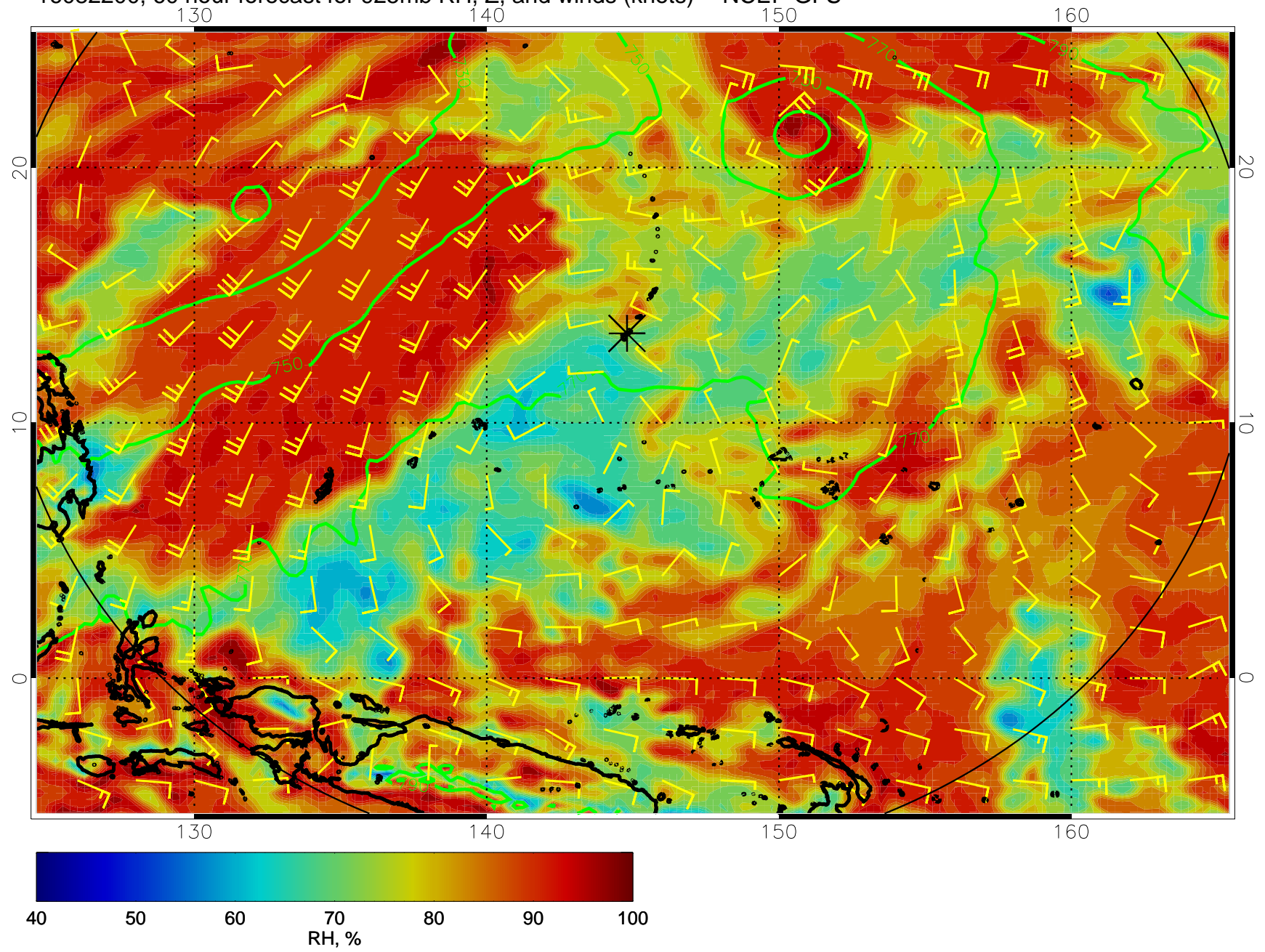
16082200, 60 hour forecast for 925mb RH, Z, and winds (knots) -- NCEP GFS
