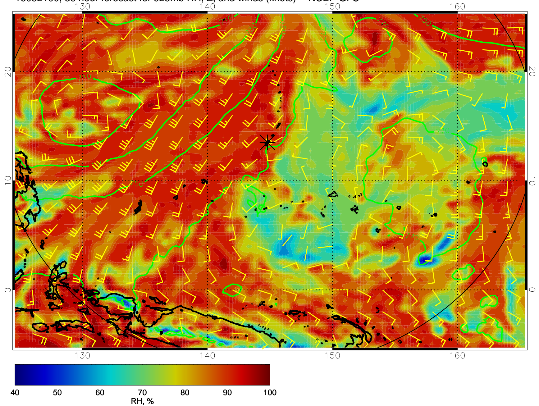
16082100, 36 hour forecast for 925mb RH, Z, and winds (knots) -- NCEP GFS
