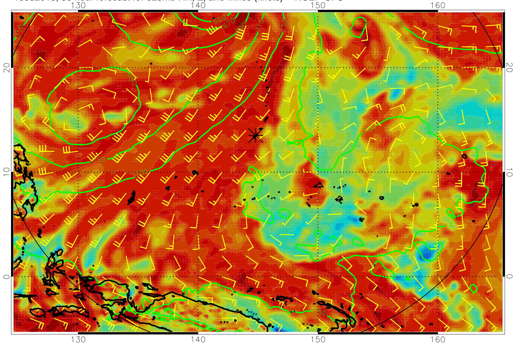
16082018, 30 hour forecast for 925mb RH, Z, and winds (knots) -- NCEP GFS
