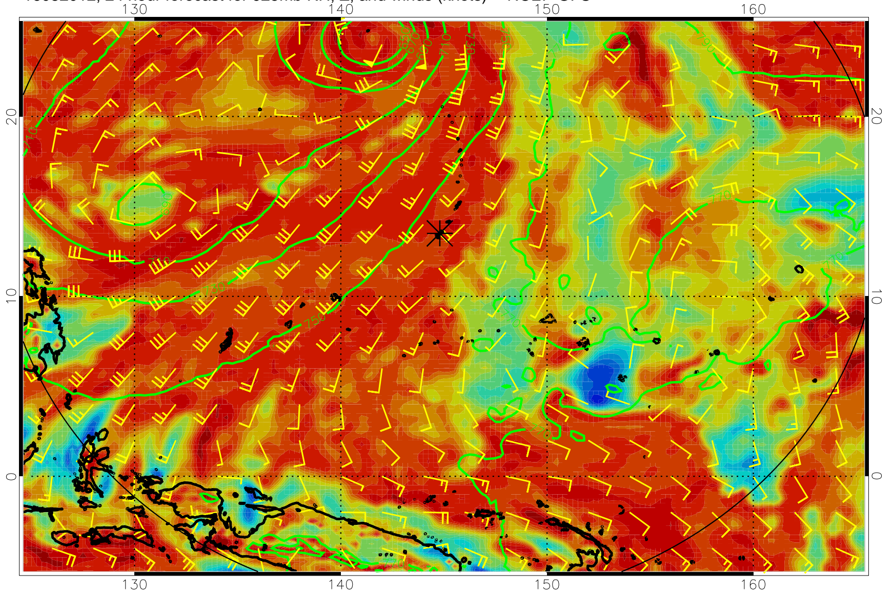
16082012, 24 hour forecast for 925mb RH, Z, and winds (knots) -- NCEP GFS
