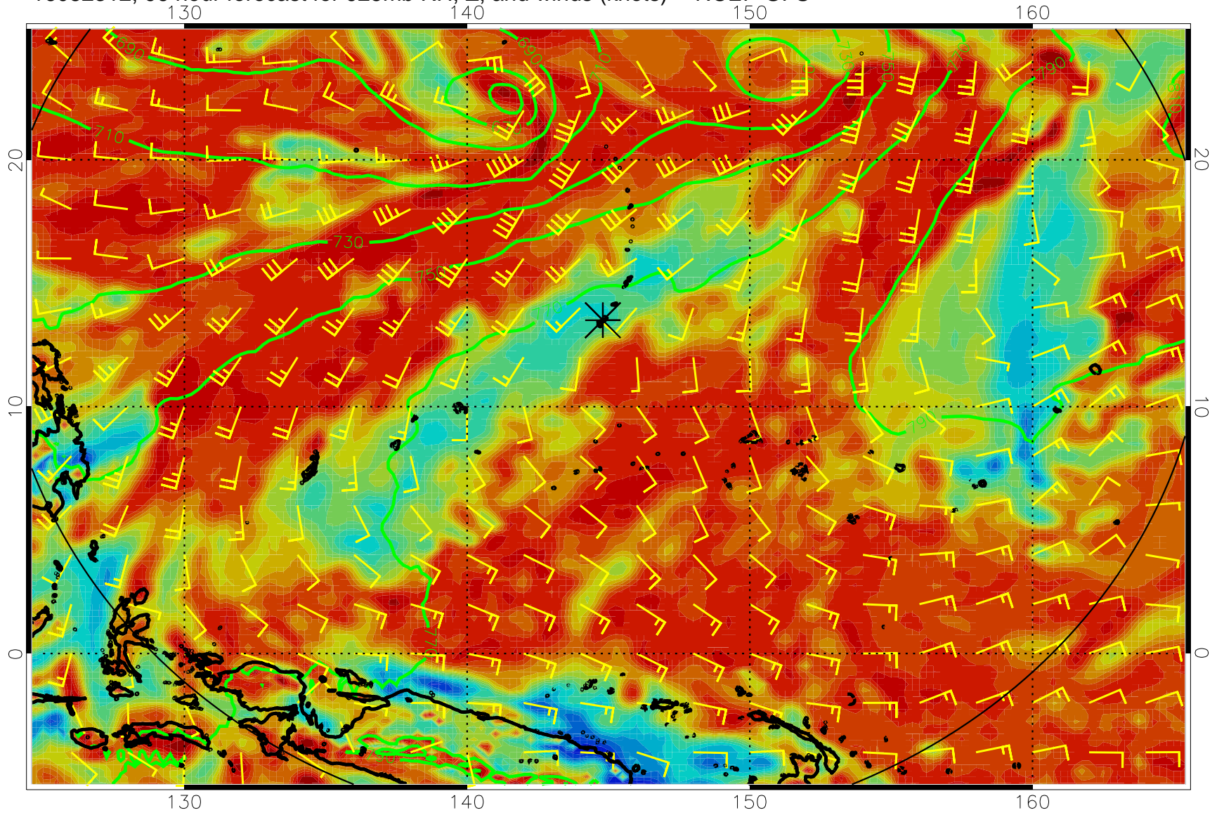
16082312, 96 hour forecast for 925mb RH, Z, and winds (knots) -- NCEP GFS
