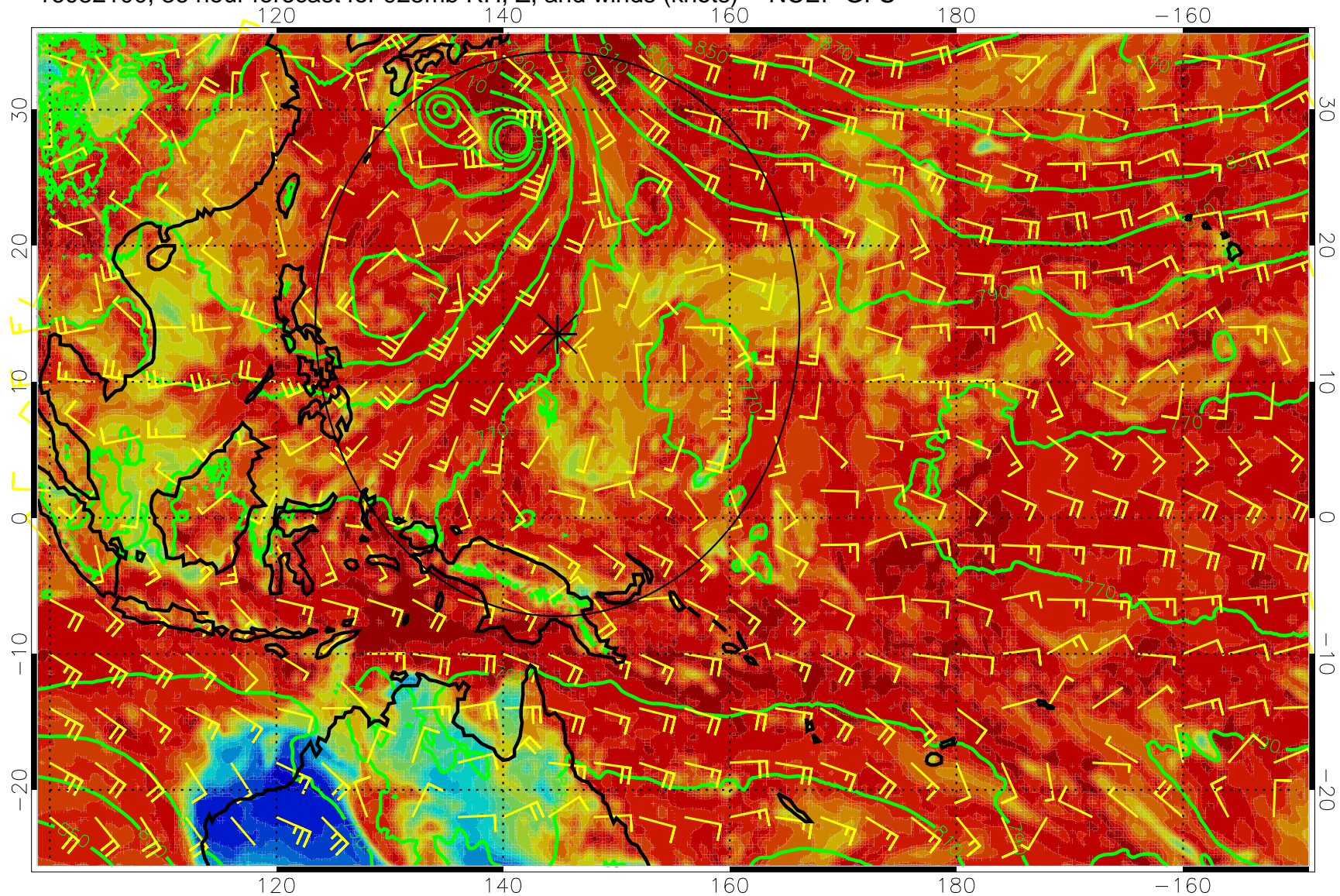
16082100, 36 hour forecast for 925mb RH, Z, and winds (knots) -- NCEP GFS
