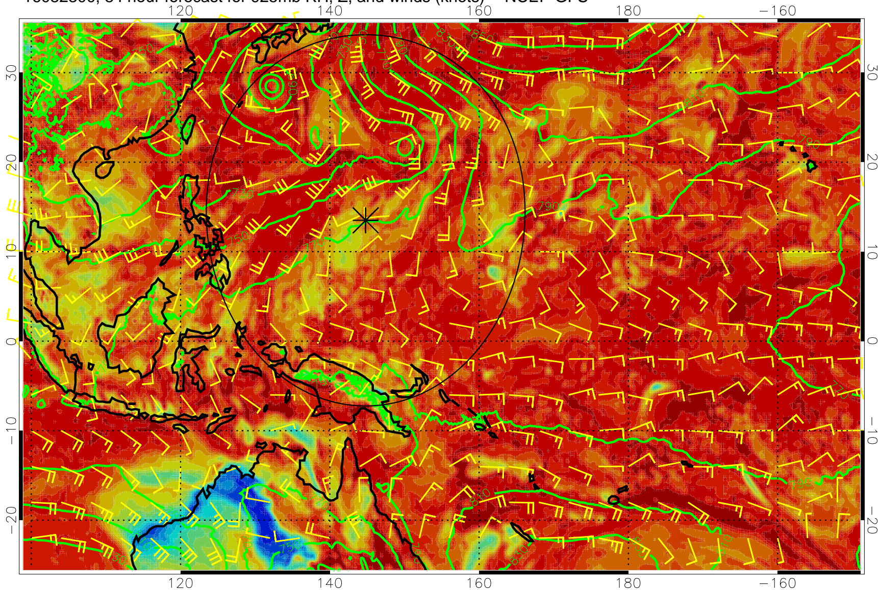
16082300, 84 hour forecast for 925mb RH, Z, and winds (knots) -- NCEP GFS
