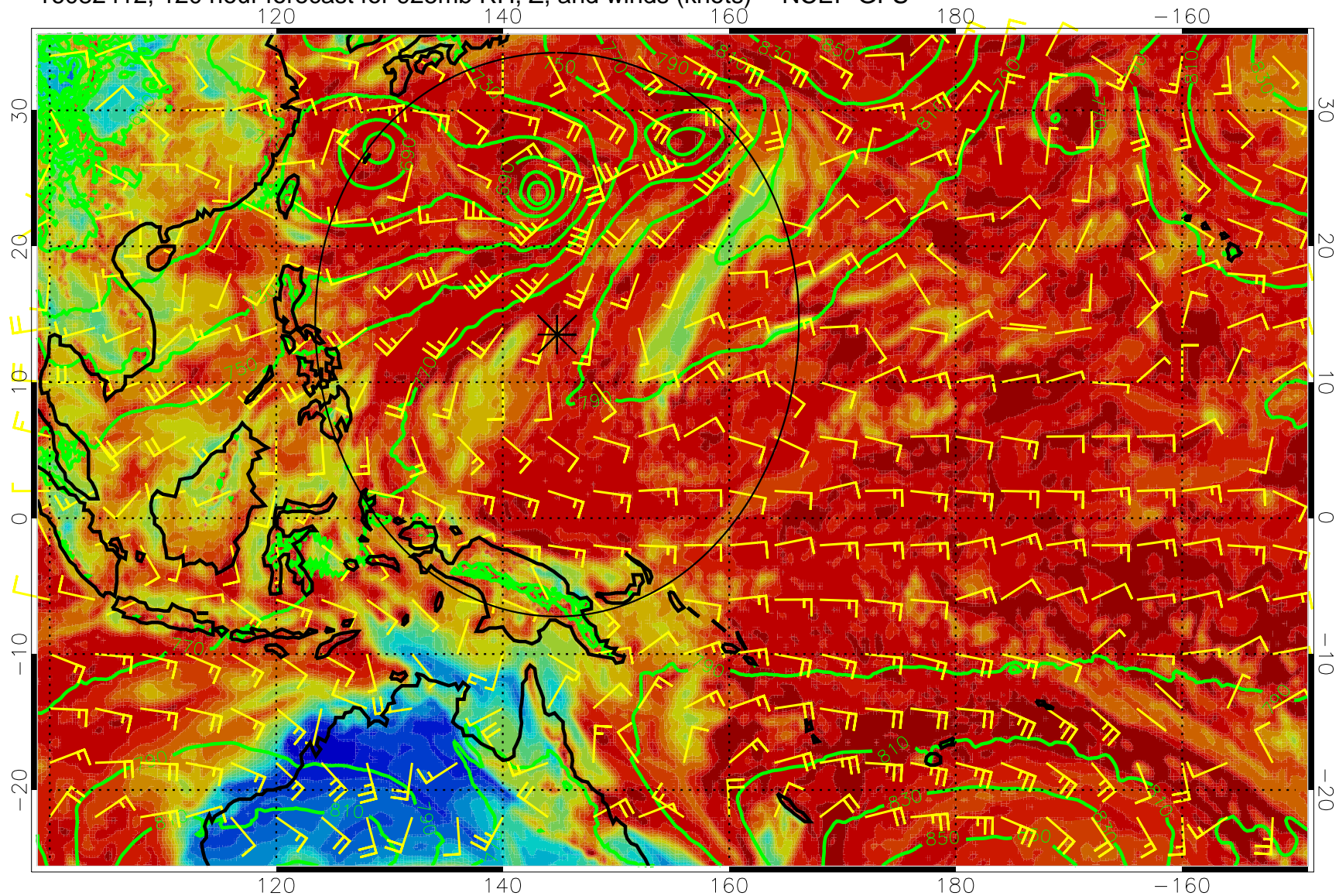
16082412, 120 hour forecast for 925mb RH, Z, and winds (knots) -- NCEP GFS
