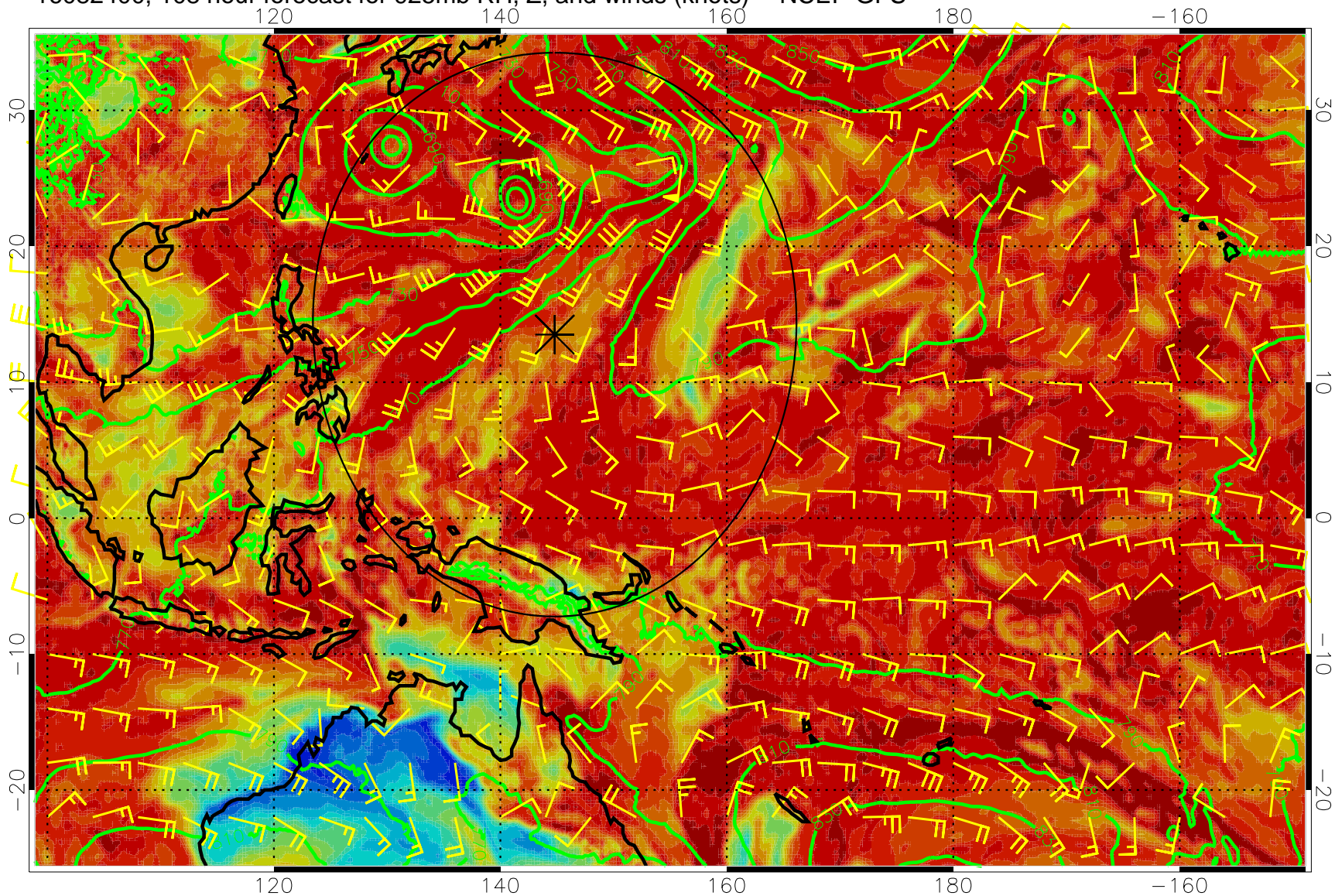
16082400, 108 hour forecast for 925mb RH, Z, and winds (knots) -- NCEP GFS
