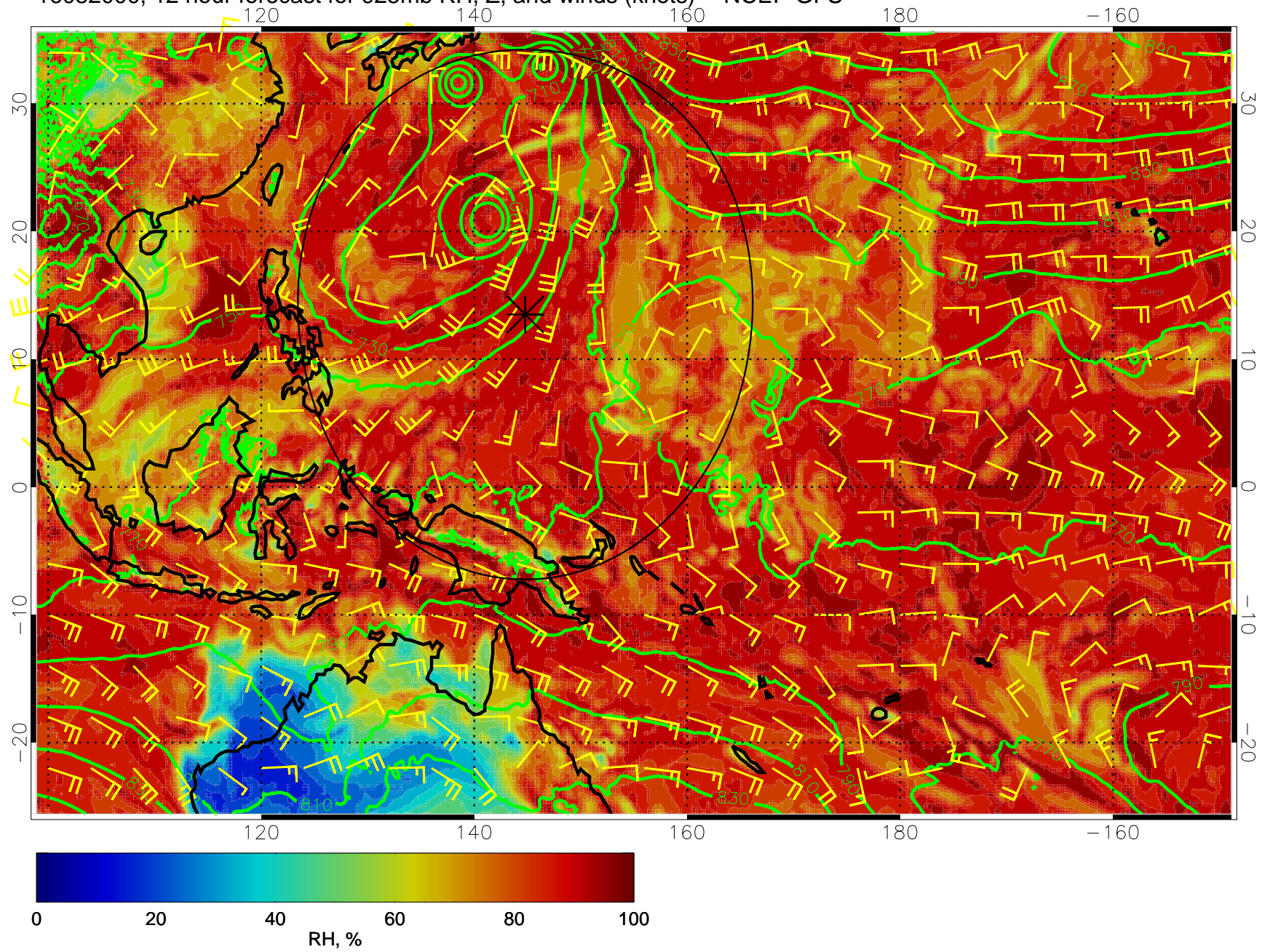
16082000, 12 hour forecast for 925mb RH, Z, and winds (knots) -- NCEP GFS
