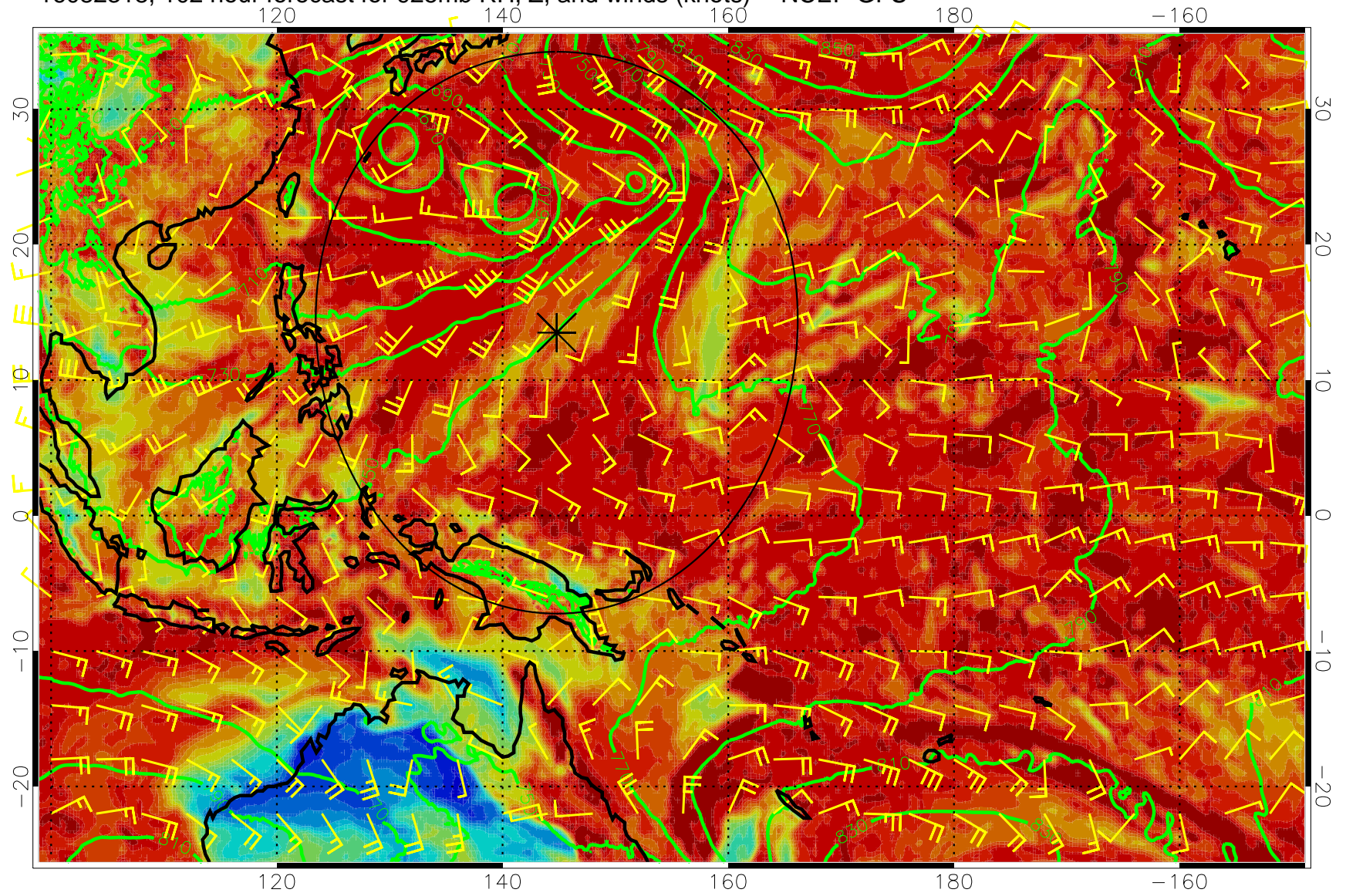
16082318, 102 hour forecast for 925mb RH, Z, and winds (knots) -- NCEP GFS
