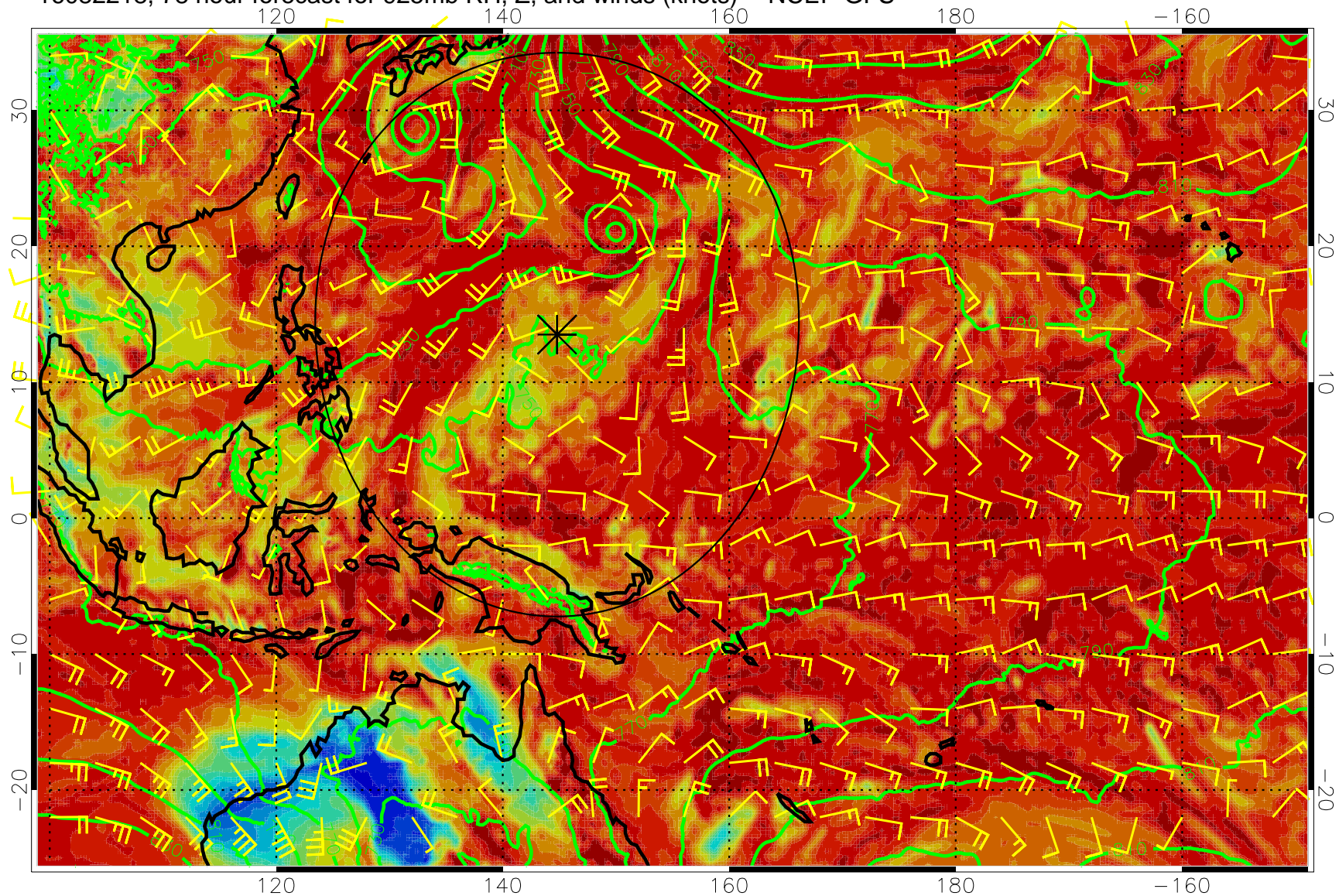
16082218, 78 hour forecast for 925mb RH, Z, and winds (knots) -- NCEP GFS
