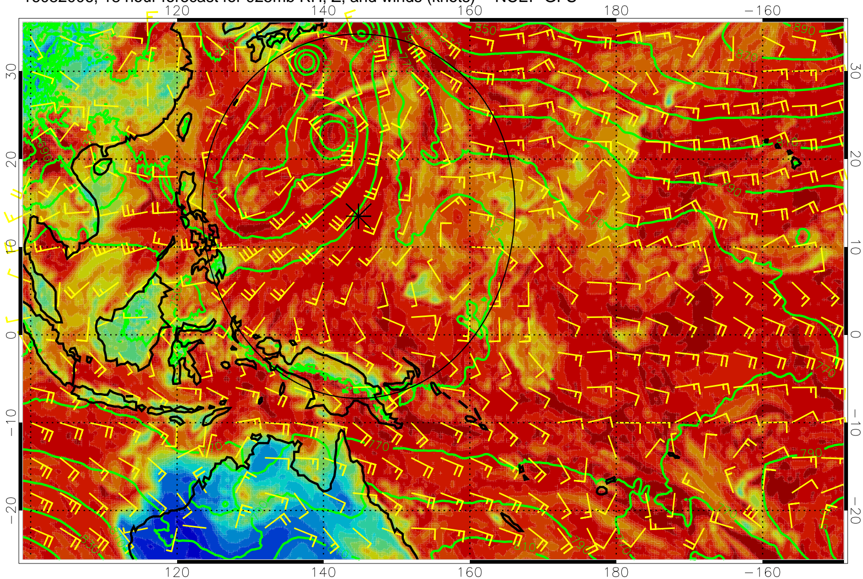
16082006, 18 hour forecast for 925mb RH, Z, and winds (knots) -- NCEP GFS
