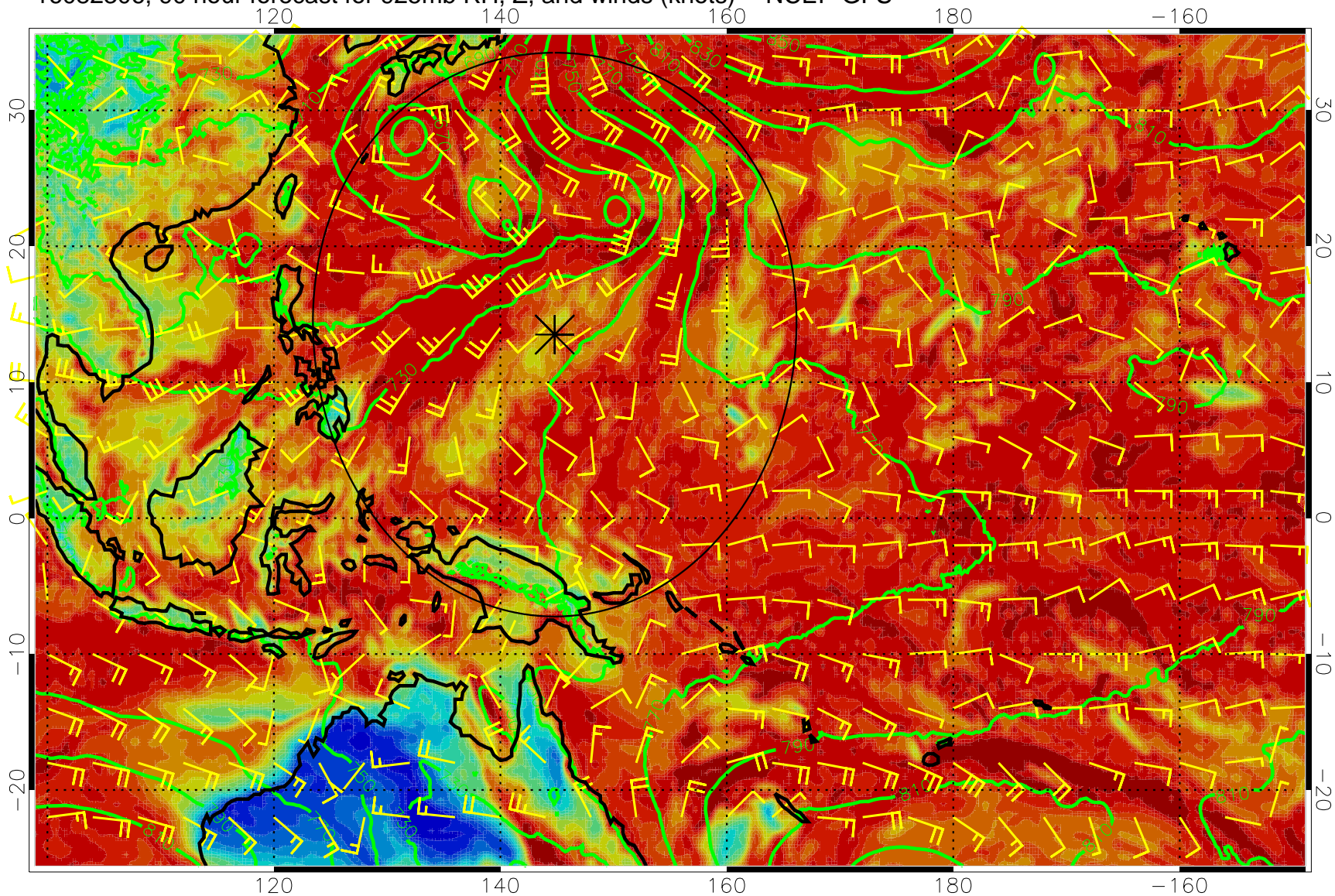
16082306, 90 hour forecast for 925mb RH, Z, and winds (knots) -- NCEP GFS
