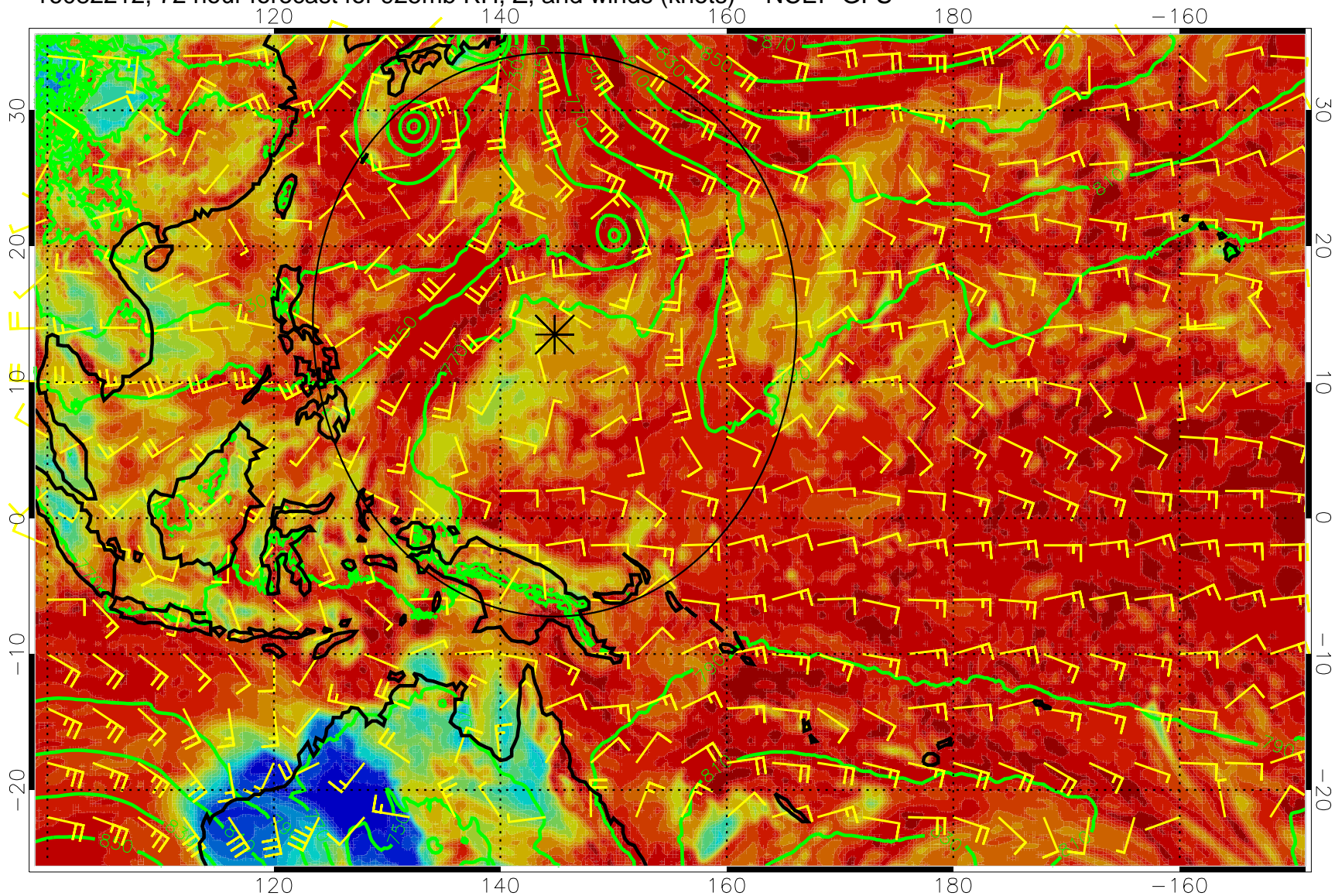
16082212, 72 hour forecast for 925mb RH, Z, and winds (knots) -- NCEP GFS
