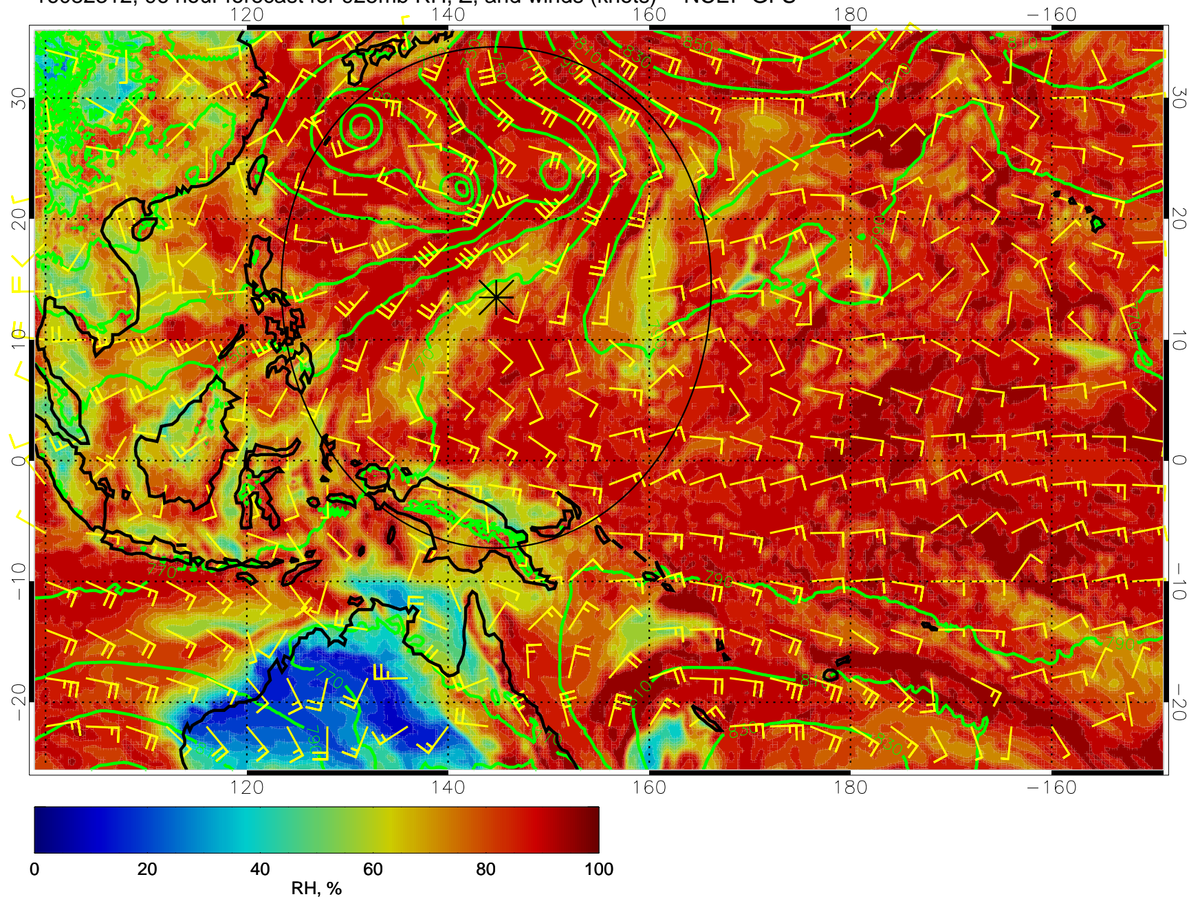
16082312, 96 hour forecast for 925mb RH, Z, and winds (knots) -- NCEP GFS
