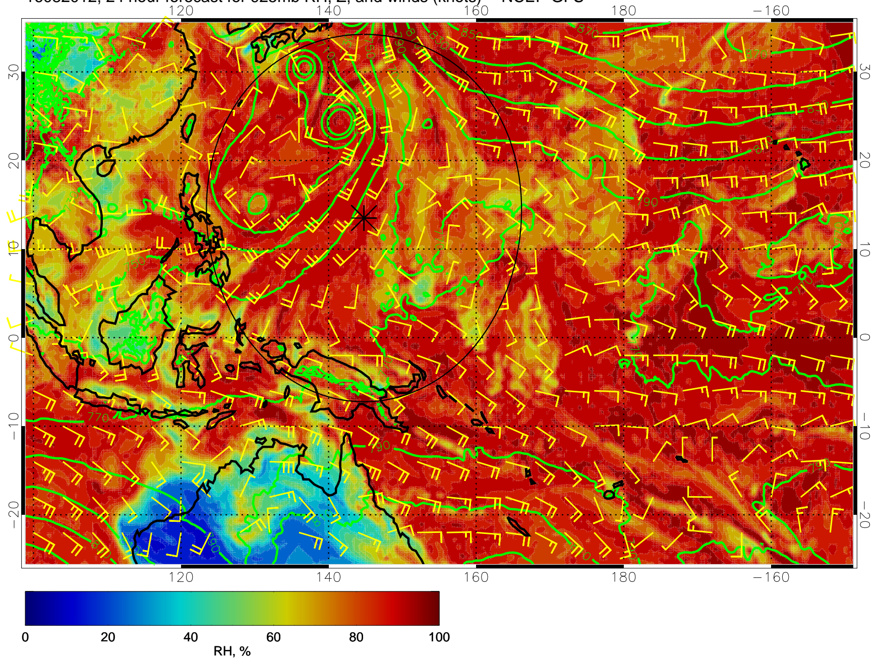
16082012, 24 hour forecast for 925mb RH, Z, and winds (knots) -- NCEP GFS
