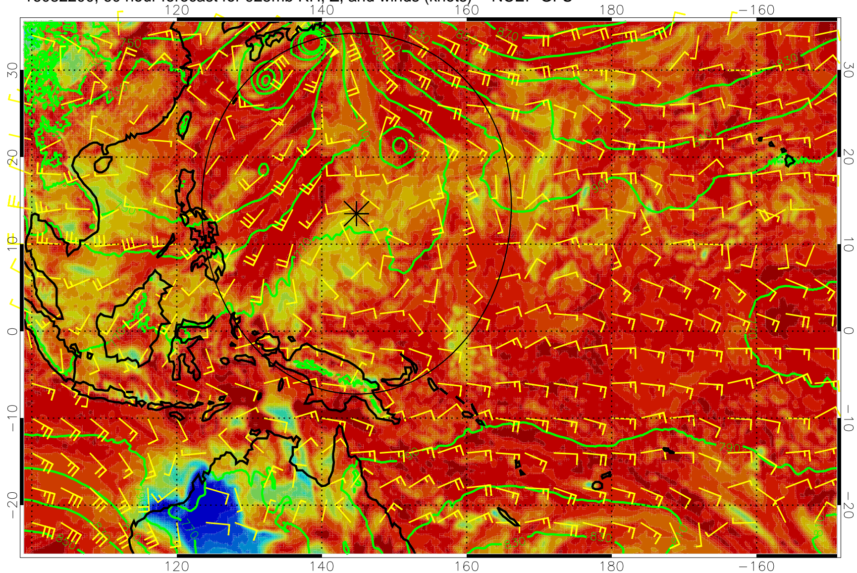
16082200, 60 hour forecast for 925mb RH, Z, and winds (knots) -- NCEP GFS
