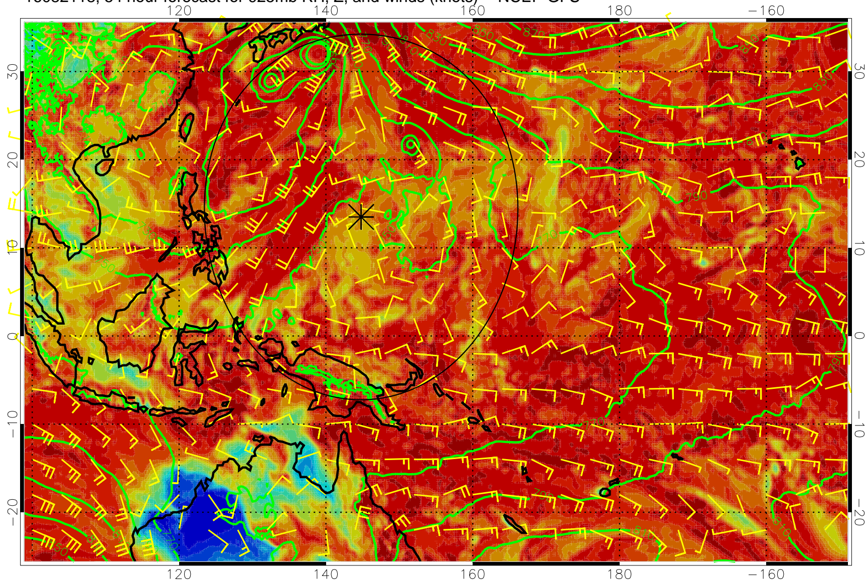
16082118, 54 hour forecast for 925mb RH, Z, and winds (knots) -- NCEP GFS
