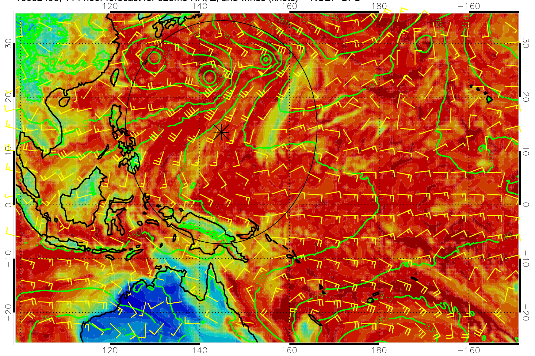
16082406, 114 hour forecast for 925mb RH, Z, and winds (knots) -- NCEP GFS
