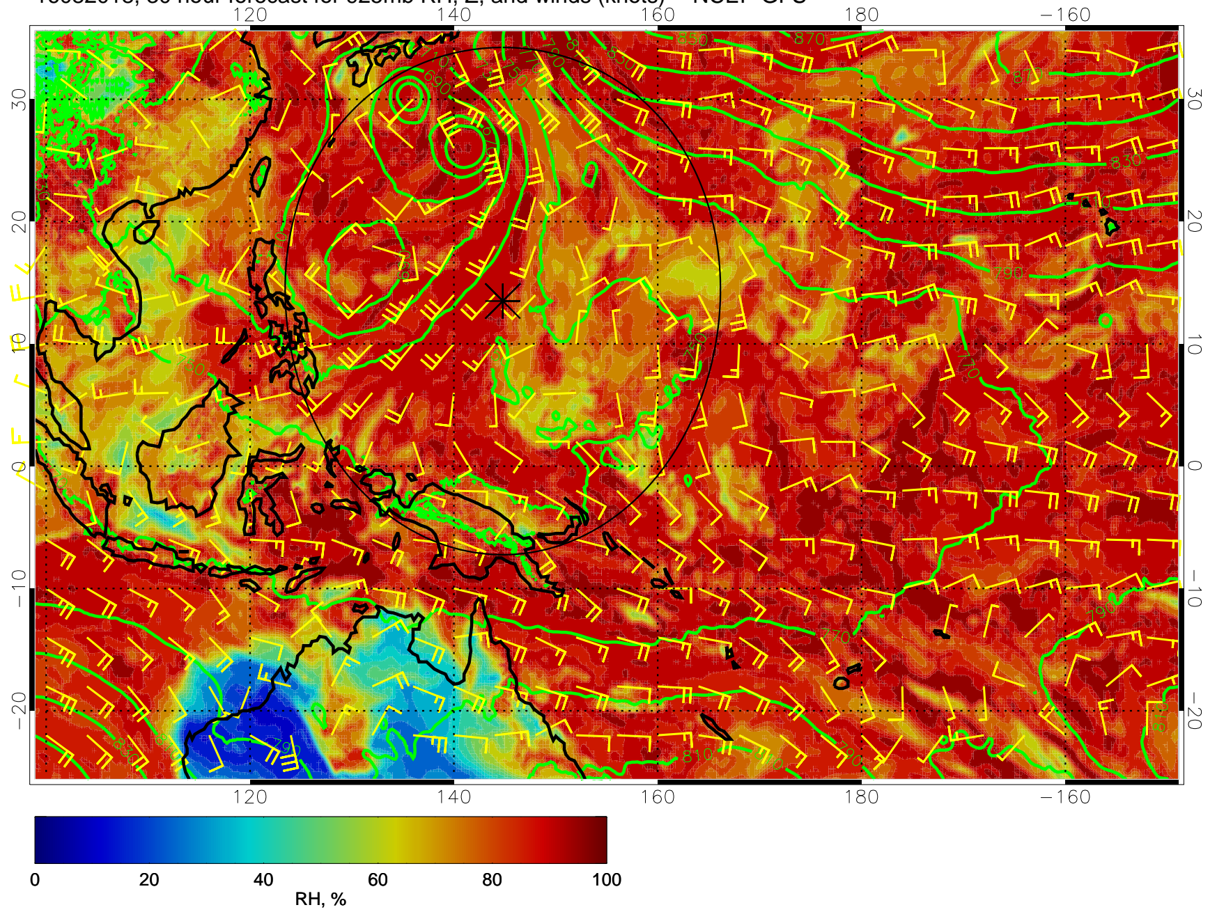
16082018, 30 hour forecast for 925mb RH, Z, and winds (knots) -- NCEP GFS
