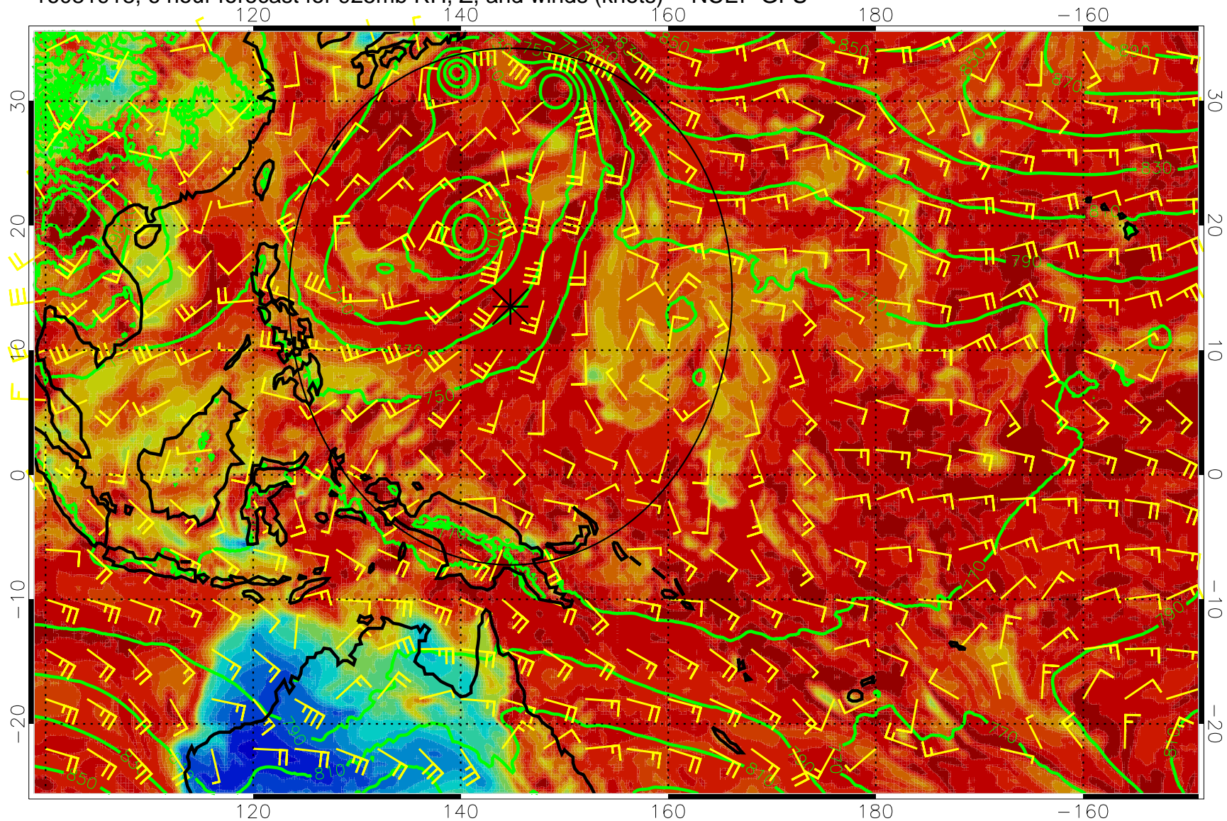
16081918, 6 hour forecast for 925mb RH, Z, and winds (knots) -- NCEP GFS
