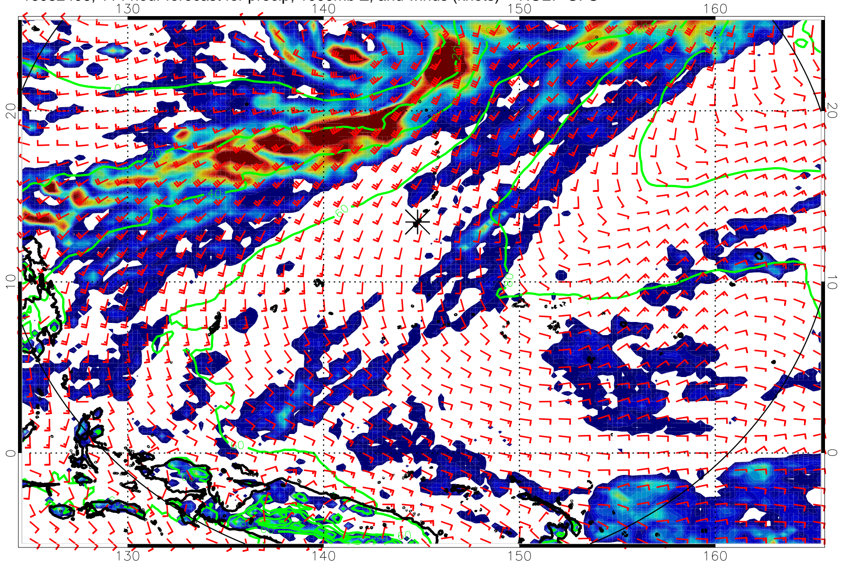
16082406, 114 hour forecast for precip, 1000mb Z, and winds (knots) -- NCEP GFS
