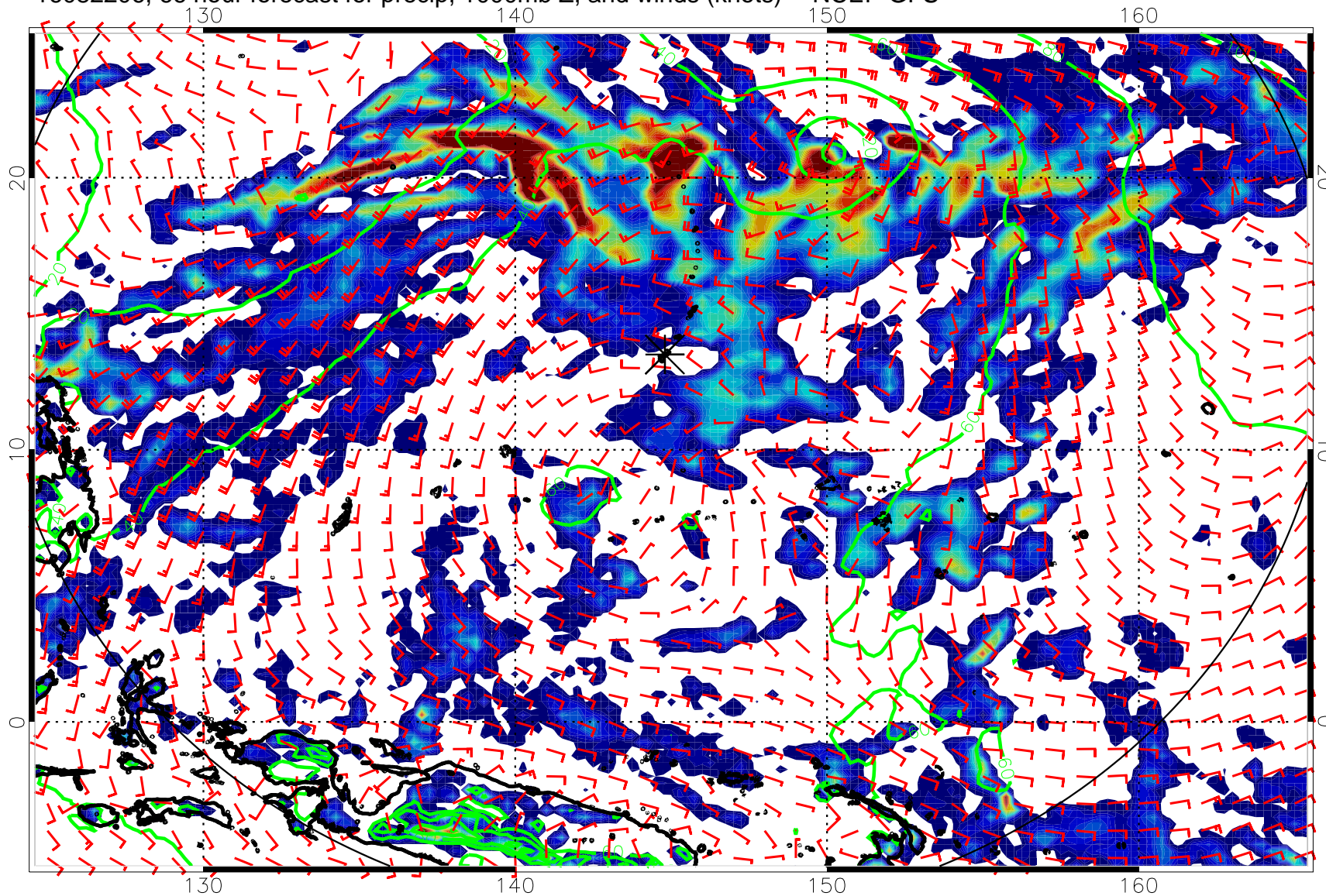
16082206, 66 hour forecast for precip, 1000mb Z, and winds (knots) -- NCEP GFS
