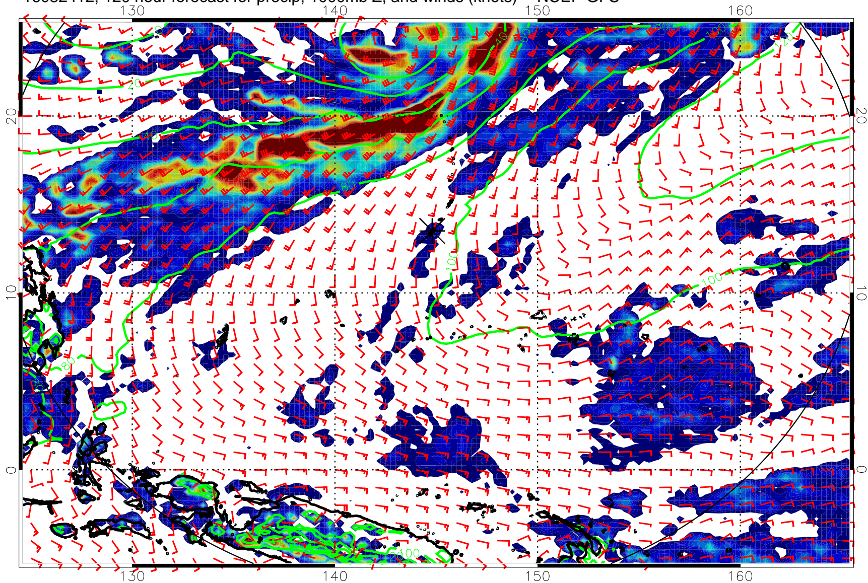
16082412, 120 hour forecast for precip, 1000mb Z, and winds (knots) -- NCEP GFS
