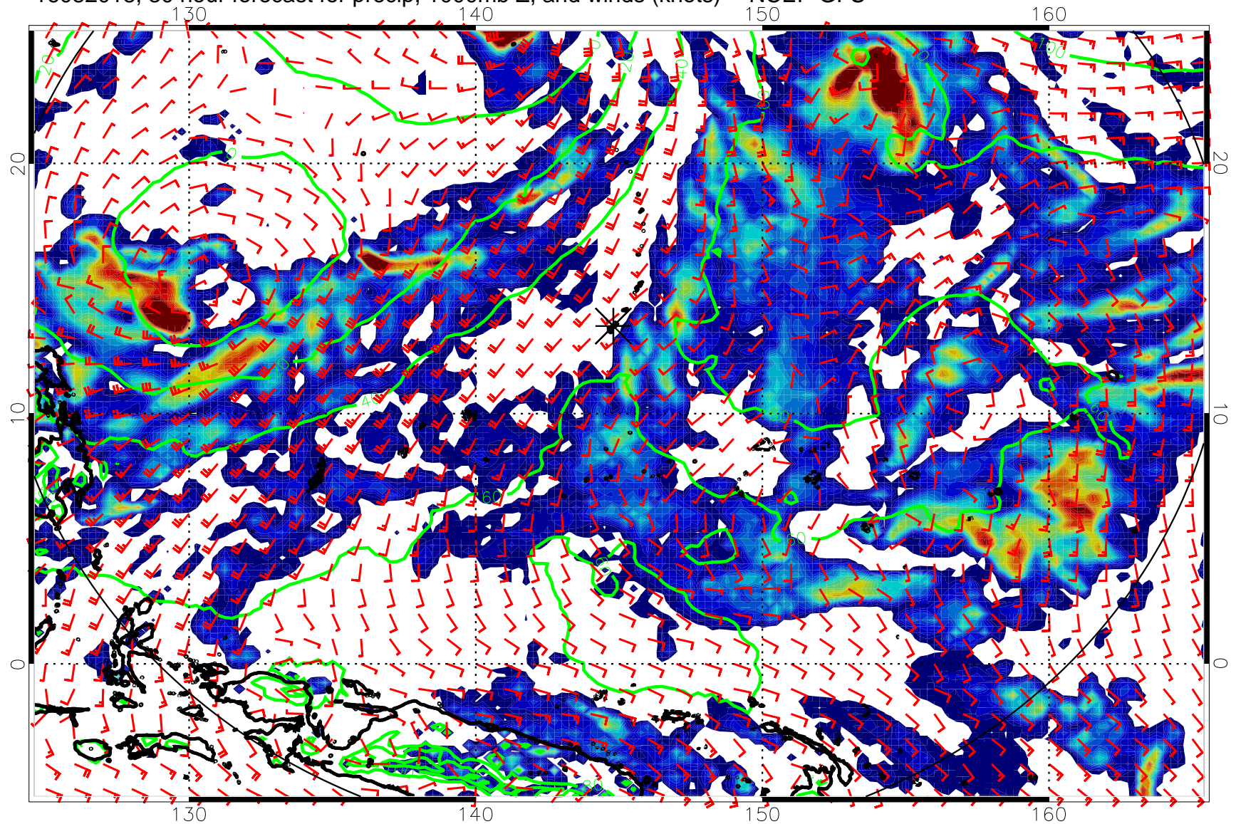
16082018, 30 hour forecast for precip, 1000mb Z, and winds (knots) -- NCEP GFS
