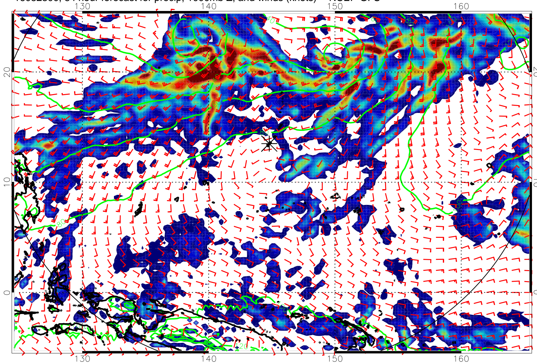
16082300, 84 hour forecast for precip, 1000mb Z, and winds (knots) -- NCEP GFS
