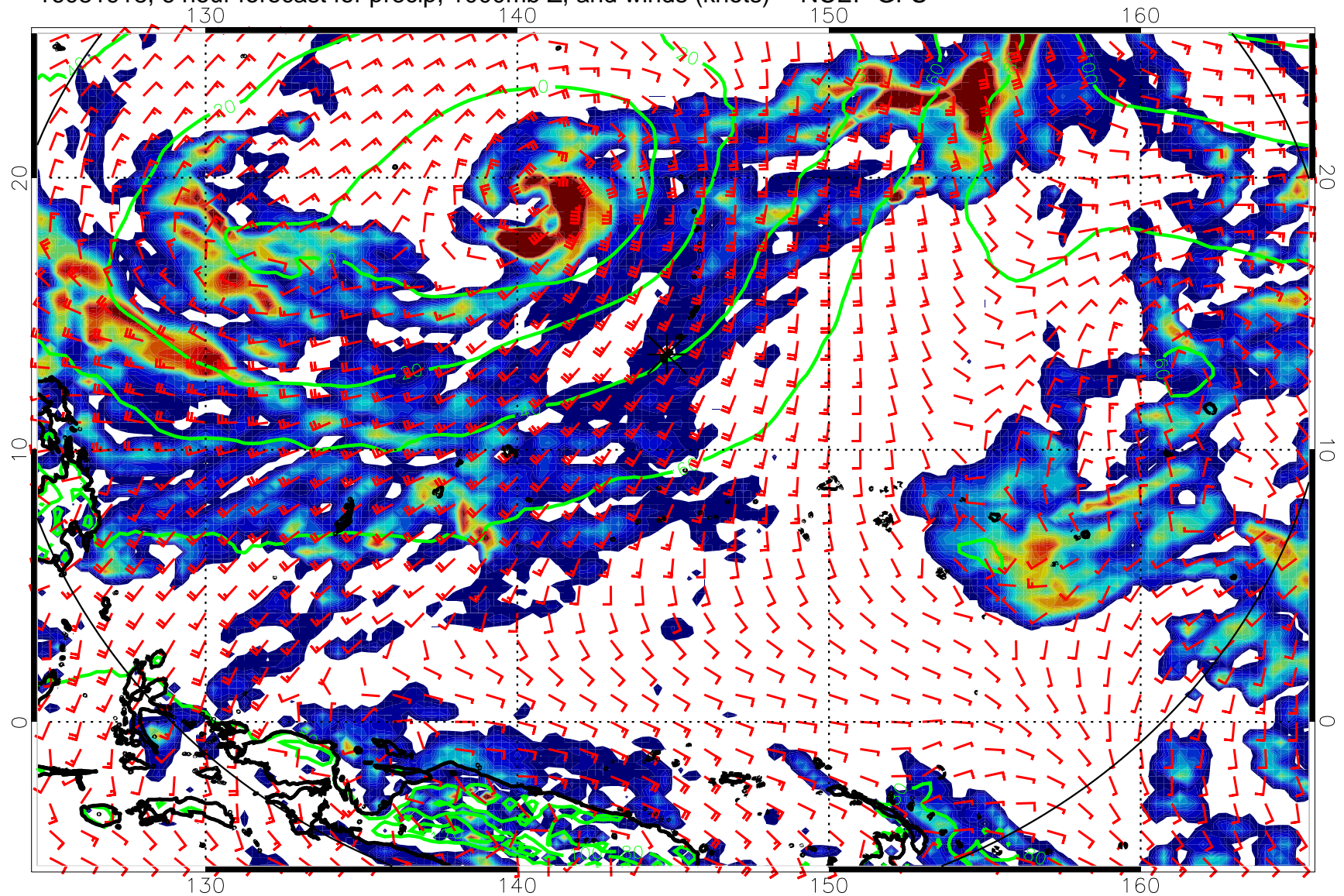
16081918, 6 hour forecast for precip, 1000mb Z, and winds (knots) -- NCEP GFS
