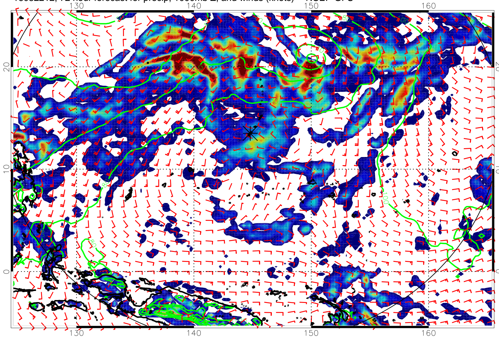
16082212, 72 hour forecast for precip, 1000mb Z, and winds (knots) -- NCEP GFS
