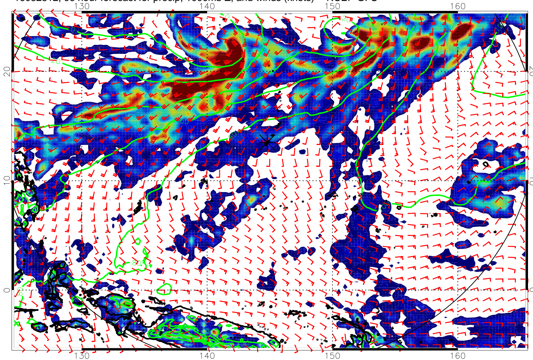
16082312, 96 hour forecast for precip, 1000mb Z, and winds (knots) -- NCEP GFS
