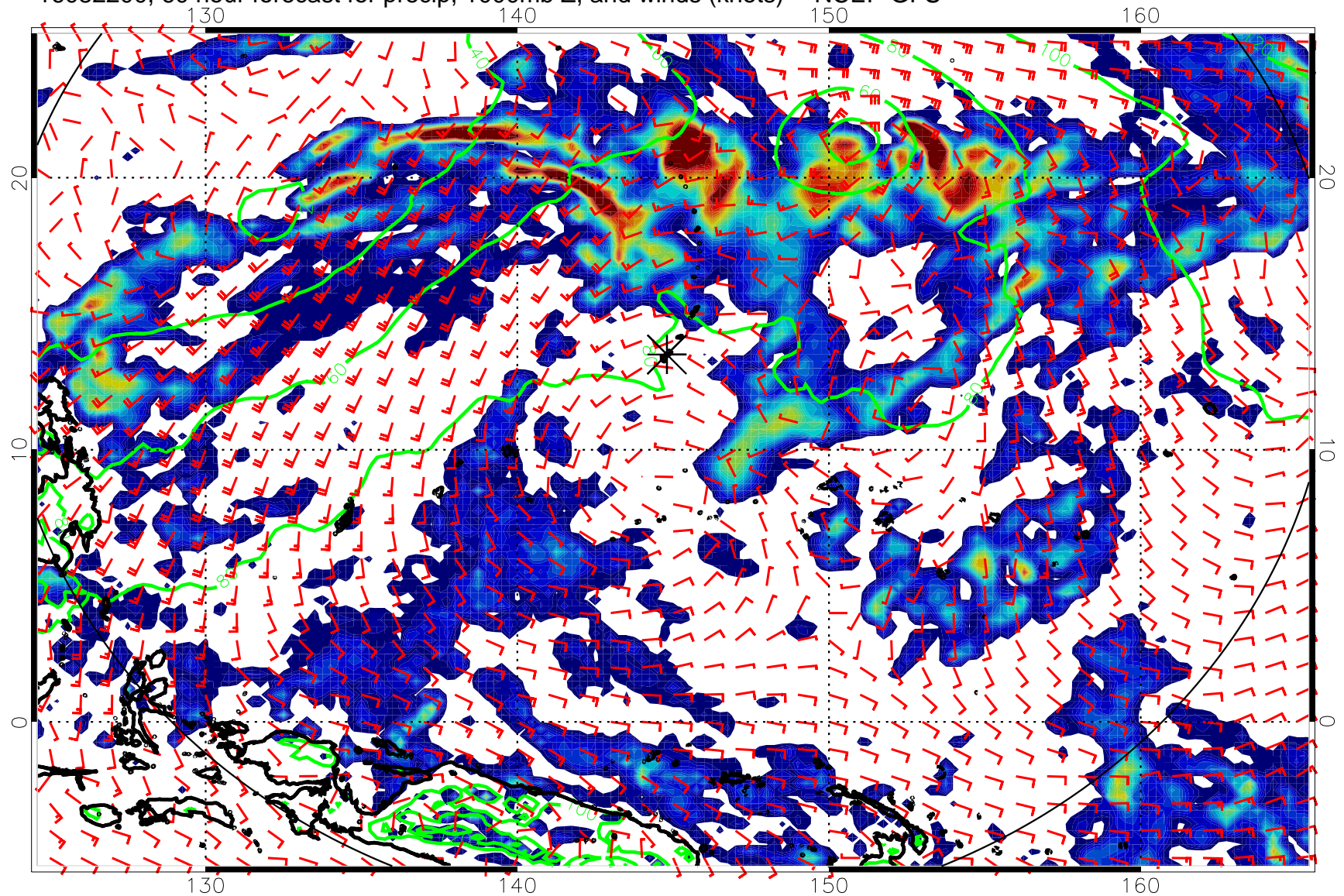
16082200, 60 hour forecast for precip, 1000mb Z, and winds (knots) -- NCEP GFS
