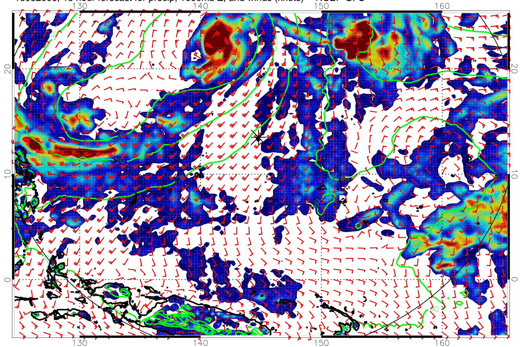
16082006, 18 hour forecast for precip, 1000mb Z, and winds (knots) -- NCEP GFS
