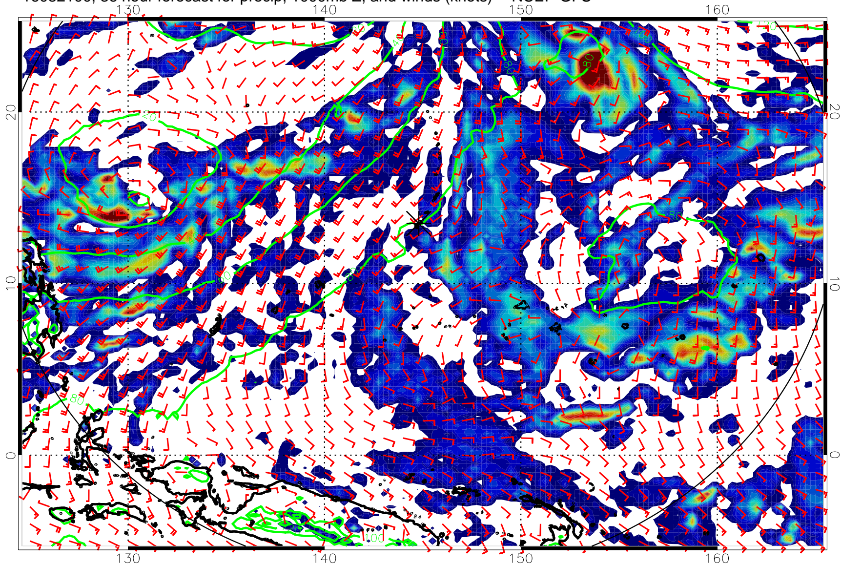
16082100, 36 hour forecast for precip, 1000mb Z, and winds (knots) -- NCEP GFS
