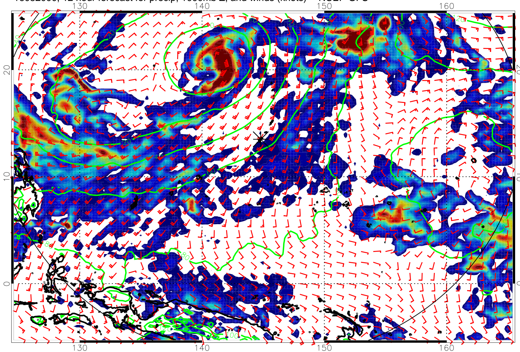
16082000, 12 hour forecast for precip, 1000mb Z, and winds (knots) -- NCEP GFS
