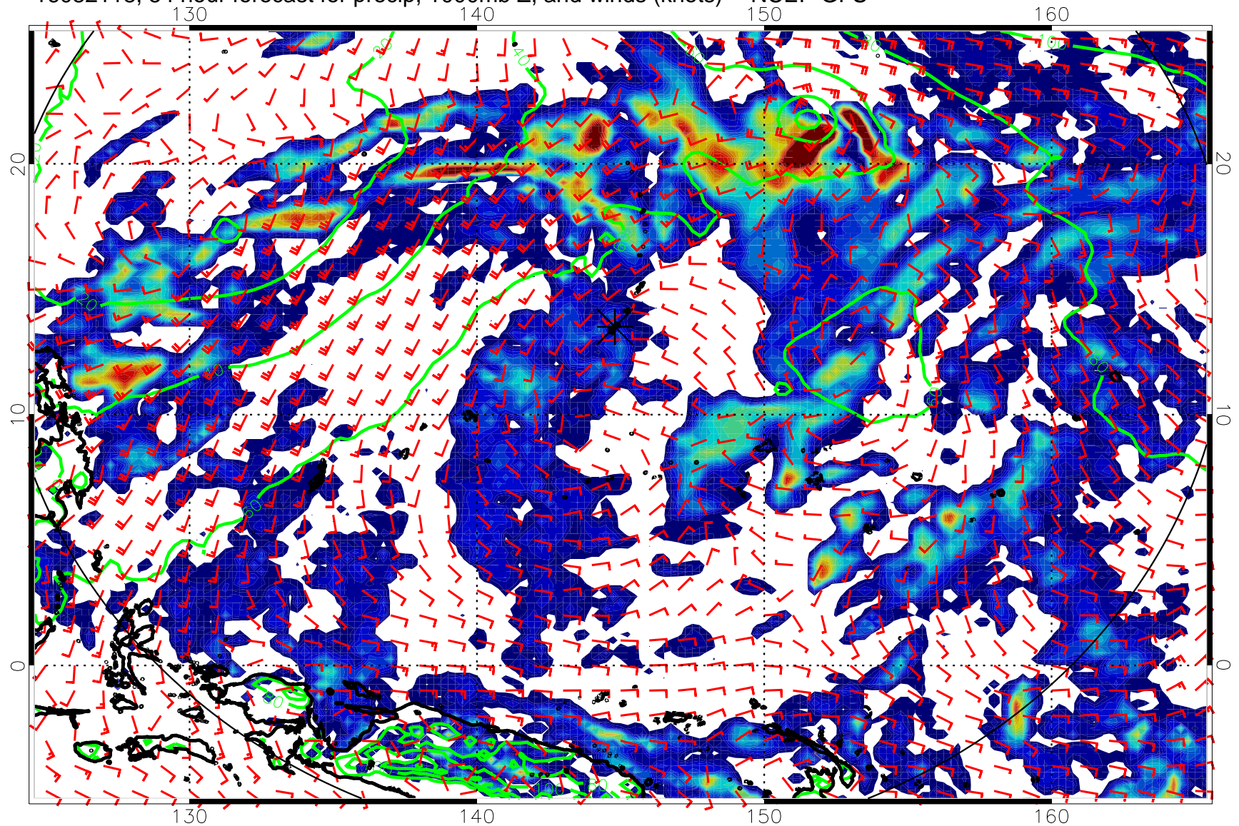
16082118, 54 hour forecast for precip, 1000mb Z, and winds (knots) -- NCEP GFS
