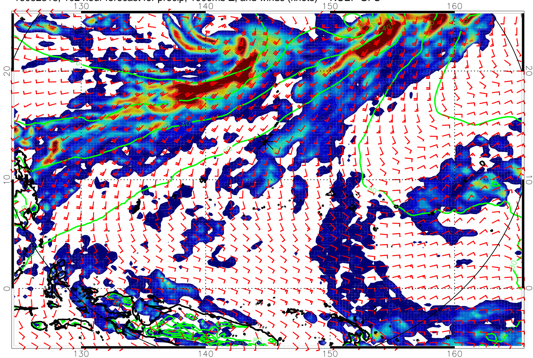
16082318, 102 hour forecast for precip, 1000mb Z, and winds (knots) -- NCEP GFS
