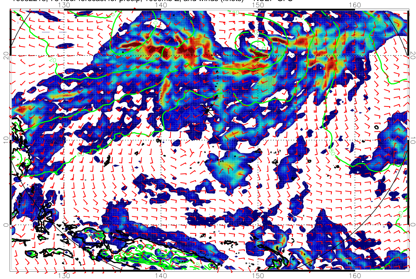
16082218, 78 hour forecast for precip, 1000mb Z, and winds (knots) -- NCEP GFS
