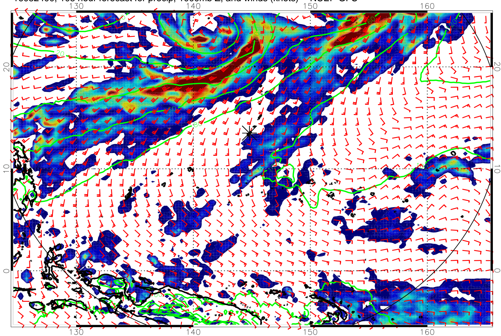
16082400, 108 hour forecast for precip, 1000mb Z, and winds (knots) -- NCEP GFS
