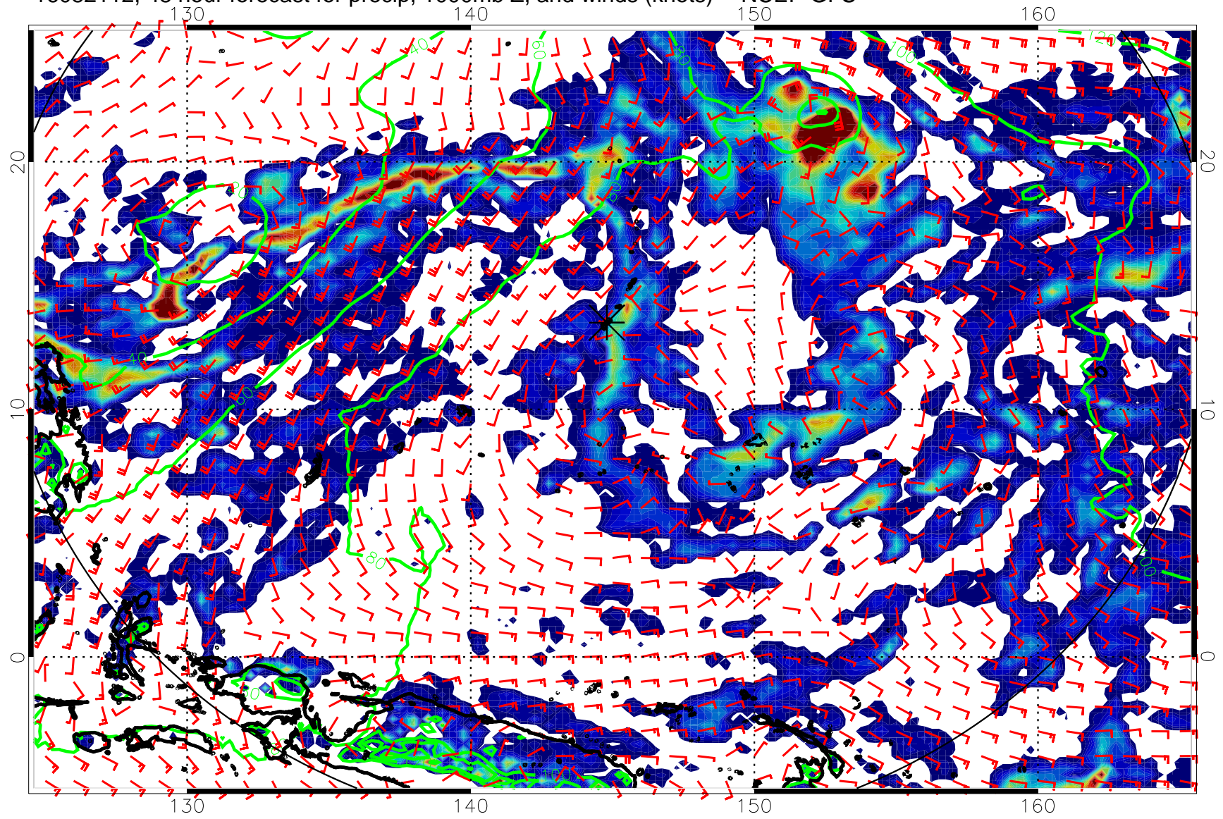
16082112, 48 hour forecast for precip, 1000mb Z, and winds (knots) -- NCEP GFS
