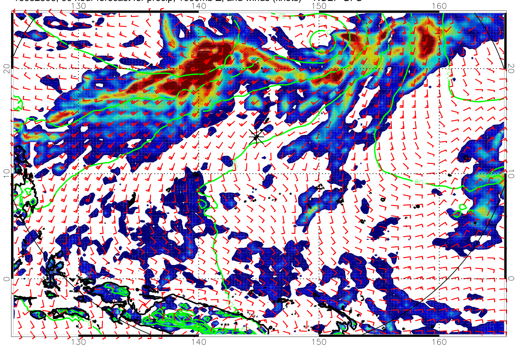
16082306, 90 hour forecast for precip, 1000mb Z, and winds (knots) -- NCEP GFS
