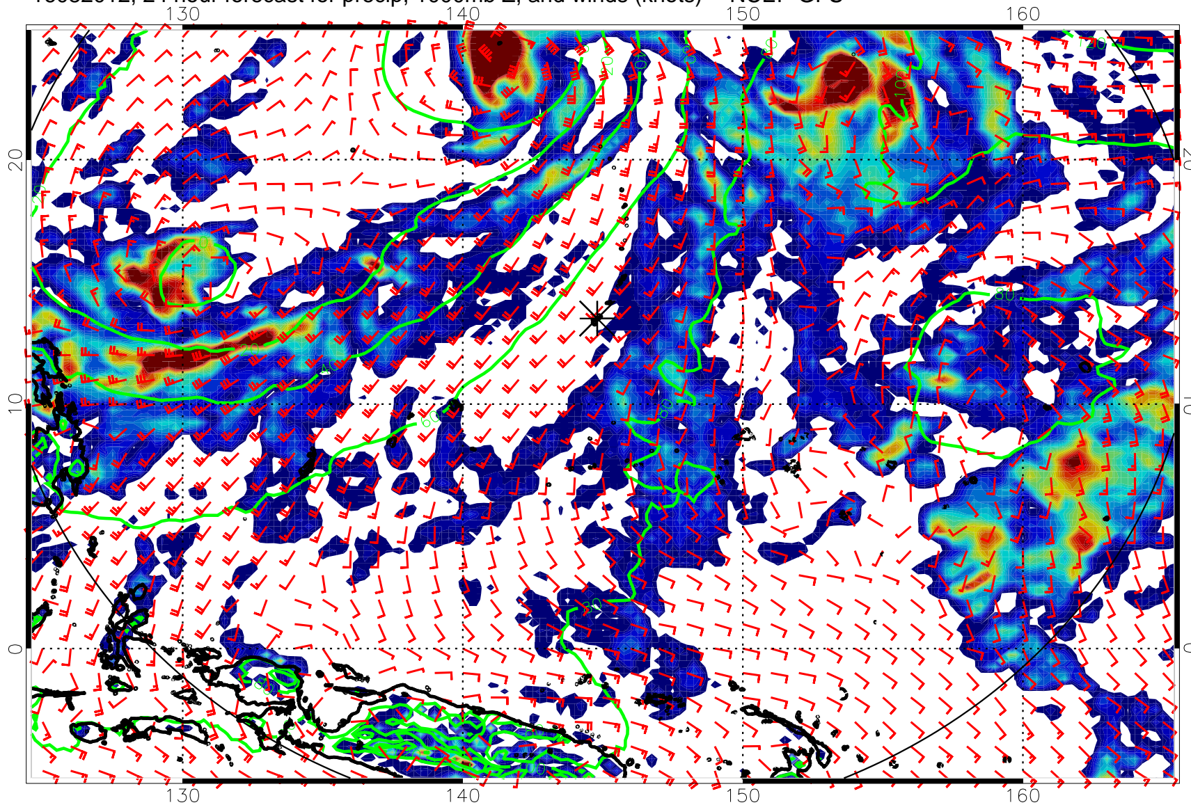
16082012, 24 hour forecast for precip, 1000mb Z, and winds (knots) -- NCEP GFS
