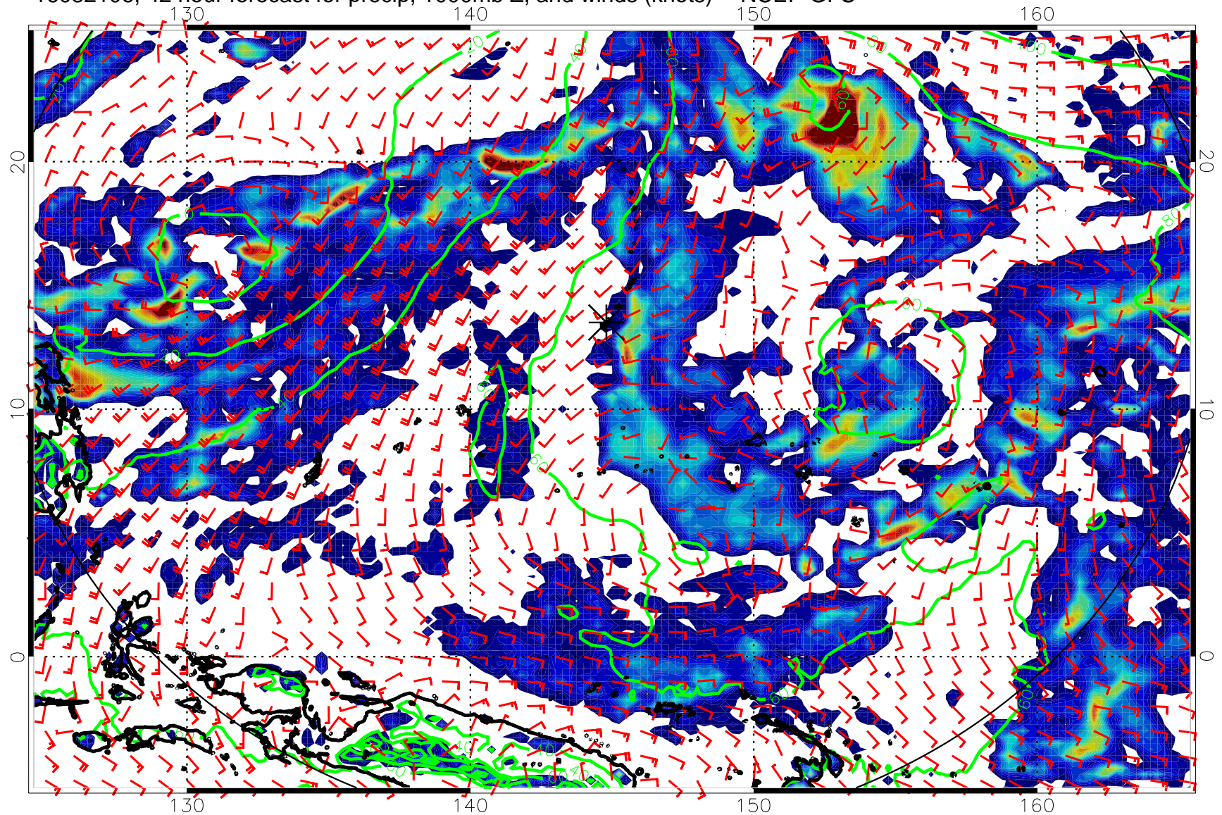
16082106, 42 hour forecast for precip, 1000mb Z, and winds (knots) -- NCEP GFS
