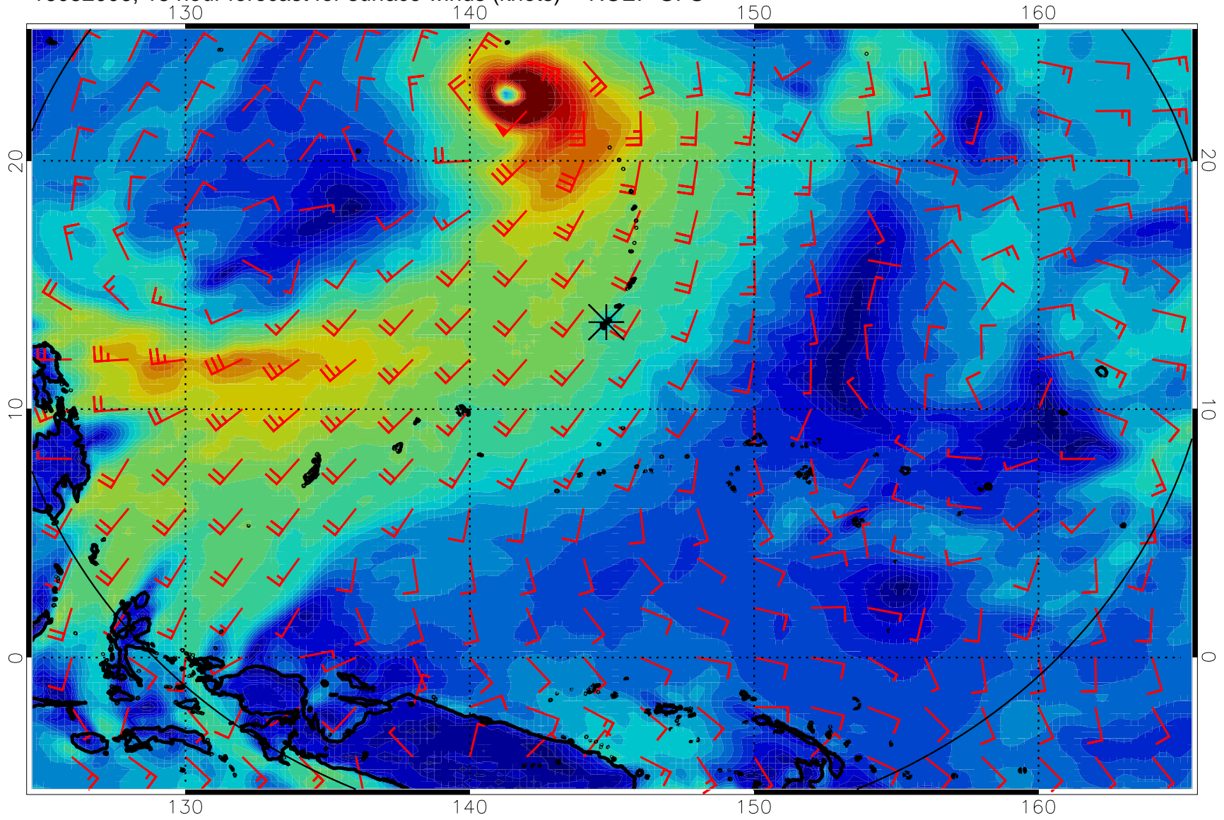
16082006, 18 hour forecast for surface winds (knots) -- NCEP GFS
