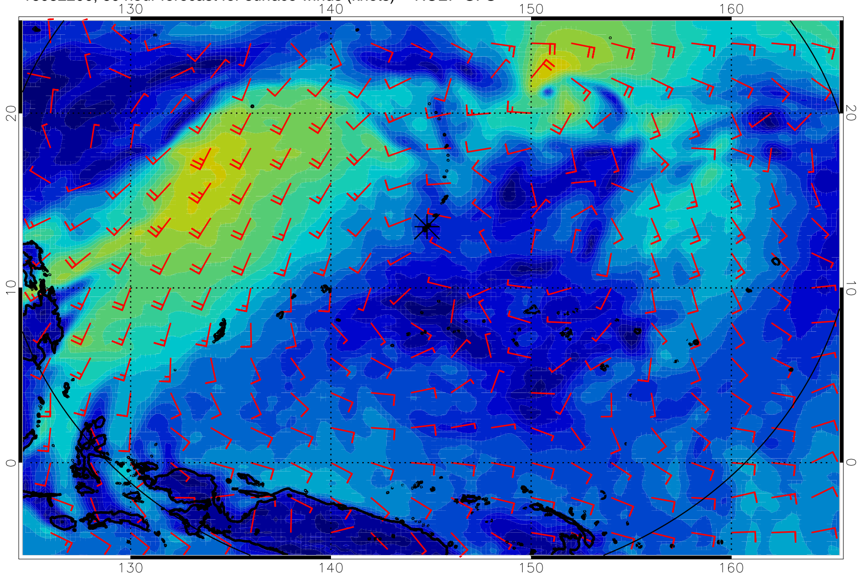
16082200, 60 hour forecast for surface winds (knots) -- NCEP GFS
