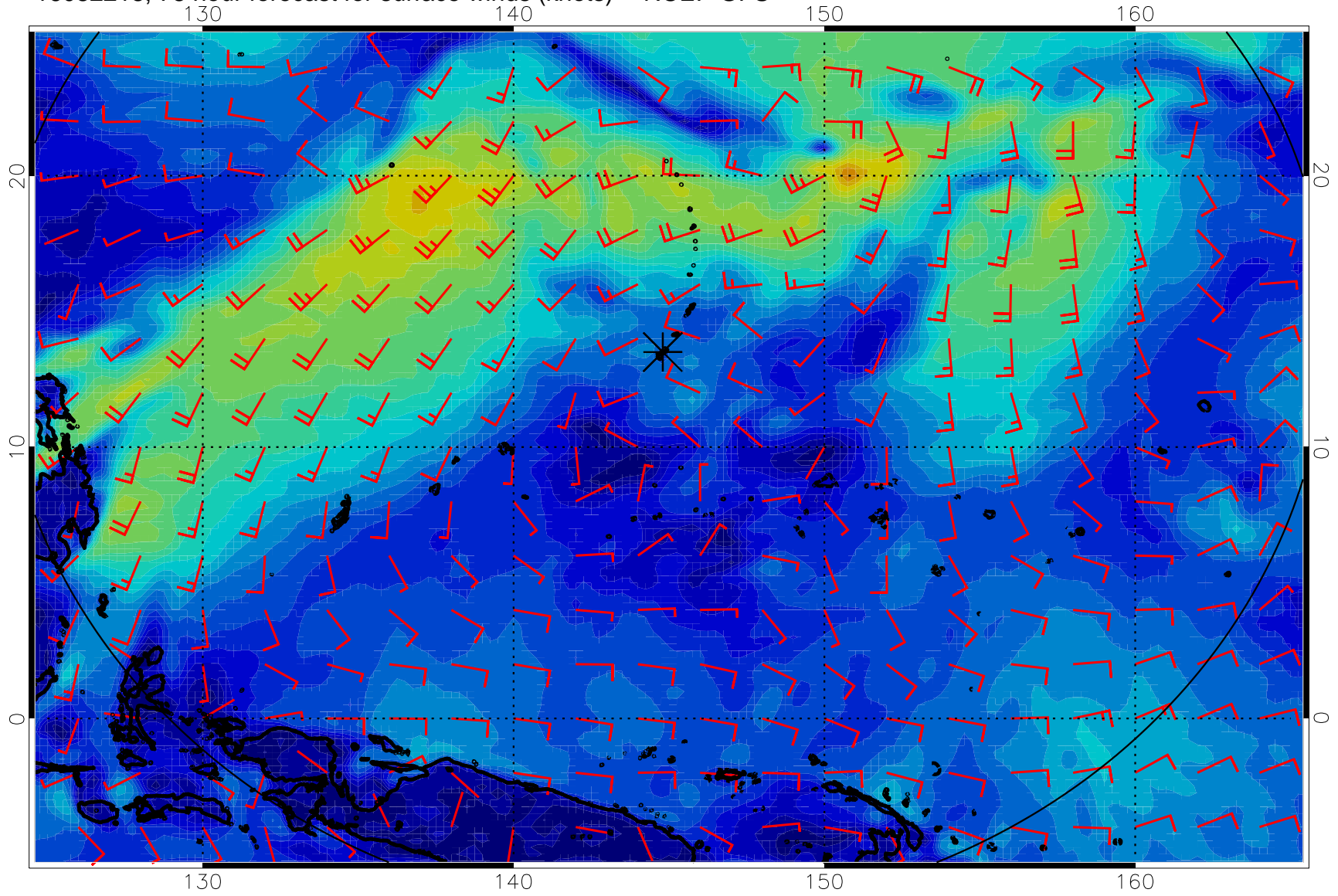
16082218, 78 hour forecast for surface winds (knots) -- NCEP GFS
