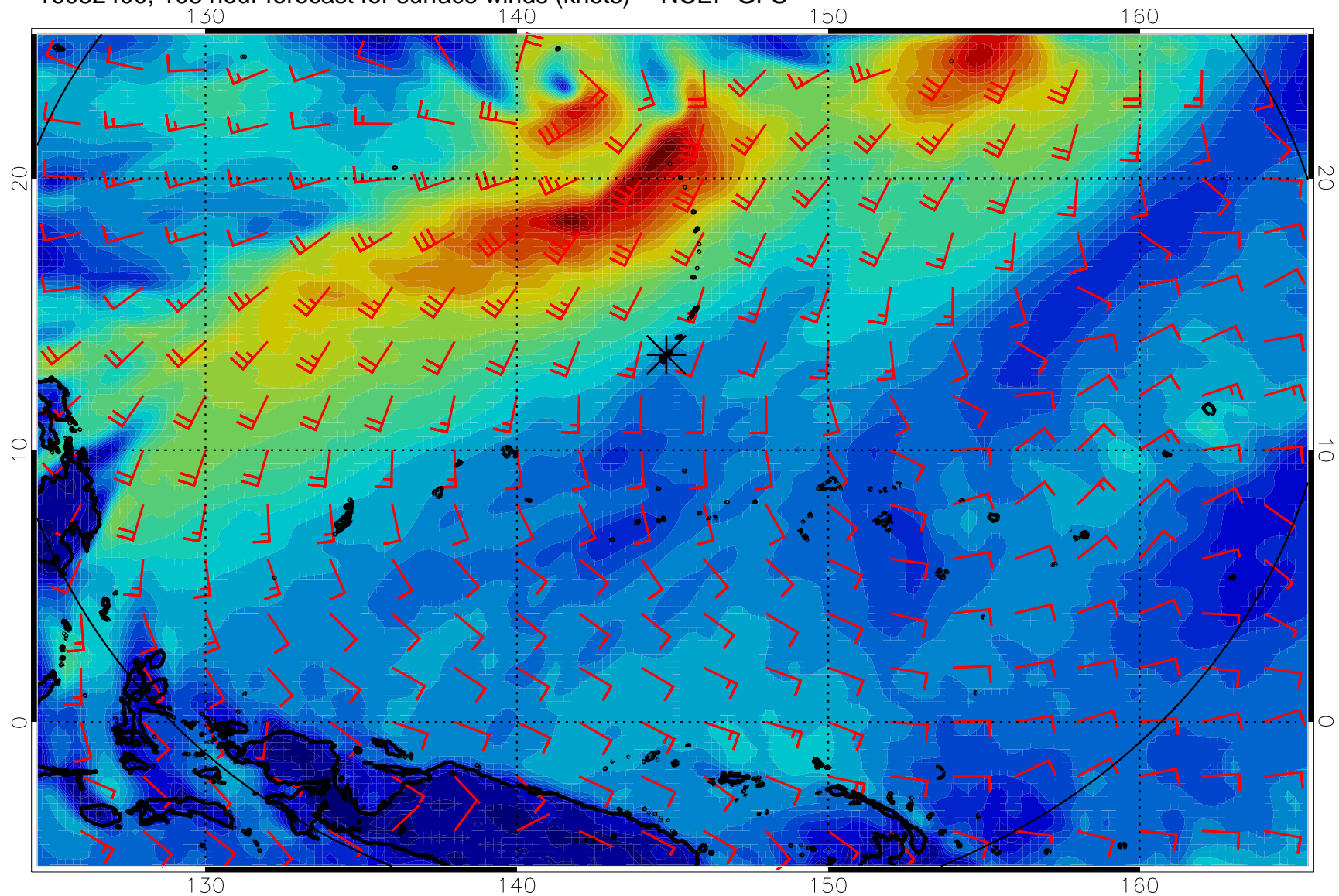
16082400, 108 hour forecast for surface winds (knots) -- NCEP GFS
