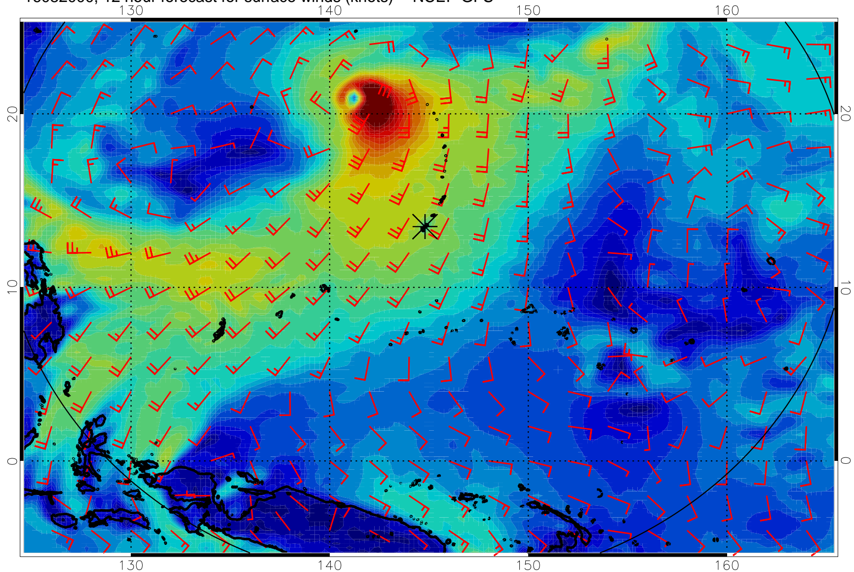
16082000, 12 hour forecast for surface winds (knots) -- NCEP GFS
