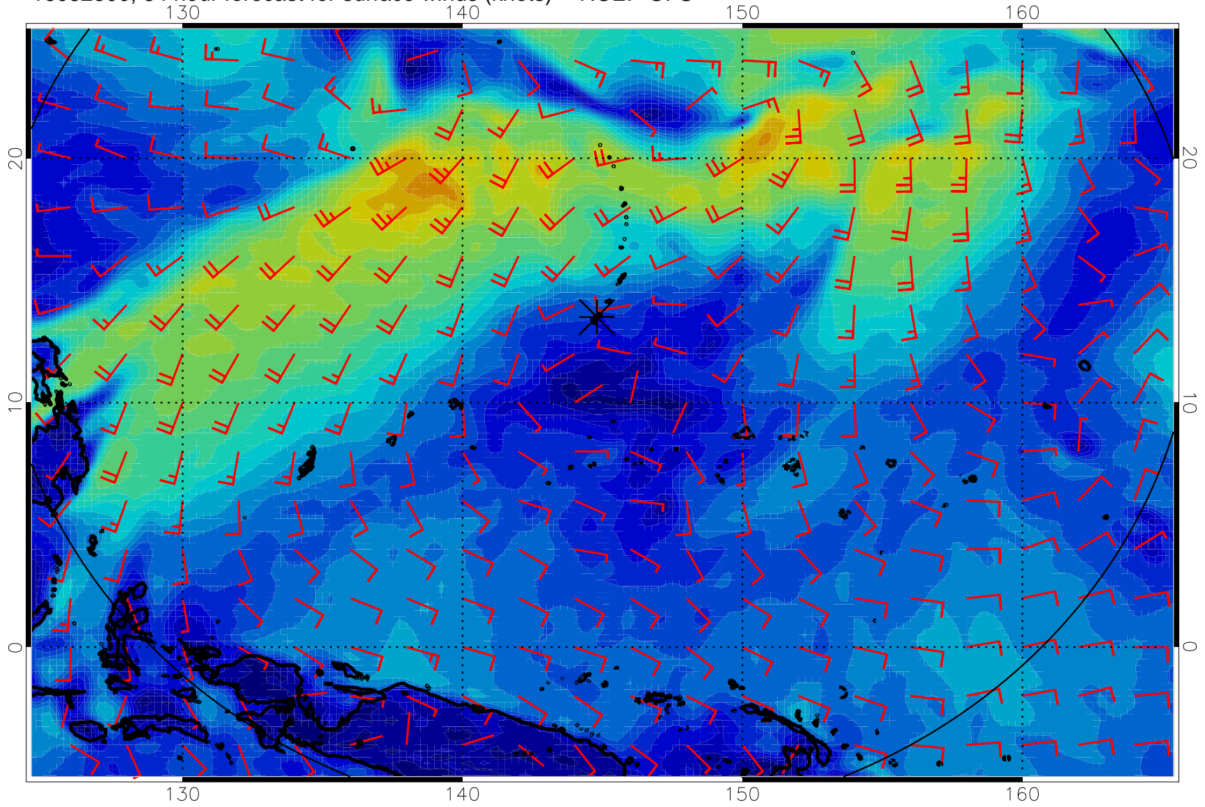
16082300, 84 hour forecast for surface winds (knots) -- NCEP GFS
