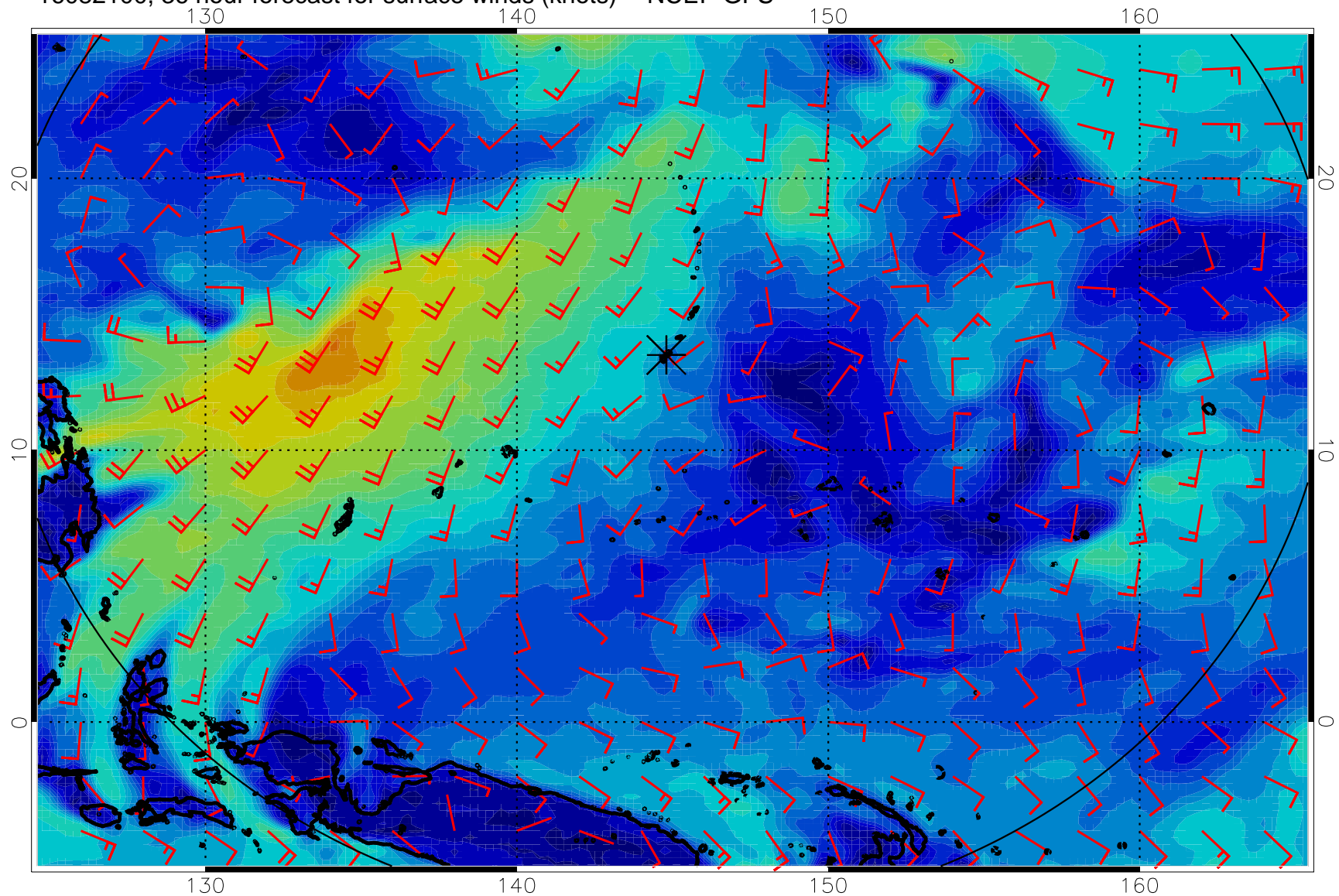
16082100, 36 hour forecast for surface winds (knots) -- NCEP GFS
