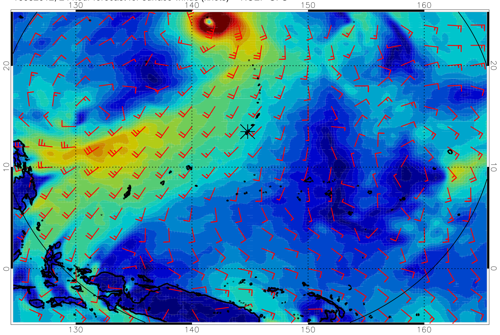
16082012, 24 hour forecast for surface winds (knots) -- NCEP GFS
