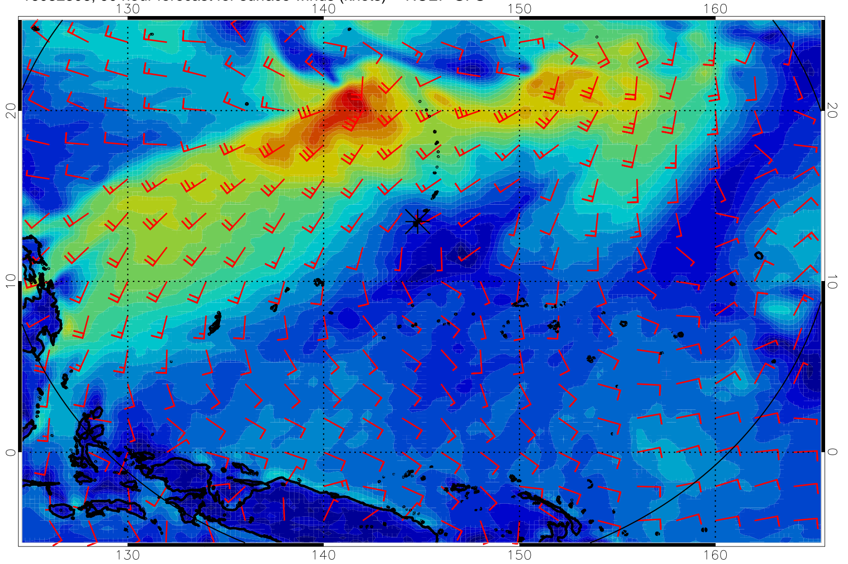
16082306, 90 hour forecast for surface winds (knots) -- NCEP GFS
