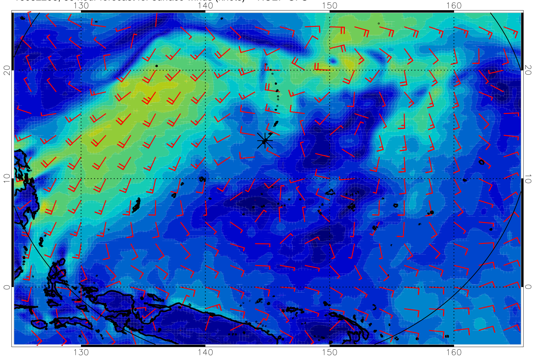
16082206, 66 hour forecast for surface winds (knots) -- NCEP GFS
