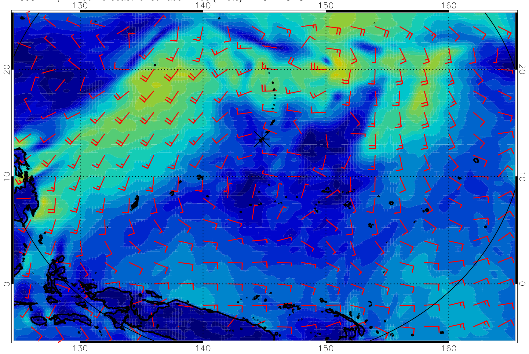
16082212, 72 hour forecast for surface winds (knots) -- NCEP GFS
