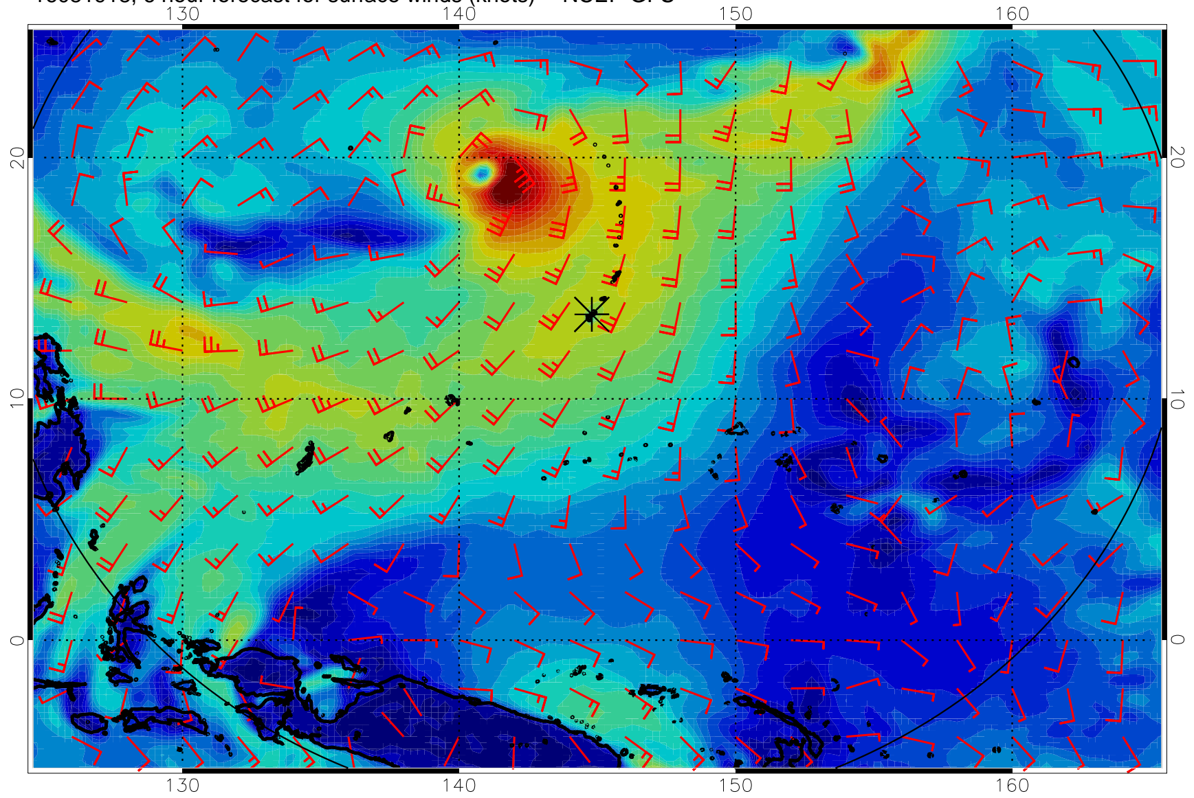
16081918, 6 hour forecast for surface winds (knots) -- NCEP GFS
