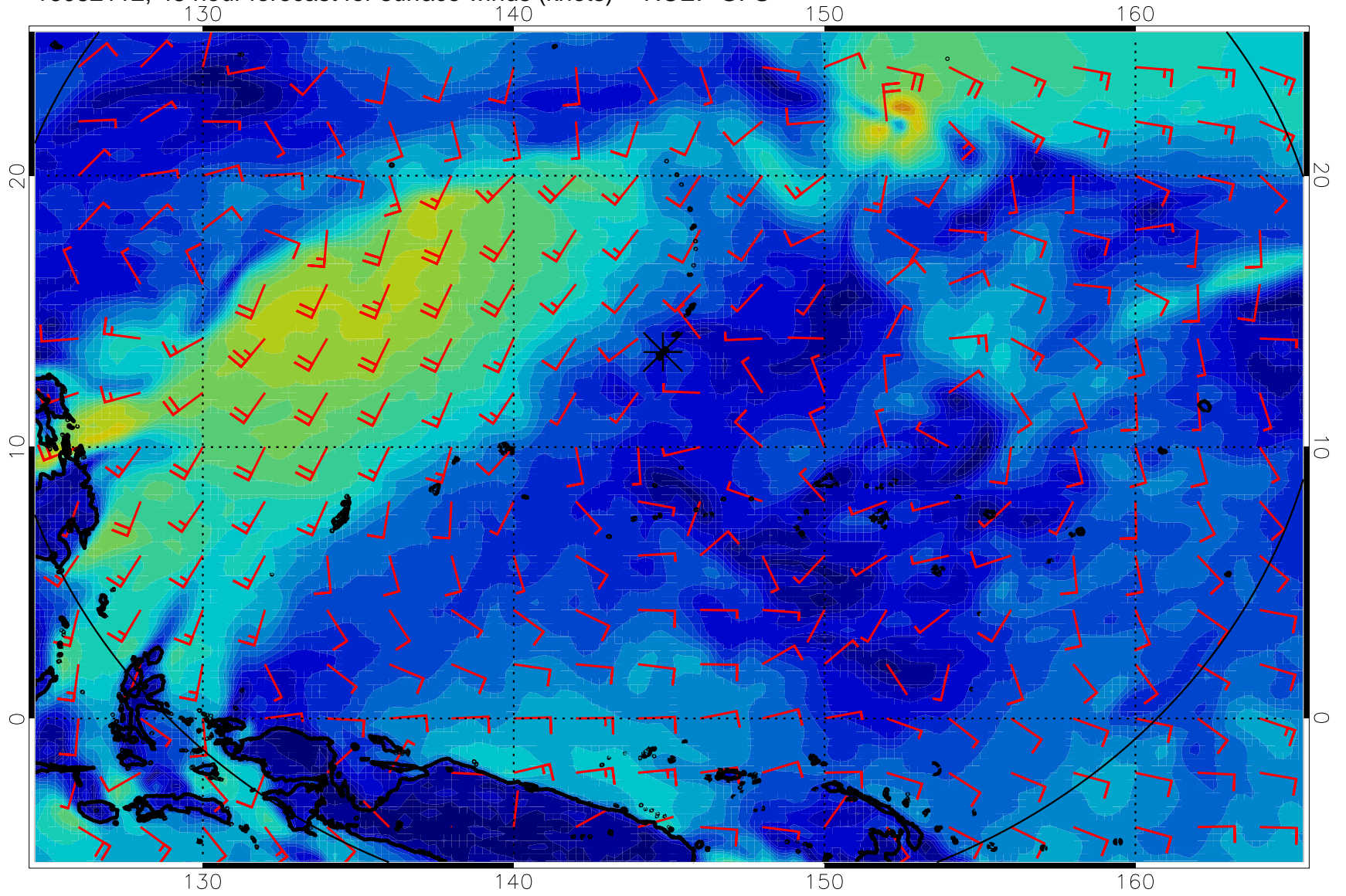
16082112, 48 hour forecast for surface winds (knots) -- NCEP GFS
