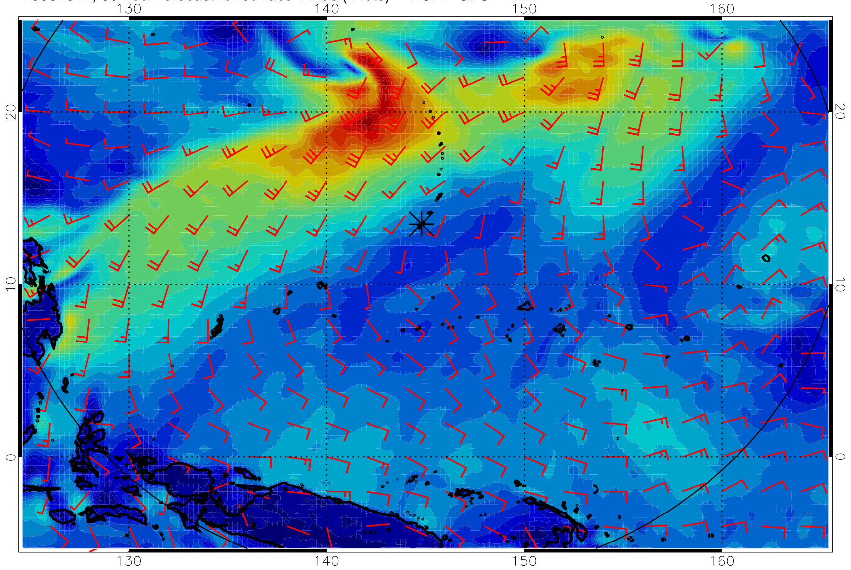
16082312, 96 hour forecast for surface winds (knots) -- NCEP GFS
