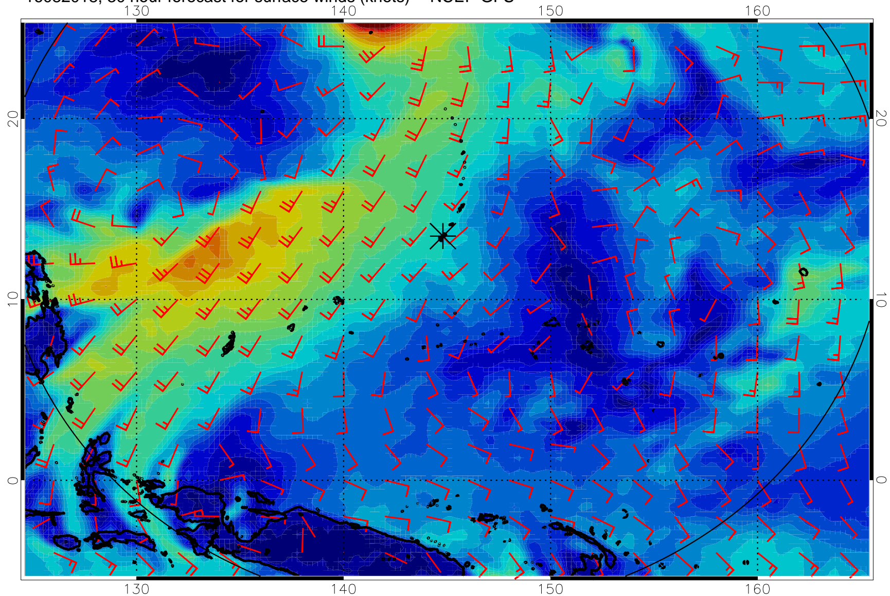
16082018, 30 hour forecast for surface winds (knots) -- NCEP GFS
