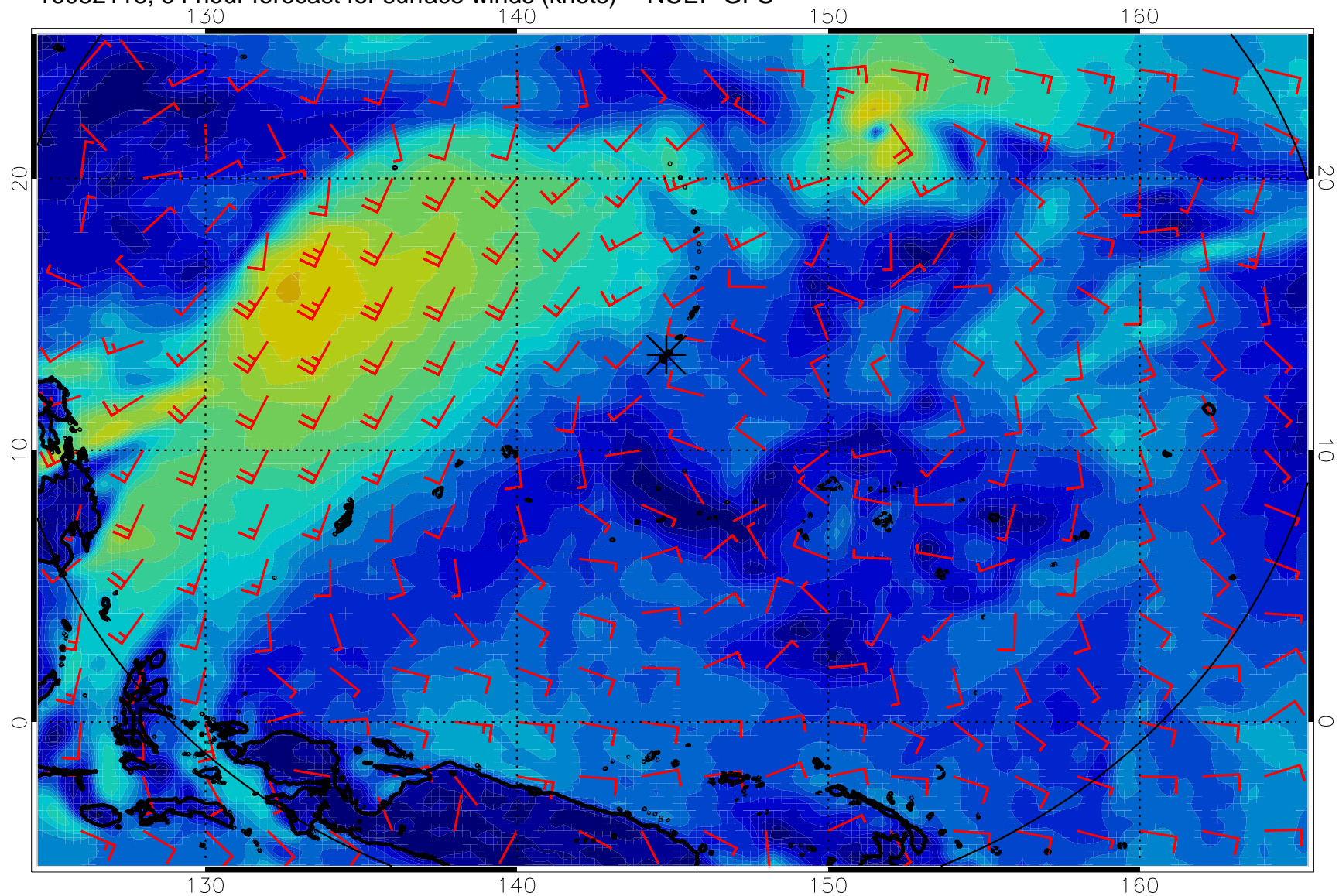
16082118, 54 hour forecast for surface winds (knots) -- NCEP GFS
