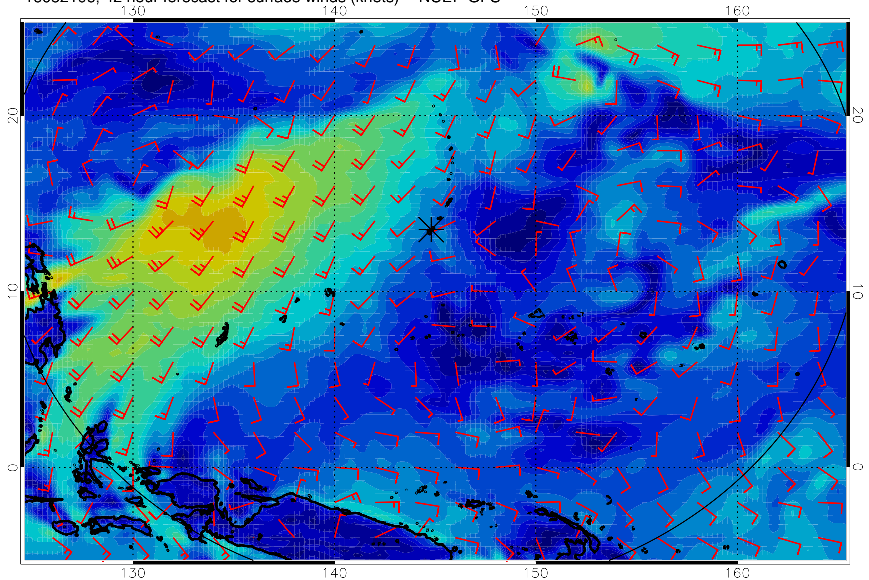
16082106, 42 hour forecast for surface winds (knots) -- NCEP GFS
