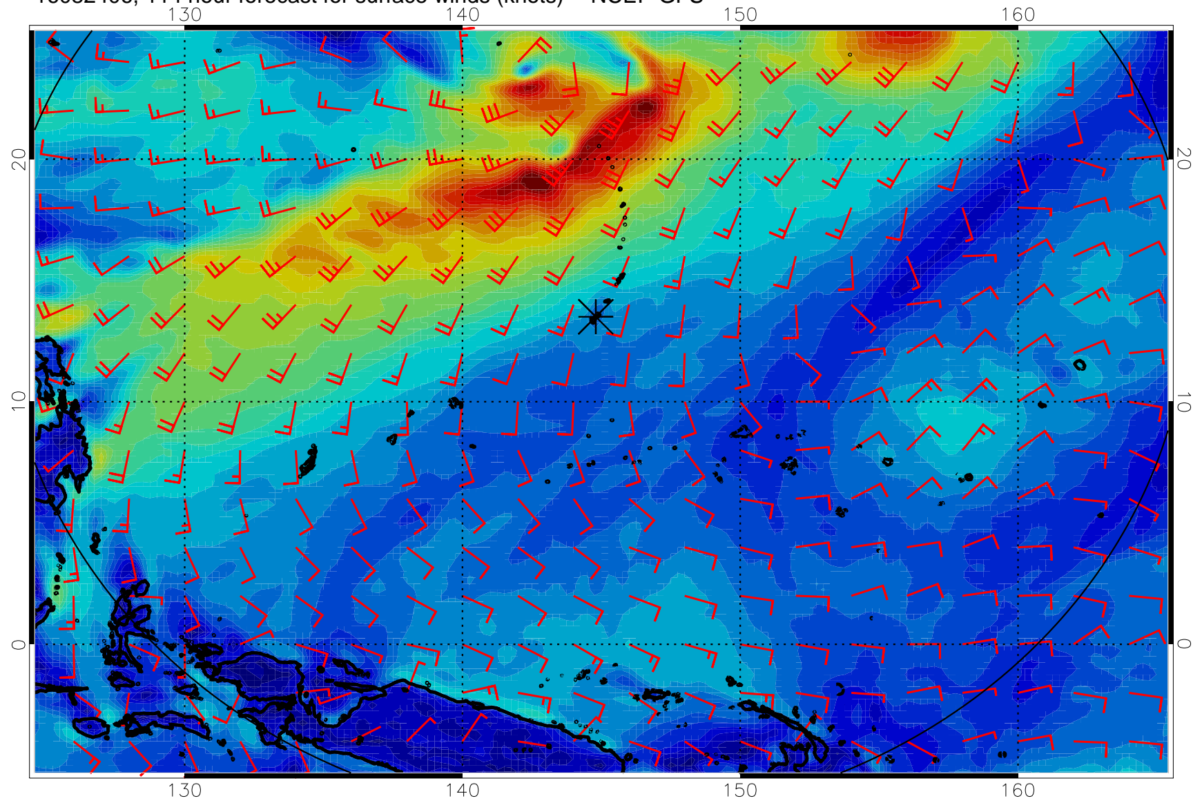
16082406, 114 hour forecast for surface winds (knots) -- NCEP GFS
