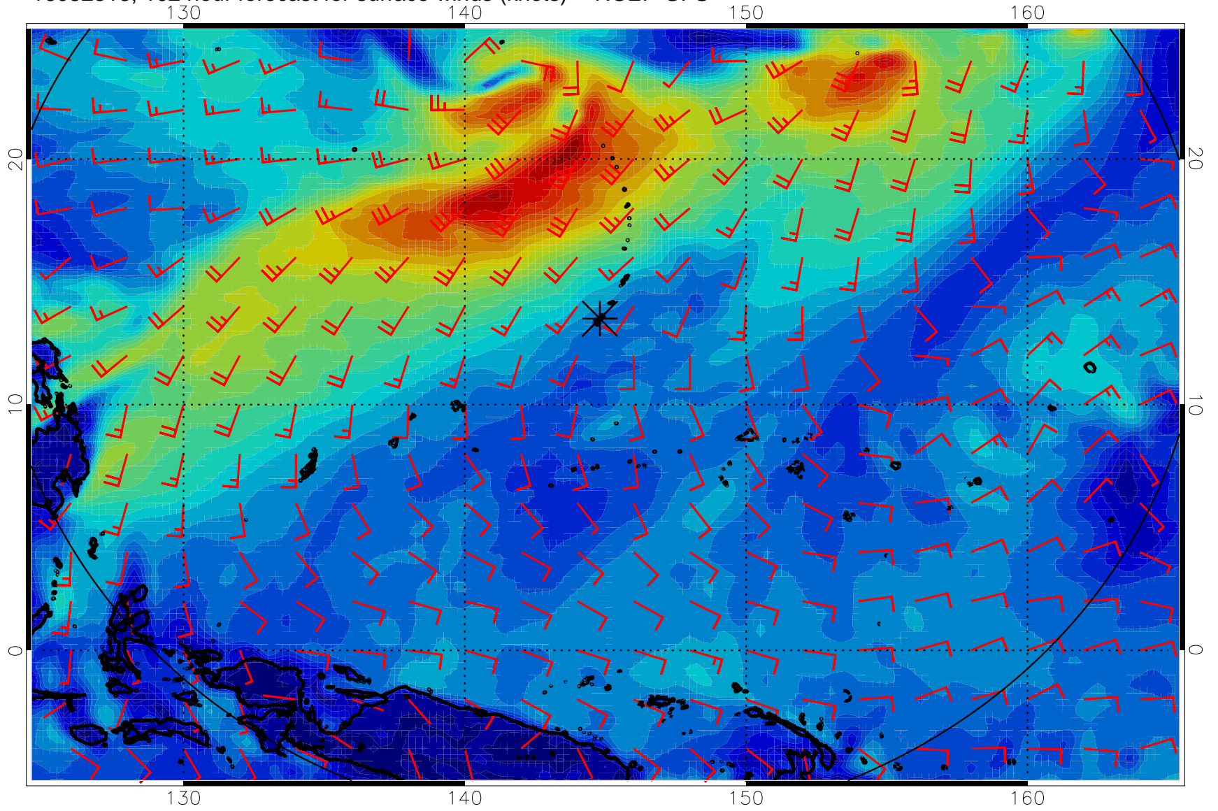
16082318, 102 hour forecast for surface winds (knots) -- NCEP GFS
