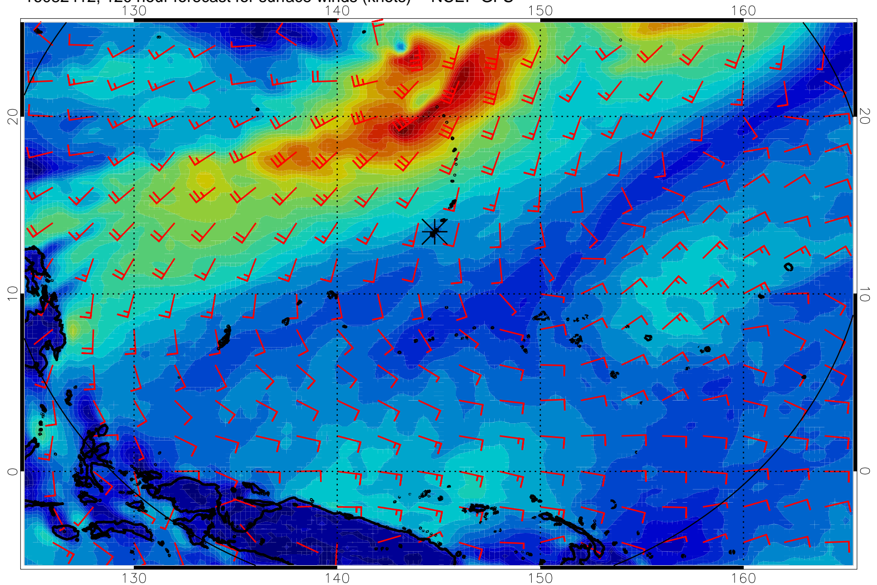
16082412, 120 hour forecast for surface winds (knots) -- NCEP GFS
