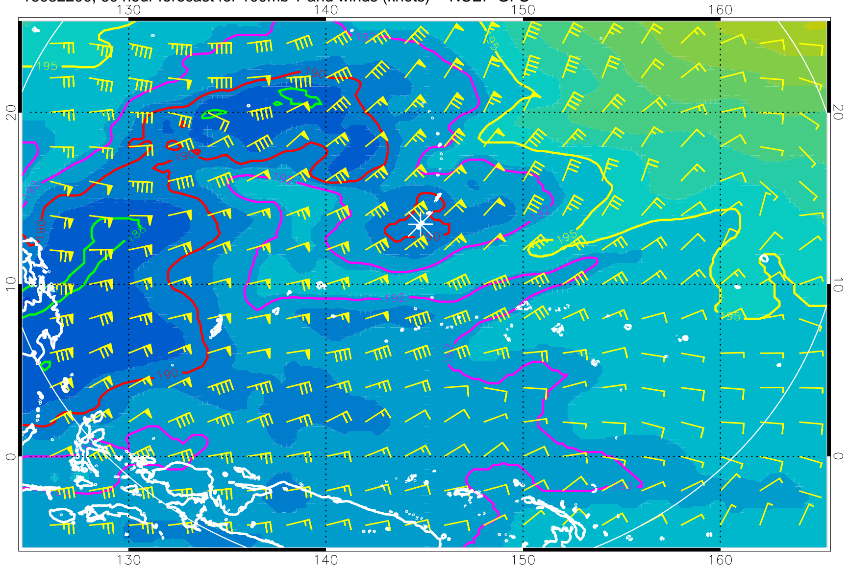
16082200, 60 hour forecast for 100mb T and winds (knots) -- NCEP GFS
