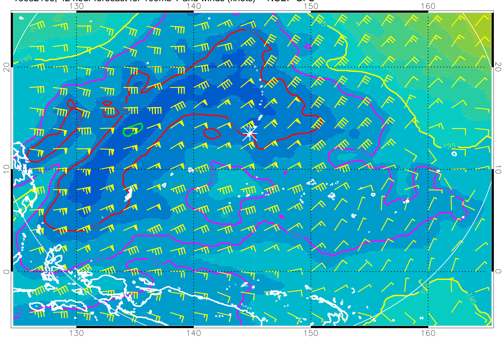
16082106, 42 hour forecast for 100mb T and winds (knots) -- NCEP GFS
