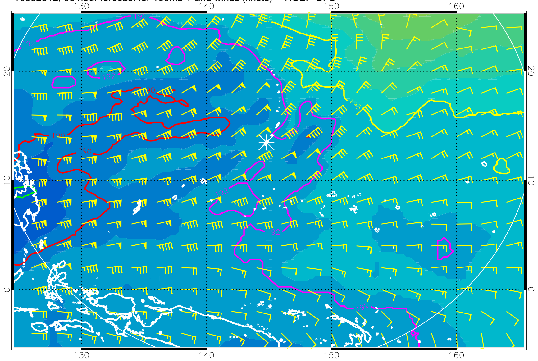
16082312, 96 hour forecast for 100mb T and winds (knots) -- NCEP GFS
