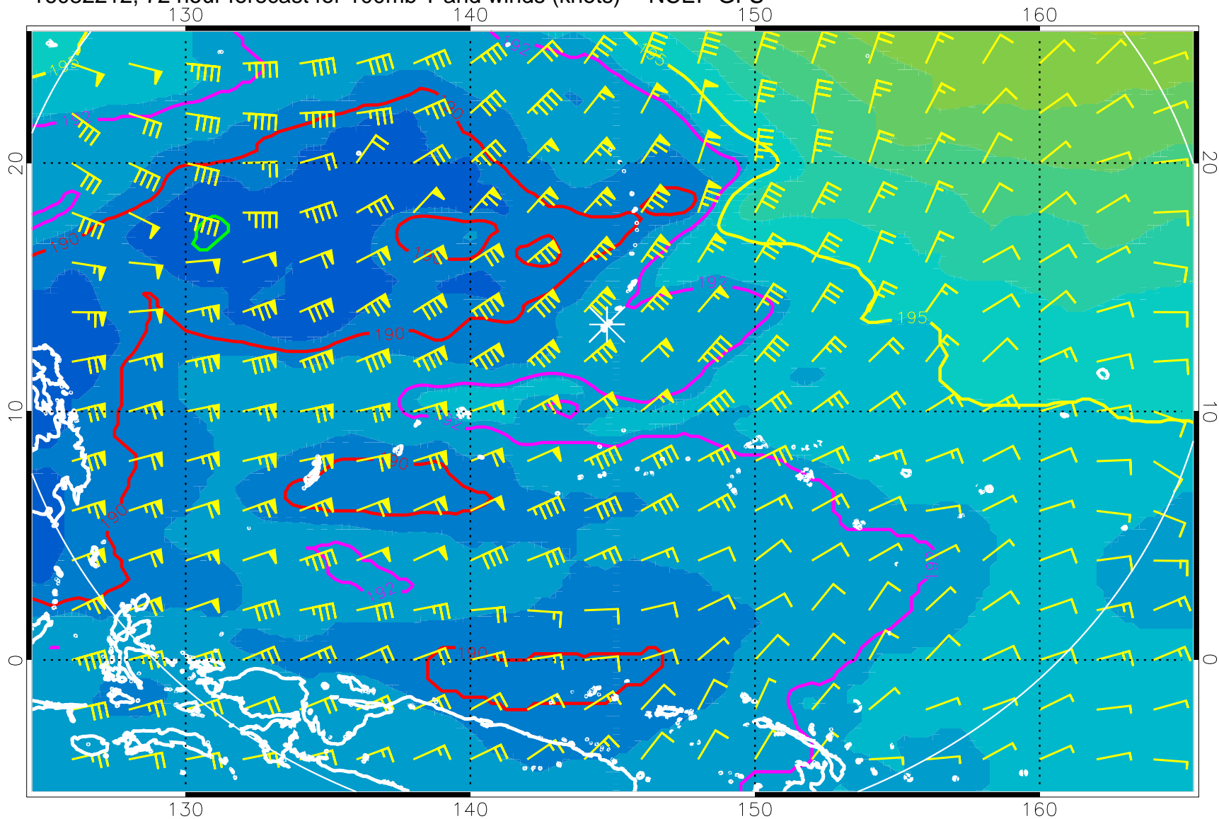
16082212, 72 hour forecast for 100mb T and winds (knots) -- NCEP GFS
