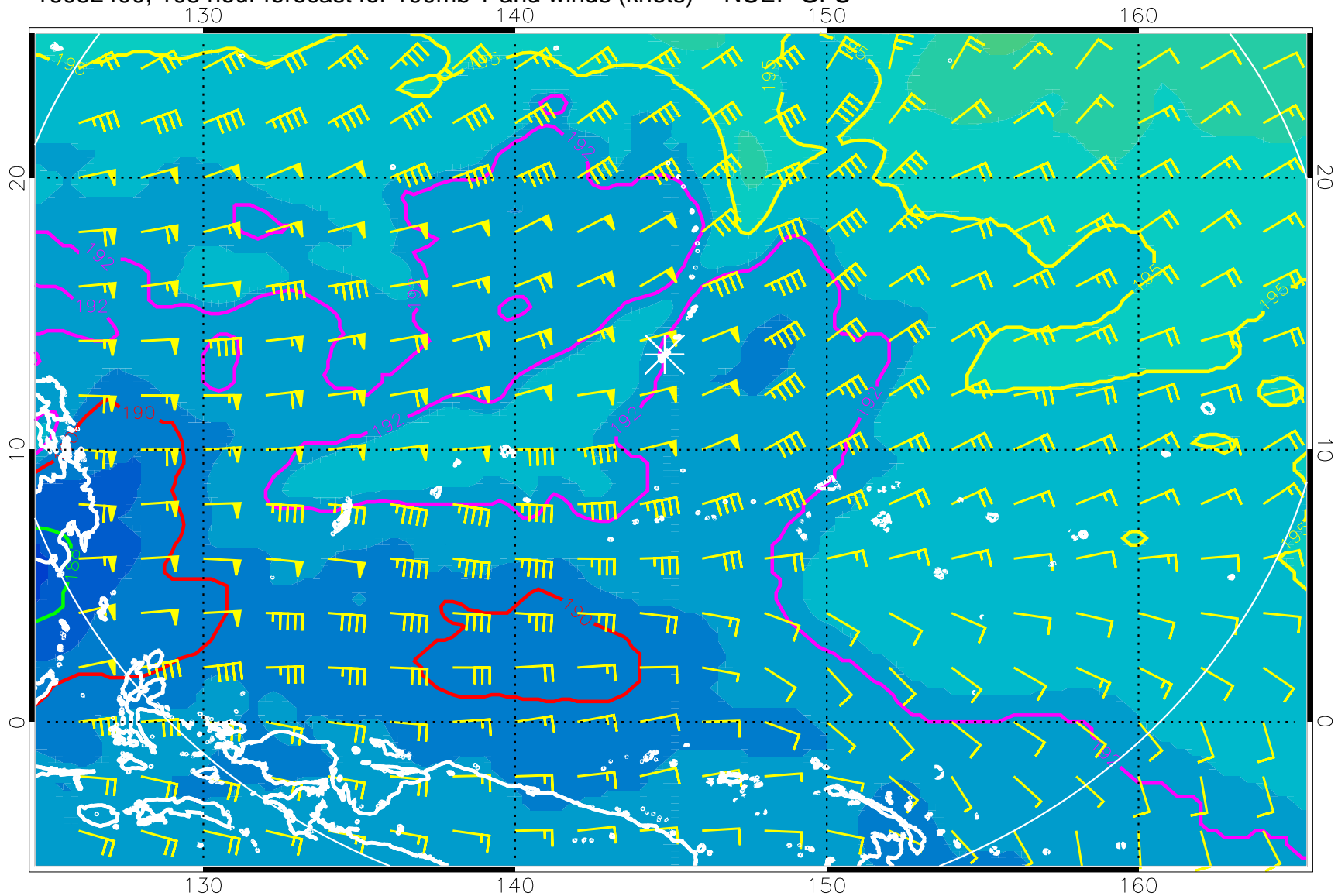
16082400, 108 hour forecast for 100mb T and winds (knots) -- NCEP GFS
