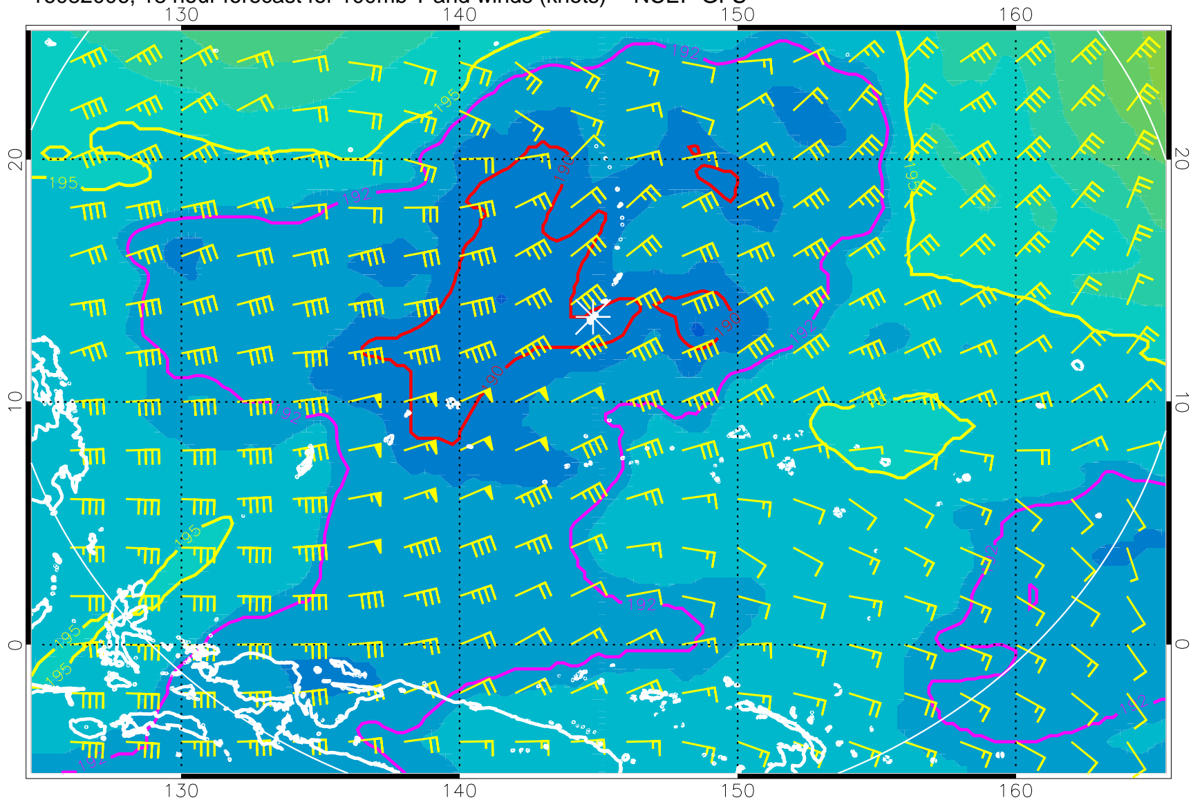
16082006, 18 hour forecast for 100mb T and winds (knots) -- NCEP GFS
