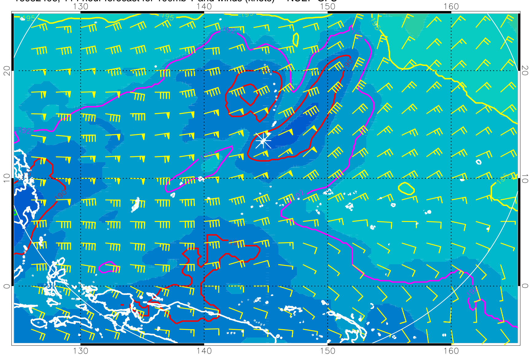
16082406, 114 hour forecast for 100mb T and winds (knots) -- NCEP GFS
