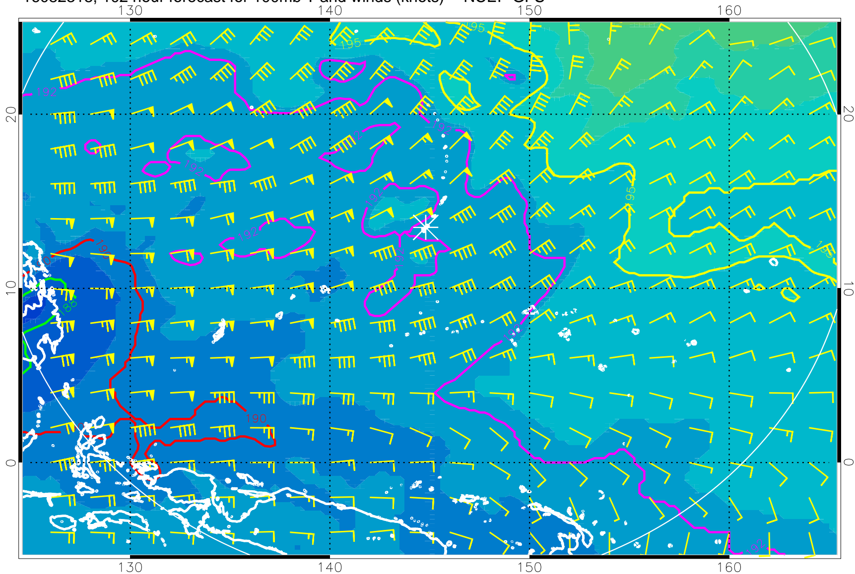
16082318, 102 hour forecast for 100mb T and winds (knots) -- NCEP GFS
