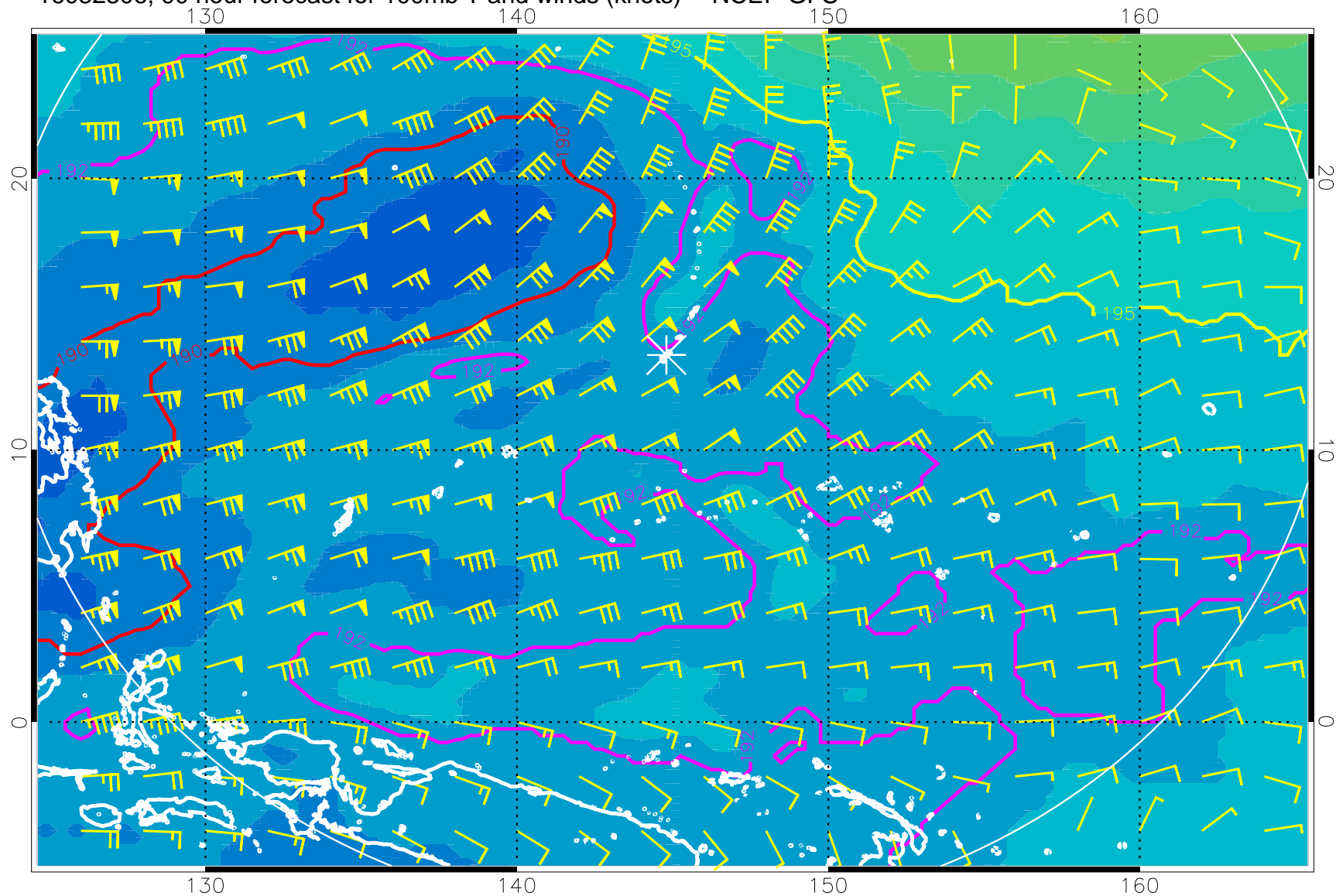
16082306, 90 hour forecast for 100mb T and winds (knots) -- NCEP GFS
