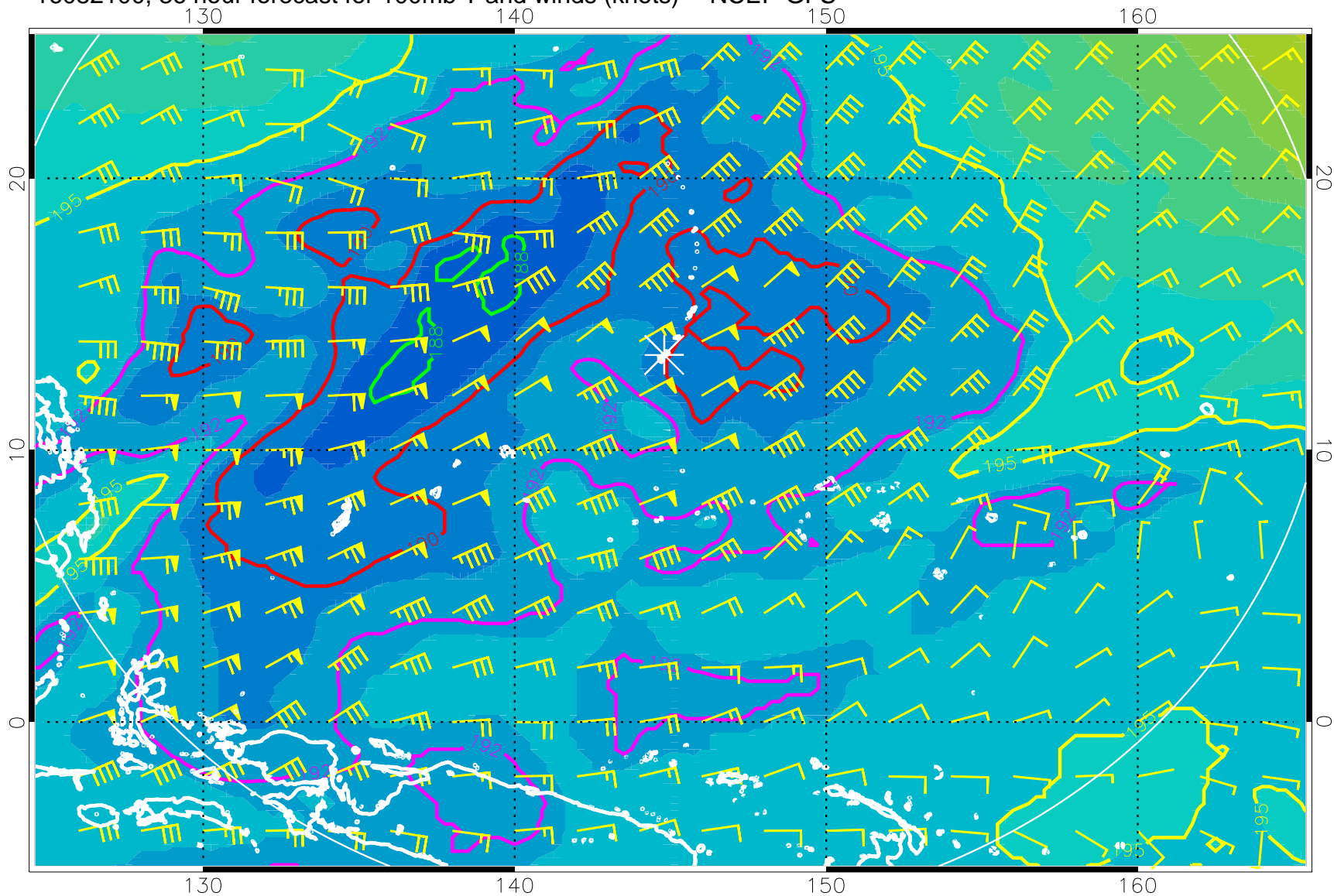
16082100, 36 hour forecast for 100mb T and winds (knots) -- NCEP GFS
