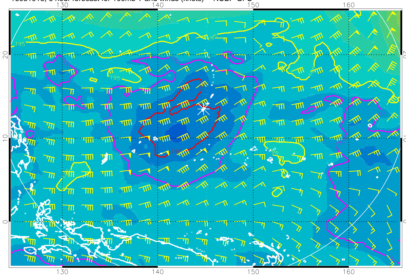
16081918, 6 hour forecast for 100mb T and winds (knots) -- NCEP GFS
