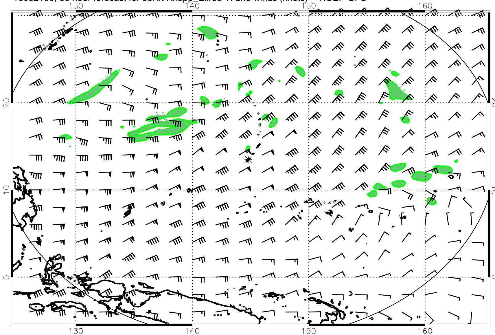
16082100, 36 hour forecast for 53Kft Knapp_Ellrod TI and winds (knots) -- NCEP GFS
