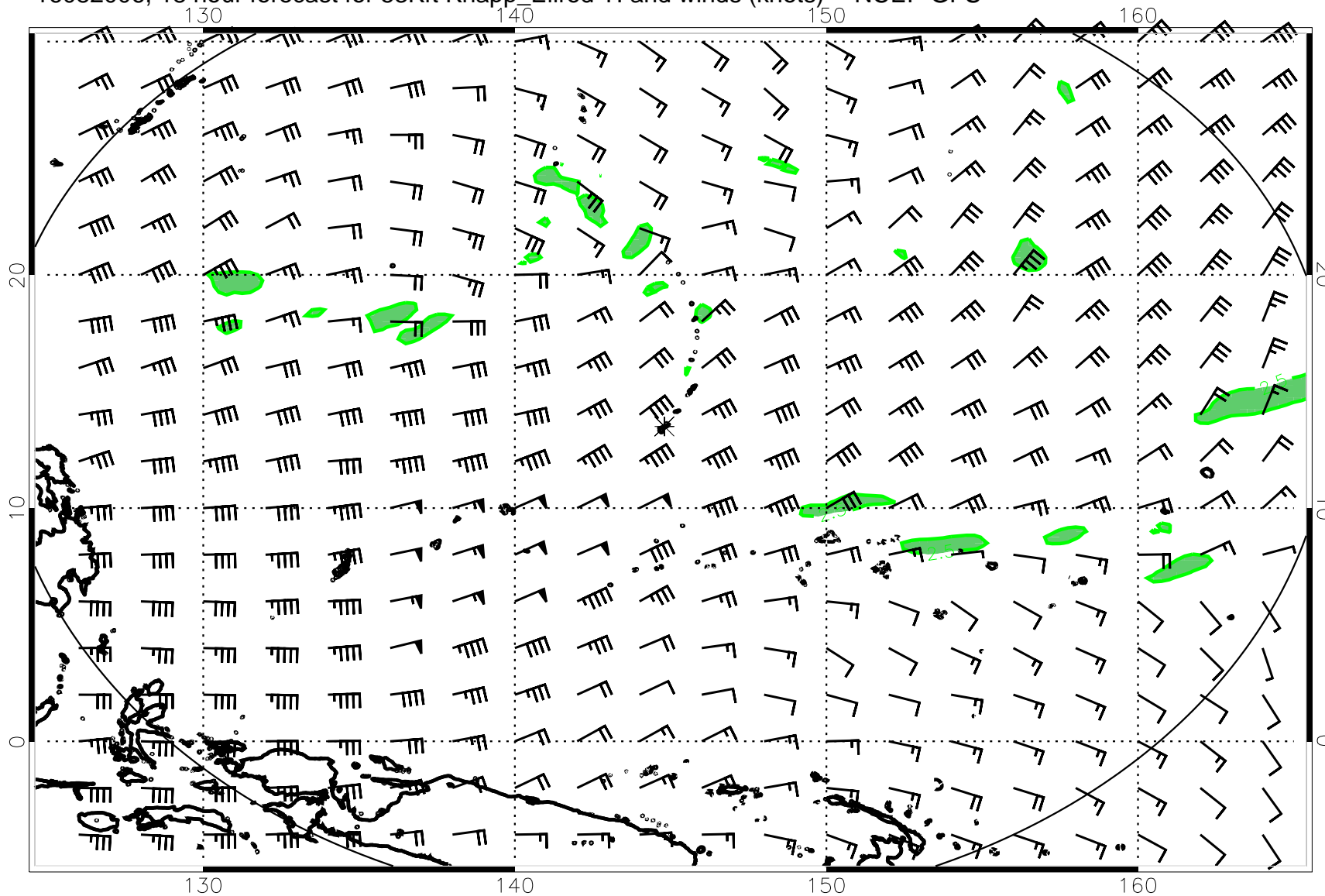
16082006, 18 hour forecast for 53Kft Knapp_Ellrod TI and winds (knots) -- NCEP GFS
