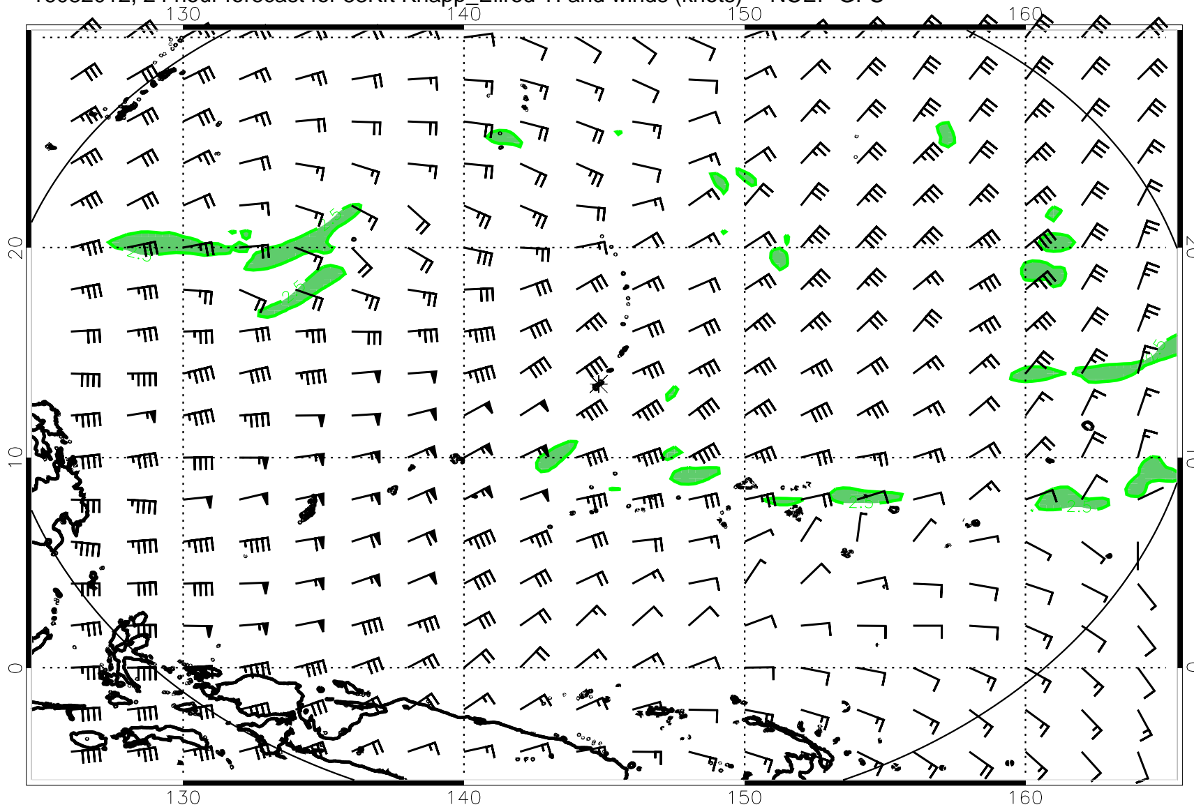
16082012, 24 hour forecast for 53Kft Knapp_Ellrod TI and winds (knots) -- NCEP GFS
