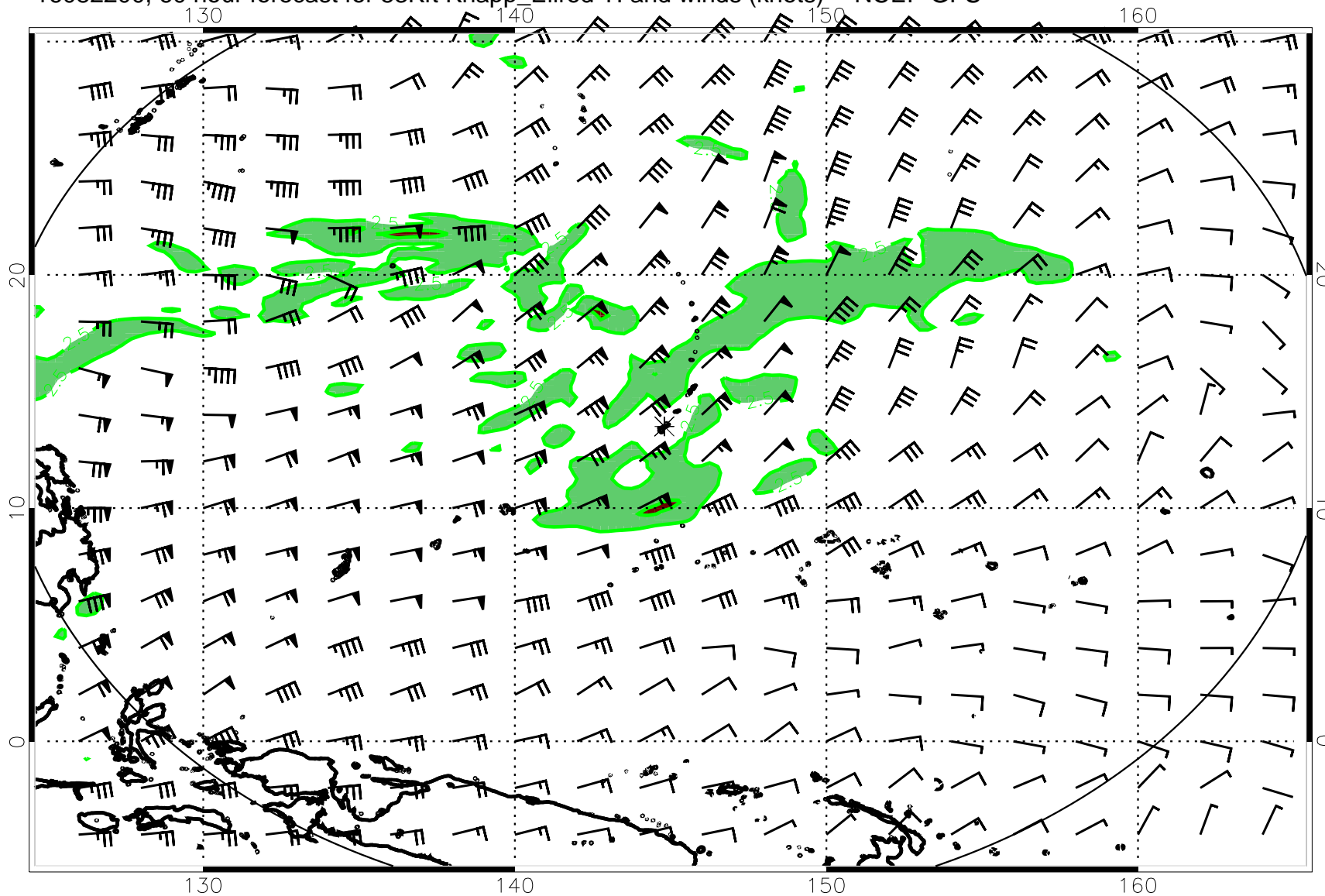
16082200, 60 hour forecast for 53Kft Knapp_Ellrod TI and winds (knots) -- NCEP GFS
