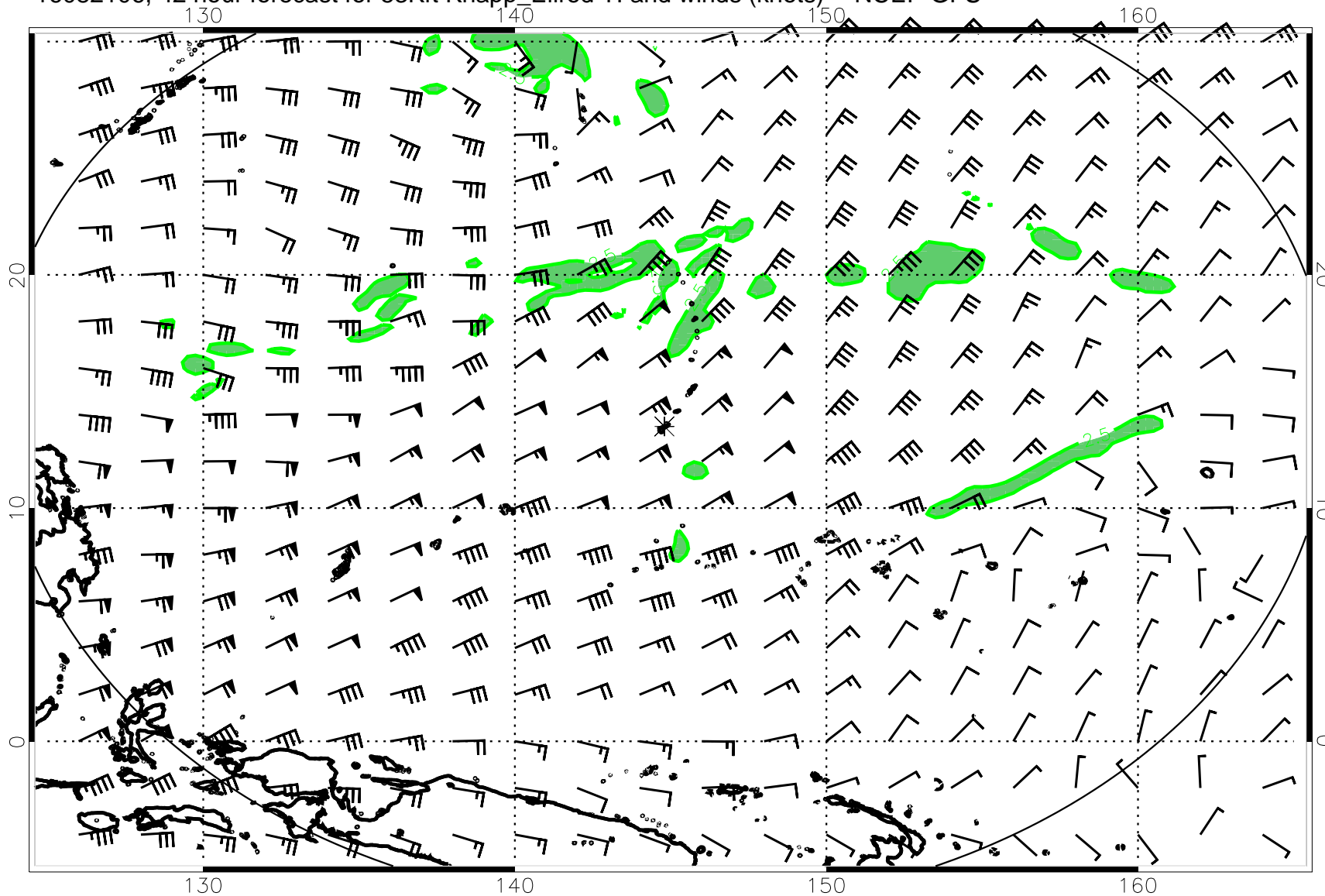
16082106, 42 hour forecast for 53Kft Knapp_Ellrod TI and winds (knots) -- NCEP GFS
