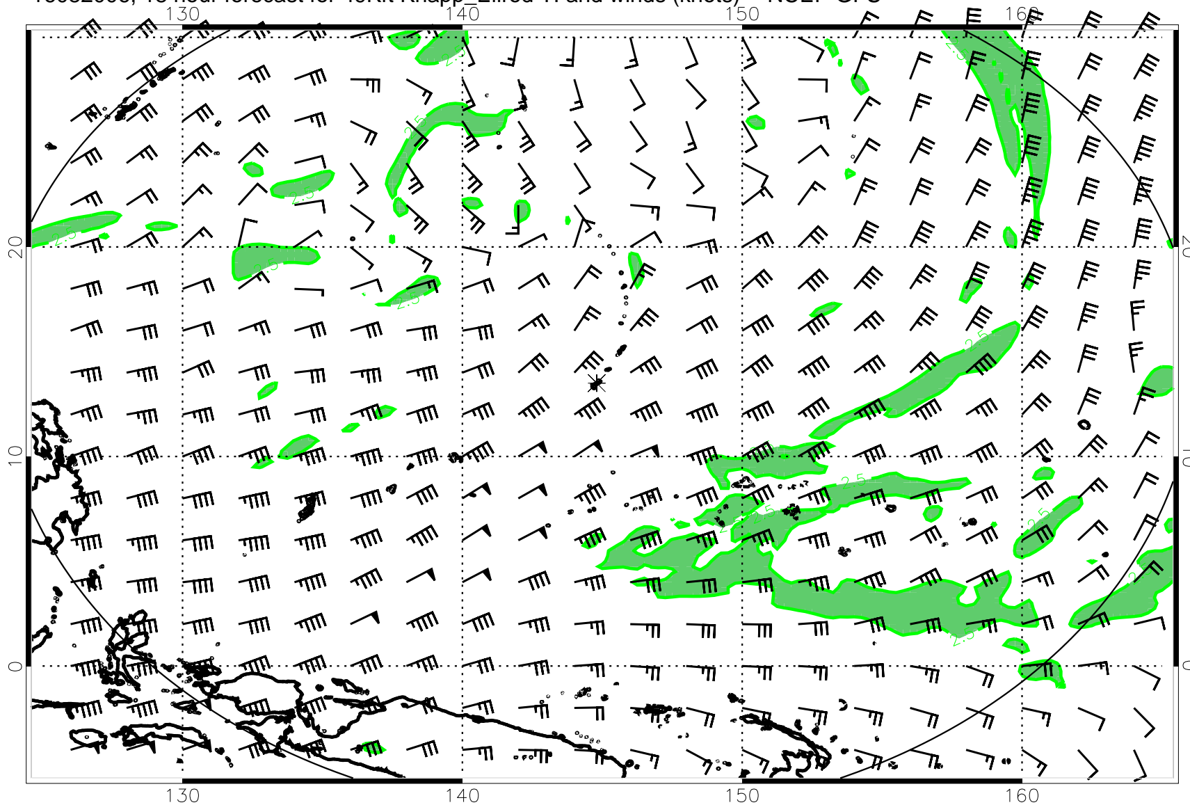
16082006, 18 hour forecast for 49Kft Knapp_Ellrod TI and winds (knots) -- NCEP GFS
