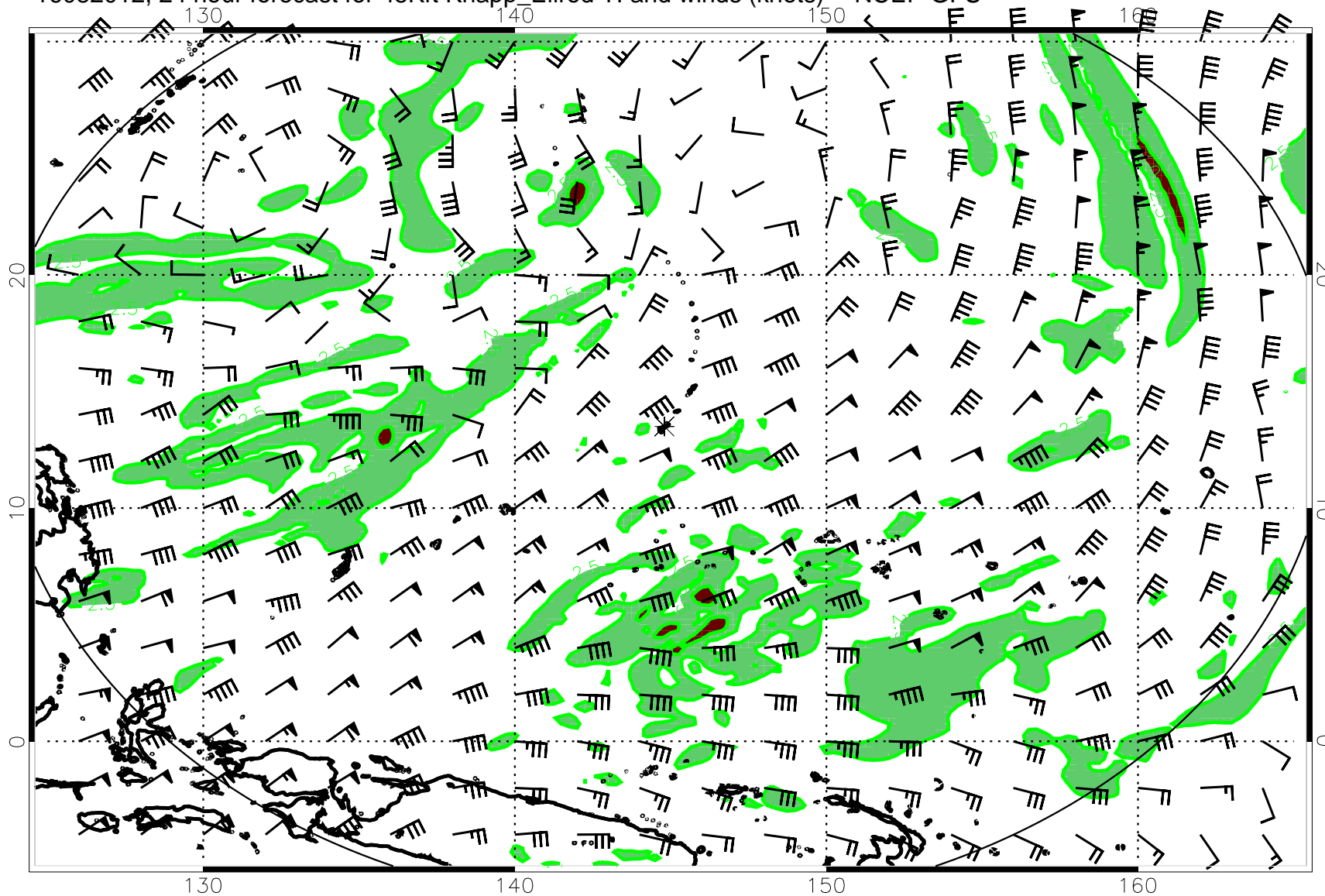
16082012, 24 hour forecast for 45Kft Knapp_Ellrod TI and winds (knots) -- NCEP GFS
