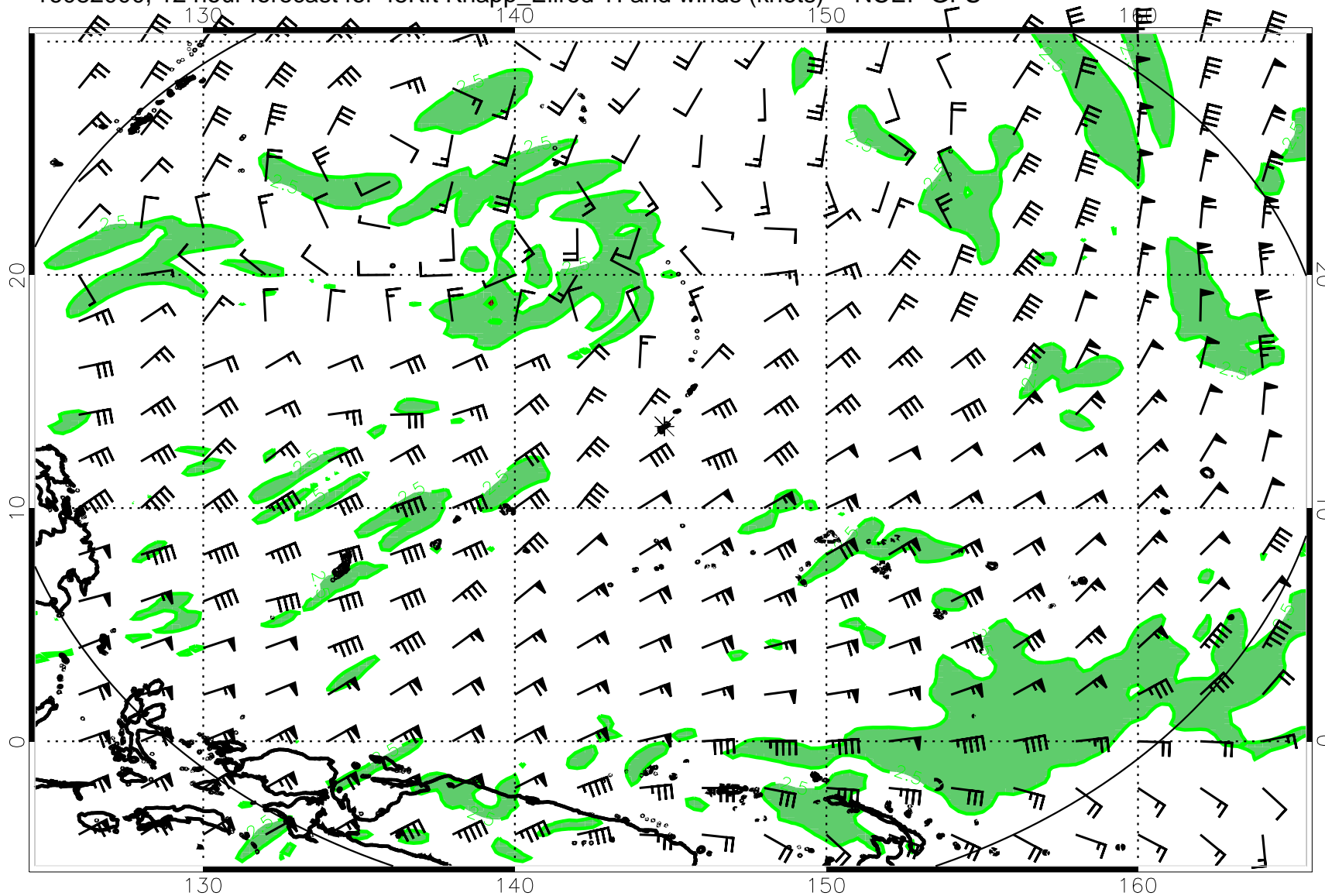
16082000, 12 hour forecast for 45Kft Knapp_Ellrod TI and winds (knots) -- NCEP GFS
