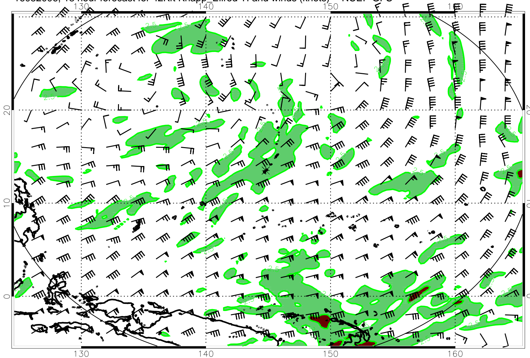
16082006, 18 hour forecast for 42Kft Knapp_Ellrod TI and winds (knots) -- NCEP GFS
