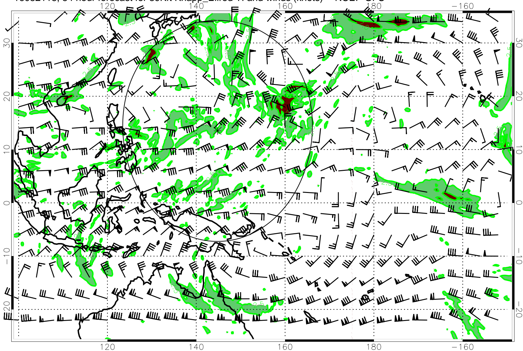
16082118, 54 hour forecast for 39Kft Knapp_Ellrod TI and winds (knots) -- NCEP GFS
