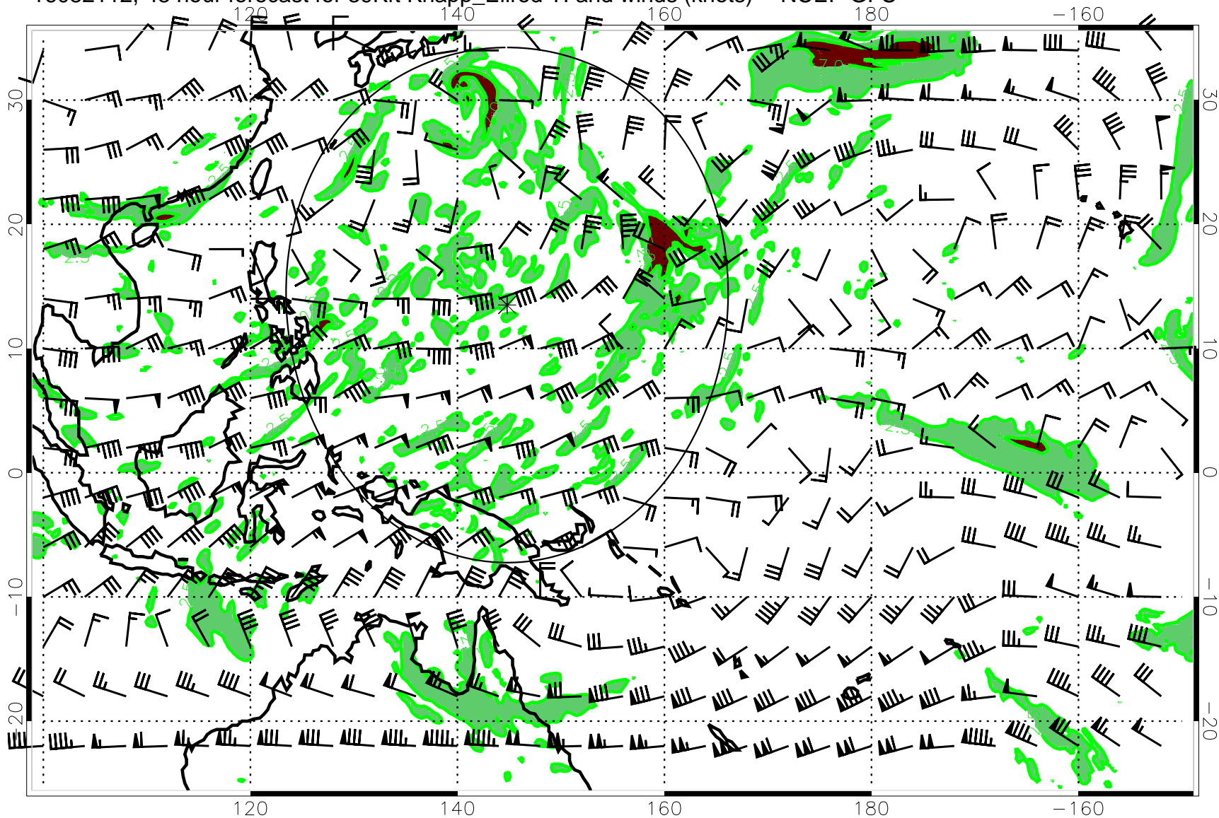
16082112, 48 hour forecast for 39Kft Knapp_Ellrod TI and winds (knots) -- NCEP GFS
