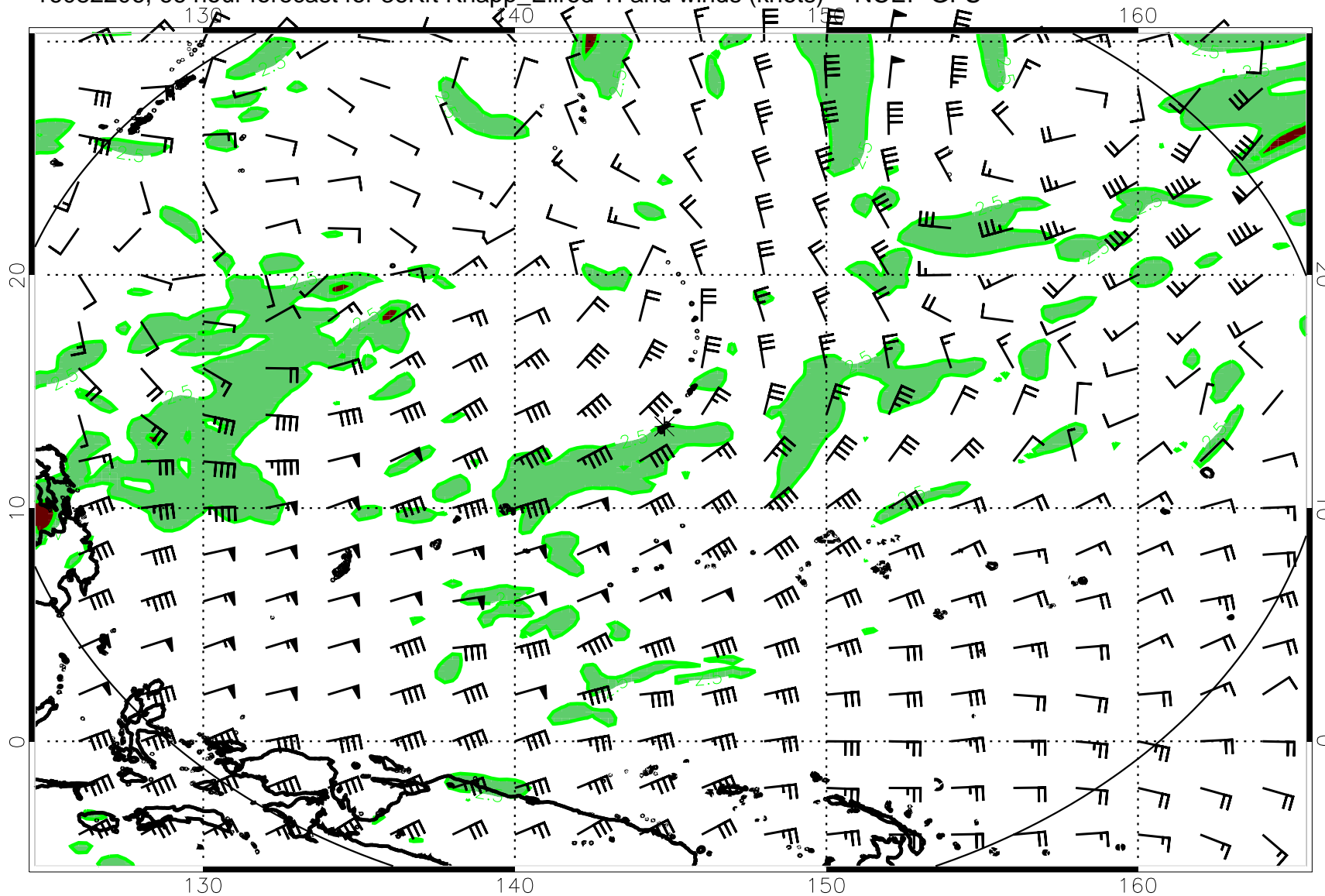
16082206, 66 hour forecast for 36Kft Knapp_Ellrod TI and winds (knots) -- NCEP GFS
