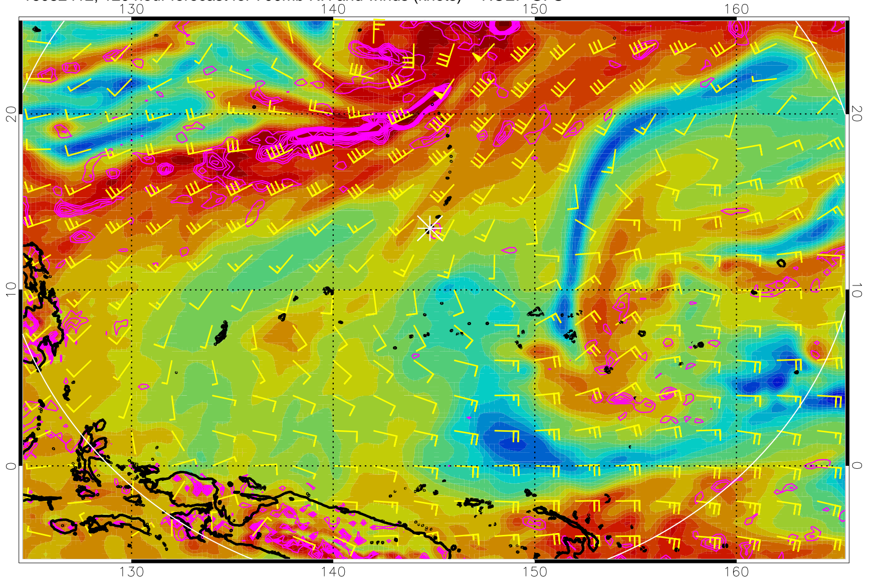
16082412, 120 hour forecast for 700mb RH and winds (knots) -- NCEP GFS
