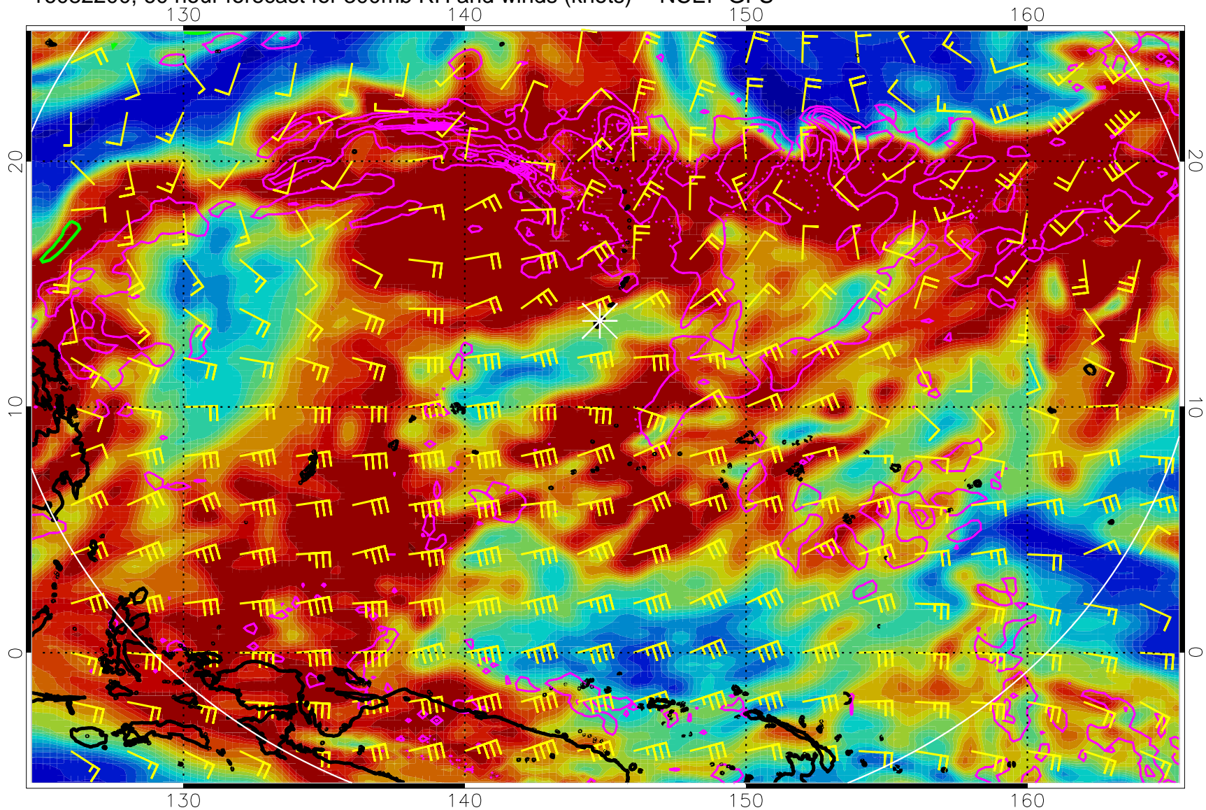
16082200, 60 hour forecast for 300mb RH and winds (knots) -- NCEP GFS
