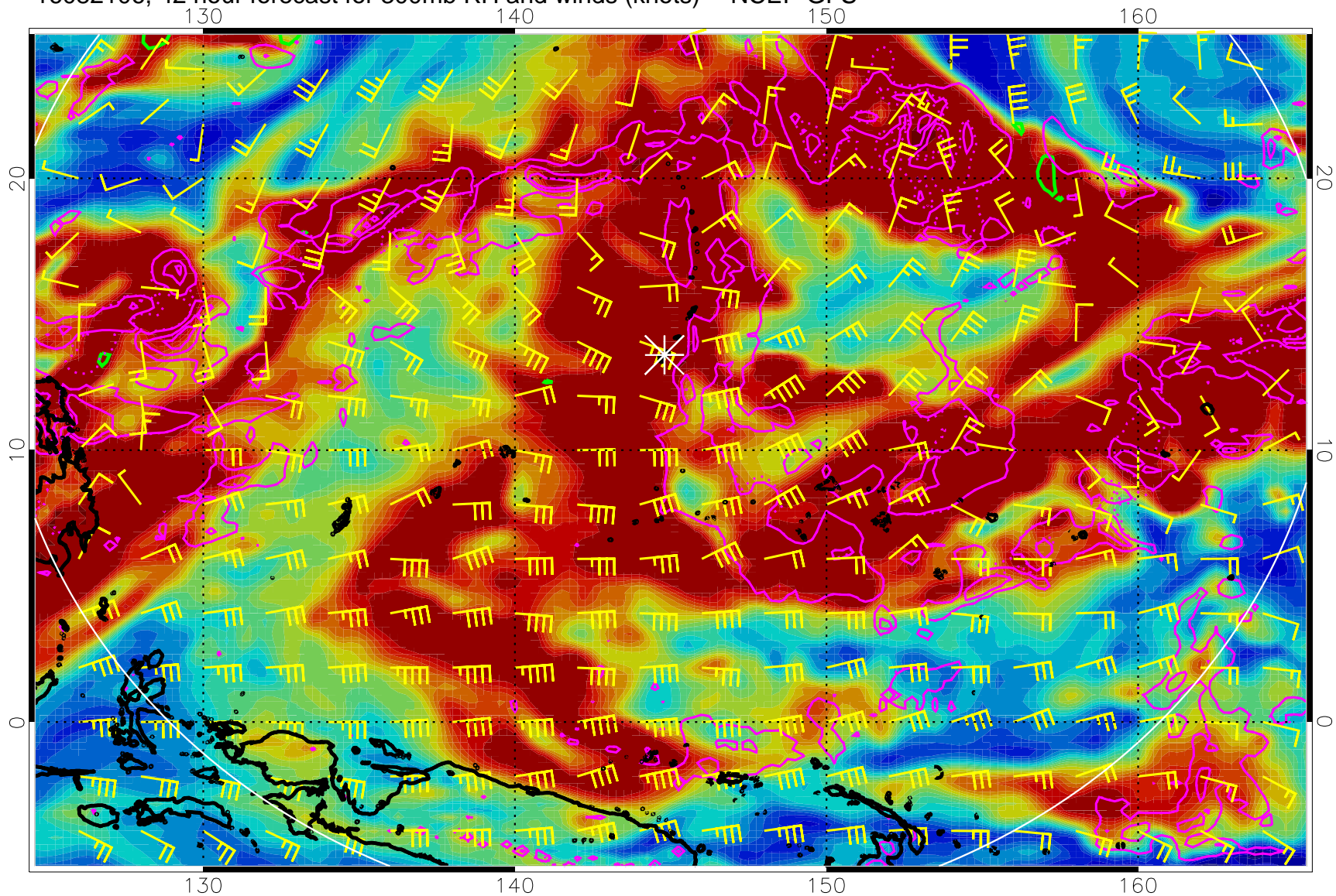
16082106, 42 hour forecast for 300mb RH and winds (knots) -- NCEP GFS
