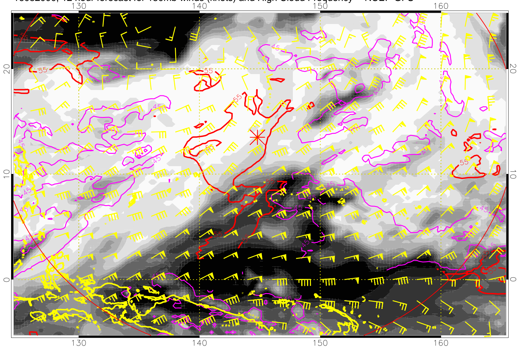
16082000, 12 hour forecast for 150mb winds (knots) and High Cloud Frequency -- NCEP GFS
