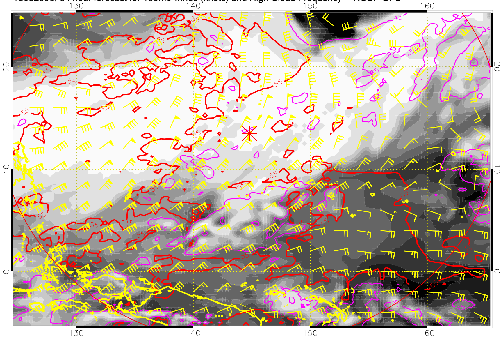
16082300, 84 hour forecast for 150mb winds (knots) and High Cloud Frequency -- NCEP GFS
