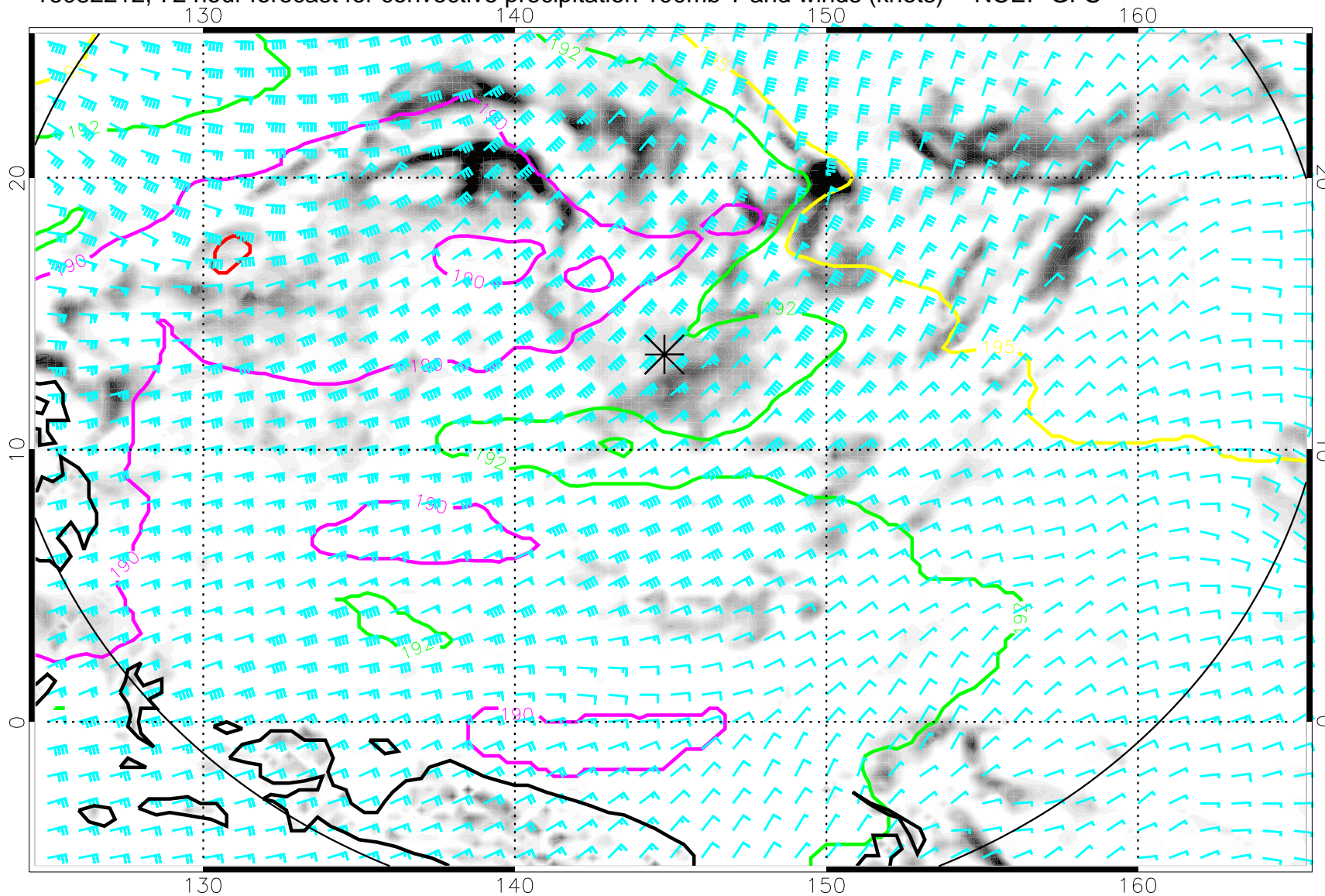
16082212, 72 hour forecast for convective precipitation 100mb T and winds (knots) -- NCEP GFS
