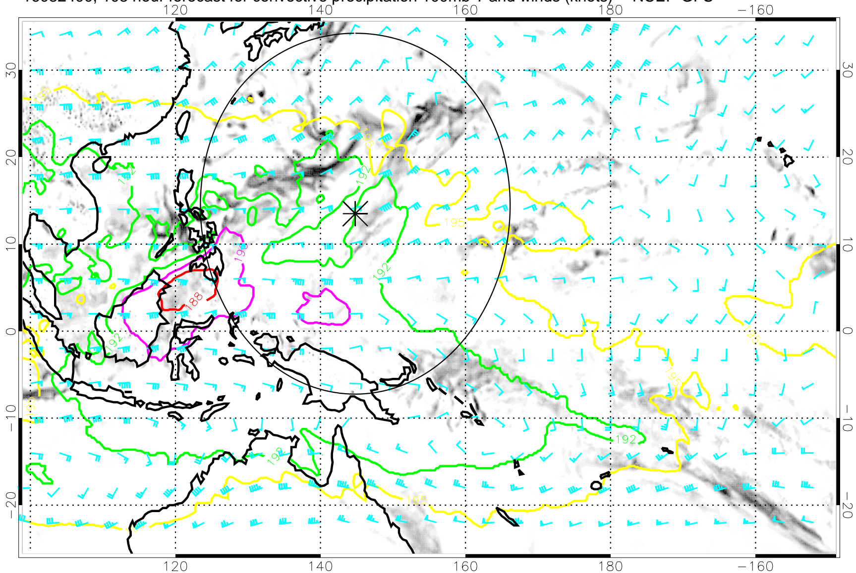
16082400, 108 hour forecast for convective precipitation 100mb T and winds (knots) -- NCEP GFS
