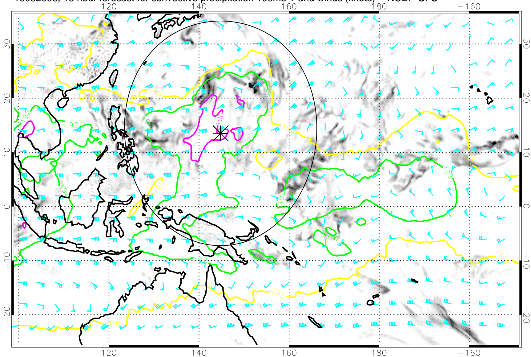
16082006, 18 hour forecast for convective precipitation 100mb T and winds (knots) -- NCEP GFS
