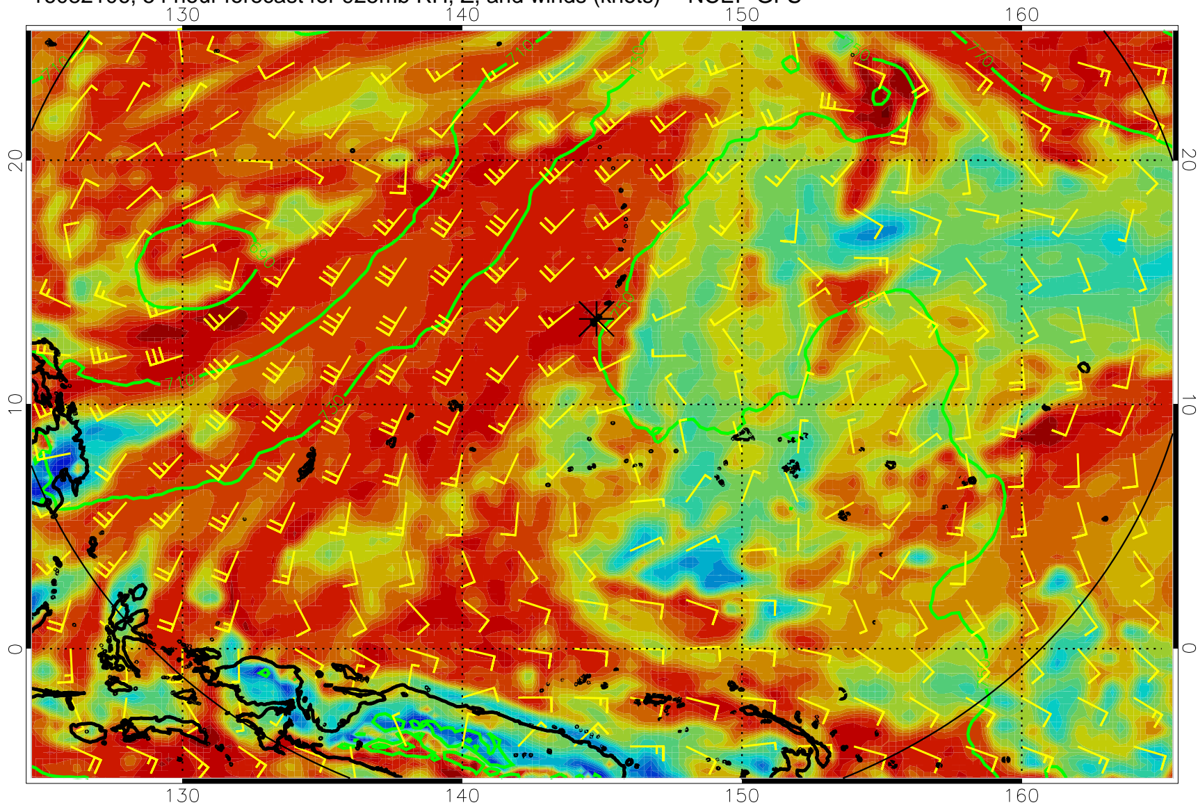
16082106, 54 hour forecast for 925mb RH, Z, and winds (knots) -- NCEP GFS
