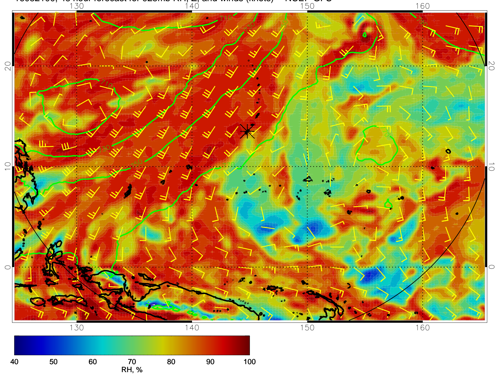
16082100, 48 hour forecast for 925mb RH, Z, and winds (knots) -- NCEP GFS
