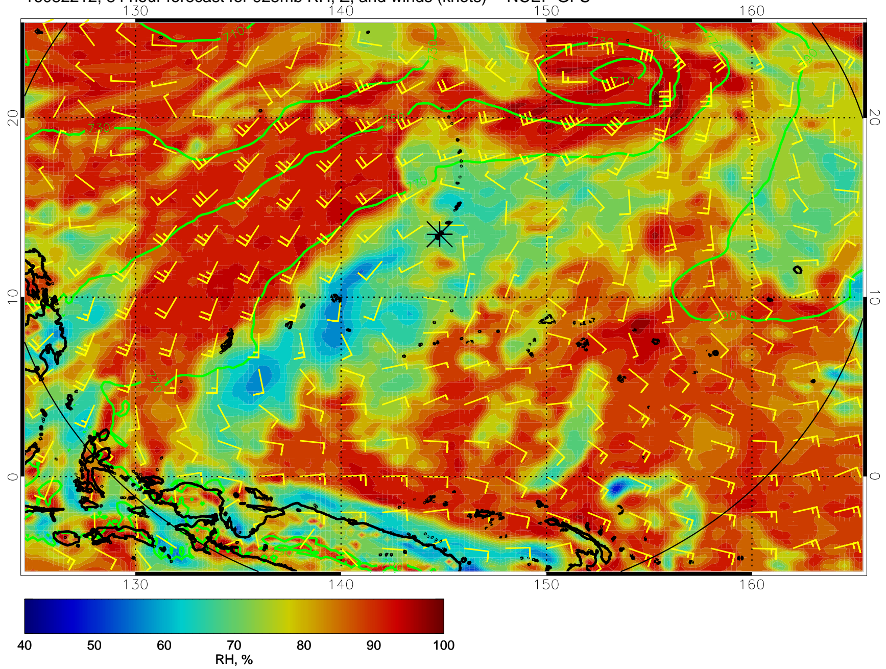
16082212, 84 hour forecast for 925mb RH, Z, and winds (knots) -- NCEP GFS
