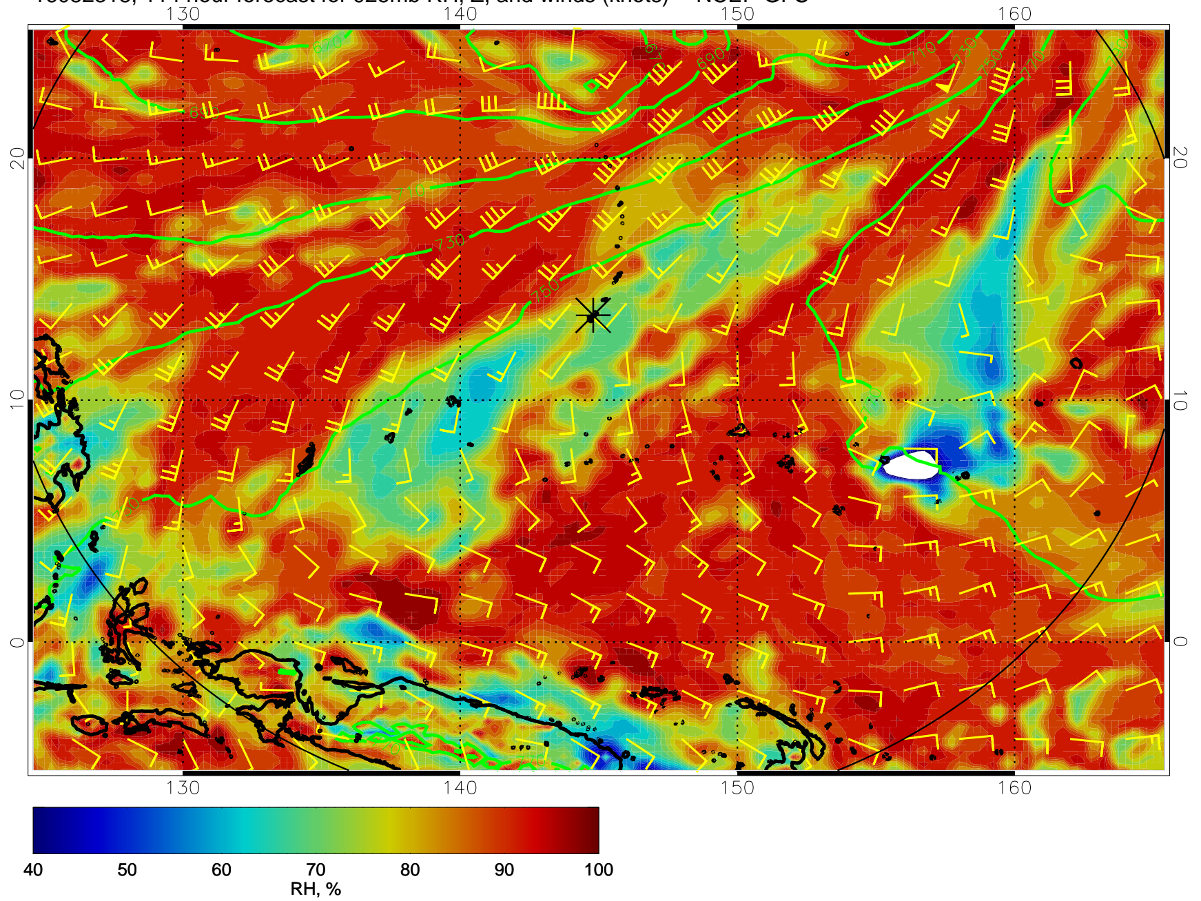
16082318, 114 hour forecast for 925mb RH, Z, and winds (knots) -- NCEP GFS
