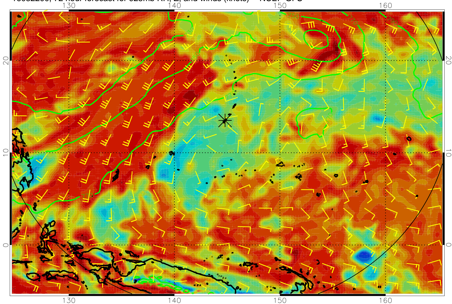
16082200, 72 hour forecast for 925mb RH, Z, and winds (knots) -- NCEP GFS
