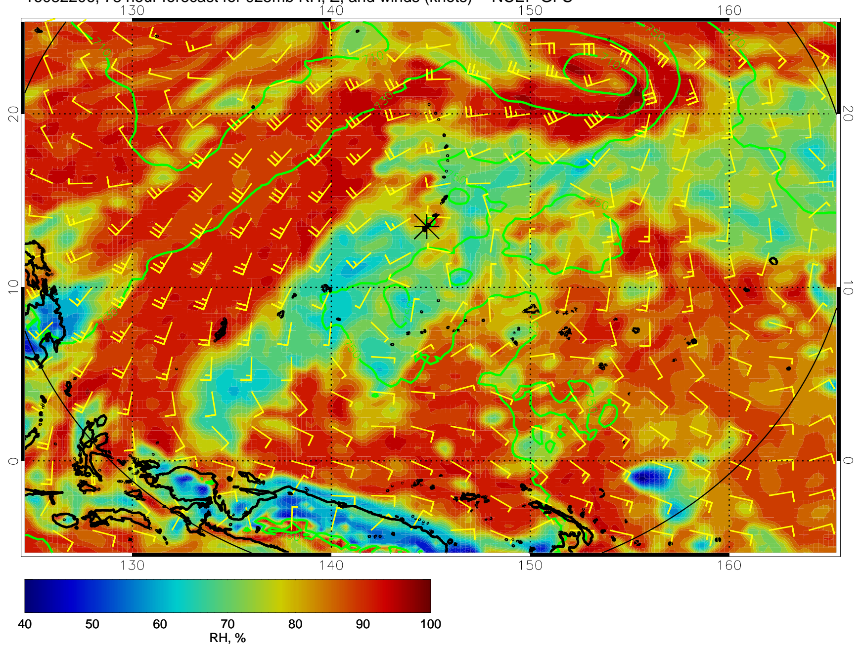
16082206, 78 hour forecast for 925mb RH, Z, and winds (knots) -- NCEP GFS
