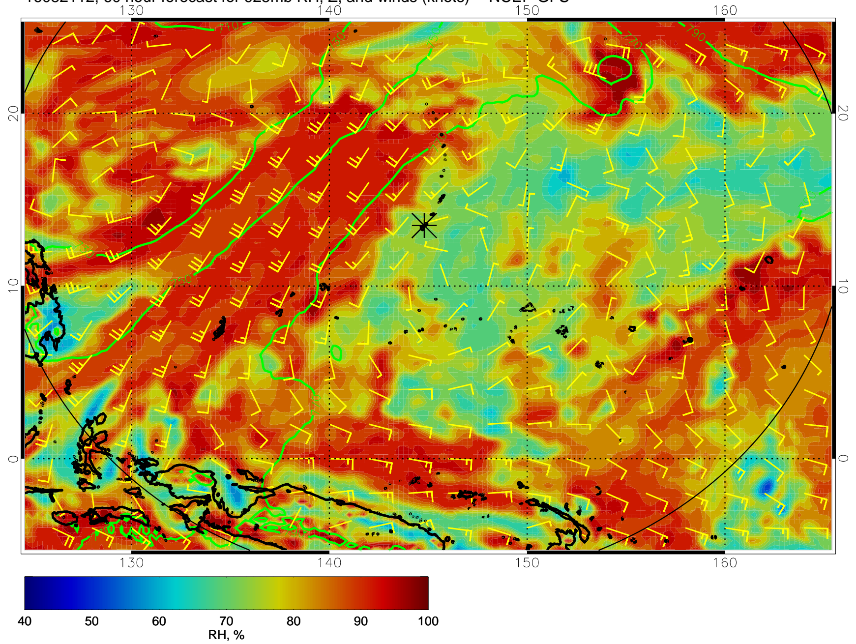
16082112, 60 hour forecast for 925mb RH, Z, and winds (knots) -- NCEP GFS
