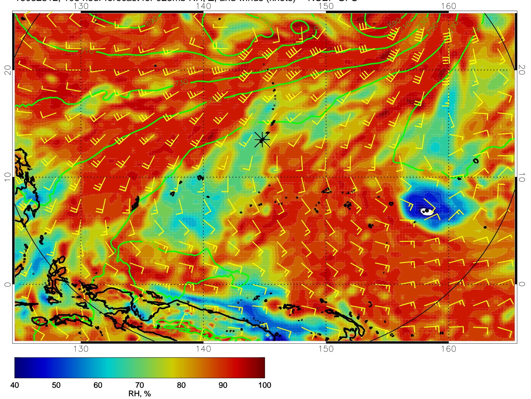
16082312, 108 hour forecast for 925mb RH, Z, and winds (knots) -- NCEP GFS
