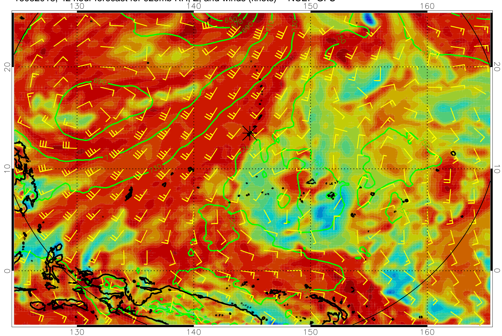
16082018, 42 hour forecast for 925mb RH, Z, and winds (knots) -- NCEP GFS
