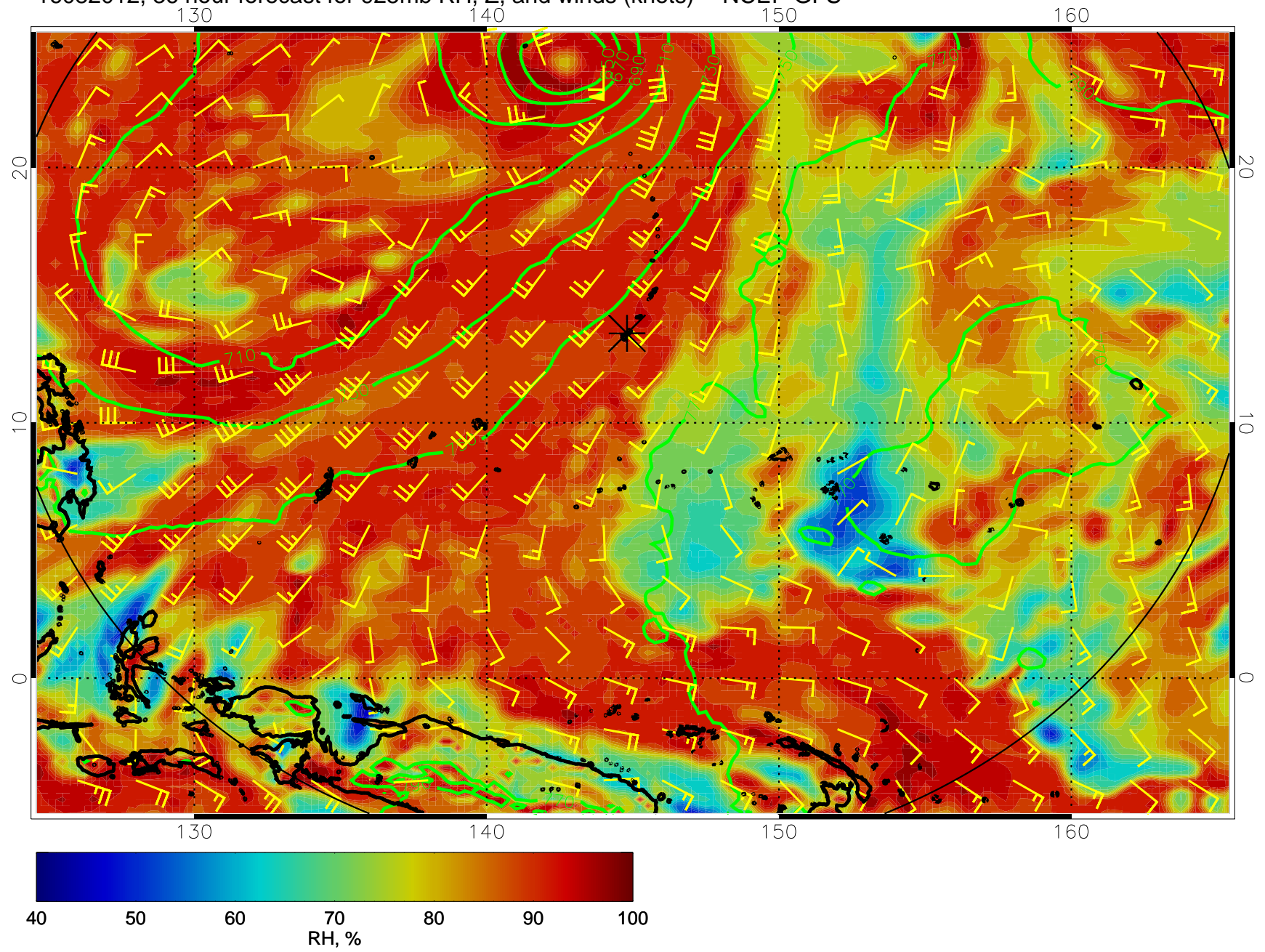
16082012, 36 hour forecast for 925mb RH, Z, and winds (knots) -- NCEP GFS
