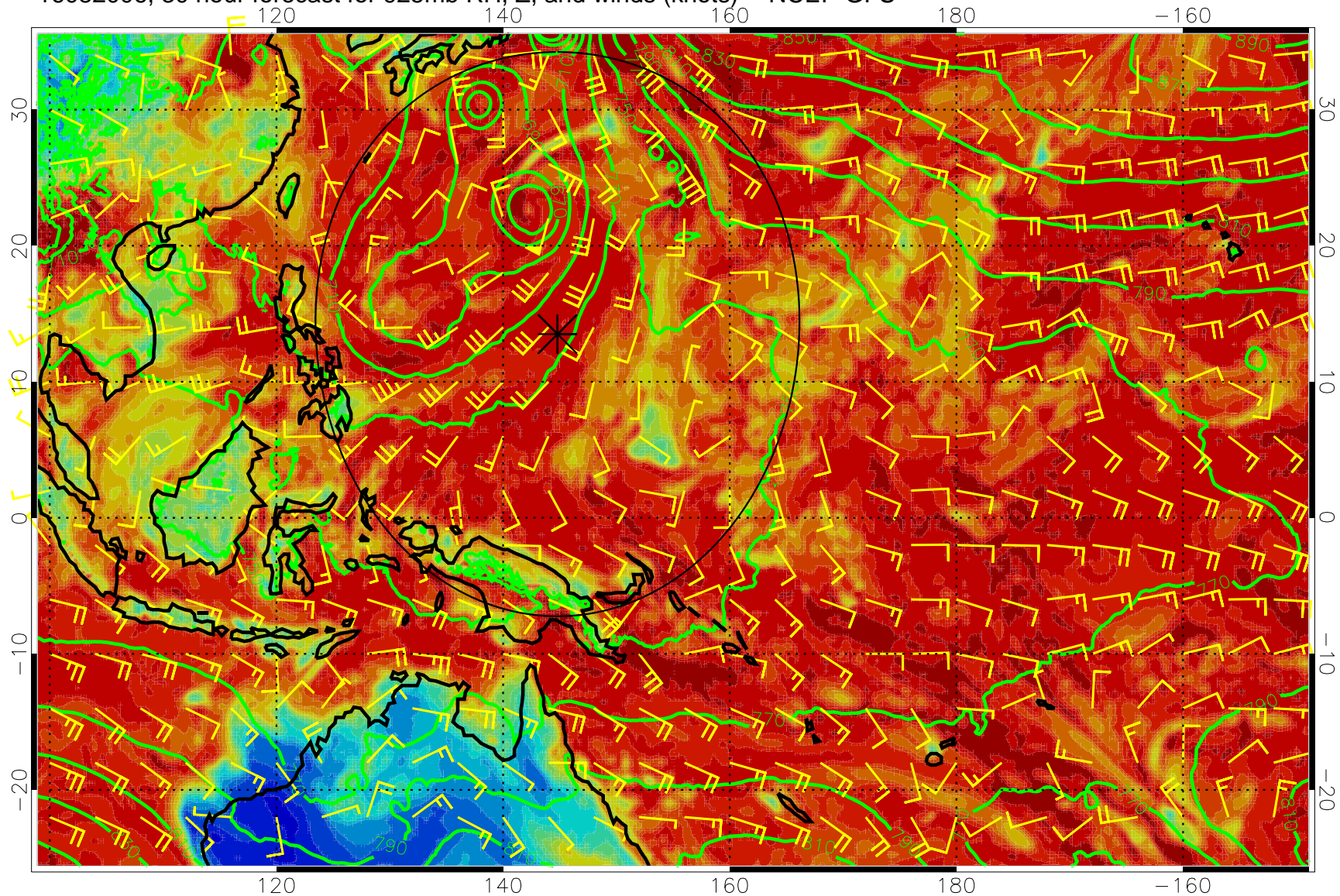
16082006, 30 hour forecast for 925mb RH, Z, and winds (knots) -- NCEP GFS
