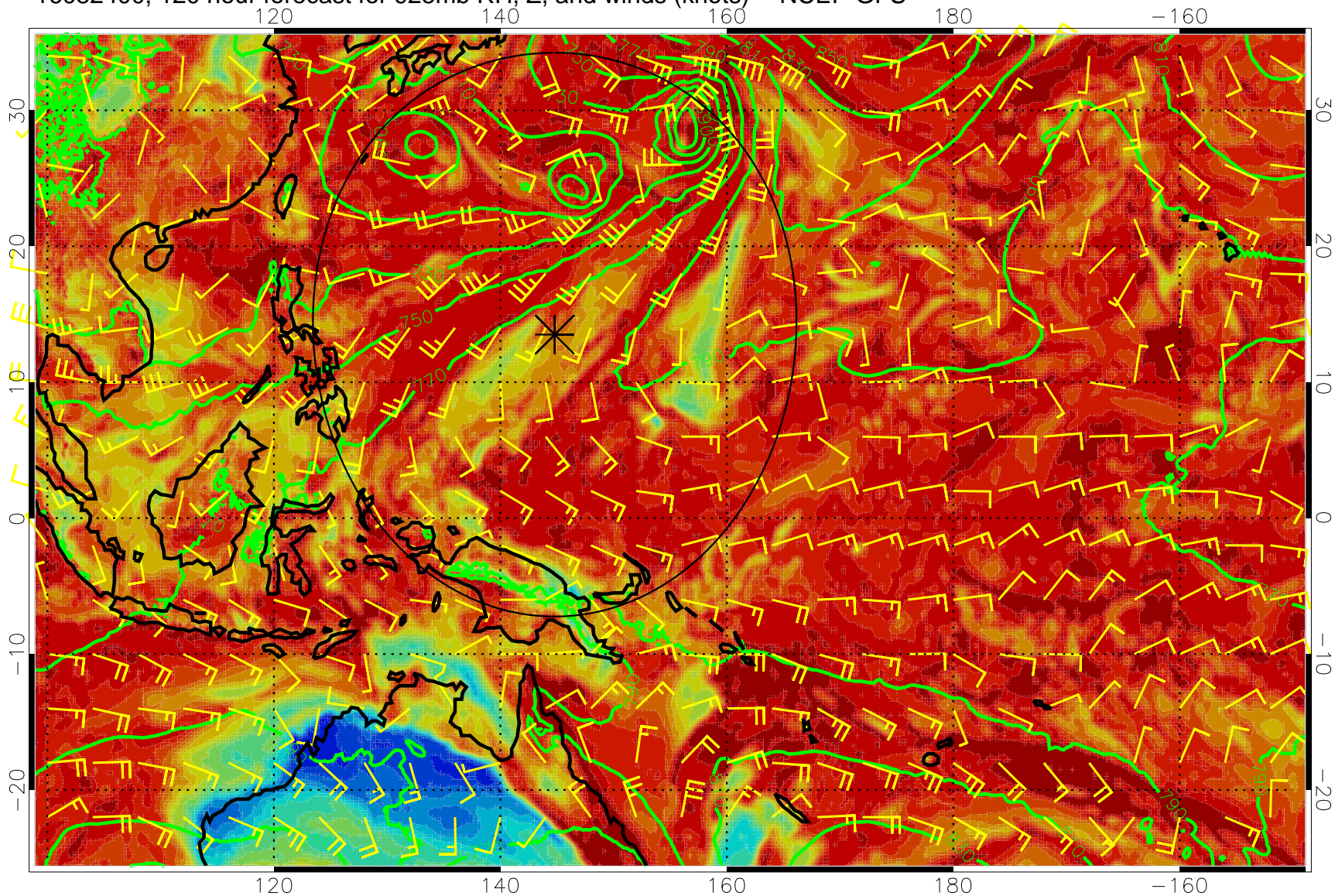
16082400, 120 hour forecast for 925mb RH, Z, and winds (knots) -- NCEP GFS
