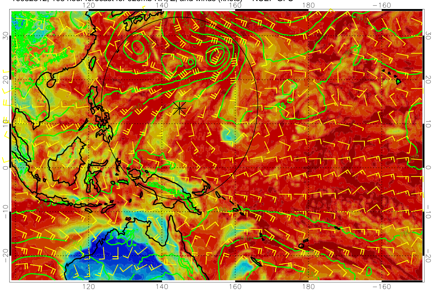
16082312, 108 hour forecast for 925mb RH, Z, and winds (knots) -- NCEP GFS
