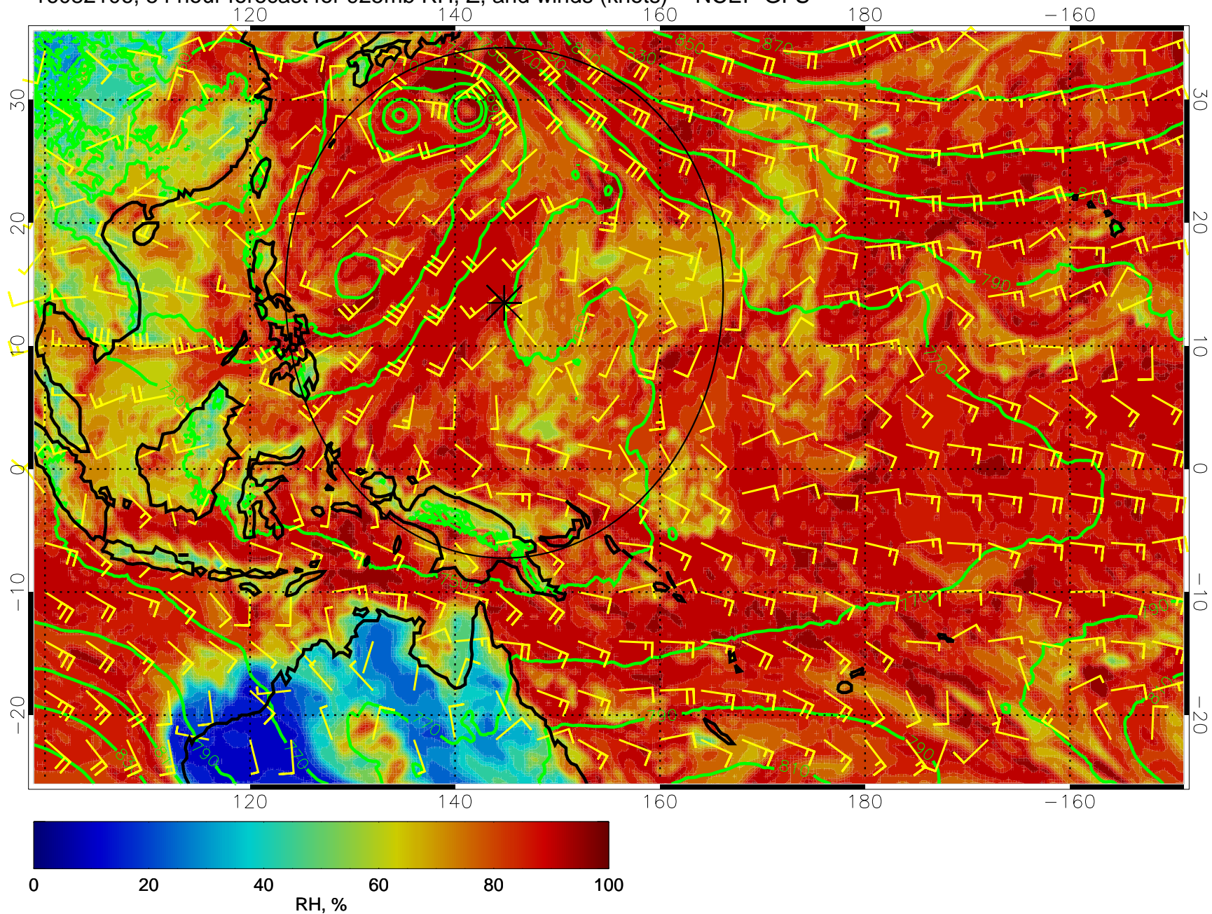
16082106, 54 hour forecast for 925mb RH, Z, and winds (knots) -- NCEP GFS
