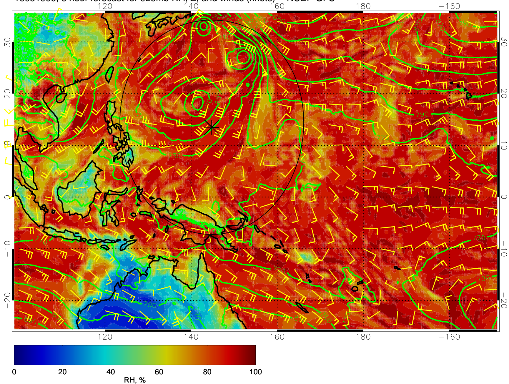
16081906, 6 hour forecast for 925mb RH, Z, and winds (knots) -- NCEP GFS
