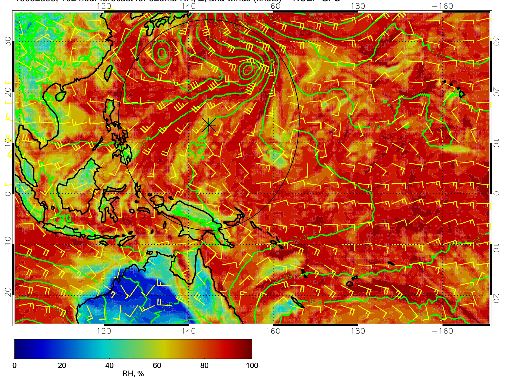
16082306, 102 hour forecast for 925mb RH, Z, and winds (knots) -- NCEP GFS
