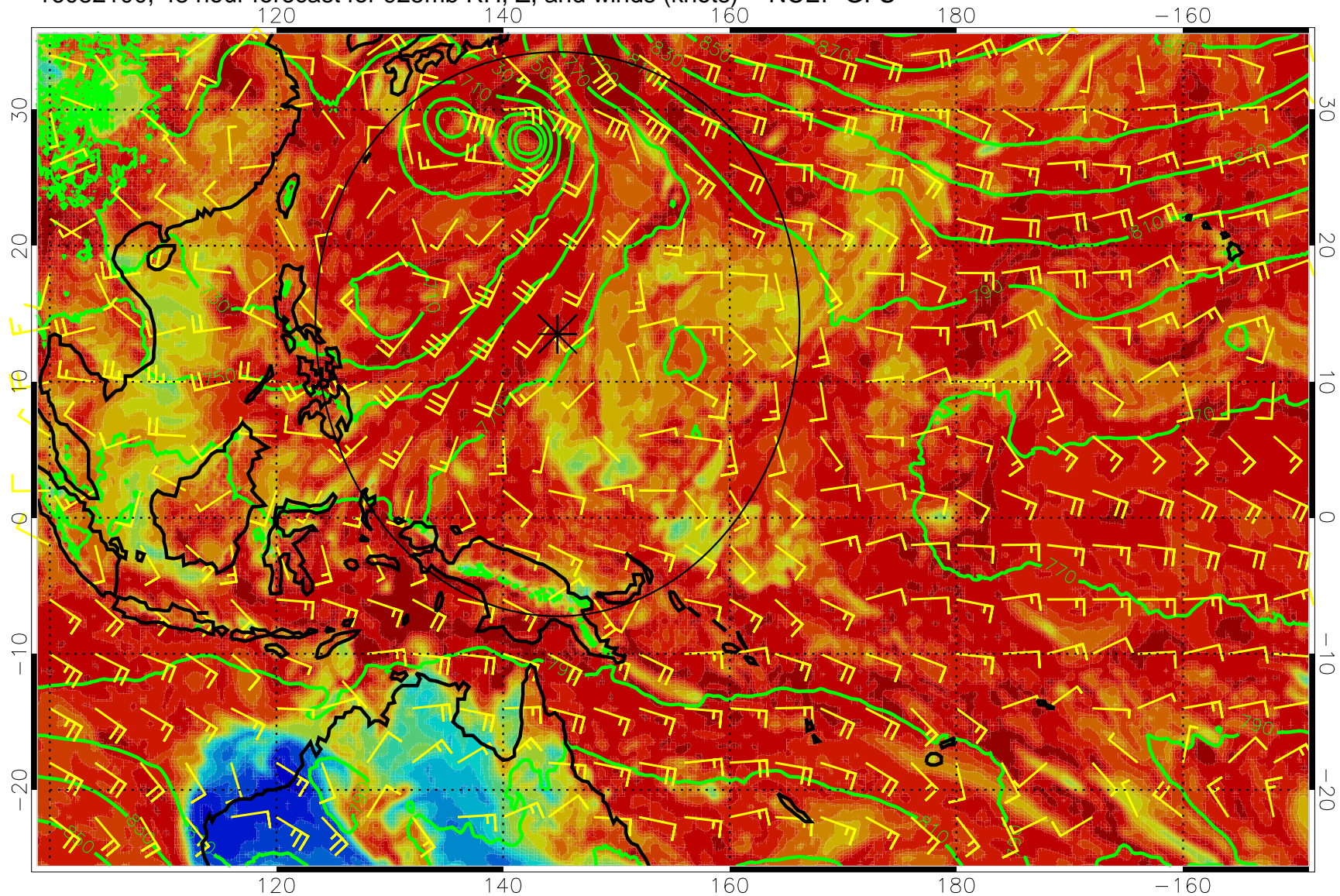
16082100, 48 hour forecast for 925mb RH, Z, and winds (knots) -- NCEP GFS
