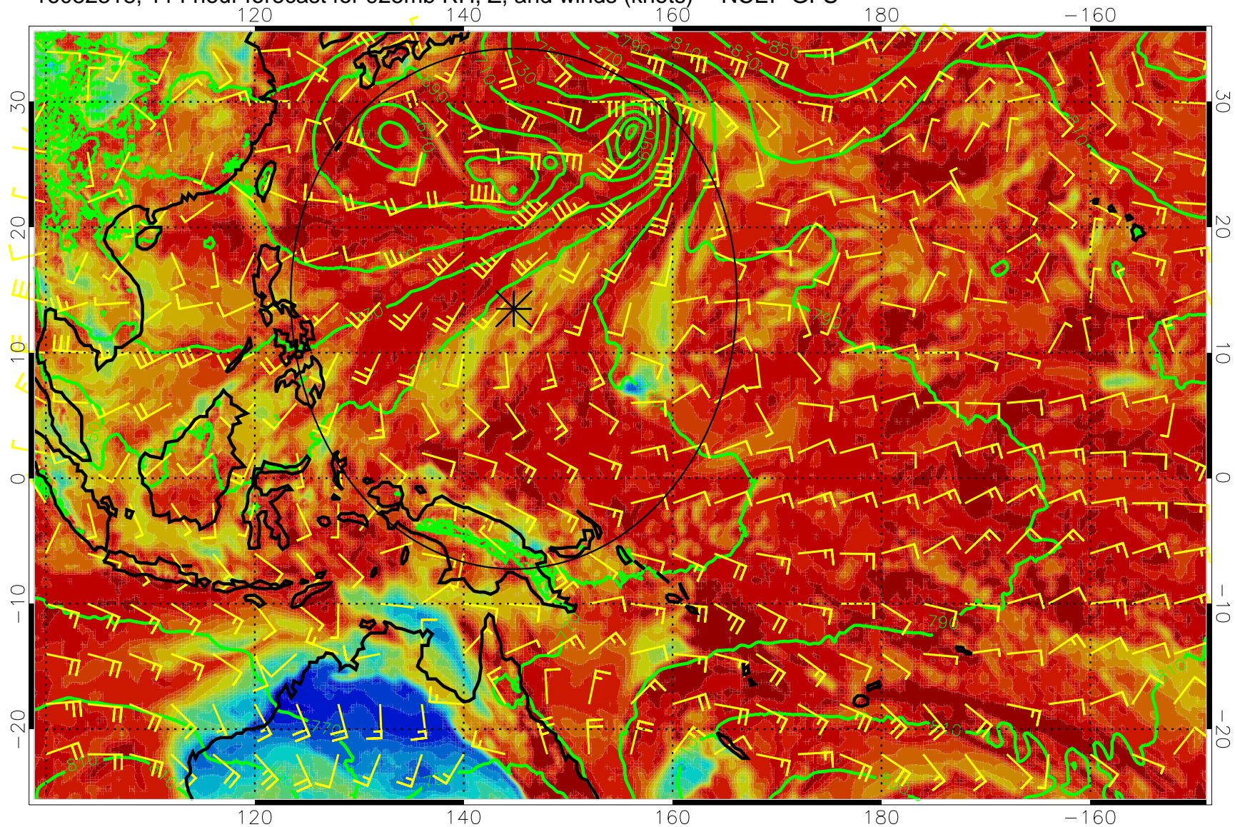
16082318, 114 hour forecast for 925mb RH, Z, and winds (knots) -- NCEP GFS
