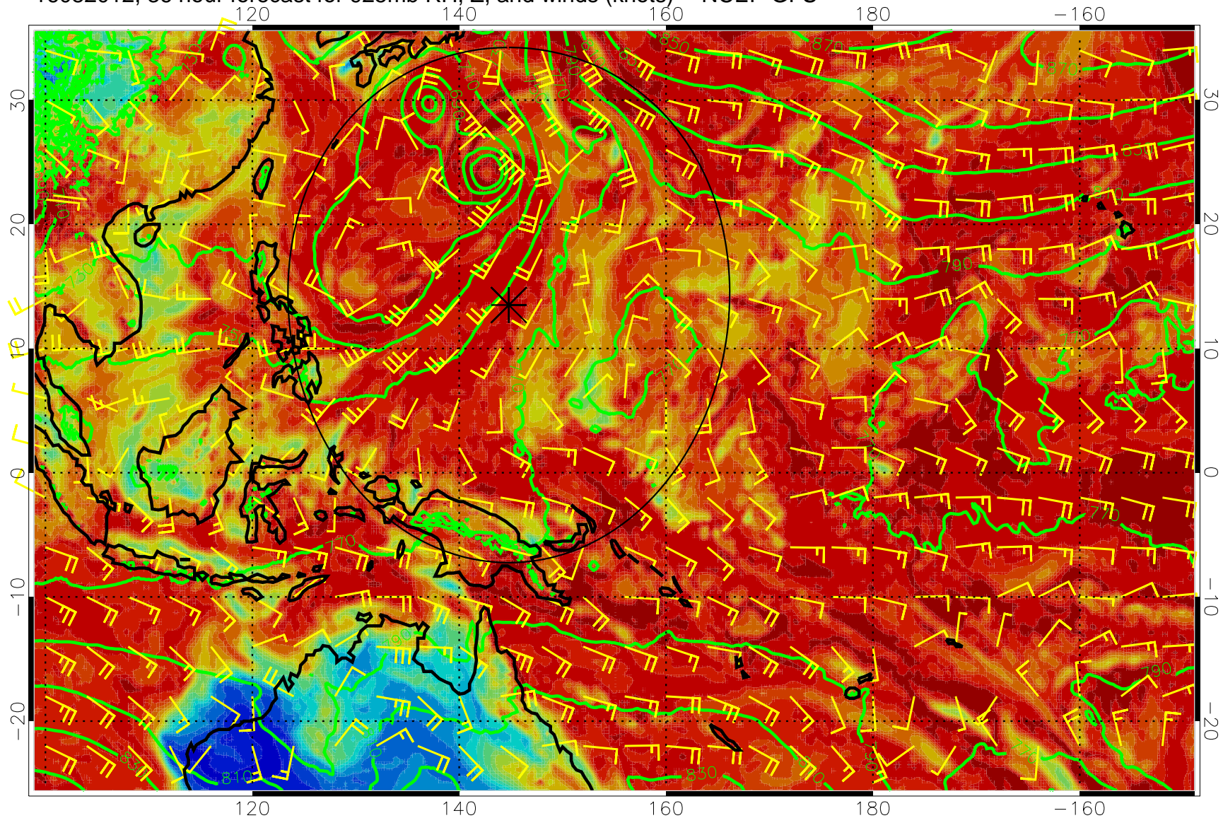
16082012, 36 hour forecast for 925mb RH, Z, and winds (knots) -- NCEP GFS
