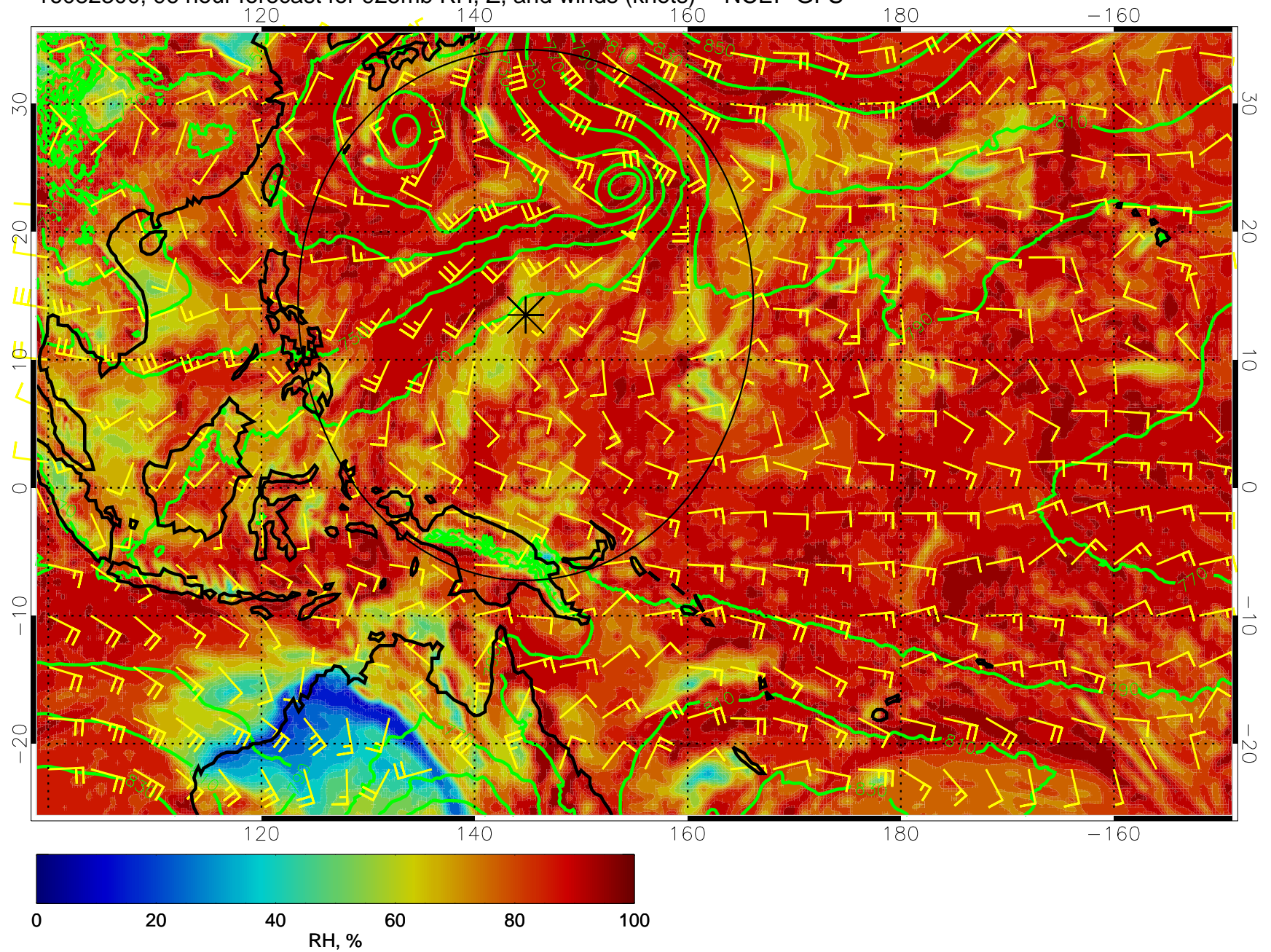
16082300, 96 hour forecast for 925mb RH, Z, and winds (knots) -- NCEP GFS
