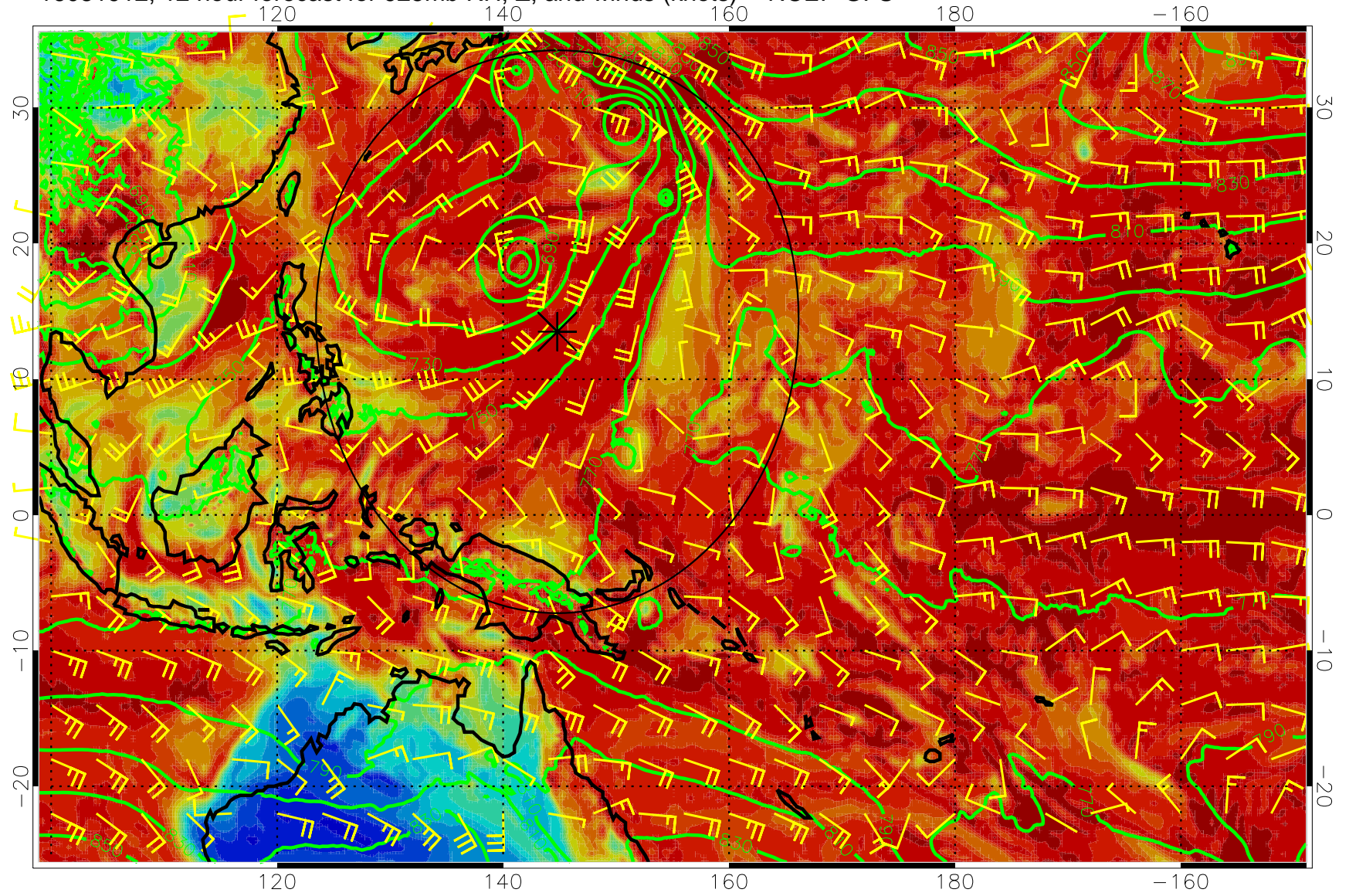
16081912, 12 hour forecast for 925mb RH, Z, and winds (knots) -- NCEP GFS
