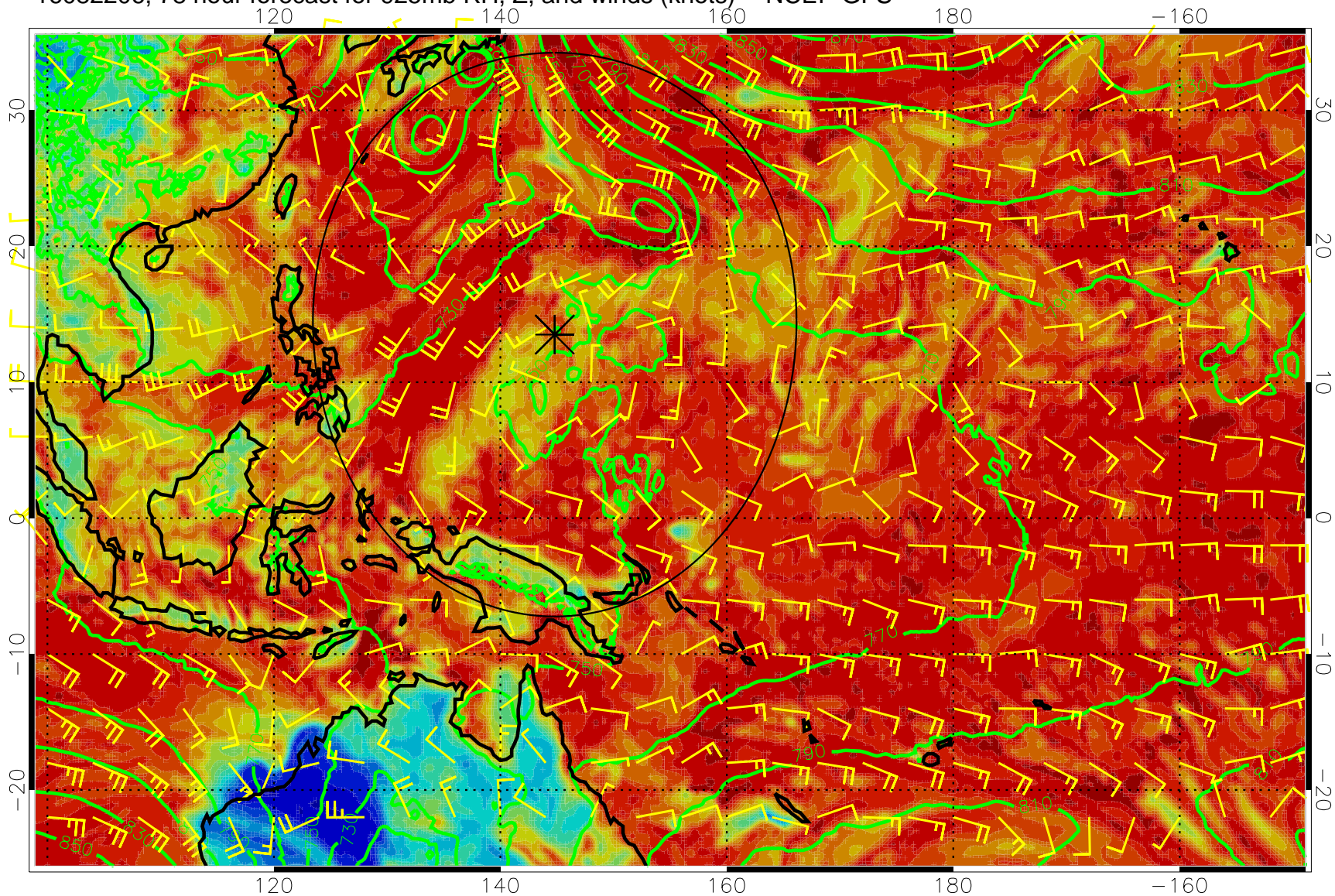
16082206, 78 hour forecast for 925mb RH, Z, and winds (knots) -- NCEP GFS
