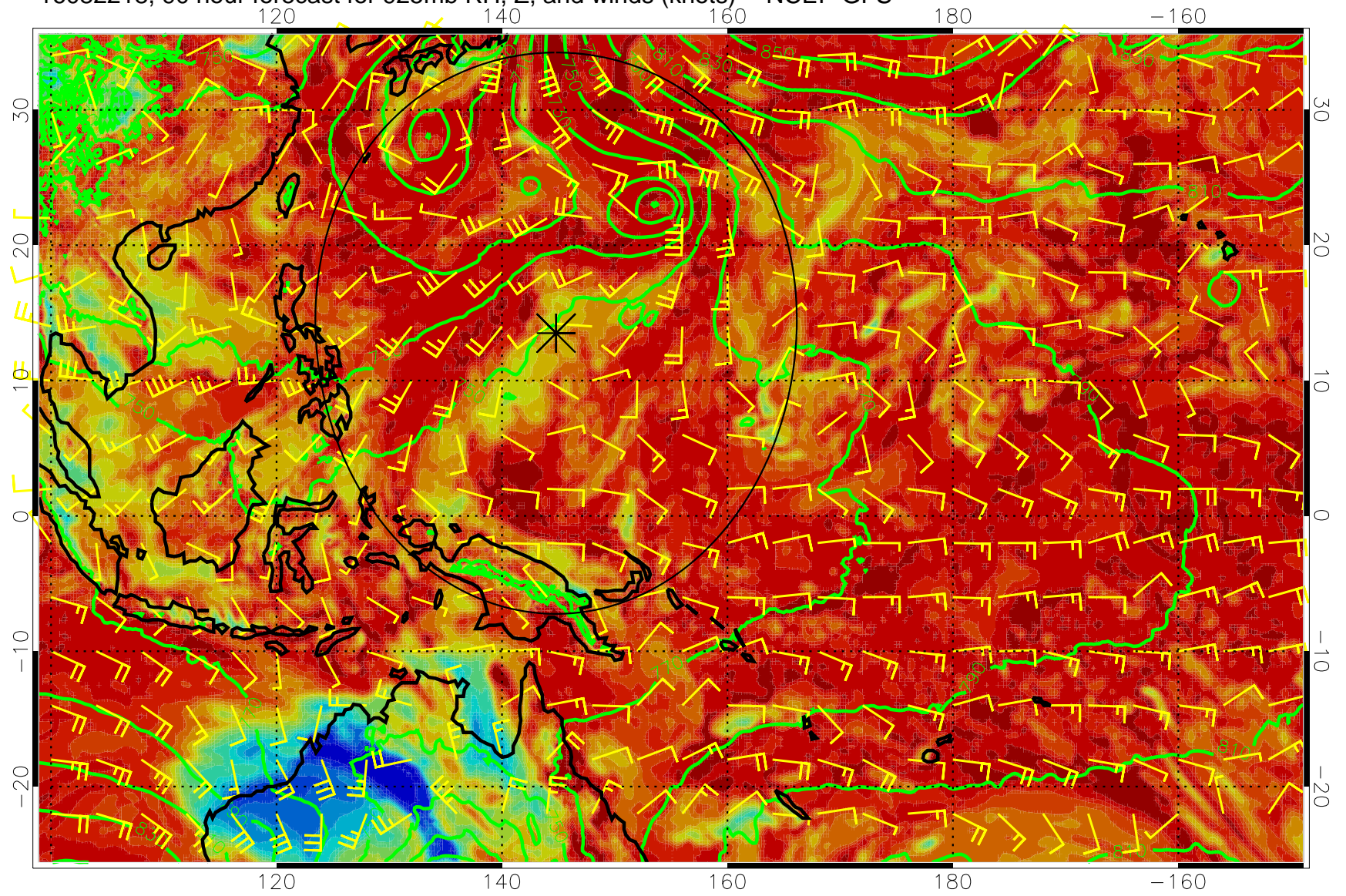
16082218, 90 hour forecast for 925mb RH, Z, and winds (knots) -- NCEP GFS
