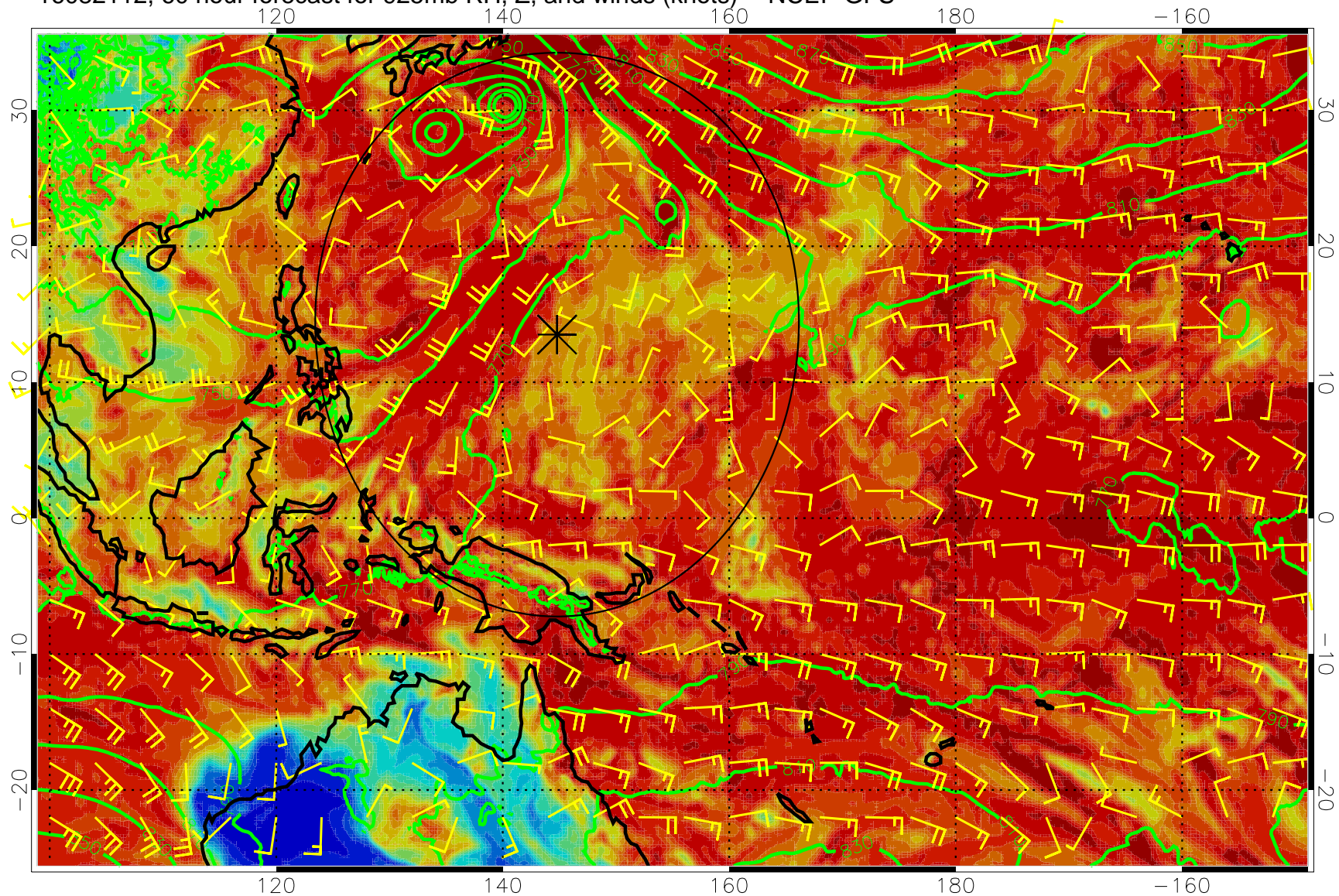
16082112, 60 hour forecast for 925mb RH, Z, and winds (knots) -- NCEP GFS
