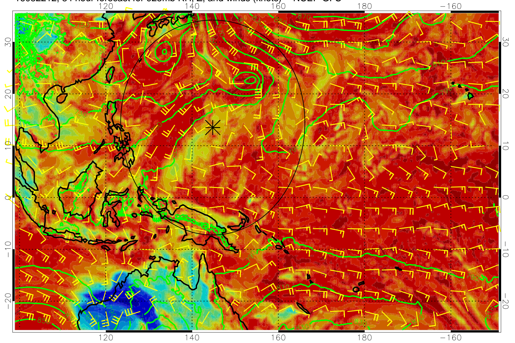
16082212, 84 hour forecast for 925mb RH, Z, and winds (knots) -- NCEP GFS
