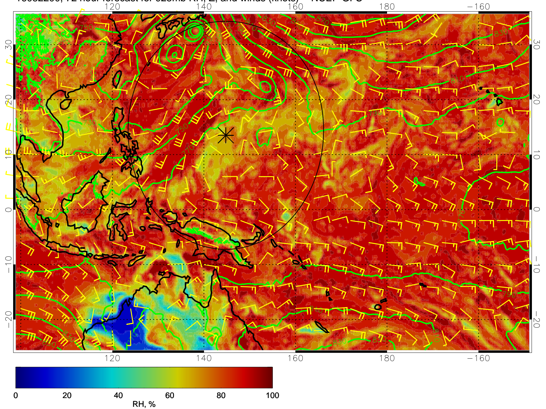
16082200, 72 hour forecast for 925mb RH, Z, and winds (knots) -- NCEP GFS
