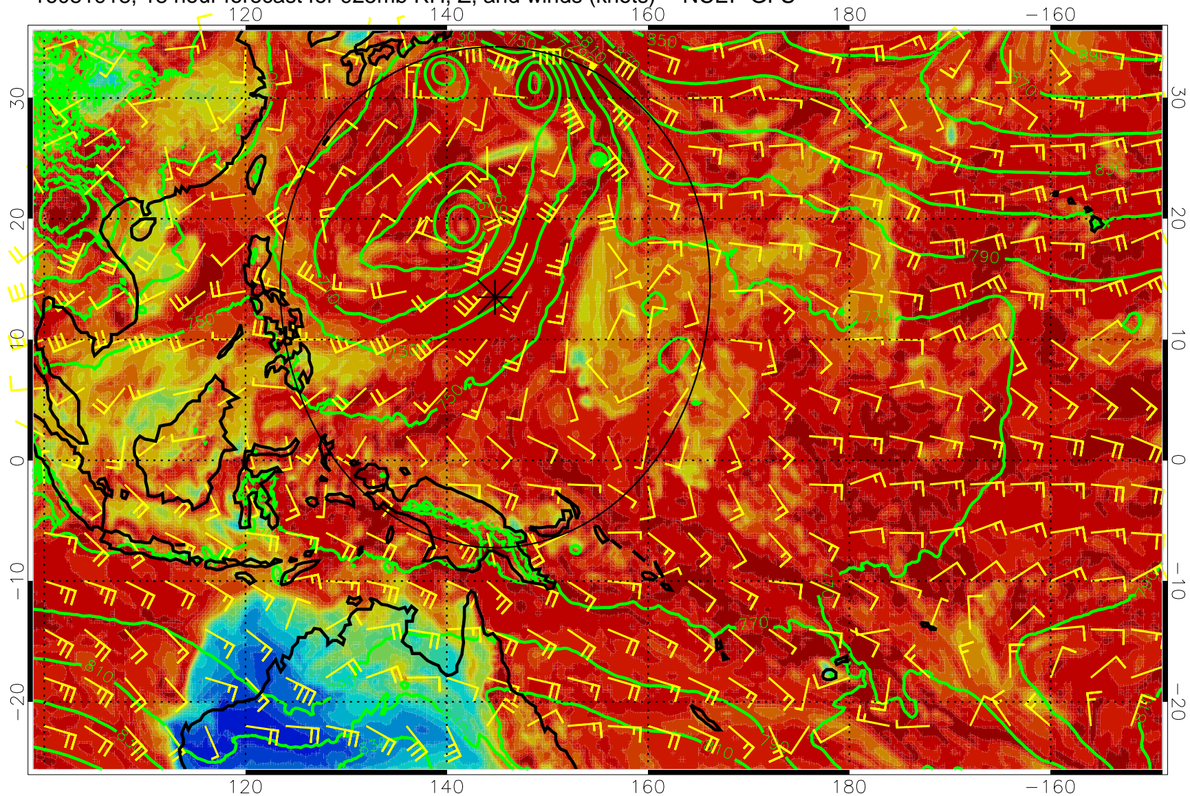
16081918, 18 hour forecast for 925mb RH, Z, and winds (knots) -- NCEP GFS
