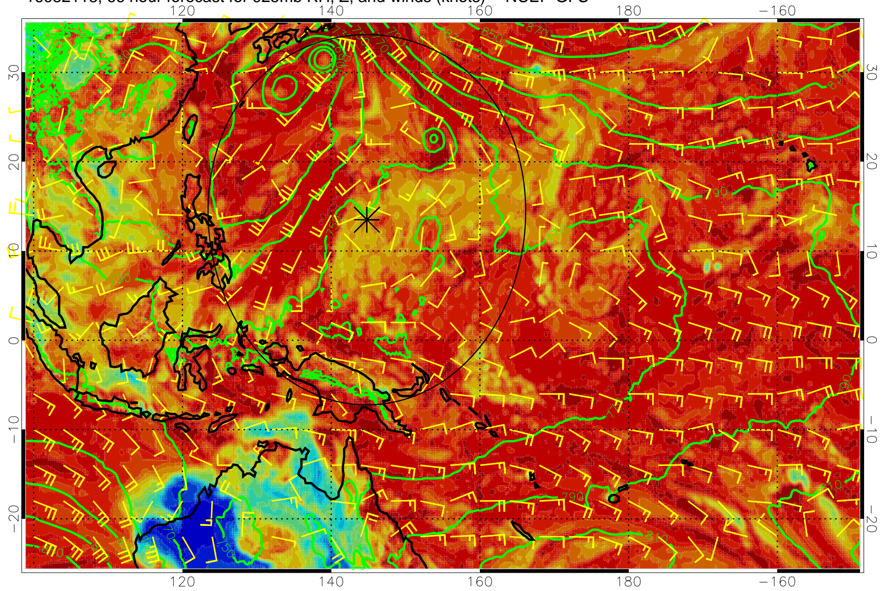
16082118, 66 hour forecast for 925mb RH, Z, and winds (knots) -- NCEP GFS
