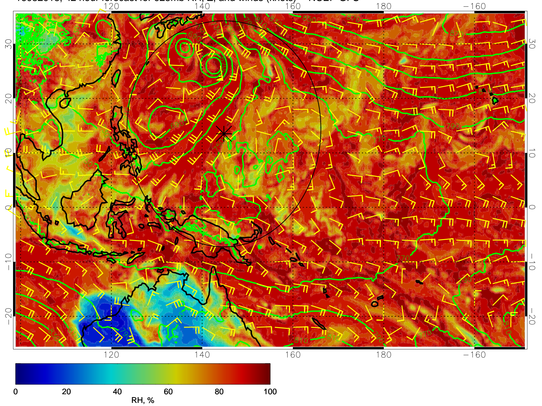
16082018, 42 hour forecast for 925mb RH, Z, and winds (knots) -- NCEP GFS
