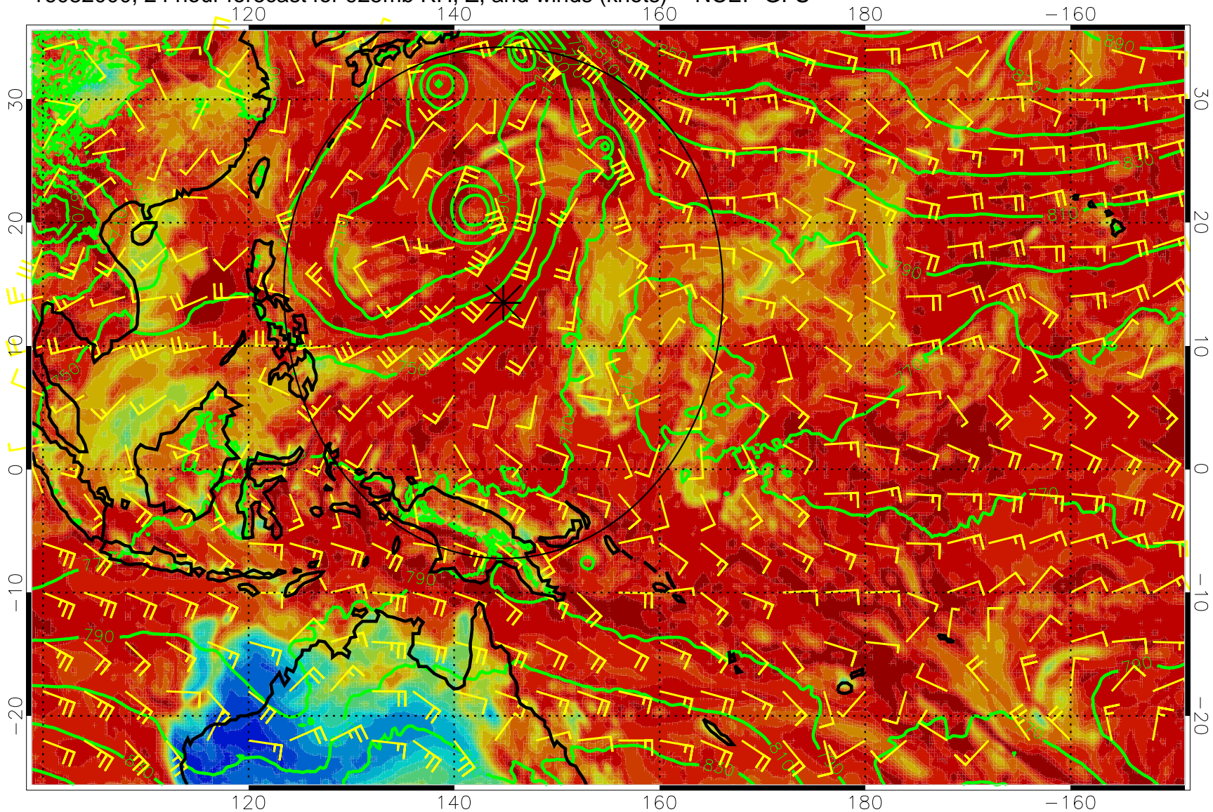
16082000, 24 hour forecast for 925mb RH, Z, and winds (knots) -- NCEP GFS
