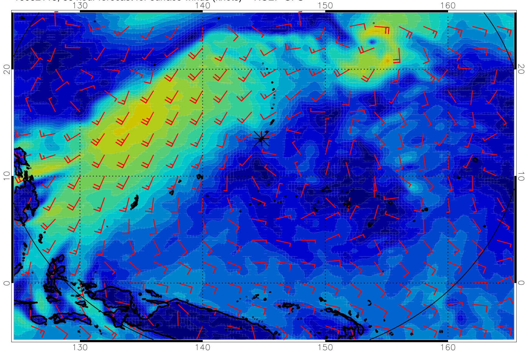
16082118, 66 hour forecast for surface winds (knots) -- NCEP GFS
