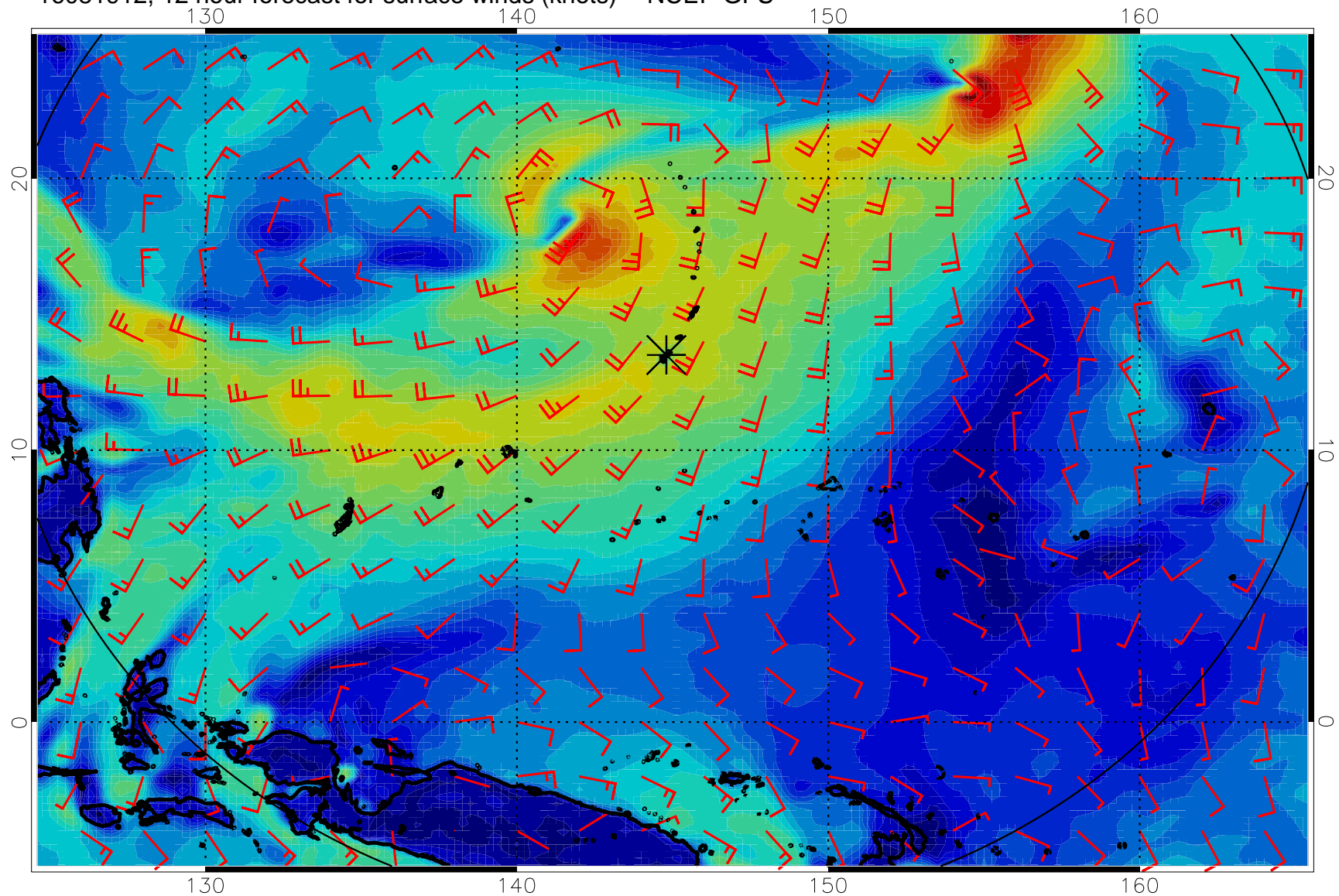
16081912, 12 hour forecast for surface winds (knots) -- NCEP GFS
