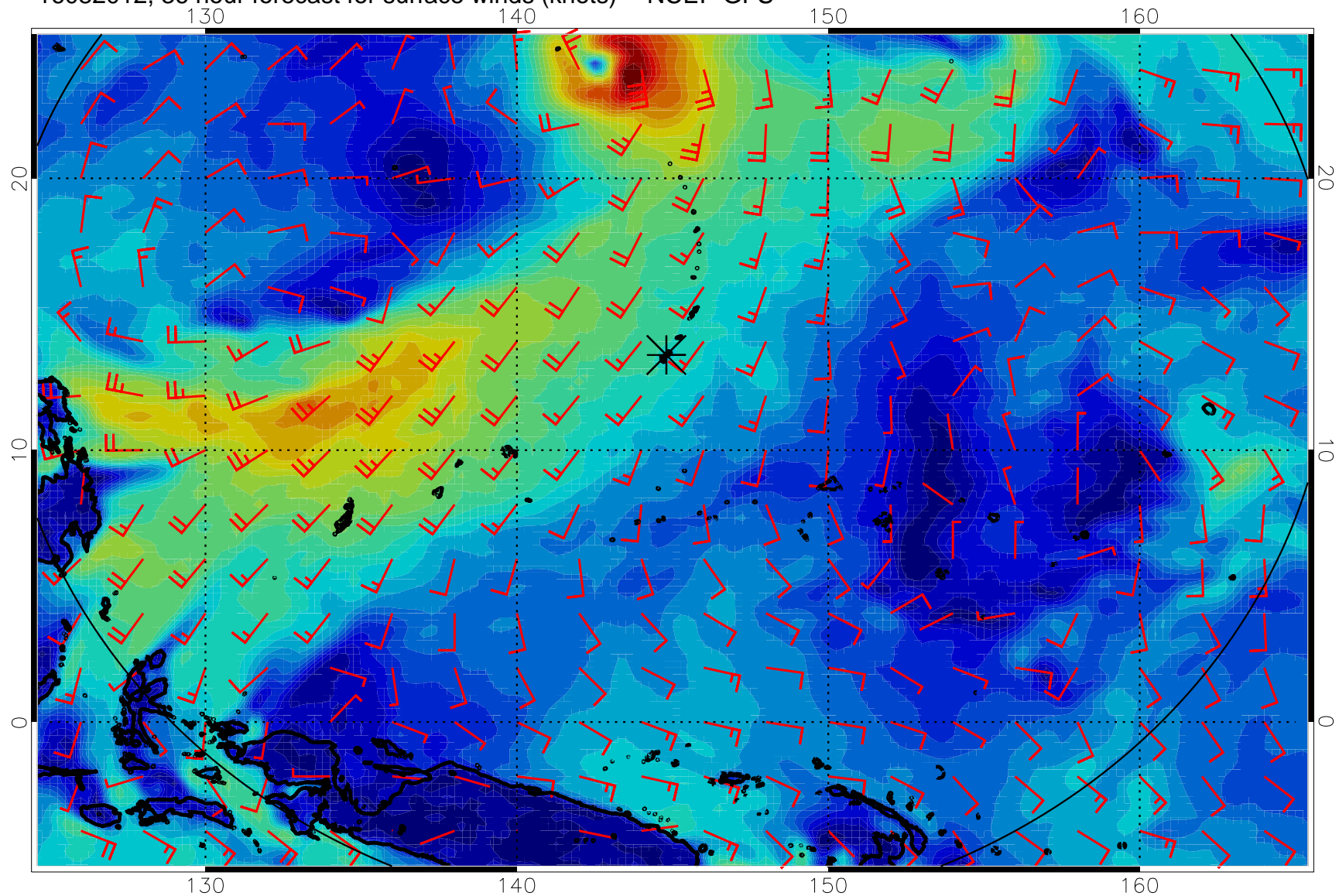
16082012, 36 hour forecast for surface winds (knots) -- NCEP GFS
