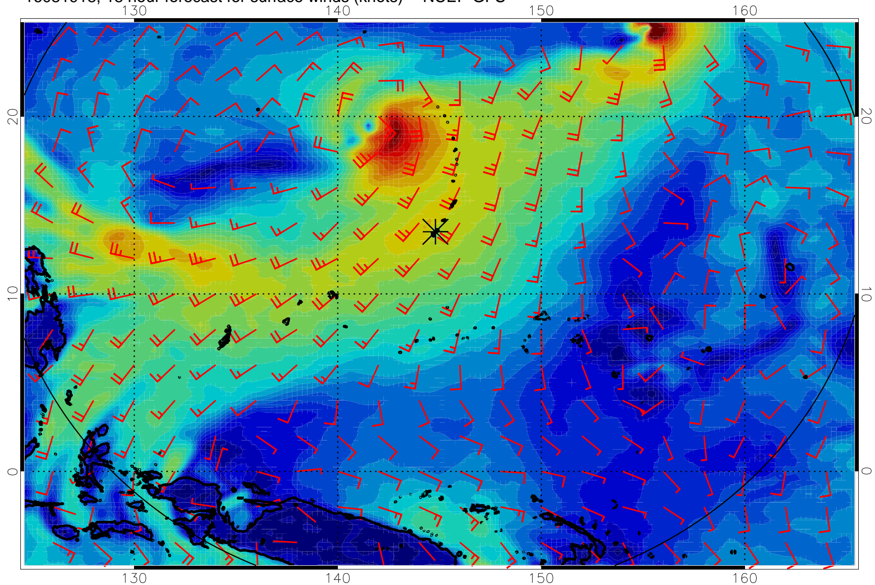
16081918, 18 hour forecast for surface winds (knots) -- NCEP GFS
