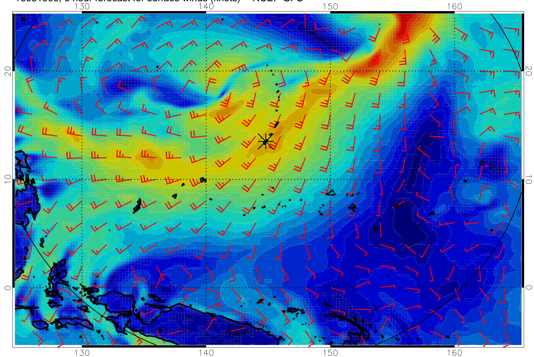
16081906, 6 hour forecast for surface winds (knots) -- NCEP GFS
