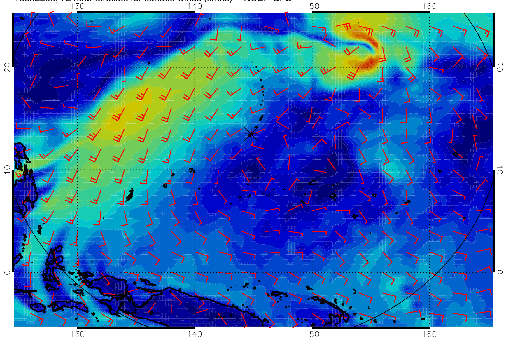
16082200, 72 hour forecast for surface winds (knots) -- NCEP GFS
