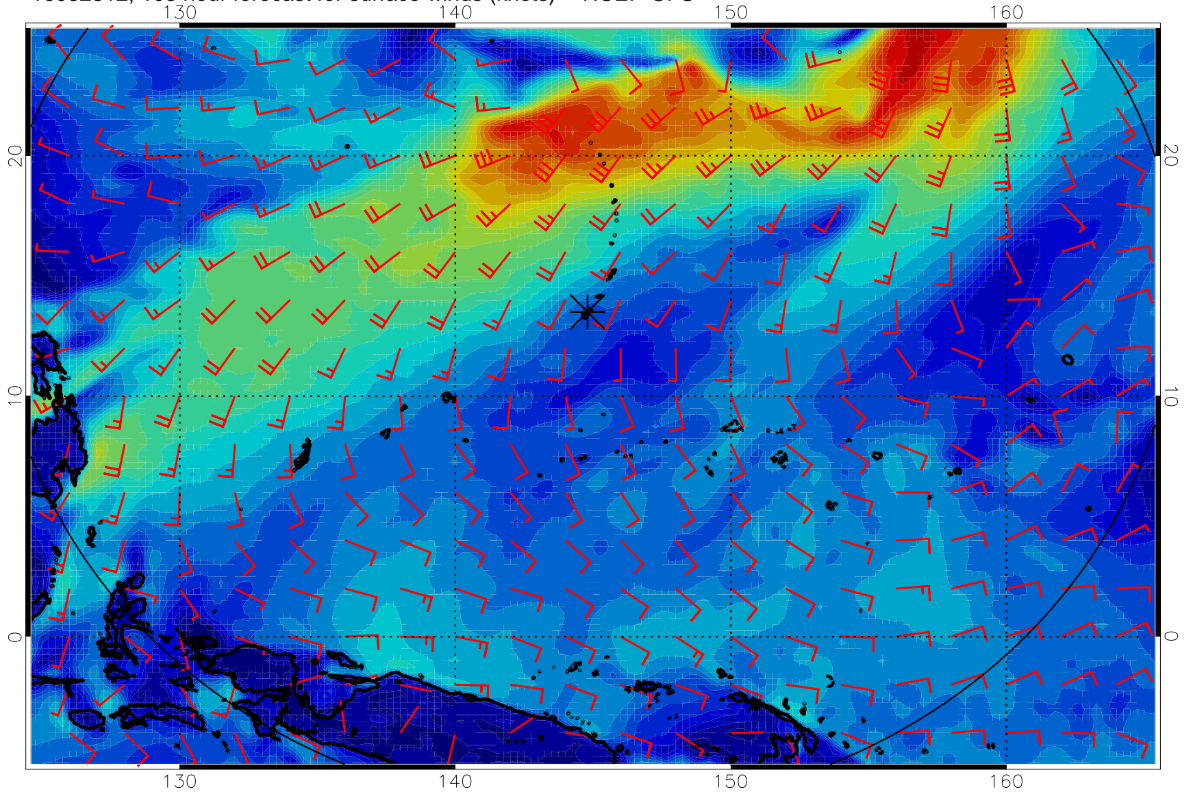
16082312, 108 hour forecast for surface winds (knots) -- NCEP GFS
