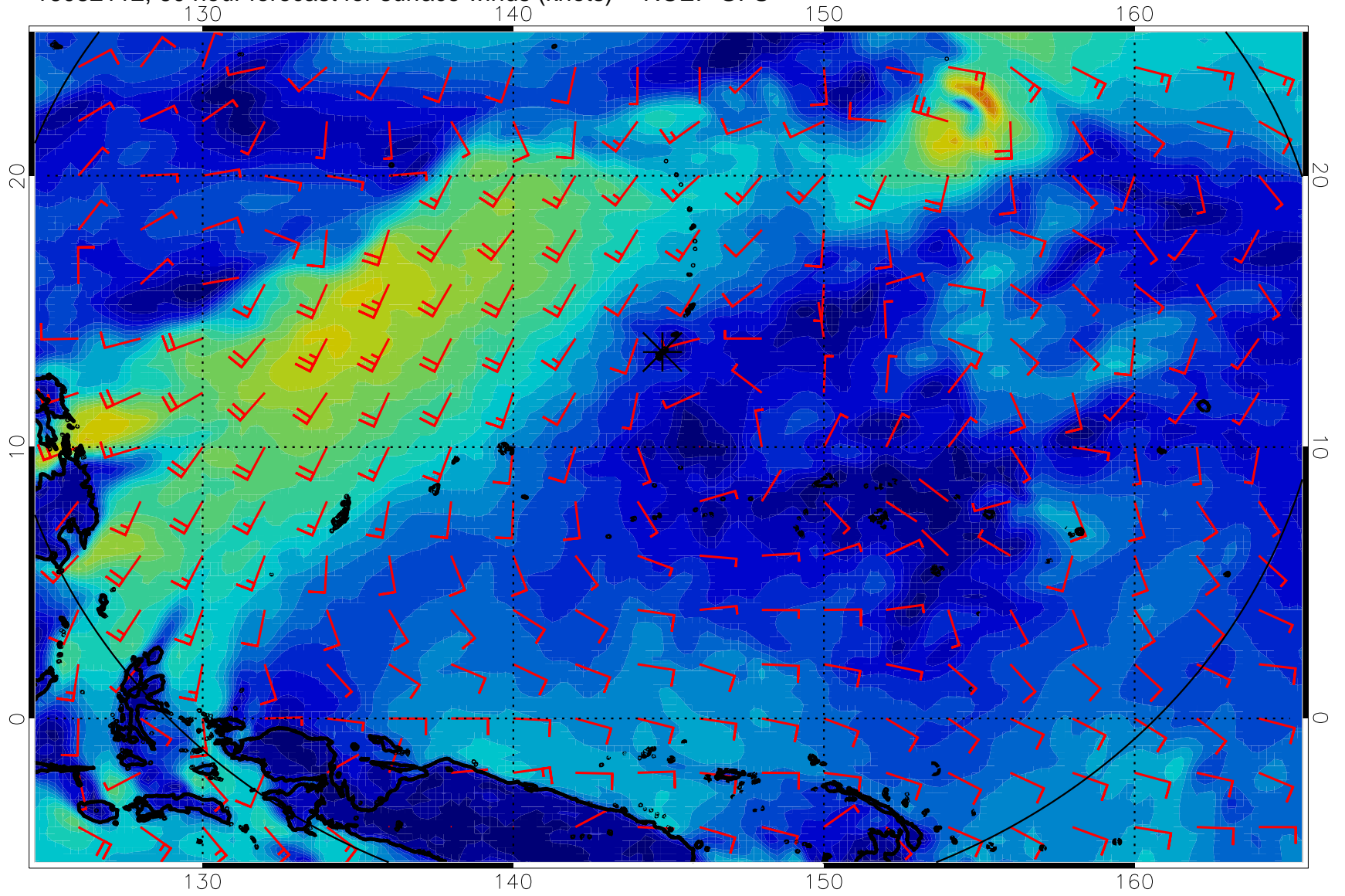
16082112, 60 hour forecast for surface winds (knots) -- NCEP GFS
