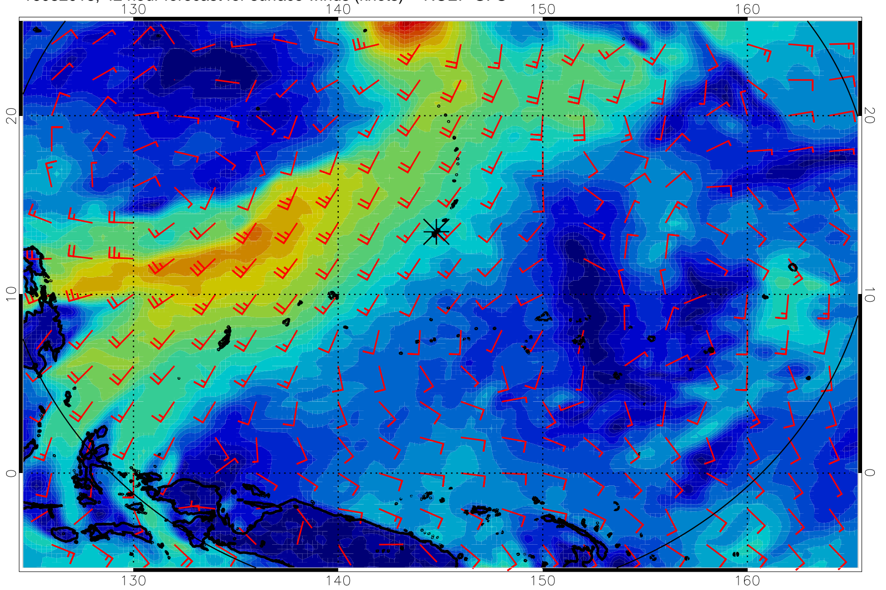
16082018, 42 hour forecast for surface winds (knots) -- NCEP GFS
