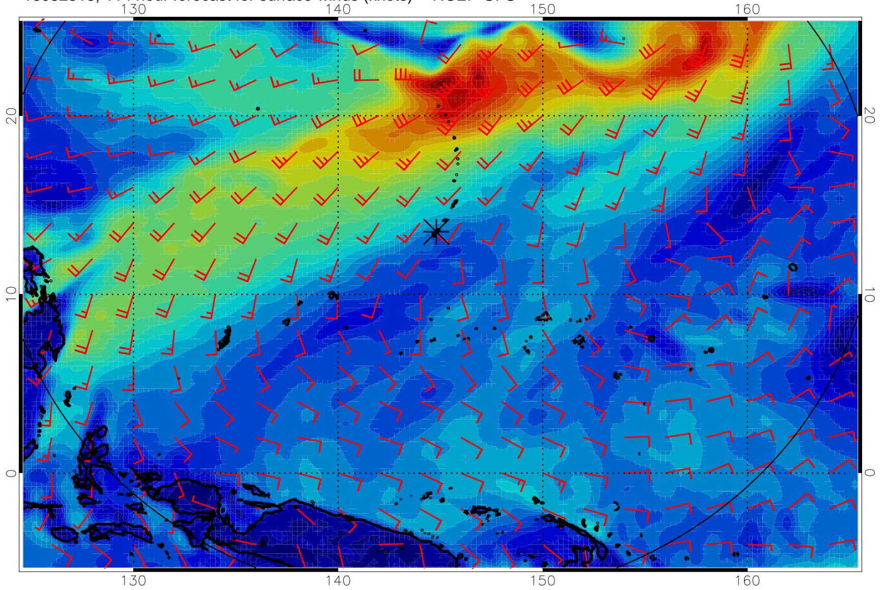
16082318, 114 hour forecast for surface winds (knots) -- NCEP GFS
