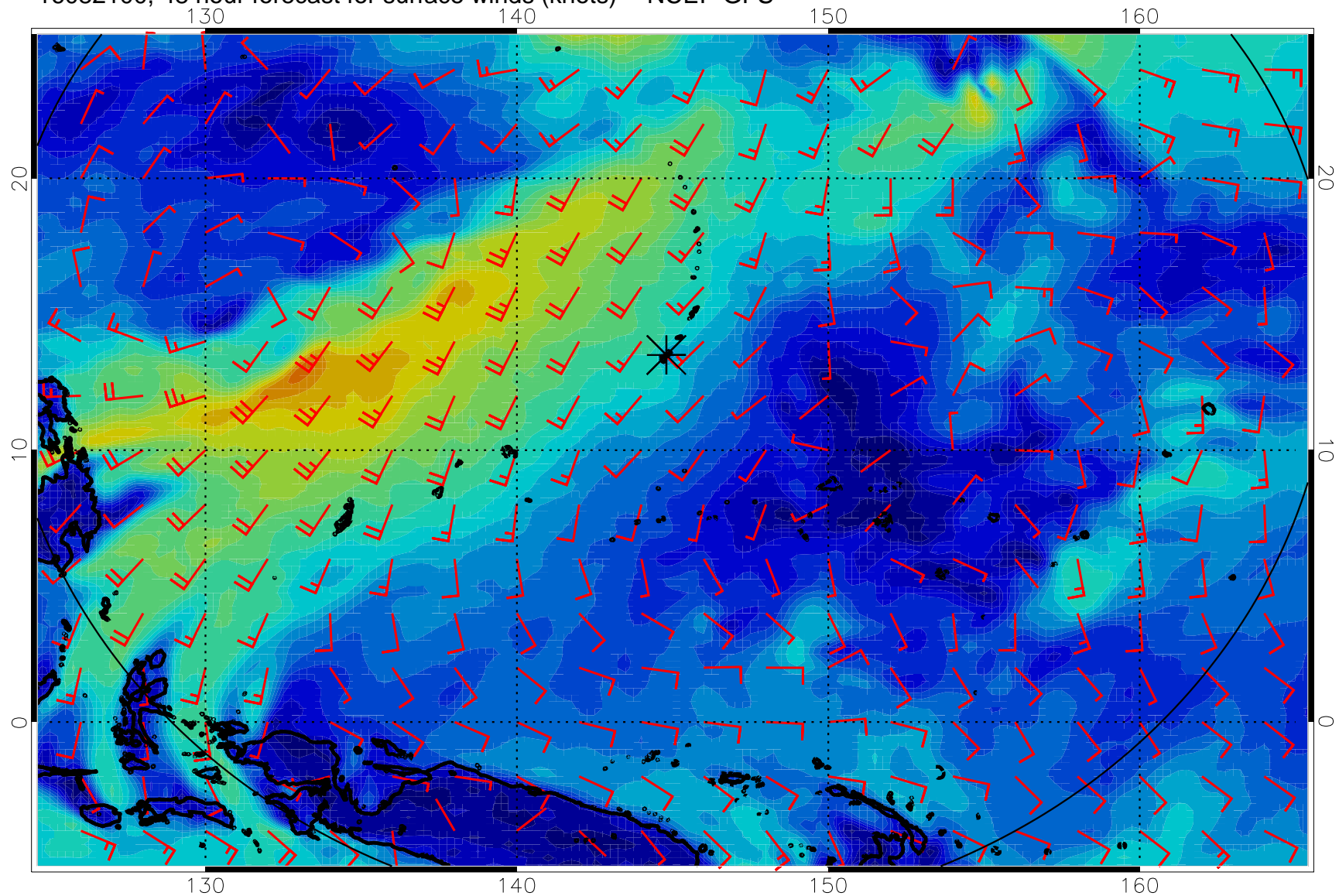
16082100, 48 hour forecast for surface winds (knots) -- NCEP GFS
