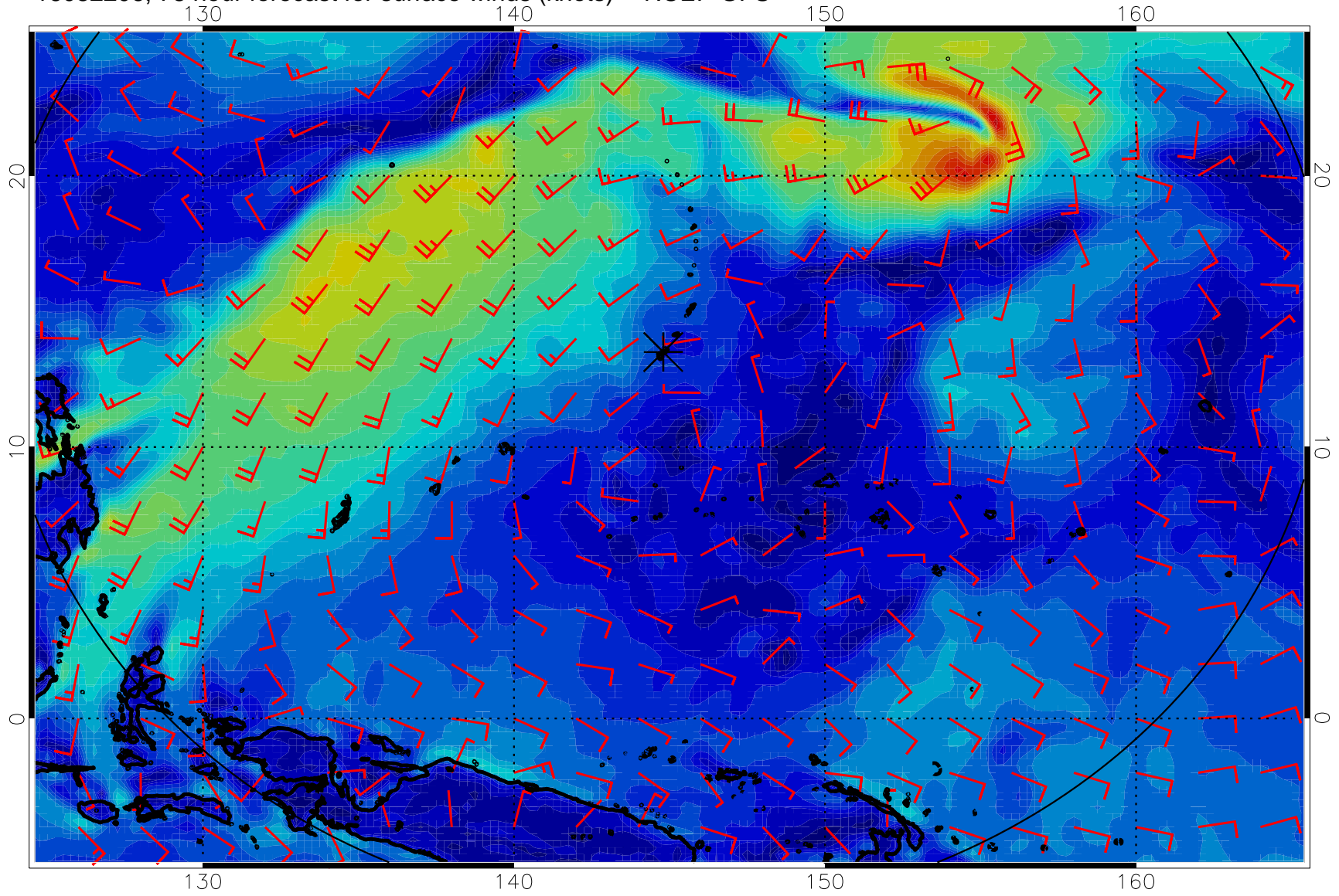
16082206, 78 hour forecast for surface winds (knots) -- NCEP GFS
