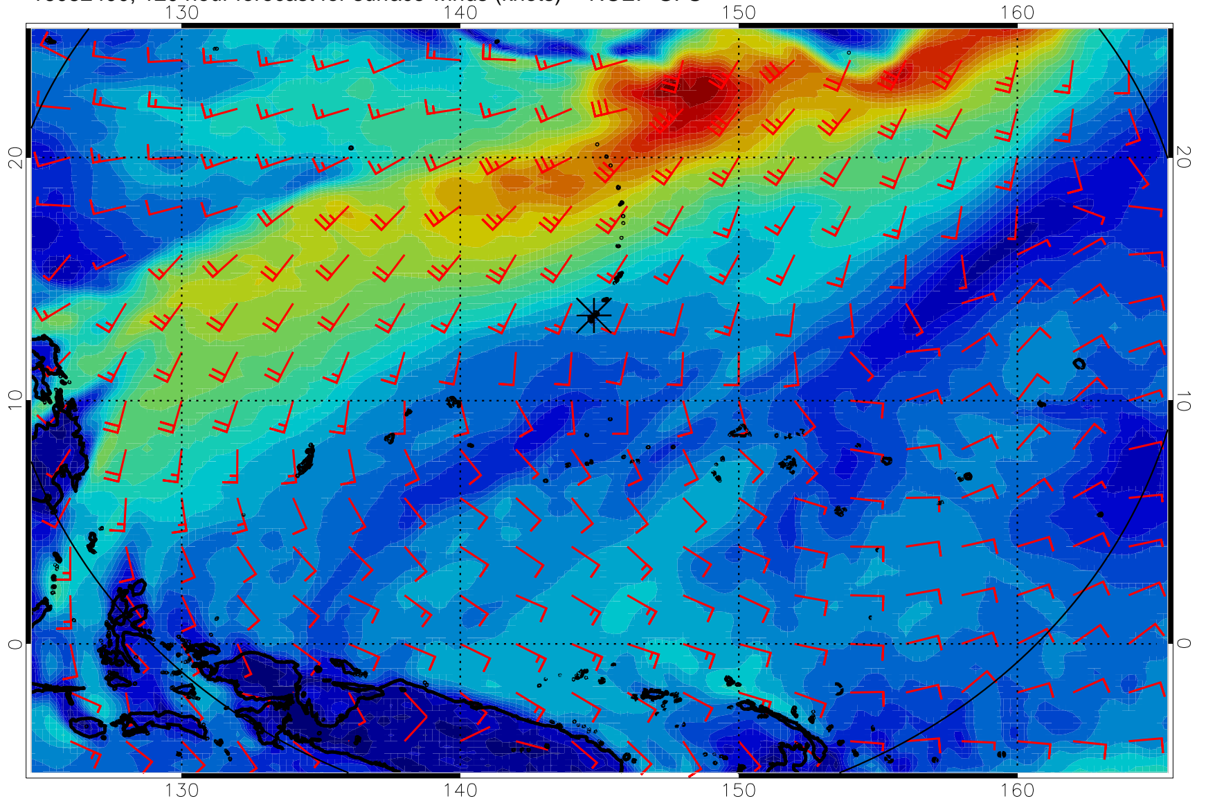
16082400, 120 hour forecast for surface winds (knots) -- NCEP GFS
