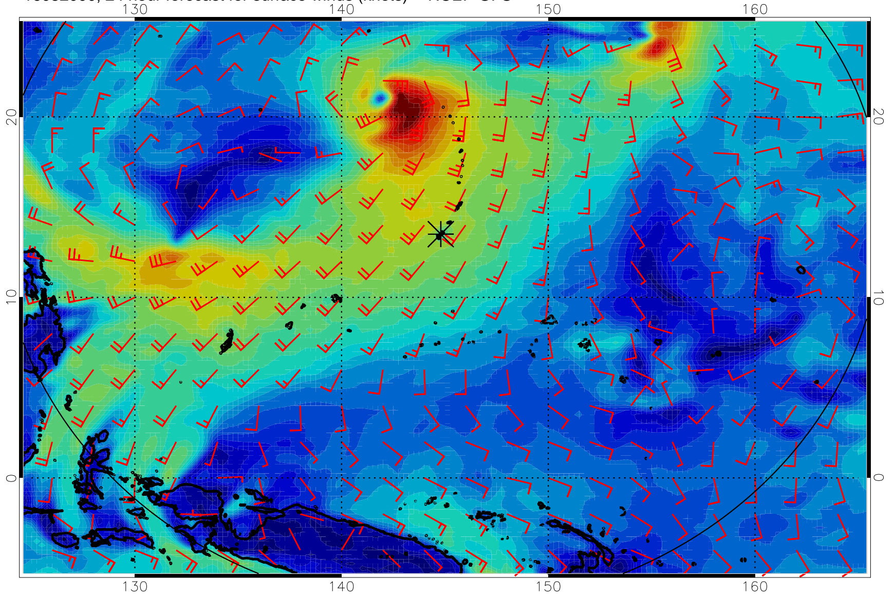
16082000, 24 hour forecast for surface winds (knots) -- NCEP GFS
