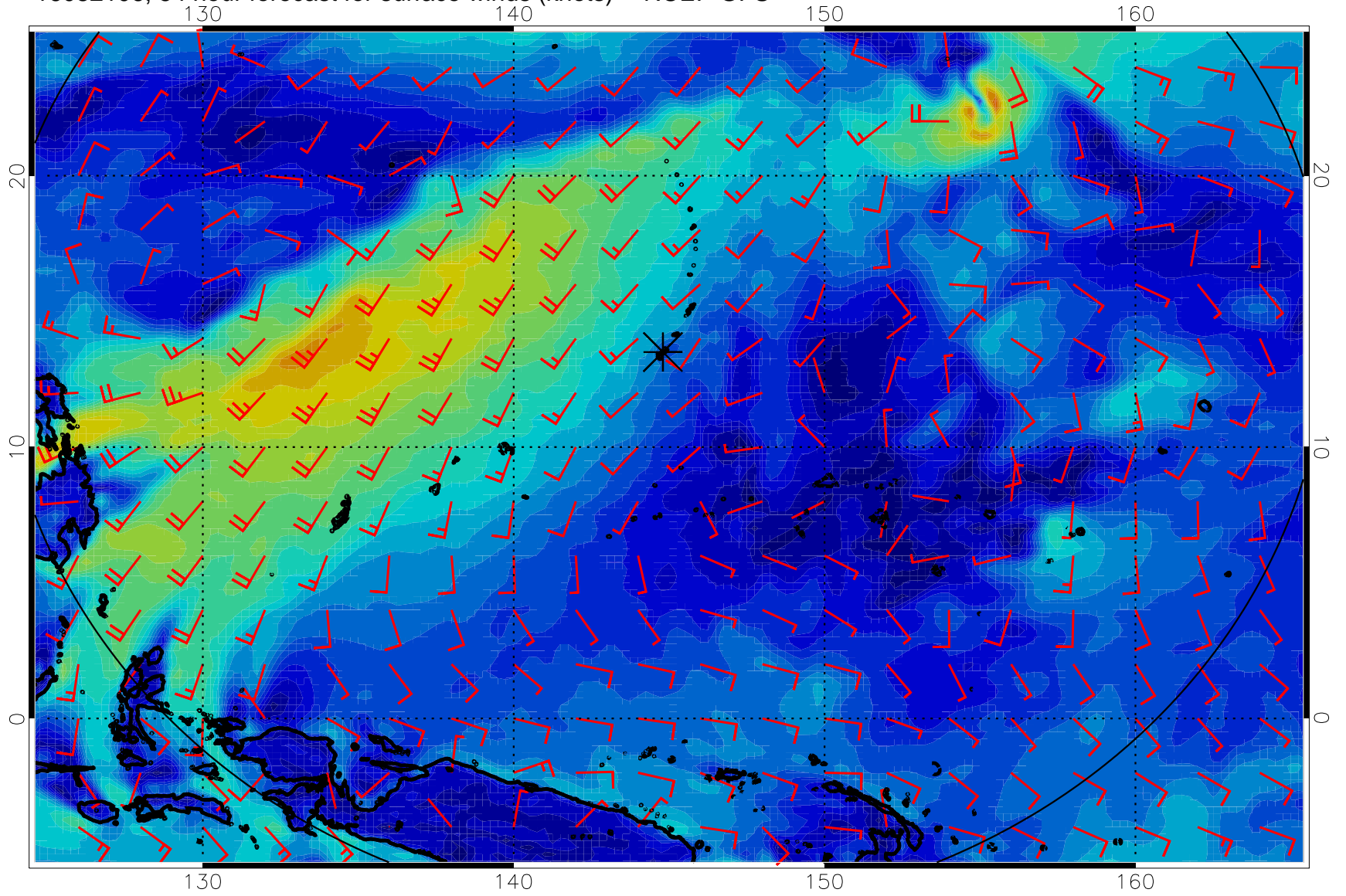
16082106, 54 hour forecast for surface winds (knots) -- NCEP GFS
