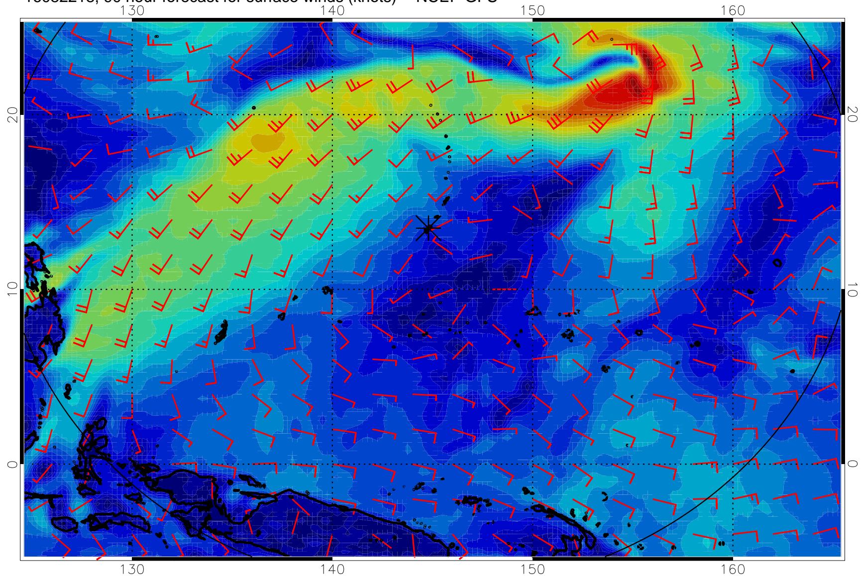
16082218, 90 hour forecast for surface winds (knots) -- NCEP GFS
