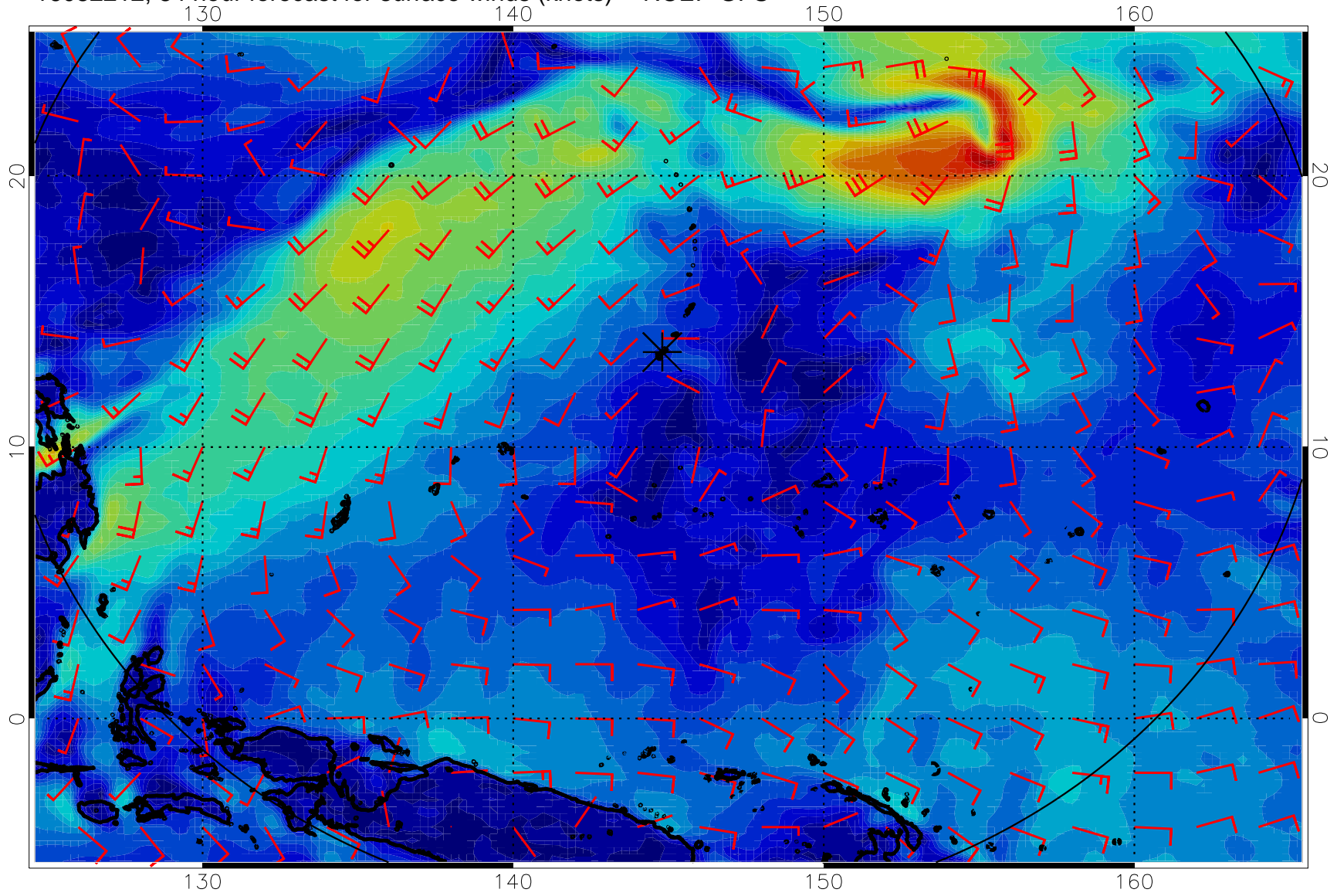
16082212, 84 hour forecast for surface winds (knots) -- NCEP GFS
