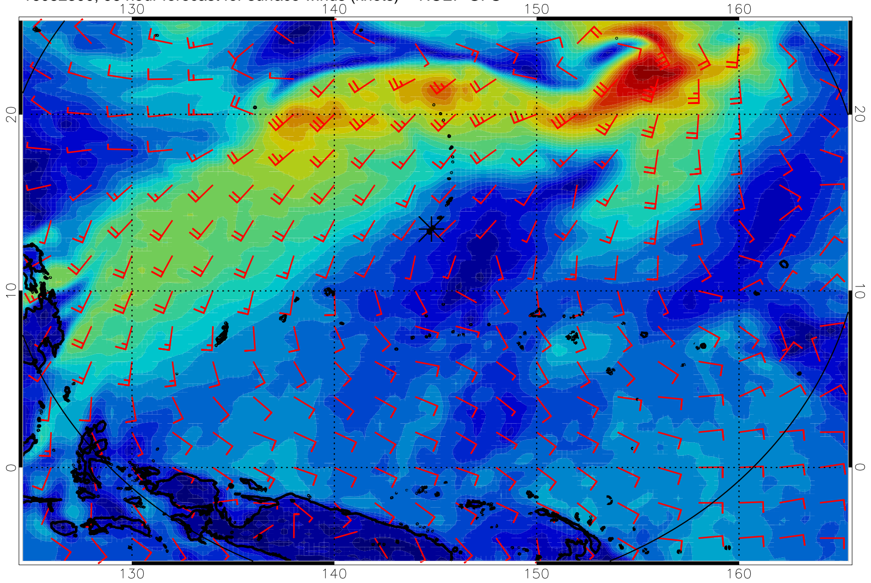
16082300, 96 hour forecast for surface winds (knots) -- NCEP GFS
