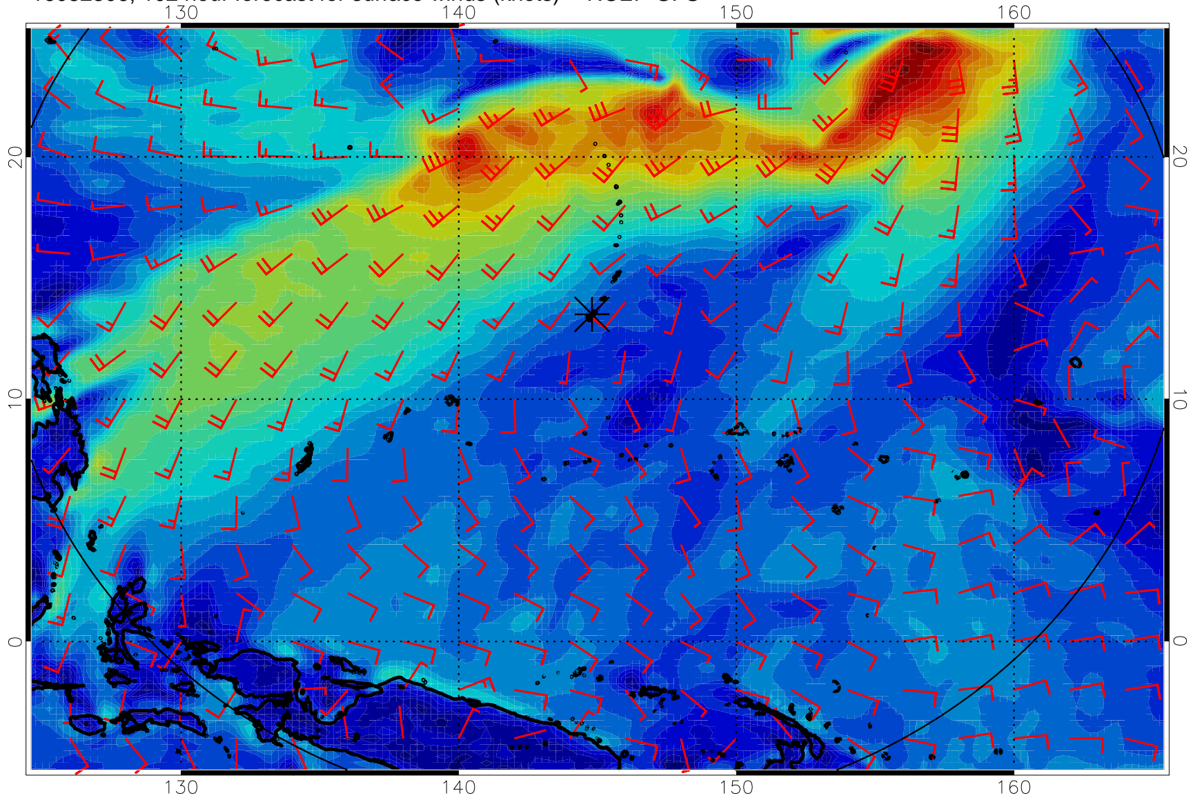
16082306, 102 hour forecast for surface winds (knots) -- NCEP GFS
