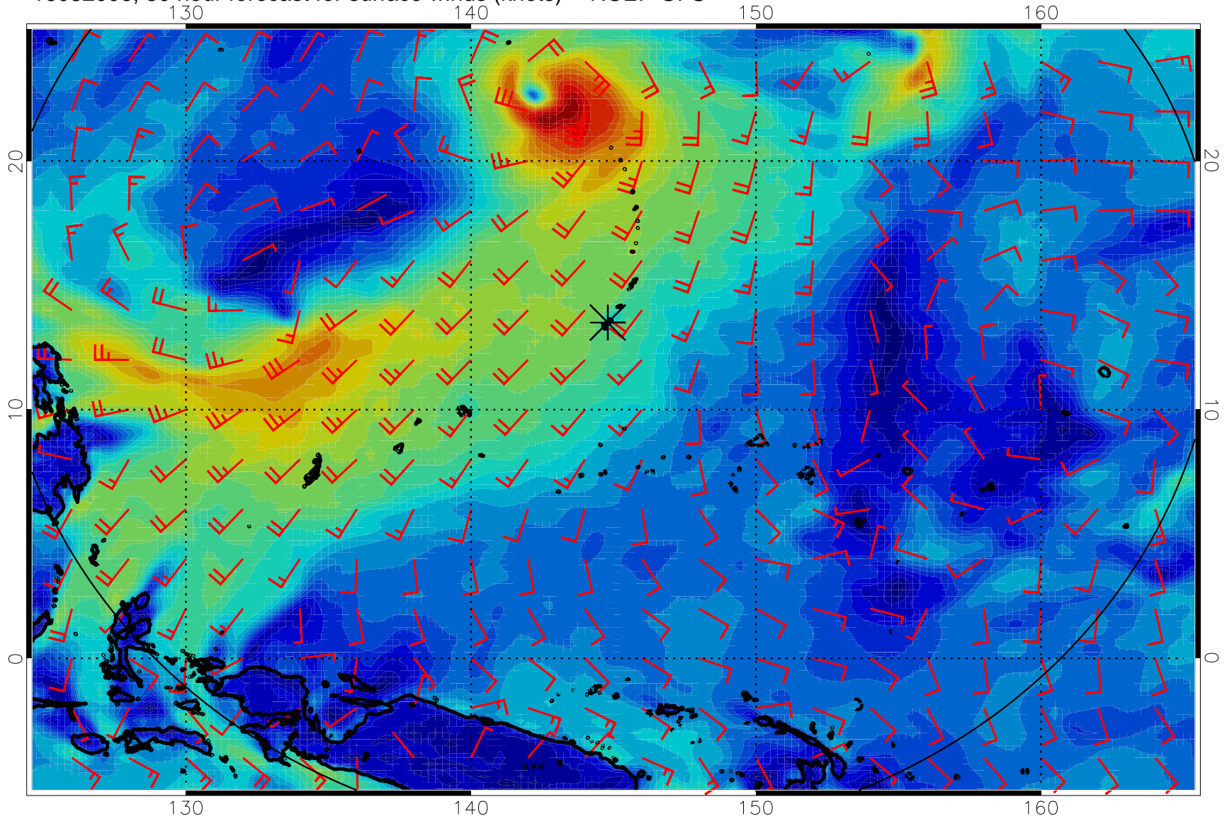
16082006, 30 hour forecast for surface winds (knots) -- NCEP GFS
