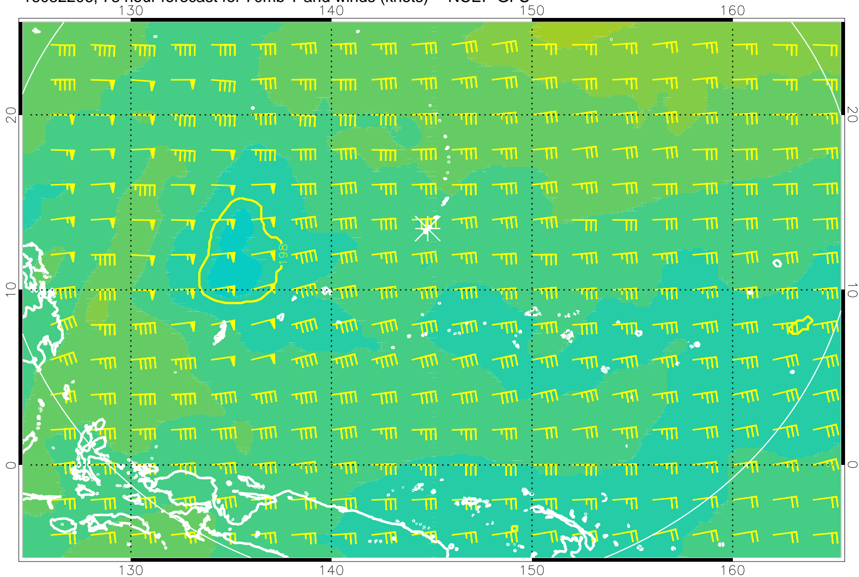
16082206, 78 hour forecast for 70mb T and winds (knots) -- NCEP GFS
