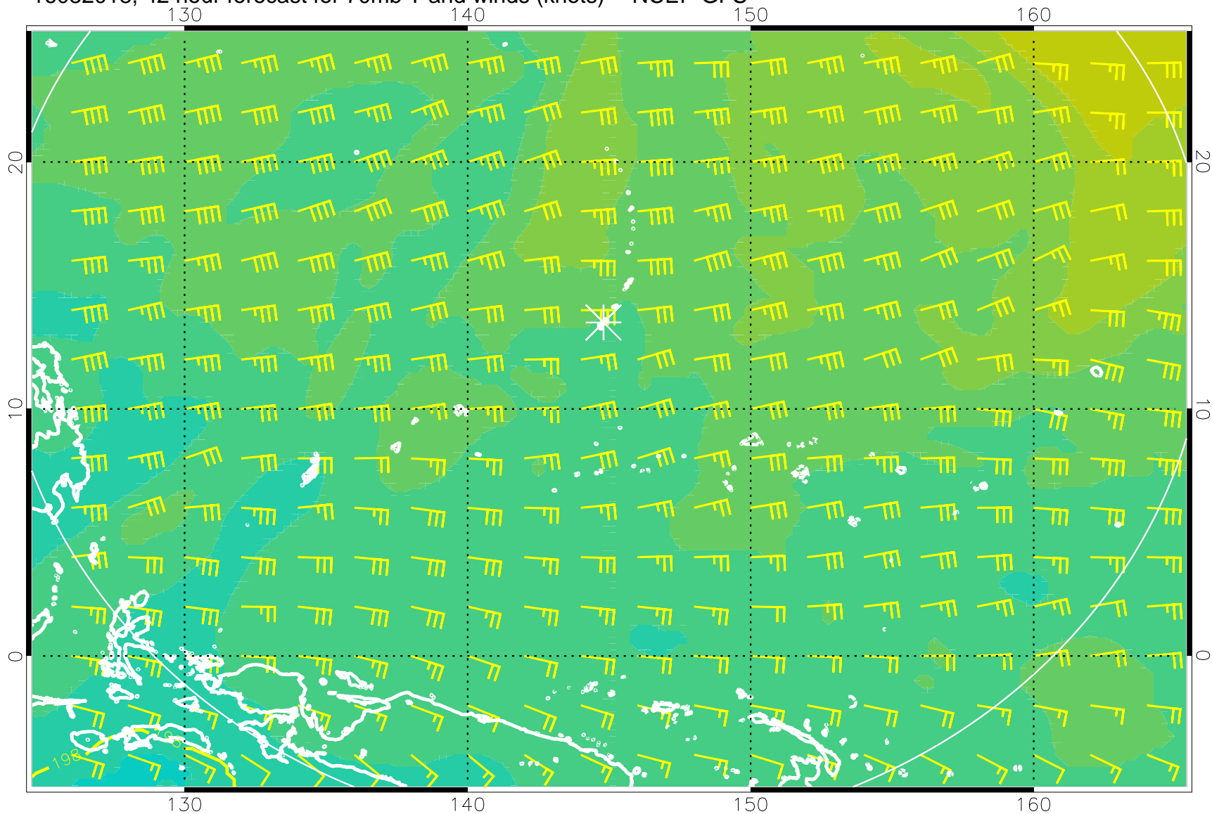
16082018, 42 hour forecast for 70mb T and winds (knots) -- NCEP GFS
