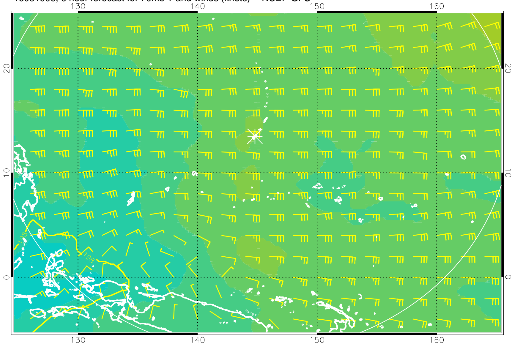
16081906, 6 hour forecast for 70mb T and winds (knots) -- NCEP GFS
