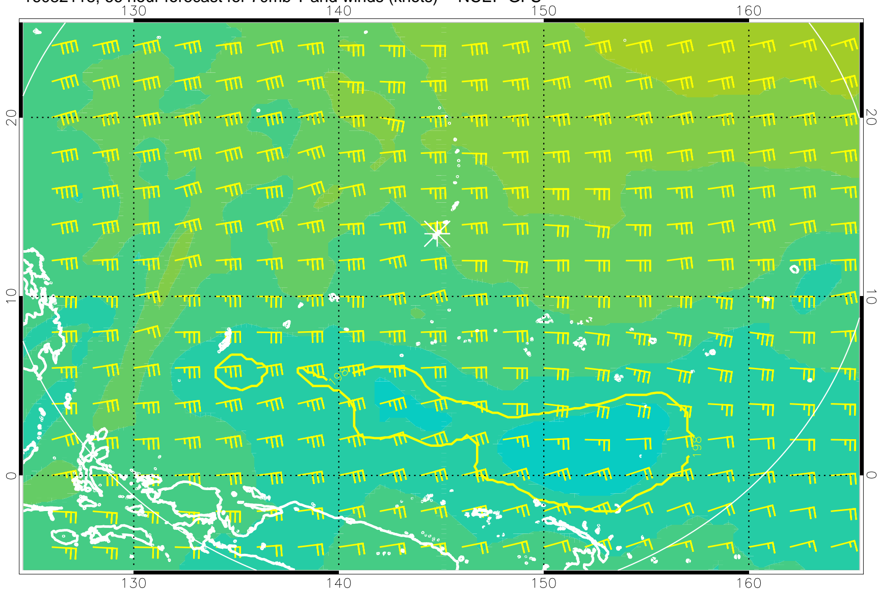
16082118, 66 hour forecast for 70mb T and winds (knots) -- NCEP GFS
