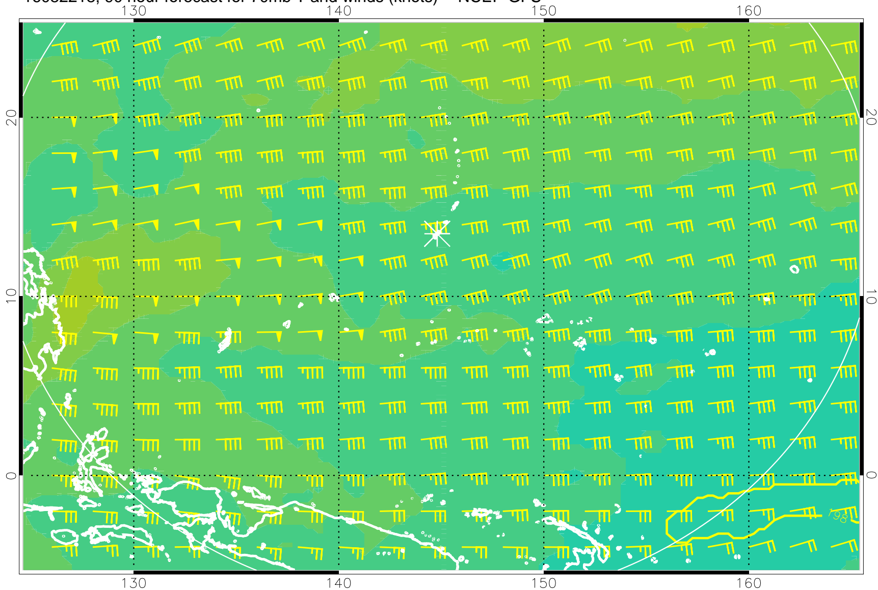
16082218, 90 hour forecast for 70mb T and winds (knots) -- NCEP GFS
