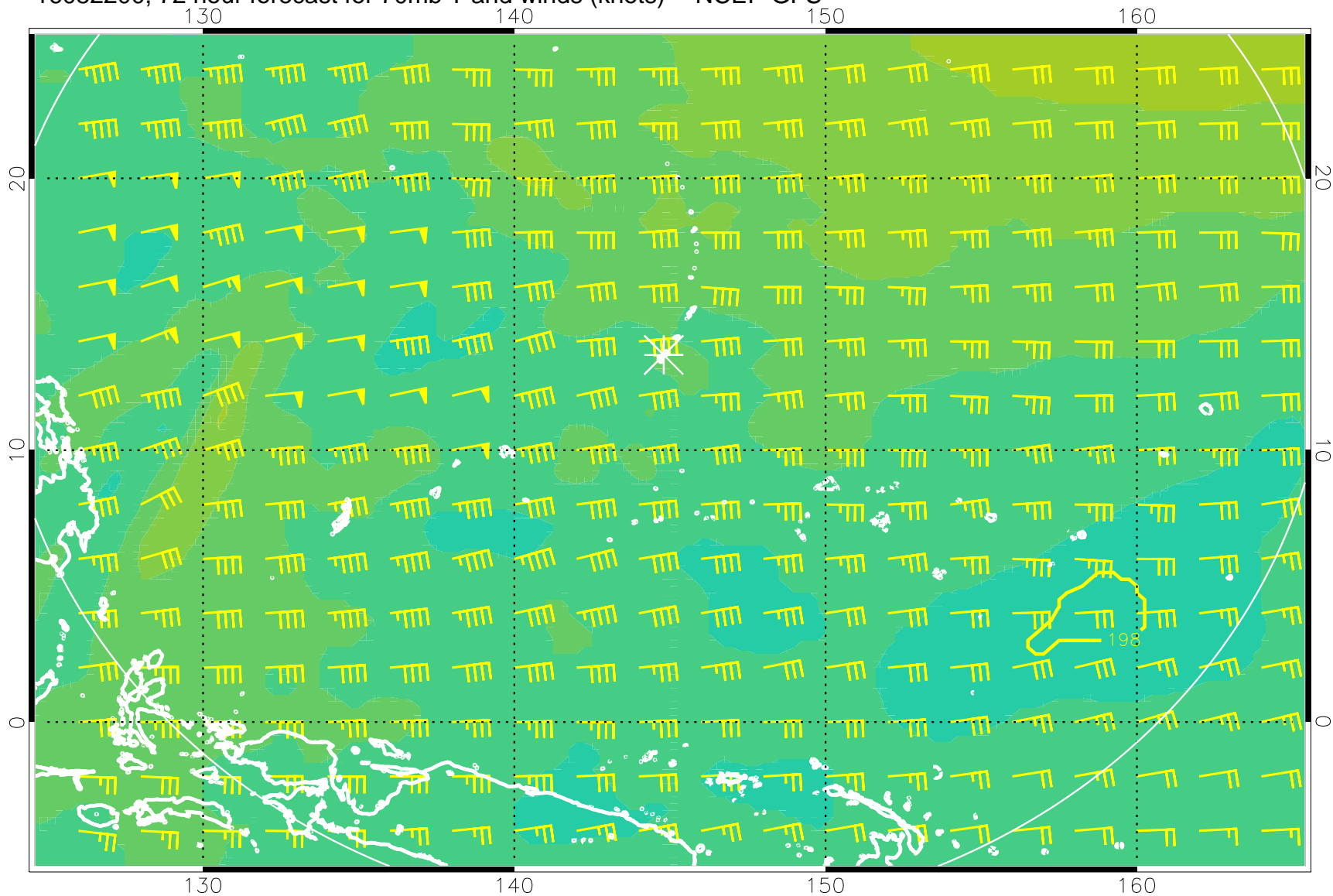
16082200, 72 hour forecast for 70mb T and winds (knots) -- NCEP GFS
