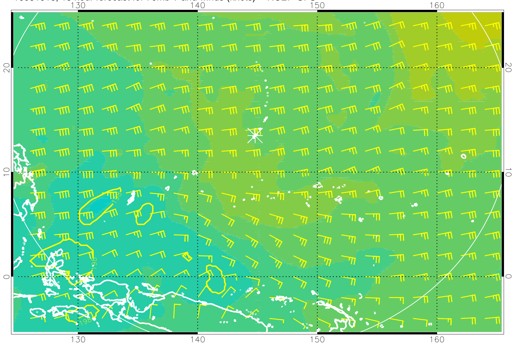
16081918, 18 hour forecast for 70mb T and winds (knots) -- NCEP GFS
