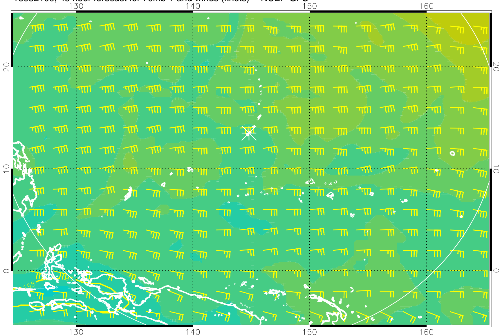
16082100, 48 hour forecast for 70mb T and winds (knots) -- NCEP GFS
