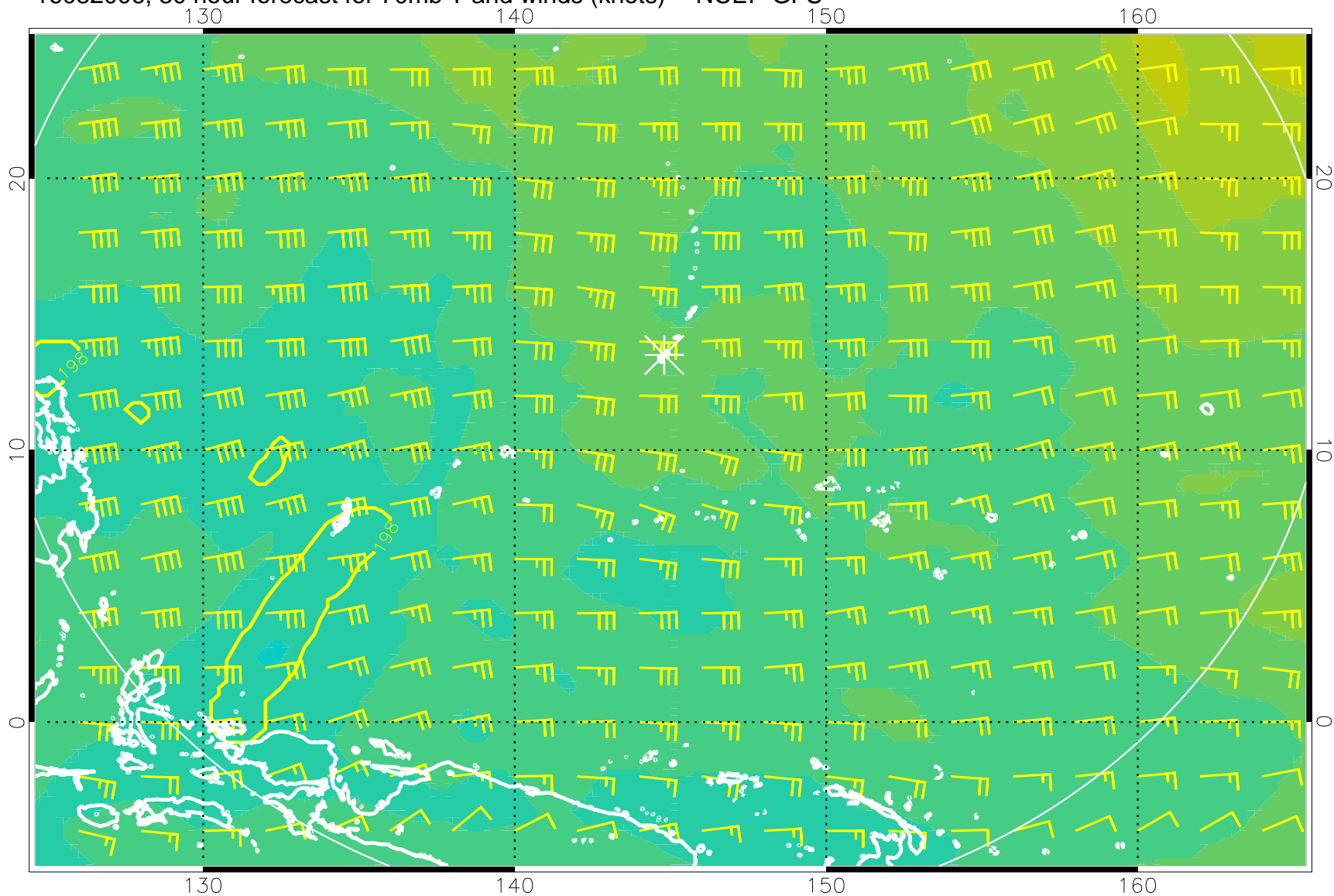
16082006, 30 hour forecast for 70mb T and winds (knots) -- NCEP GFS
