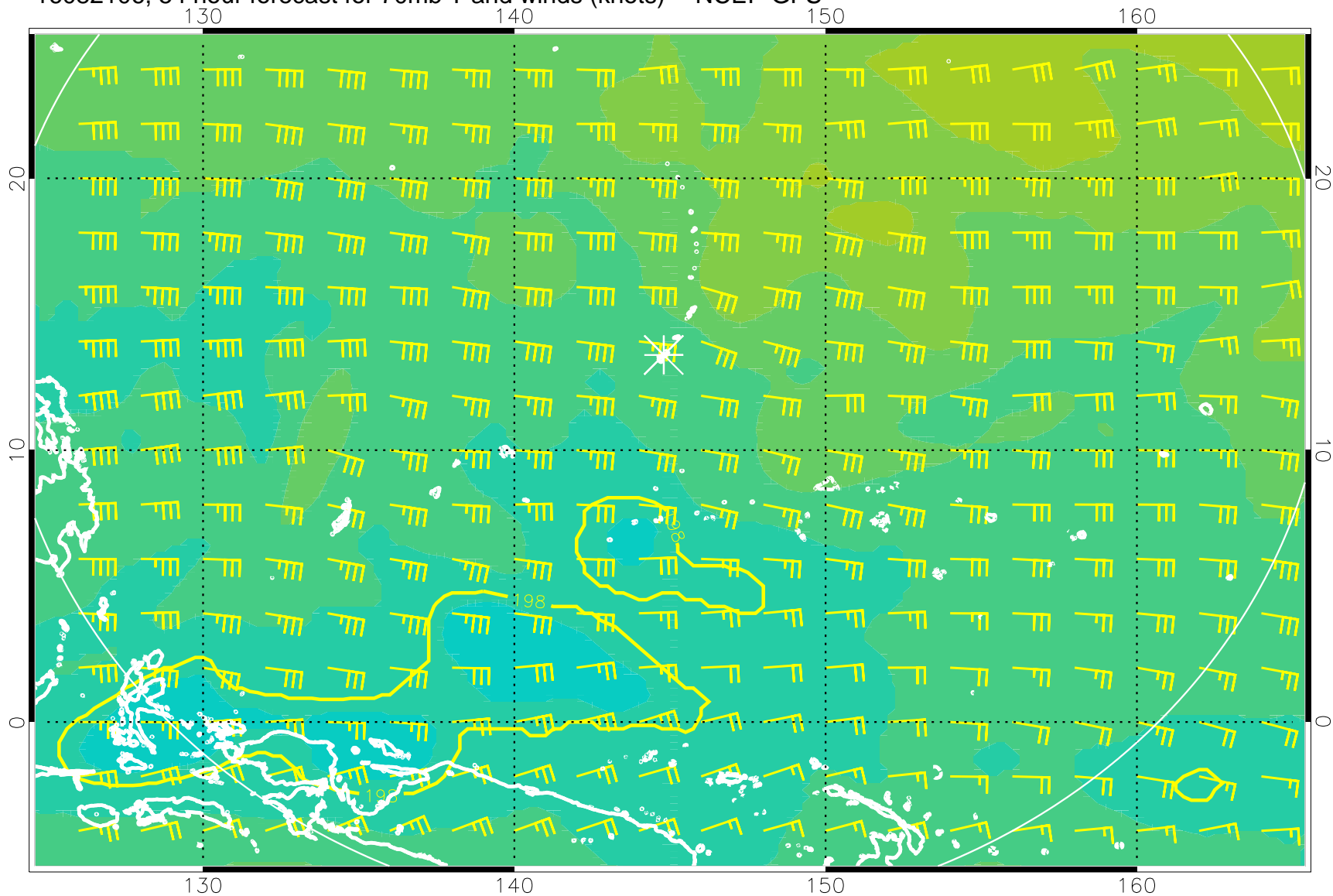
16082106, 54 hour forecast for 70mb T and winds (knots) -- NCEP GFS
