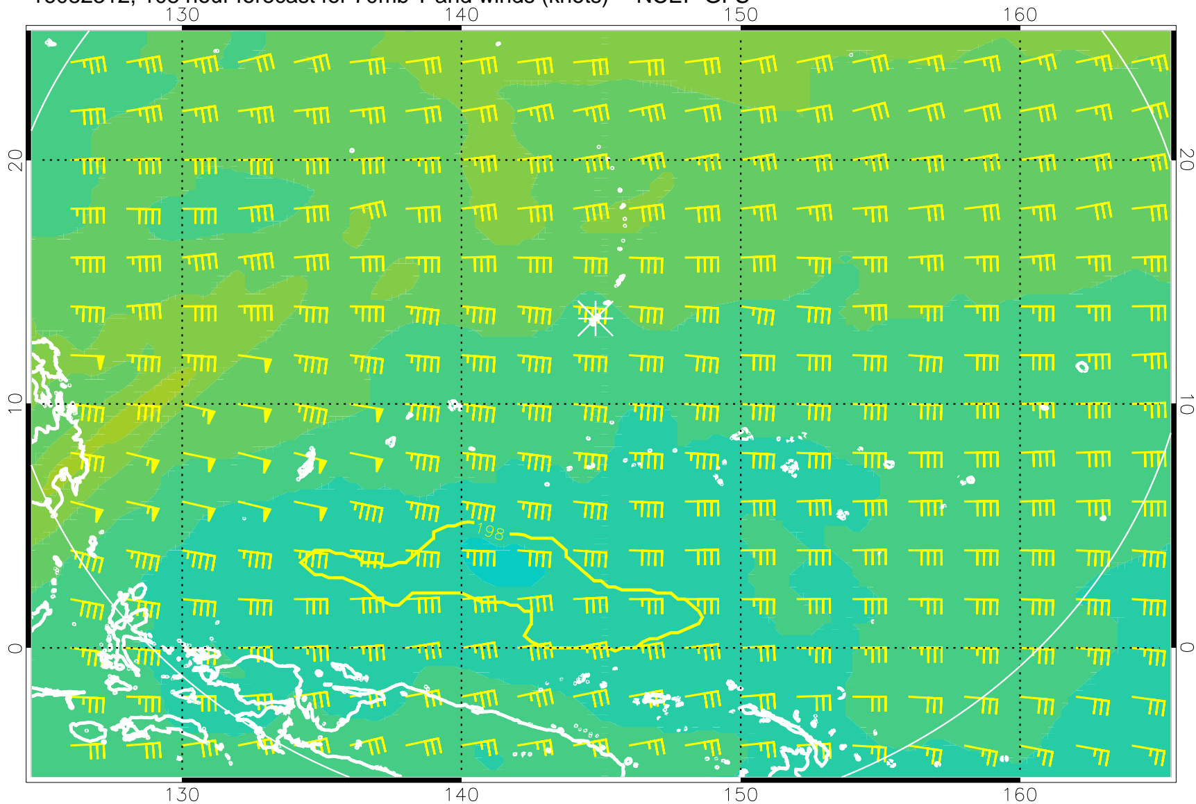
16082312, 108 hour forecast for 70mb T and winds (knots) -- NCEP GFS
