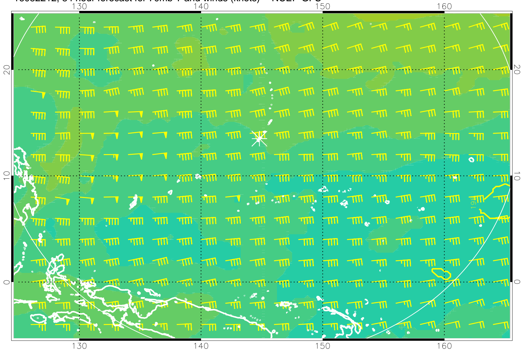
16082212, 84 hour forecast for 70mb T and winds (knots) -- NCEP GFS
