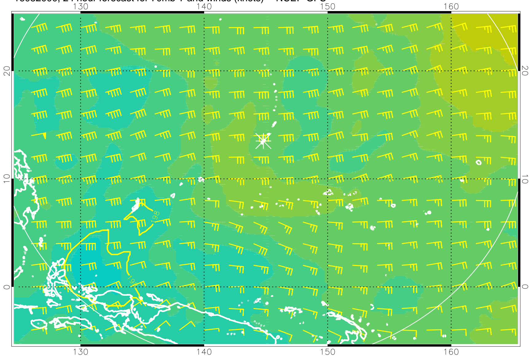
16082000, 24 hour forecast for 70mb T and winds (knots) -- NCEP GFS
