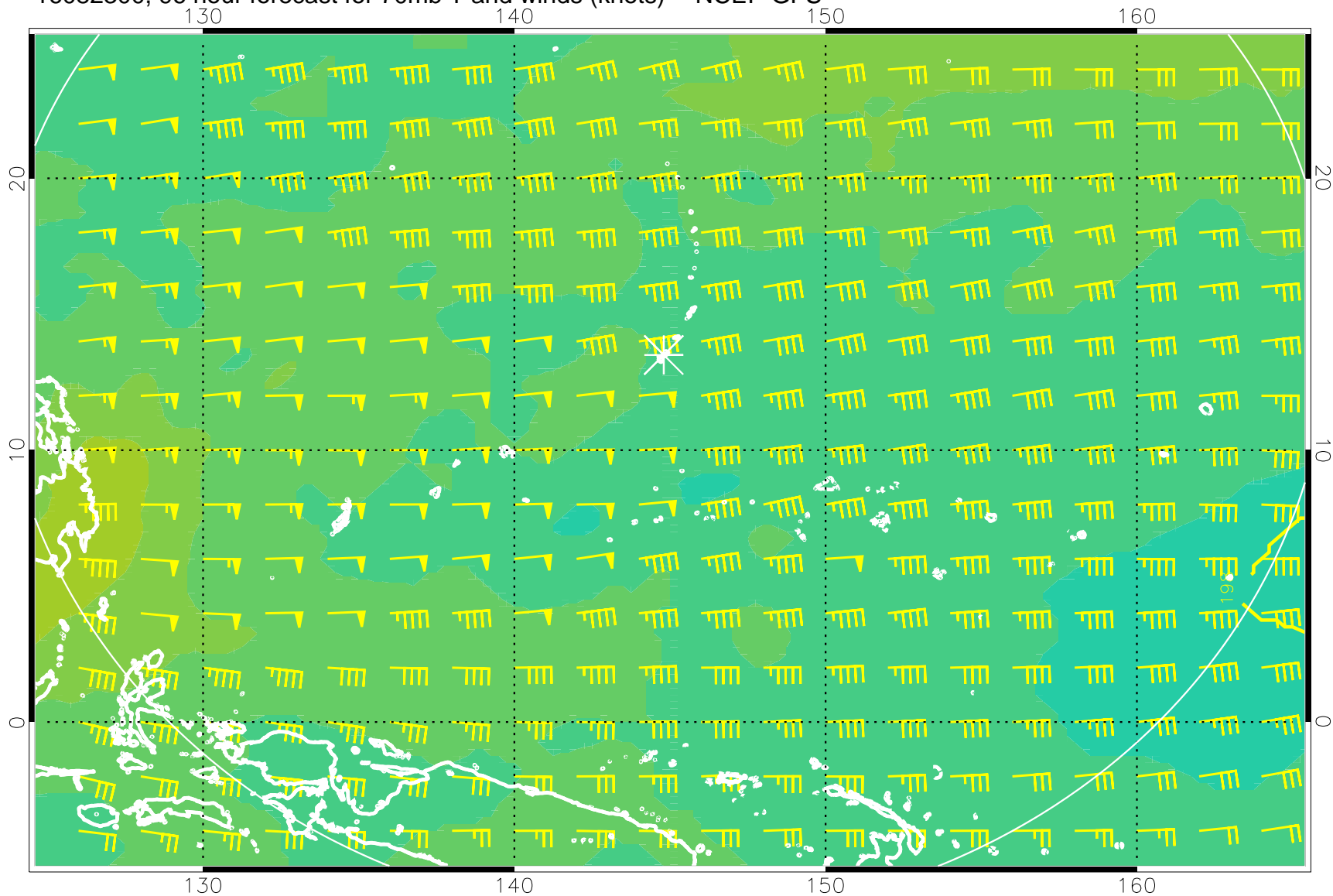
16082300, 96 hour forecast for 70mb T and winds (knots) -- NCEP GFS
