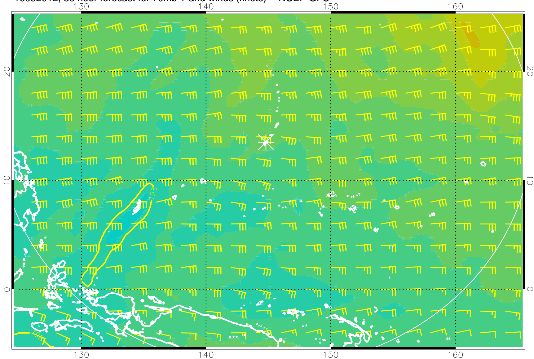
16082012, 36 hour forecast for 70mb T and winds (knots) -- NCEP GFS
