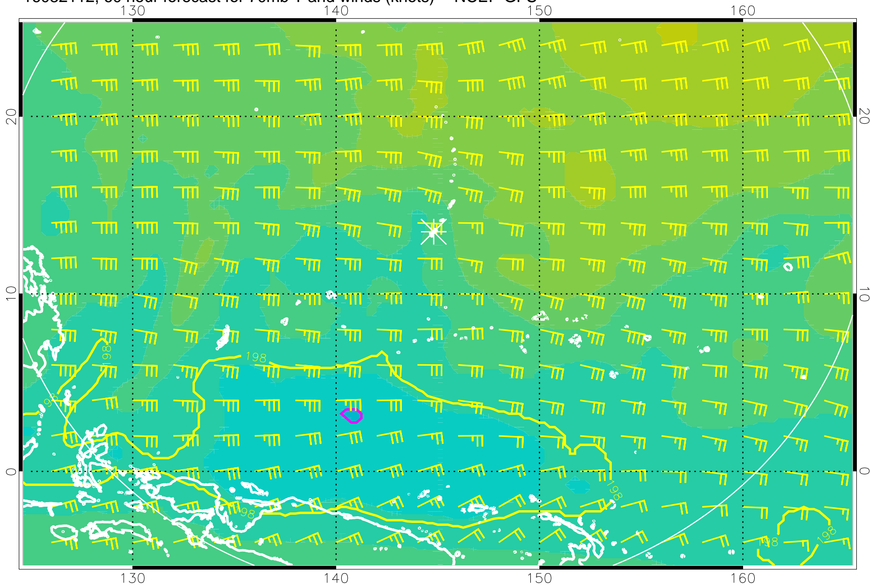
16082112, 60 hour forecast for 70mb T and winds (knots) -- NCEP GFS
