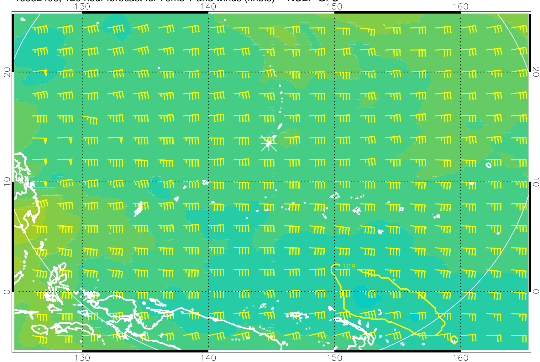
16082400, 120 hour forecast for 70mb T and winds (knots) -- NCEP GFS
