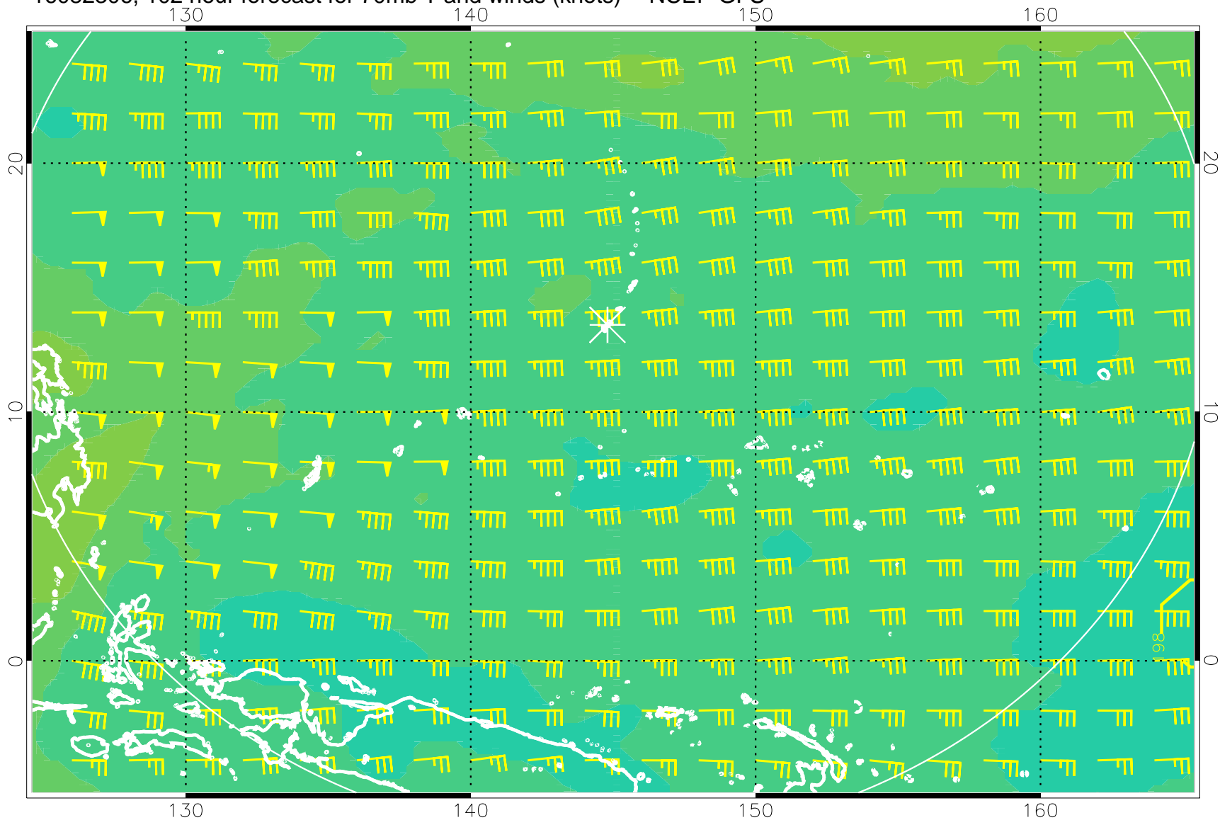
16082306, 102 hour forecast for 70mb T and winds (knots) -- NCEP GFS
