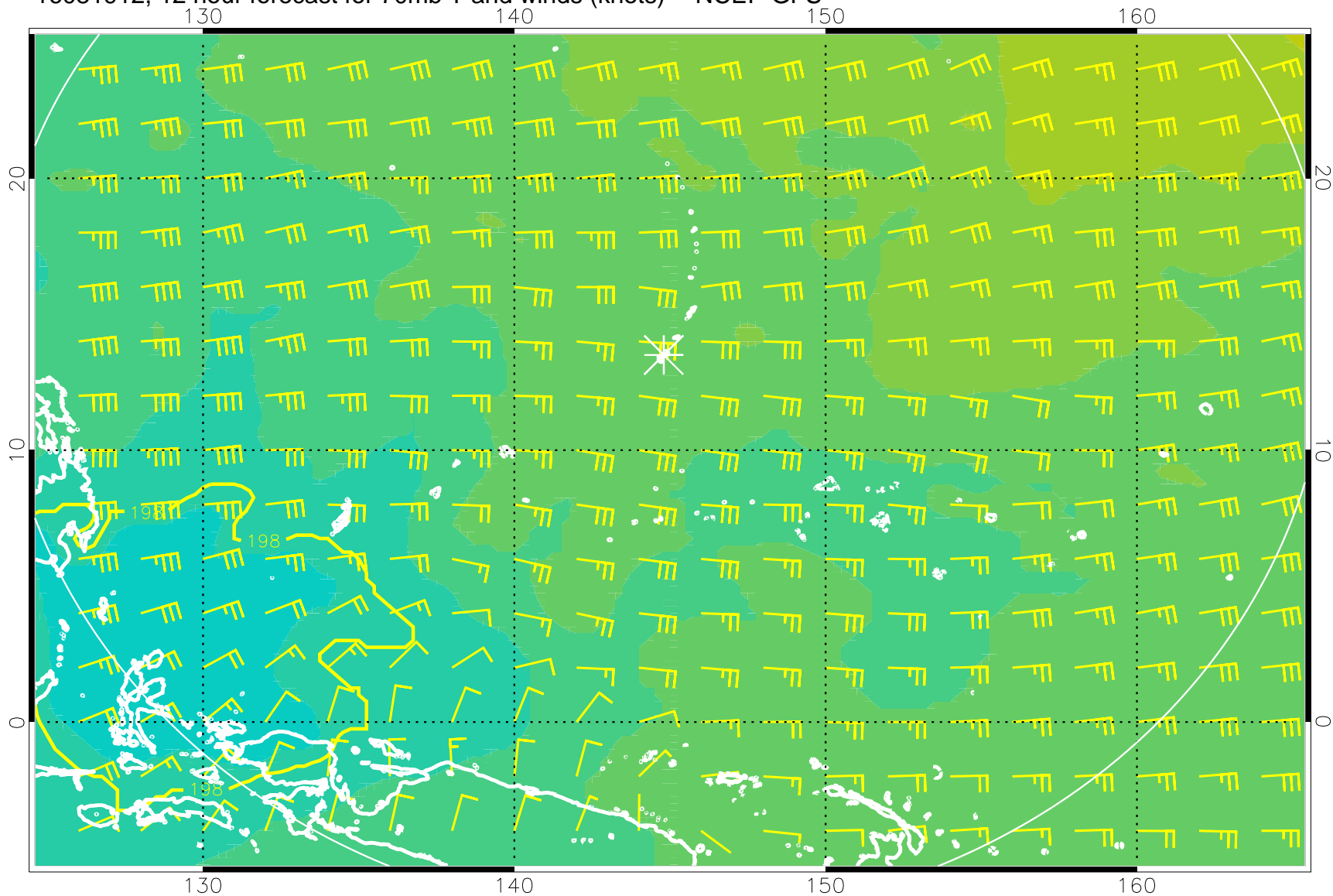
16081912, 12 hour forecast for 70mb T and winds (knots) -- NCEP GFS
