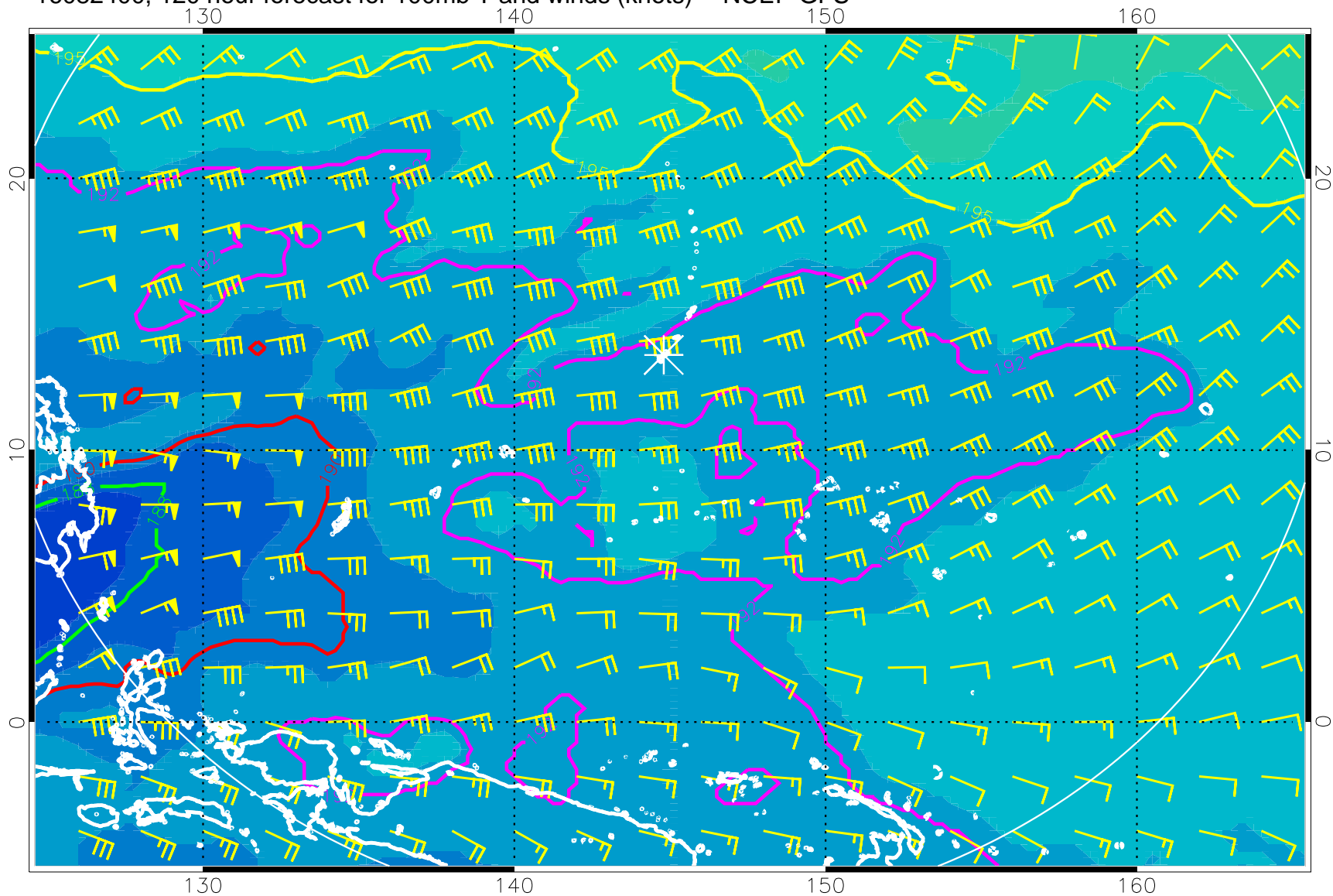
16082400, 120 hour forecast for 100mb T and winds (knots) -- NCEP GFS
