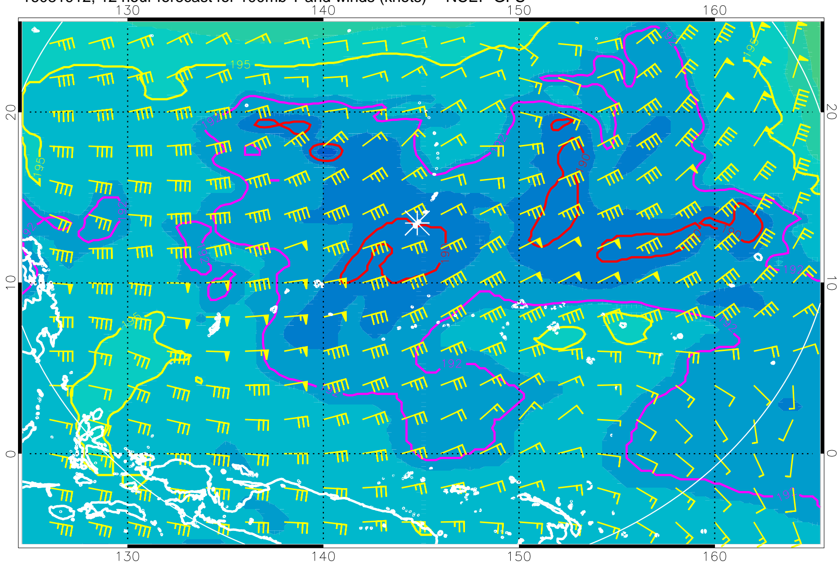
16081912, 12 hour forecast for 100mb T and winds (knots) -- NCEP GFS
