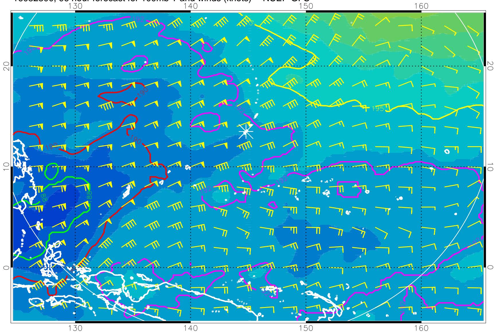
16082300, 96 hour forecast for 100mb T and winds (knots) -- NCEP GFS
