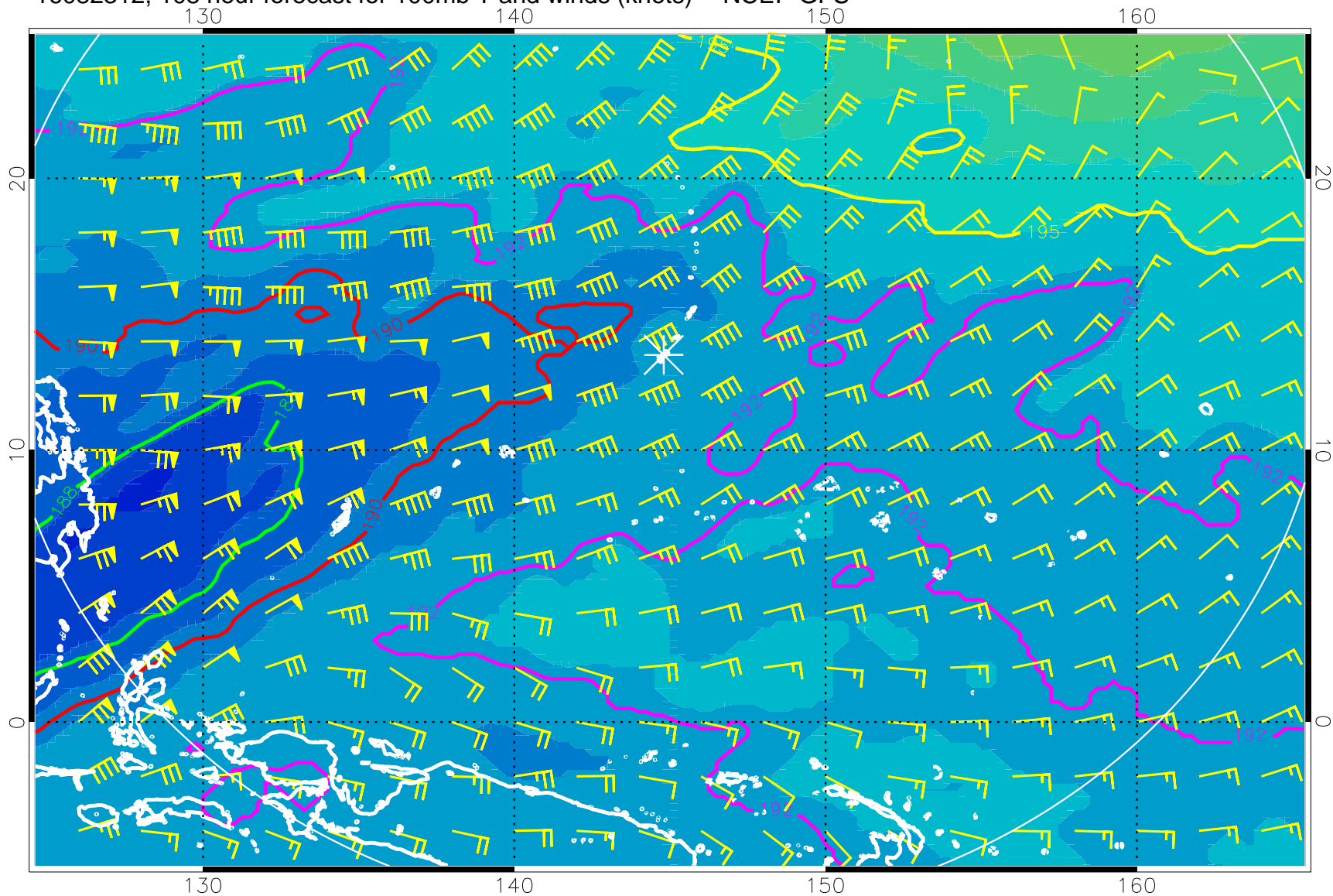
16082312, 108 hour forecast for 100mb T and winds (knots) -- NCEP GFS
