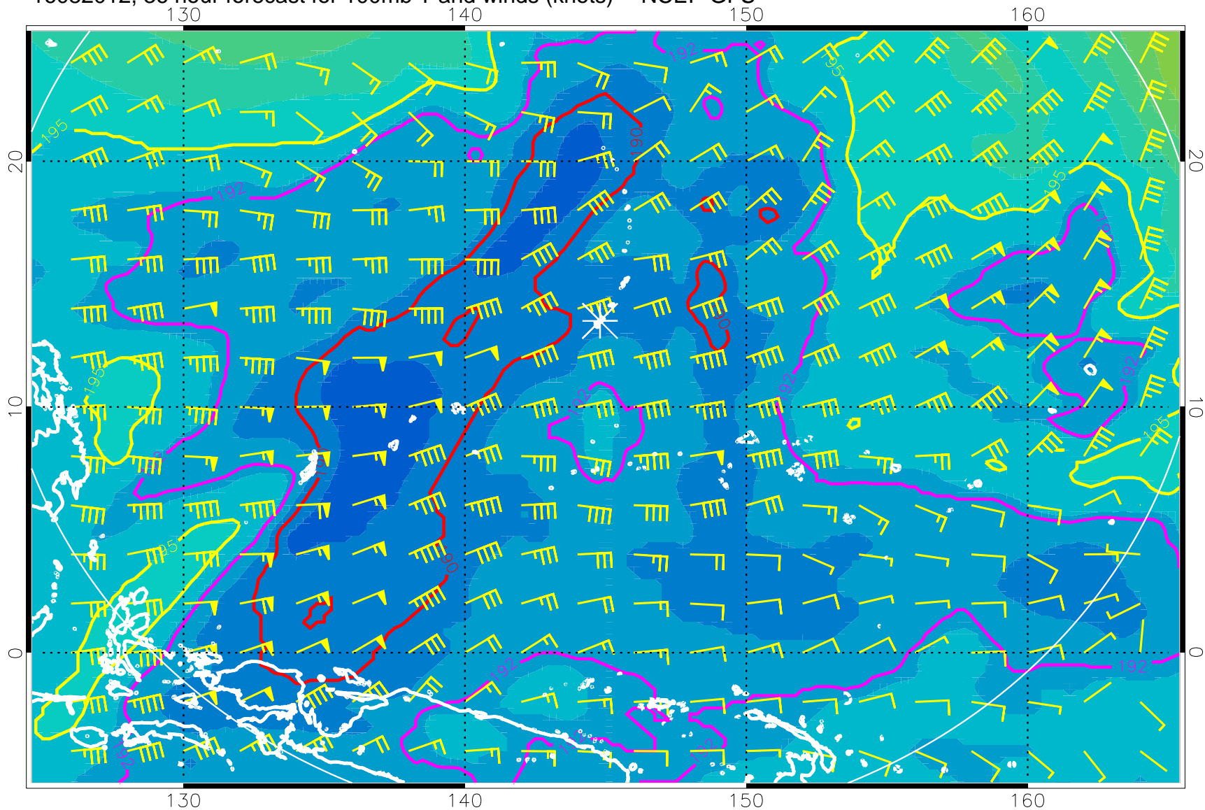
16082012, 36 hour forecast for 100mb T and winds (knots) -- NCEP GFS
