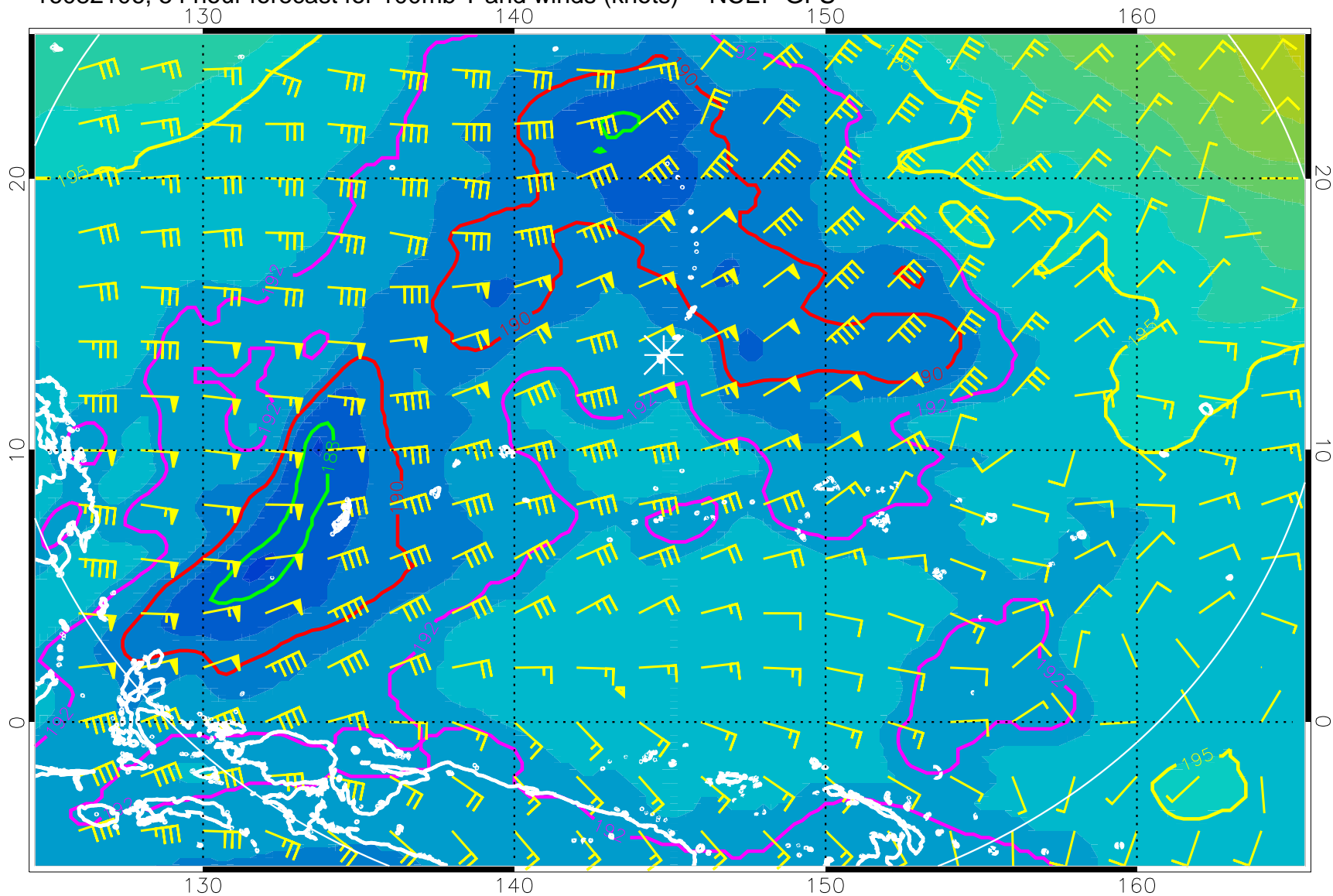
16082106, 54 hour forecast for 100mb T and winds (knots) -- NCEP GFS
