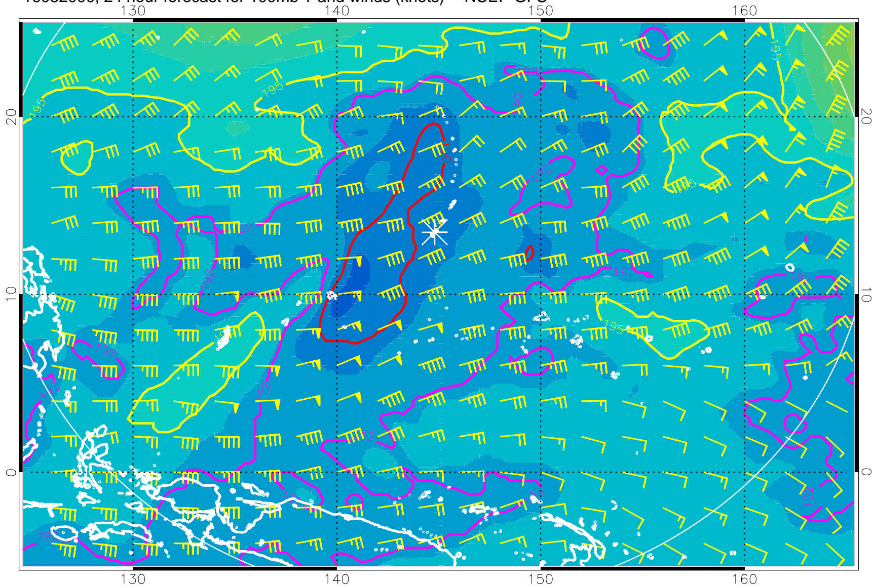
16082000, 24 hour forecast for 100mb T and winds (knots) -- NCEP GFS
