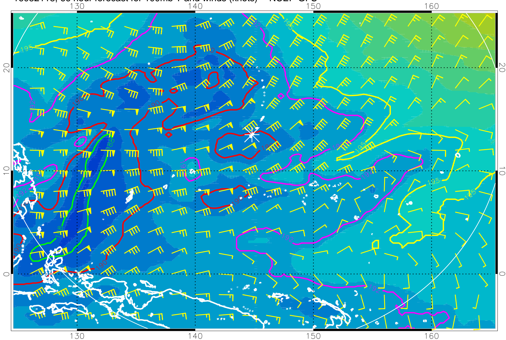
16082118, 66 hour forecast for 100mb T and winds (knots) -- NCEP GFS
