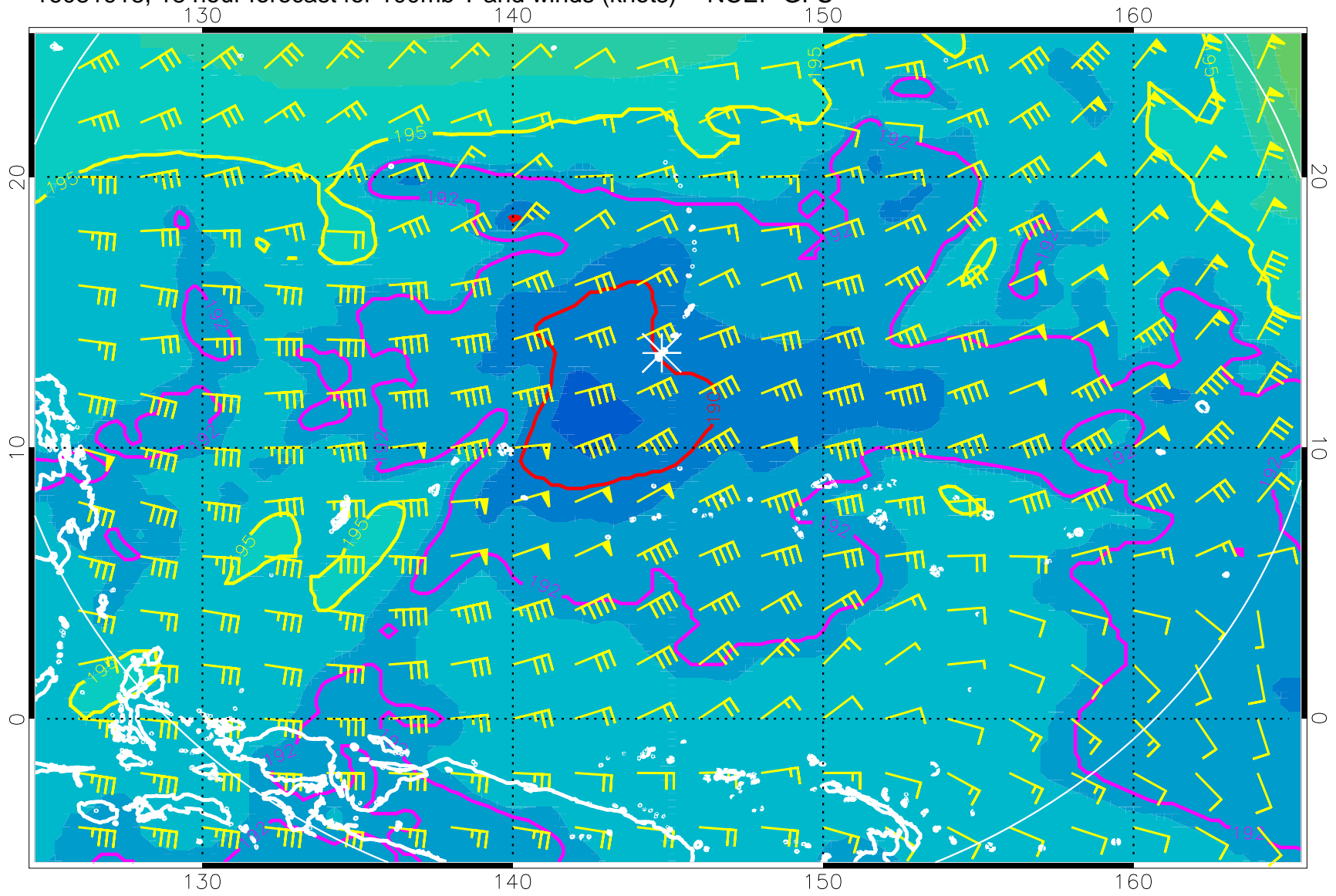
16081918, 18 hour forecast for 100mb T and winds (knots) -- NCEP GFS
