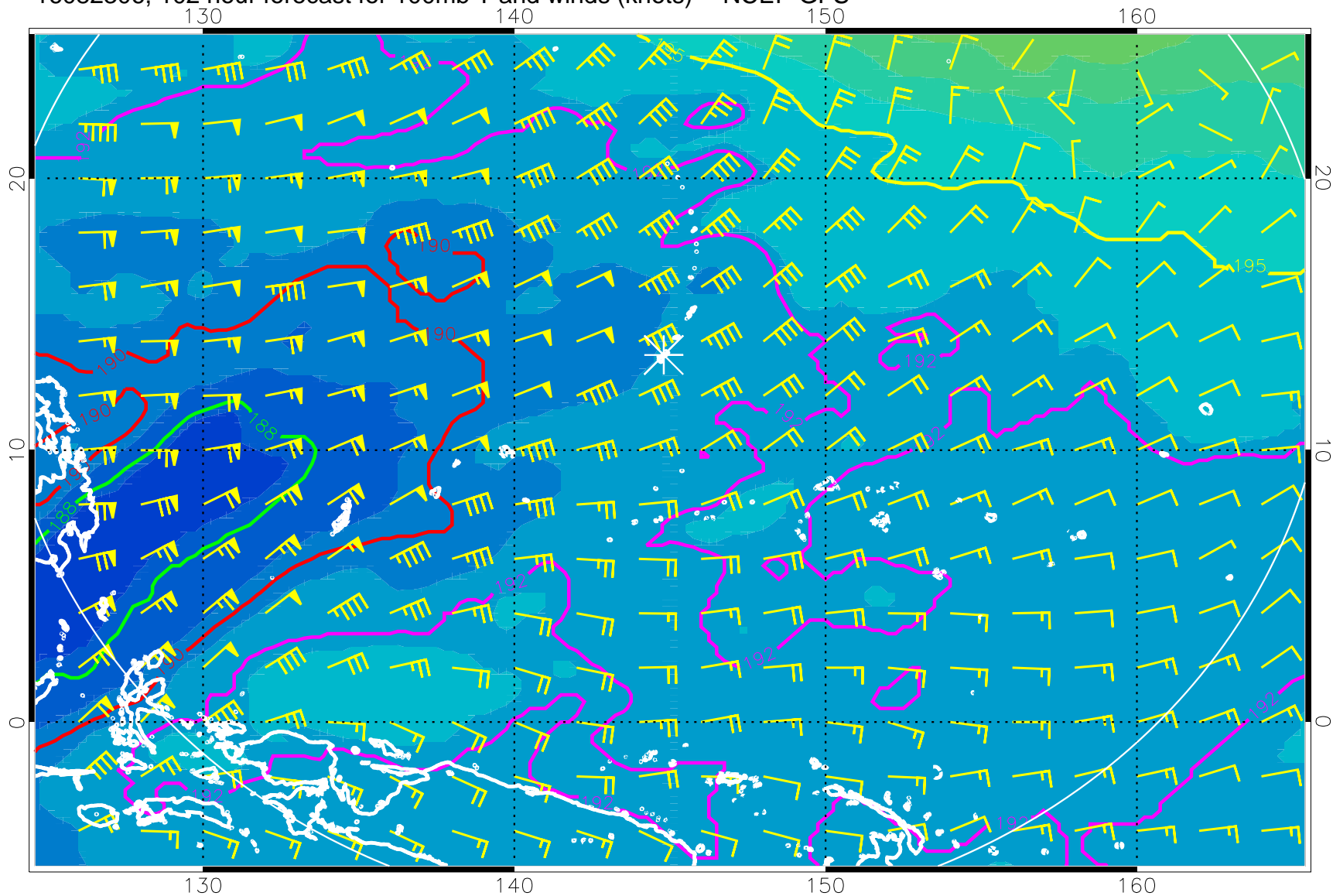
16082306, 102 hour forecast for 100mb T and winds (knots) -- NCEP GFS
