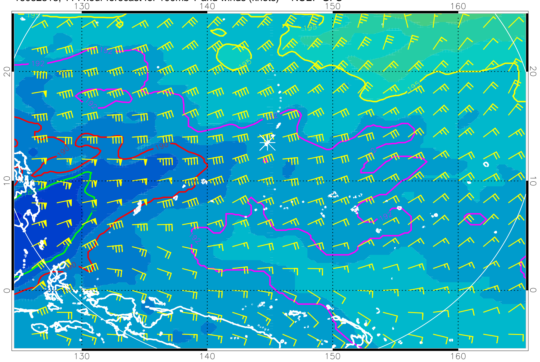
16082318, 114 hour forecast for 100mb T and winds (knots) -- NCEP GFS
