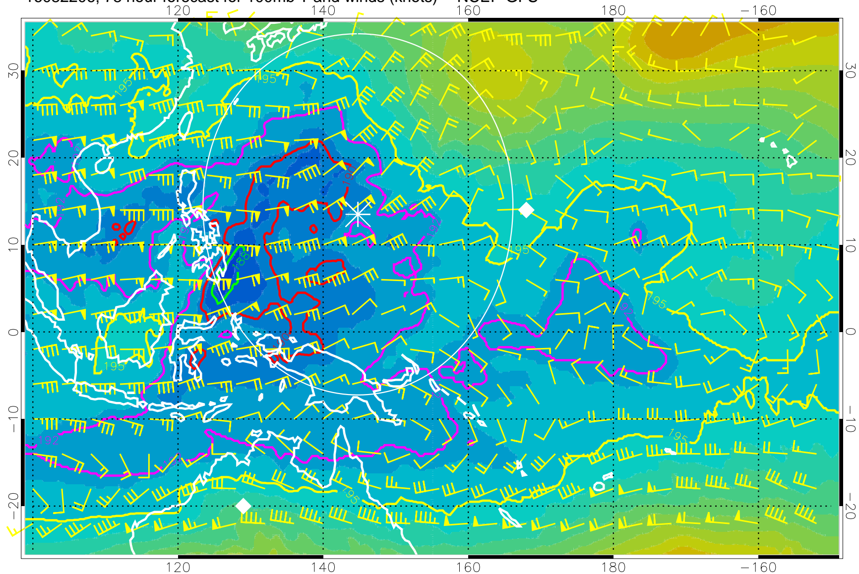
16082206, 78 hour forecast for 100mb T and winds (knots) -- NCEP GFS
