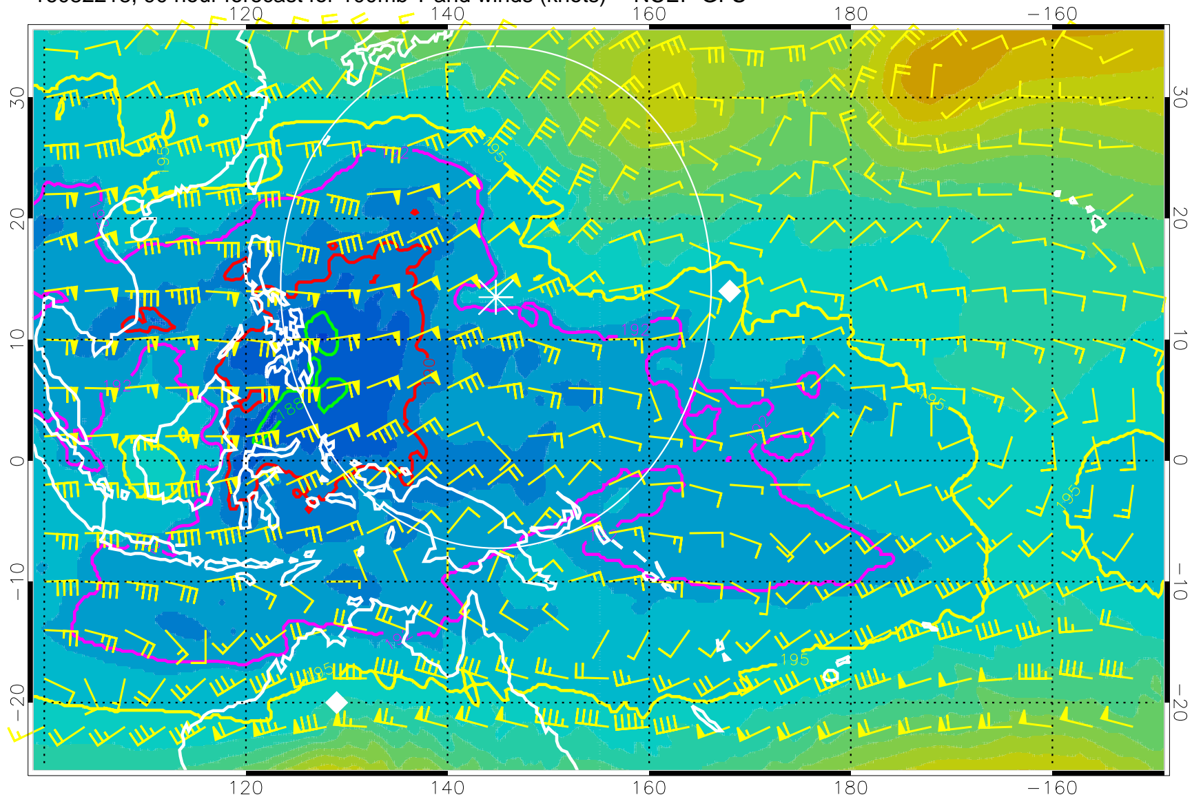
16082218, 90 hour forecast for 100mb T and winds (knots) -- NCEP GFS
