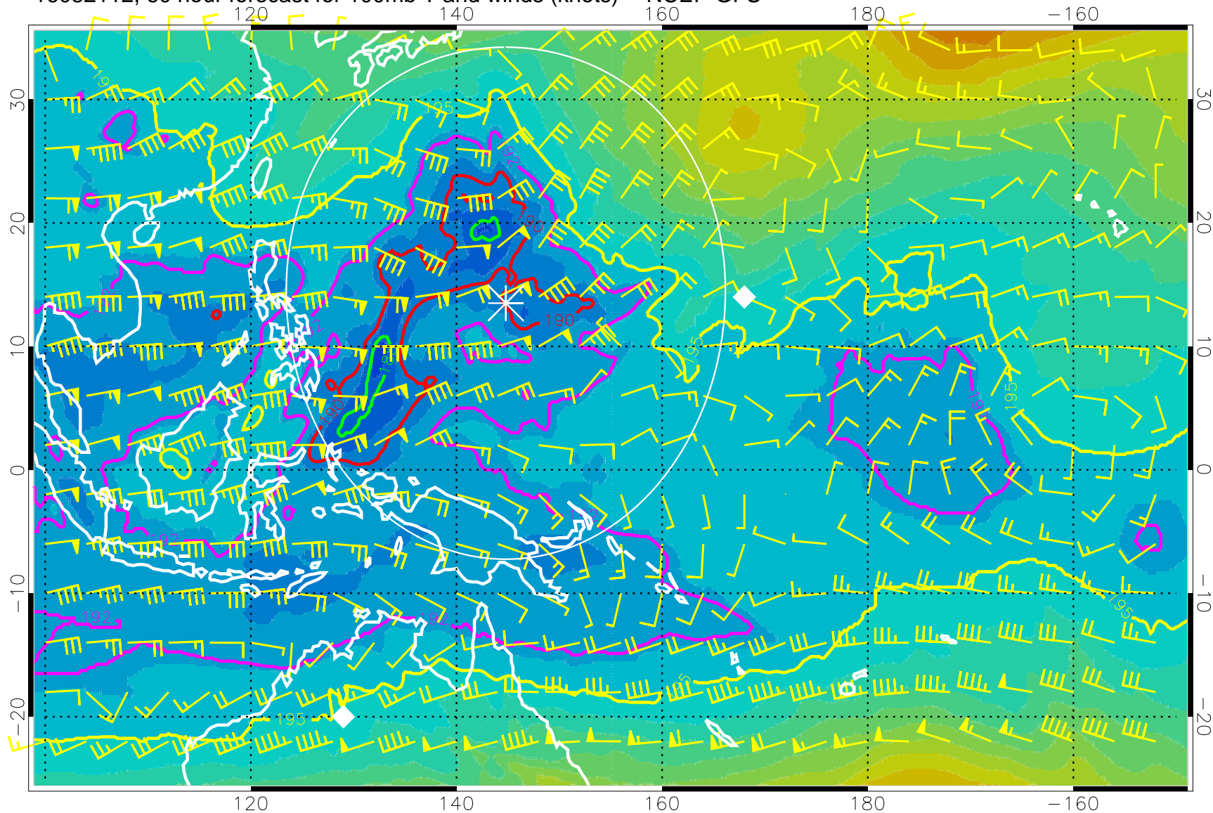
16082112, 60 hour forecast for 100mb T and winds (knots) -- NCEP GFS
