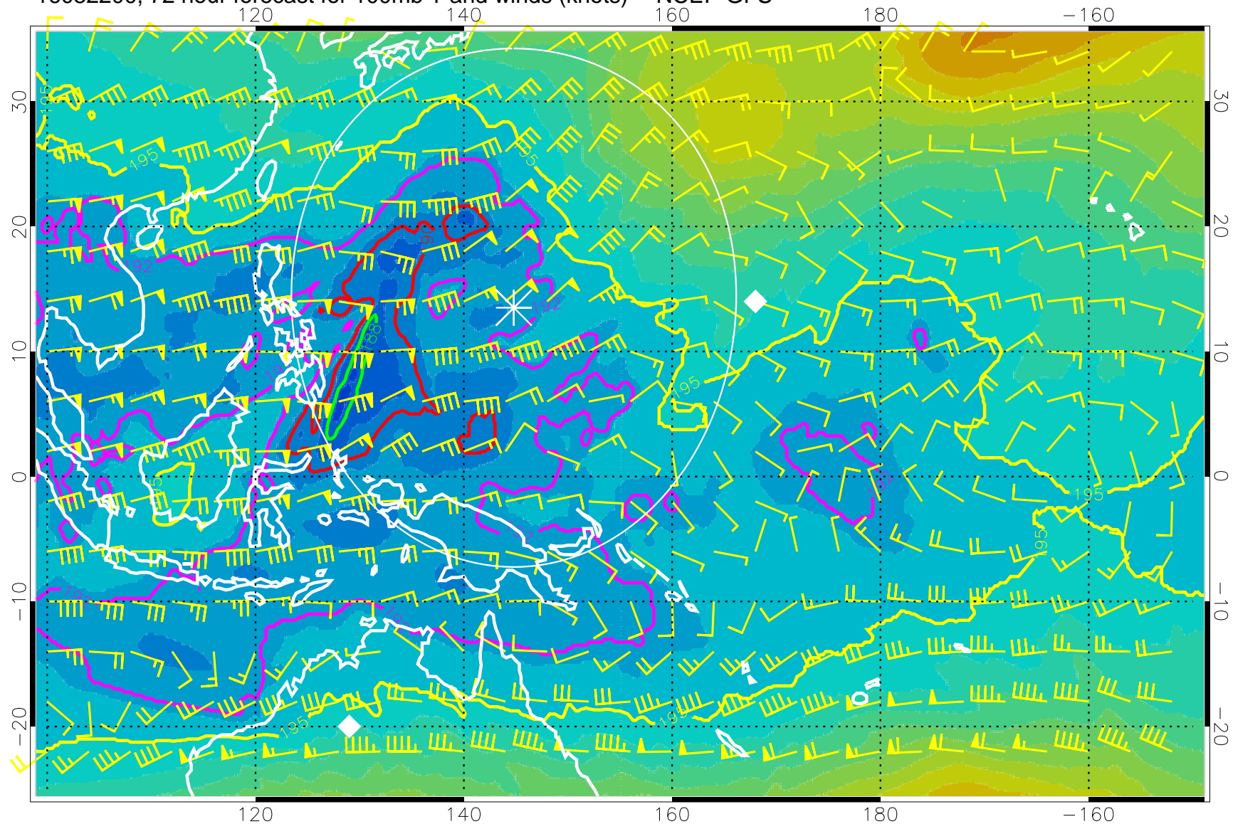
16082200, 72 hour forecast for 100mb T and winds (knots) -- NCEP GFS
