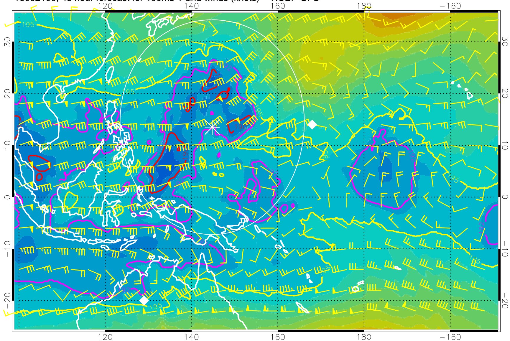
16082100, 48 hour forecast for 100mb T and winds (knots) -- NCEP GFS
