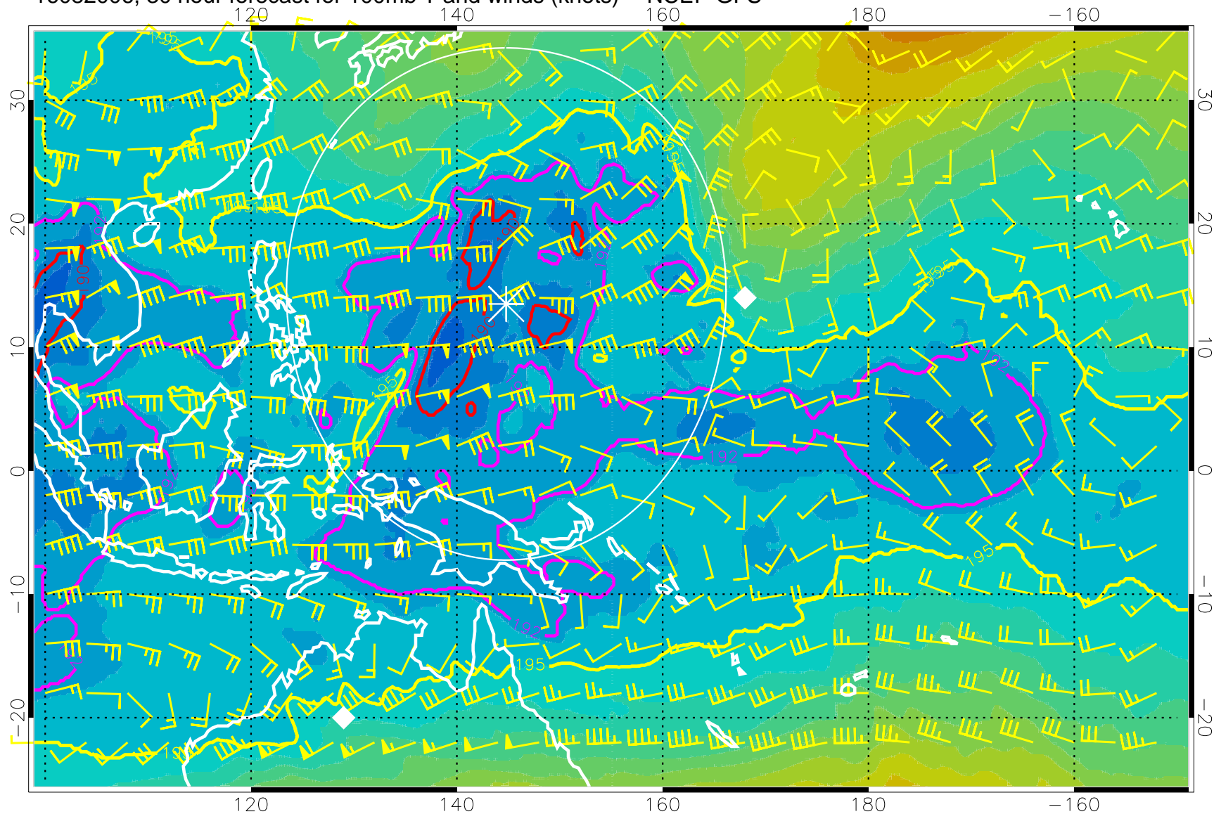
16082006, 30 hour forecast for 100mb T and winds (knots) -- NCEP GFS
