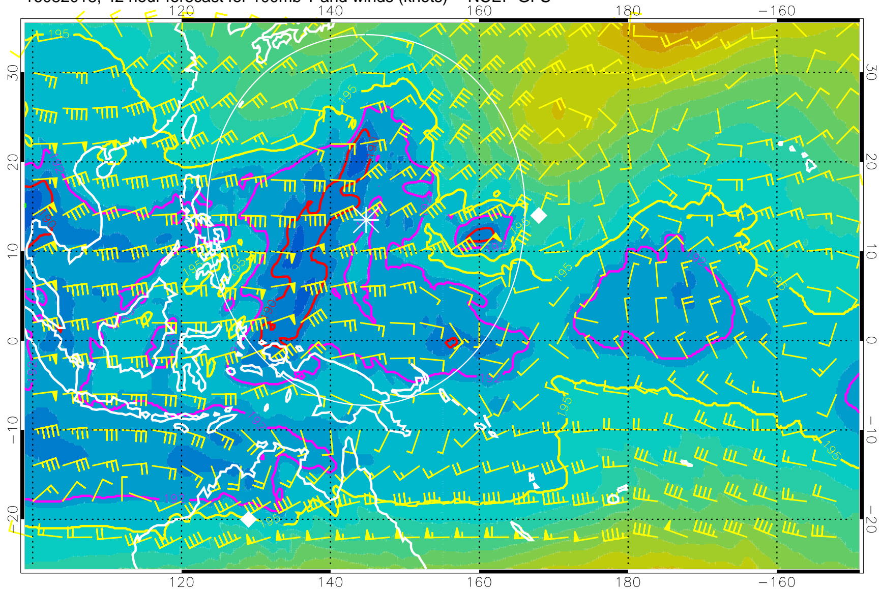
16082018, 42 hour forecast for 100mb T and winds (knots) -- NCEP GFS
