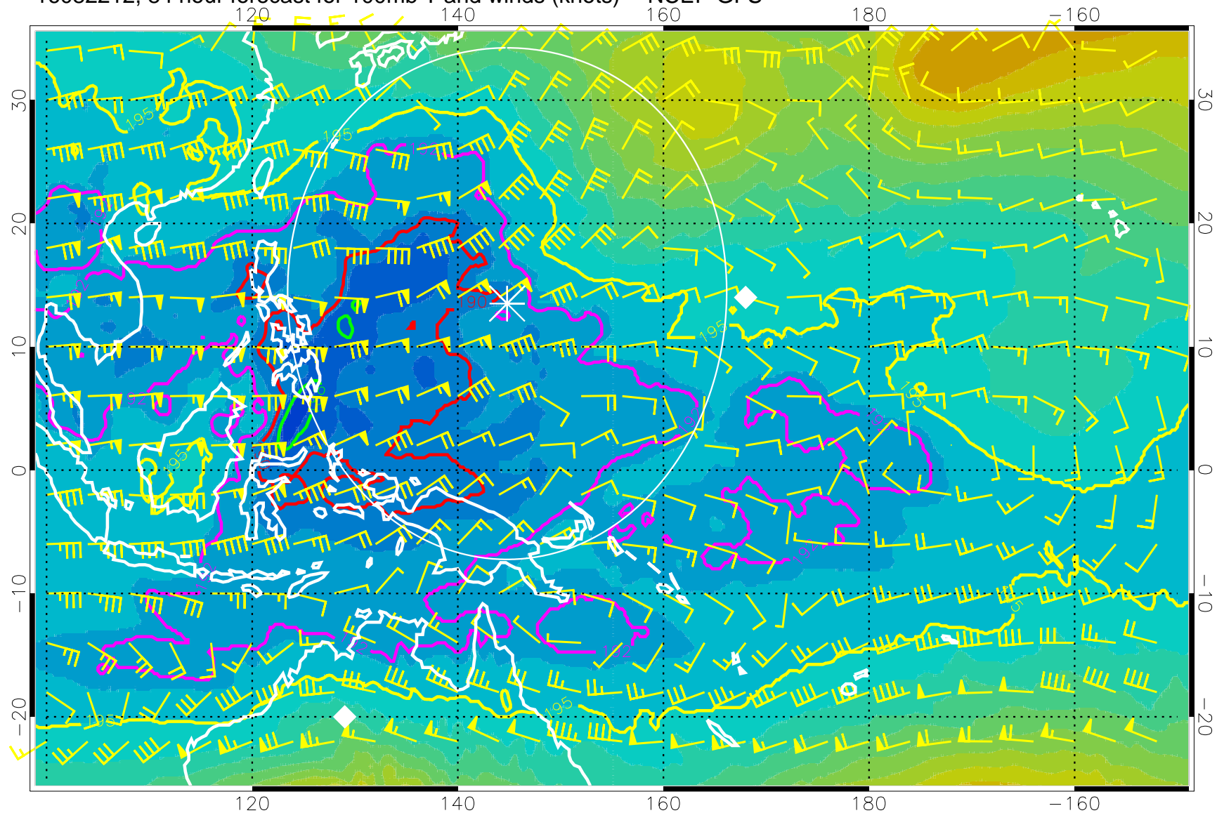
16082212, 84 hour forecast for 100mb T and winds (knots) -- NCEP GFS
