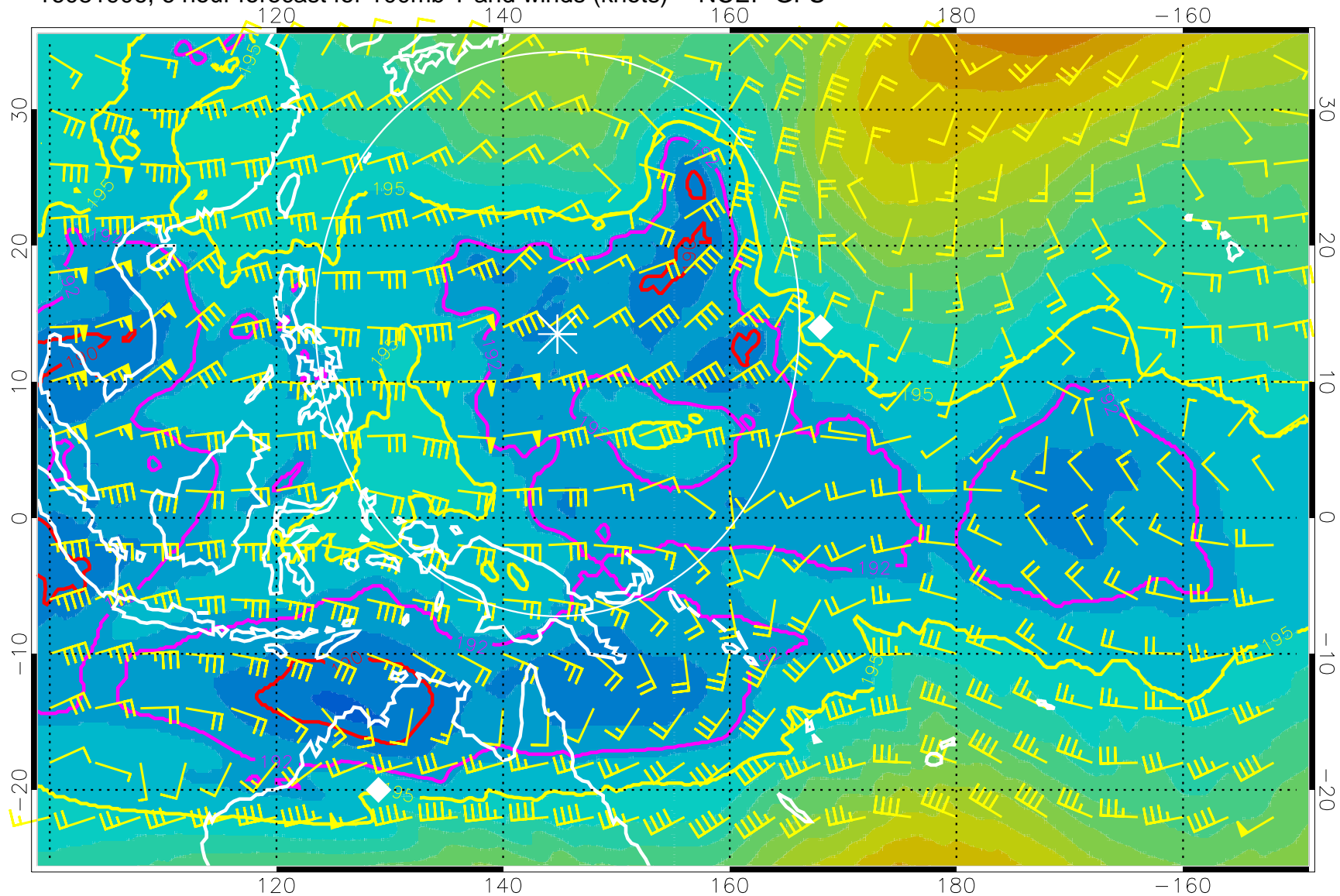
16081906, 6 hour forecast for 100mb T and winds (knots) -- NCEP GFS
