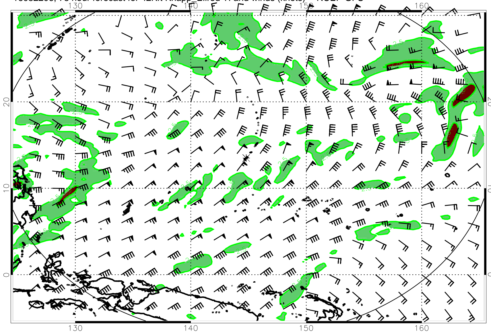
16082206, 78 hour forecast for 42Kft Knapp_Ellrod TI and winds (knots) -- NCEP GFS
