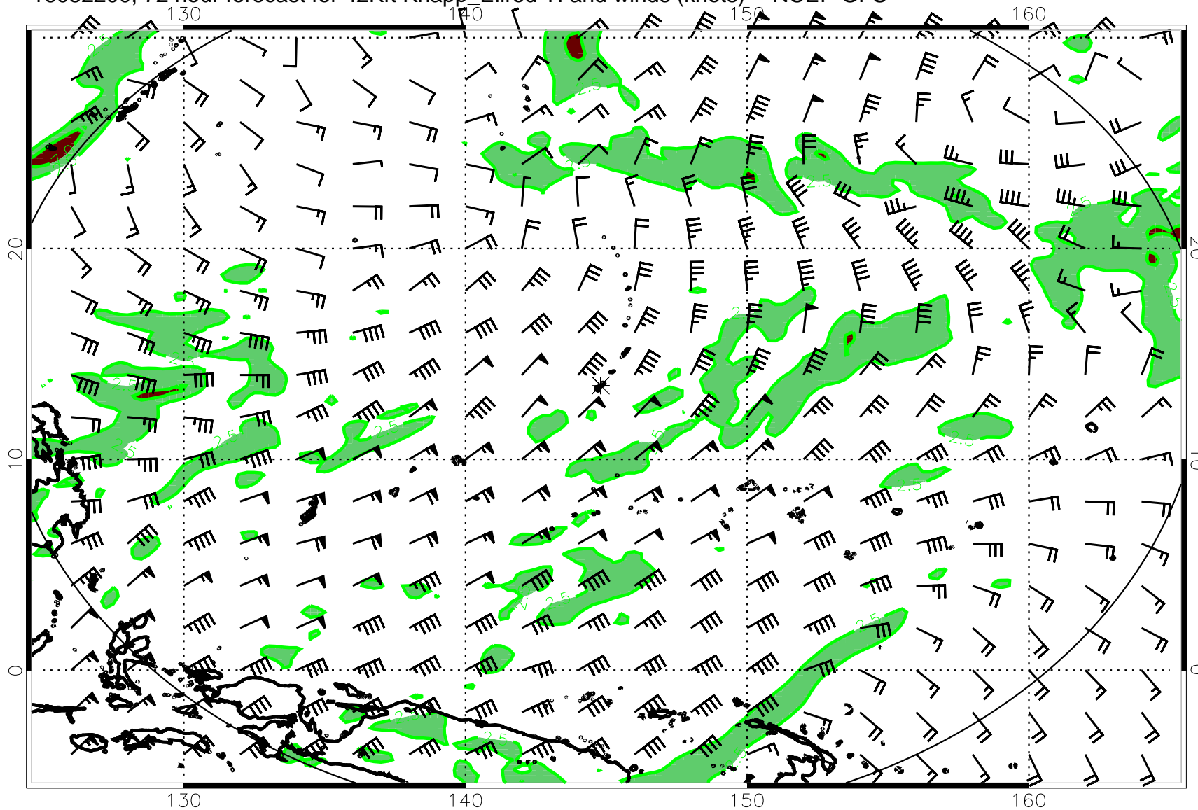
16082200, 72 hour forecast for 42Kft Knapp_Ellrod TI and winds (knots) -- NCEP GFS
