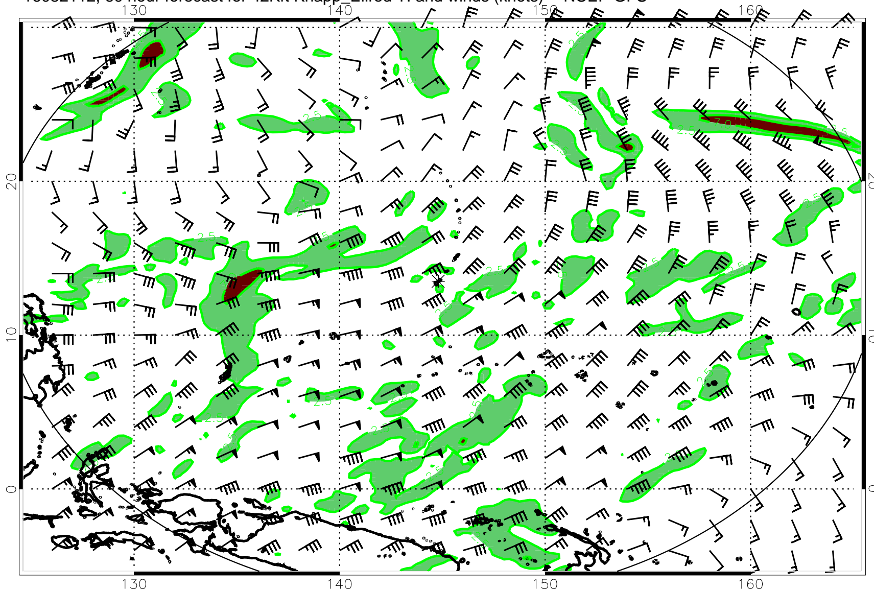
16082112, 60 hour forecast for 42Kft Knapp_Ellrod TI and winds (knots) -- NCEP GFS
