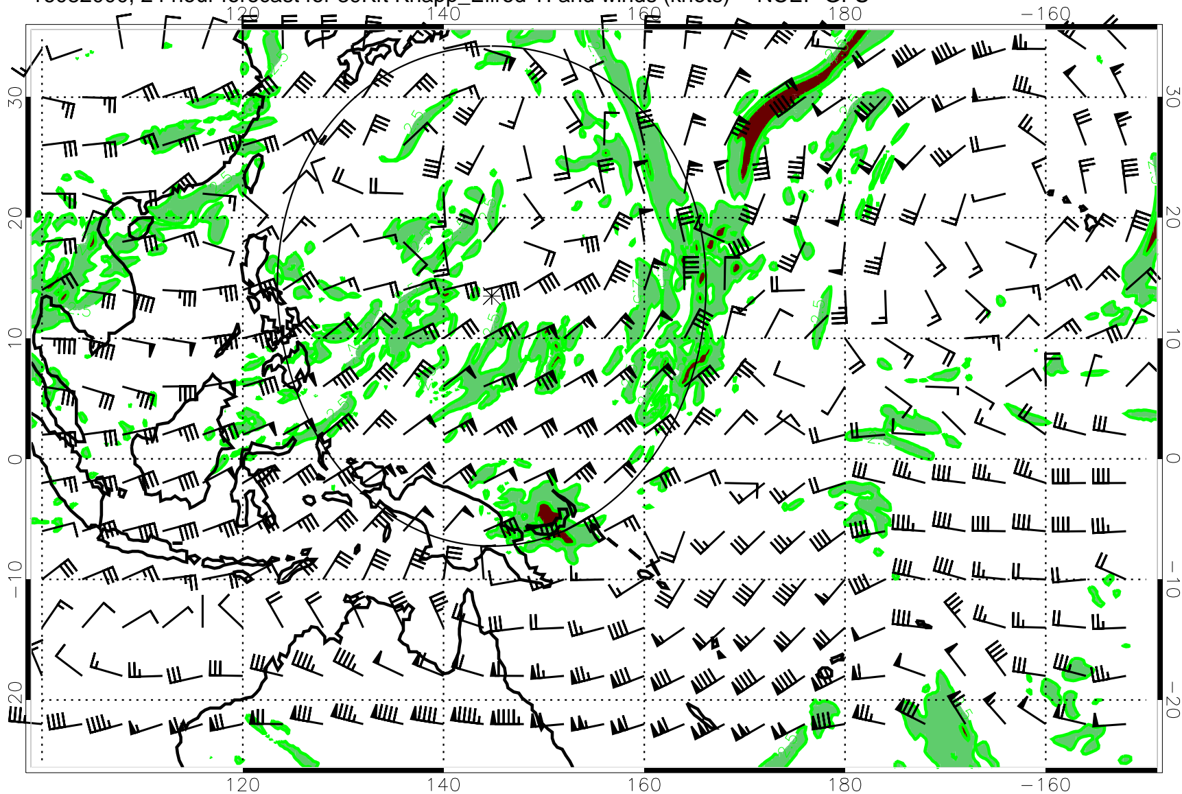
16082000, 24 hour forecast for 39Kft Knapp_Ellrod TI and winds (knots) -- NCEP GFS
