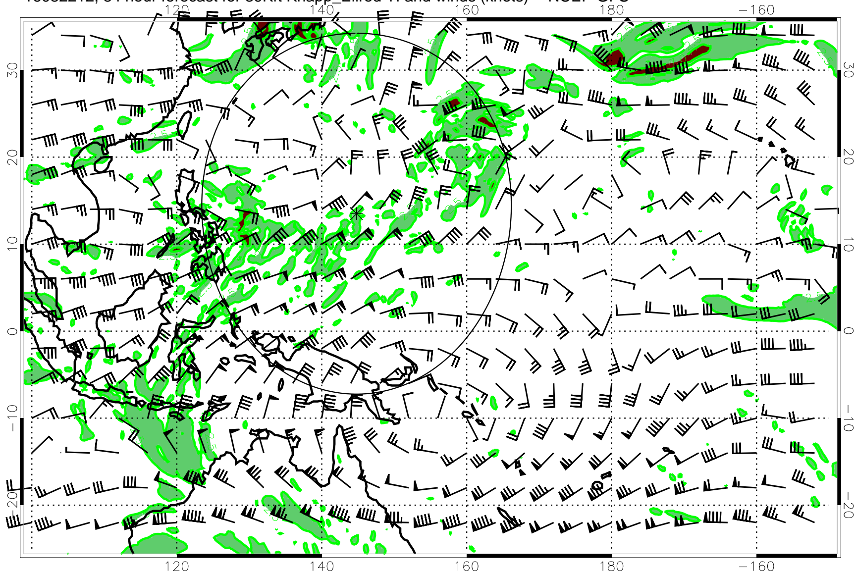
16082212, 84 hour forecast for 39Kft Knapp_Ellrod TI and winds (knots) -- NCEP GFS
