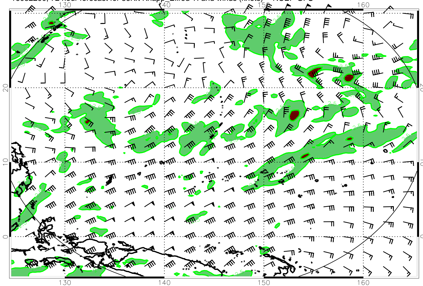
16082200, 72 hour forecast for 36Kft Knapp_Ellrod TI and winds (knots) -- NCEP GFS
