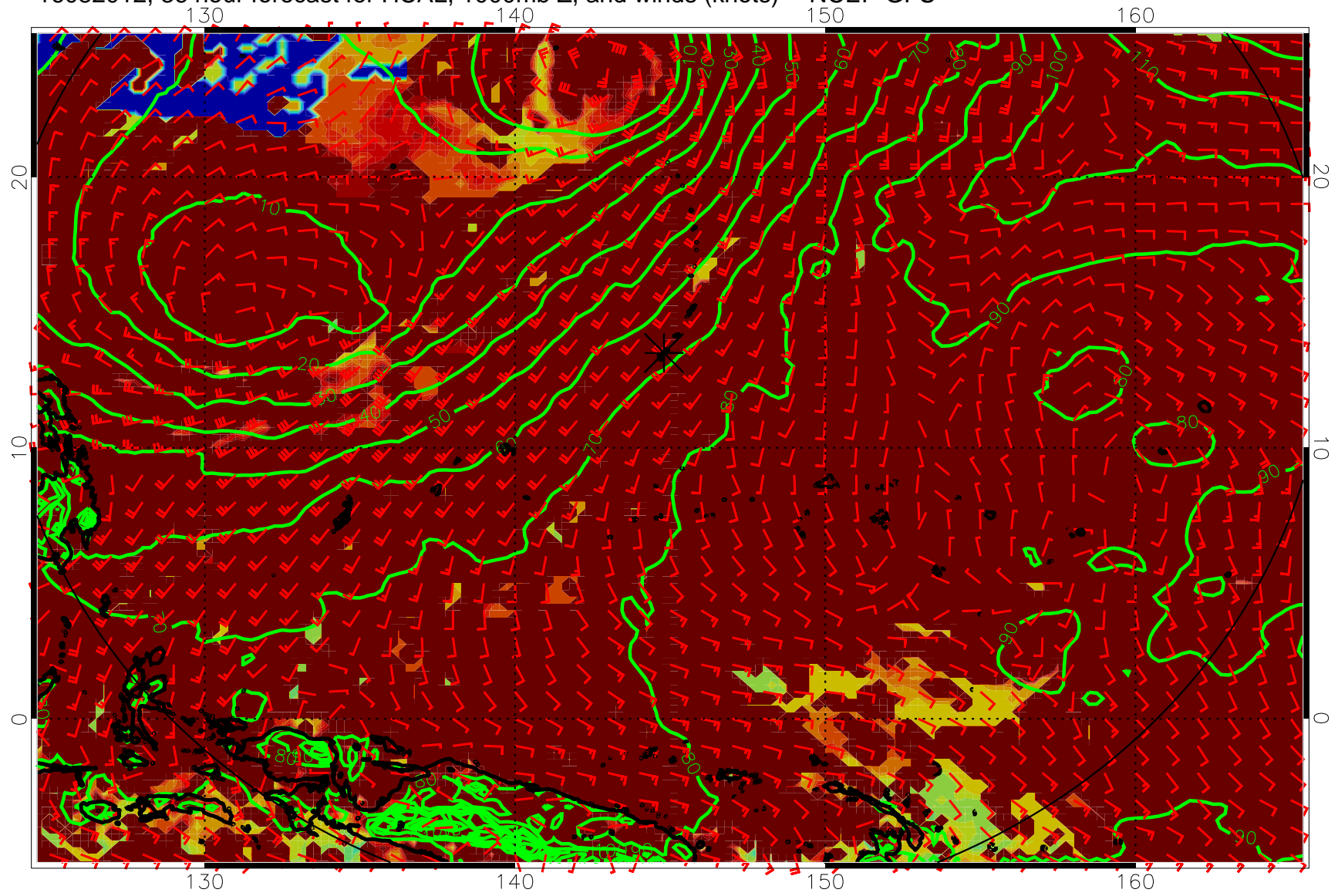
16082012, 36 hour forecast for HCAL, 1000mb Z, and winds (knots) -- NCEP GFS
