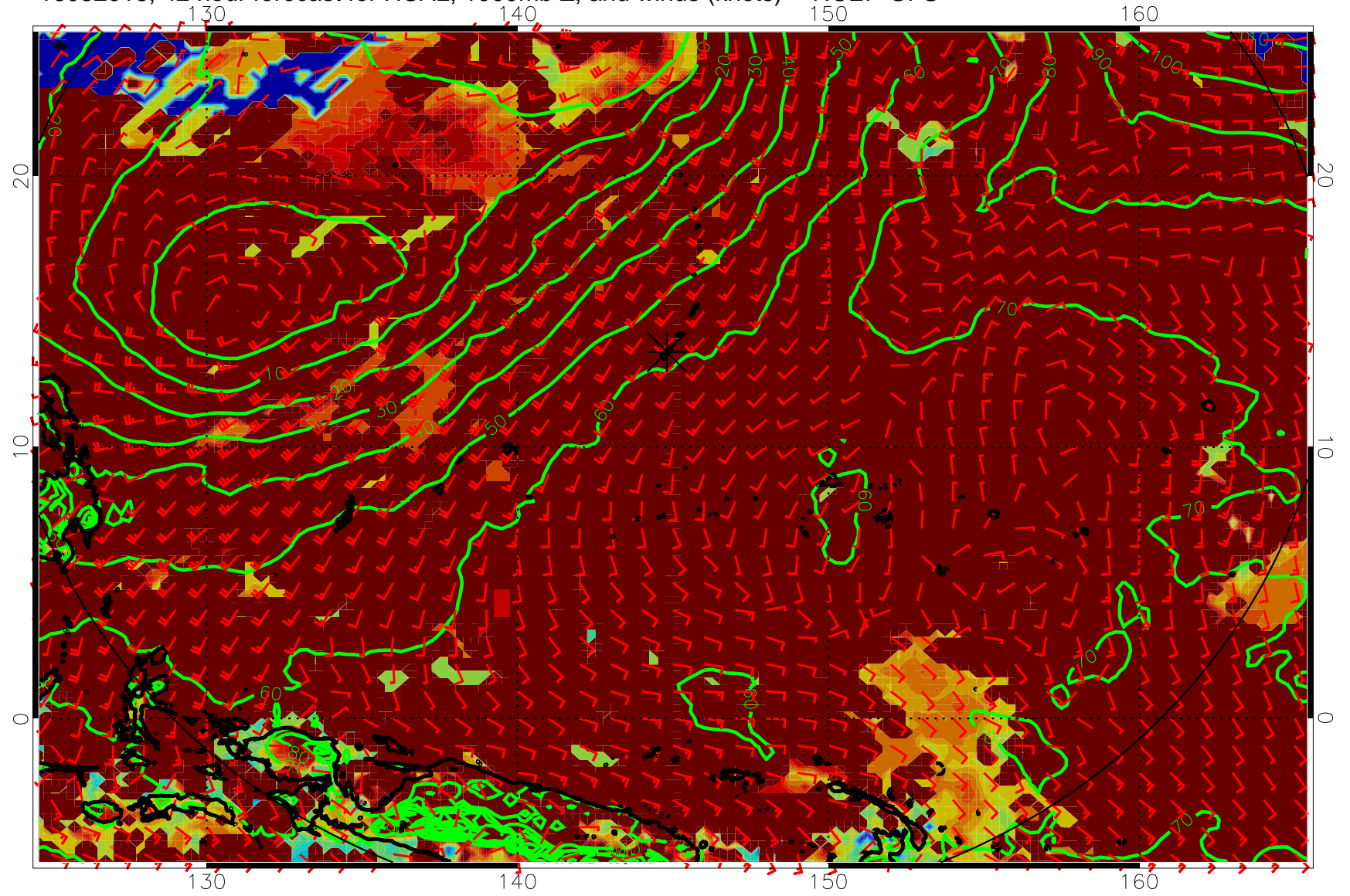
16082018, 42 hour forecast for HCAL, 1000mb Z, and winds (knots) -- NCEP GFS
