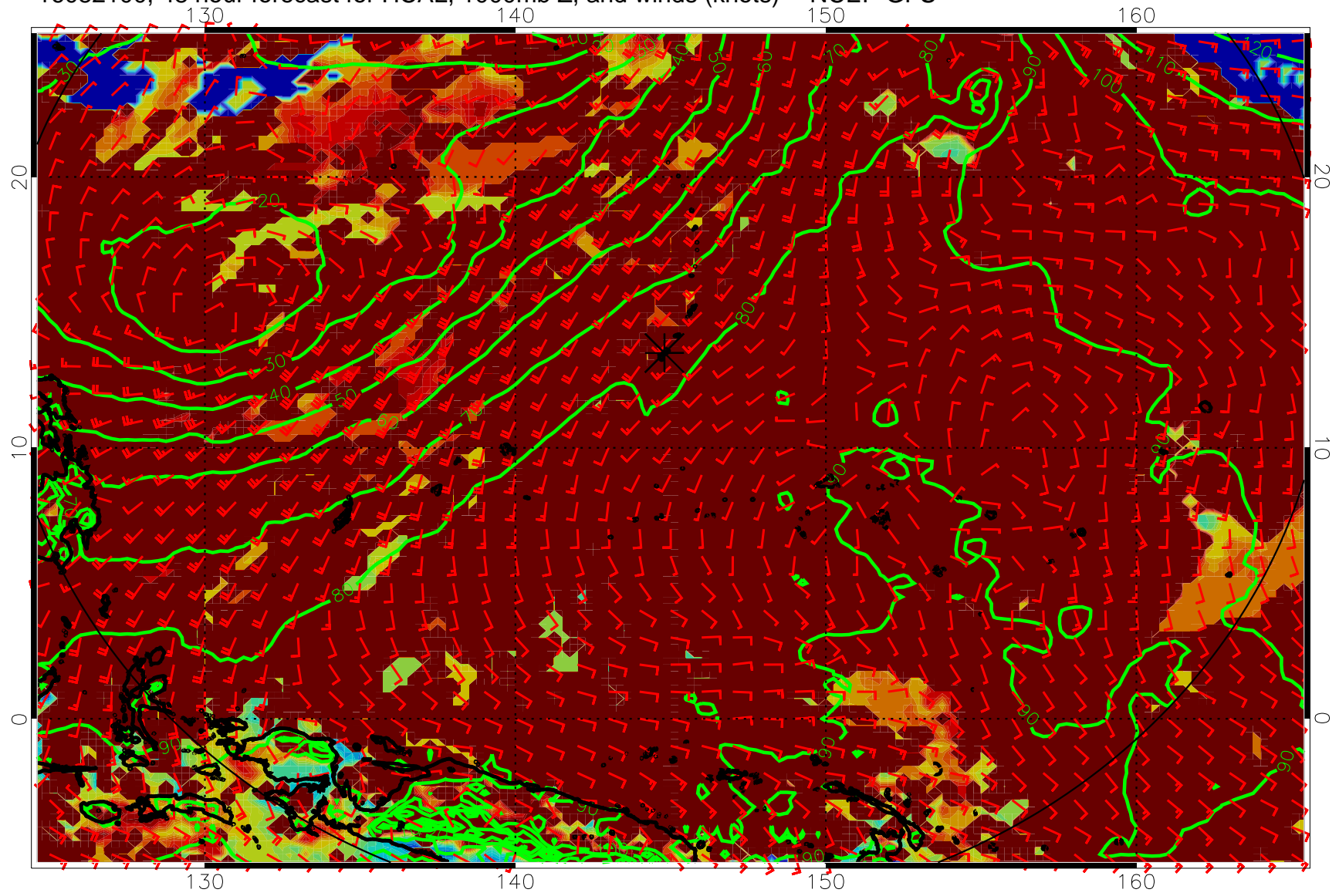
16082100, 48 hour forecast for HCAL, 1000mb Z, and winds (knots) -- NCEP GFS
