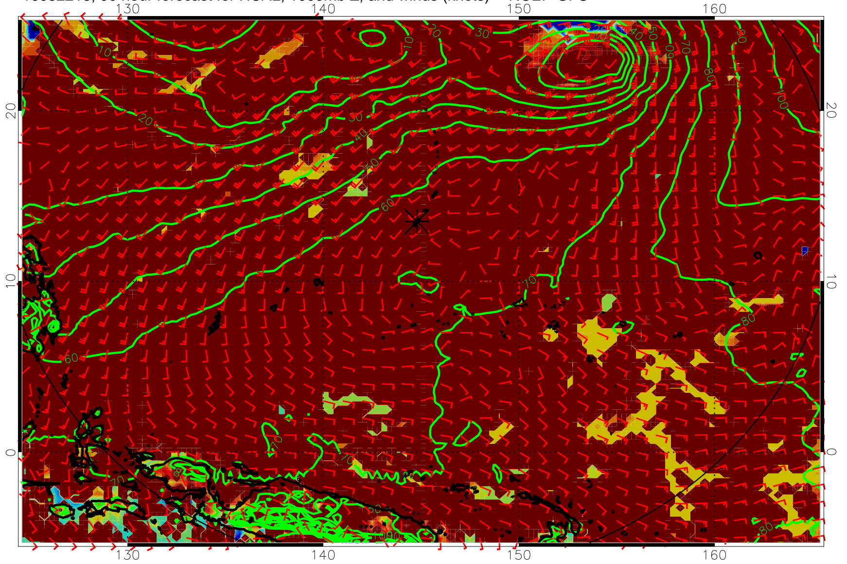
16082218, 90 hour forecast for HCAL, 1000mb Z, and winds (knots) -- NCEP GFS
