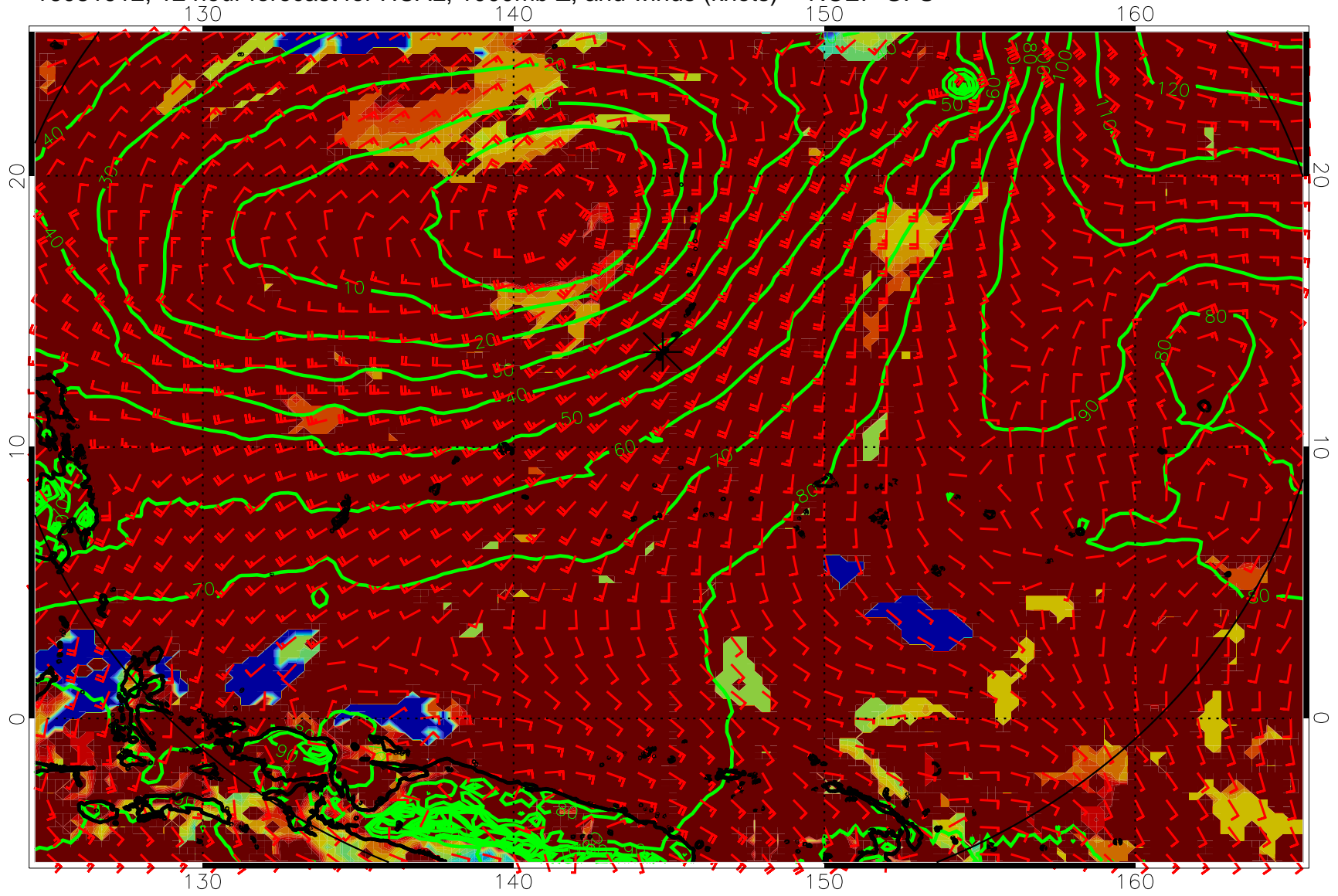
16081912, 12 hour forecast for HCAL, 1000mb Z, and winds (knots) -- NCEP GFS
