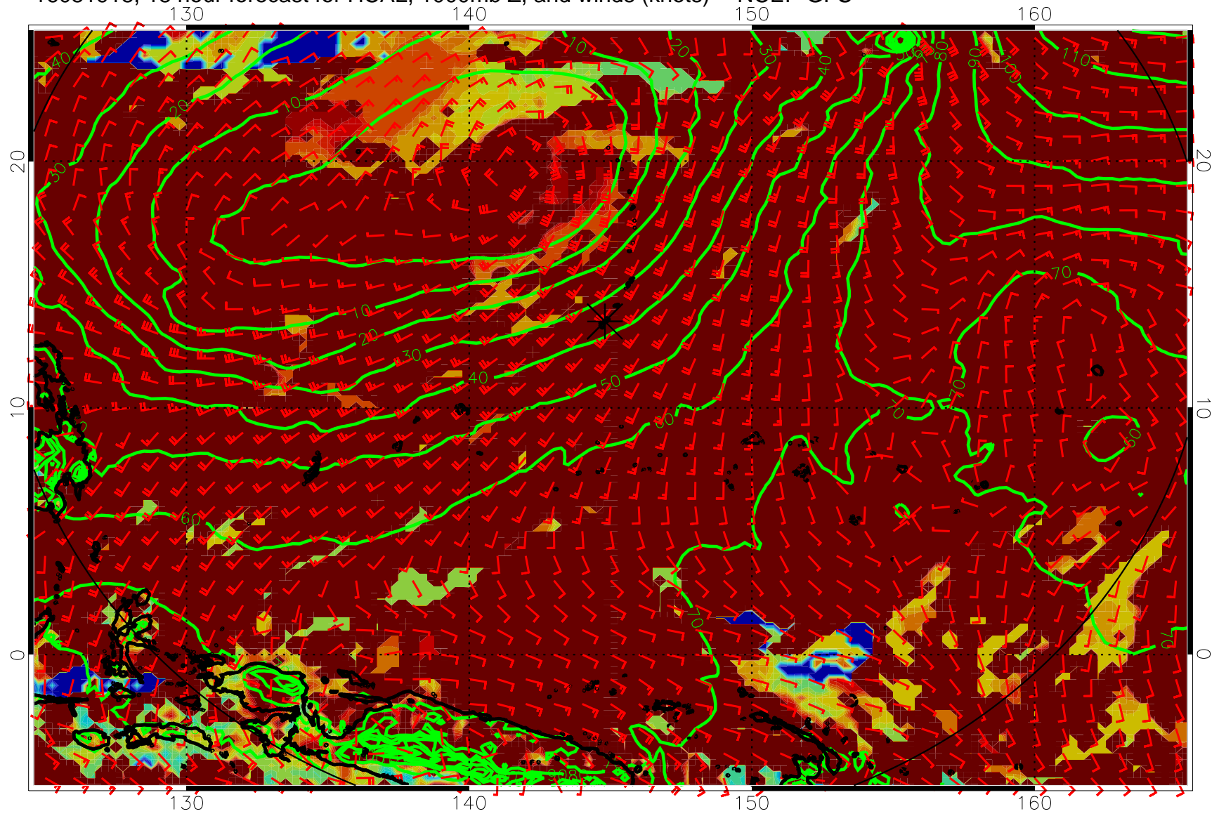
16081918, 18 hour forecast for HCAL, 1000mb Z, and winds (knots) -- NCEP GFS
