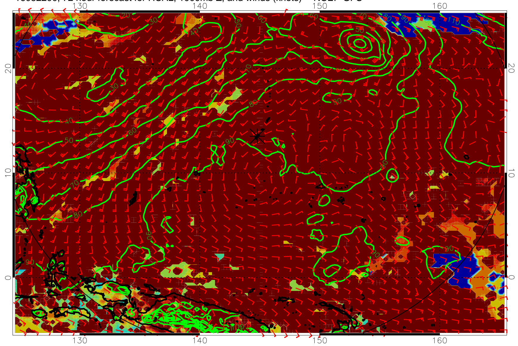
16082200, 72 hour forecast for HCAL, 1000mb Z, and winds (knots) -- NCEP GFS
