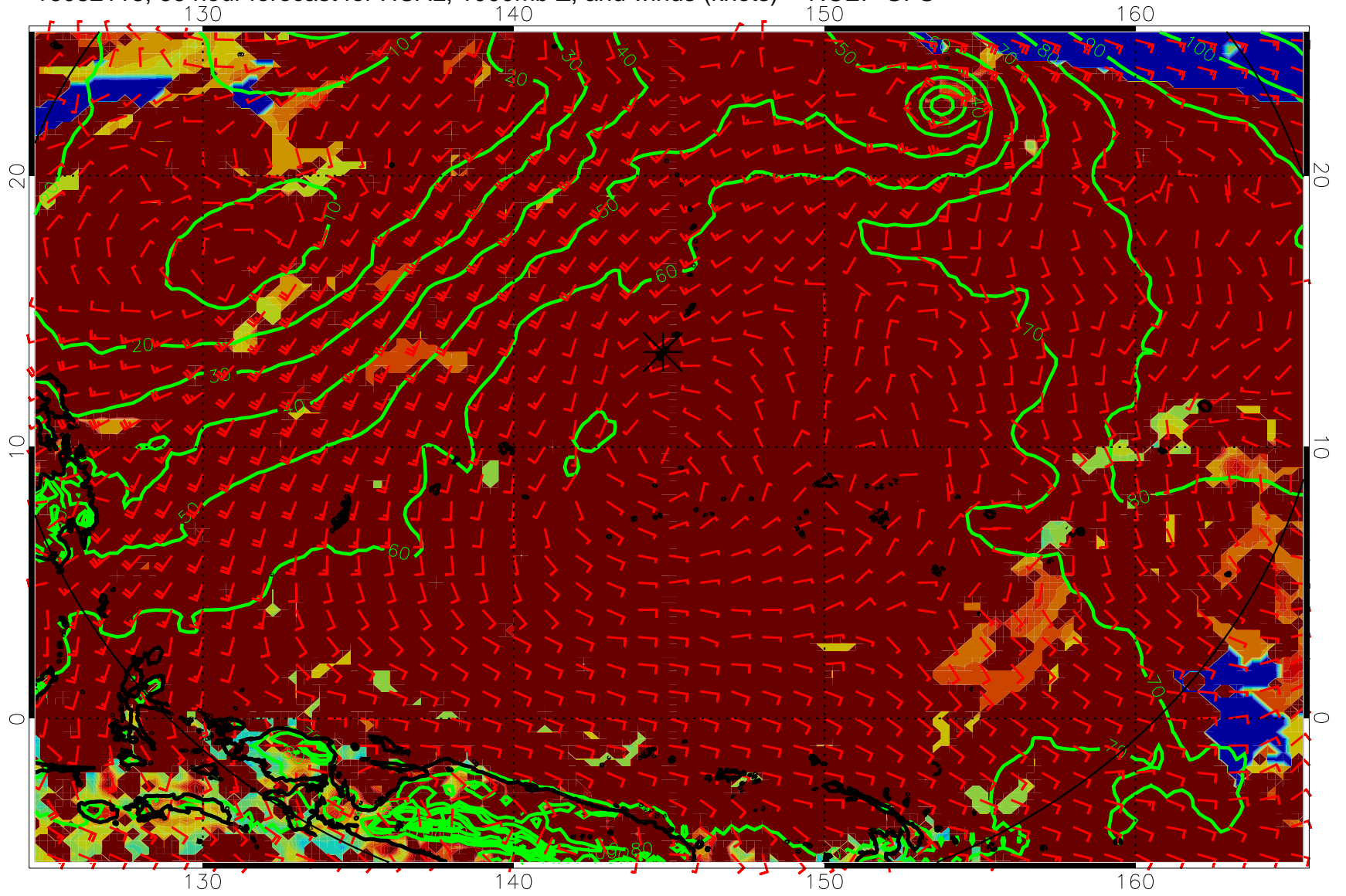
16082118, 66 hour forecast for HCAL, 1000mb Z, and winds (knots) -- NCEP GFS
