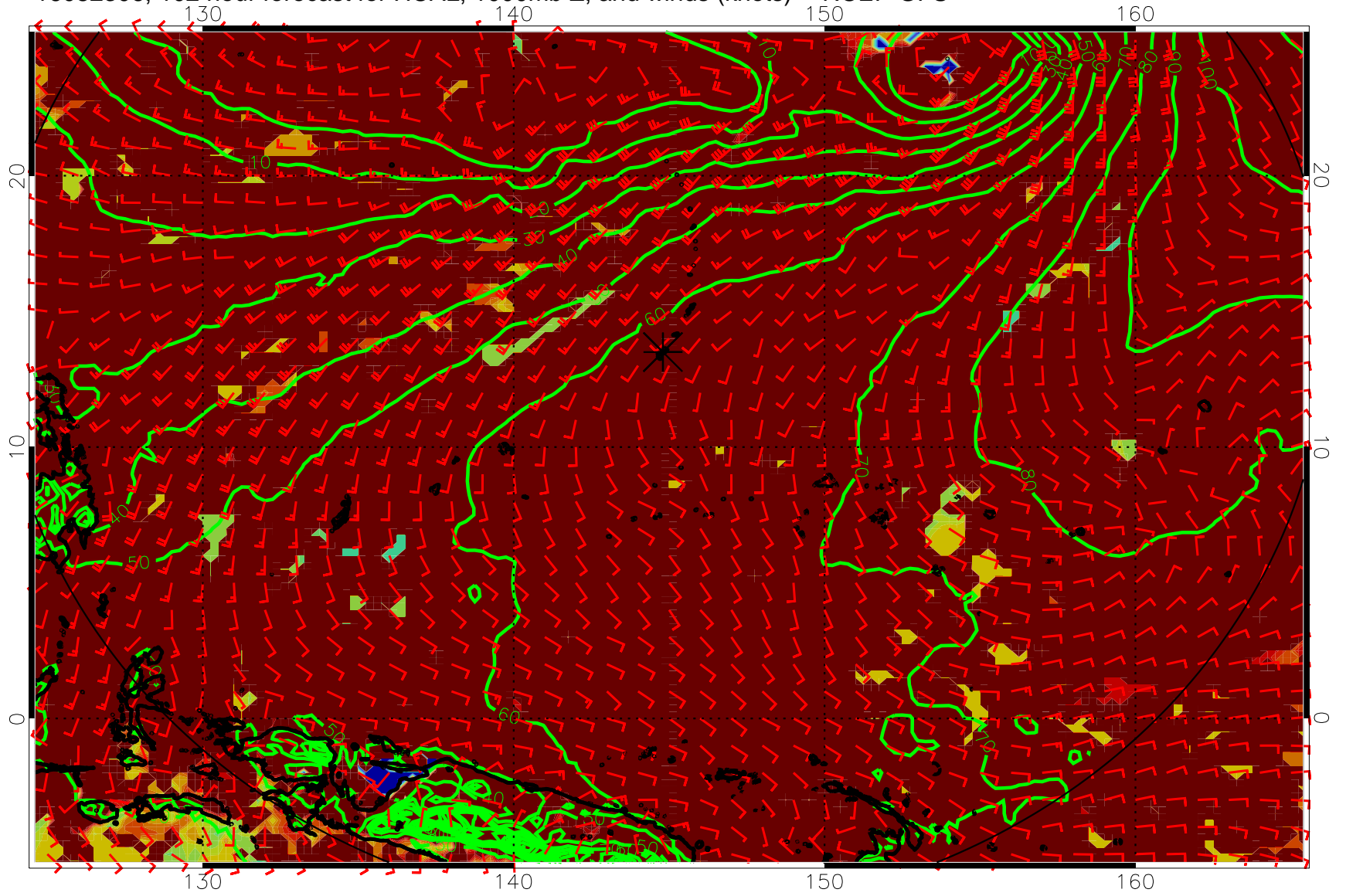
16082306, 102 hour forecast for HCAL, 1000mb Z, and winds (knots) -- NCEP GFS
