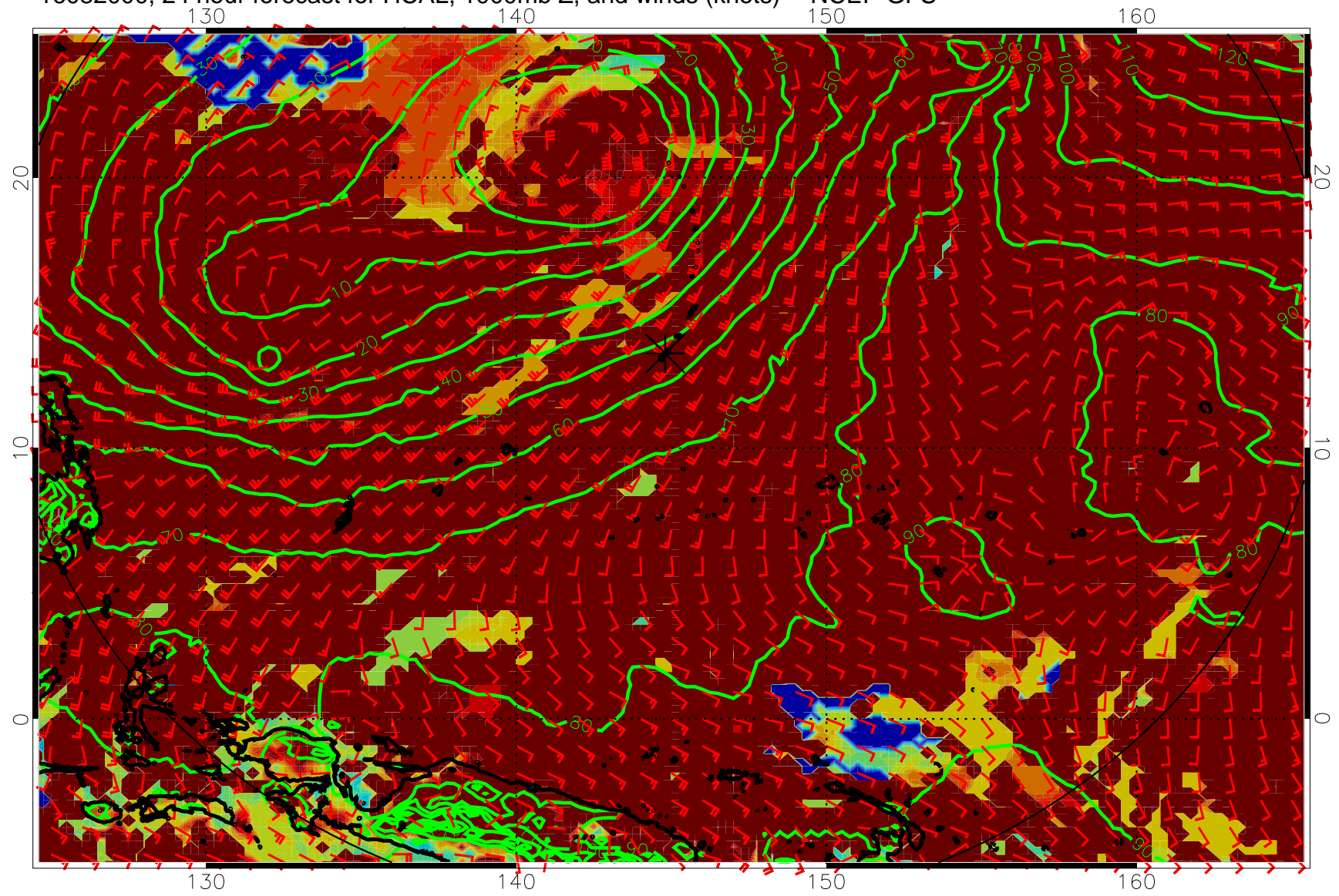
16082000, 24 hour forecast for HCAL, 1000mb Z, and winds (knots) -- NCEP GFS
