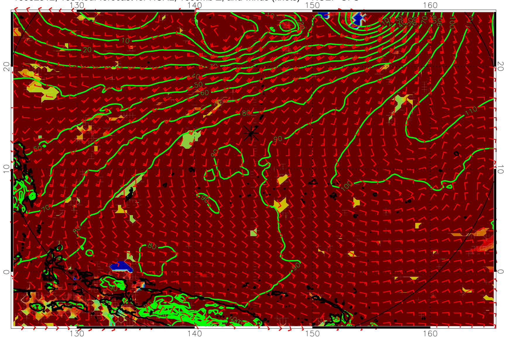
16082312, 108 hour forecast for HCAL, 1000mb Z, and winds (knots) -- NCEP GFS
