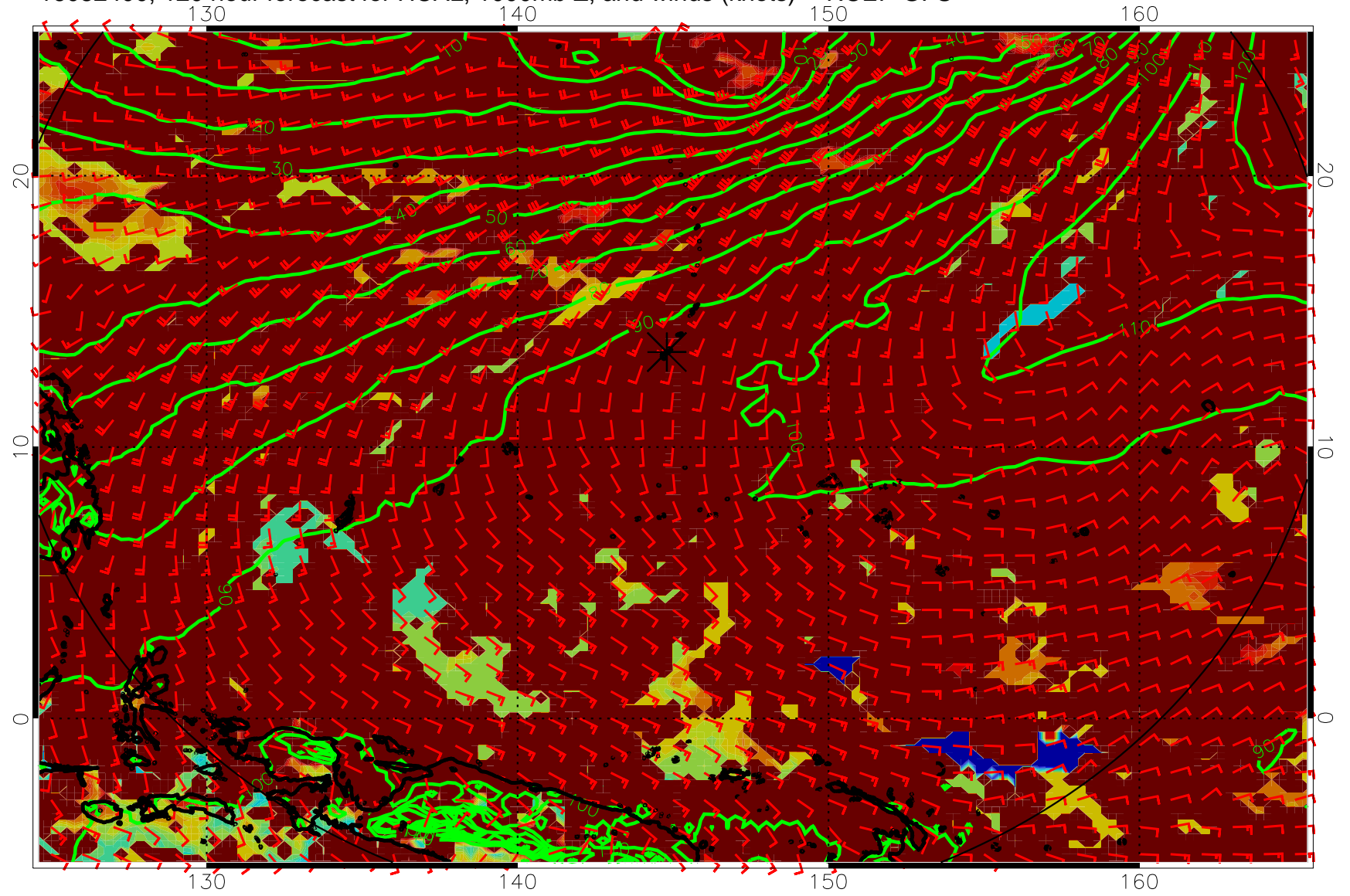
16082400, 120 hour forecast for HCAL, 1000mb Z, and winds (knots) -- NCEP GFS
