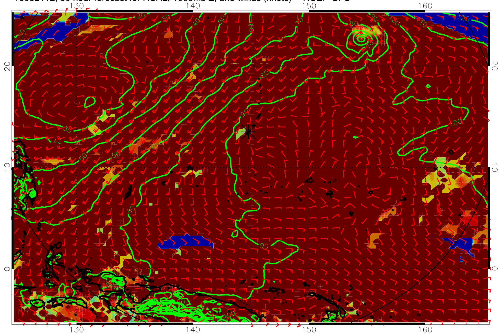
16082112, 60 hour forecast for HCAL, 1000mb Z, and winds (knots) -- NCEP GFS
