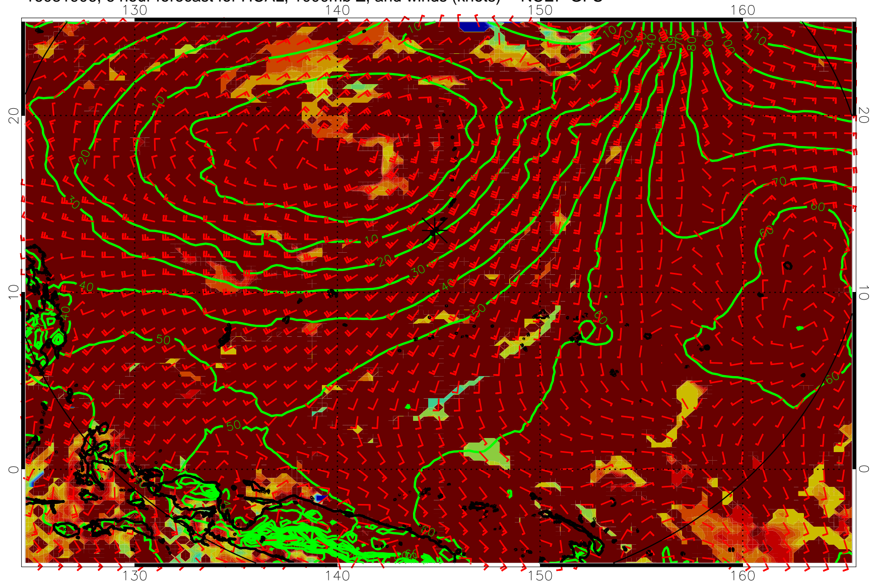
16081906, 6 hour forecast for HCAL, 1000mb Z, and winds (knots) -- NCEP GFS
