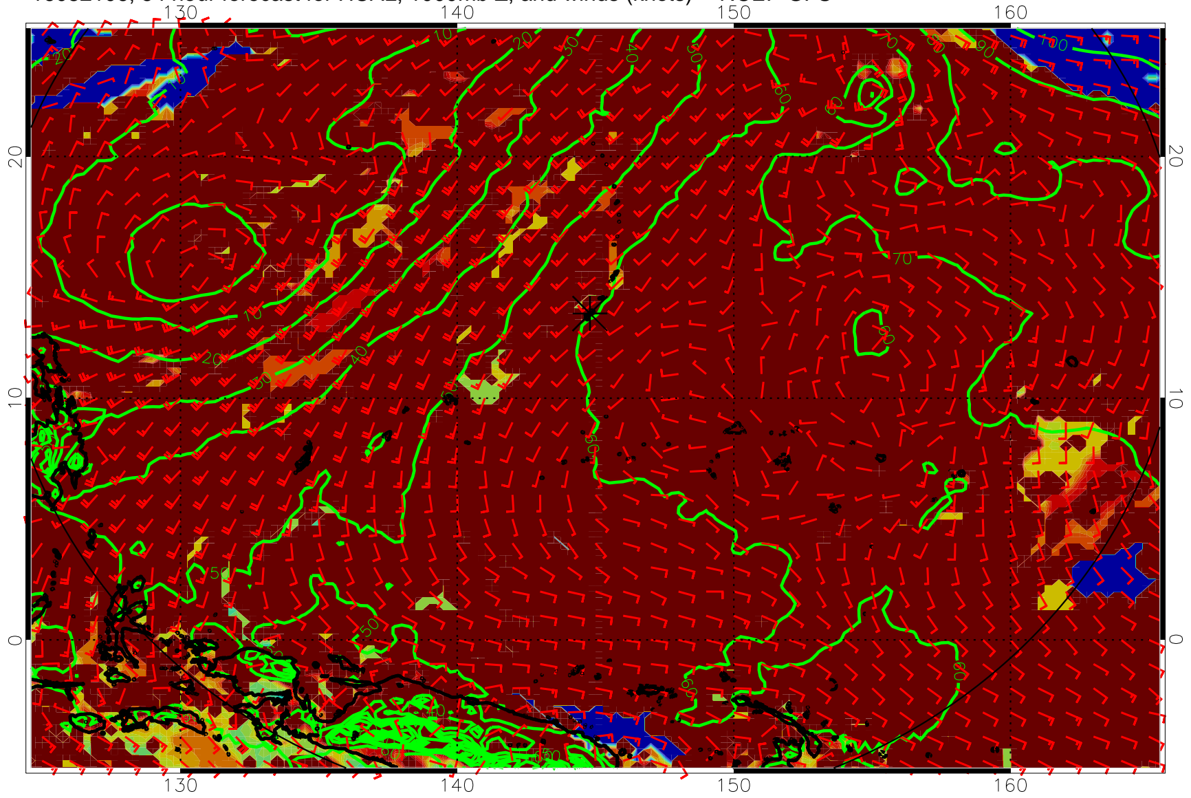
16082106, 54 hour forecast for HCAL, 1000mb Z, and winds (knots) -- NCEP GFS
