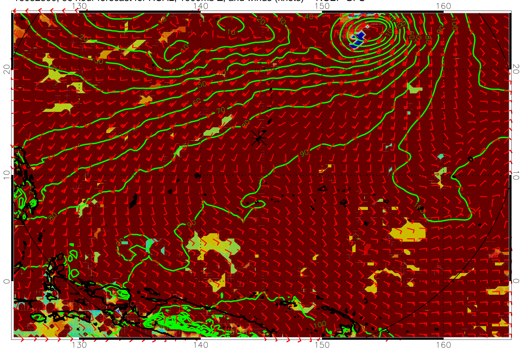
16082300, 96 hour forecast for HCAL, 1000mb Z, and winds (knots) -- NCEP GFS
