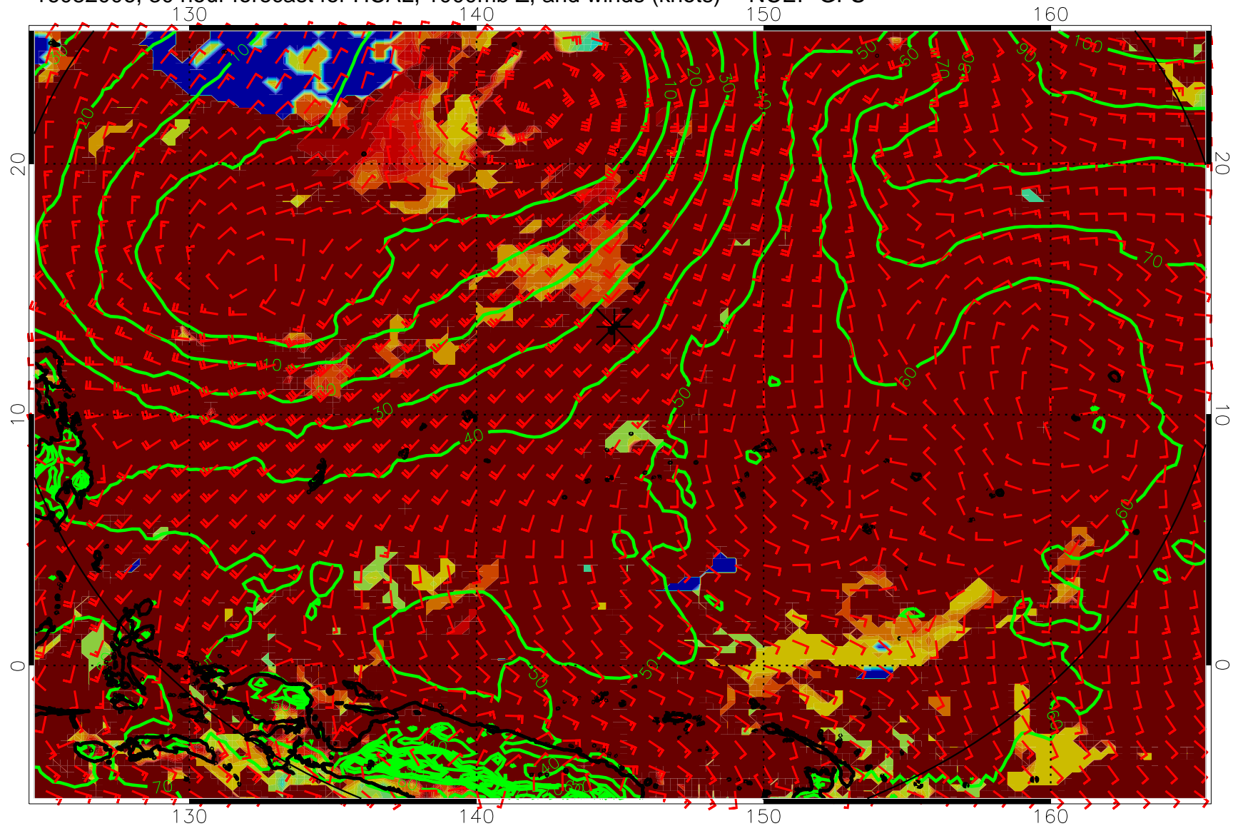
16082006, 30 hour forecast for HCAL, 1000mb Z, and winds (knots) -- NCEP GFS
