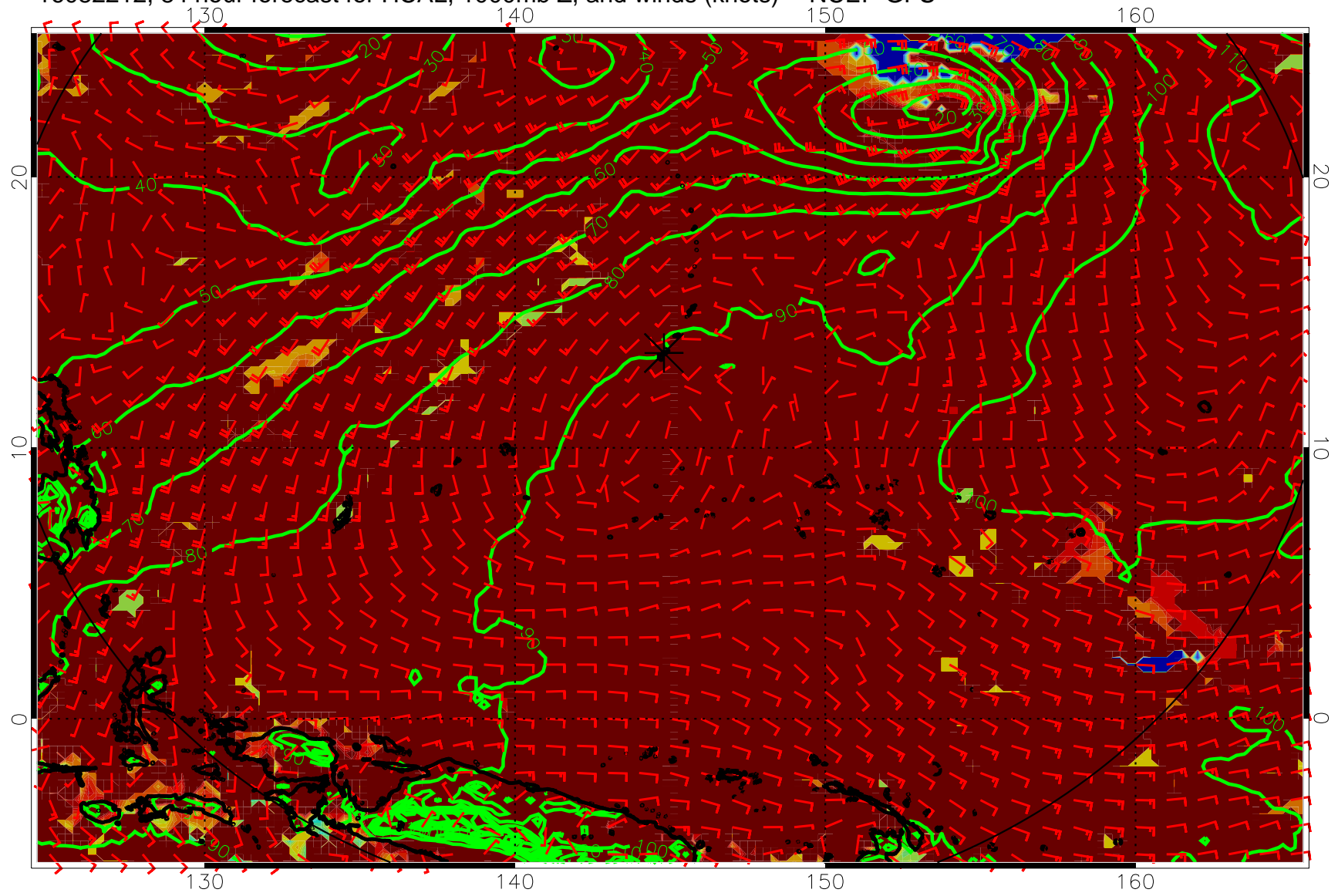
16082212, 84 hour forecast for HCAL, 1000mb Z, and winds (knots) -- NCEP GFS
