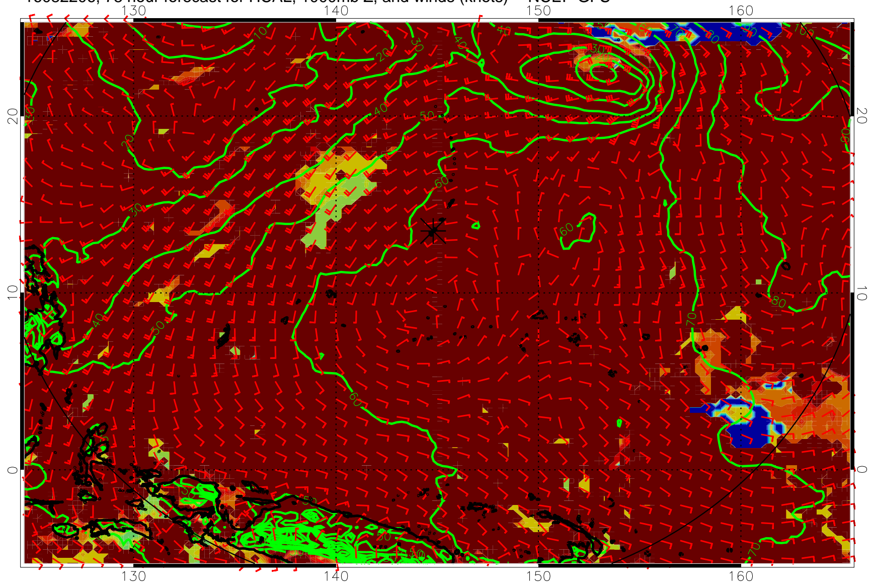
16082206, 78 hour forecast for HCAL, 1000mb Z, and winds (knots) -- NCEP GFS
