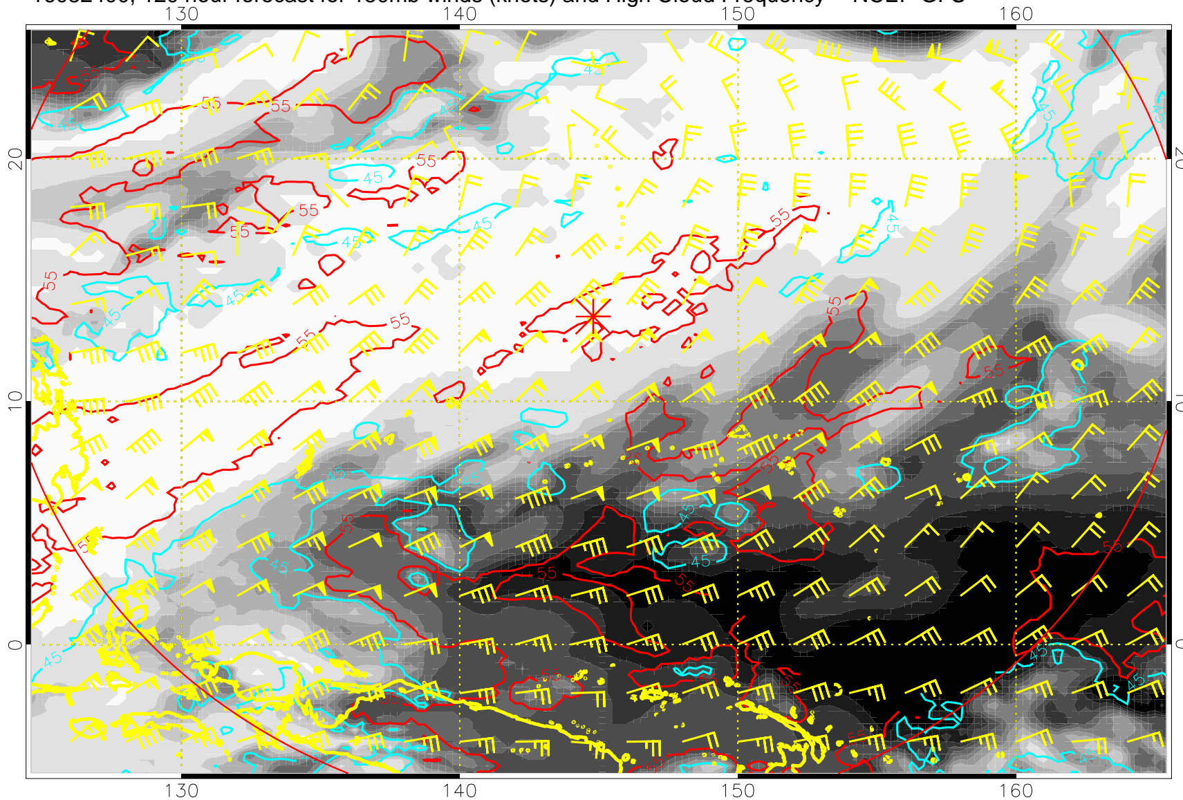
16082400, 120 hour forecast for 150mb winds (knots) and High Cloud Frequency -- NCEP GFS
