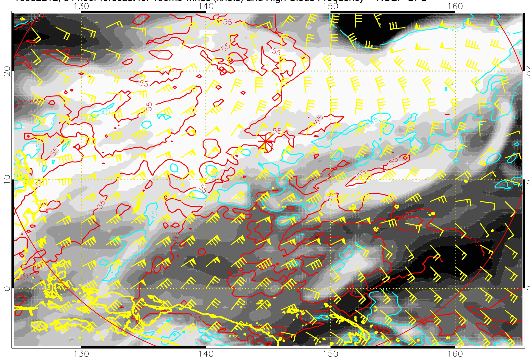
16082212, 84 hour forecast for 150mb winds (knots) and High Cloud Frequency -- NCEP GFS
