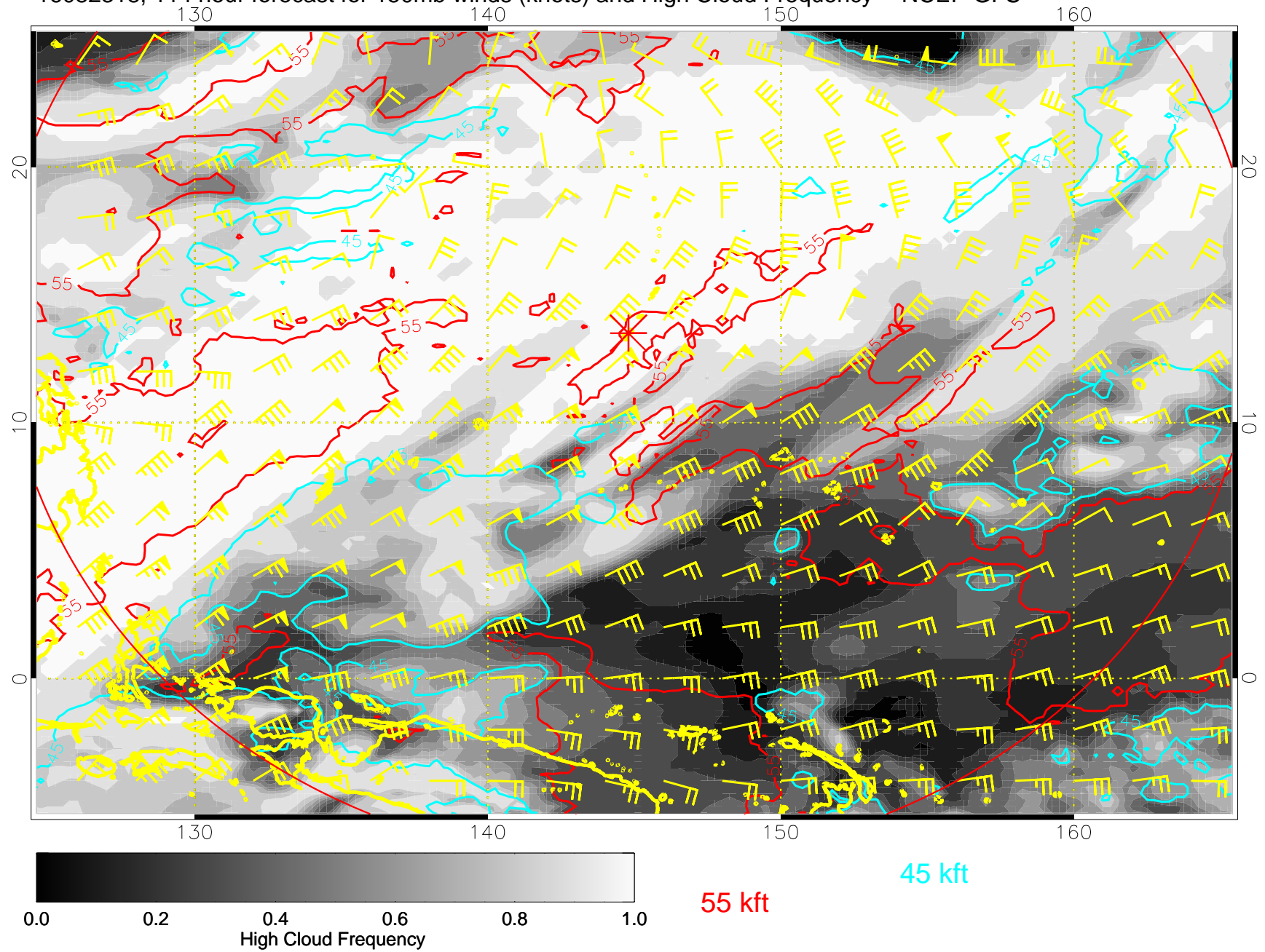
16082318, 114 hour forecast for 150mb winds (knots) and High Cloud Frequency -- NCEP GFS
