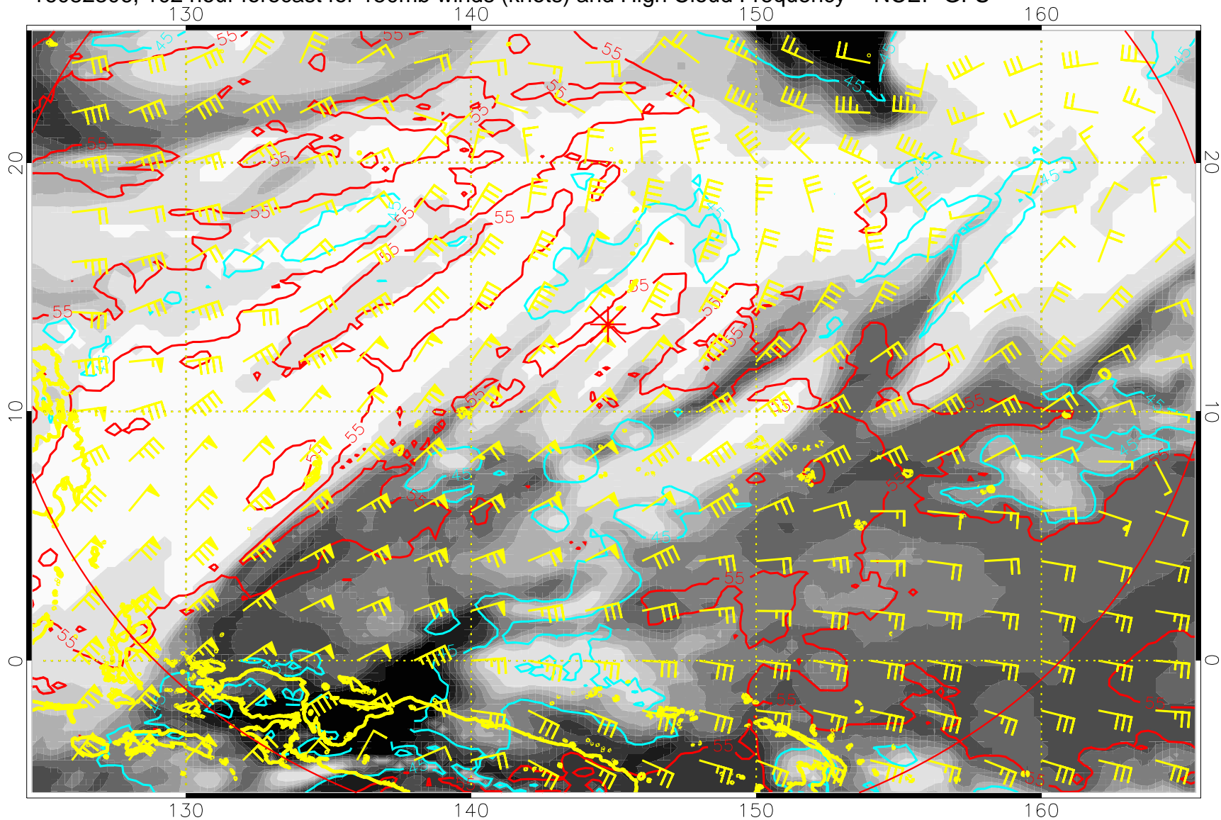
16082306, 102 hour forecast for 150mb winds (knots) and High Cloud Frequency -- NCEP GFS
