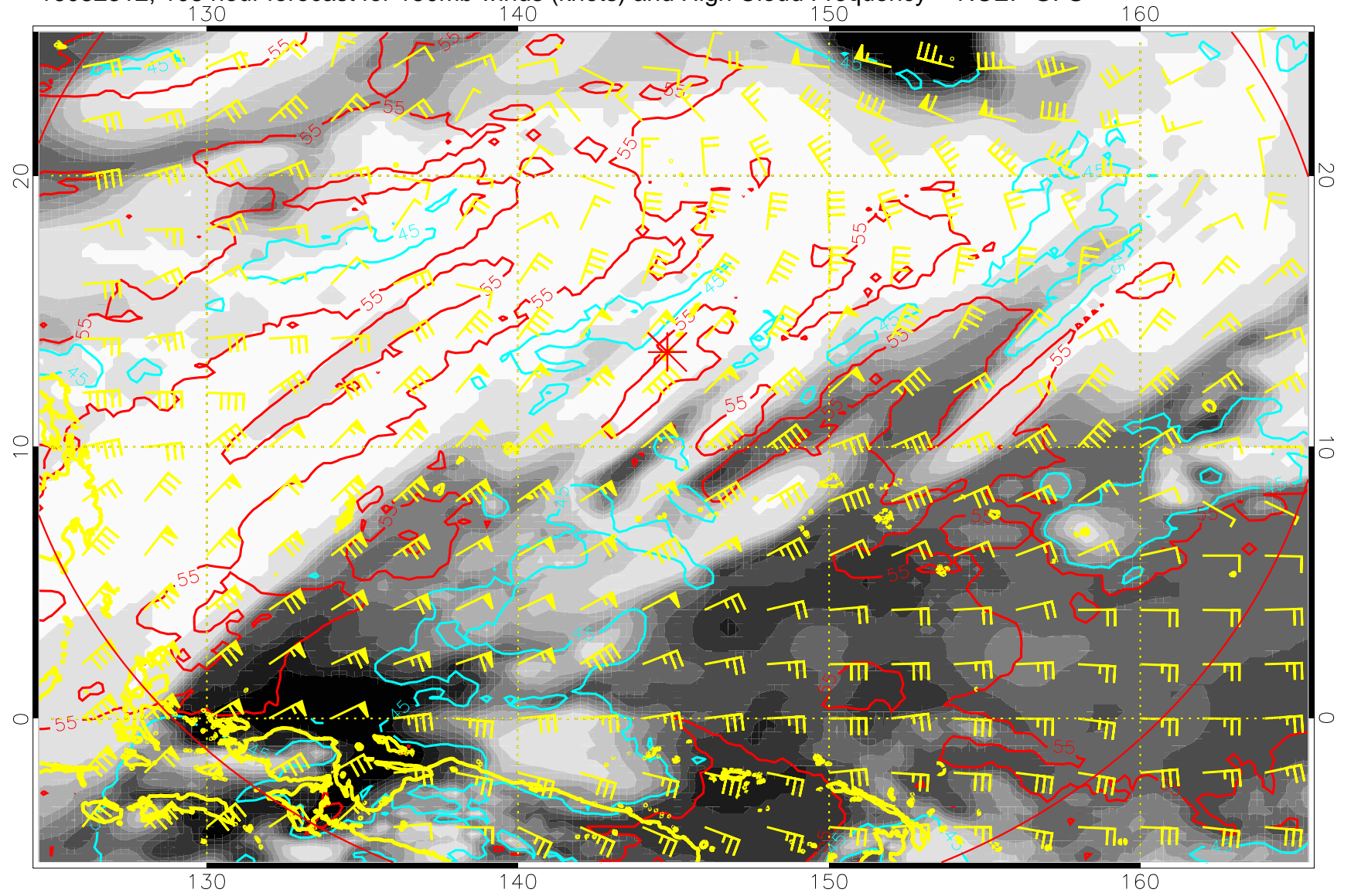
16082312, 108 hour forecast for 150mb winds (knots) and High Cloud Frequency -- NCEP GFS
