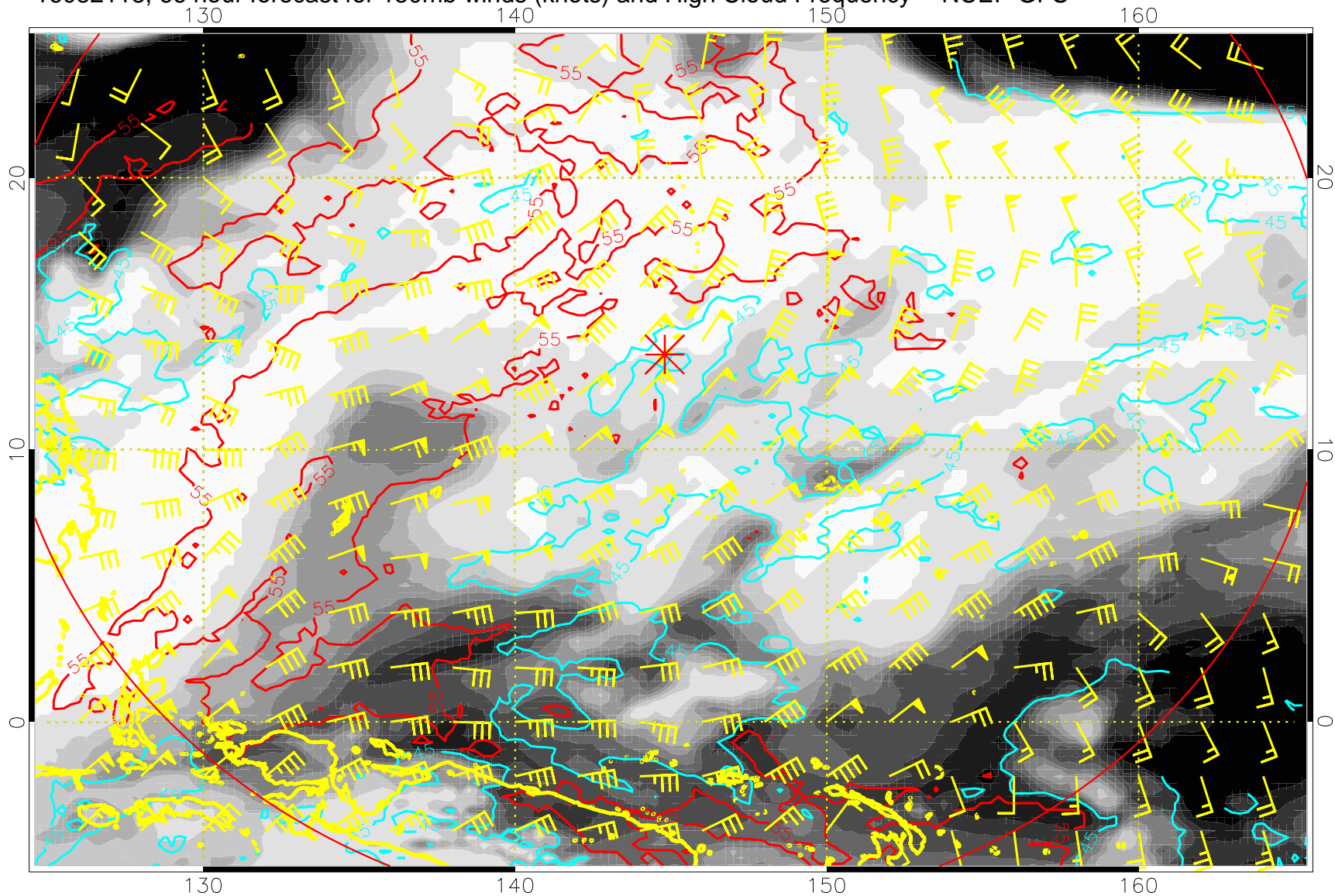
16082118, 66 hour forecast for 150mb winds (knots) and High Cloud Frequency -- NCEP GFS
