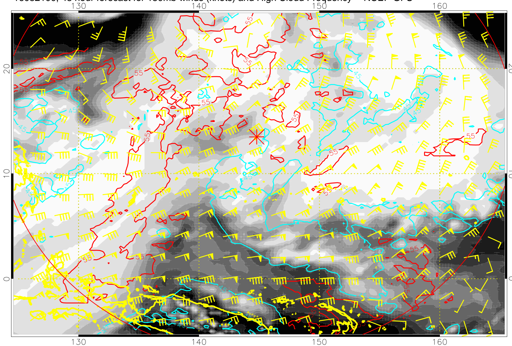
16082100, 48 hour forecast for 150mb winds (knots) and High Cloud Frequency -- NCEP GFS
