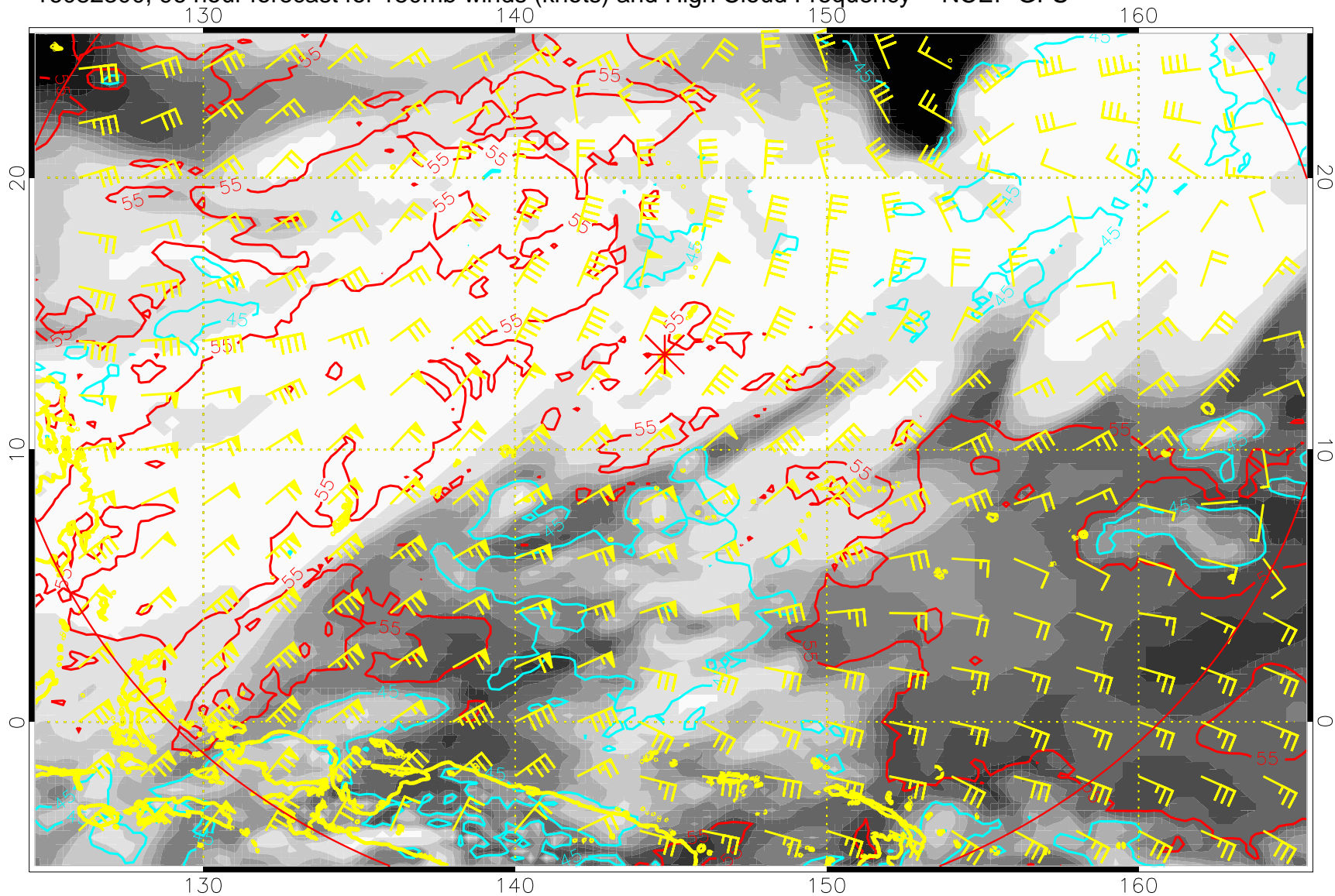
16082300, 96 hour forecast for 150mb winds (knots) and High Cloud Frequency -- NCEP GFS
