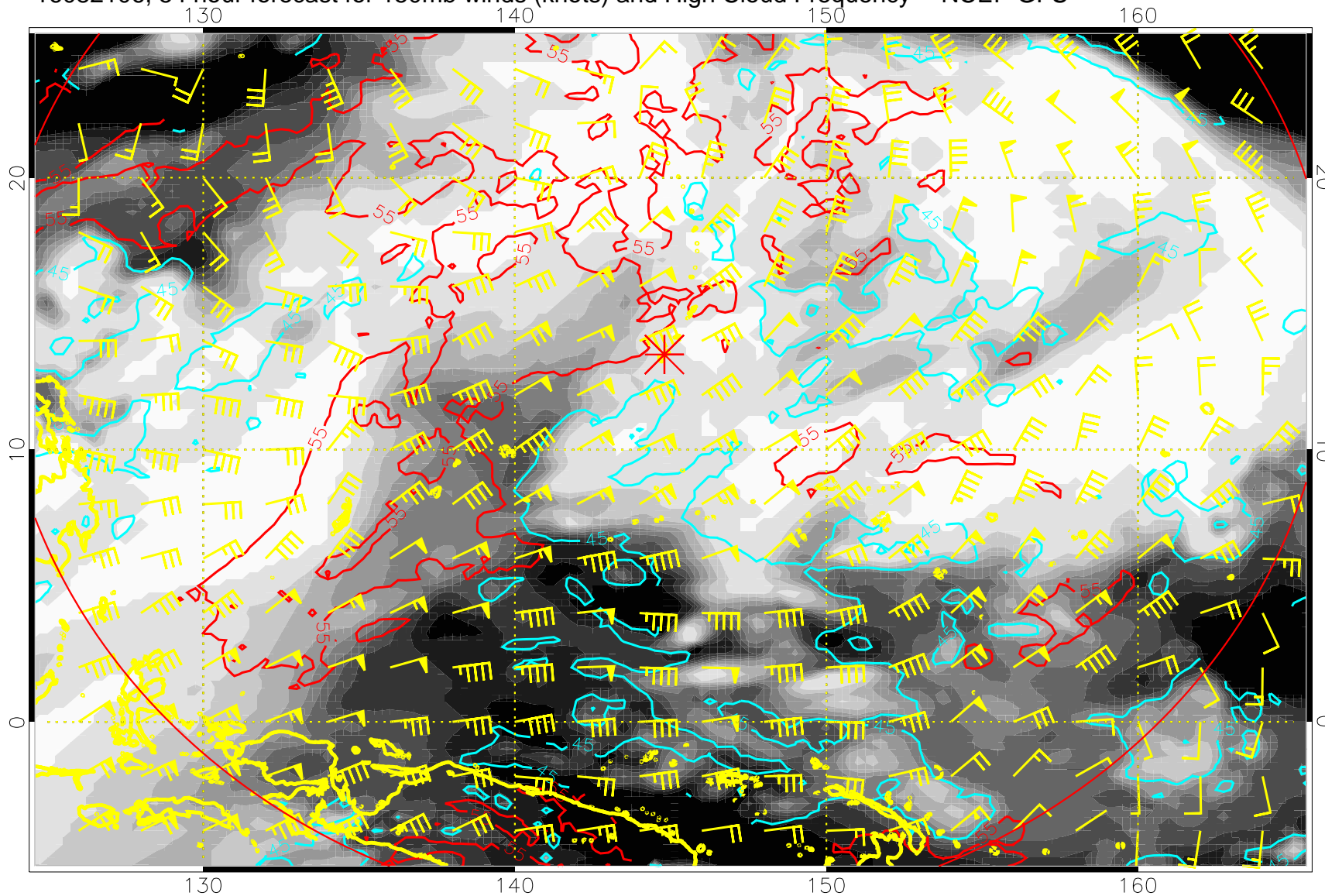
16082106, 54 hour forecast for 150mb winds (knots) and High Cloud Frequency -- NCEP GFS
