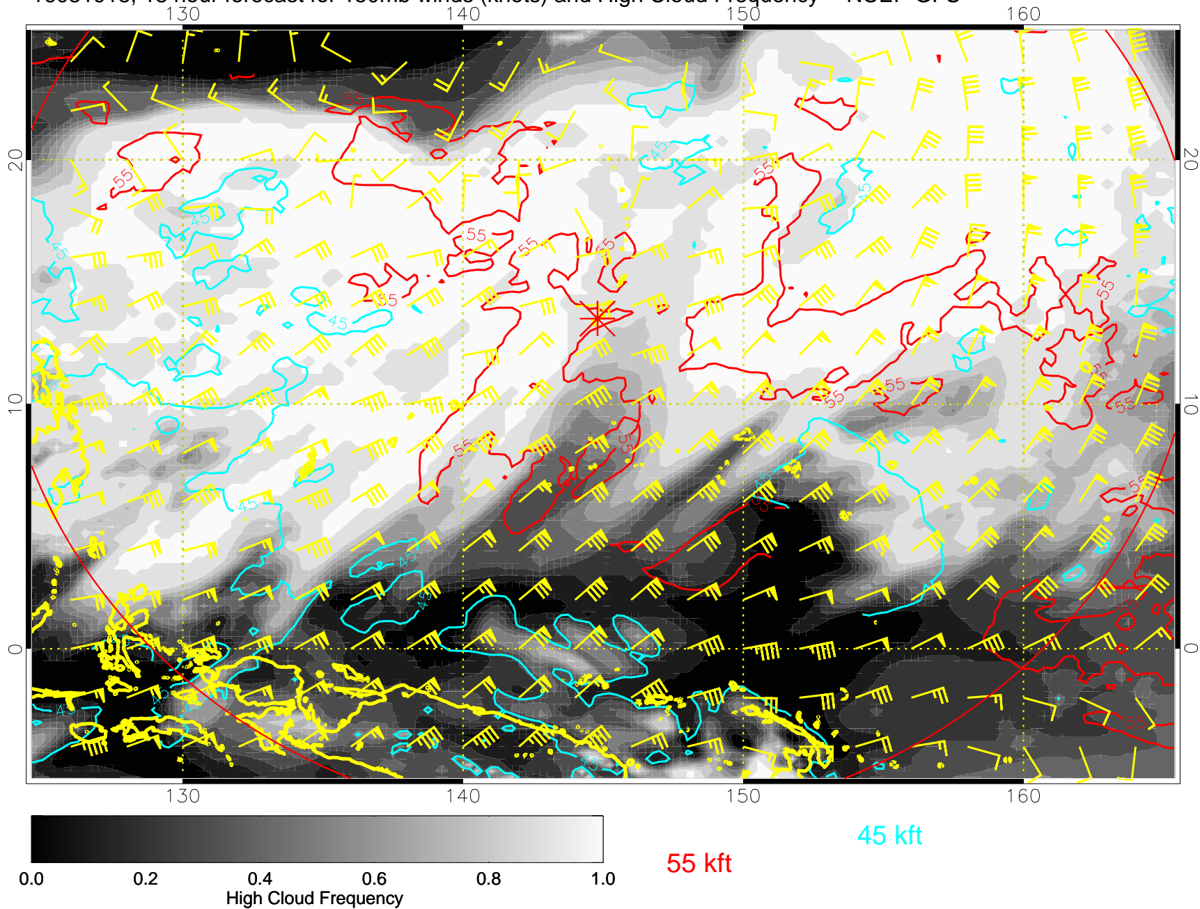
16081918, 18 hour forecast for 150mb winds (knots) and High Cloud Frequency -- NCEP GFS
