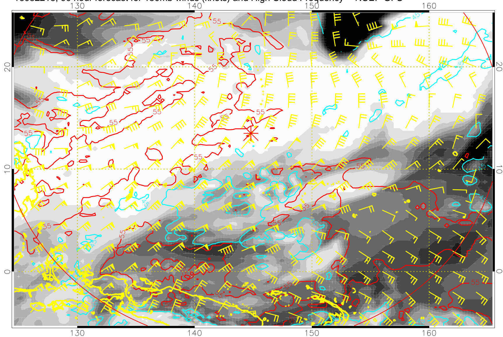
16082218, 90 hour forecast for 150mb winds (knots) and High Cloud Frequency -- NCEP GFS
