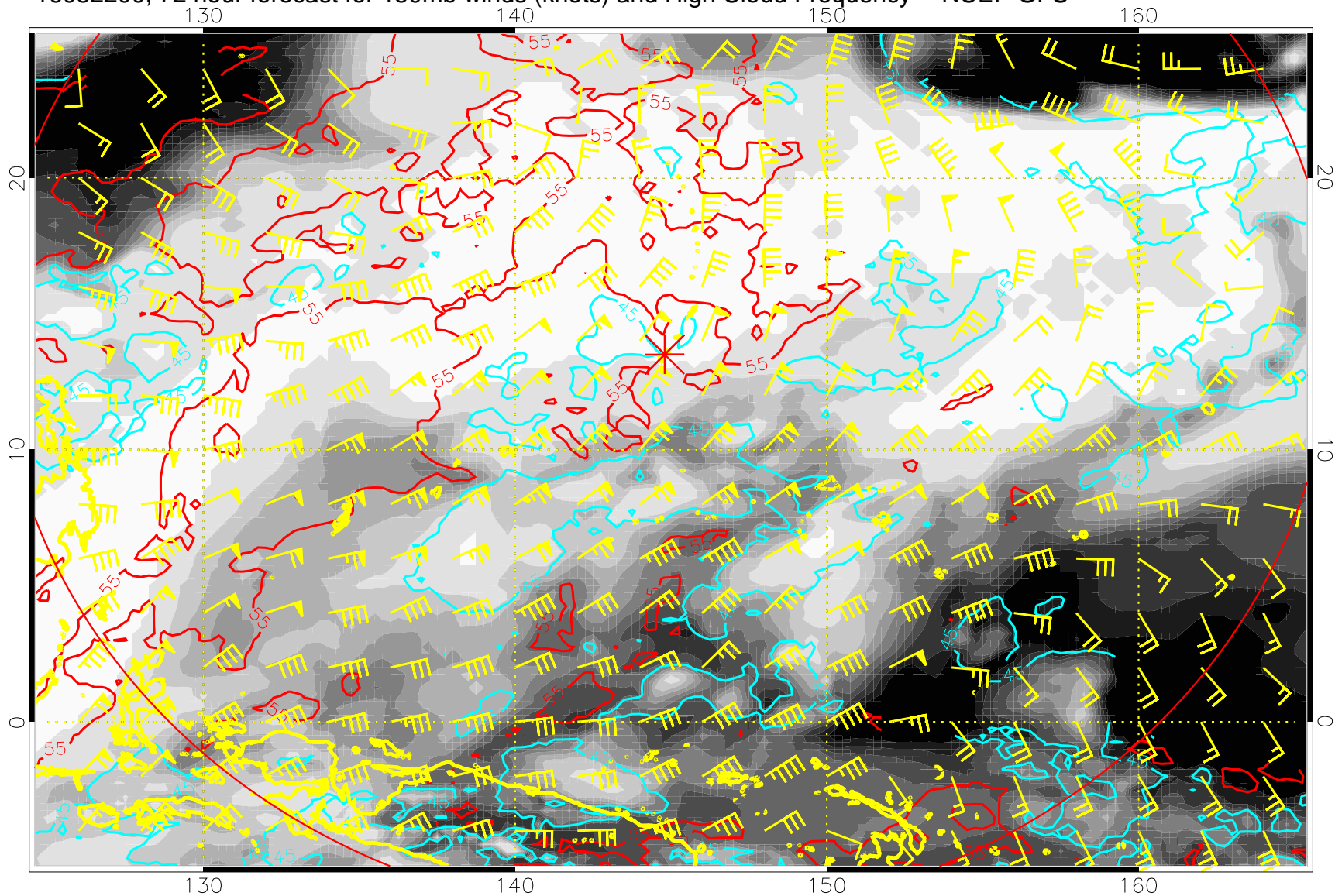
16082200, 72 hour forecast for 150mb winds (knots) and High Cloud Frequency -- NCEP GFS
