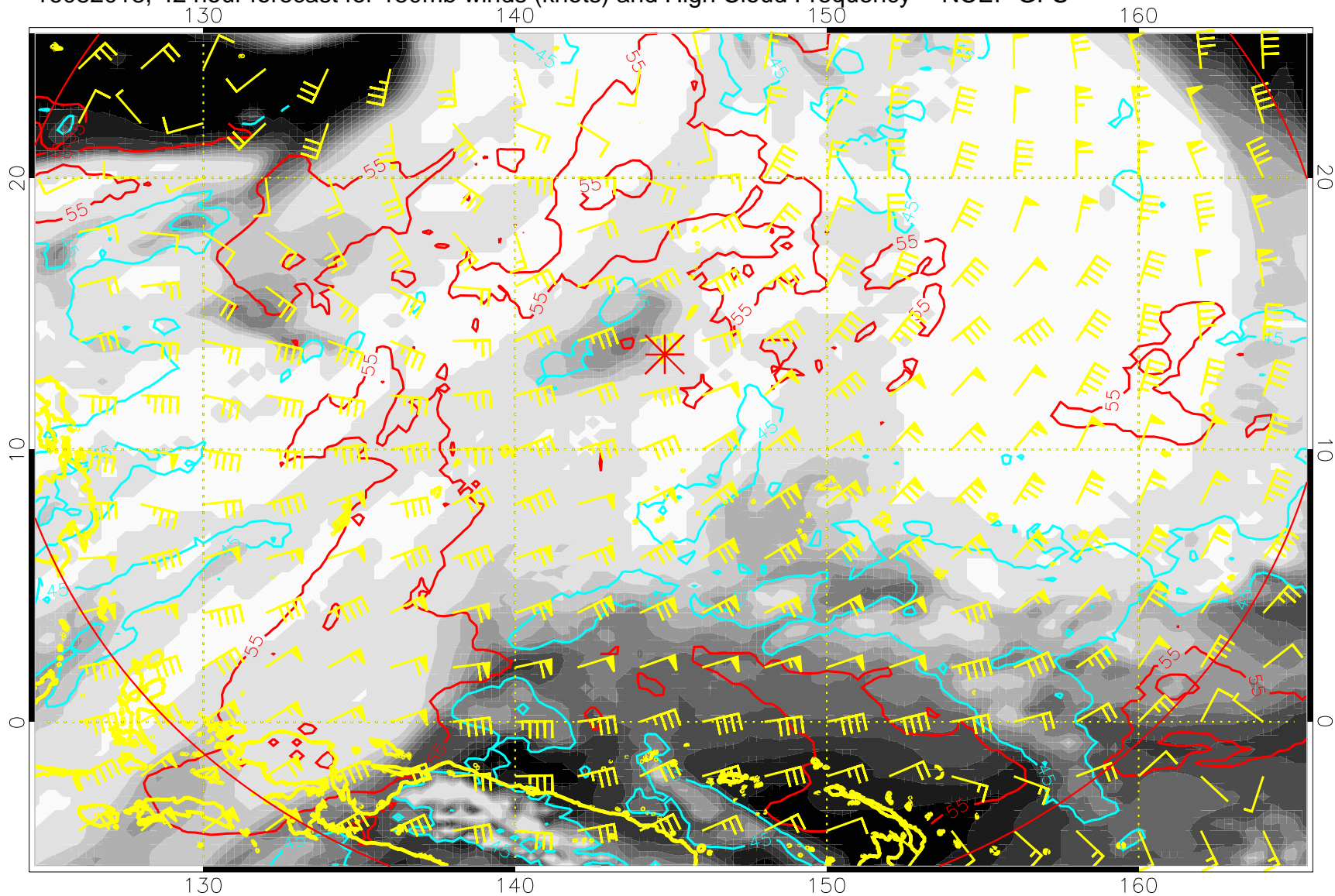
16082018, 42 hour forecast for 150mb winds (knots) and High Cloud Frequency -- NCEP GFS
