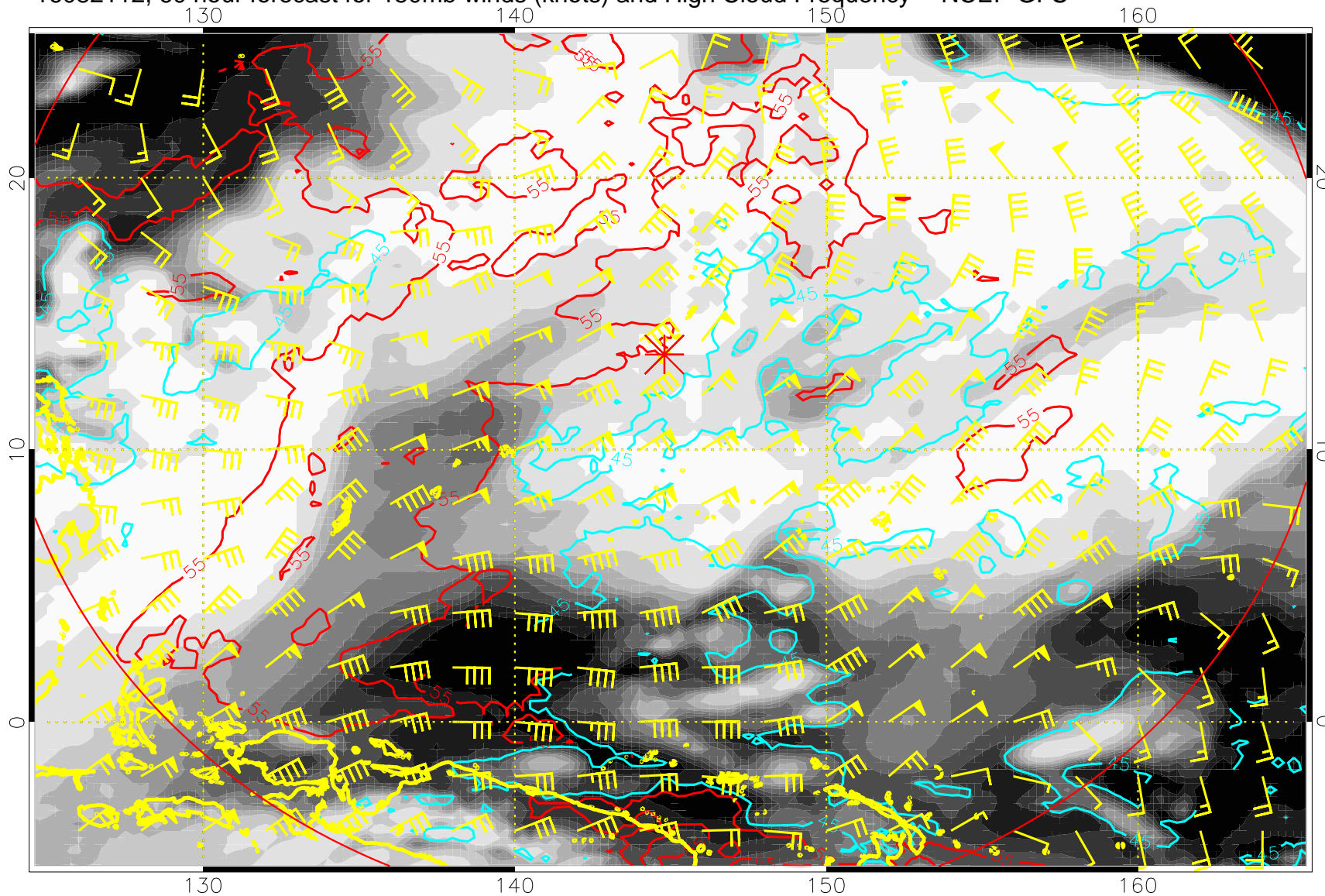
16082112, 60 hour forecast for 150mb winds (knots) and High Cloud Frequency -- NCEP GFS
