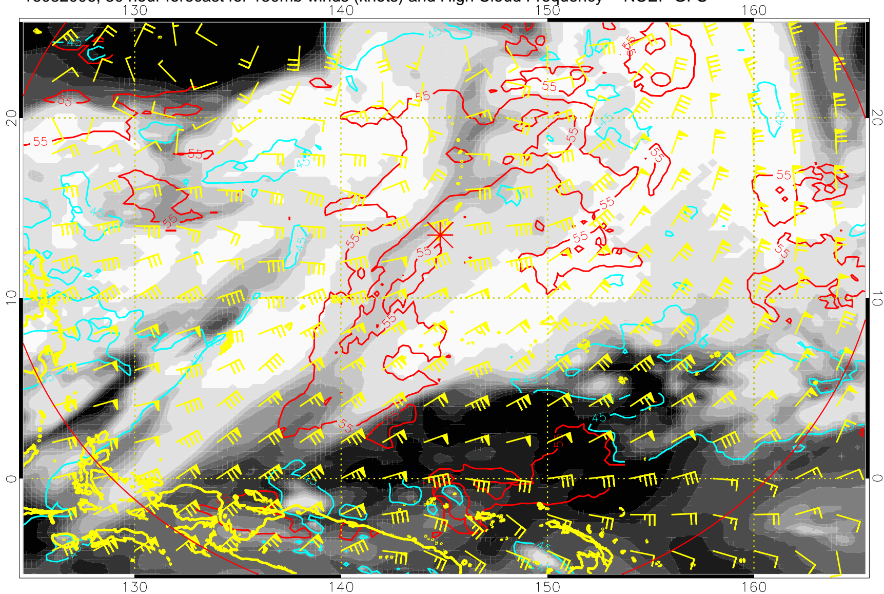
16082006, 30 hour forecast for 150mb winds (knots) and High Cloud Frequency -- NCEP GFS
