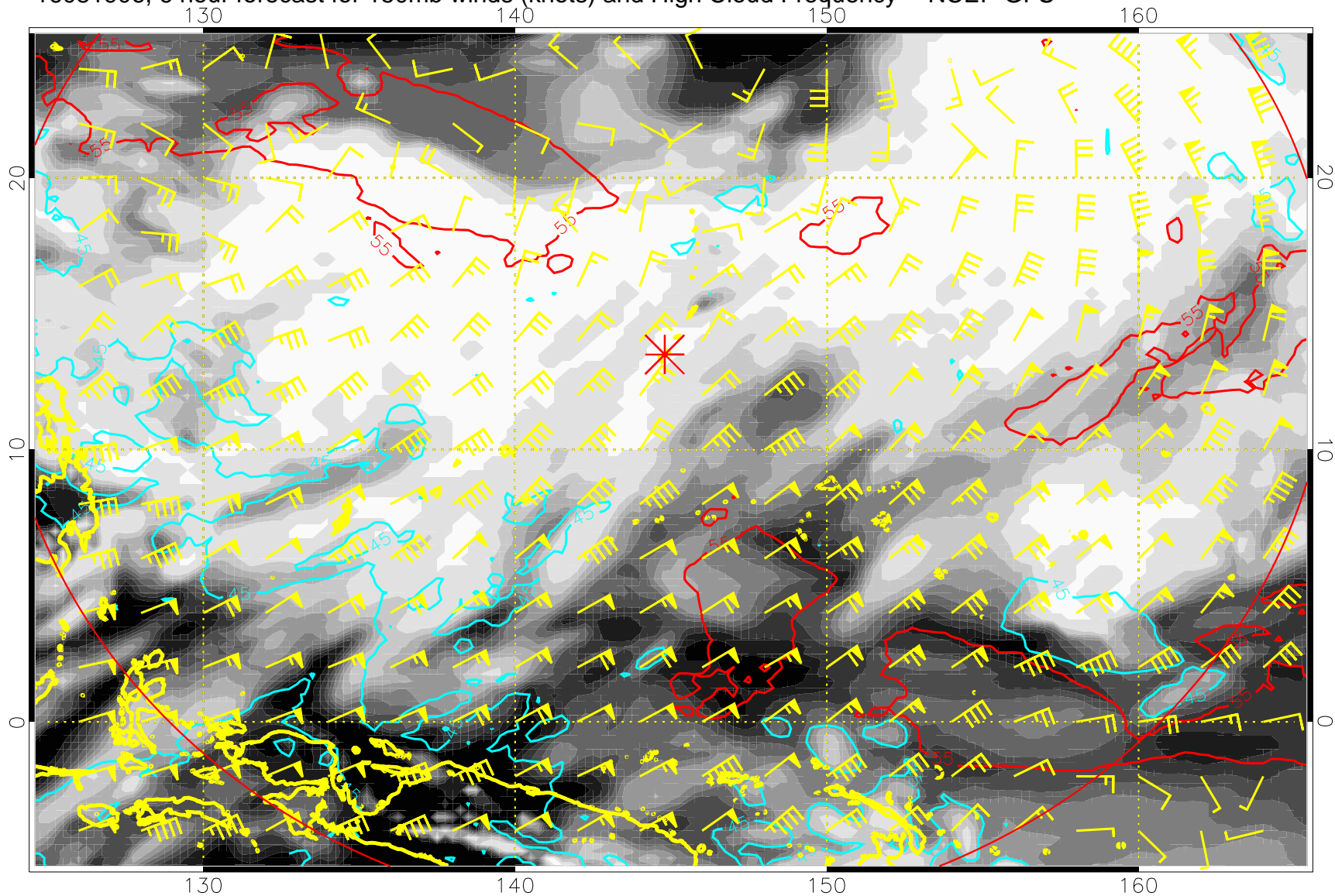
16081906, 6 hour forecast for 150mb winds (knots) and High Cloud Frequency -- NCEP GFS
