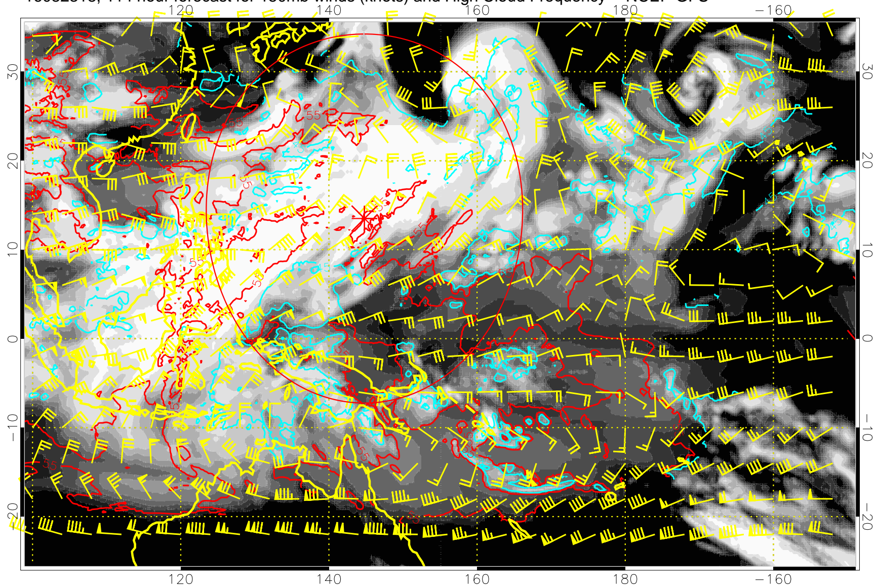
16082318, 114 hour forecast for 150mb winds (knots) and High Cloud Frequency -- NCEP GFS
