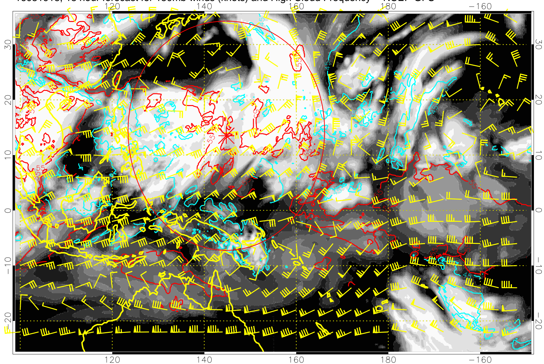
16081918, 18 hour forecast for 150mb winds (knots) and High Cloud Frequency -- NCEP GFS
