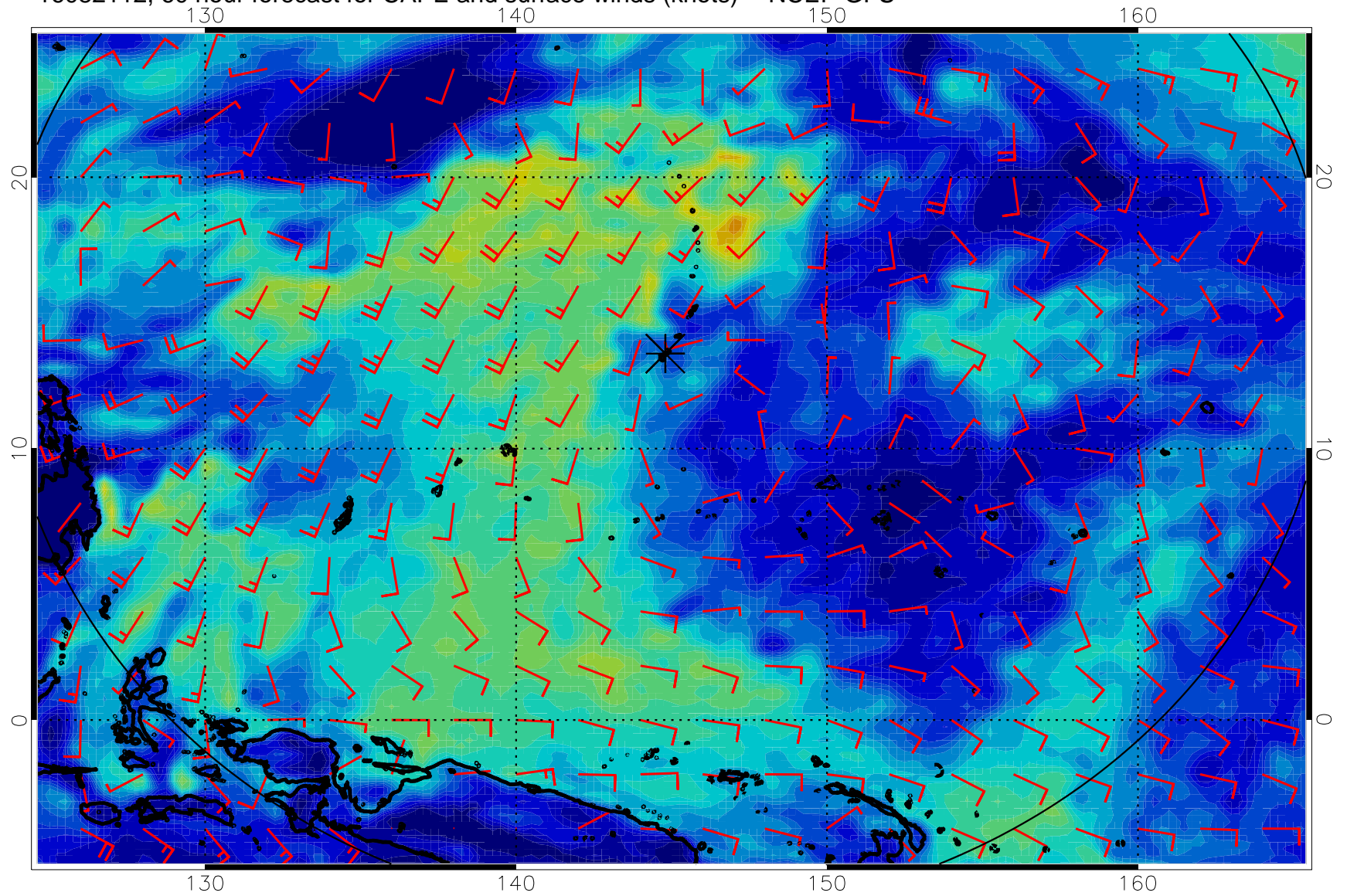
16082112, 60 hour forecast for CAPE and surface winds (knots) -- NCEP GFS
