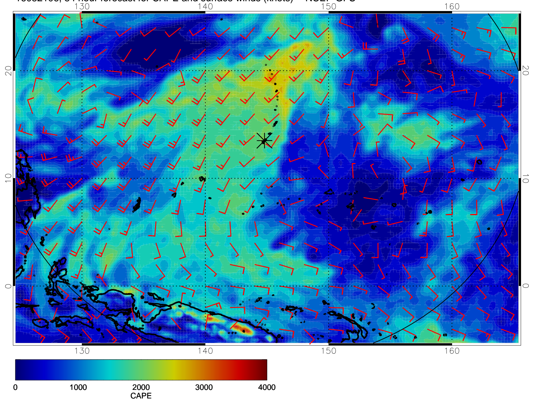
16082106, 54 hour forecast for CAPE and surface winds (knots) -- NCEP GFS
