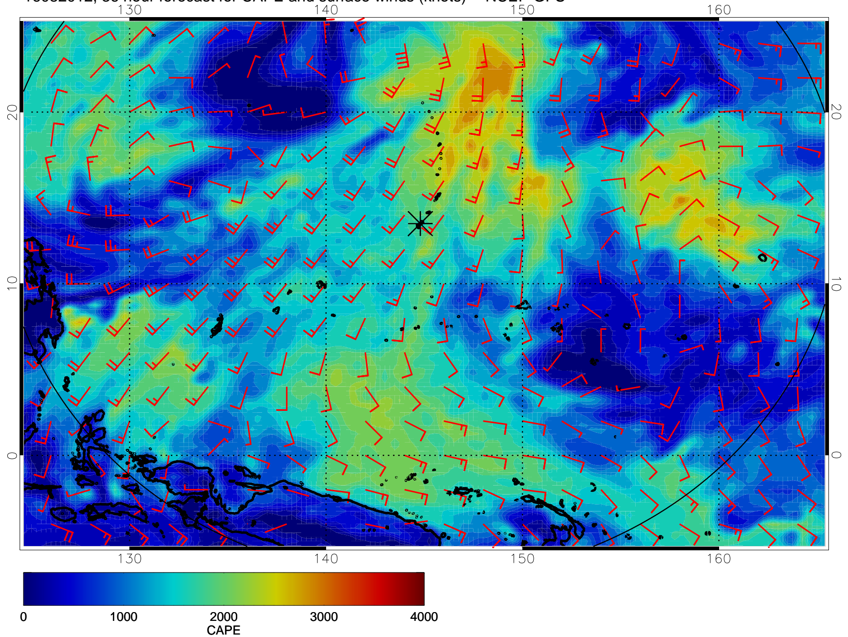
16082012, 36 hour forecast for CAPE and surface winds (knots) -- NCEP GFS
