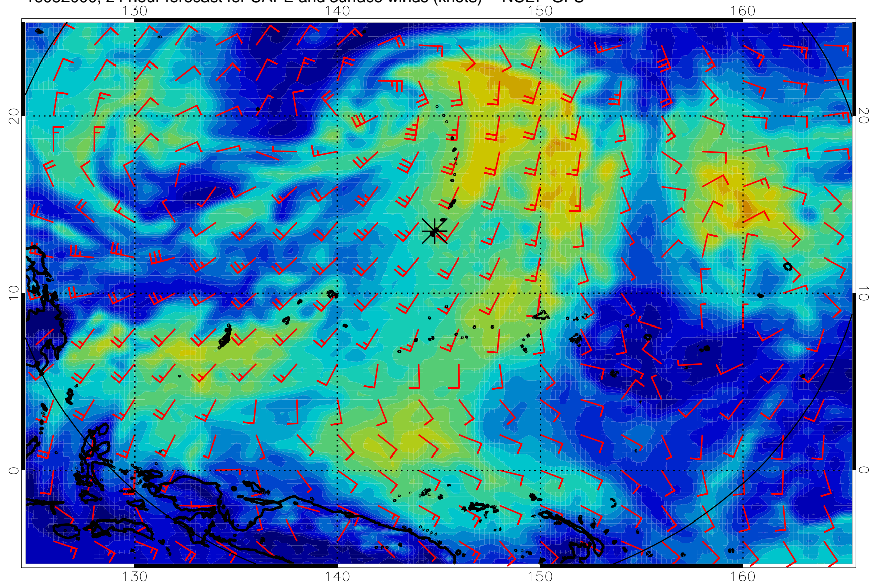
16082000, 24 hour forecast for CAPE and surface winds (knots) -- NCEP GFS
