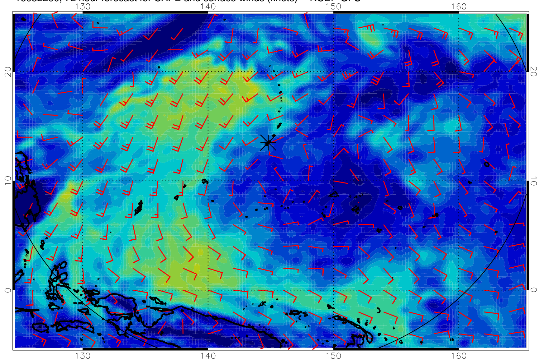
16082200, 72 hour forecast for CAPE and surface winds (knots) -- NCEP GFS
