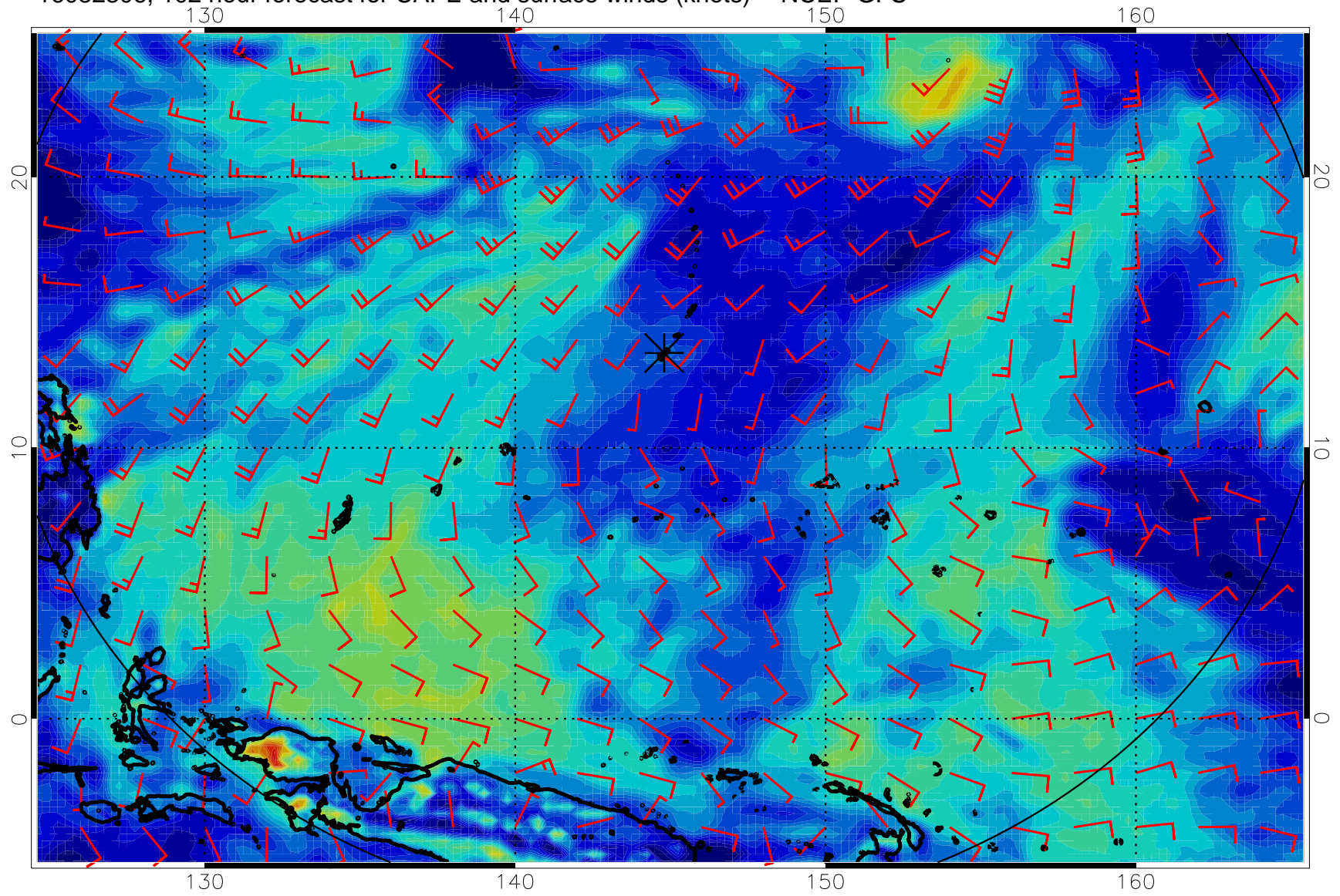
16082306, 102 hour forecast for CAPE and surface winds (knots) -- NCEP GFS
