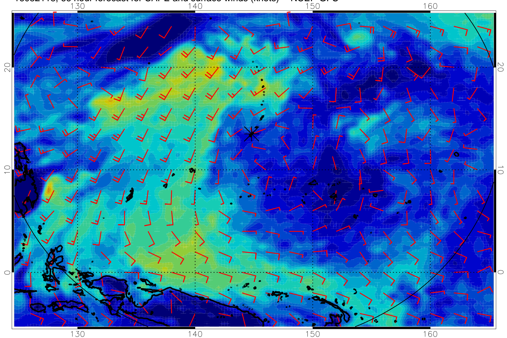
16082118, 66 hour forecast for CAPE and surface winds (knots) -- NCEP GFS
