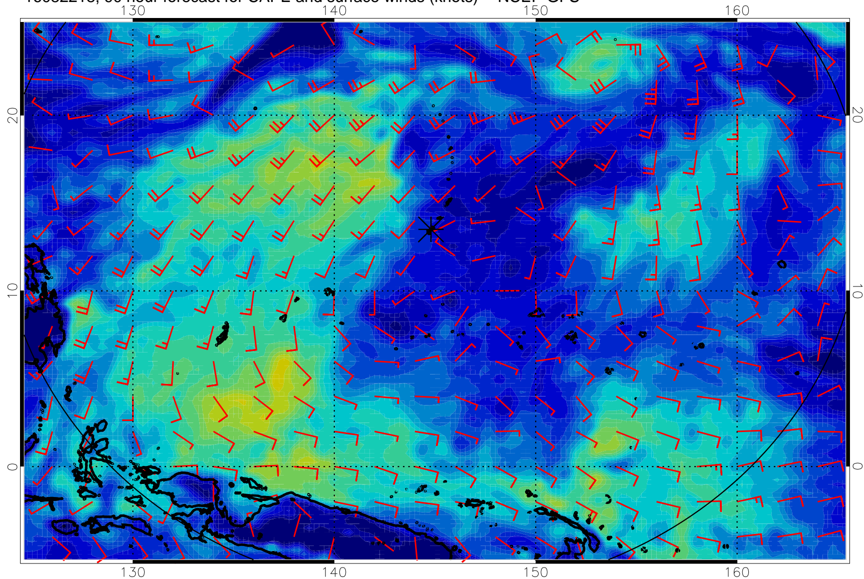
16082218, 90 hour forecast for CAPE and surface winds (knots) -- NCEP GFS
