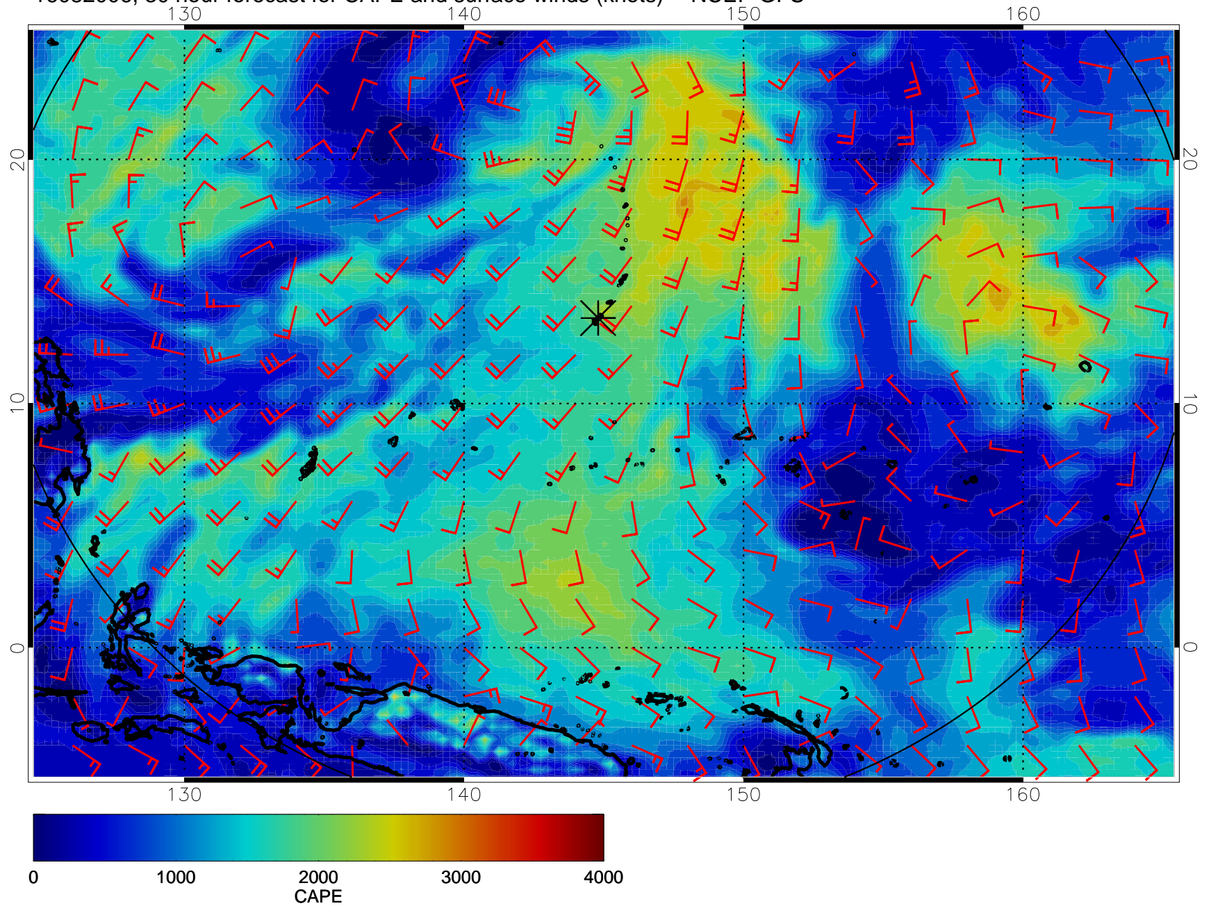
16082006, 30 hour forecast for CAPE and surface winds (knots) -- NCEP GFS
