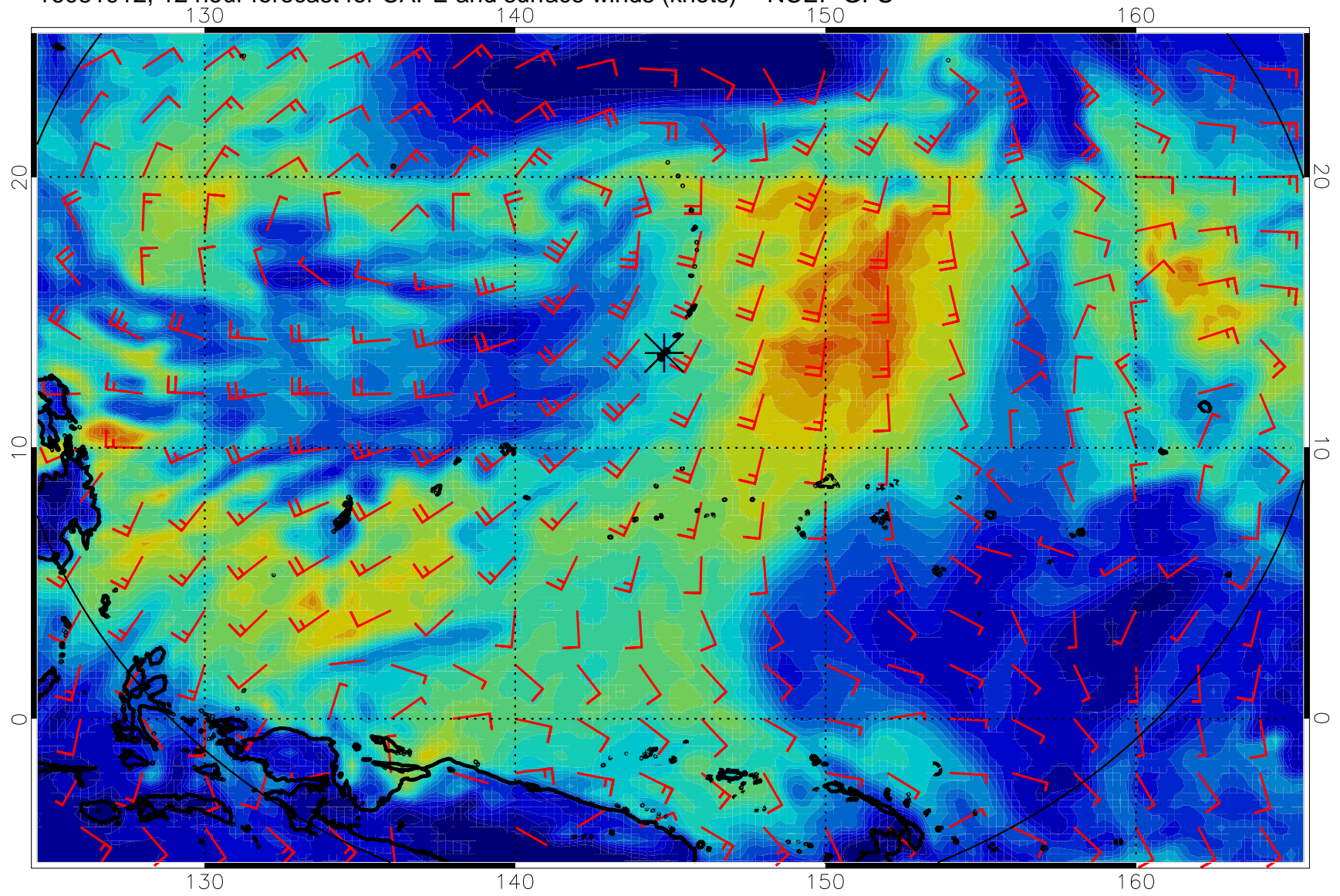
16081912, 12 hour forecast for CAPE and surface winds (knots) -- NCEP GFS
