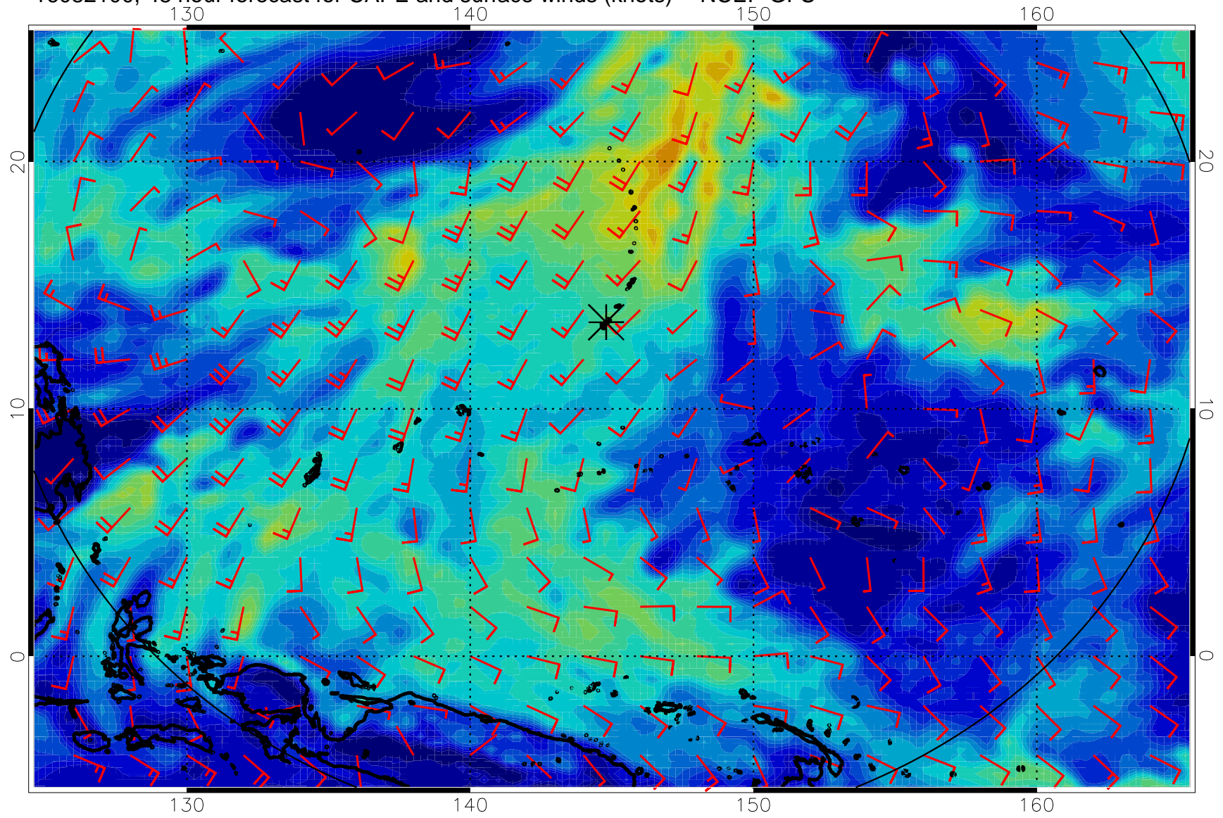
16082100, 48 hour forecast for CAPE and surface winds (knots) -- NCEP GFS
