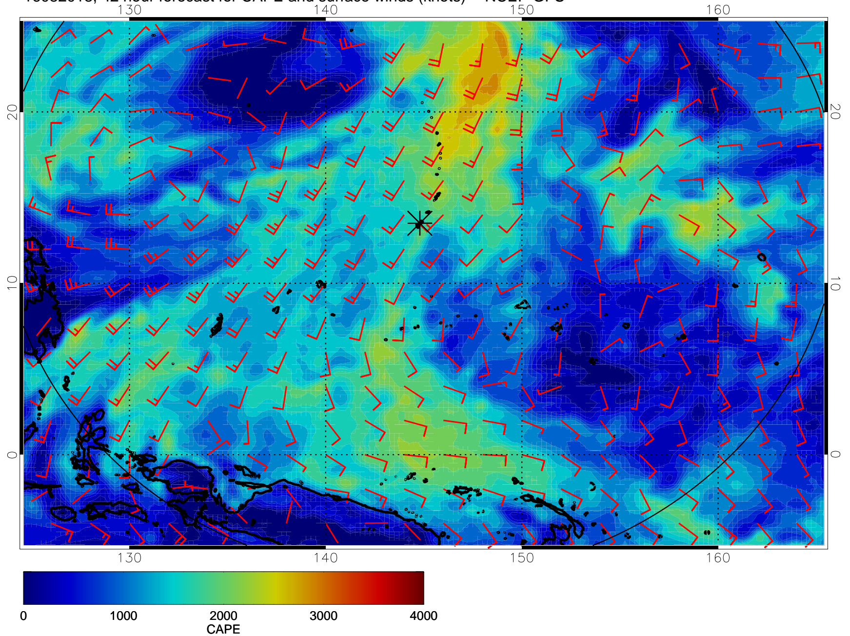
16082018, 42 hour forecast for CAPE and surface winds (knots) -- NCEP GFS
