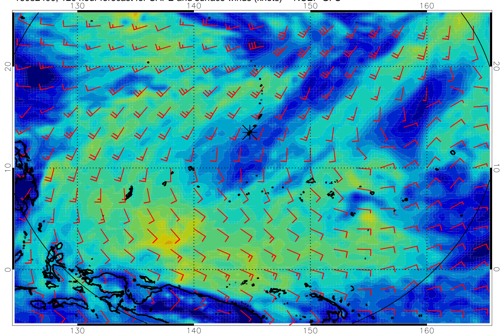
16082400, 120 hour forecast for CAPE and surface winds (knots) -- NCEP GFS
