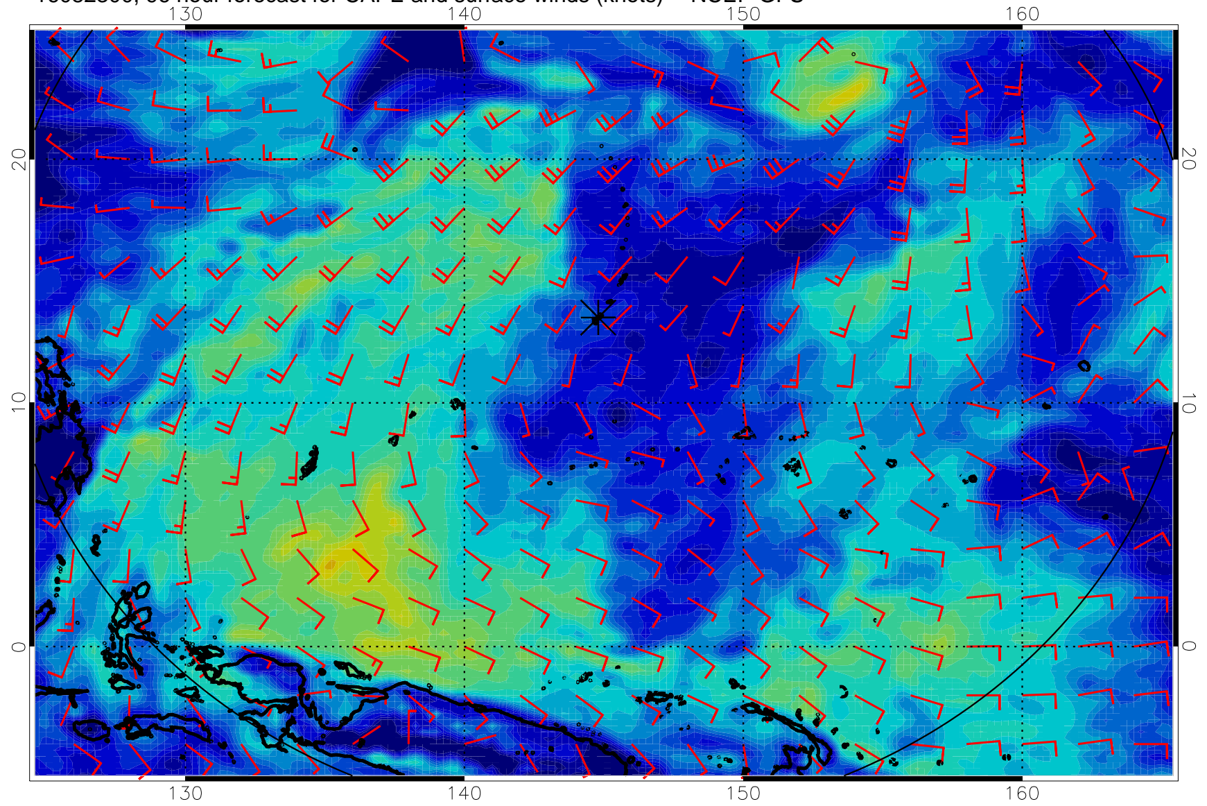
16082300, 96 hour forecast for CAPE and surface winds (knots) -- NCEP GFS
