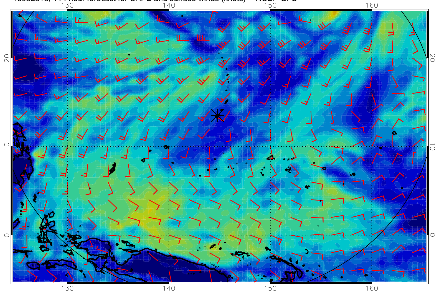
16082318, 114 hour forecast for CAPE and surface winds (knots) -- NCEP GFS
