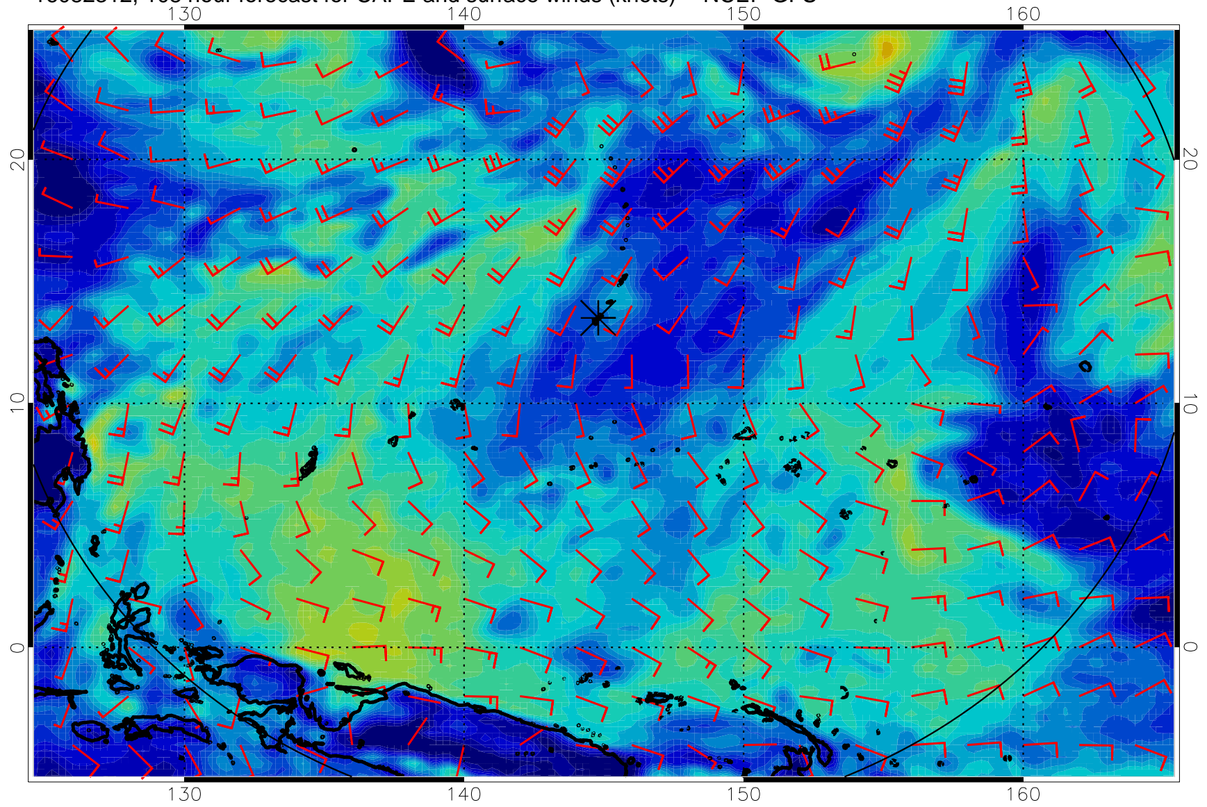
16082312, 108 hour forecast for CAPE and surface winds (knots) -- NCEP GFS
