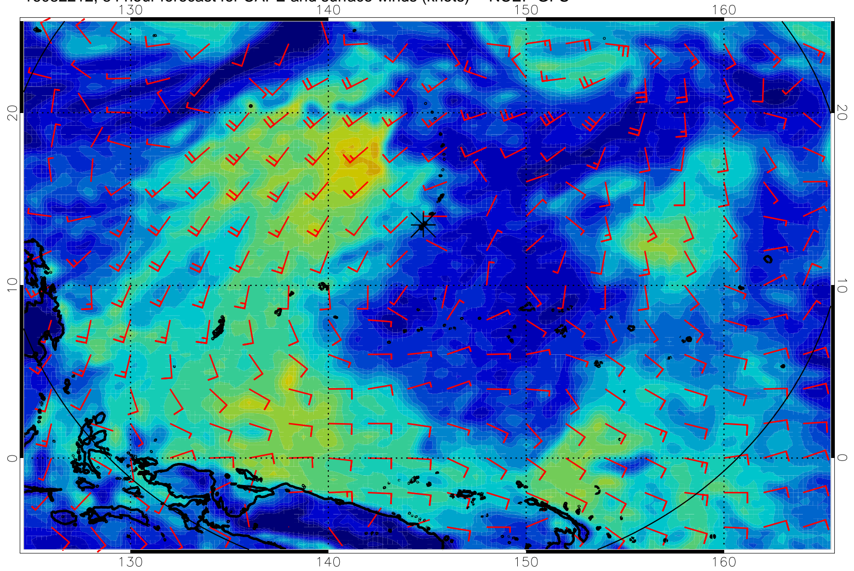
16082212, 84 hour forecast for CAPE and surface winds (knots) -- NCEP GFS
