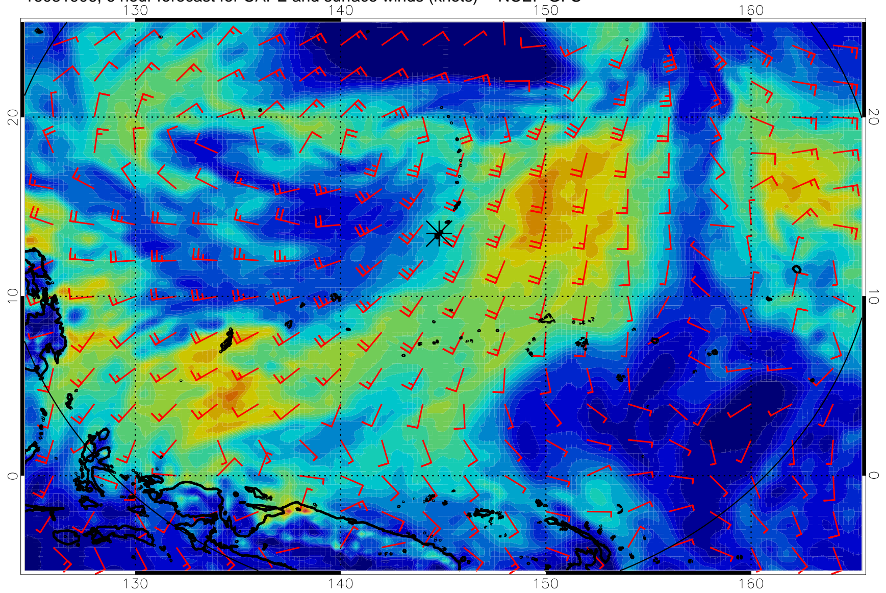
16081906, 6 hour forecast for CAPE and surface winds (knots) -- NCEP GFS
