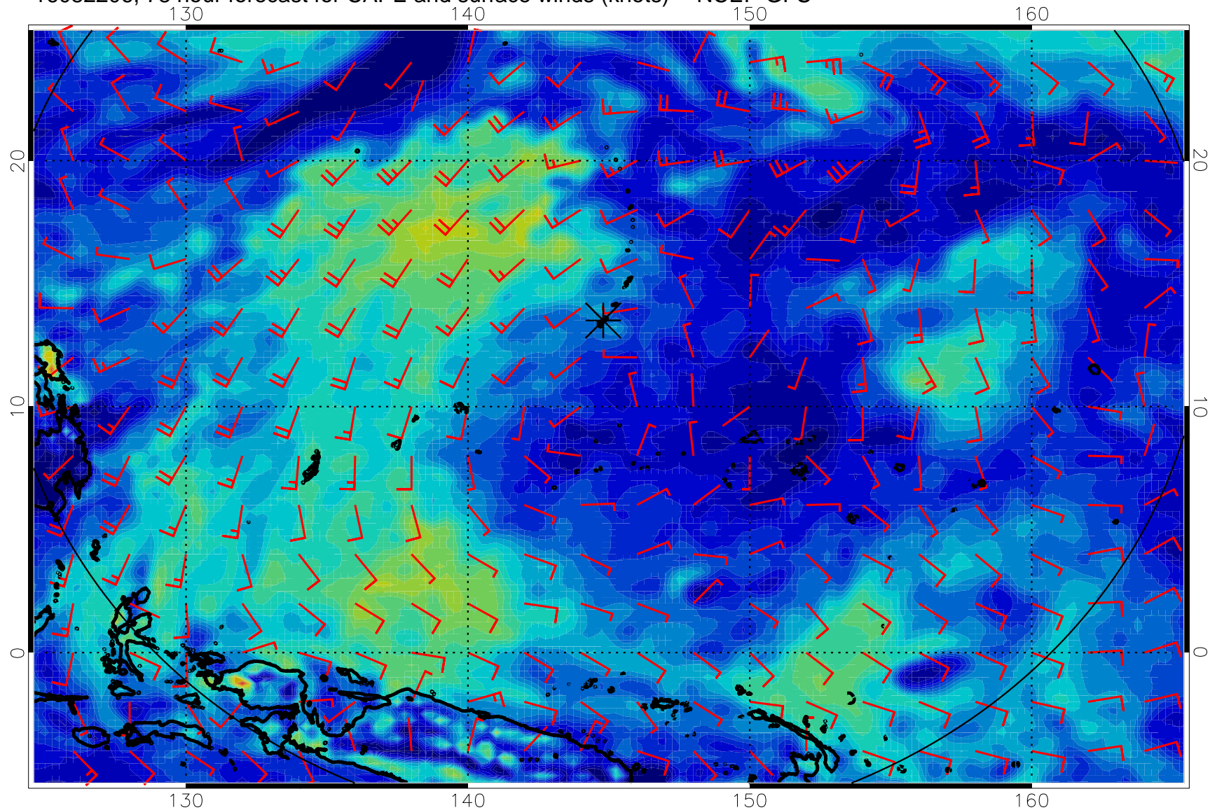
16082206, 78 hour forecast for CAPE and surface winds (knots) -- NCEP GFS
