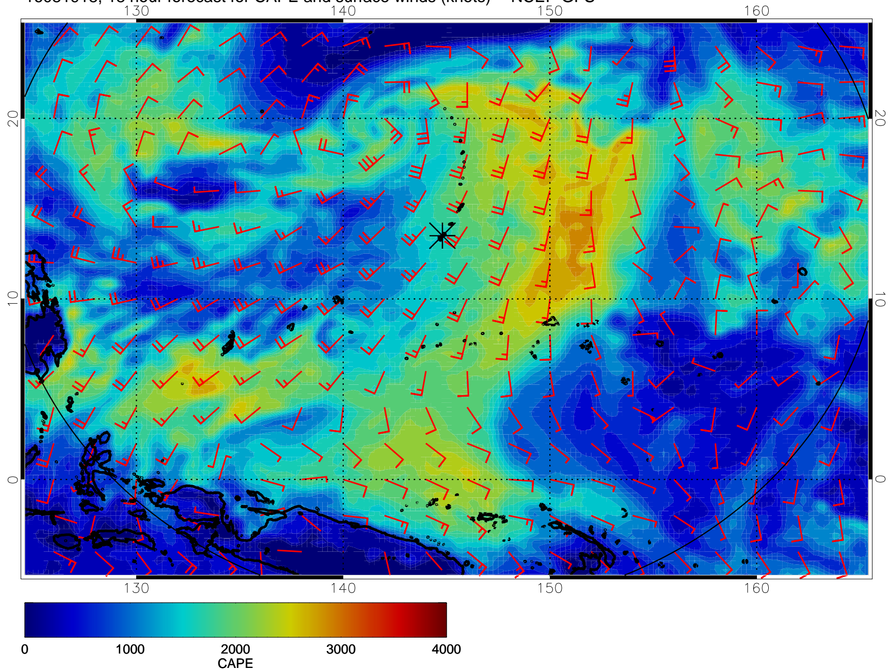
16081918, 18 hour forecast for CAPE and surface winds (knots) -- NCEP GFS
