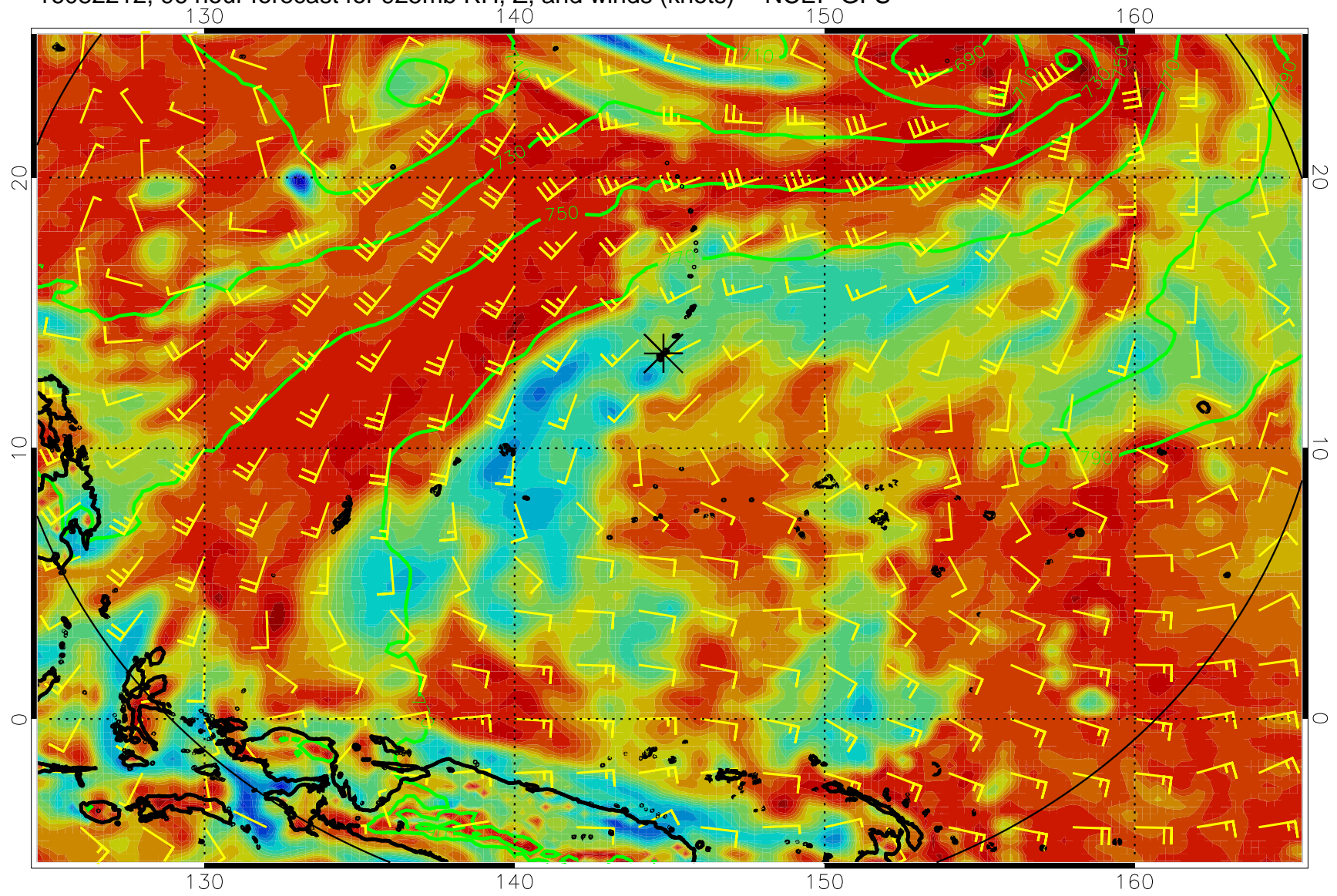
16082212, 96 hour forecast for 925mb RH, Z, and winds (knots) -- NCEP GFS
