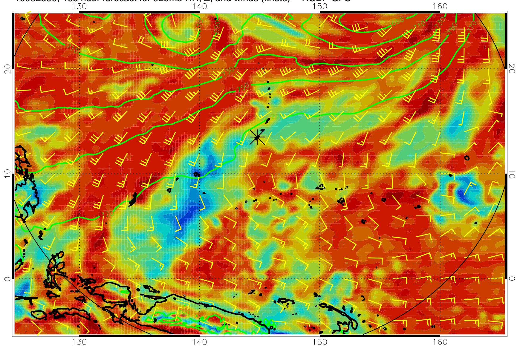
16082300, 108 hour forecast for 925mb RH, Z, and winds (knots) -- NCEP GFS
