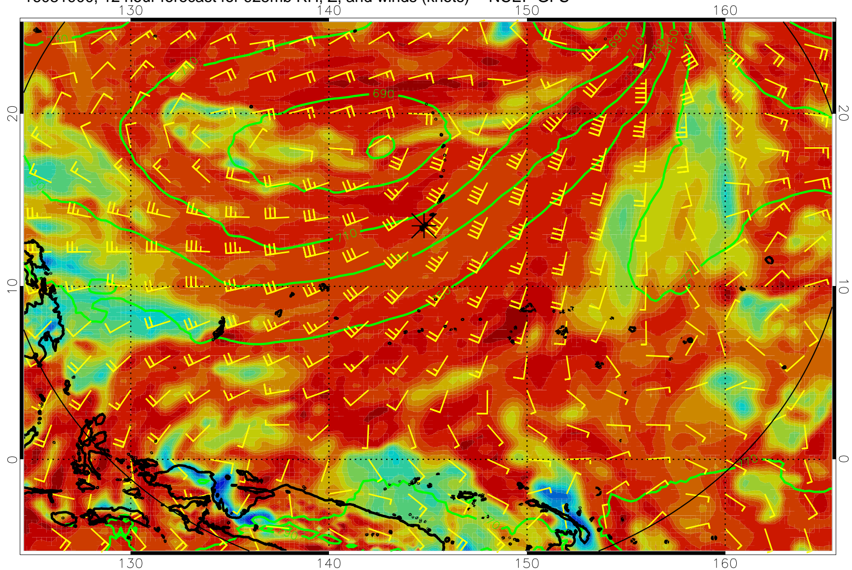
16081900, 12 hour forecast for 925mb RH, Z, and winds (knots) -- NCEP GFS
