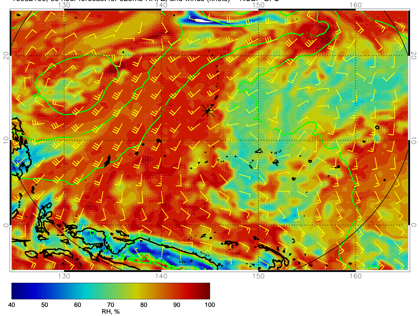
16082106, 66 hour forecast for 925mb RH, Z, and winds (knots) -- NCEP GFS
