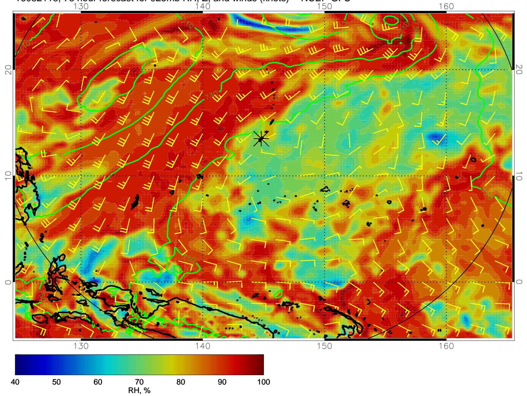
16082118, 78 hour forecast for 925mb RH, Z, and winds (knots) -- NCEP GFS
