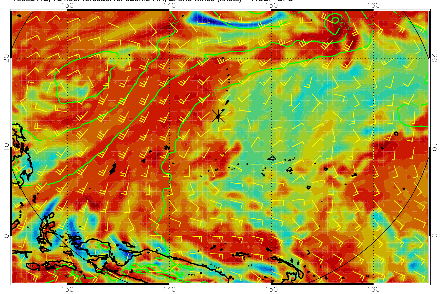
16082112, 72 hour forecast for 925mb RH, Z, and winds (knots) -- NCEP GFS
