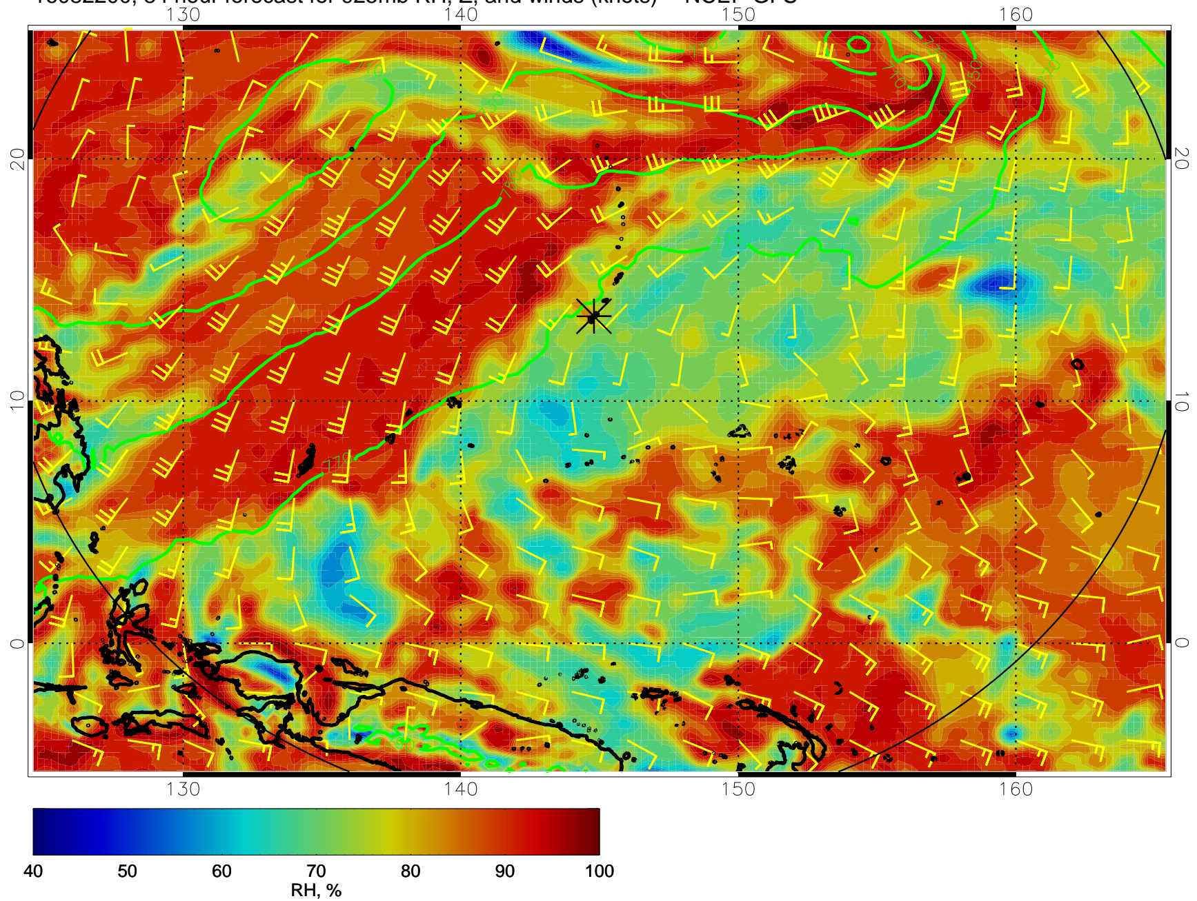
16082200, 84 hour forecast for 925mb RH, Z, and winds (knots) -- NCEP GFS
