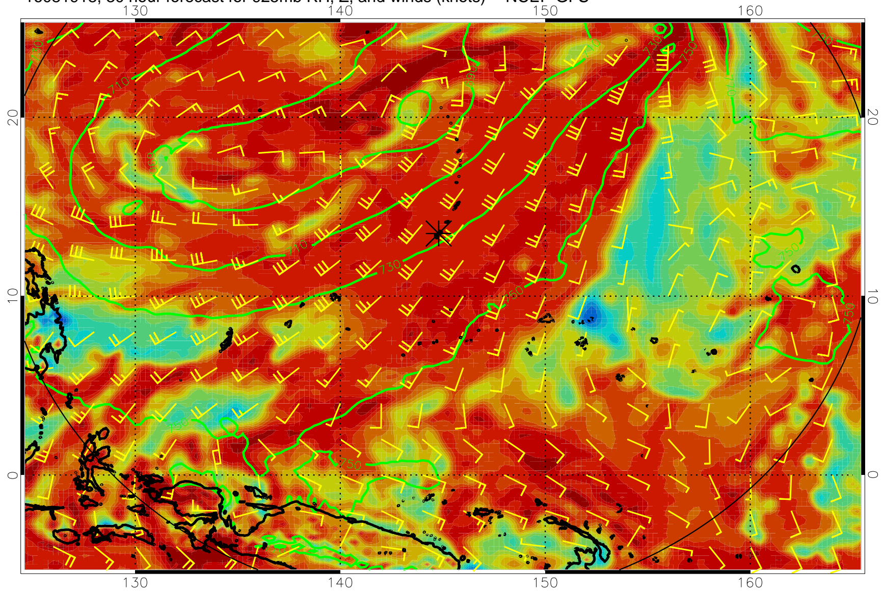
16081918, 30 hour forecast for 925mb RH, Z, and winds (knots) -- NCEP GFS
