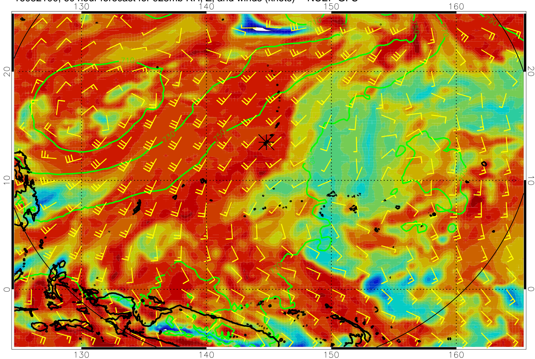
16082100, 60 hour forecast for 925mb RH, Z, and winds (knots) -- NCEP GFS
