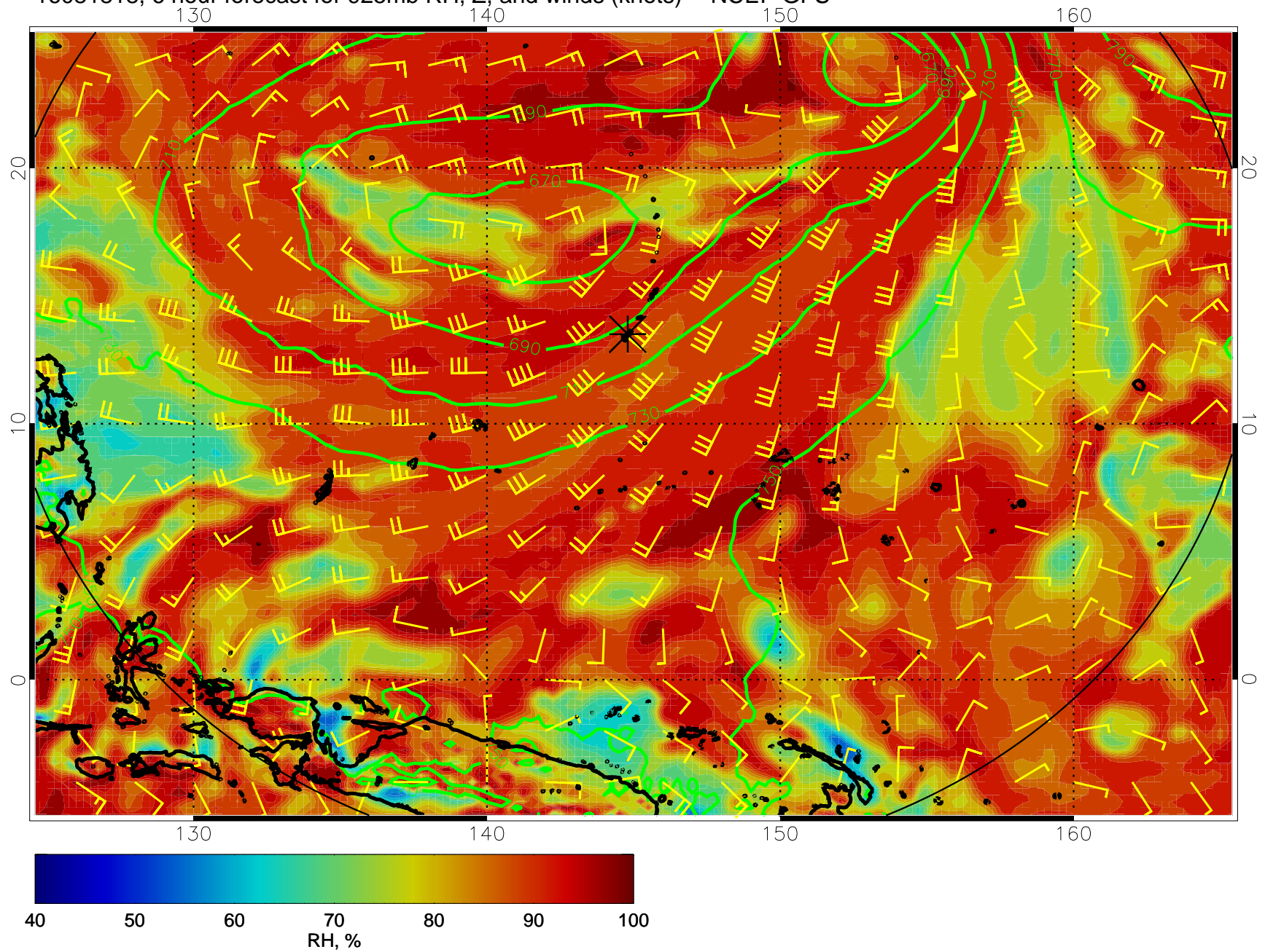
16081818, 6 hour forecast for 925mb RH, Z, and winds (knots) -- NCEP GFS
