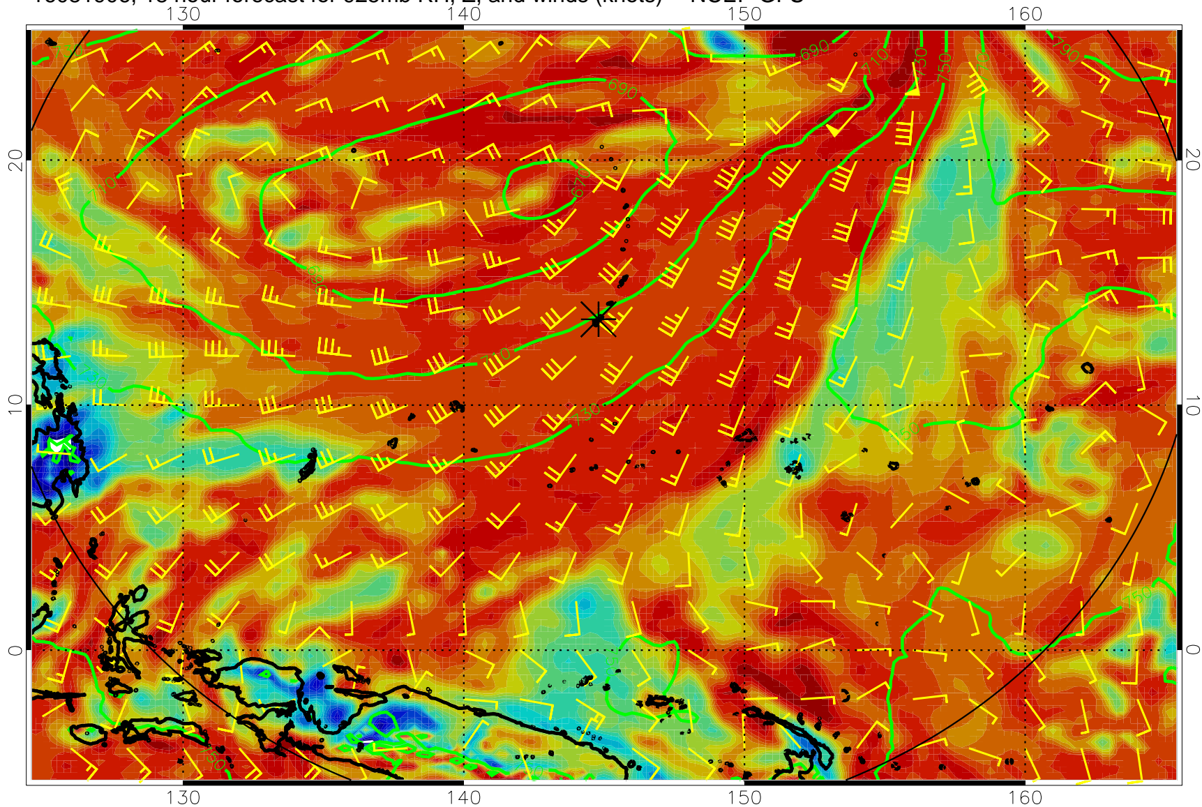
16081906, 18 hour forecast for 925mb RH, Z, and winds (knots) -- NCEP GFS
