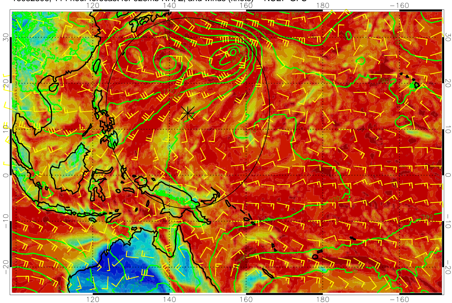
16082306, 114 hour forecast for 925mb RH, Z, and winds (knots) -- NCEP GFS
