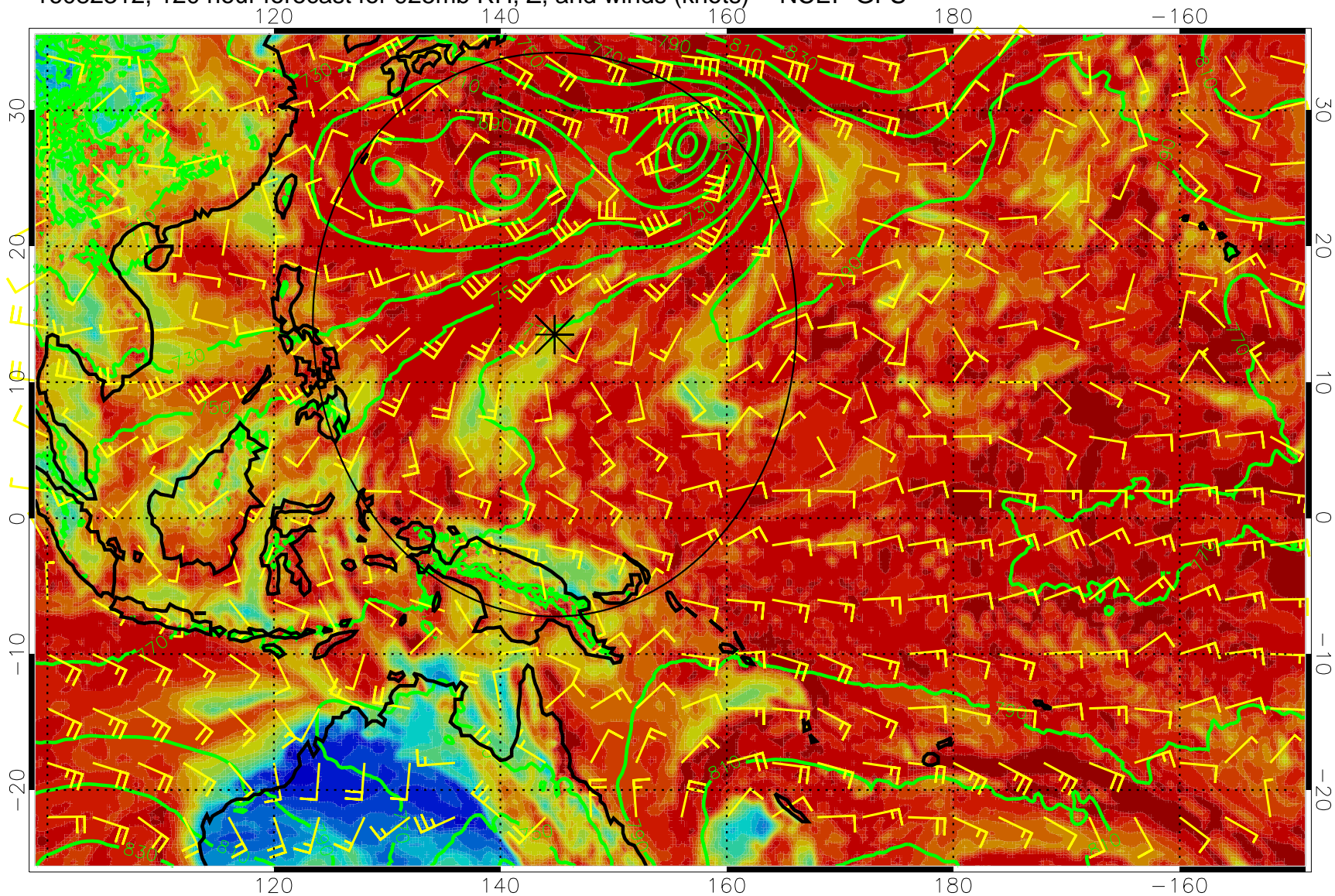
16082312, 120 hour forecast for 925mb RH, Z, and winds (knots) -- NCEP GFS
