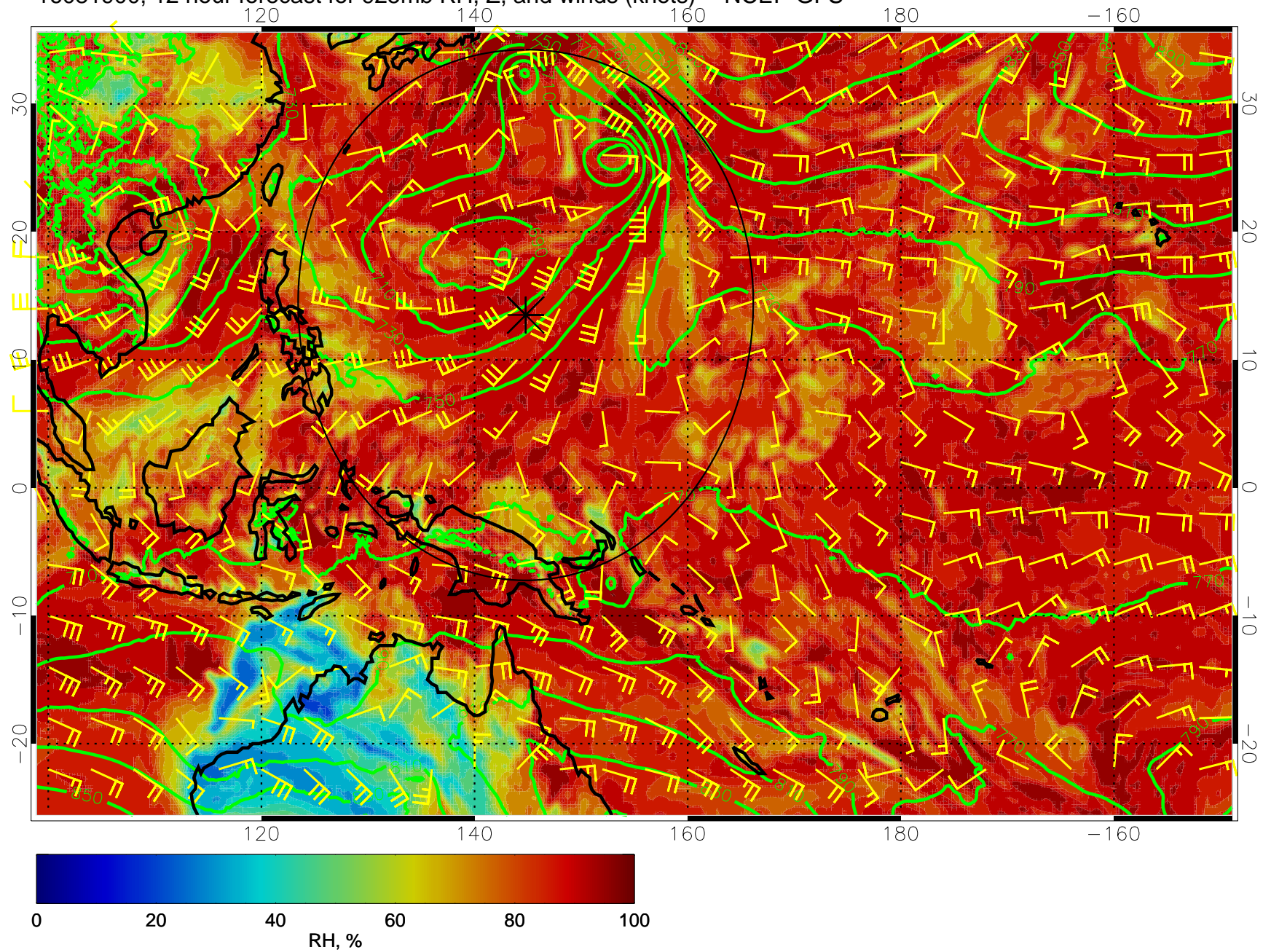
16081900, 12 hour forecast for 925mb RH, Z, and winds (knots) -- NCEP GFS
