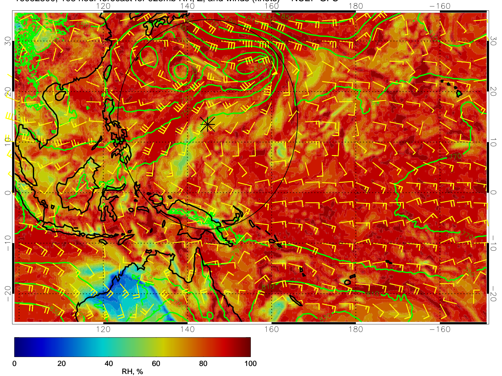
16082300, 108 hour forecast for 925mb RH, Z, and winds (knots) -- NCEP GFS
