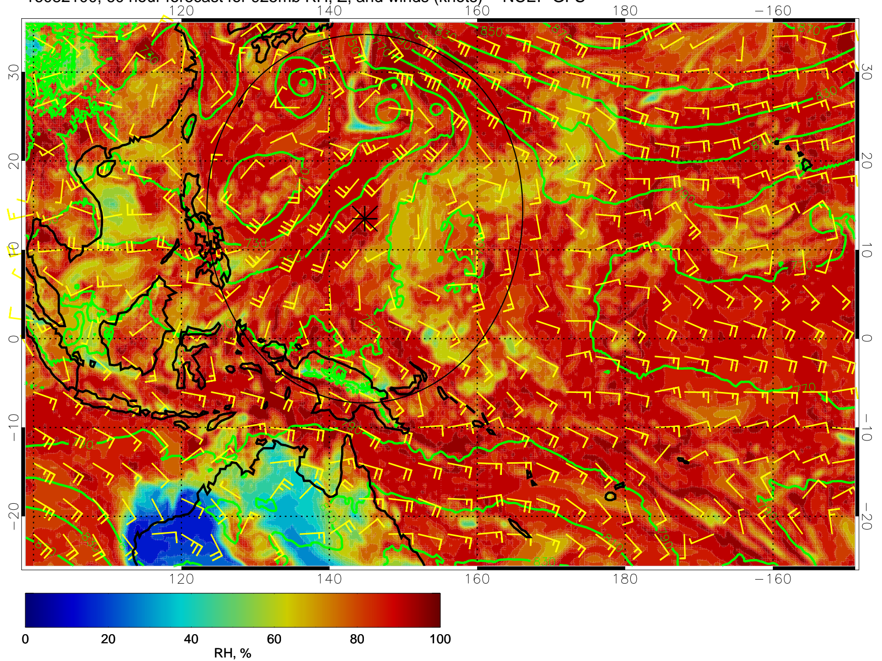
16082100, 60 hour forecast for 925mb RH, Z, and winds (knots) -- NCEP GFS
