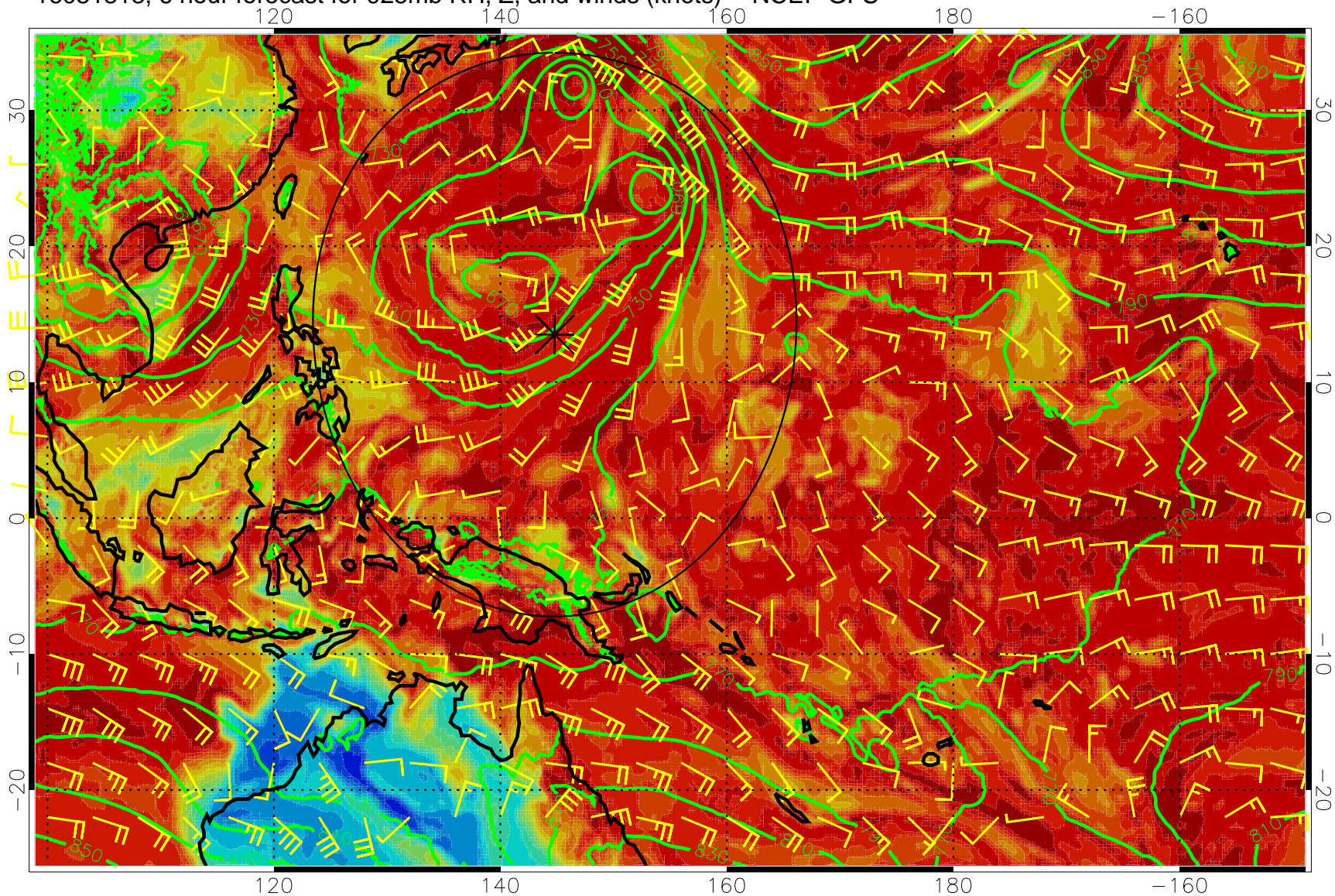
16081818, 6 hour forecast for 925mb RH, Z, and winds (knots) -- NCEP GFS
