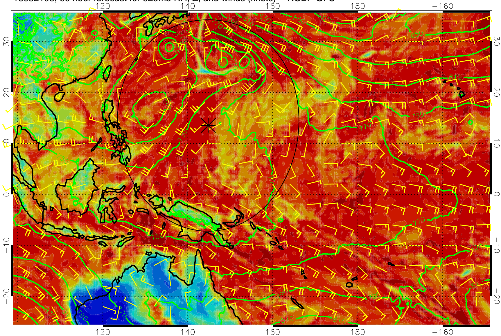
16082106, 66 hour forecast for 925mb RH, Z, and winds (knots) -- NCEP GFS
