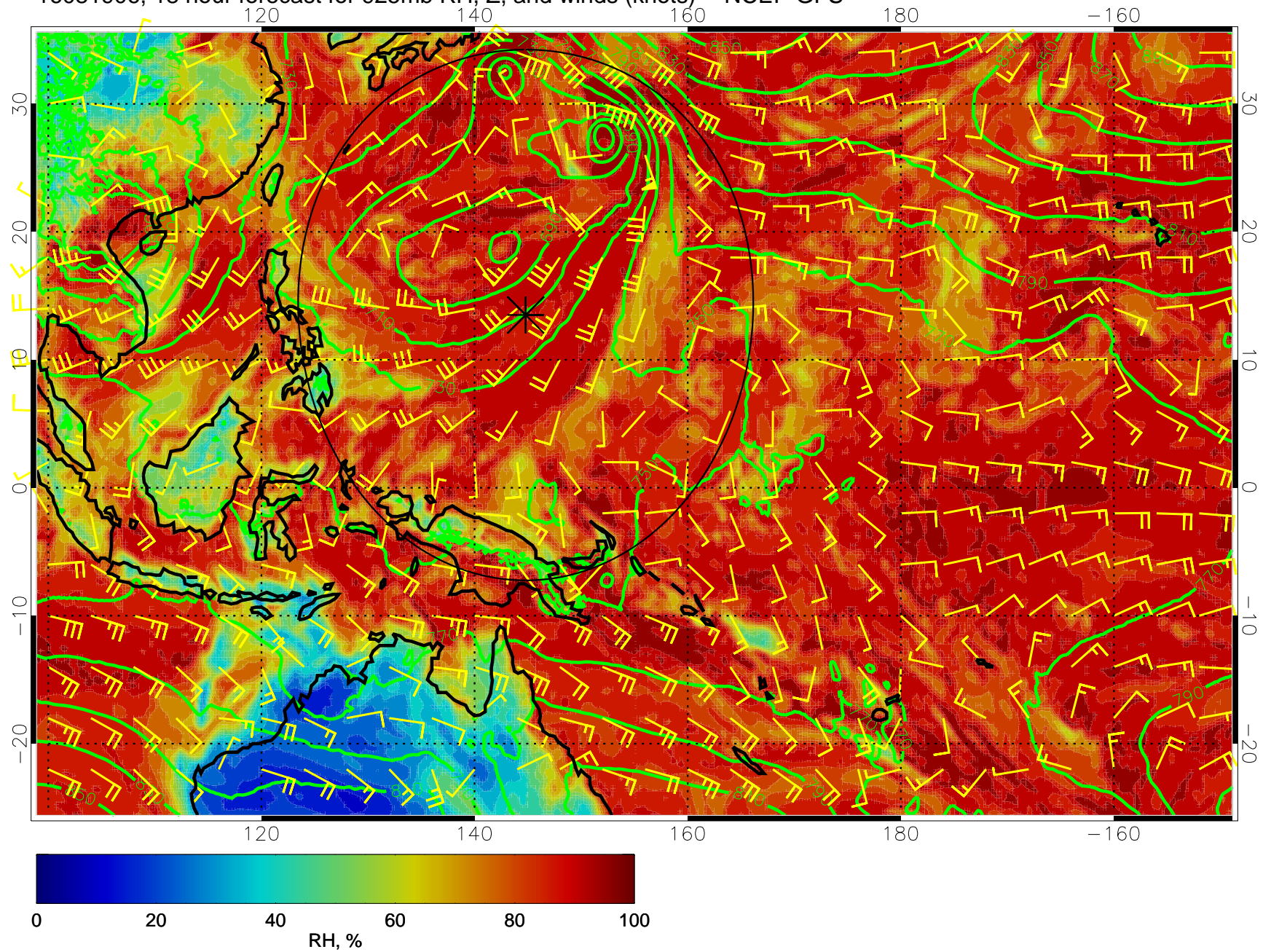
16081906, 18 hour forecast for 925mb RH, Z, and winds (knots) -- NCEP GFS
