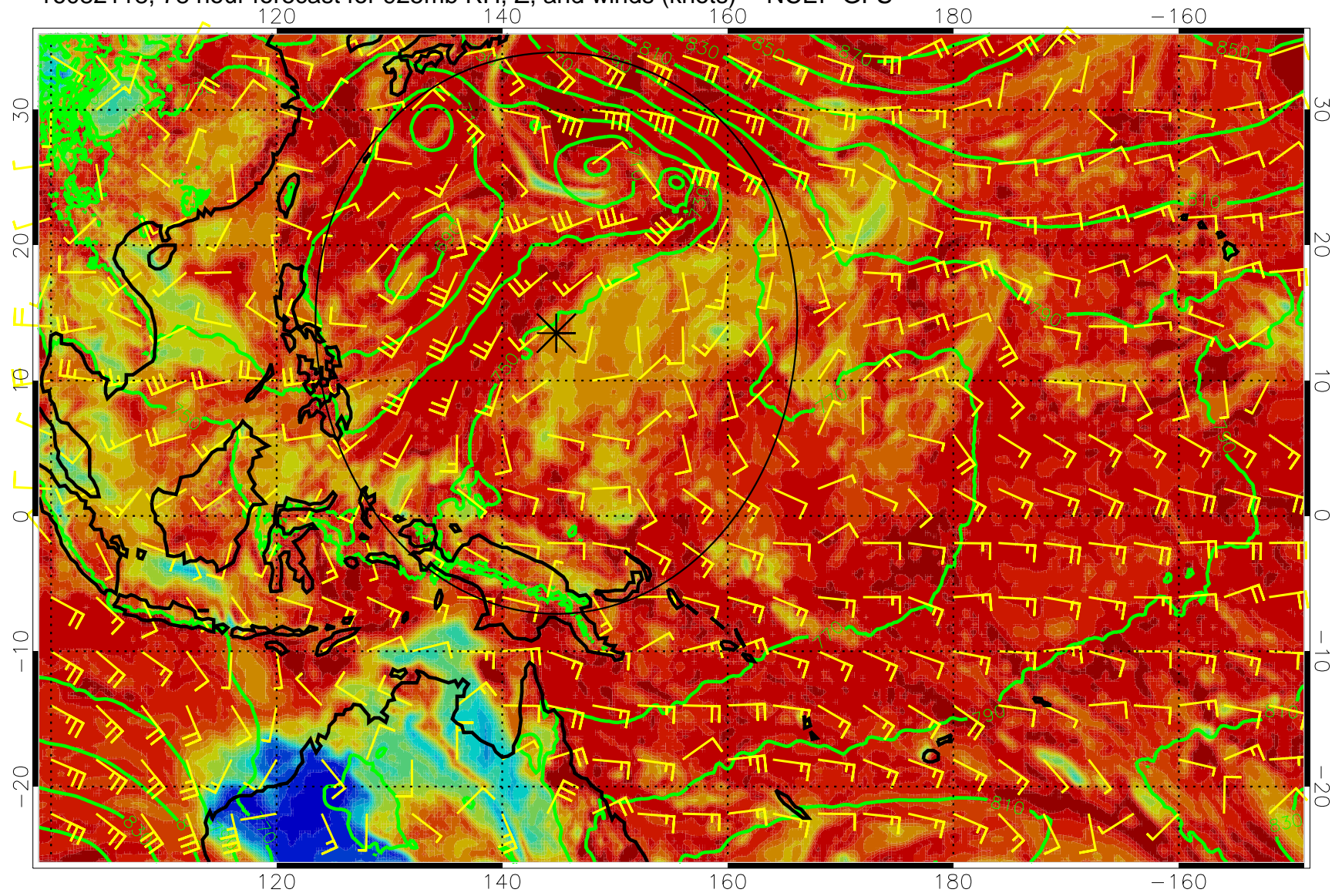
16082118, 78 hour forecast for 925mb RH, Z, and winds (knots) -- NCEP GFS
