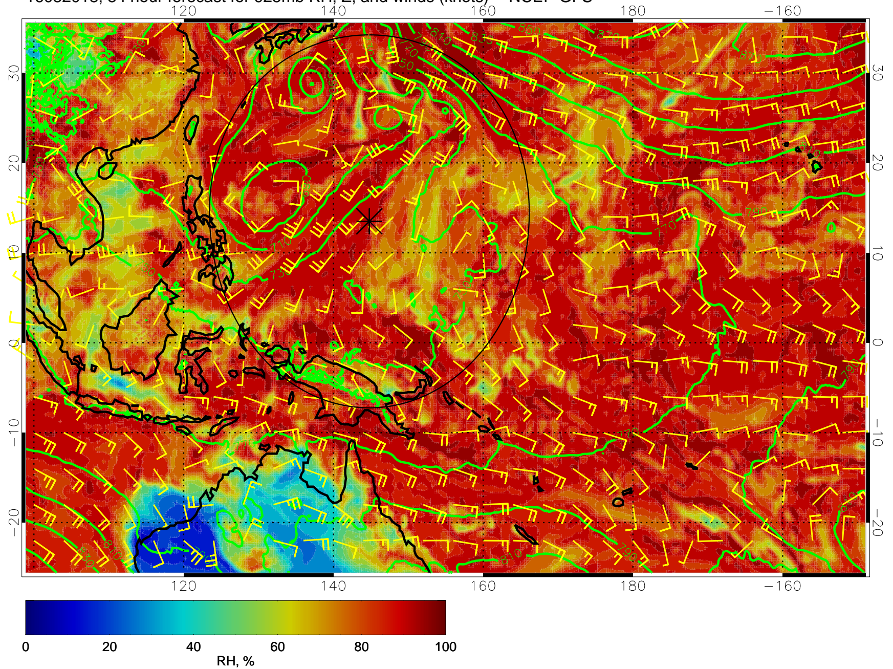
16082018, 54 hour forecast for 925mb RH, Z, and winds (knots) -- NCEP GFS
