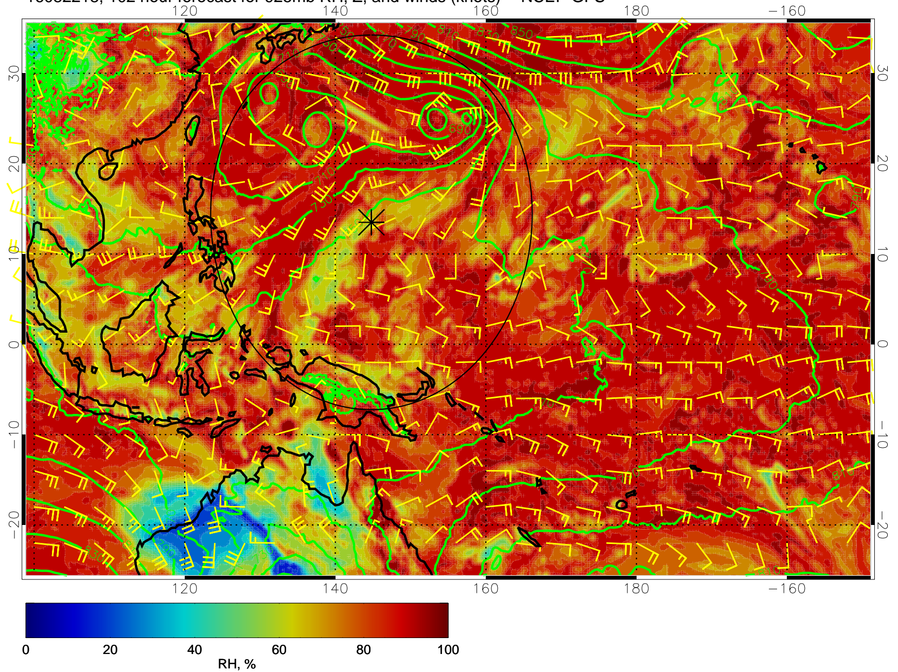
16082218, 102 hour forecast for 925mb RH, Z, and winds (knots) -- NCEP GFS
