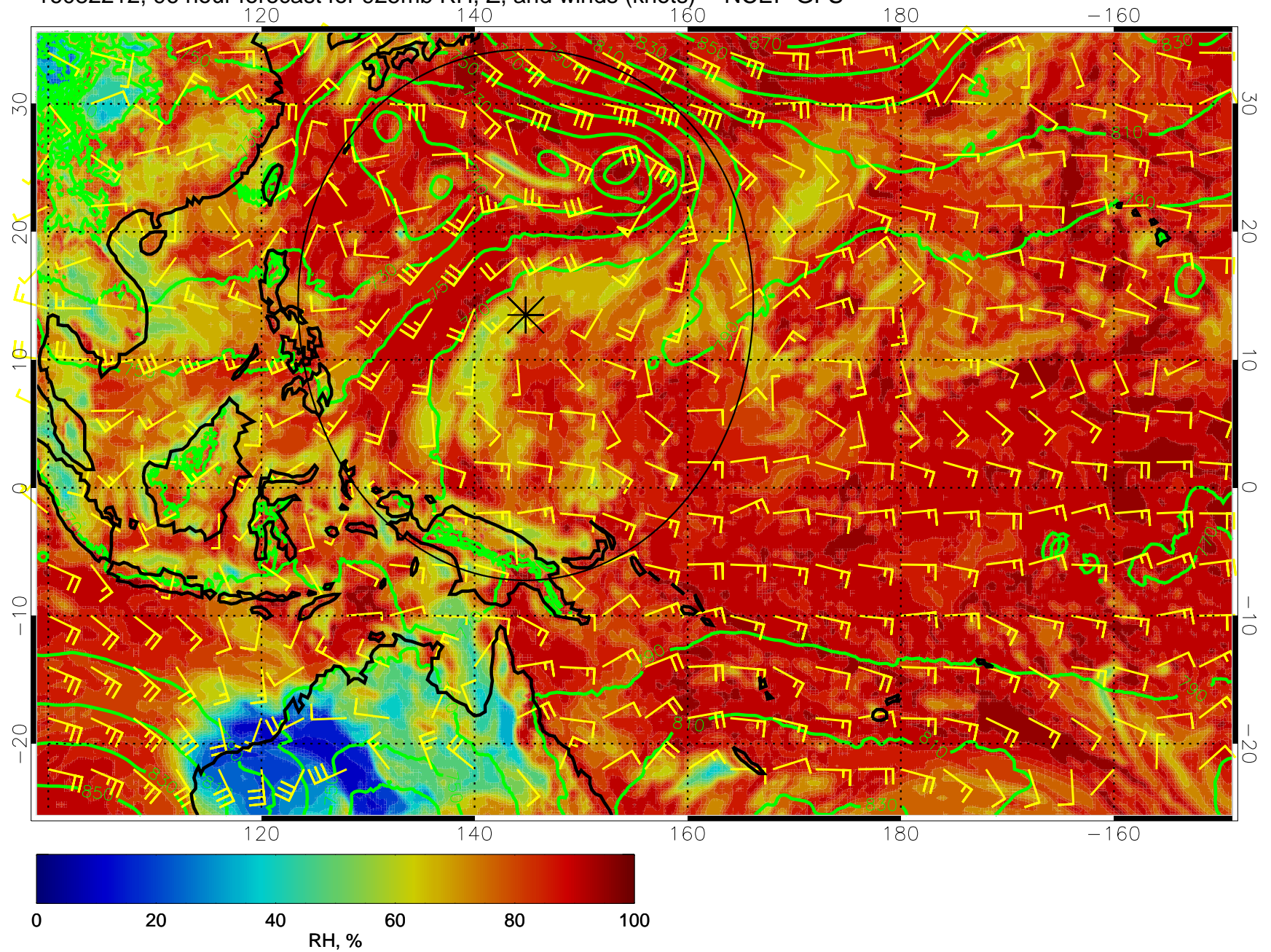
16082212, 96 hour forecast for 925mb RH, Z, and winds (knots) -- NCEP GFS
