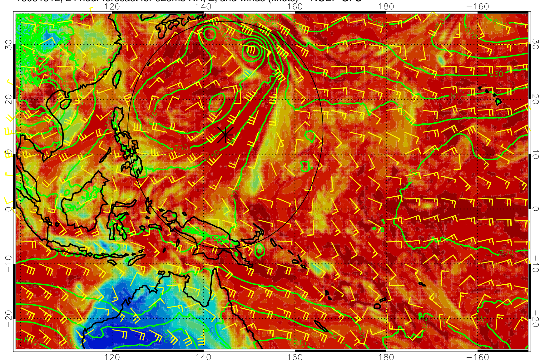
16081912, 24 hour forecast for 925mb RH, Z, and winds (knots) -- NCEP GFS
