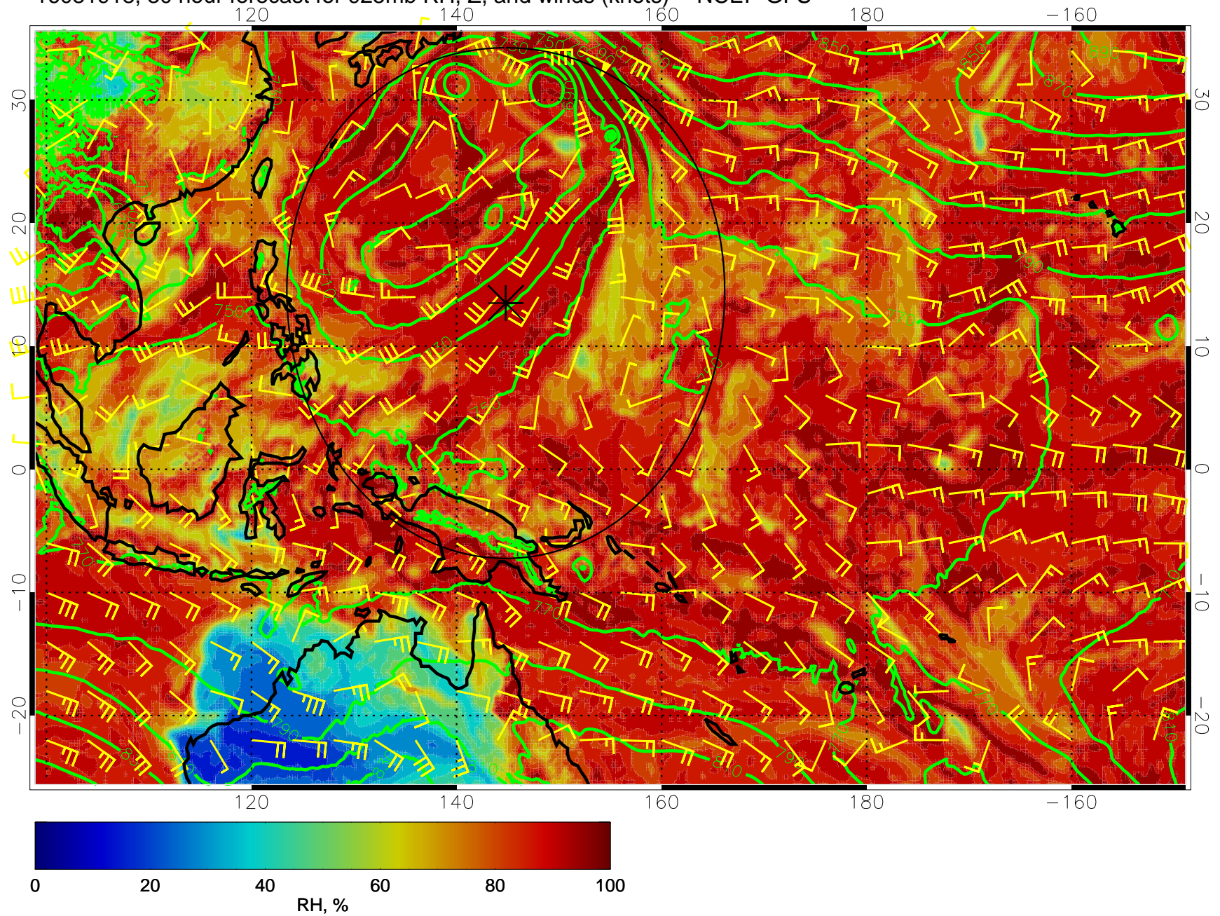
16081918, 30 hour forecast for 925mb RH, Z, and winds (knots) -- NCEP GFS
