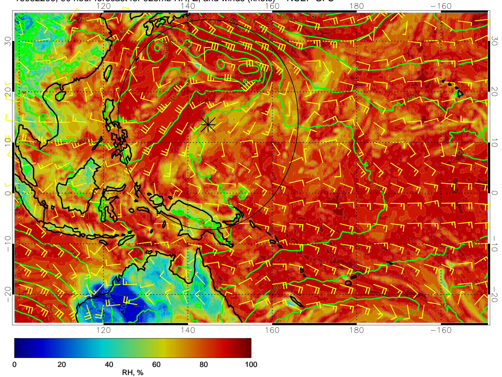
16082206, 90 hour forecast for 925mb RH, Z, and winds (knots) -- NCEP GFS
