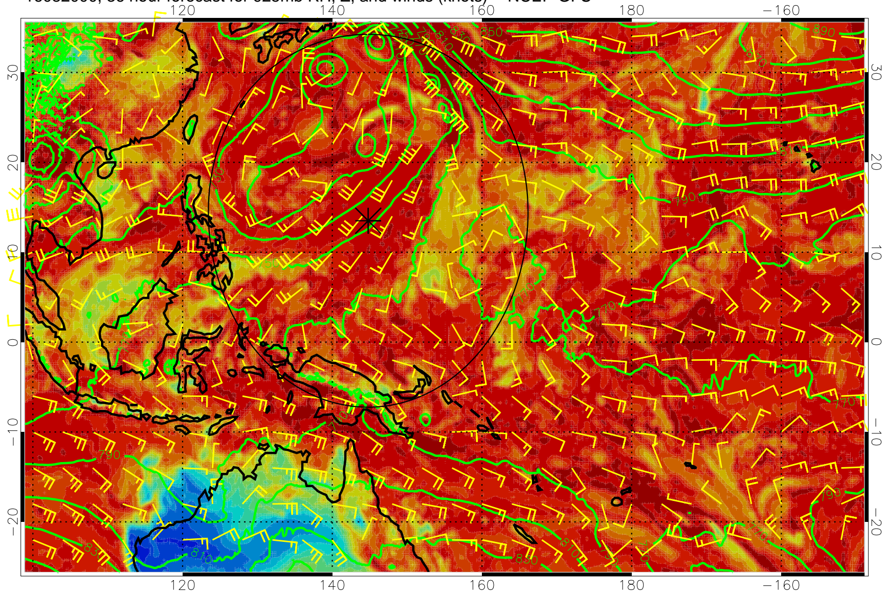
16082000, 36 hour forecast for 925mb RH, Z, and winds (knots) -- NCEP GFS
