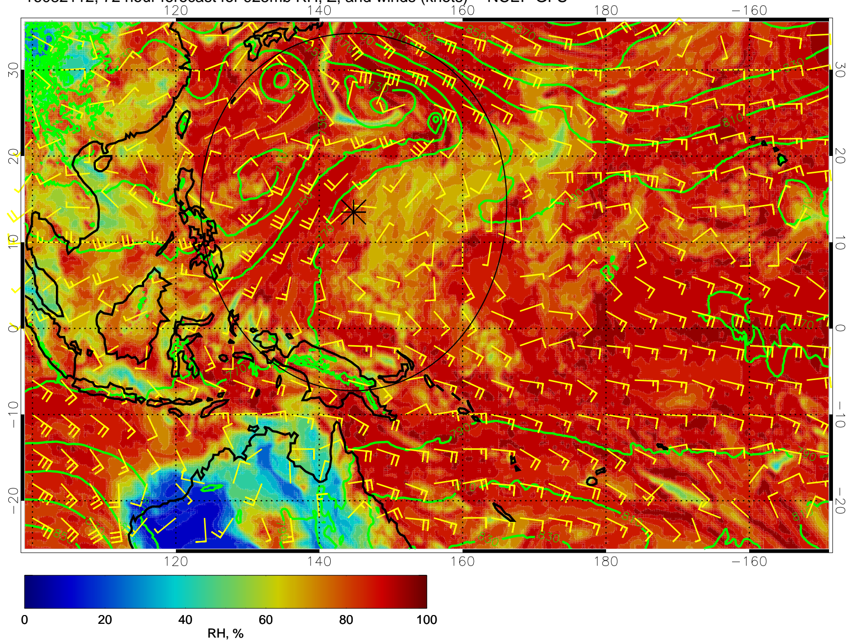
16082112, 72 hour forecast for 925mb RH, Z, and winds (knots) -- NCEP GFS
