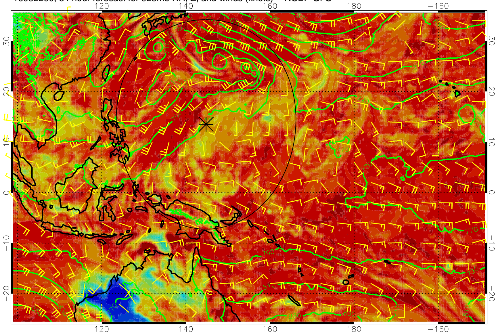
16082200, 84 hour forecast for 925mb RH, Z, and winds (knots) -- NCEP GFS
