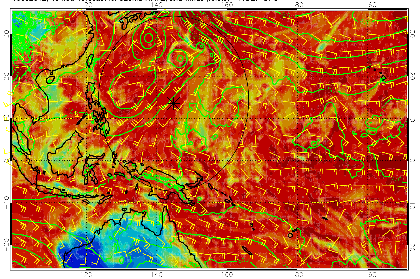
16082012, 48 hour forecast for 925mb RH, Z, and winds (knots) -- NCEP GFS
