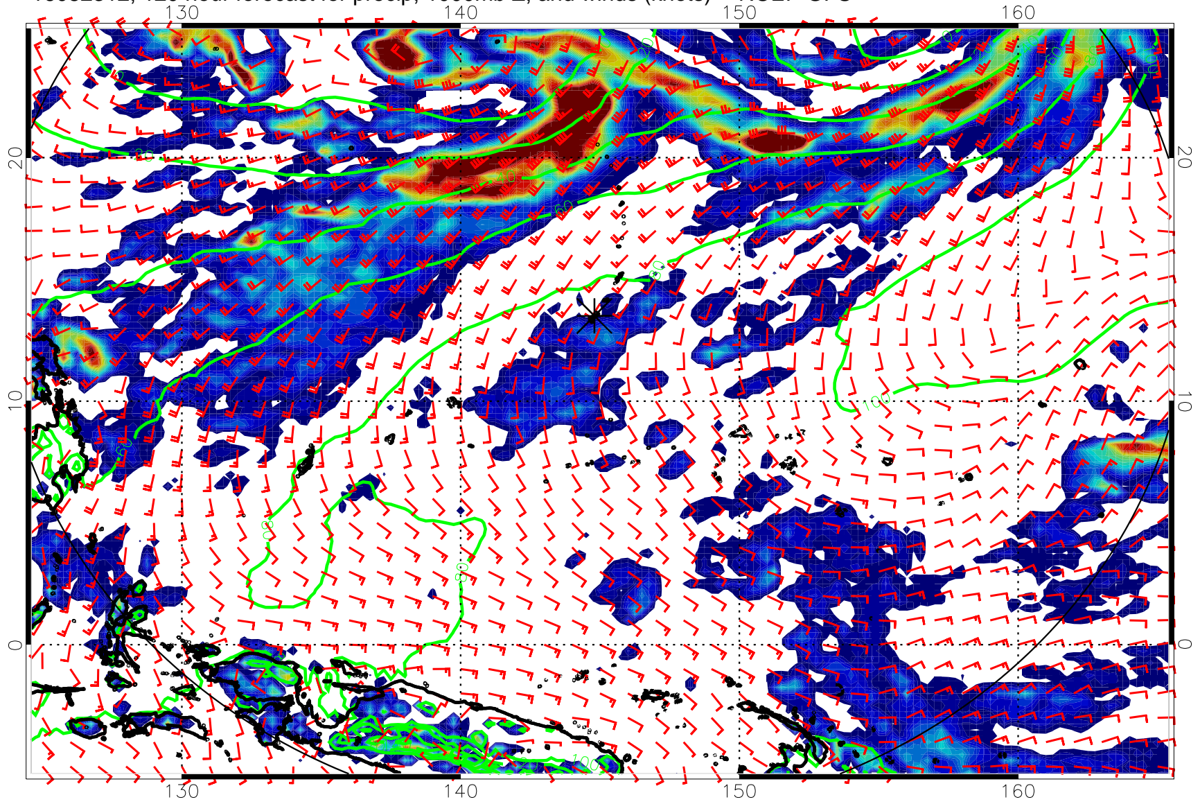
16082312, 120 hour forecast for precip, 1000mb Z, and winds (knots) -- NCEP GFS
