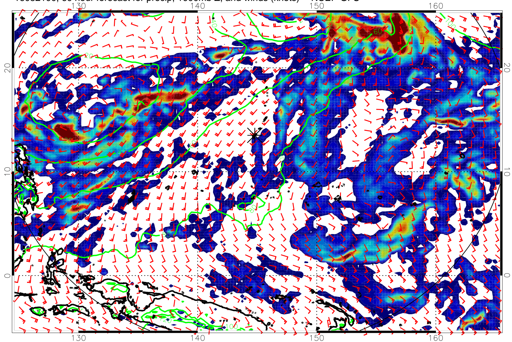
16082100, 60 hour forecast for precip, 1000mb Z, and winds (knots) -- NCEP GFS
