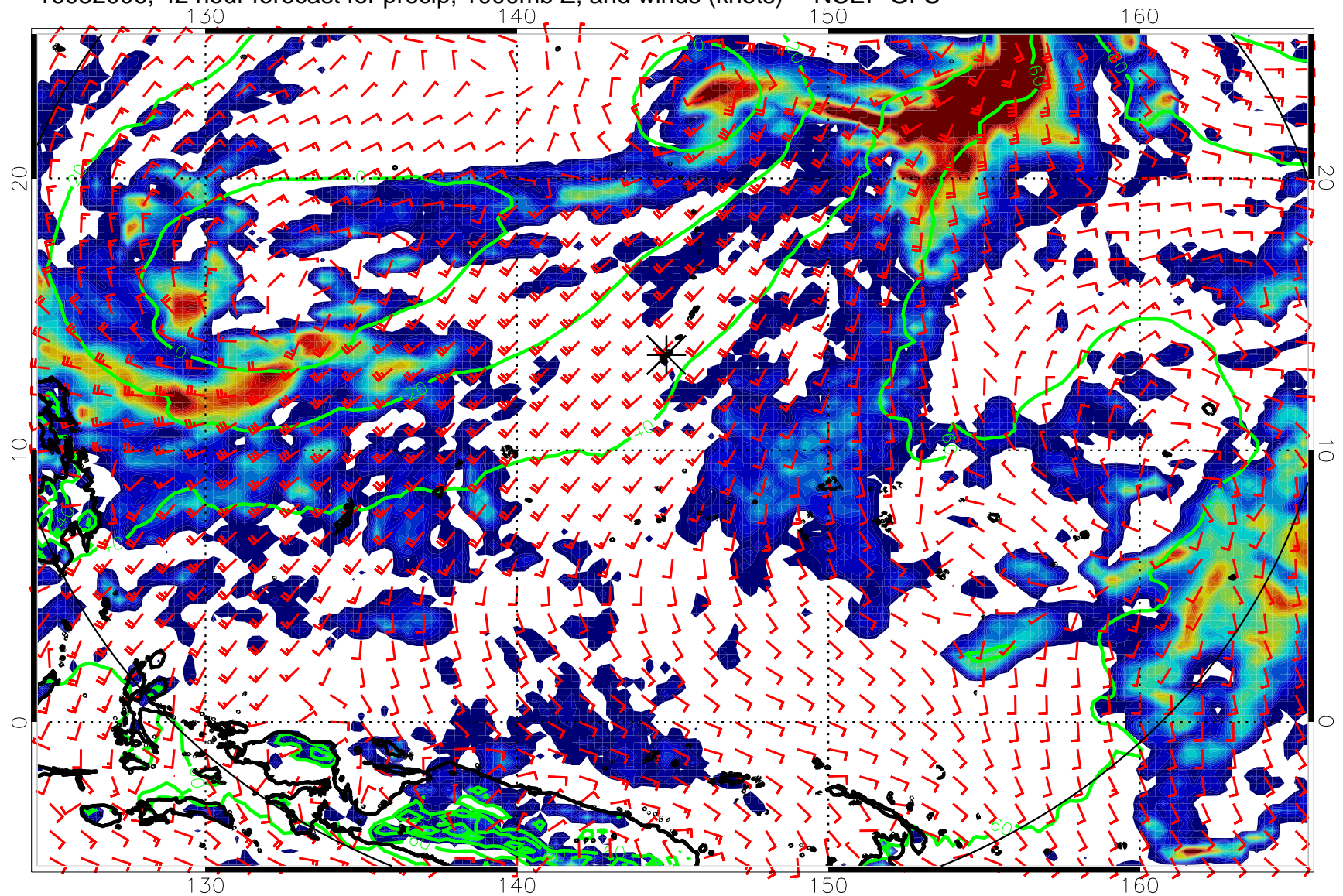
16082006, 42 hour forecast for precip, 1000mb Z, and winds (knots) -- NCEP GFS
