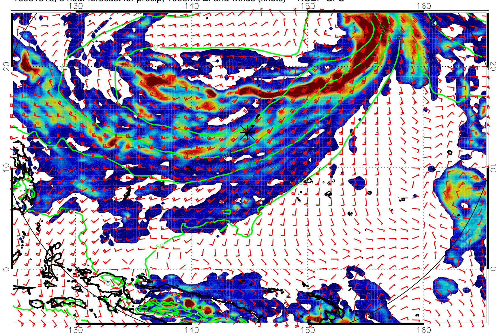
16081818, 6 hour forecast for precip, 1000mb Z, and winds (knots) -- NCEP GFS
