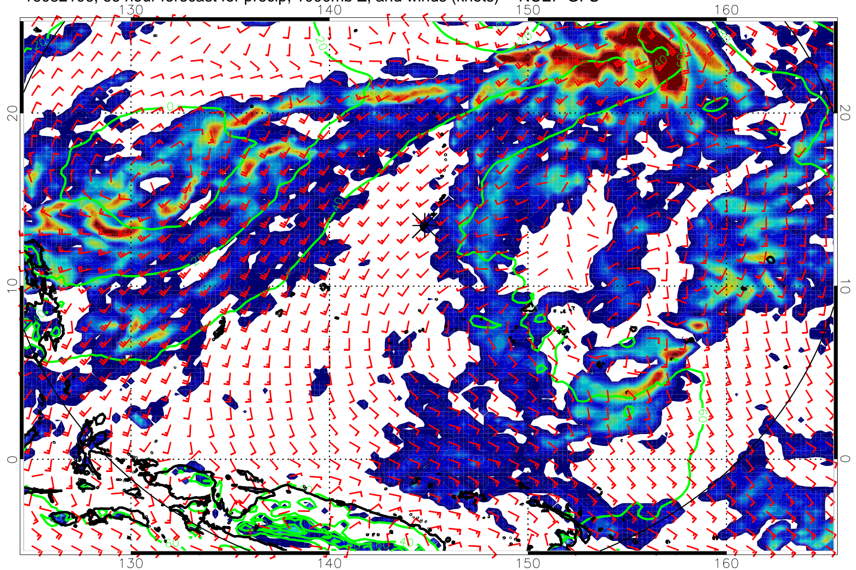
16082106, 66 hour forecast for precip, 1000mb Z, and winds (knots) -- NCEP GFS
