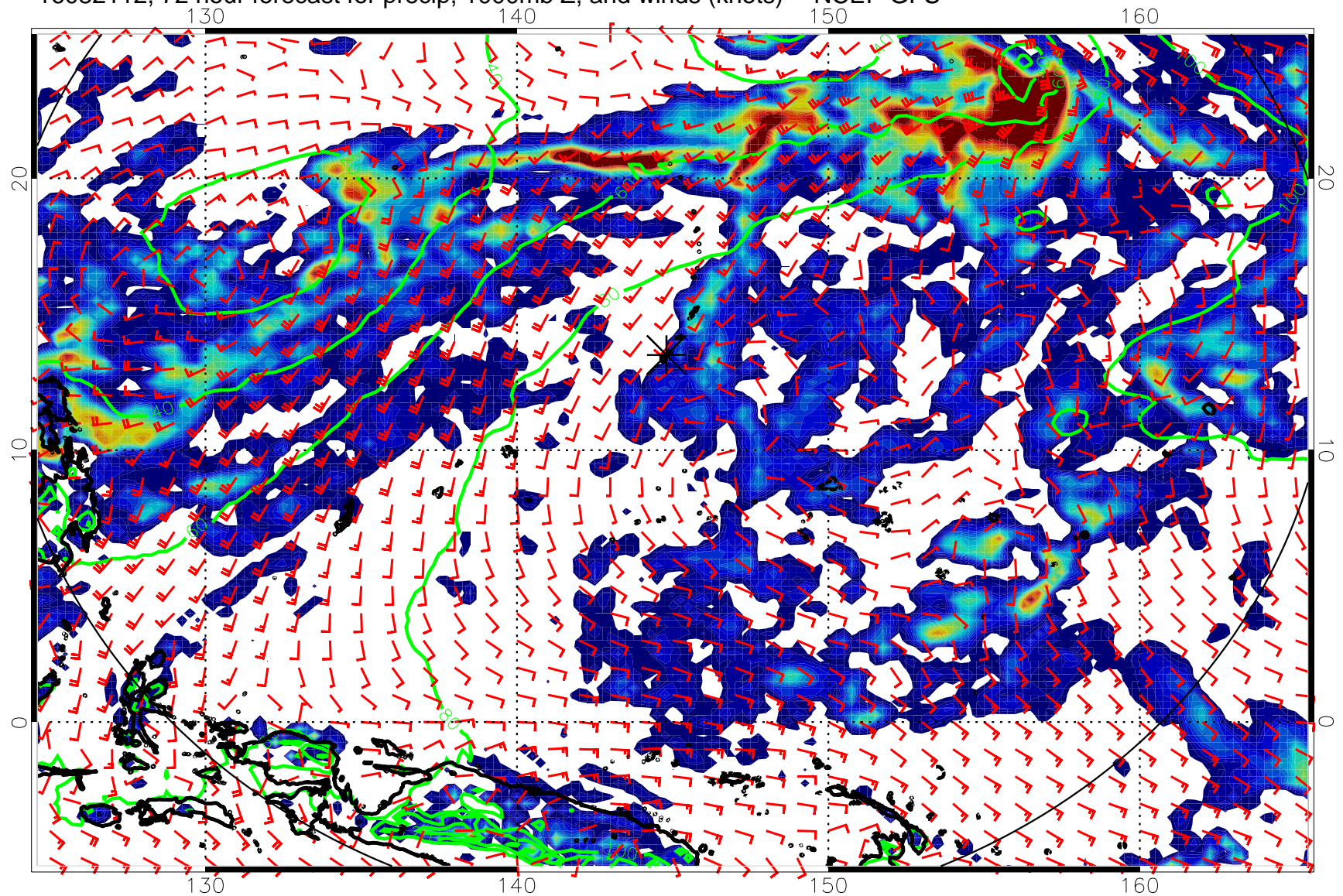
16082112, 72 hour forecast for precip, 1000mb Z, and winds (knots) -- NCEP GFS
