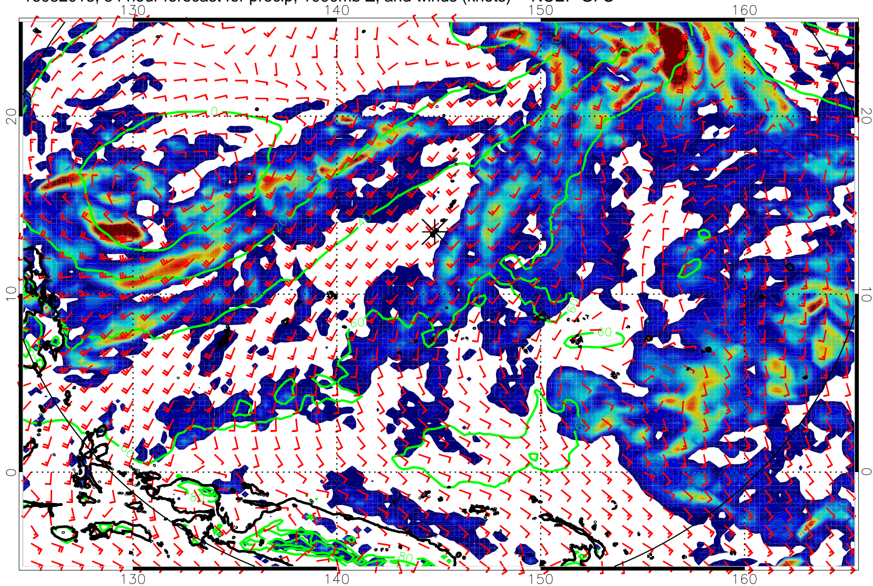
16082018, 54 hour forecast for precip, 1000mb Z, and winds (knots) -- NCEP GFS
