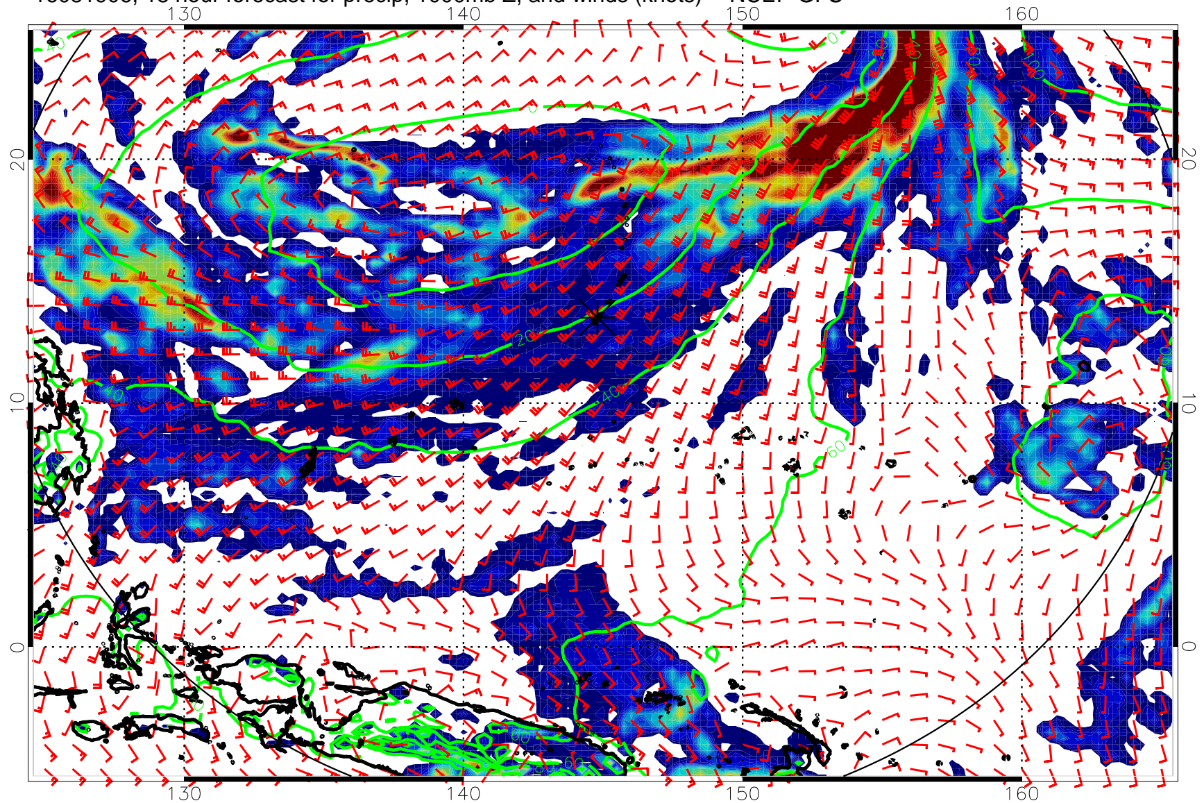
16081906, 18 hour forecast for precip, 1000mb Z, and winds (knots) -- NCEP GFS
