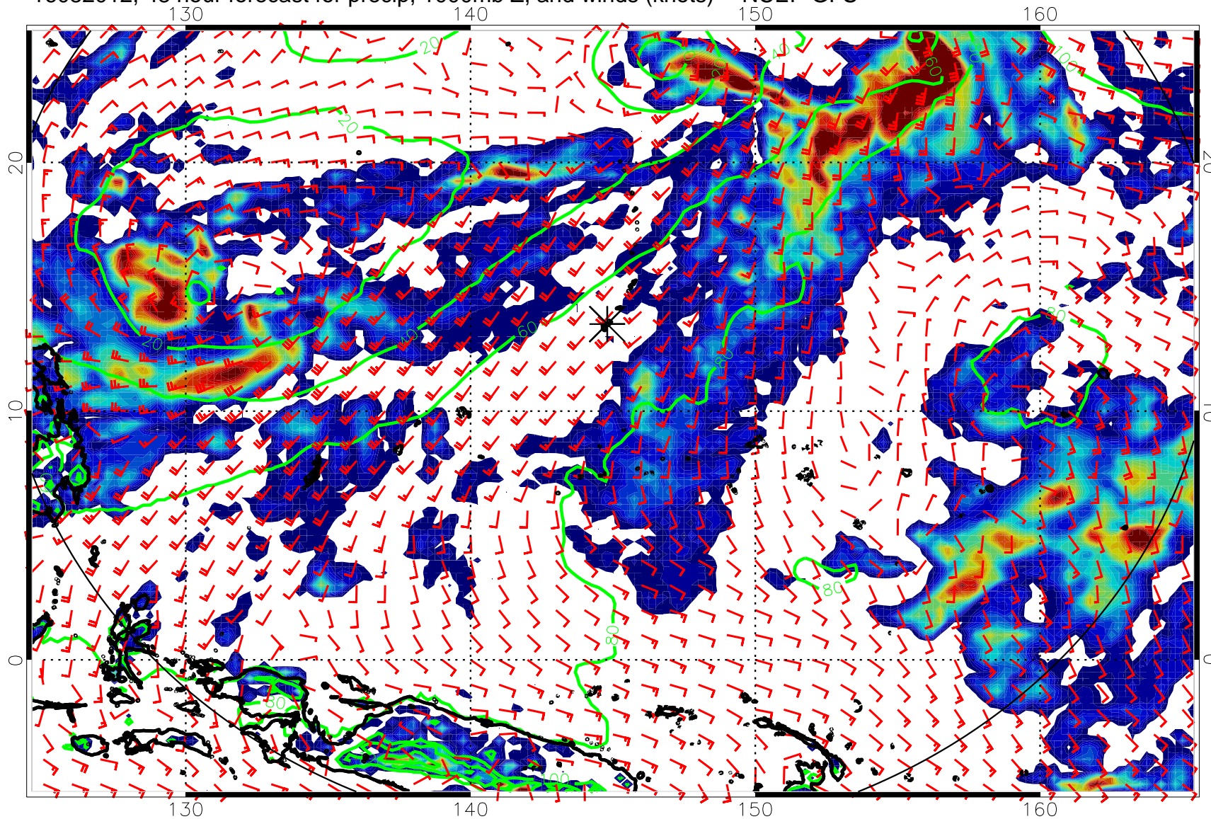
16082012, 48 hour forecast for precip, 1000mb Z, and winds (knots) -- NCEP GFS
