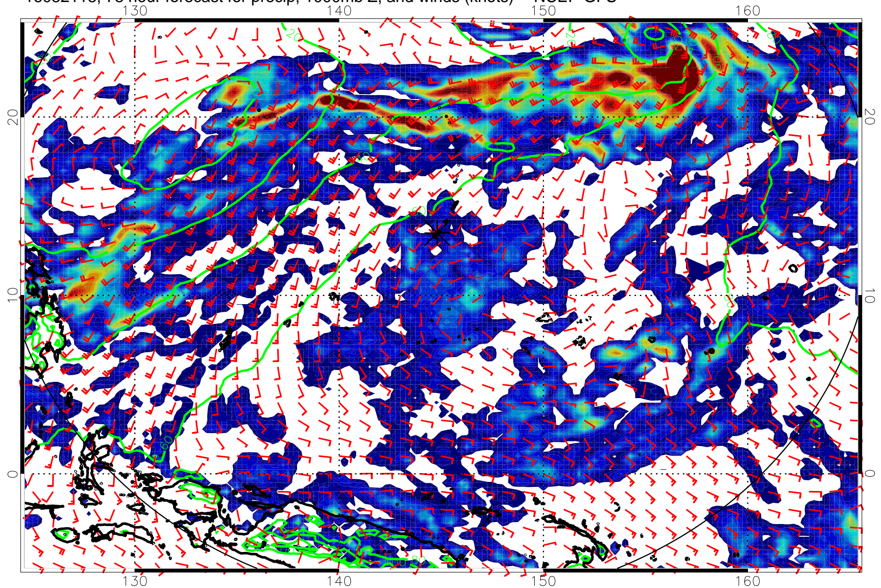
16082118, 78 hour forecast for precip, 1000mb Z, and winds (knots) -- NCEP GFS
