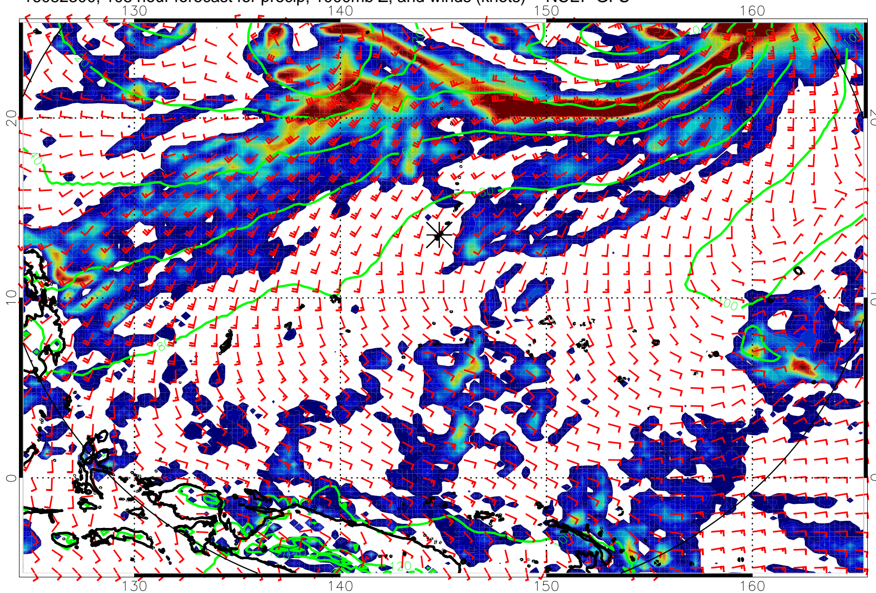
16082300, 108 hour forecast for precip, 1000mb Z, and winds (knots) -- NCEP GFS
