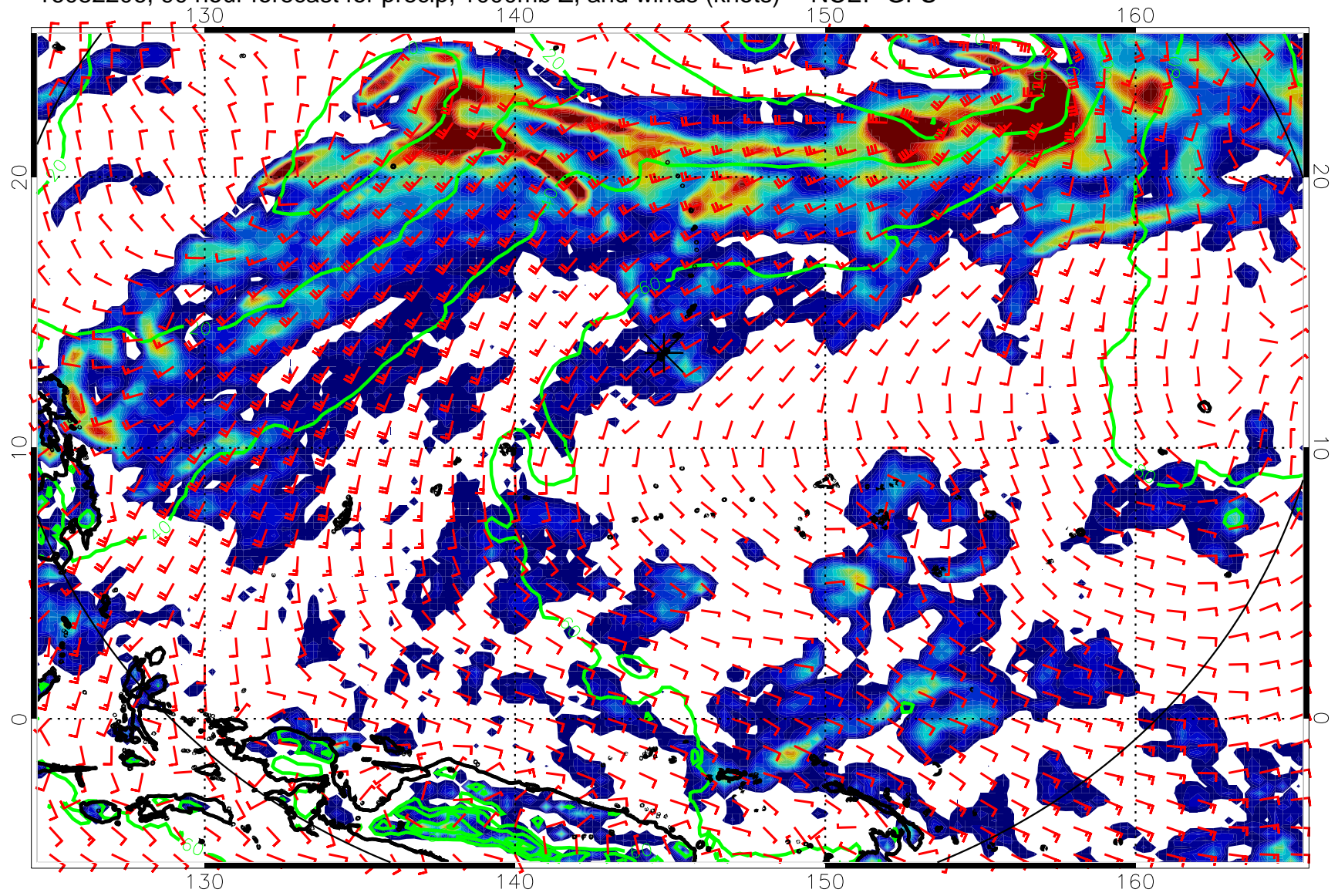
16082206, 90 hour forecast for precip, 1000mb Z, and winds (knots) -- NCEP GFS
