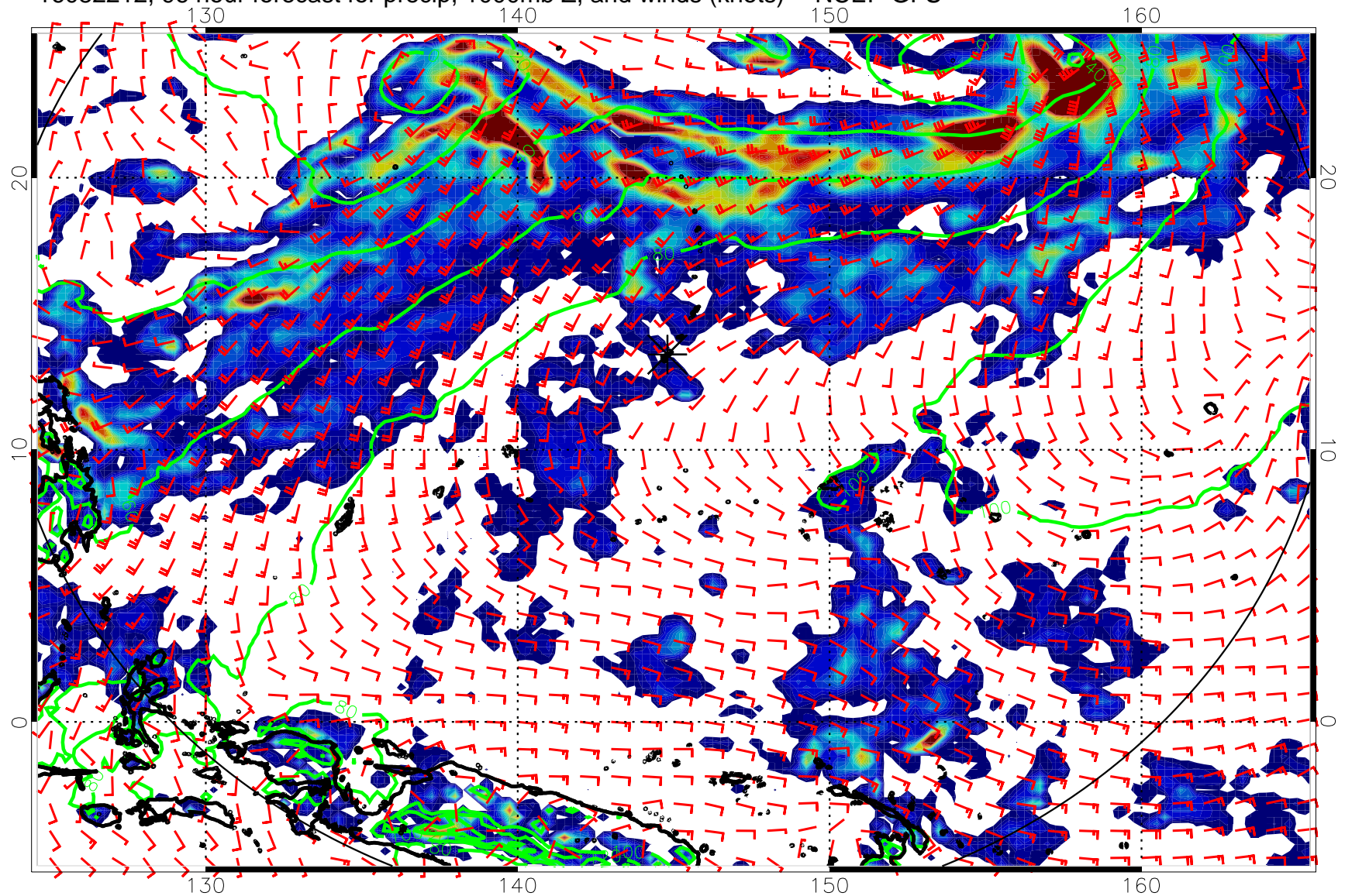
16082212, 96 hour forecast for precip, 1000mb Z, and winds (knots) -- NCEP GFS
