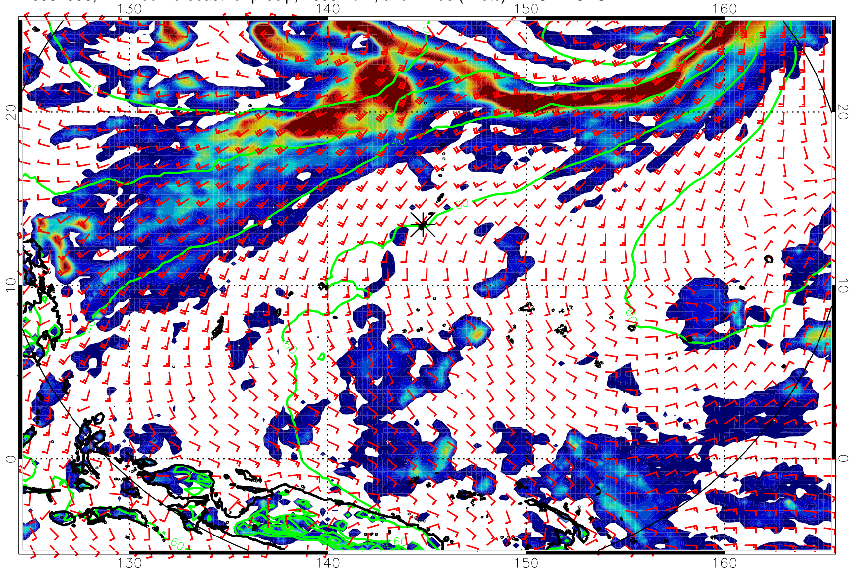
16082306, 114 hour forecast for precip, 1000mb Z, and winds (knots) -- NCEP GFS
