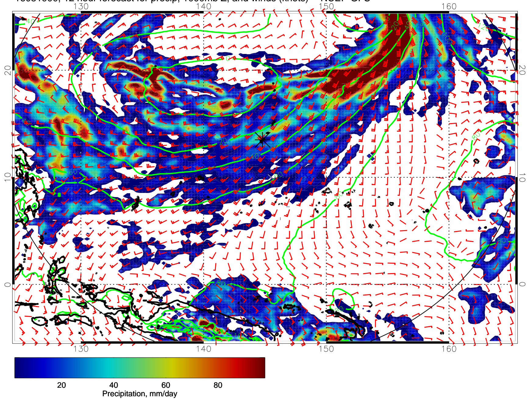
16081900, 12 hour forecast for precip, 1000mb Z, and winds (knots) -- NCEP GFS
