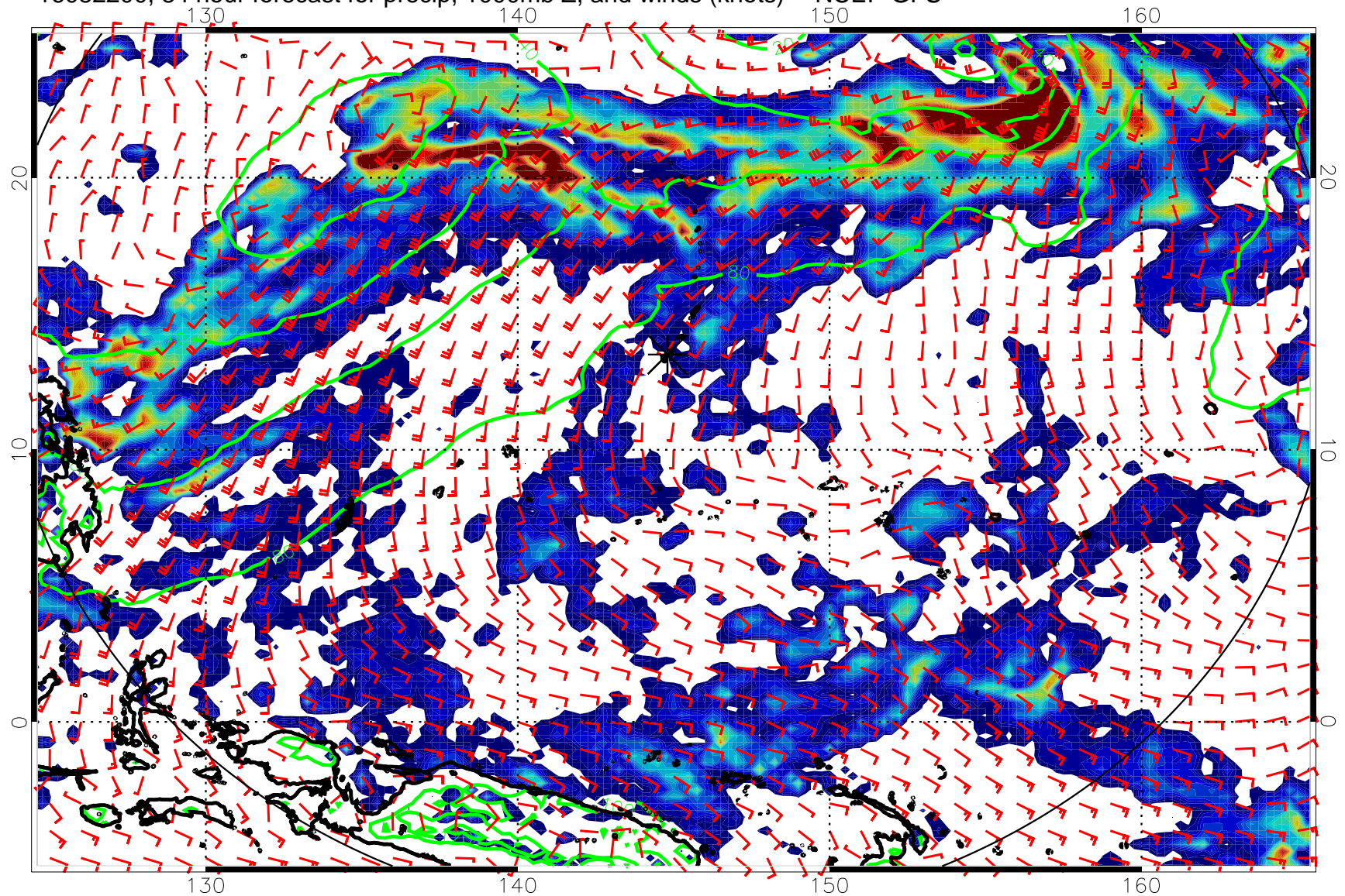
16082200, 84 hour forecast for precip, 1000mb Z, and winds (knots) -- NCEP GFS
