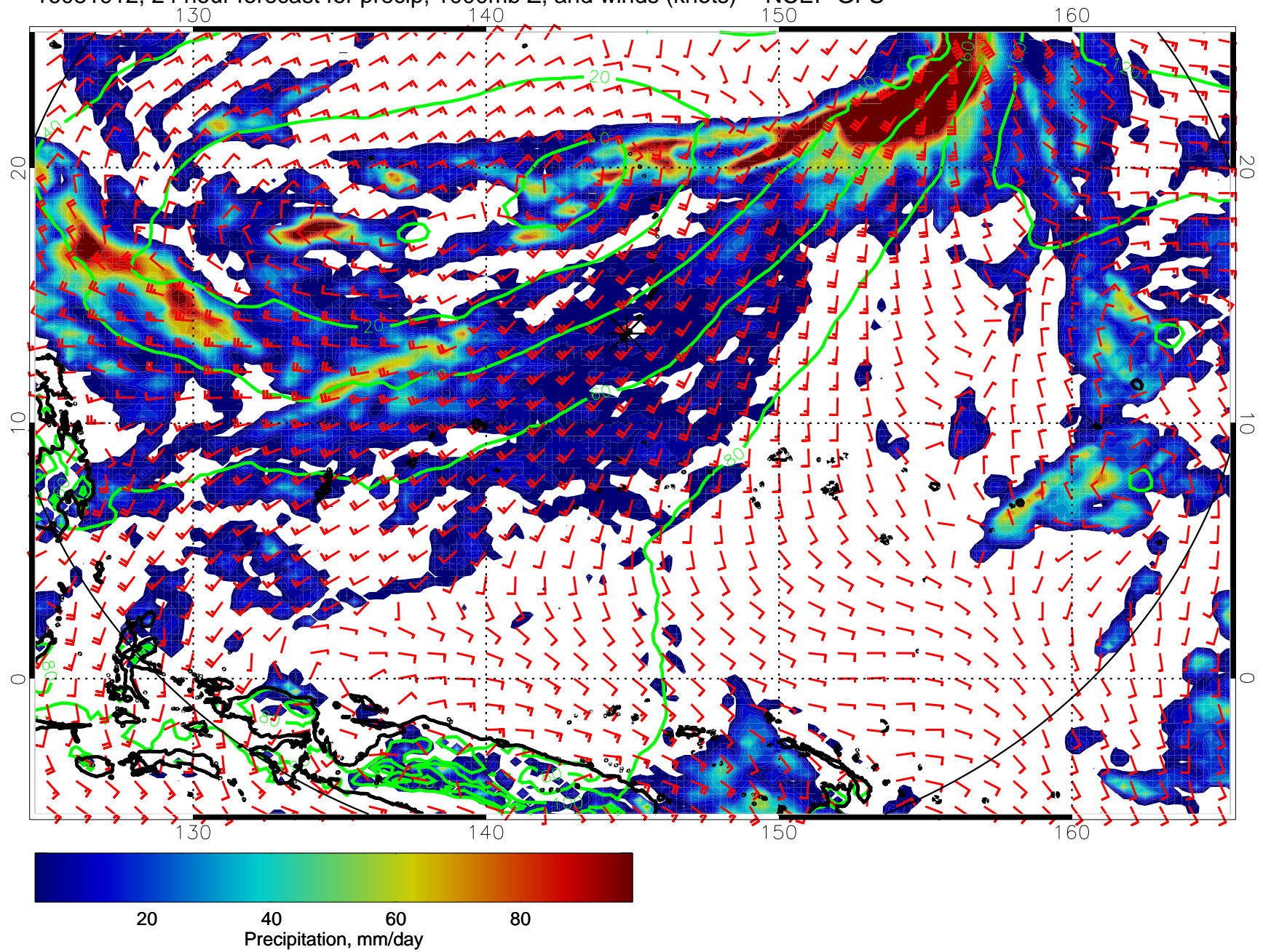
16081912, 24 hour forecast for precip, 1000mb Z, and winds (knots) -- NCEP GFS
