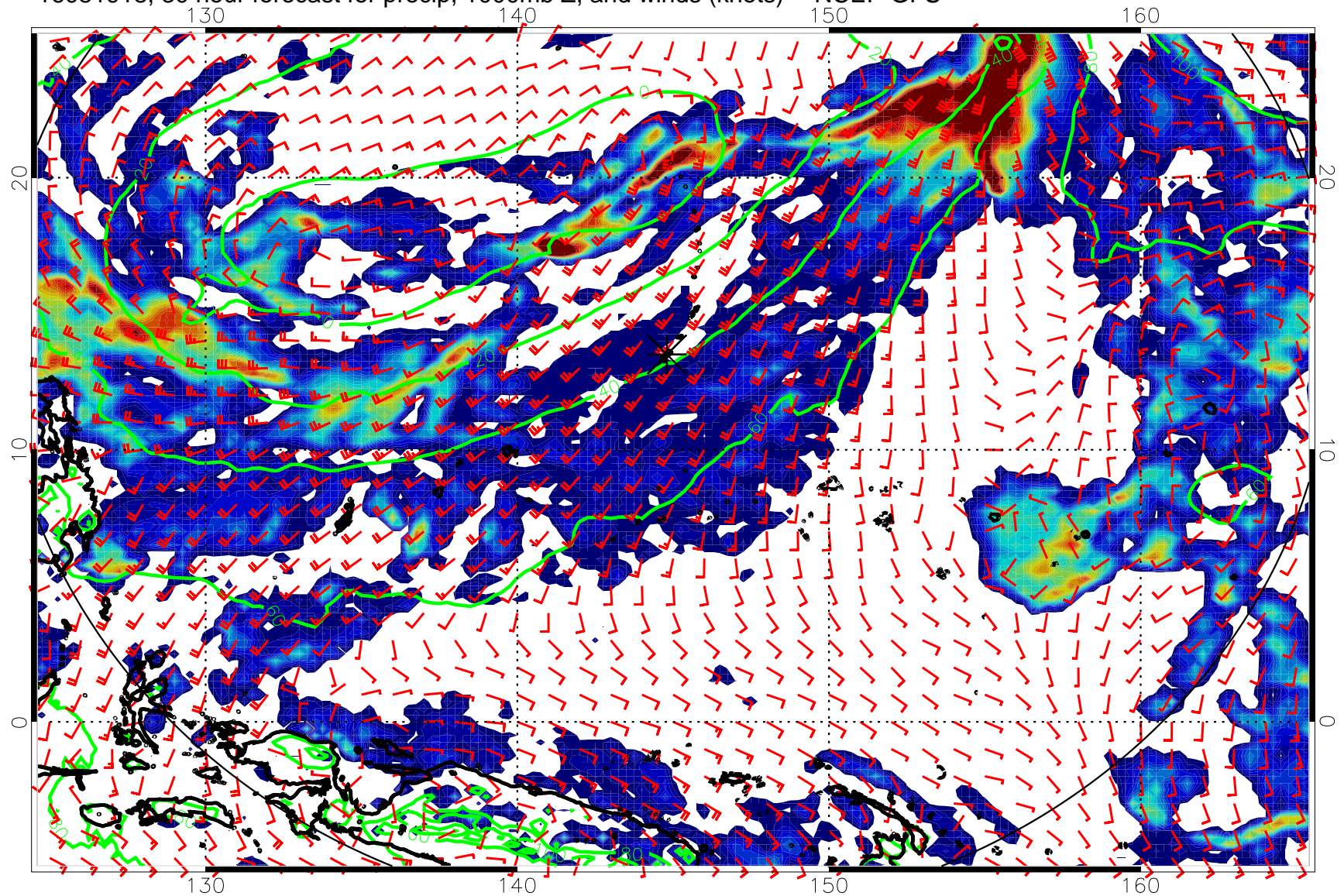
16081918, 30 hour forecast for precip, 1000mb Z, and winds (knots) -- NCEP GFS
