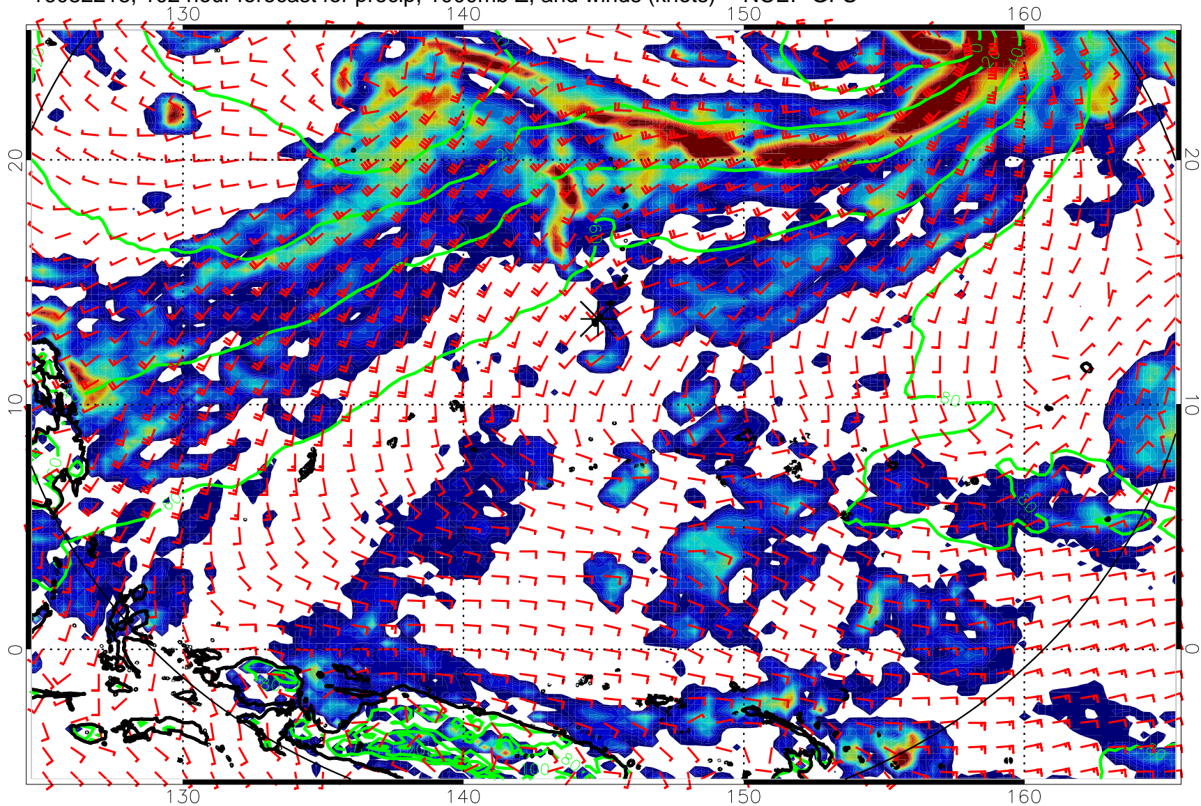
16082218, 102 hour forecast for precip, 1000mb Z, and winds (knots) -- NCEP GFS
