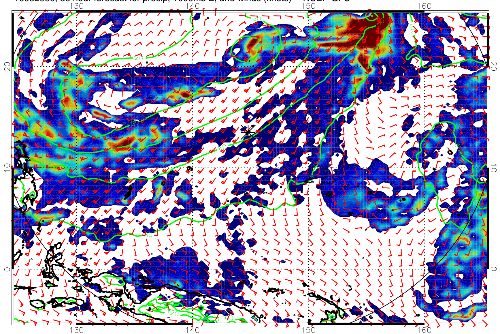
16082000, 36 hour forecast for precip, 1000mb Z, and winds (knots) -- NCEP GFS
