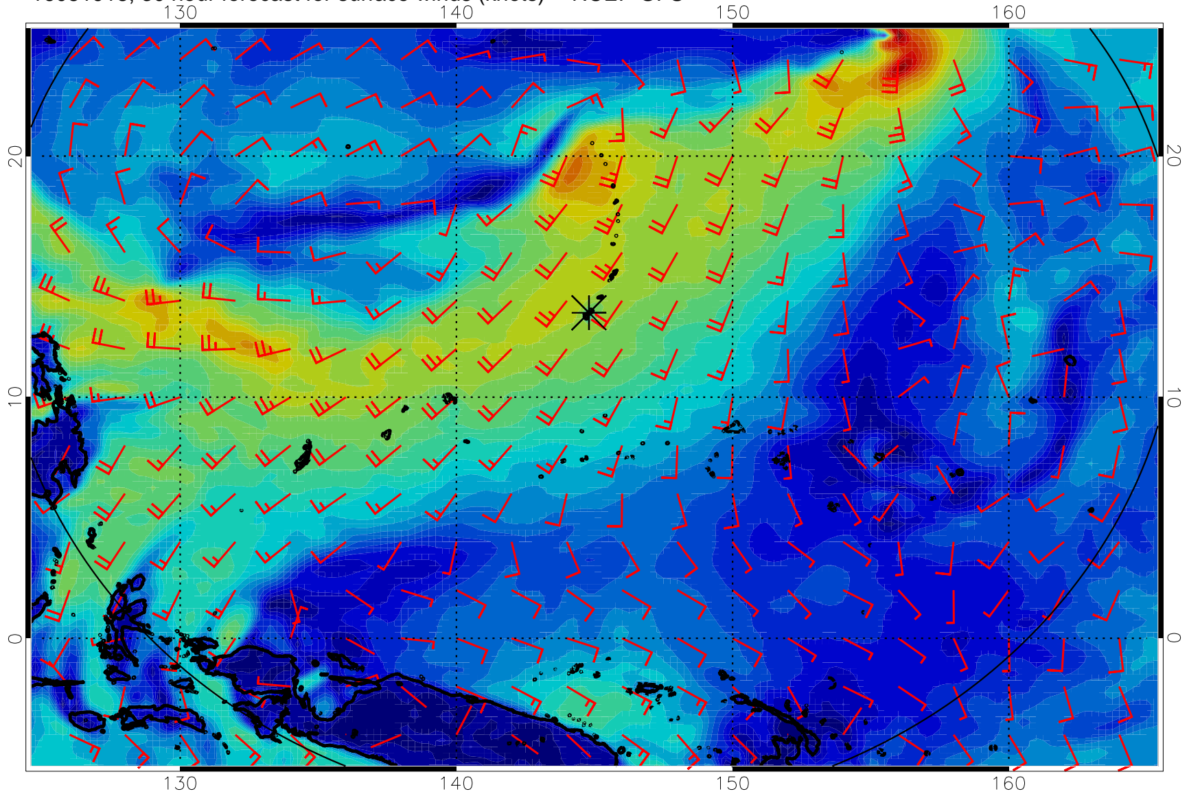
16081918, 30 hour forecast for surface winds (knots) -- NCEP GFS
