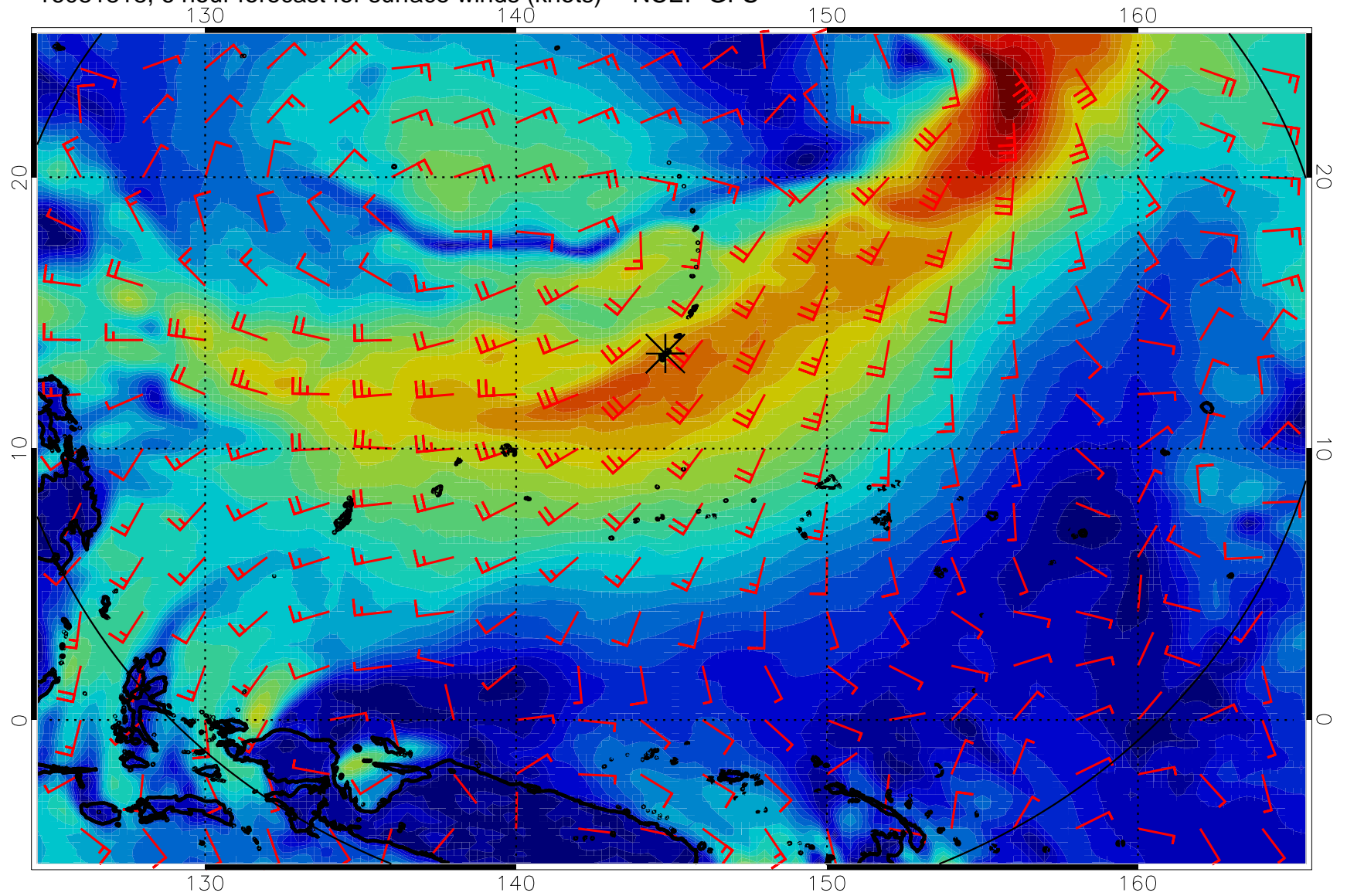
16081818, 6 hour forecast for surface winds (knots) -- NCEP GFS
