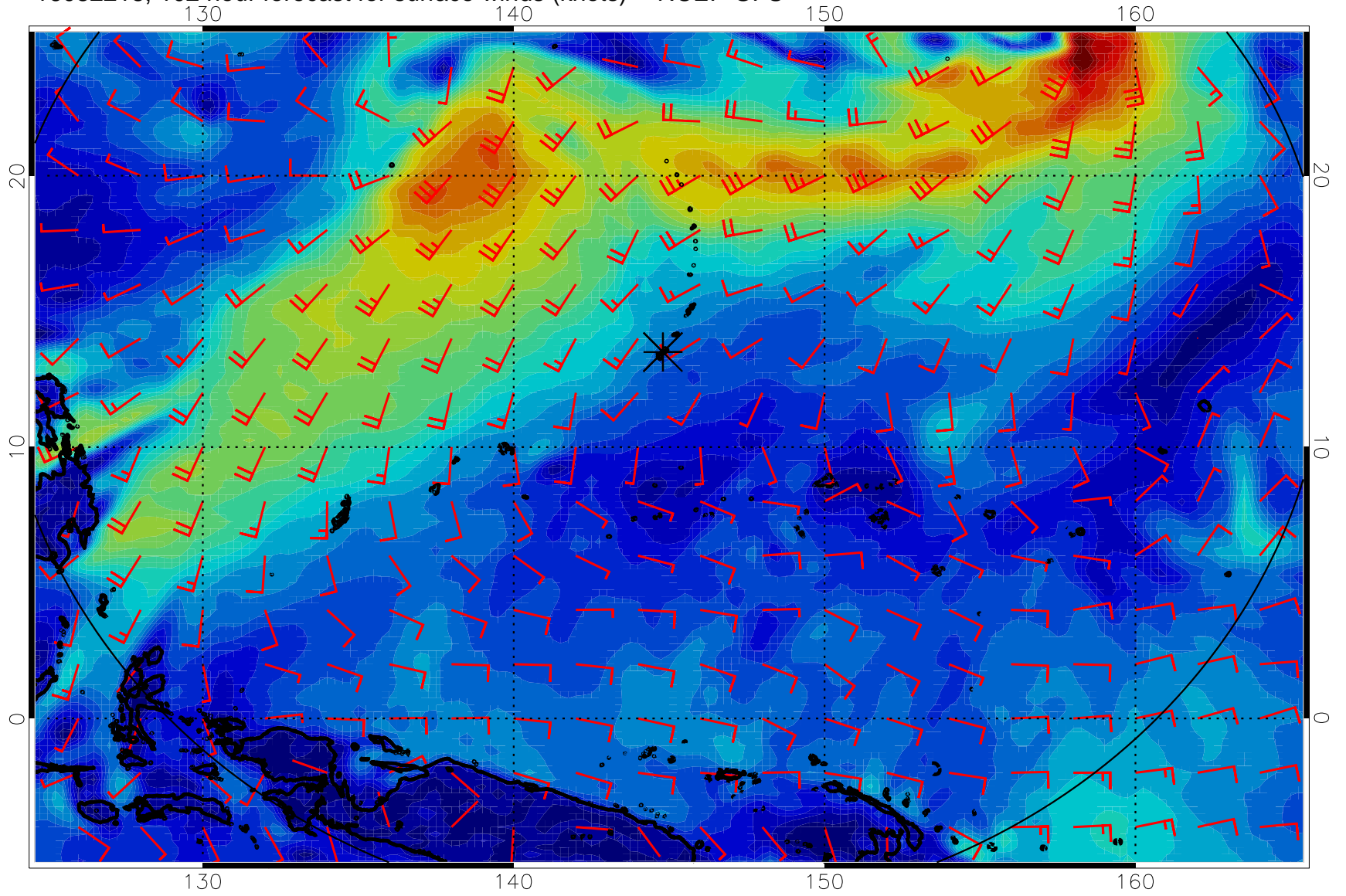
16082218, 102 hour forecast for surface winds (knots) -- NCEP GFS
