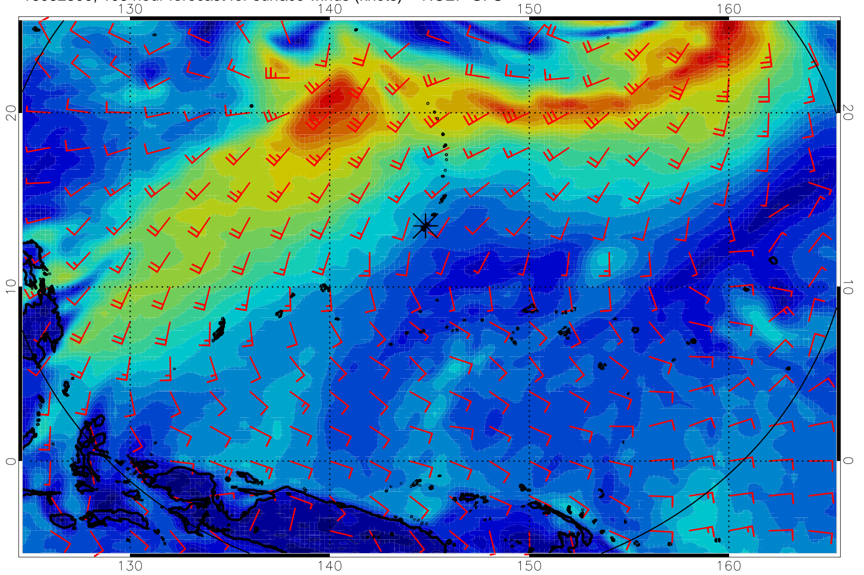
16082300, 108 hour forecast for surface winds (knots) -- NCEP GFS
