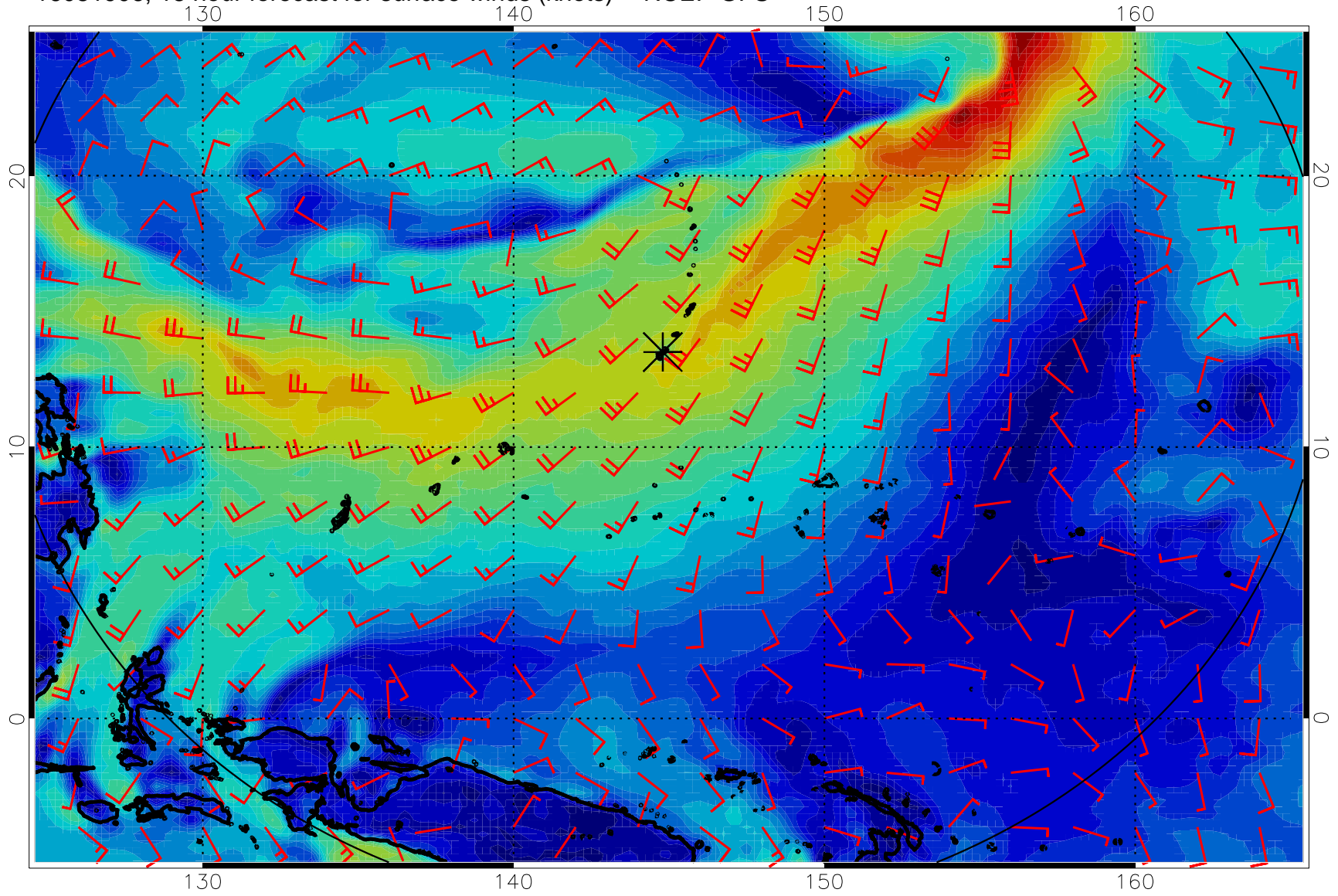
16081906, 18 hour forecast for surface winds (knots) -- NCEP GFS
