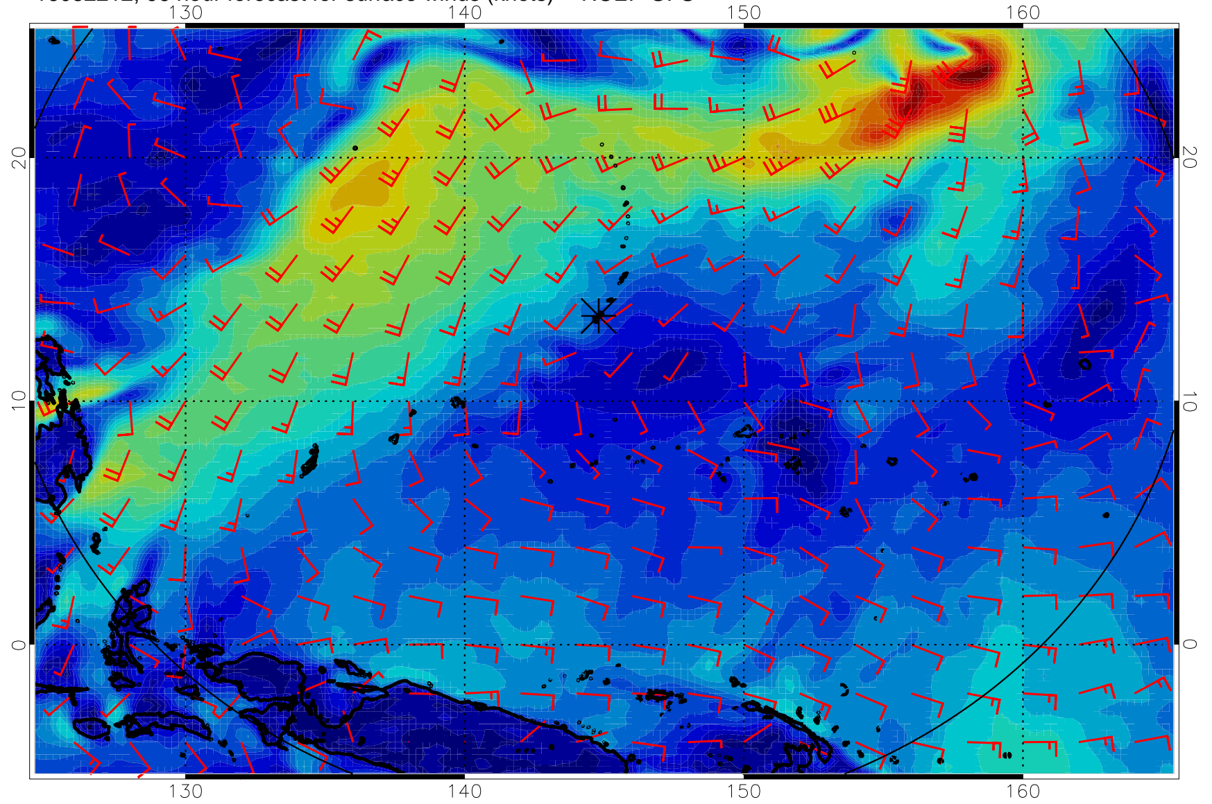
16082212, 96 hour forecast for surface winds (knots) -- NCEP GFS
