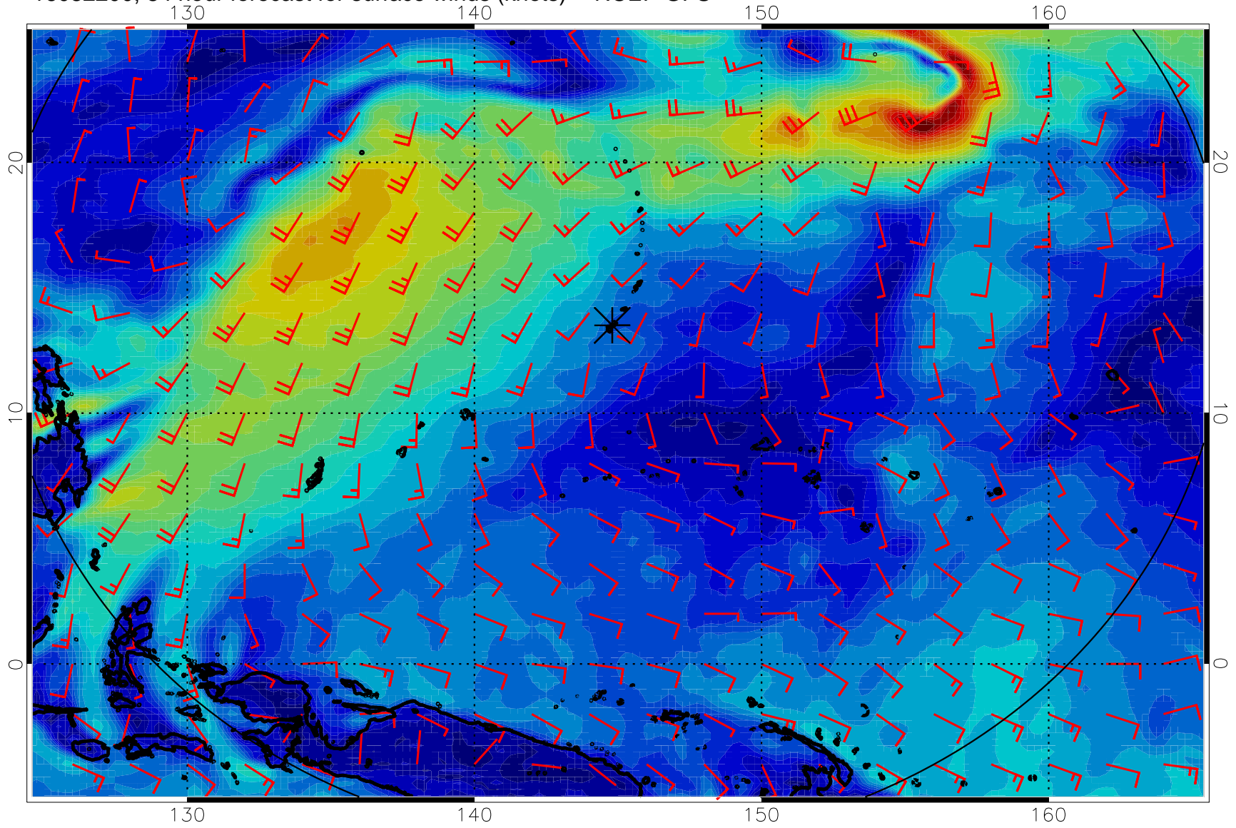
16082200, 84 hour forecast for surface winds (knots) -- NCEP GFS
