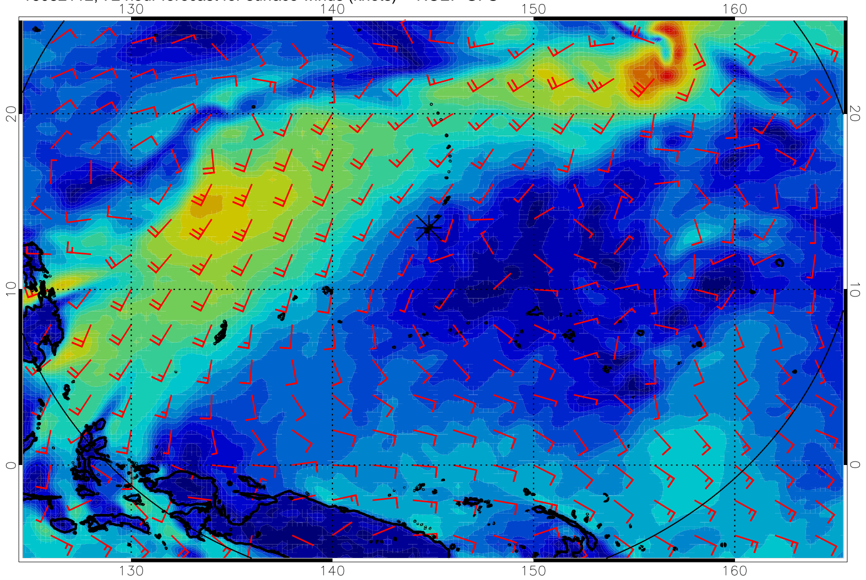
16082112, 72 hour forecast for surface winds (knots) -- NCEP GFS
