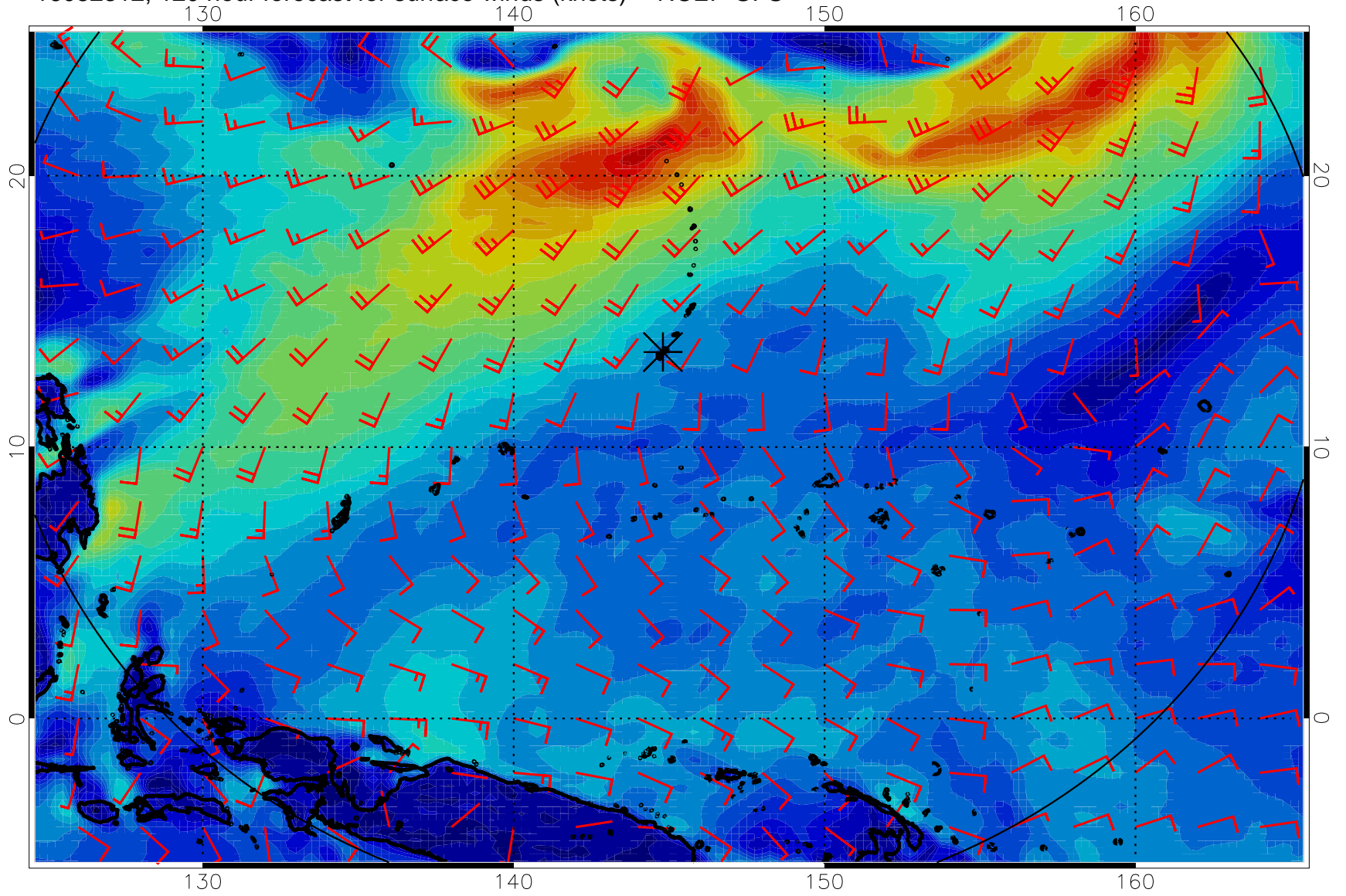
16082312, 120 hour forecast for surface winds (knots) -- NCEP GFS
