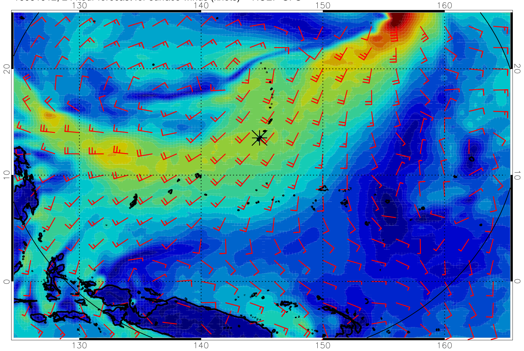
16081912, 24 hour forecast for surface winds (knots) -- NCEP GFS
