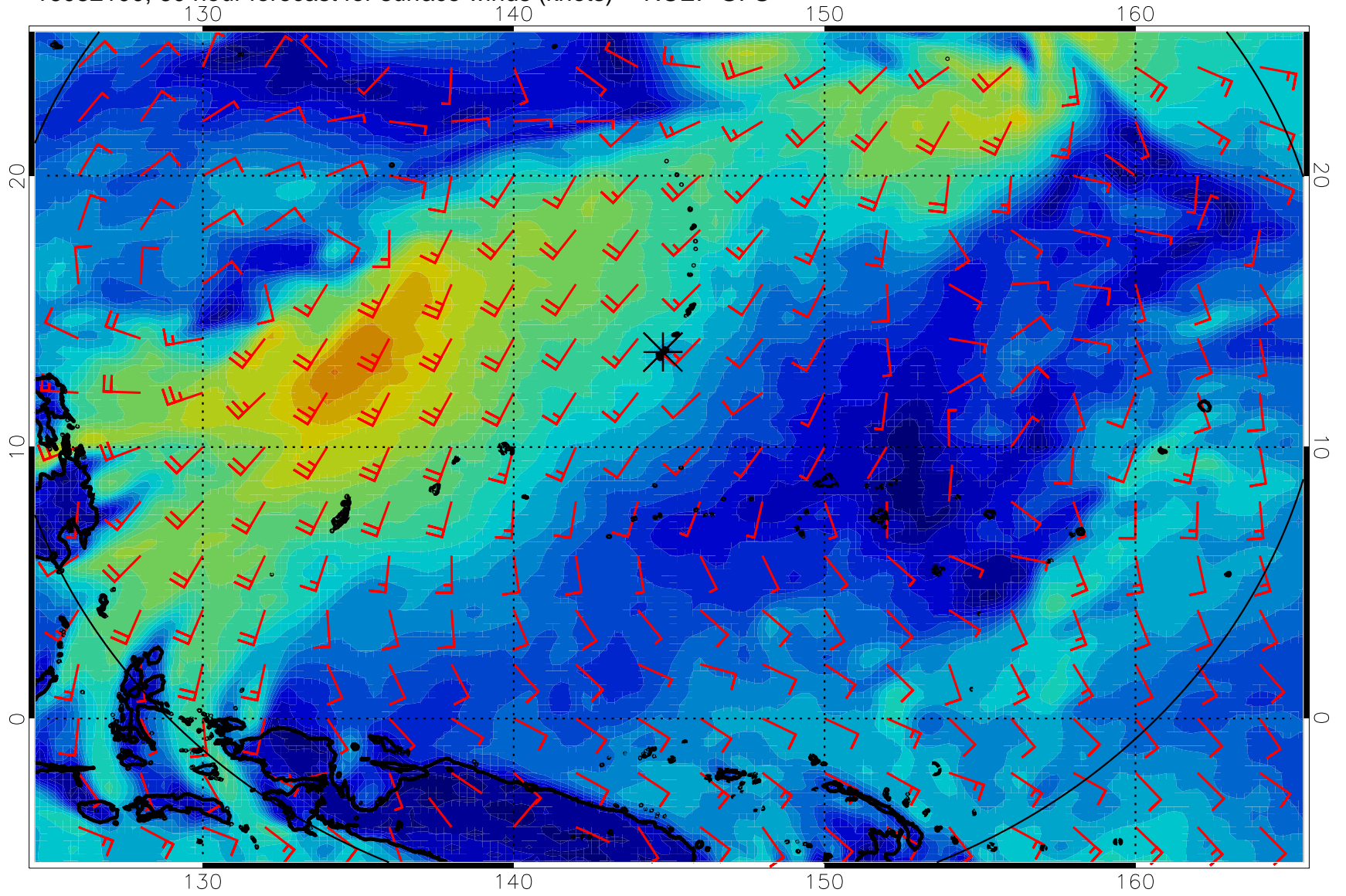
16082100, 60 hour forecast for surface winds (knots) -- NCEP GFS
