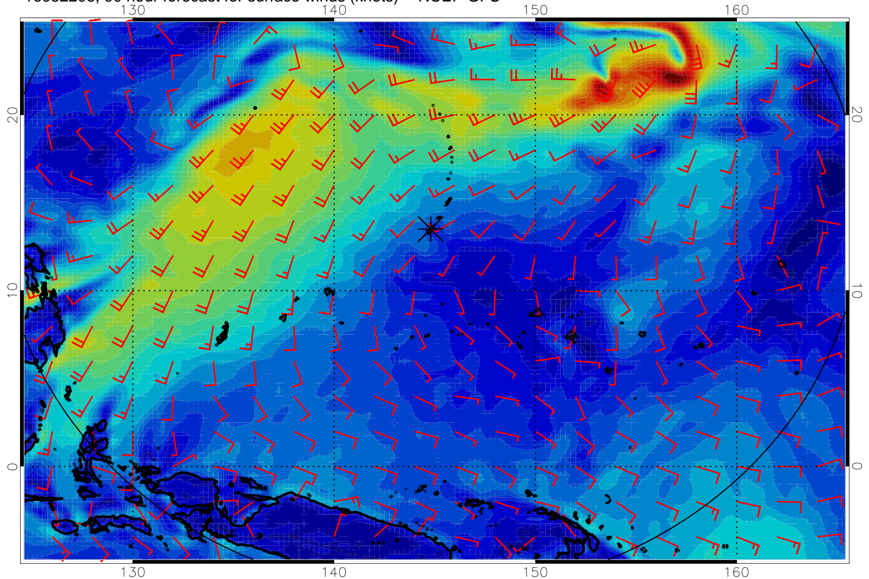
16082206, 90 hour forecast for surface winds (knots) -- NCEP GFS
