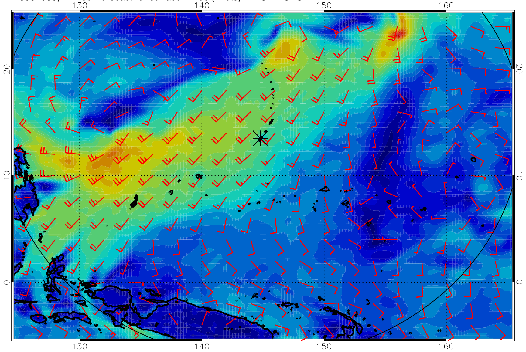
16082006, 42 hour forecast for surface winds (knots) -- NCEP GFS
