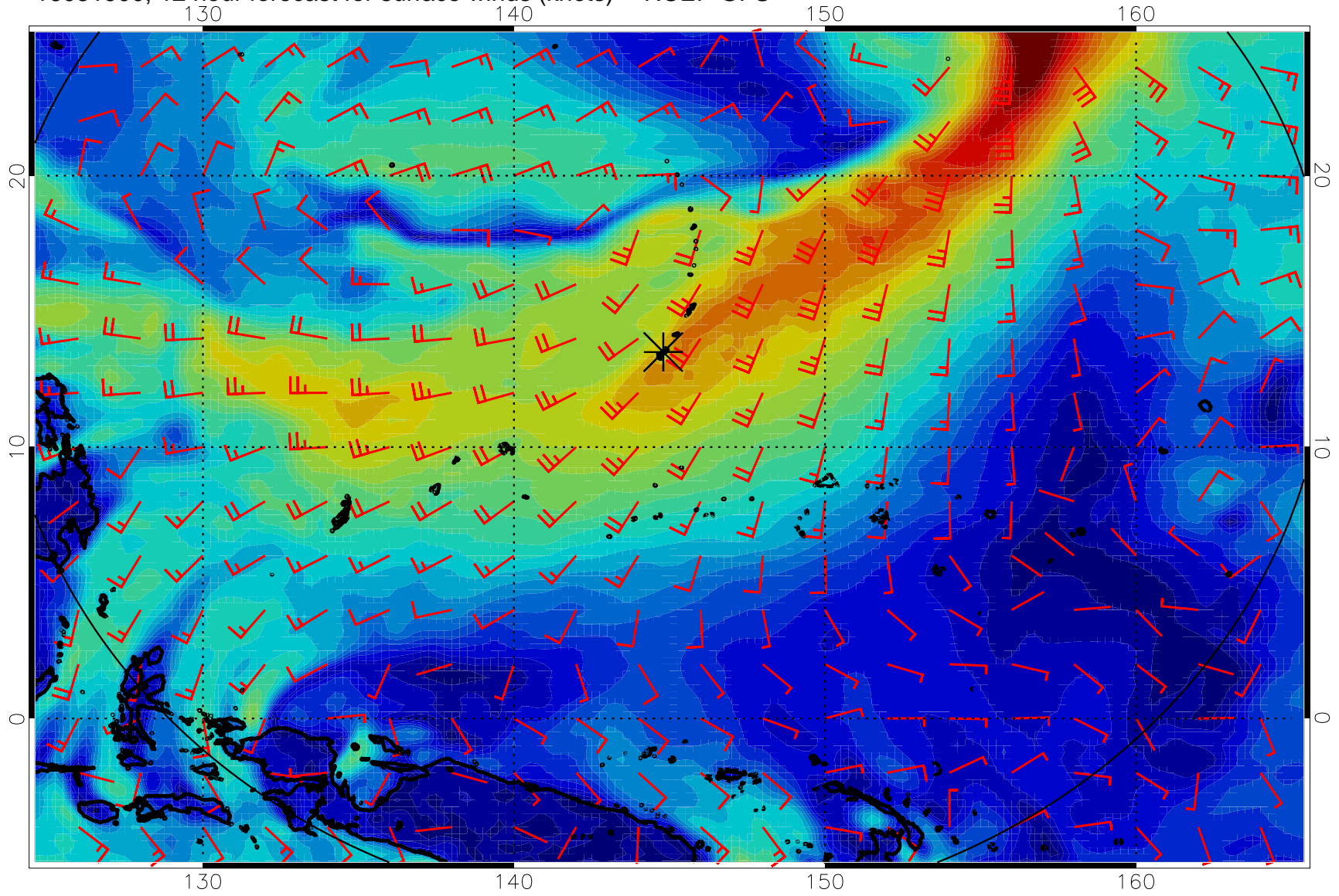
16081900, 12 hour forecast for surface winds (knots) -- NCEP GFS
