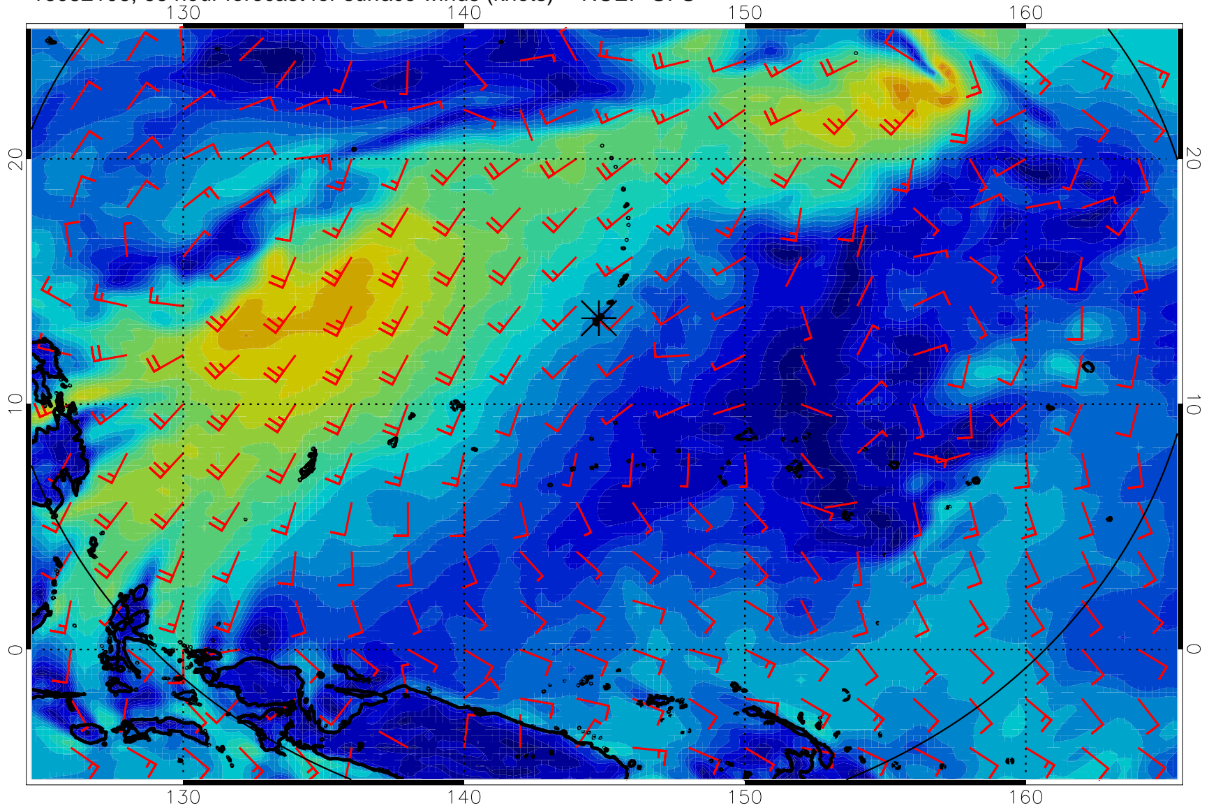
16082106, 66 hour forecast for surface winds (knots) -- NCEP GFS
