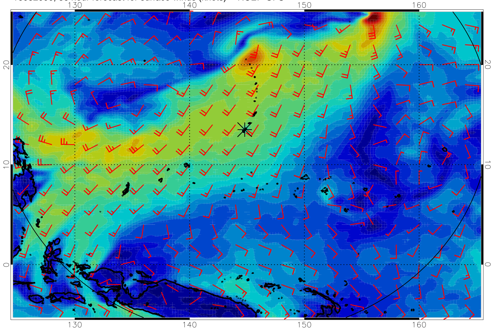
16082000, 36 hour forecast for surface winds (knots) -- NCEP GFS
