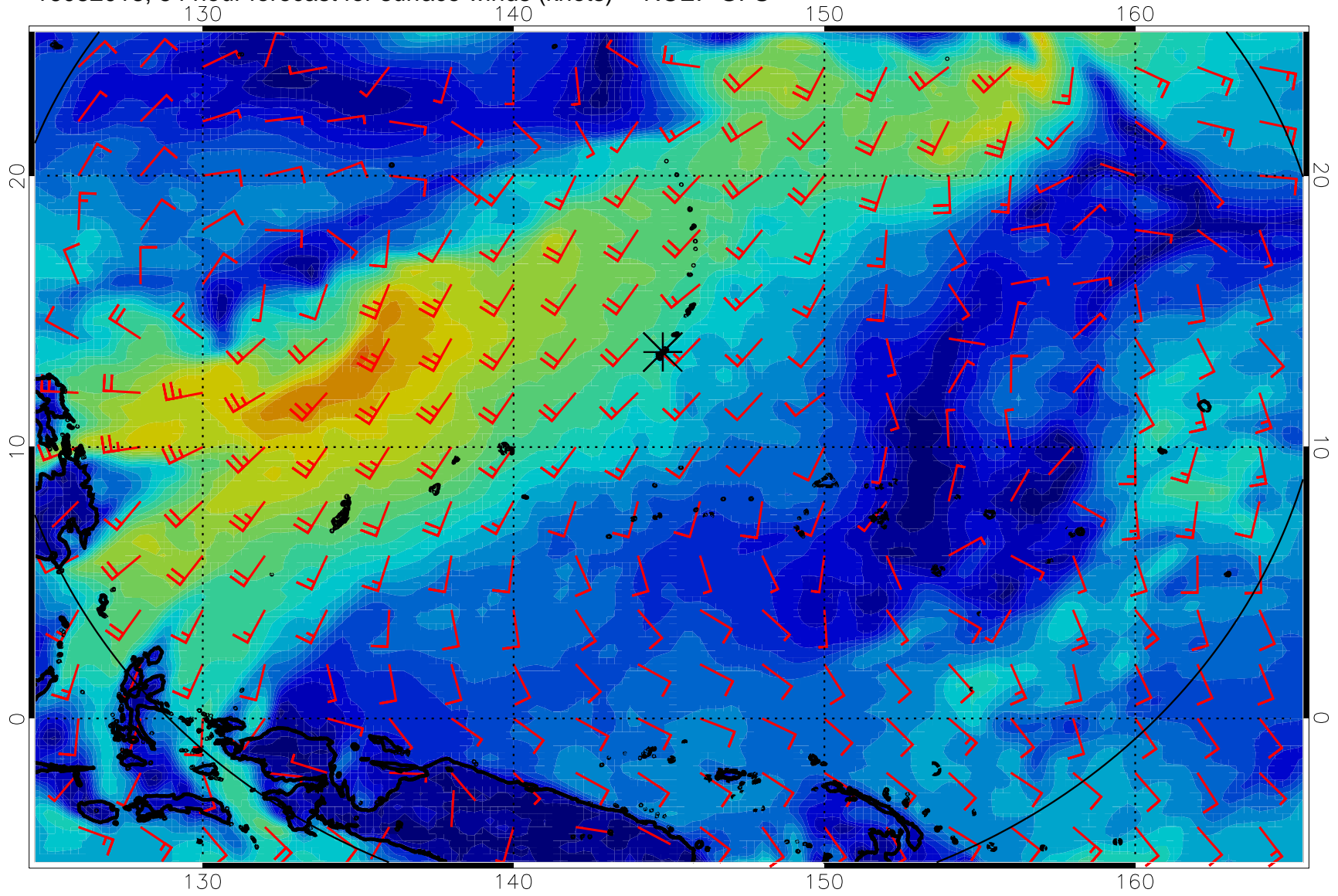
16082018, 54 hour forecast for surface winds (knots) -- NCEP GFS
