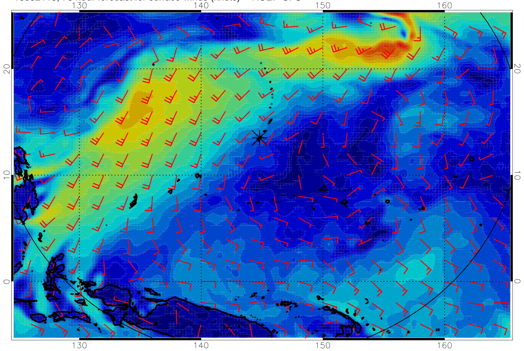
16082118, 78 hour forecast for surface winds (knots) -- NCEP GFS
