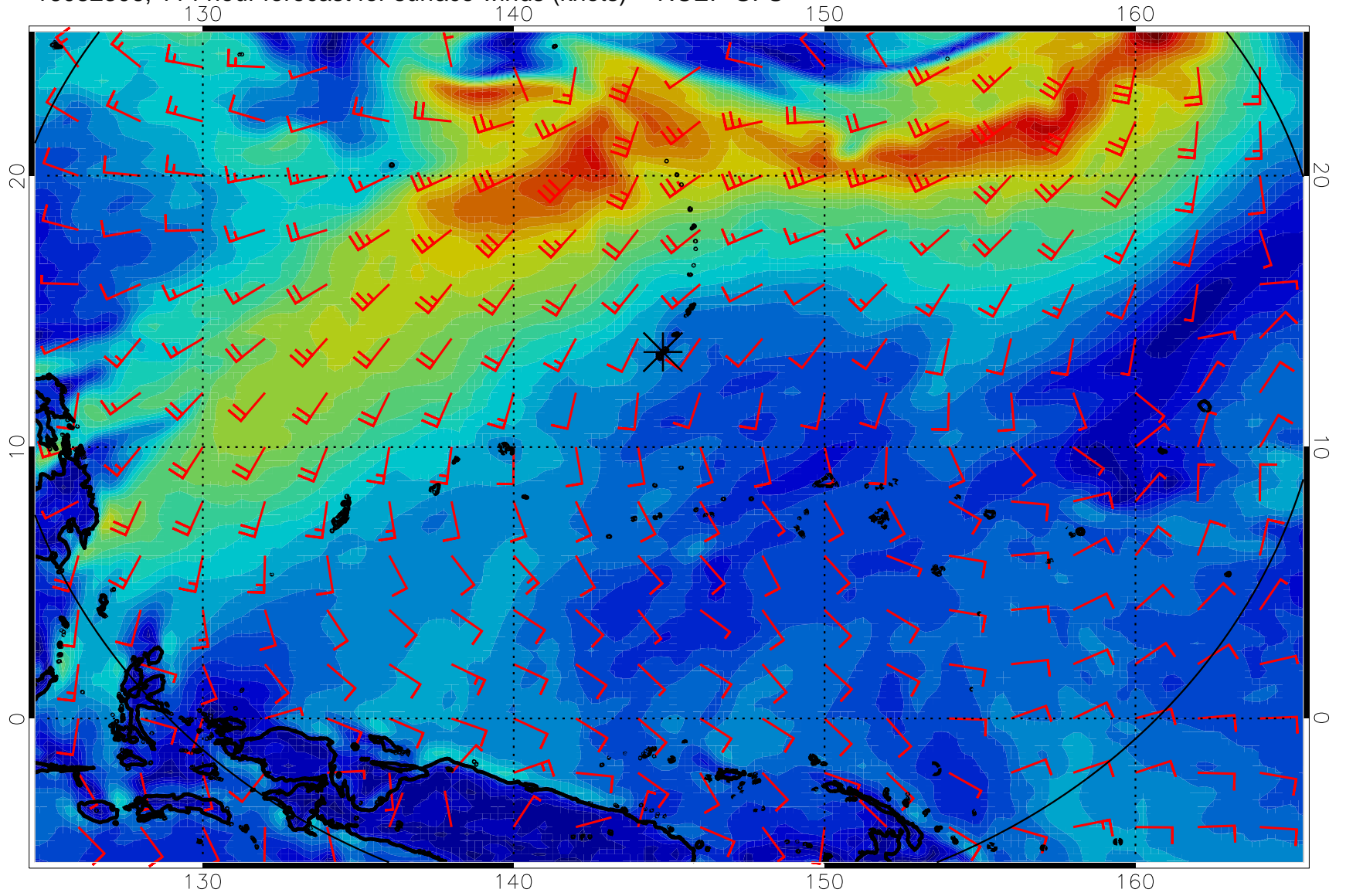
16082306, 114 hour forecast for surface winds (knots) -- NCEP GFS
