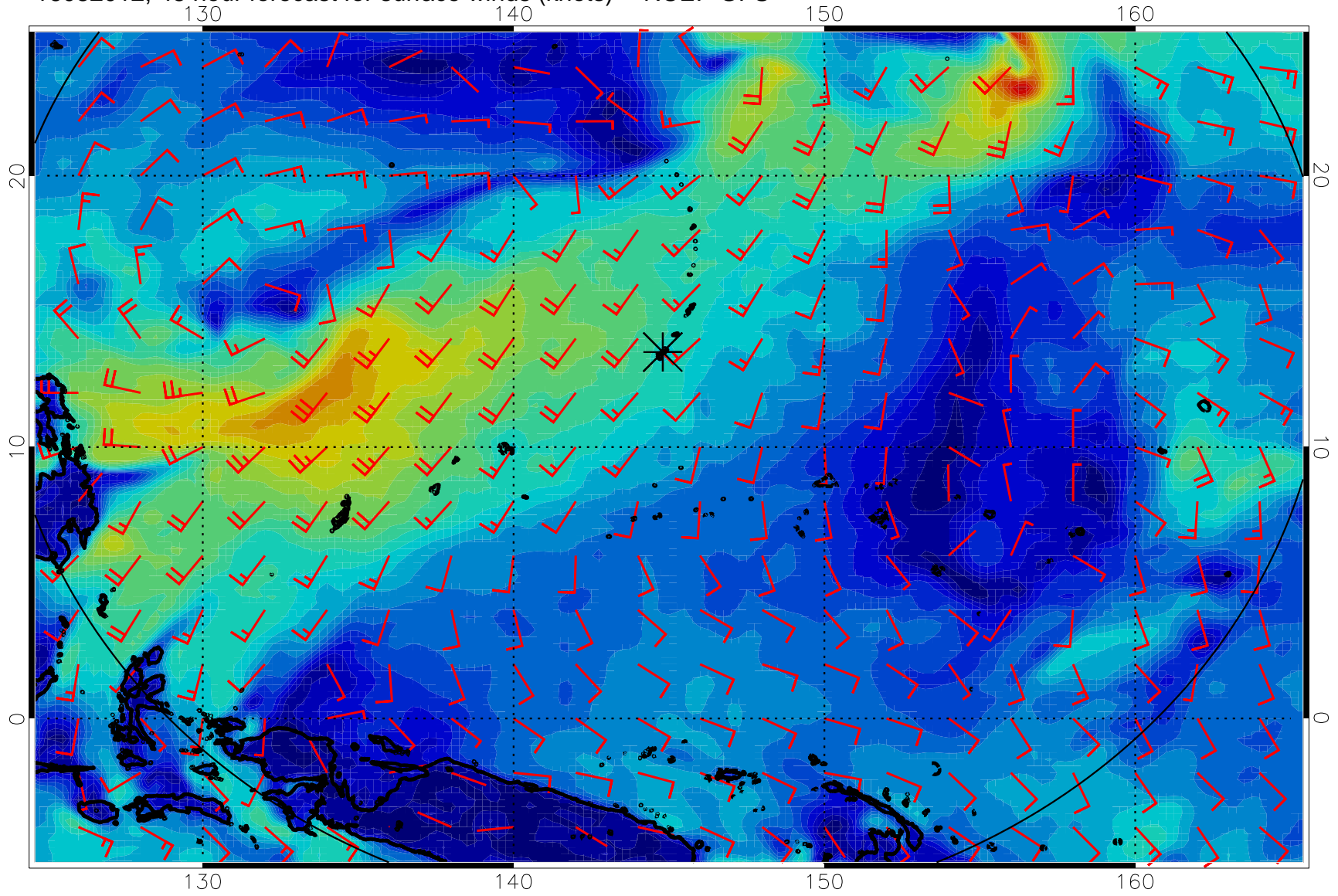
16082012, 48 hour forecast for surface winds (knots) -- NCEP GFS
