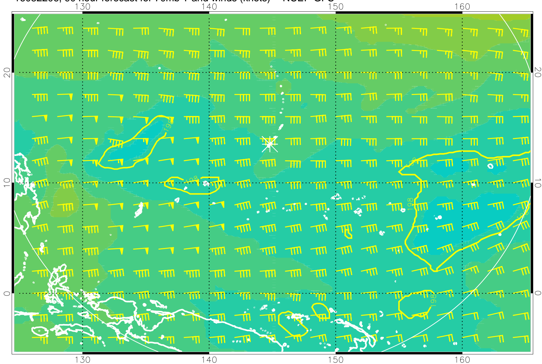
16082206, 90 hour forecast for 70mb T and winds (knots) -- NCEP GFS
