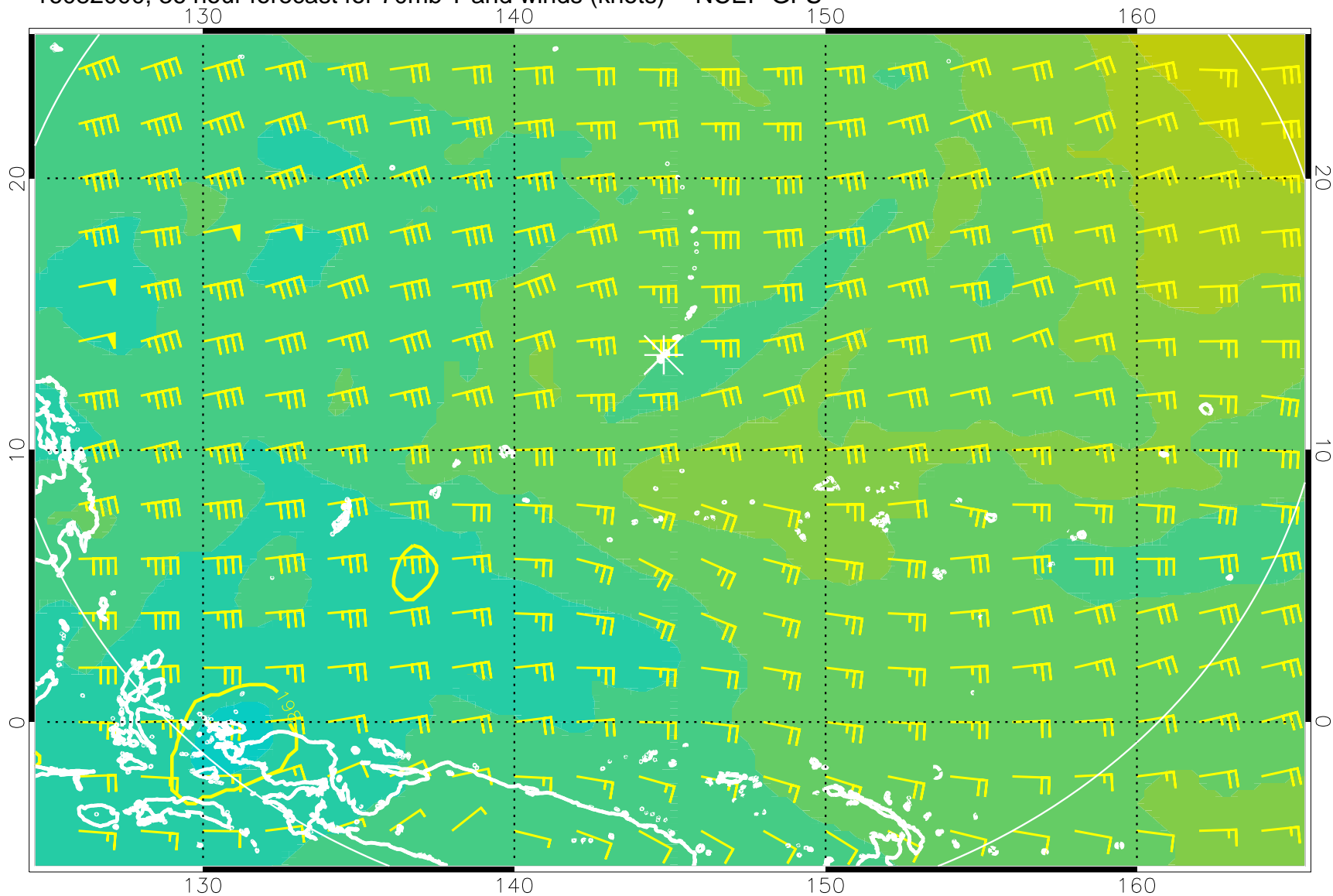
16082000, 36 hour forecast for 70mb T and winds (knots) -- NCEP GFS
