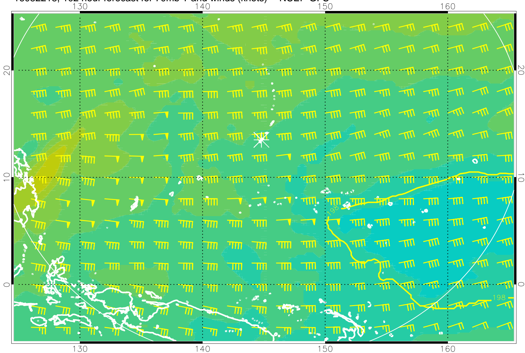
16082218, 102 hour forecast for 70mb T and winds (knots) -- NCEP GFS
