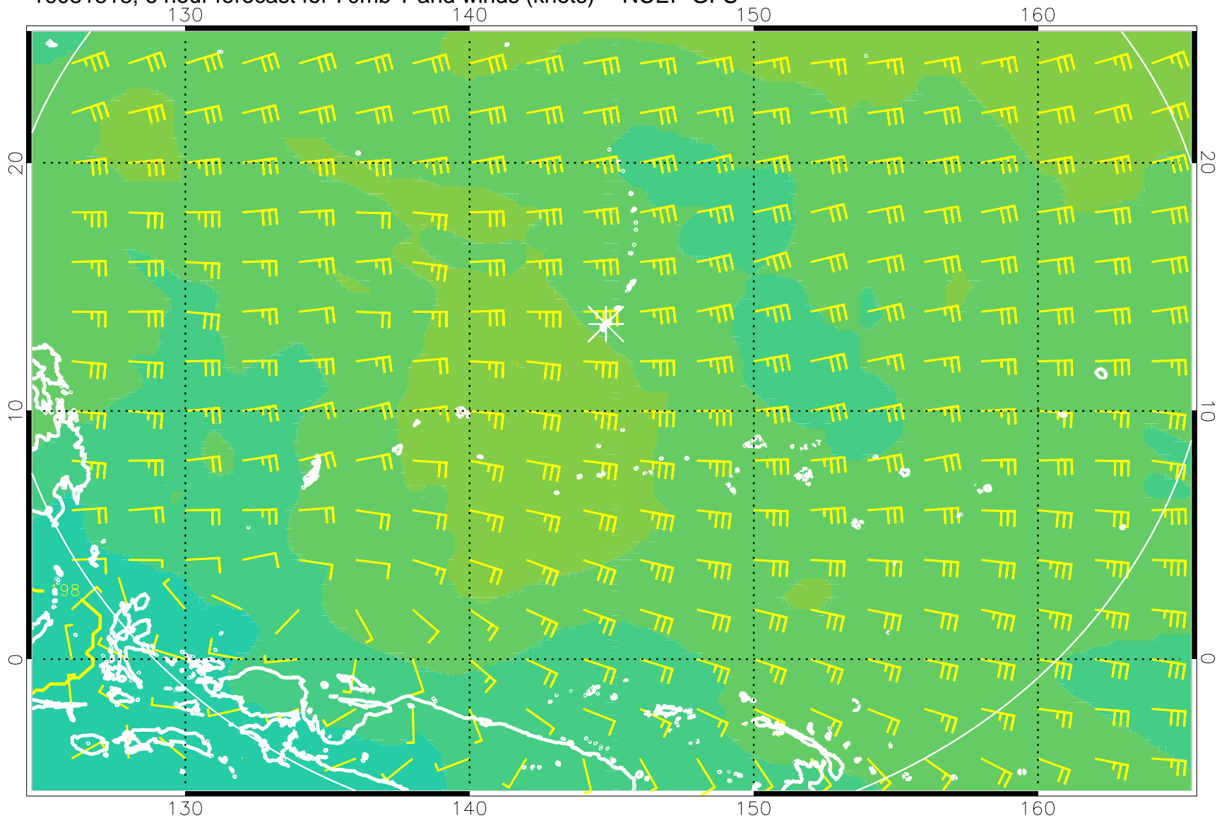
16081818, 6 hour forecast for 70mb T and winds (knots) -- NCEP GFS
