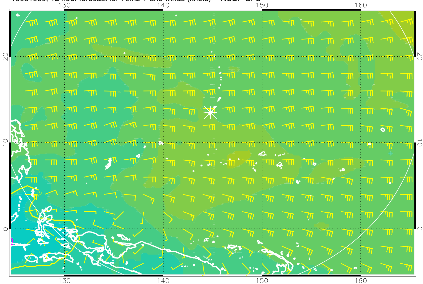
16081900, 12 hour forecast for 70mb T and winds (knots) -- NCEP GFS
