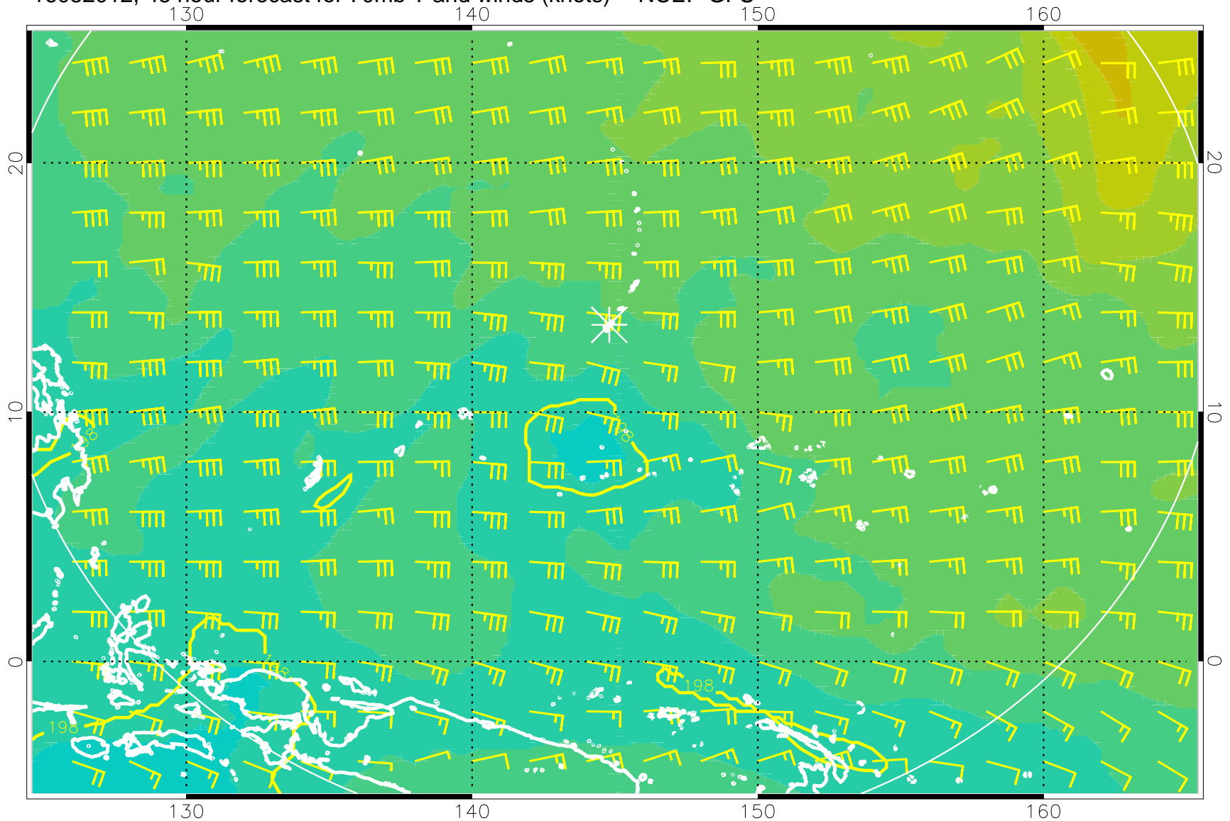
16082012, 48 hour forecast for 70mb T and winds (knots) -- NCEP GFS
