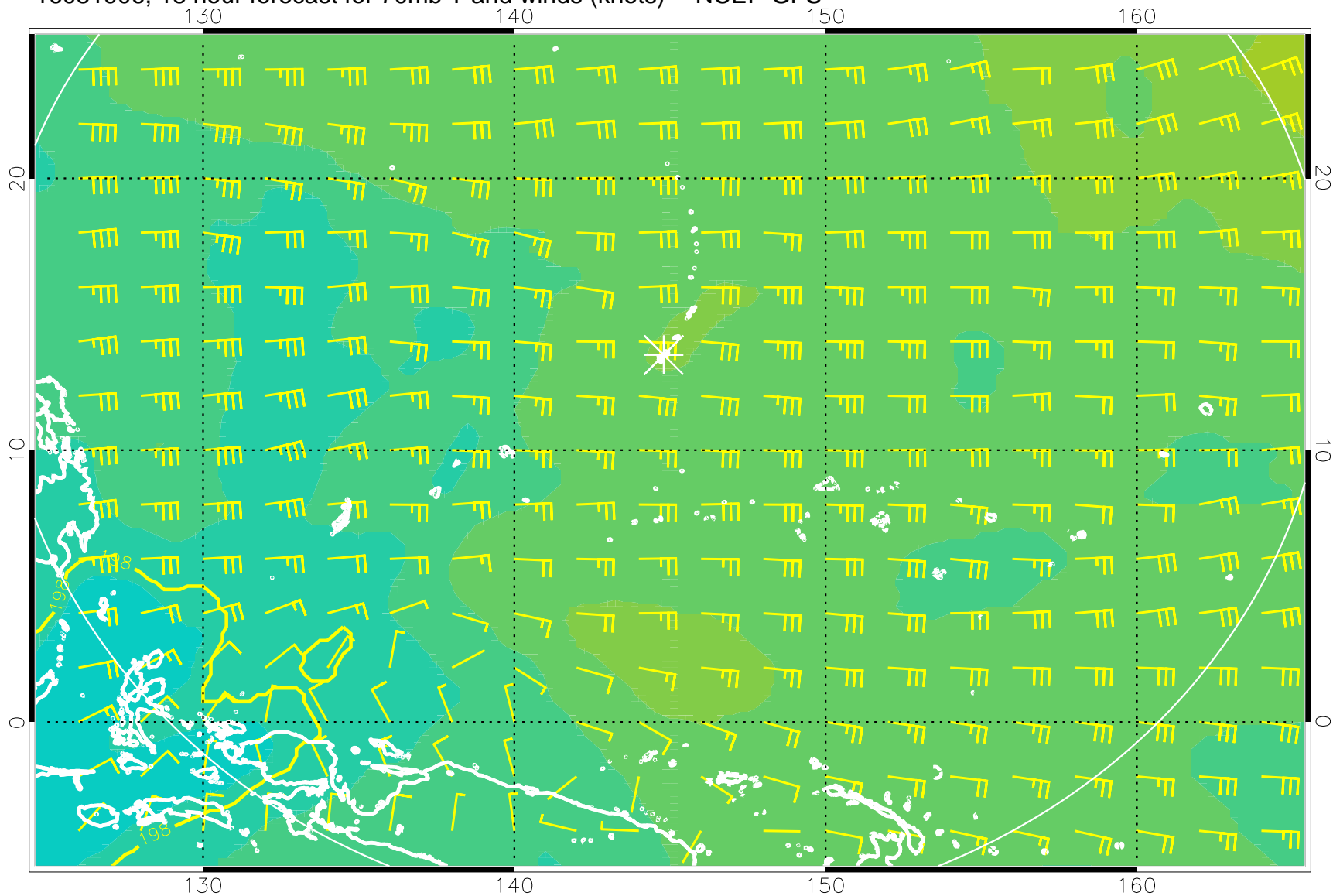
16081906, 18 hour forecast for 70mb T and winds (knots) -- NCEP GFS
