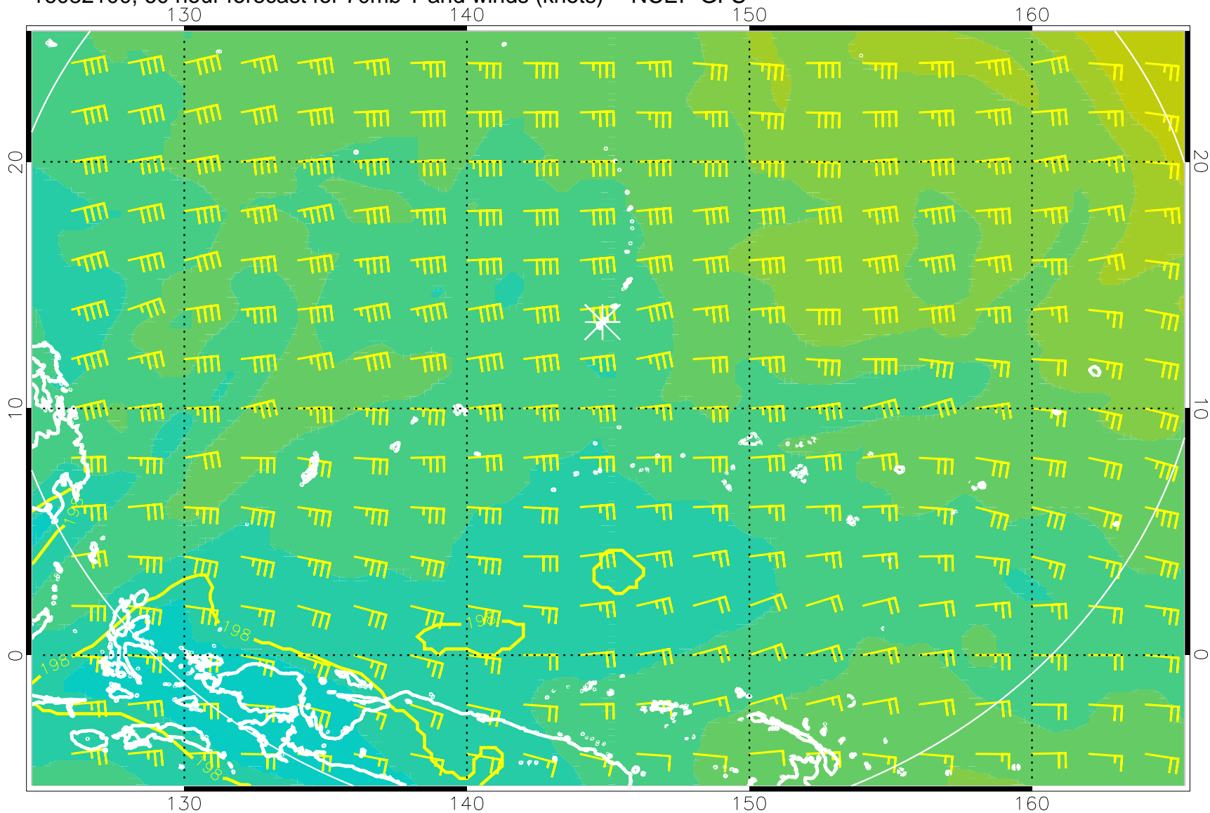
16082100, 60 hour forecast for 70mb T and winds (knots) -- NCEP GFS
