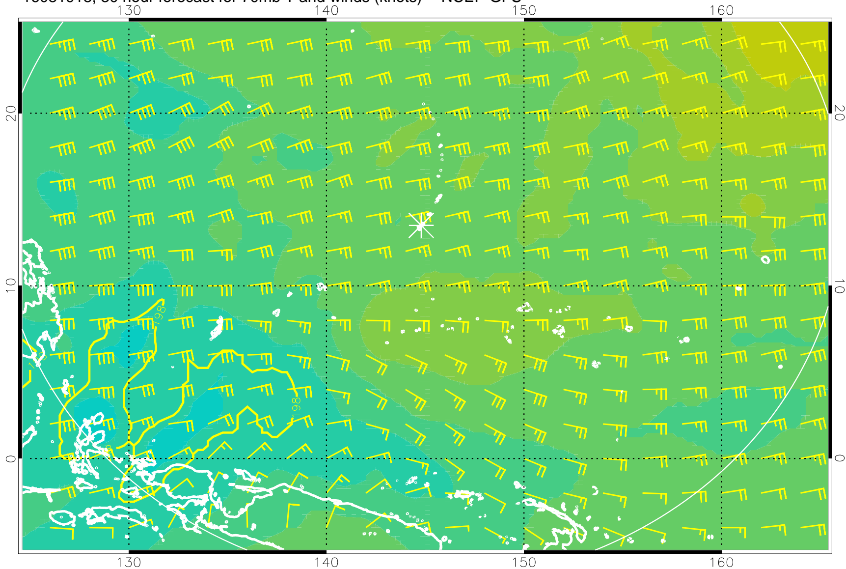
16081918, 30 hour forecast for 70mb T and winds (knots) -- NCEP GFS
