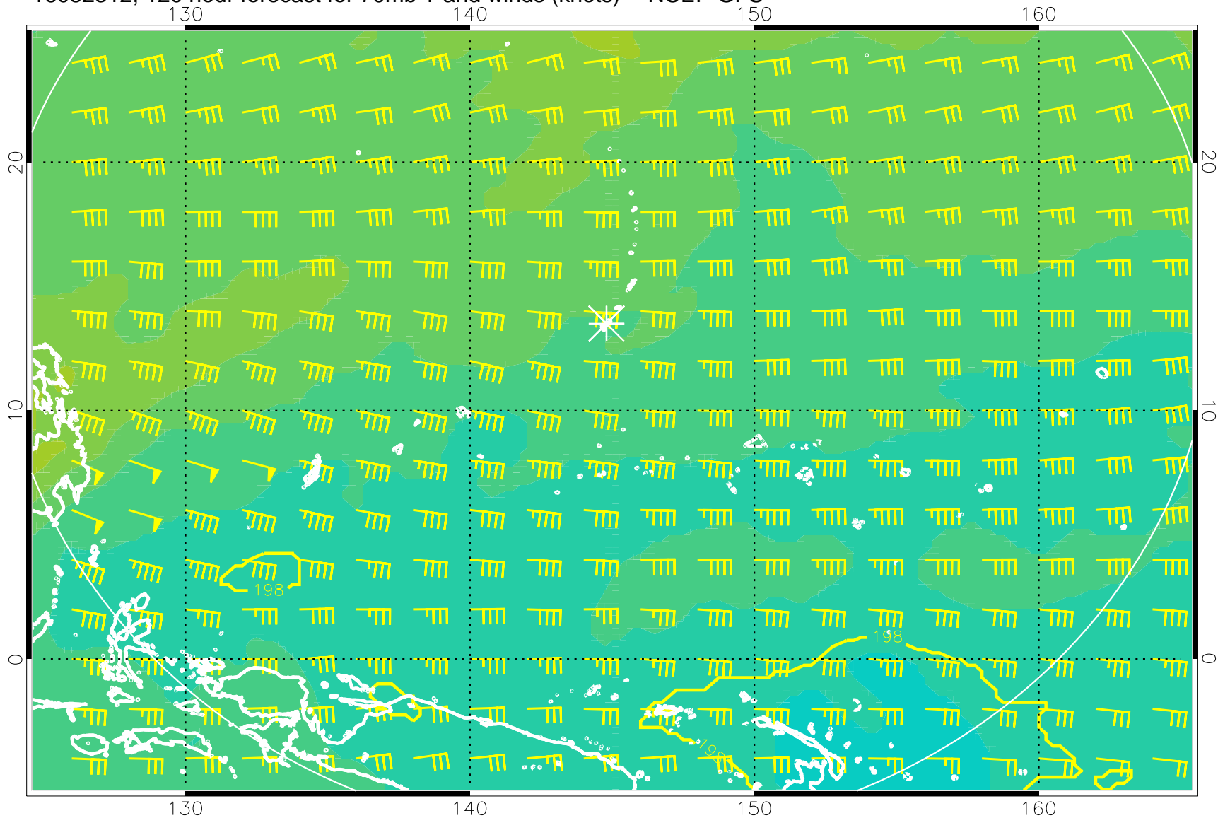
16082312, 120 hour forecast for 70mb T and winds (knots) -- NCEP GFS
