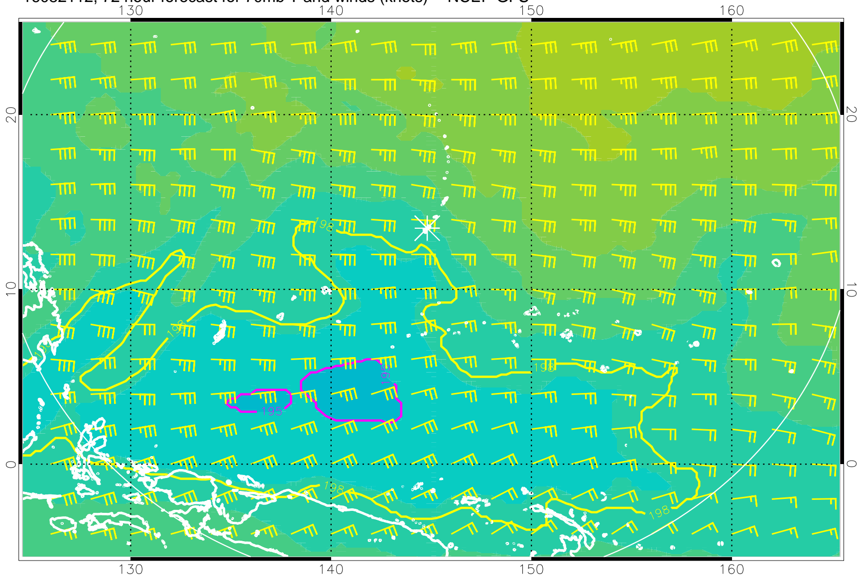
16082112, 72 hour forecast for 70mb T and winds (knots) -- NCEP GFS
