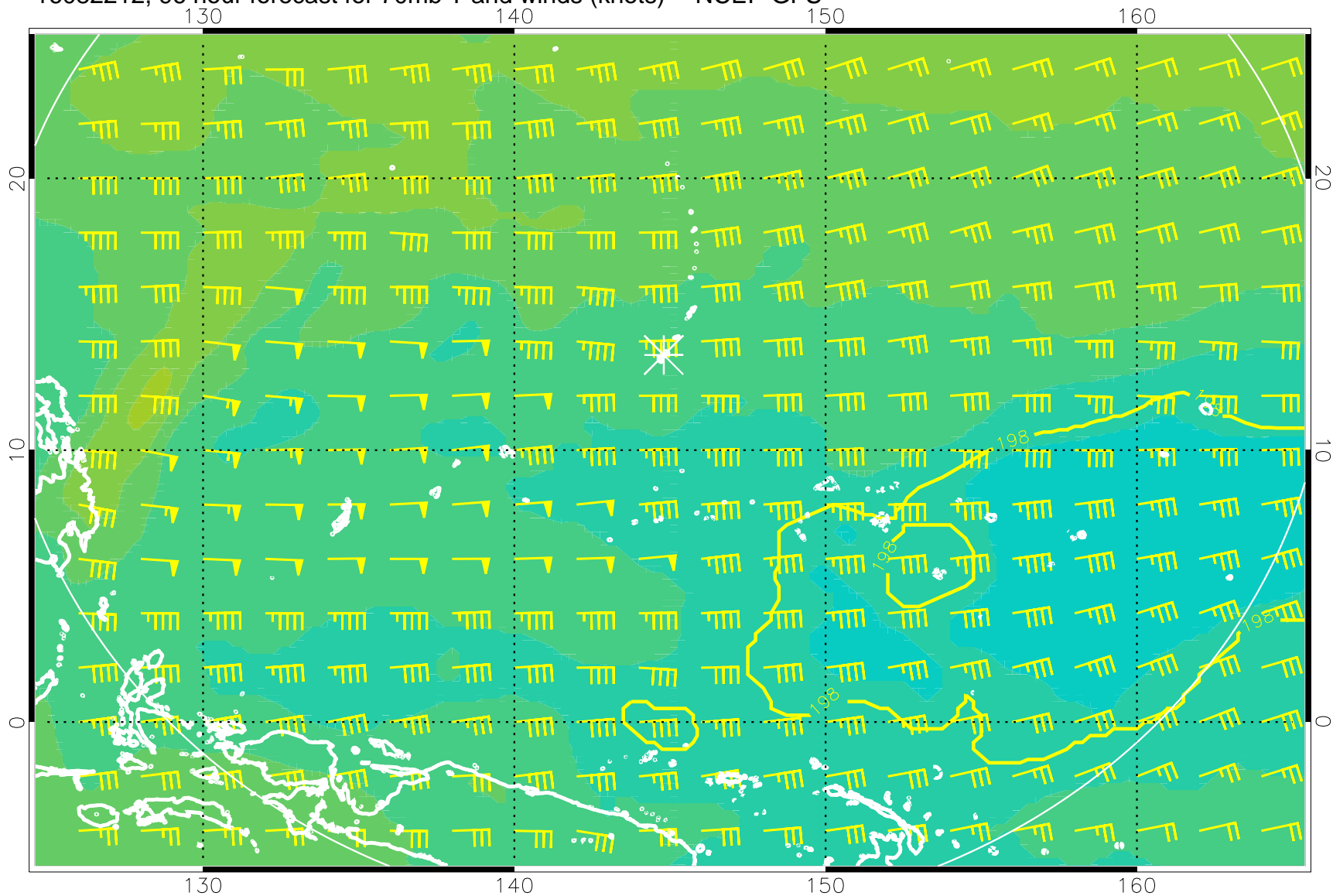
16082212, 96 hour forecast for 70mb T and winds (knots) -- NCEP GFS
