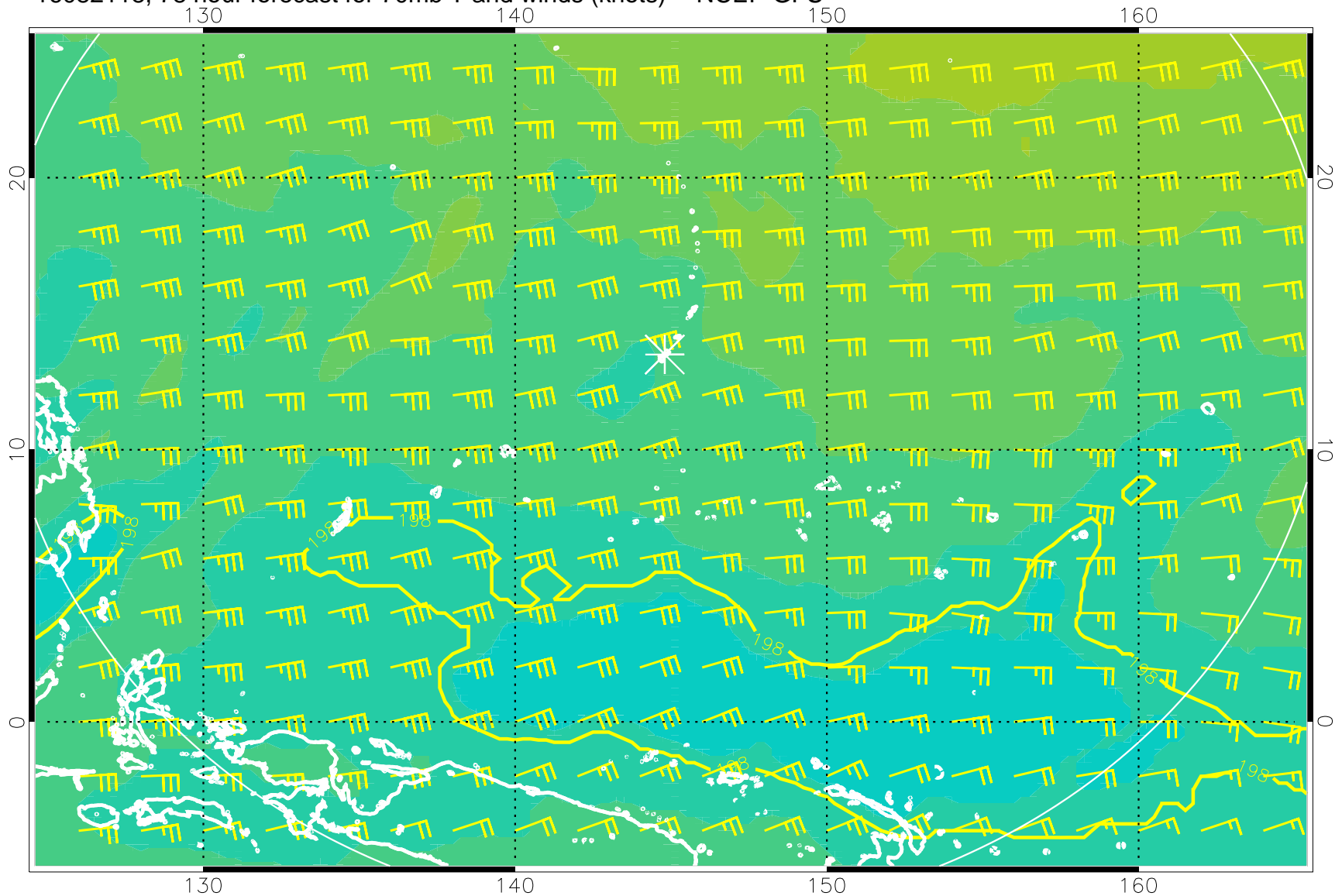
16082118, 78 hour forecast for 70mb T and winds (knots) -- NCEP GFS
