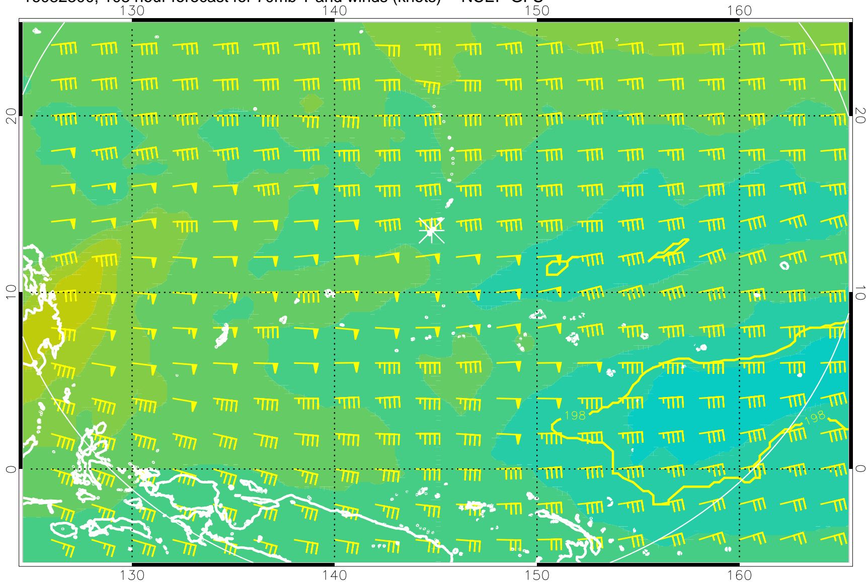
16082300, 108 hour forecast for 70mb T and winds (knots) -- NCEP GFS
