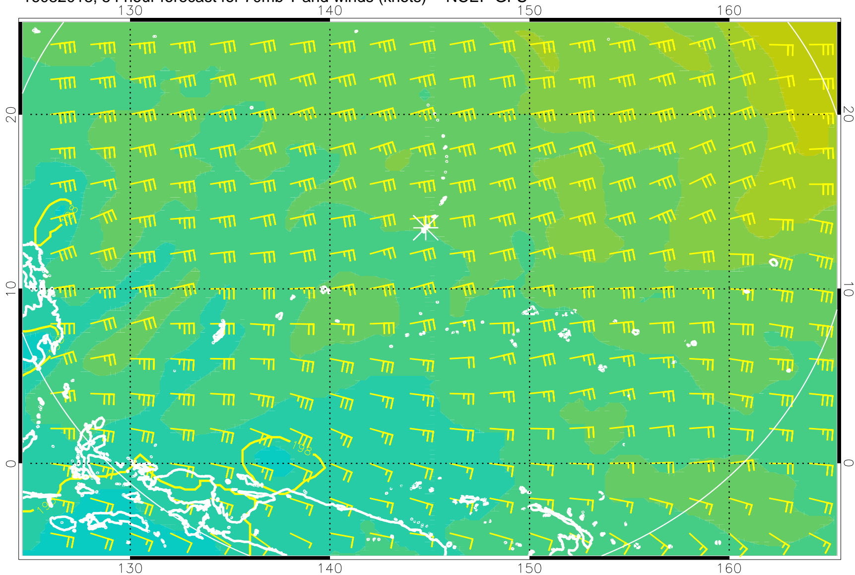
16082018, 54 hour forecast for 70mb T and winds (knots) -- NCEP GFS
