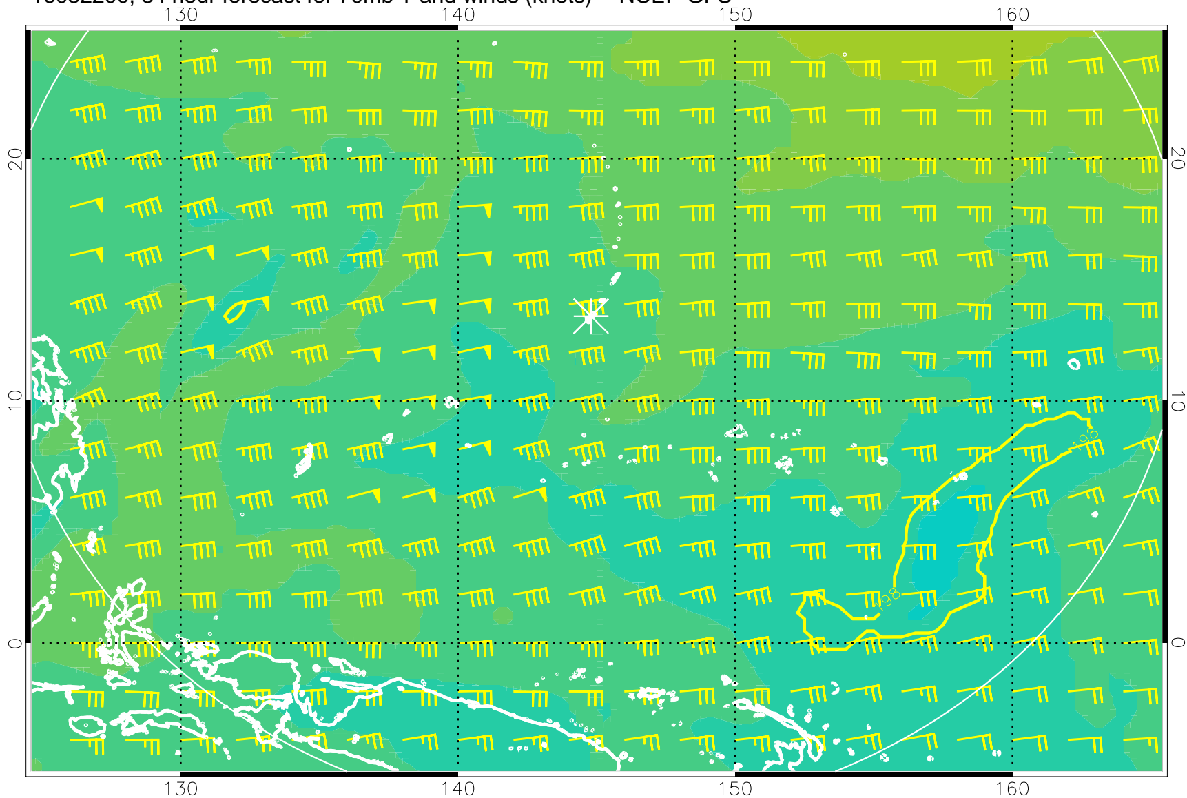
16082200, 84 hour forecast for 70mb T and winds (knots) -- NCEP GFS
