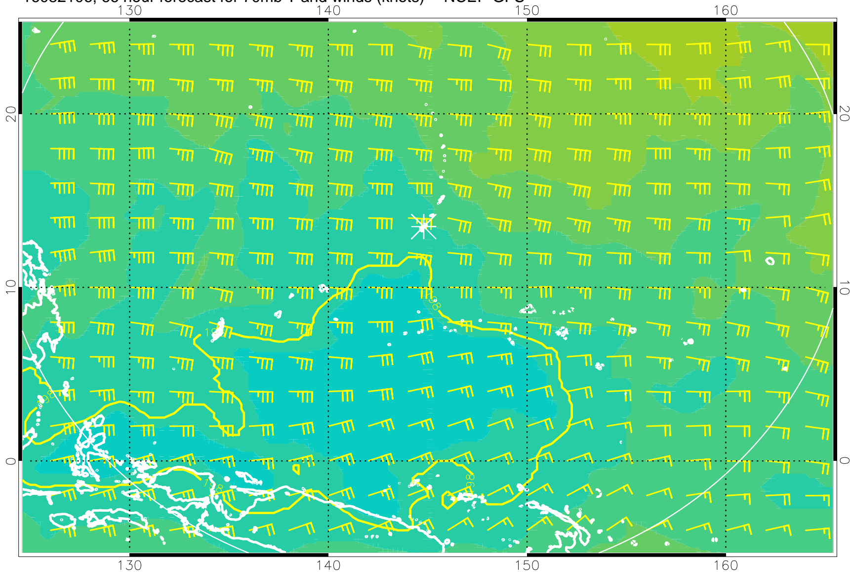
16082106, 66 hour forecast for 70mb T and winds (knots) -- NCEP GFS
