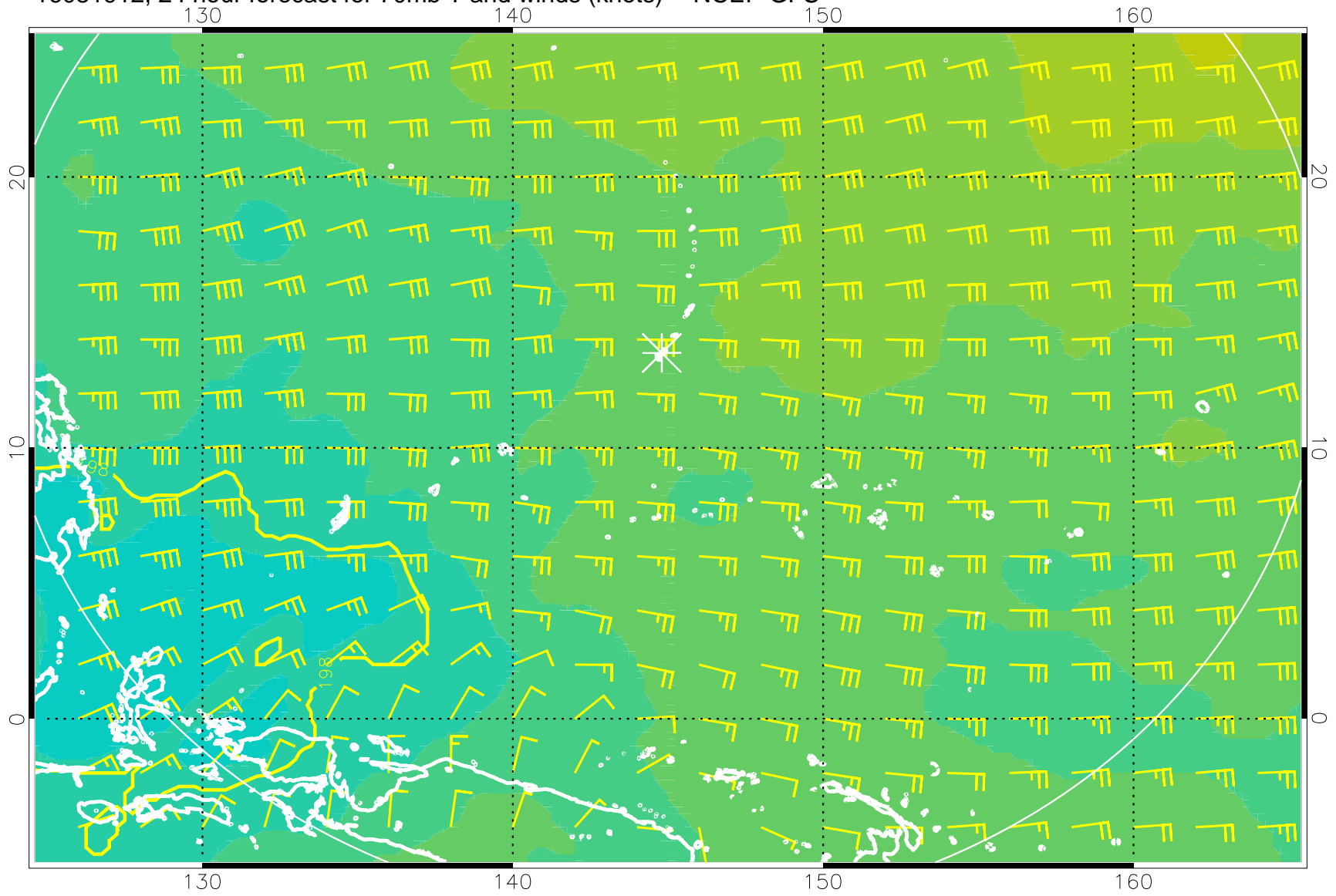
16081912, 24 hour forecast for 70mb T and winds (knots) -- NCEP GFS
