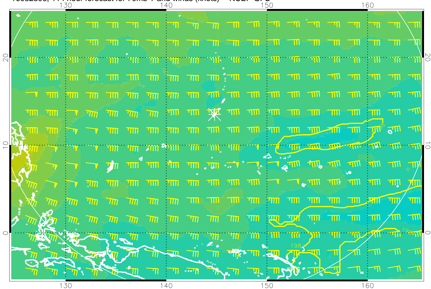
16082306, 114 hour forecast for 70mb T and winds (knots) -- NCEP GFS
